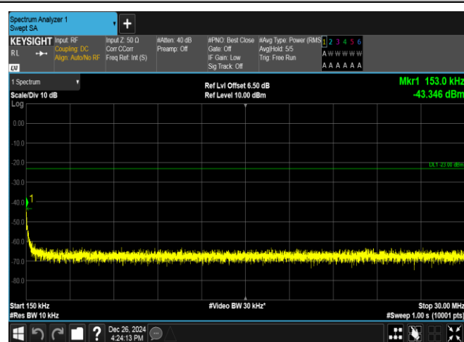
EGPRS850-251-8-0.15~30MHz-PASS
