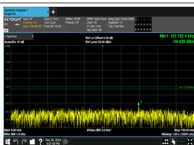
GPRS850-190-5-0.009~0.15MHz-PASS
