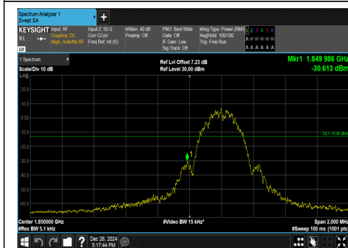
EGPRS1900-512-2-PASS
