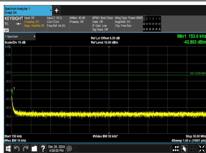
GPRS850-190-5-0.15~30MHz-PASS
