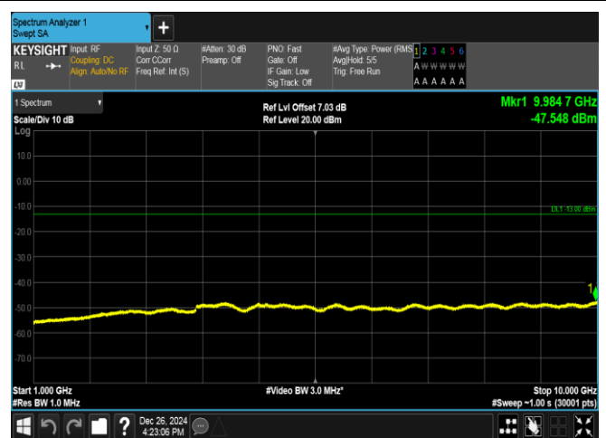
EGPRS850-128-8-1000~10000MHz-PASS
