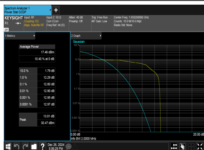
EGPRS1900-512-2-PASS
