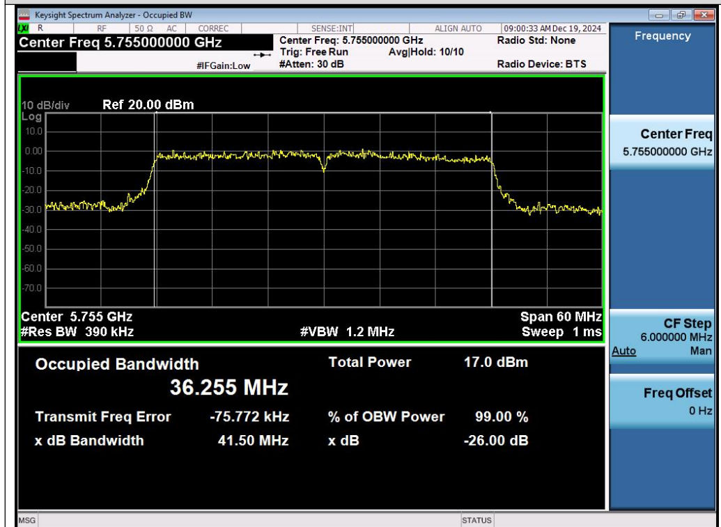
Test_Graph_802.11n40_ANT1_5755_MCS0_OBW
