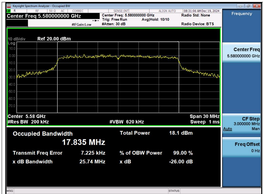
Test_Graph_802.11n20_ANT1_5580_MCS0_OBW
