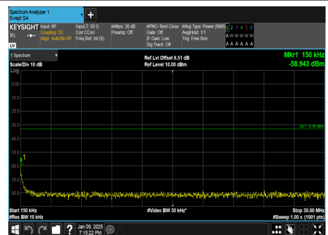
Band66-1.4MHz-QPSK-131979-6RB#0-0.15~30-PASS
