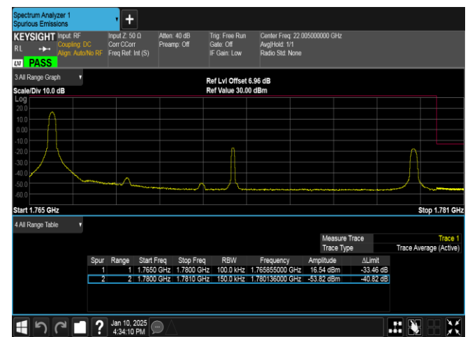
Band66-15MHz-16QAM-132597-1RB#0-PASS
