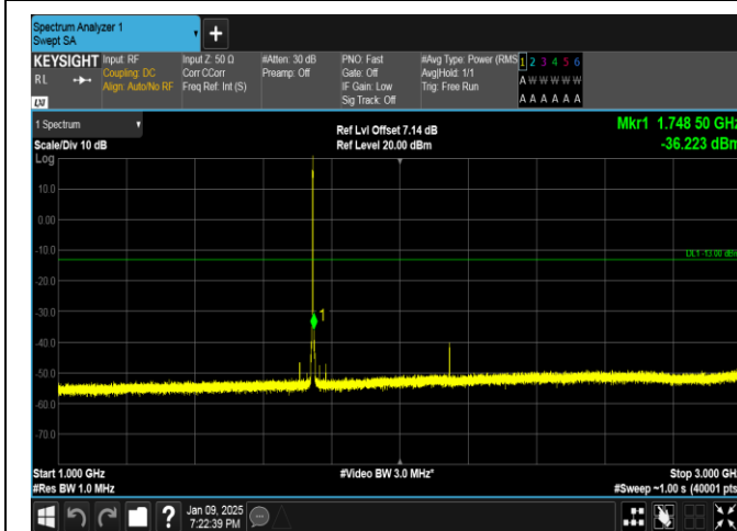
Band66-1.4MHz-QPSK-132322-6RB#0-1000~3000-PASS
