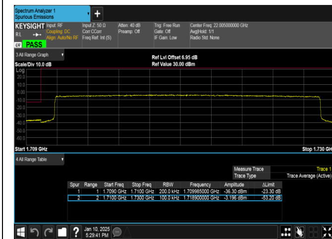
Band66-20MHz-QPSK-132072-100RB#0-PASS
