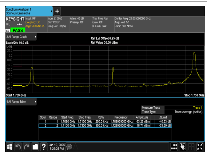
Band66-20MHz-16QAM-132072-1RB#99-PASS
