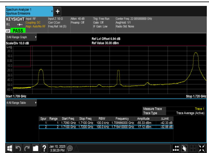
Band66-10MHz-16QAM-132022-1RB#49-PASS
