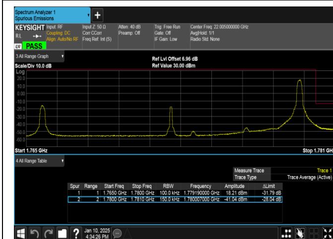
Band66-15MHz-QPSK-132597-1RB#74-PASS
