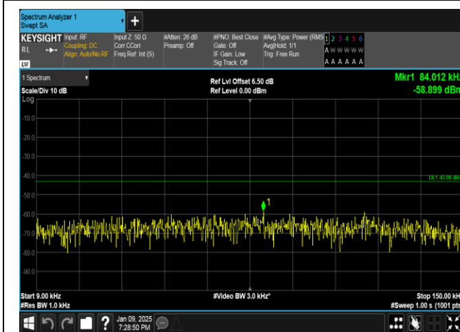
Band66-1.4MHz-QPSK-132665-6RB#0-0.009~0.15-PASS
