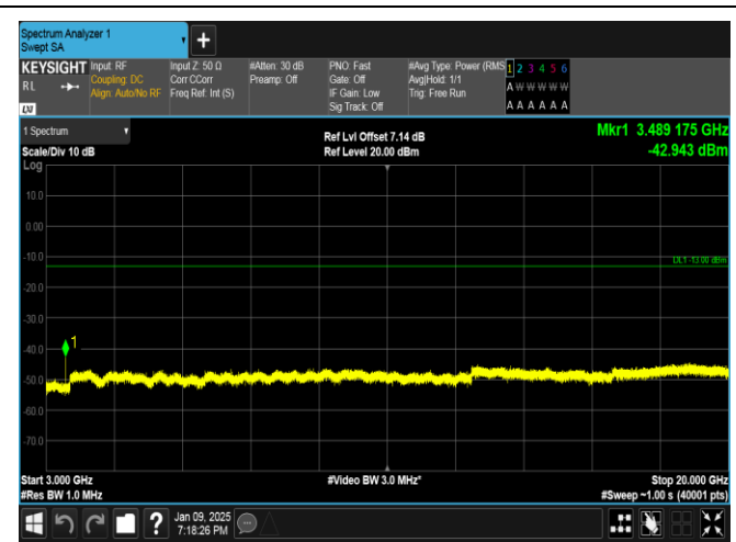
Band66-1.4MHz-QPSK-132322-1RB#0-3000~20000-PASS
