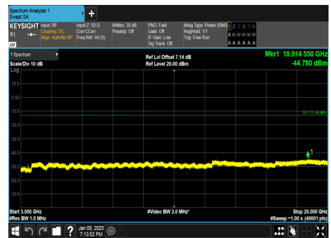
Band66-1.4MHz-QPSK-131979-1RB#5-3000~20000-PASS
