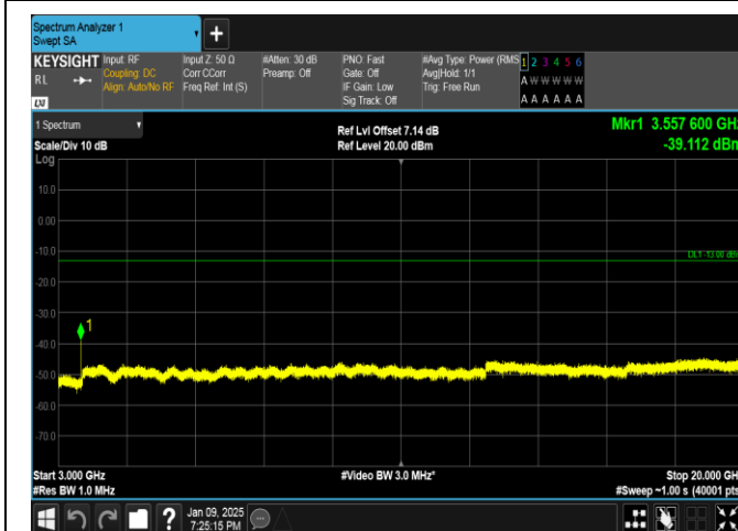
Band66-1.4MHz-QPSK-132665-1RB#0-3000~20000-PASS
