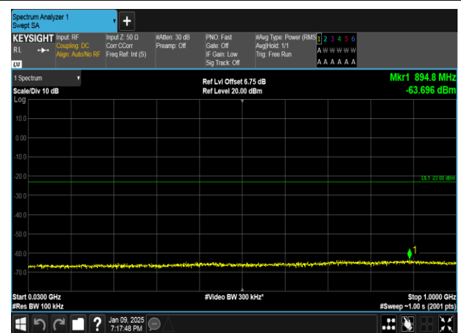
Band66-1.4MHz-QPSK-132322-1RB#0-30~1000-PASS
