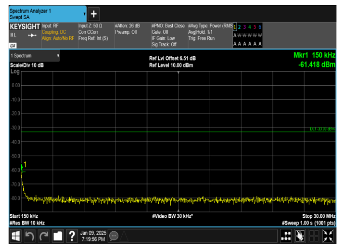
Band66-1.4MHz-QPSK-132322-1RB#5-0.15~30-PASS
