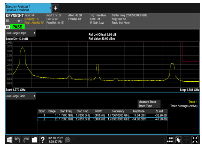
Band66-10MHz-16QAM-132622-1RB#0-PASS
