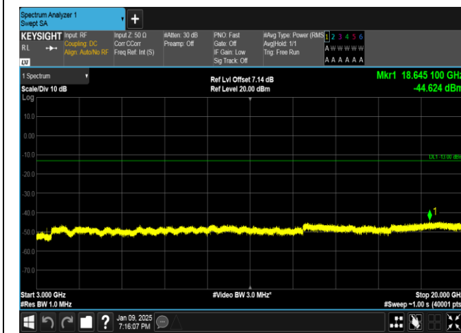
Band66-1.4MHz-QPSK-131979-6RB#0-3000~20000-PASS
