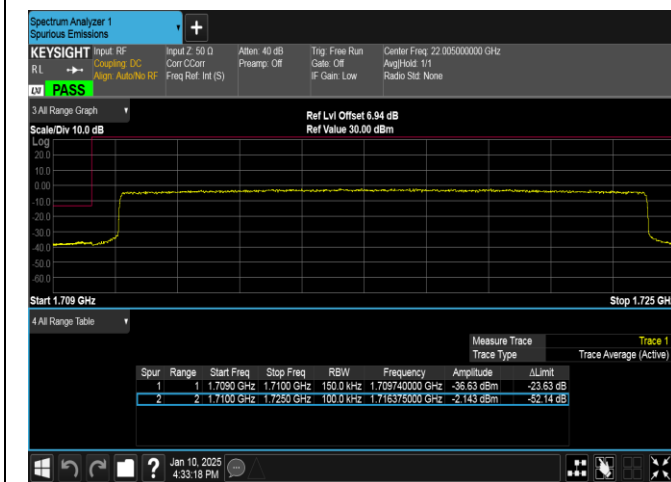
Band66-15MHz-QPSK-132047-75RB#0-PASS
