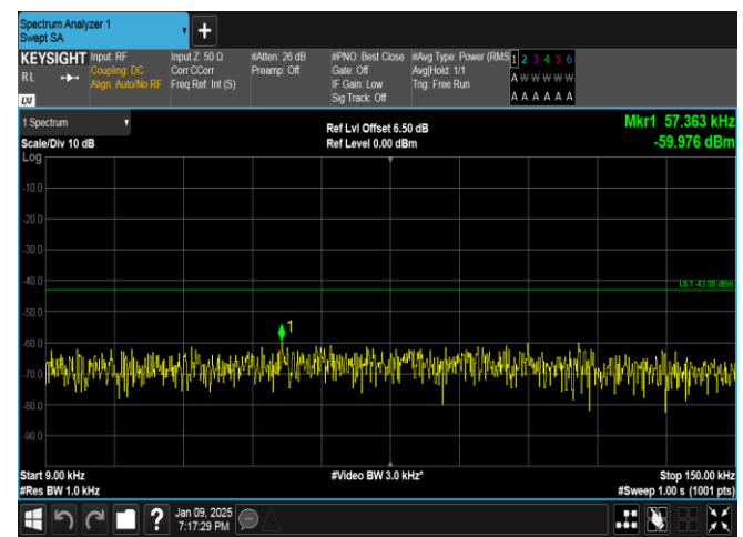
Band66-1.4MHz-QPSK-132322-1RB#0-0.009~0.15-PASS
