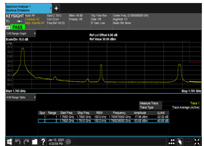
Band66-15MHz-QPSK-132597-1RB#0-PASS
