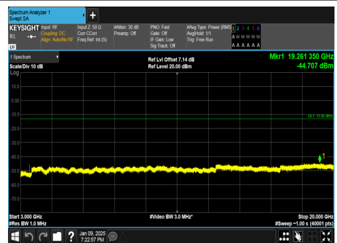
Band66-1.4MHz-QPSK-132322-6RB#0-3000~20000-PASS
