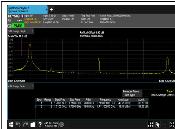
Band66-20MHz-16QAM-132072-1RB#0-PASS
