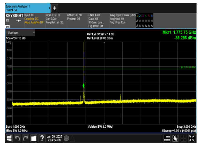
Band66-1.4MHz-QPSK-132665-1RB#0-1000~3000-PASS
