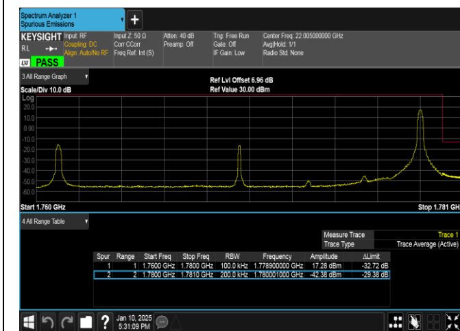
Band66-20MHz-16QAM-132572-1RB#99-PASS
