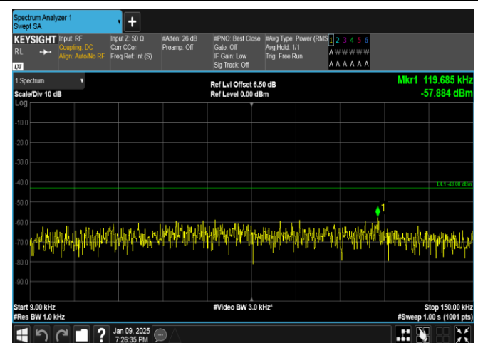
Band66-1.4MHz-QPSK-132665-1RB#5-0.009~0.15-PASS
