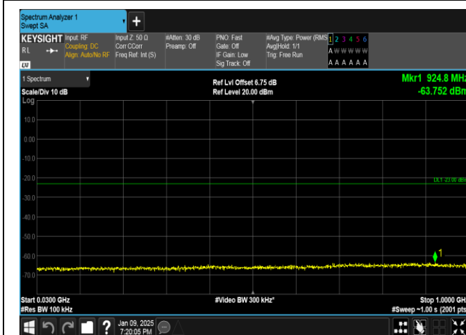
Band66-1.4MHz-QPSK-132322-1RB#5-30~1000-PASS
