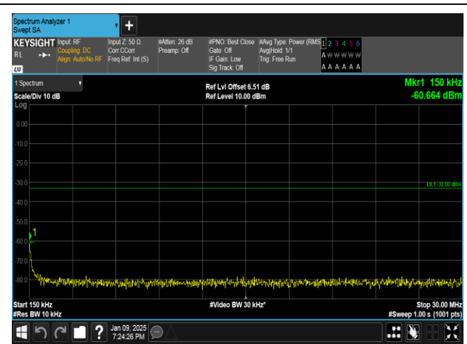
Band66-1.4MHz-QPSK-132665-1RB#0-0.15~30-PASS
