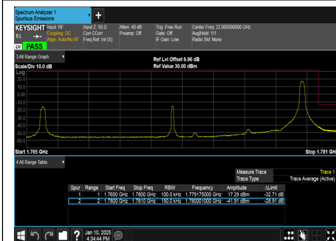
Band66-15MHz-16QAM-132597-1RB#74-PASS
