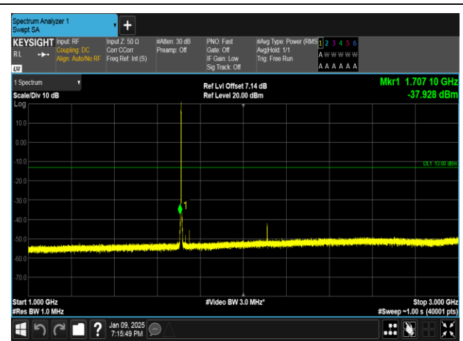
Band66-1.4MHz-QPSK-131979-6RB#0-1000~3000-PASS
