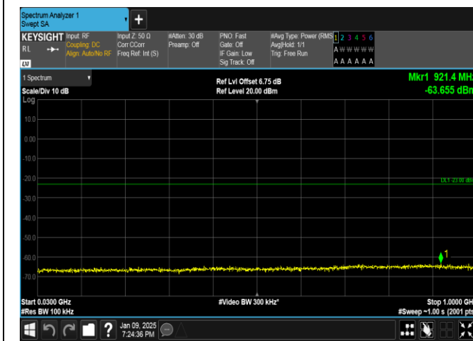
Band66-1.4MHz-QPSK-132665-1RB#0-30~1000-PASS
