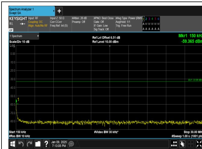
Band66-1.4MHz-QPSK-131979-1RB#5-0.15~30-PASS
