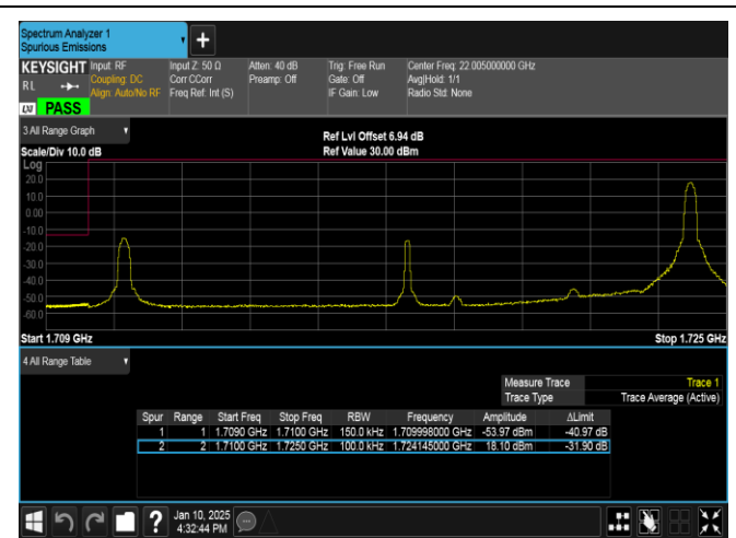
Band66-15MHz-QPSK-132047-1RB#74-PASS
