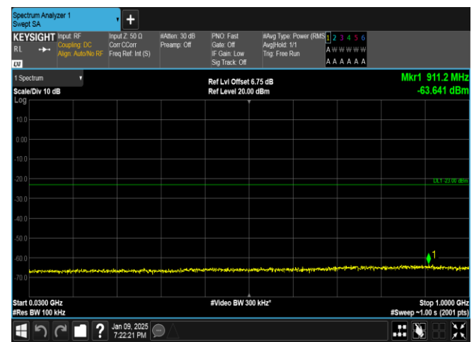
Band66-1.4MHz-QPSK-132322-6RB#0-30~1000-PASS
