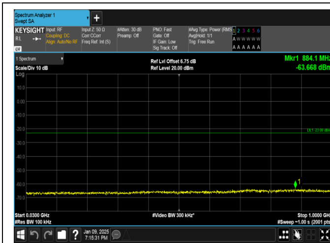
Band66-1.4MHz-QPSK-131979-6RB#0-30~1000-PASS
