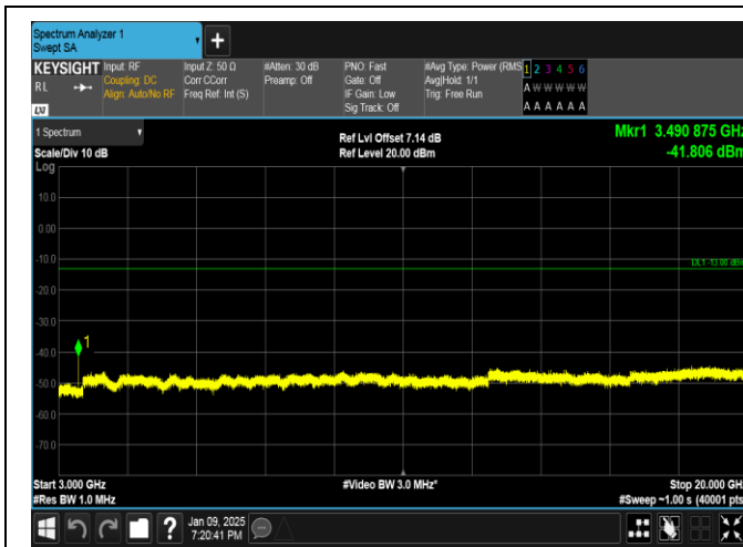
Band66-1.4MHz-QPSK-132322-1RB#5-3000~20000-PASS
