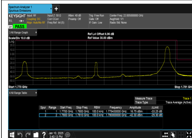
Band66-10MHz-16QAM-132622-1RB#49-PASS
