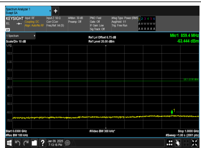
Band66-1.4MHz-QPSK-131979-1RB#5-30~1000-PASS
