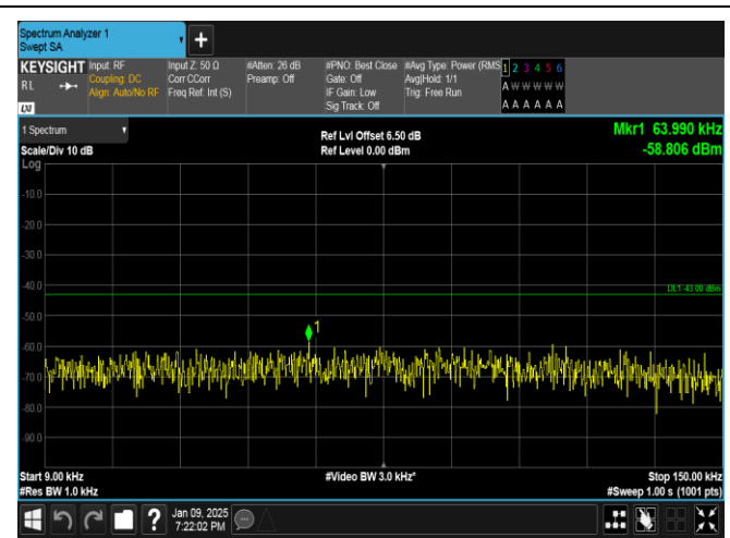
Band66-1.4MHz-QPSK-132322-6RB#0-0.009~0.15-PASS
