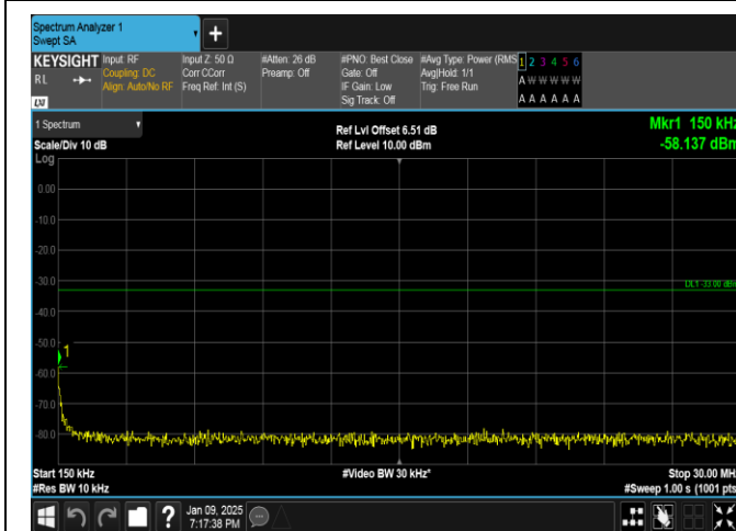
Band66-1.4MHz-QPSK-132322-1RB#0-0.15~30-PASS
