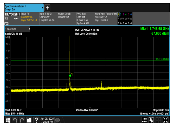
Band66-1.4MHz-QPSK-132322-1RB#5-1000~3000-PASS
