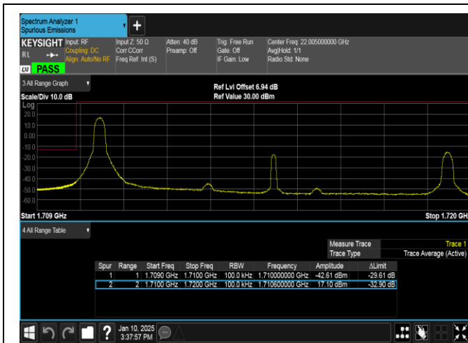
Band66-10MHz-16QAM-132022-1RB#0-PASS
