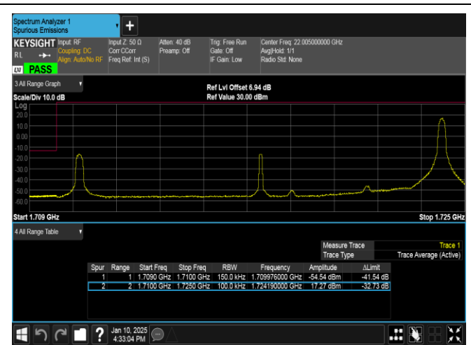
Band66-15MHz-16QAM-132047-1RB#74-PASS
