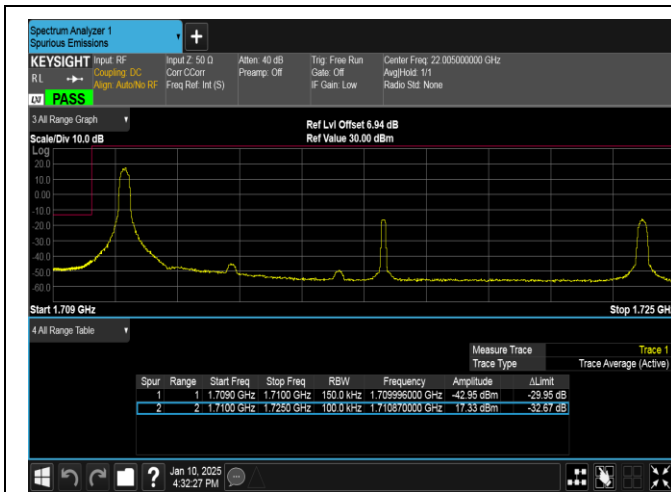
Band66-15MHz-16QAM-132047-1RB#0-PASS
