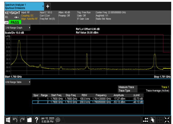
Band66-20MHz-16QAM-132572-1RB#0-PASS
