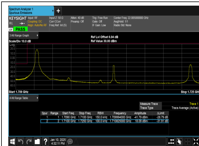
Band66-15MHz-QPSK-132047-1RB#0-PASS
