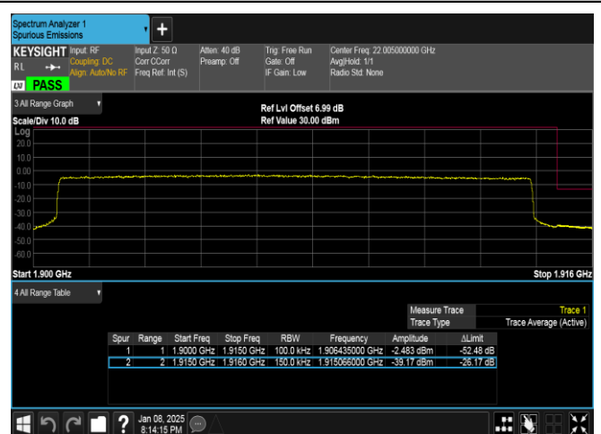
Band25-15MHz-16QAM-26615-75RB#0-PASS
