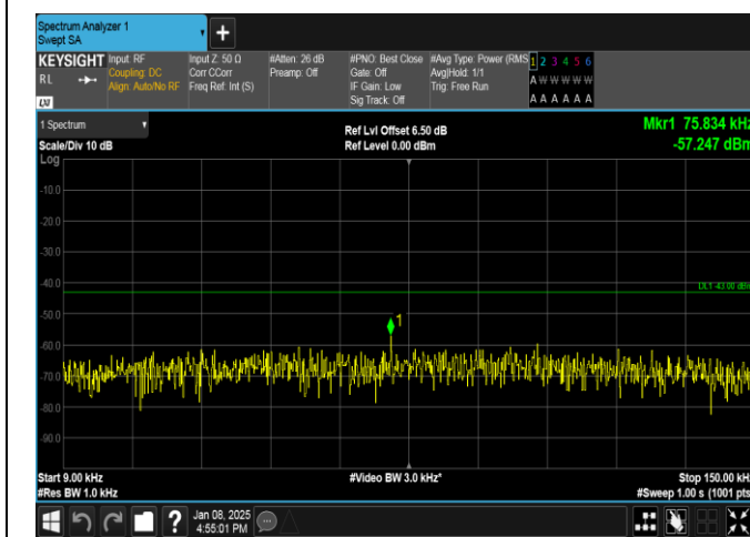
Band25-1.4MHz-QPSK-26365-1RB#5-0.009~0.15-PASS
