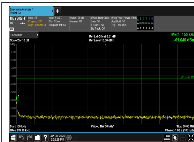
Band25-1.4MHz-QPSK-26683-1RB#5-0.15~30-PASS
