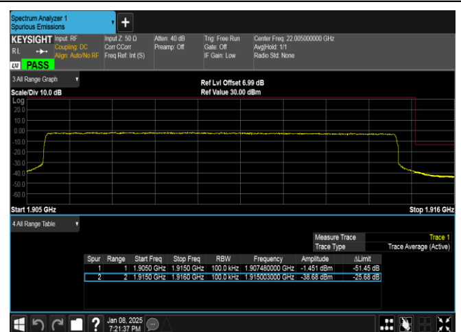
Band25-10MHz-16QAM-26640-50RB#0-PASS
