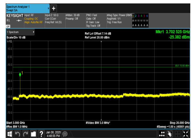
Band25-1.4MHz-QPSK-26047-1RB#5-3000~20000-PASS
