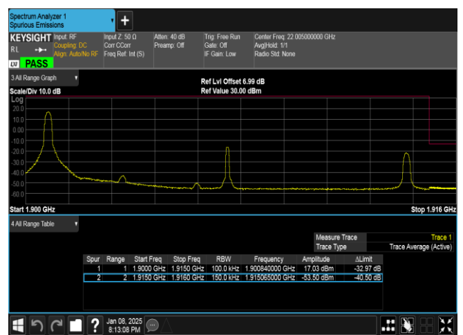
Band25-15MHz-16QAM-26615-1RB#0-PASS
