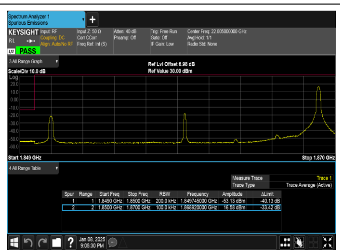
Band25-20MHz-16QAM-26140-1RB#99-PASS
