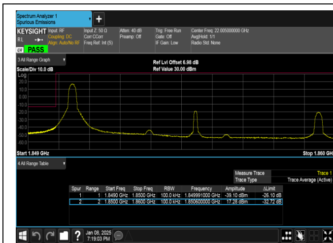
Band25-10MHz-16QAM-26090-1RB#0-PASS
