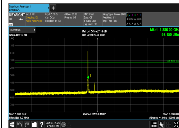
Band25-1.4MHz-QPSK-26365-6RB#0-1000~3000-PASS
