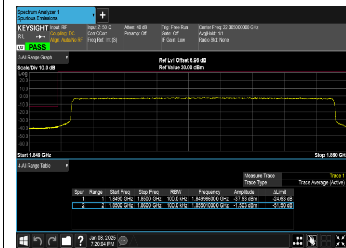
Band25-10MHz-16QAM-26090-50RB#0-PASS
