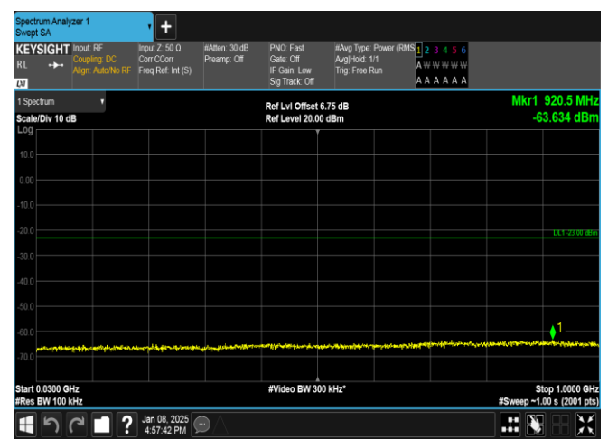
Band25-1.4MHz-QPSK-26365-6RB#0-30~1000-PASS
