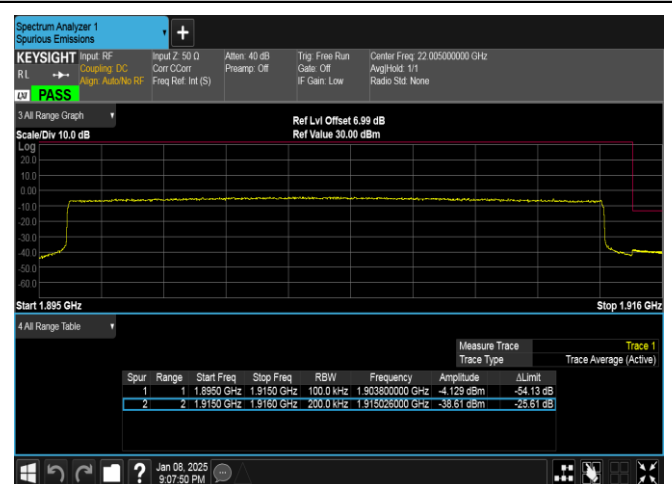
Band25-20MHz-16QAM-26590-100RB#0-PASS
