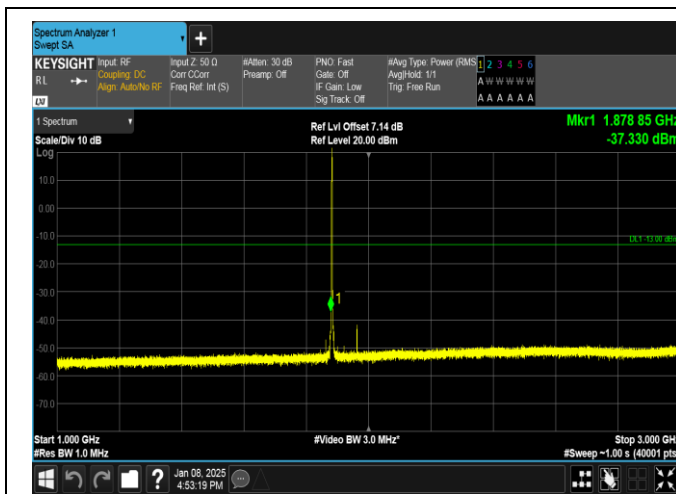
Band25-1.4MHz-QPSK-26365-1RB#0-1000~3000-PASS
