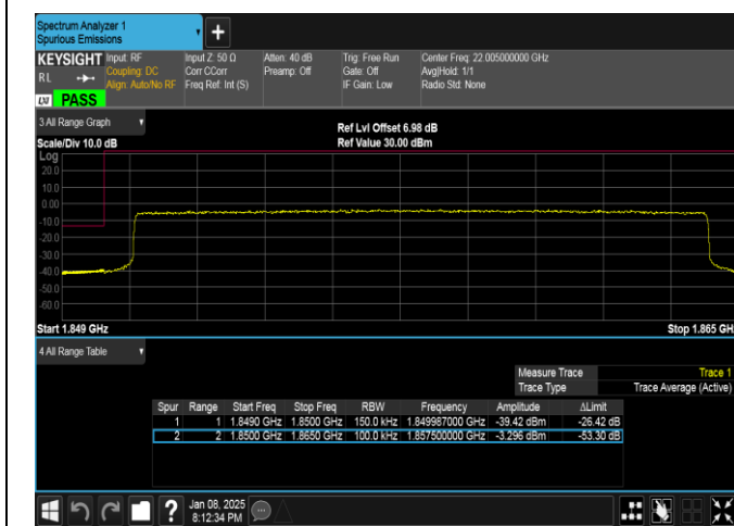
Band25-15MHz-16QAM-26115-75RB#0-PASS
