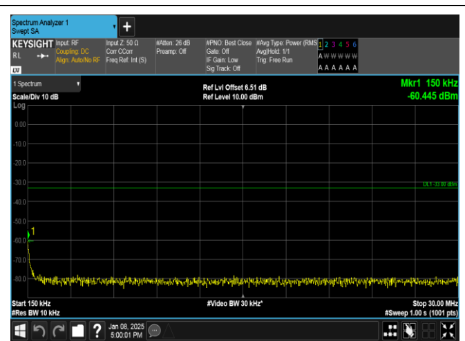
Band25-1.4MHz-QPSK-26683-1RB#0-0.15~30-PASS
