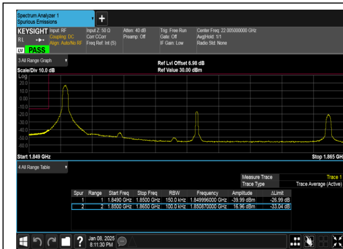
Band25-15MHz-16QAM-26115-1RB#0-PASS
