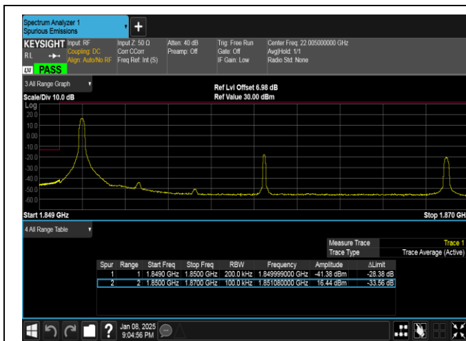
Band25-20MHz-16QAM-26140-1RB#0-PASS
