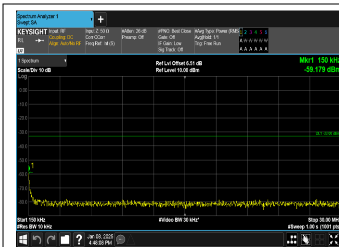
Band25-1.4MHz-QPSK-26047-1RB#5-0.15~30-PASS
