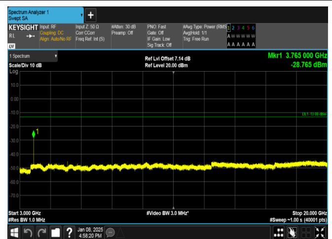
Band25-1.4MHz-QPSK-26365-6RB#0-3000~20000-PASS
