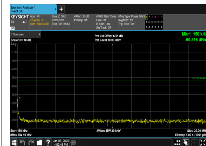
Band25-1.4MHz-QPSK-26365-1RB#0-0.15~30-PASS
