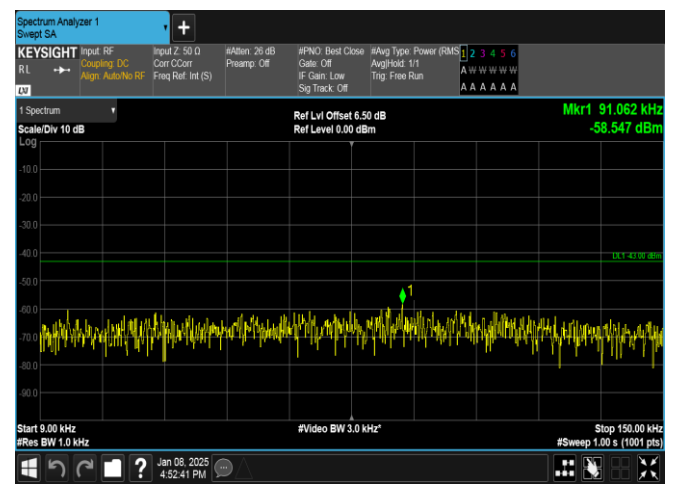
Band25-1.4MHz-QPSK-26365-1RB#0-0.009~0.15-PASS
