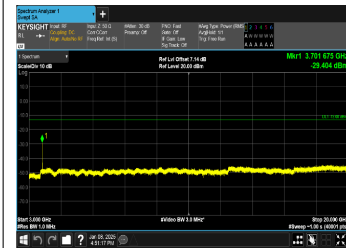
Band25-1.4MHz-QPSK-26047-6RB#0-3000~20000-PASS
