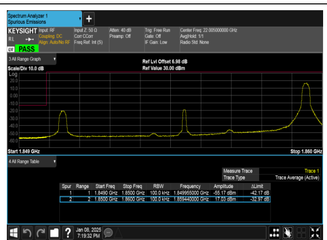
Band25-10MHz-16QAM-26090-1RB#49-PASS
