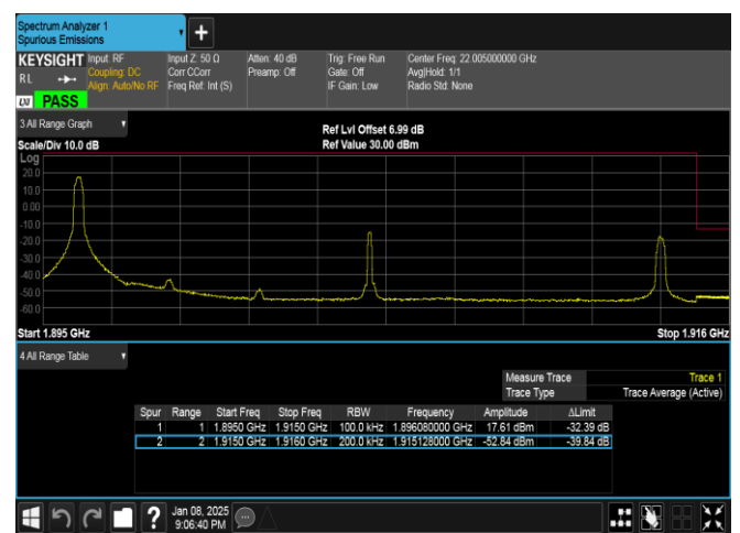
Band25-20MHz-16QAM-26590-1RB#0-PASS
