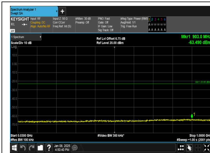
Band25-1.4MHz-QPSK-26047-6RB#0-30~1000-PASS
