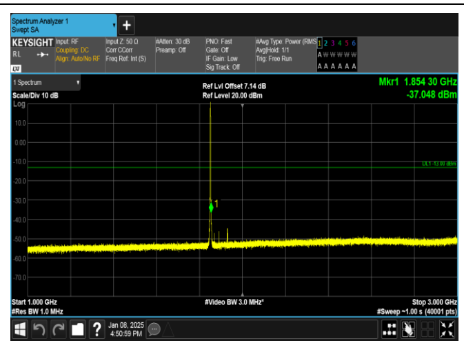
Band25-1.4MHz-QPSK-26047-6RB#0-1000~3000-PASS
