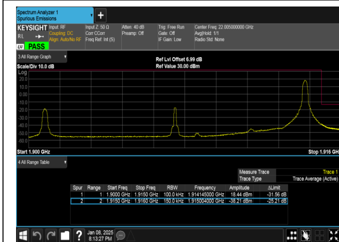
Band25-15MHz-QPSK-26615-1RB#74-PASS
