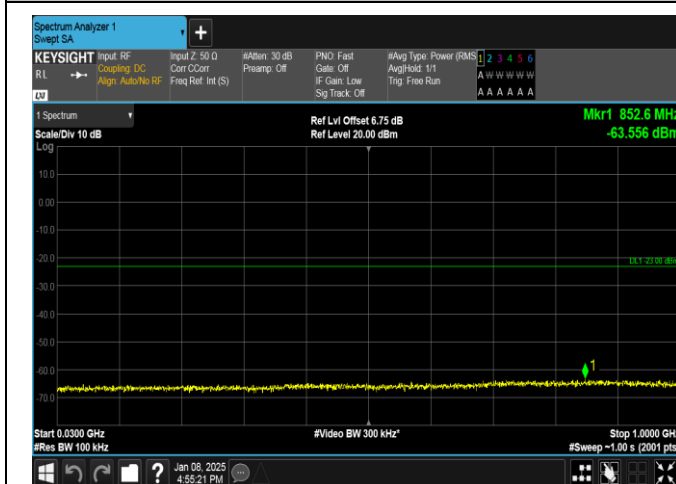
Band25-1.4MHz-QPSK-26365-1RB#5-30~1000-PASS
