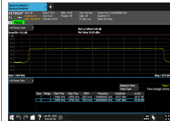
Band25-20MHz-QPSK-26140-100RB#0-PASS
