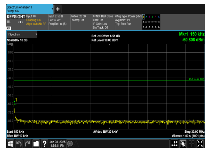
Band25-1.4MHz-QPSK-26365-1RB#5-0.15~30-PASS
