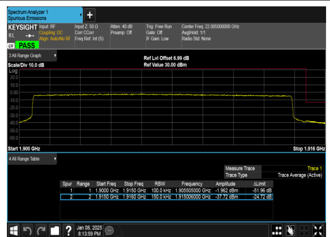
Band25-15MHz-QPSK-26615-75RB#0-PASS
