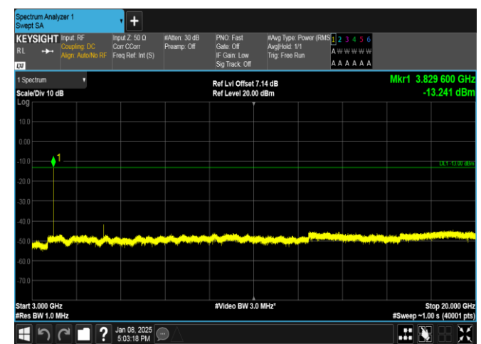
Band25-1.4MHz-QPSK-26683-1RB#5-3000~20000-PASS
