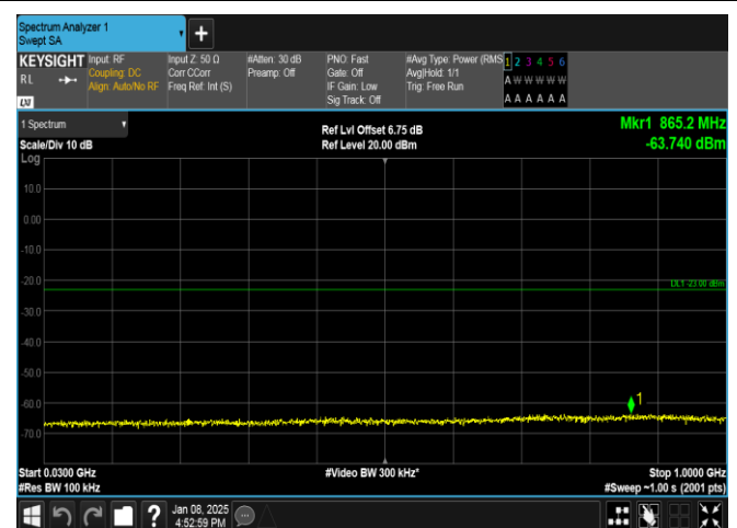
Band25-1.4MHz-QPSK-26365-1RB#0-30~1000-PASS
