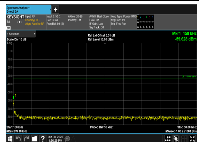
Band25-1.4MHz-QPSK-26047-6RB#0-0.15~30-PASS
