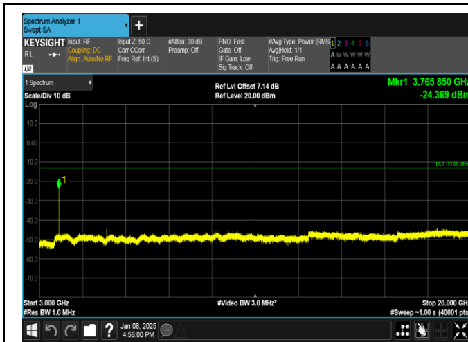
Band25-1.4MHz-QPSK-26365-1RB#5-3000~20000-PASS
