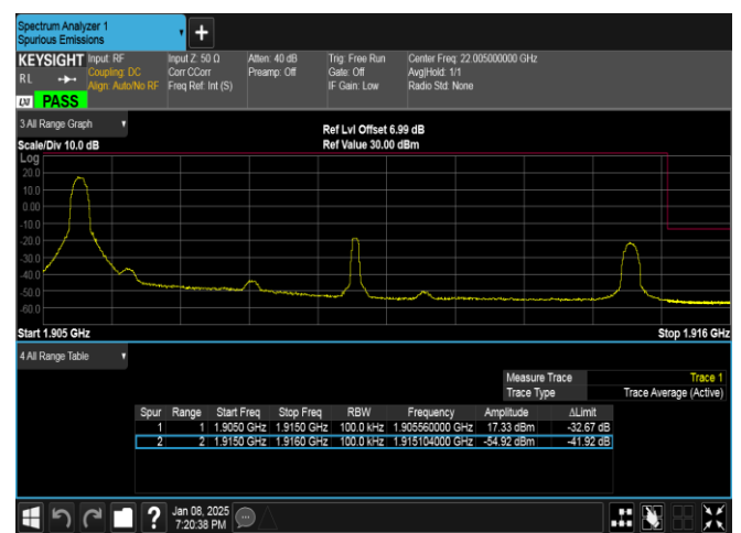
Band25-10MHz-16QAM-26640-1RB#0-PASS
