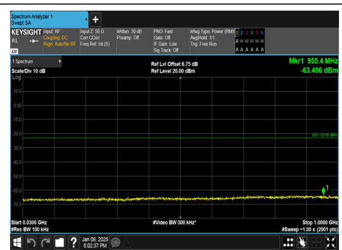
Band25-1.4MHz-QPSK-26683-1RB#5-30~1000-PASS
