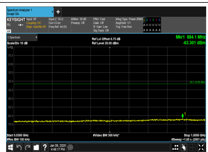
Band25-1.4MHz-QPSK-26047-1RB#5-30~1000-PASS
