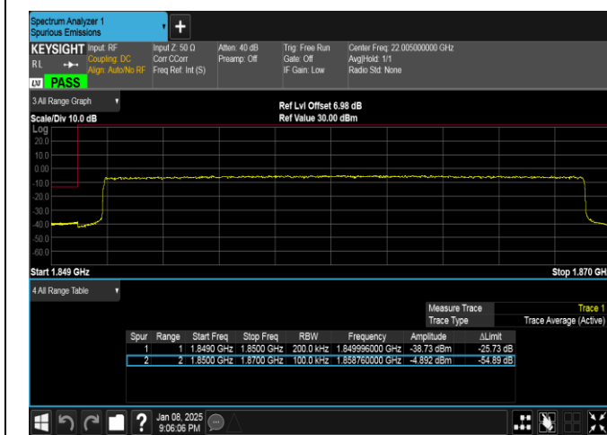
Band25-20MHz-16QAM-26140-100RB#0-PASS
