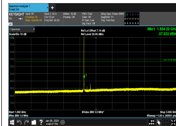
Band25-1.4MHz-QPSK-26047-1RB#5-1000~3000-PASS
