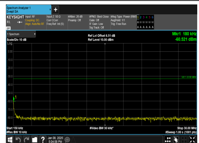
Band25-1.4MHz-QPSK-26683-6RB#0-0.15~30-PASS
