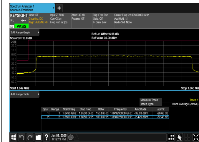
Band25-15MHz-QPSK-26115-75RB#0-PASS
