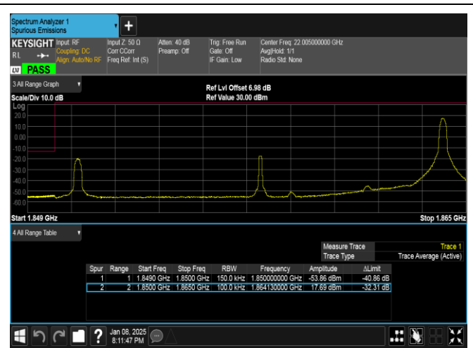
Band25-15MHz-QPSK-26115-1RB#74-PASS
