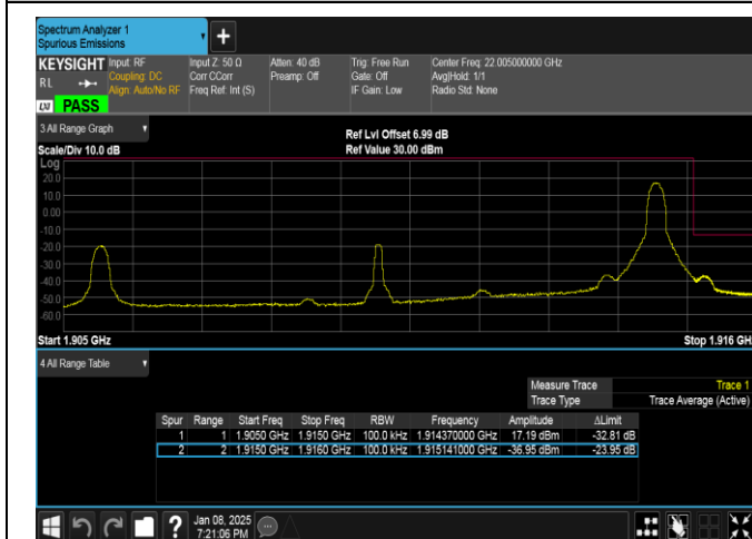
Band25-10MHz-16QAM-26640-1RB#49-PASS
