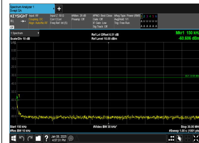
Band25-1.4MHz-QPSK-26365-6RB#0-0.15~30-PASS
