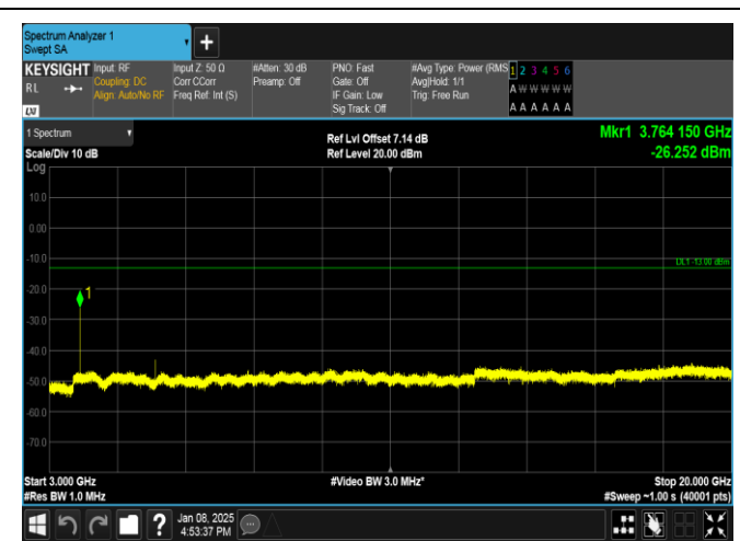
Band25-1.4MHz-QPSK-26365-1RB#0-3000~20000-PASS
