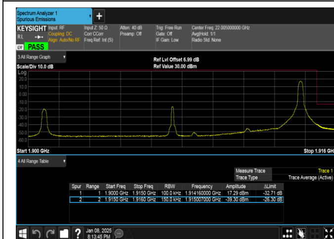
Band25-15MHz-16QAM-26615-1RB#74-PASS
