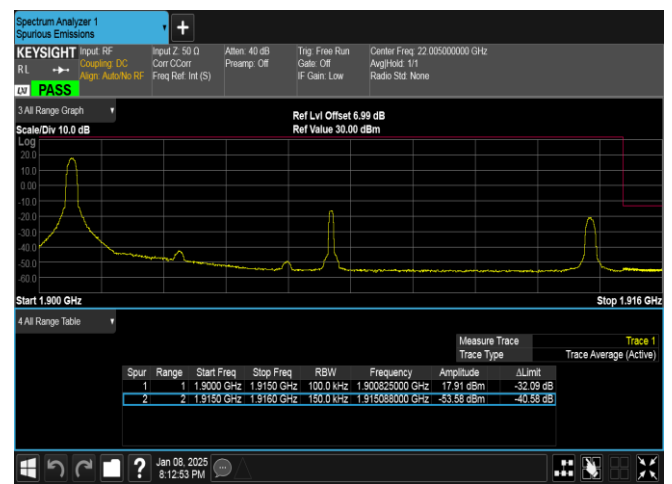
Band25-15MHz-QPSK-26615-1RB#0-PASS
