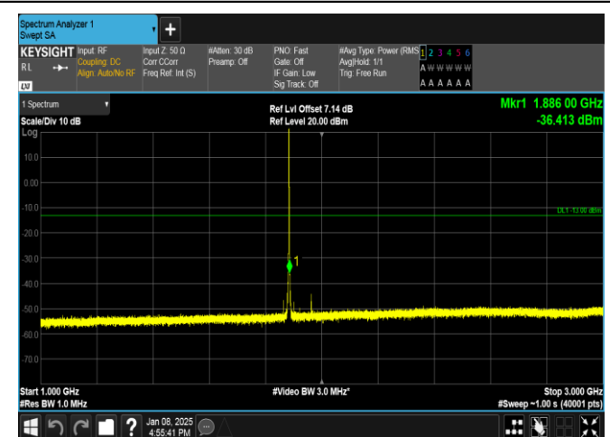
Band25-1.4MHz-QPSK-26365-1RB#5-1000~3000-PASS
