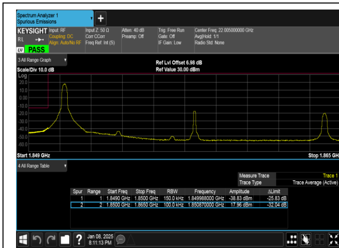
Band25-15MHz-QPSK-26115-1RB#0-PASS
