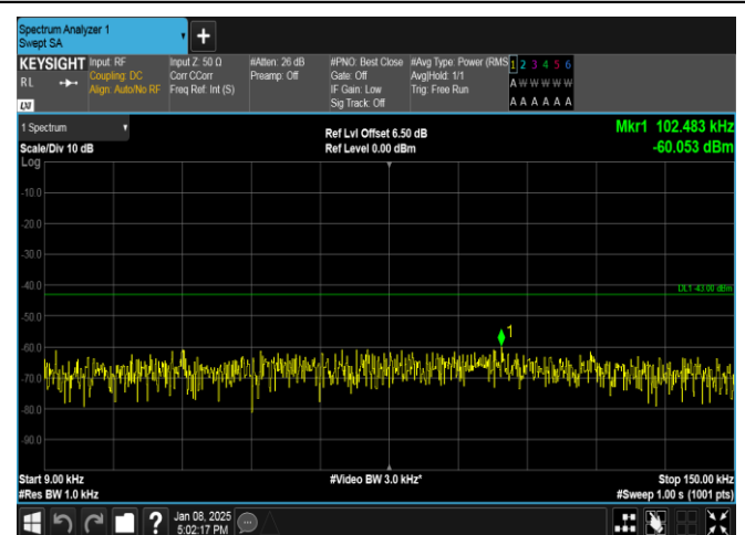
Band25-1.4MHz-QPSK-26683-1RB#5-0.009~0.15-PASS
