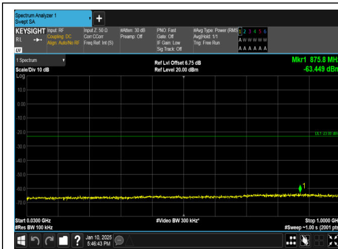
Band66-20MHz-16QAM-132322-100RB#0-30~1000-PASS
