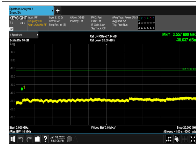
Band66-20MHz-16QAM-132572-1RB#99-3000~20000-PASS
