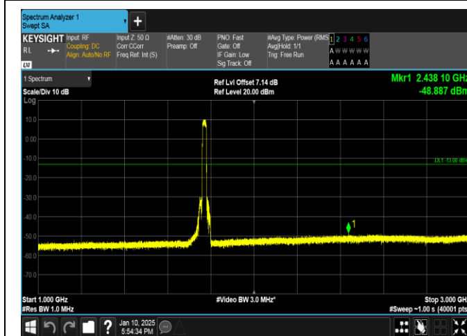
Band66-20MHz-16QAM-132572-100RB#0-1000~3000-PASS
