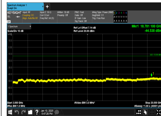
Band66-20MHz-16QAM-132322-100RB#0-3000~20000-PASS
