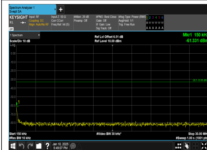
Band66-20MHz-16QAM-132572-1RB#0-0.15~30-PASS
