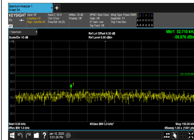
Band66-20MHz-16QAM-132572-1RB#99-0.009~0.15-PASS
