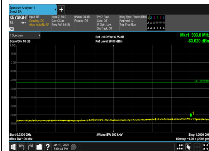
Band66-20MHz-16QAM-132572-1RB#99-30~1000-PASS
