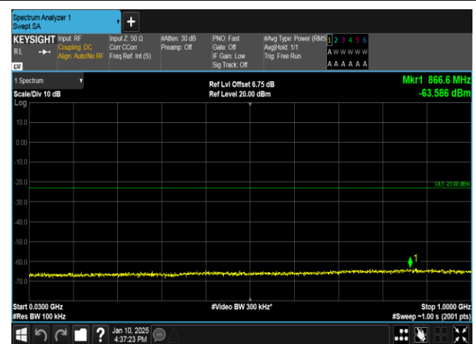
Band66-15MHz-16QAM-132047-1RB#0-30~1000-PASS
