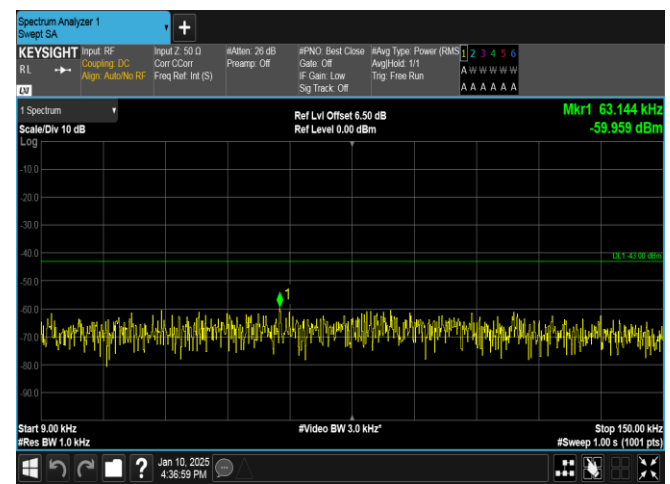
Band66-15MHz-16QAM-132047-1RB#0-0.009~0.15-PASS
