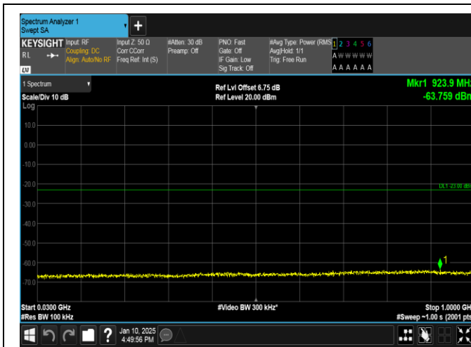
Band66-15MHz-16QAM-132322-75RB#0-30~1000-PASS
