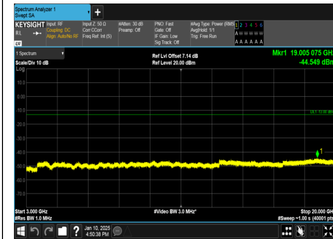
Band66-15MHz-16QAM-132322-75RB#0-3000~20000-PASS
