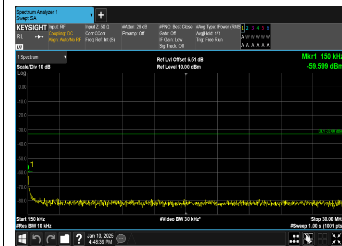
Band66-15MHz-QPSK-132322-75RB#0-0.15~30-PASS
