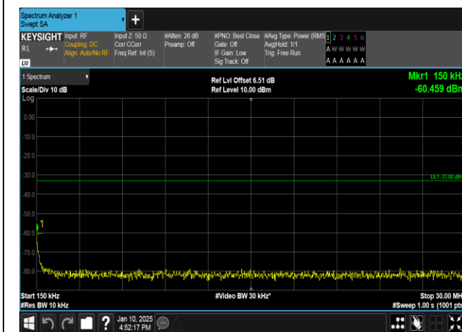
Band66-15MHz-16QAM-132597-1RB#0-0.15~30-PASS
