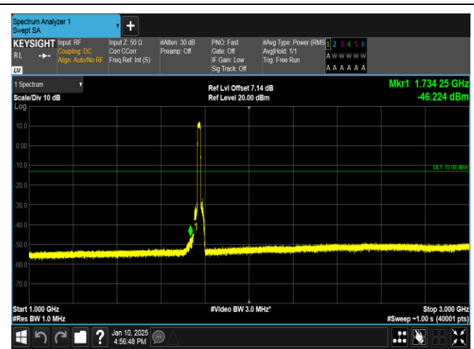
Band66-15MHz-QPSK-132597-75RB#0-1000~3000-PASS
