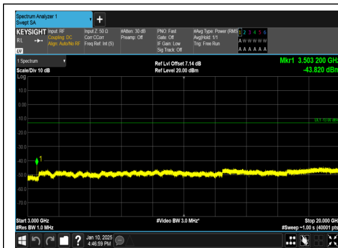
Band66-15MHz-QPSK-132322-1RB#74-3000~20000-PASS
