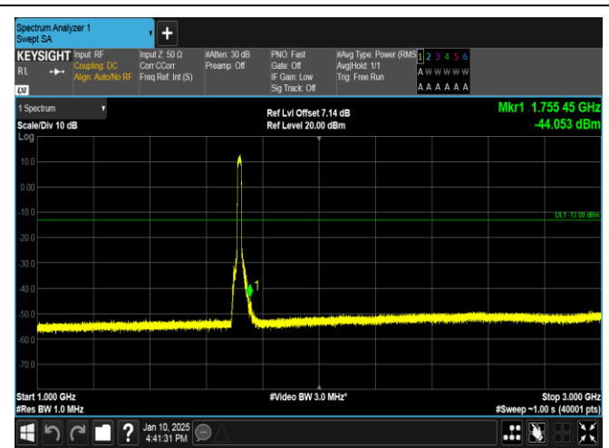
Band66-15MHz-QPSK-132047-75RB#0-1000~3000-PASS
