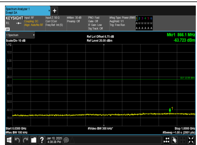
Band66-15MHz-QPSK-132047-1RB#74-30~1000-PASS
