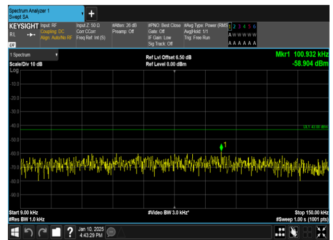
Band66-15MHz-QPSK-132322-1RB#0-0.009~0.15-PASS
