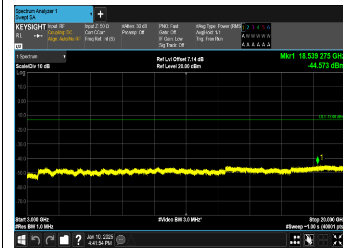
Band66-15MHz-QPSK-132047-75RB#0-3000~20000-PASS
