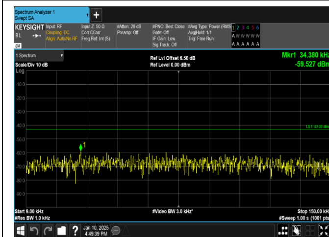
Band66-15MHz-16QAM-132322-75RB#0-0.009~0.15-PASS
