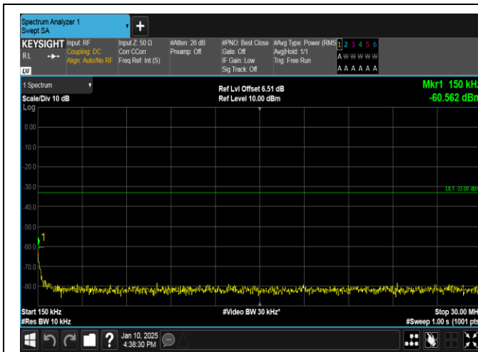
Band66-15MHz-QPSK-132047-1RB#74-0.15~30-PASS
