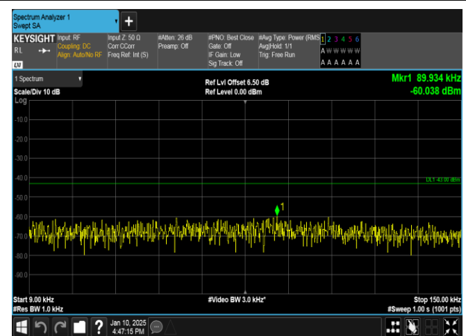
Band66-15MHz-16QAM-132322-1RB#74-0.009~0.15-PASS
