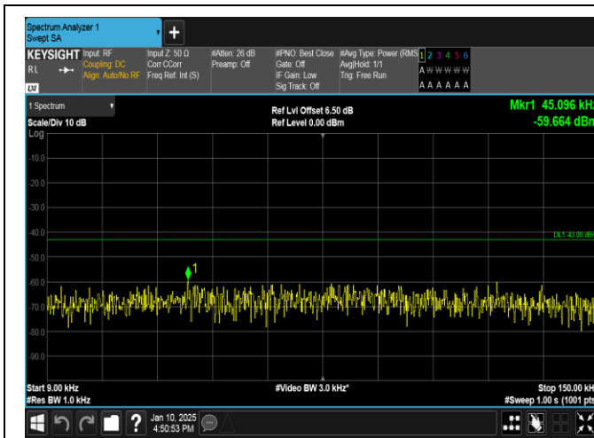
Band66-15MHz-QPSK-132597-1RB#0-0.009~0.15-PASS
