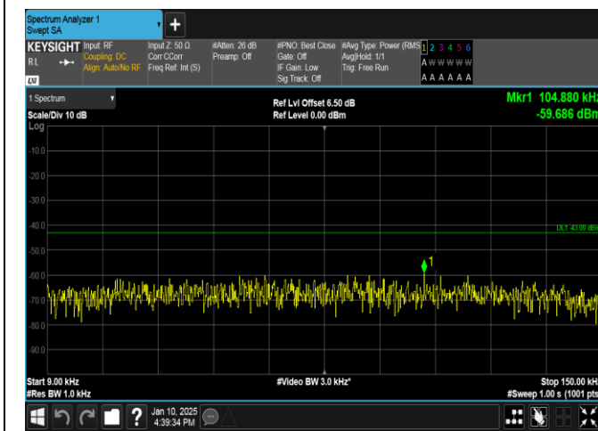
Band66-15MHz-16QAM-132047-1RB#74-0.009~0.15-PASS
