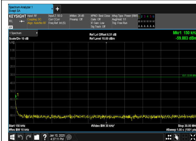
Band66-15MHz-16QAM-132047-1RB#0-0.15~30-PASS
