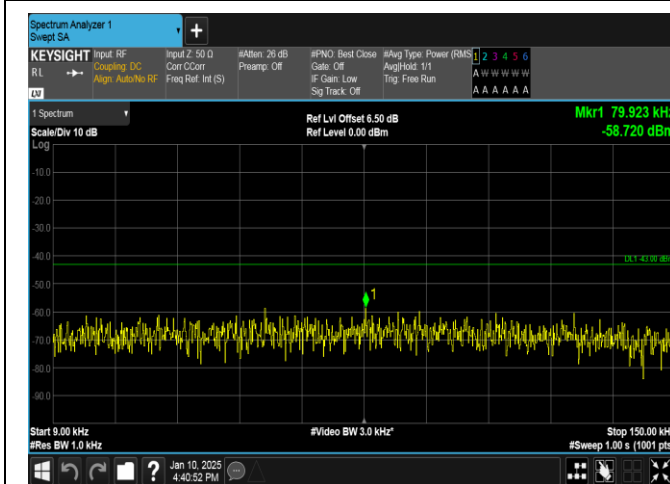
Band66-15MHz-QPSK-132047-75RB#0-0.009~0.15-PASS
