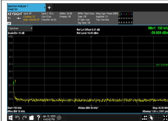
Band66-15MHz-QPSK-132322-1RB#0-0.15~30-PASS
