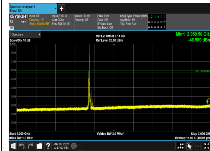
Band66-15MHz-16QAM-132322-1RB#74-1000~3000-PASS
