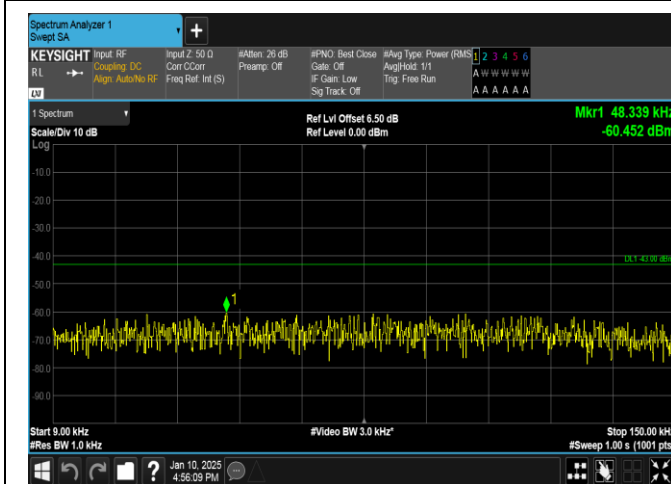
Band66-15MHz-QPSK-132597-75RB#0-0.009~0.15-PASS
