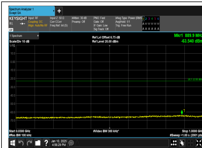
Band66-15MHz-QPSK-132597-75RB#0-30~1000-PASS
