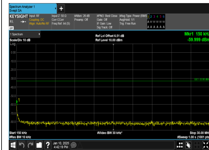
Band66-15MHz-16QAM-132047-75RB#0-0.15~30-PASS
