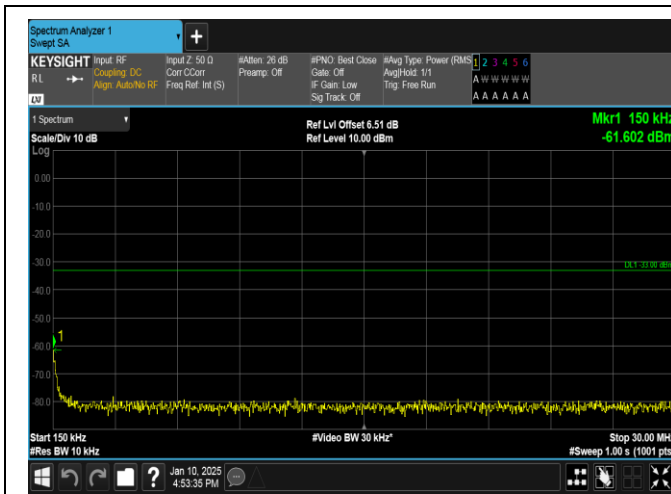
Band66-15MHz-QPSK-132597-1RB#74-0.15~30-PASS
