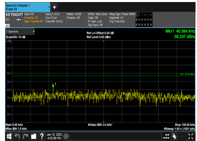
Band66-15MHz-16QAM-132597-1RB#0-0.009~0.15-PASS
