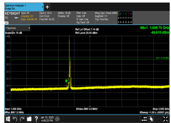
Band66-15MHz-16QAM-132322-1RB#0-1000~3000-PASS
