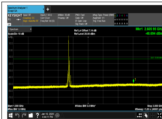
Band66-15MHz-QPSK-132322-1RB#0-1000~3000-PASS
