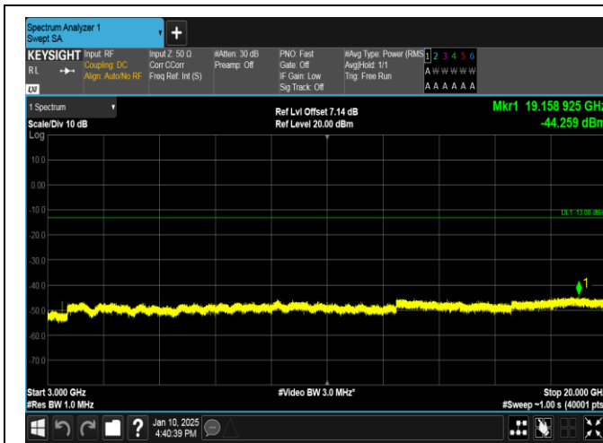
Band66-15MHz-16QAM-132047-1RB#74-3000~20000-PASS
