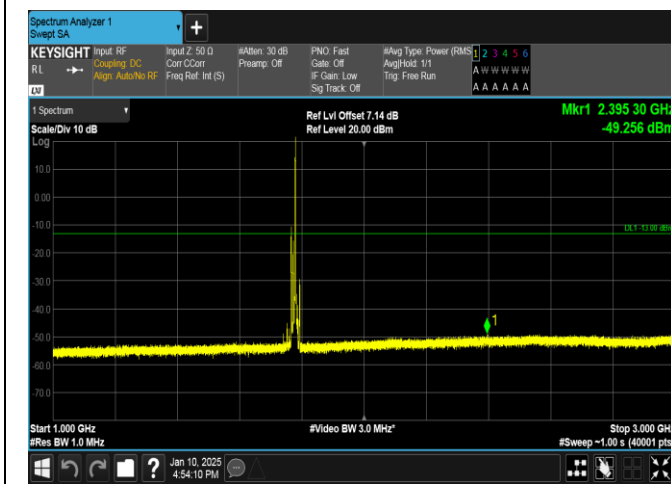
Band66-15MHz-QPSK-132597-1RB#74-1000~3000-PASS
