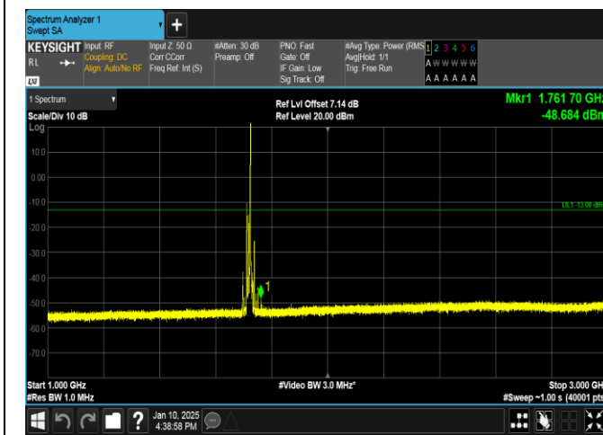
Band66-15MHz-QPSK-132047-1RB#74-1000~3000-PASS
