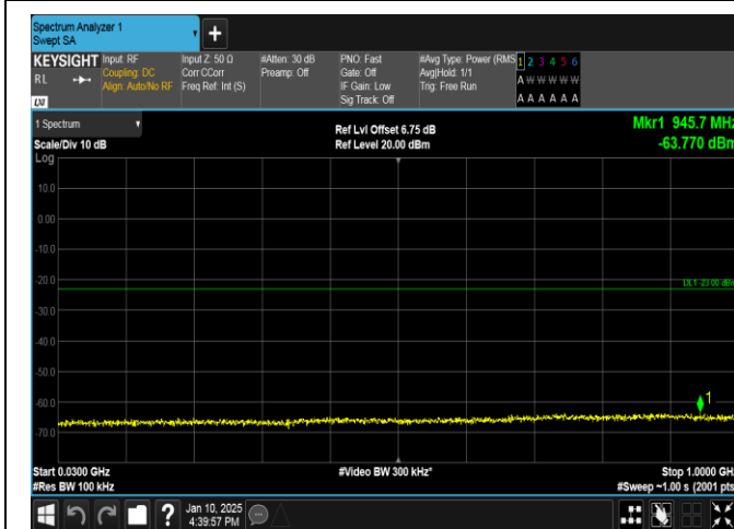
Band66-15MHz-16QAM-132047-1RB#74-30~1000-PASS
