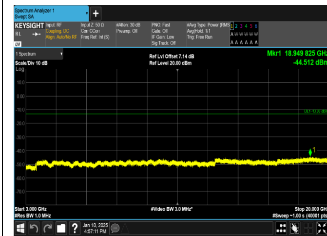
Band66-15MHz-QPSK-132597-75RB#0-3000~20000-PASS
