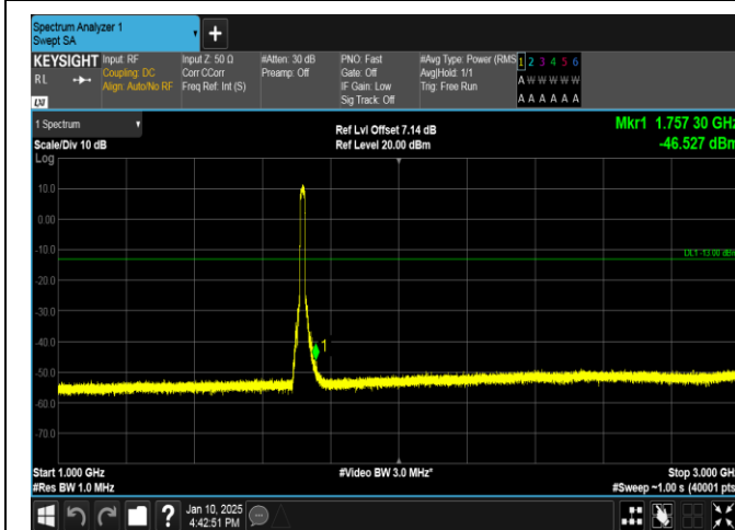
Band66-15MHz-16QAM-132047-75RB#0-1000~3000-PASS
