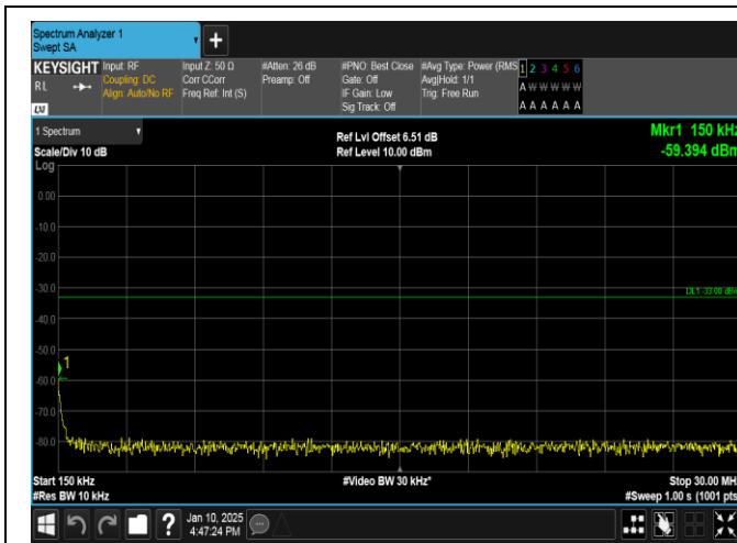
Band66-15MHz-16QAM-132322-1RB#74-0.15~30-PASS
