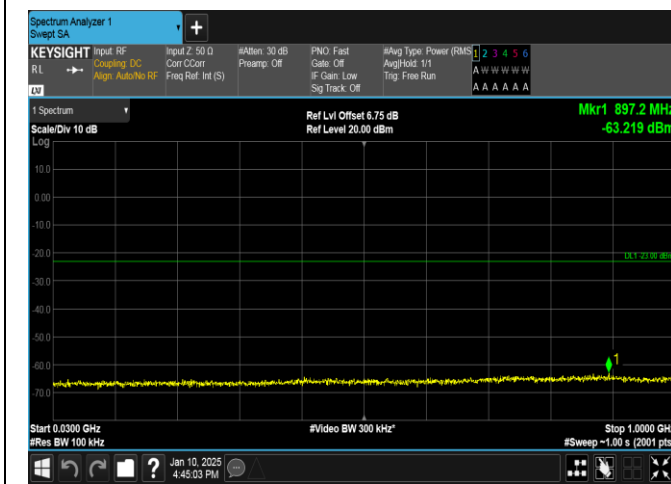
Band66-15MHz-16QAM-132322-1RB#0-30~1000-PASS
