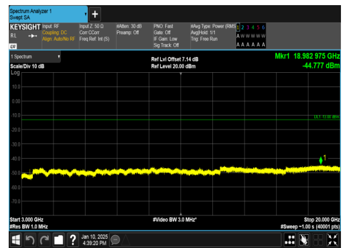
Band66-15MHz-QPSK-132047-1RB#74-3000~20000-PASS
