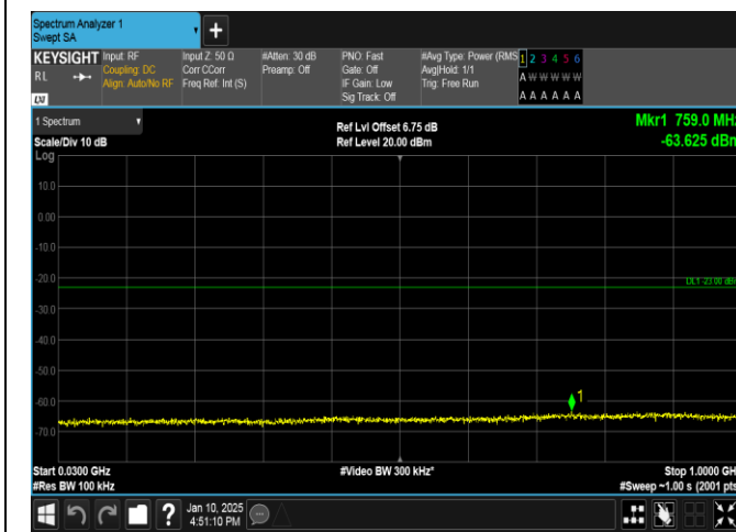
Band66-15MHz-QPSK-132597-1RB#0-30~1000-PASS
