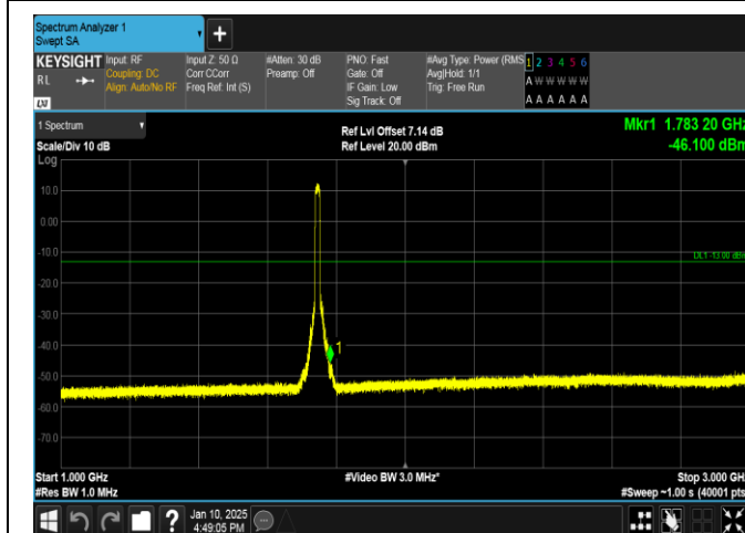
Band66-15MHz-QPSK-132322-75RB#0-1000~3000-PASS
