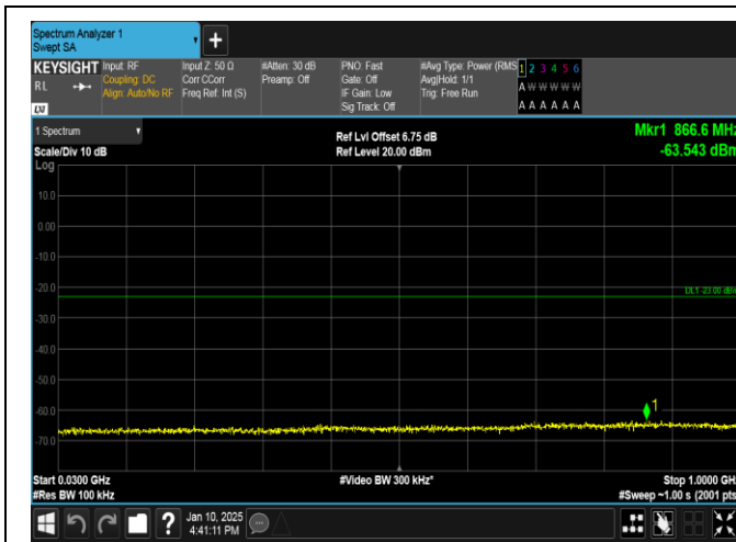
Band66-15MHz-QPSK-132047-75RB#0-30~1000-PASS
