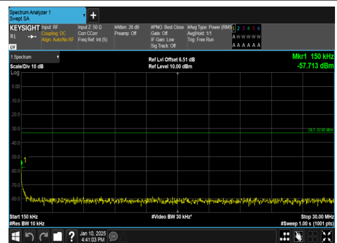
Band66-15MHz-QPSK-132047-75RB#0-0.15~30-PASS
