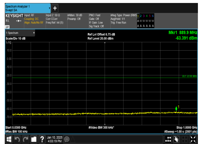
Band66-10MHz-16QAM-132622-50RB#0-30~1000-PASS
