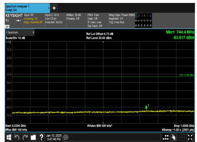
Band66-10MHz-16QAM-132022-50RB#0-30~1000-PASS
