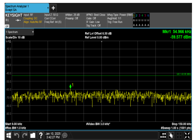
Band66-10MHz-16QAM-132022-1RB#0-0.009~0.15-PASS
