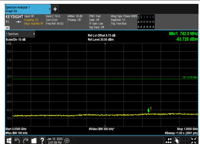
Band66-10MHz-16QAM-132622-1RB#0-30~1000-PASS
