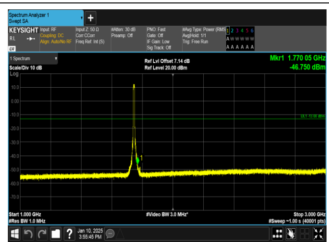
Band66-10MHz-16QAM-132322-50RB#0-1000~3000-PASS
