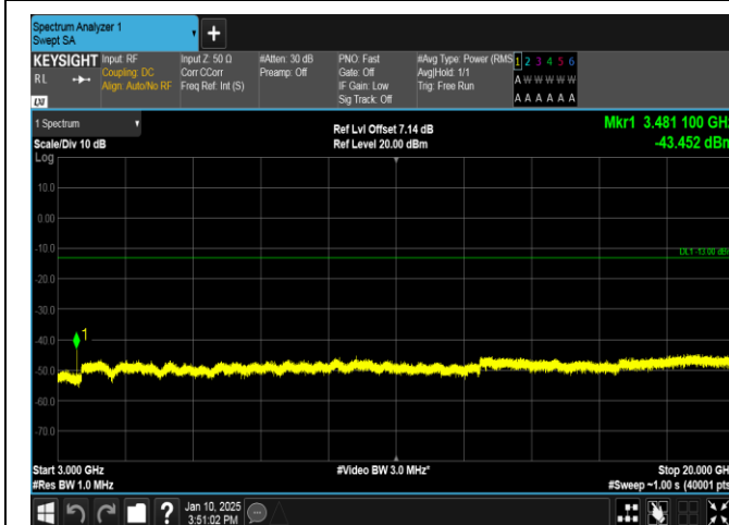
Band66-10MHz-16QAM-132322-1RB#0-3000~20000-PASS
