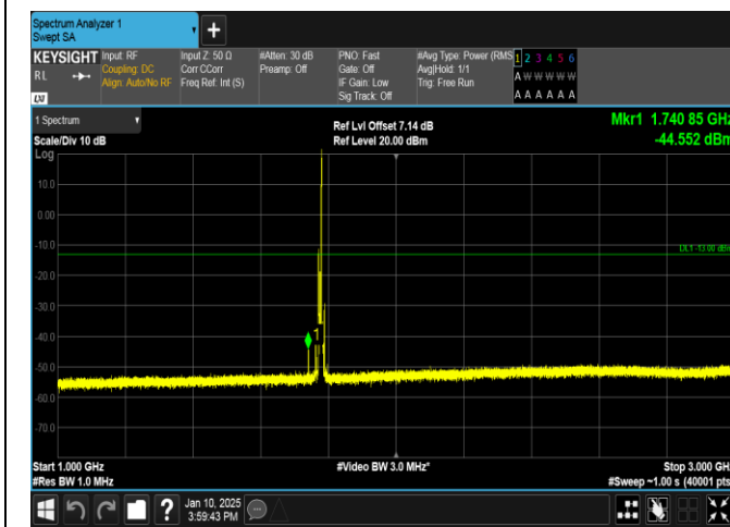
Band66-10MHz-QPSK-132622-1RB#49-1000~3000-PASS
