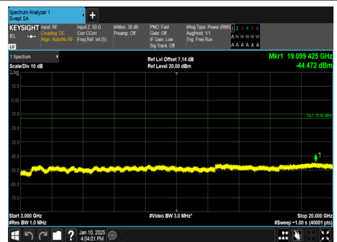
Band66-10MHz-16QAM-132622-50RB#0-3000~20000-PASS
