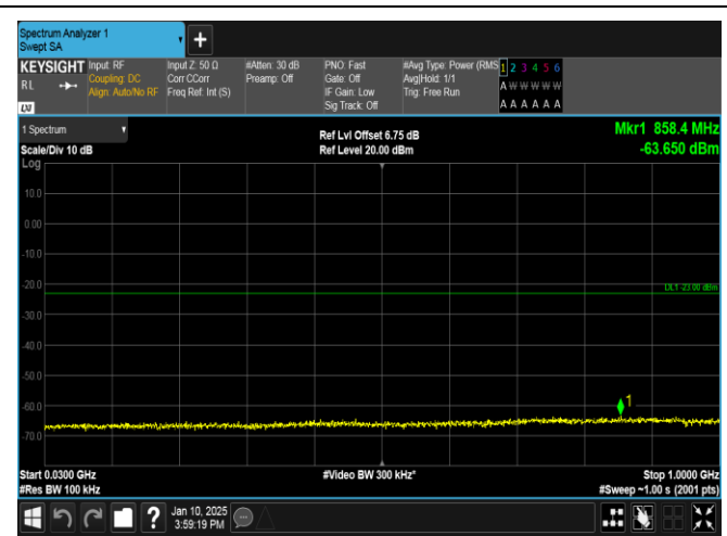
Band66-10MHz-QPSK-132622-1RB#49-30~1000-PASS
