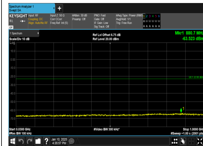
Band66-15MHz-QPSK-132047-1RB#0-30~1000-PASS
