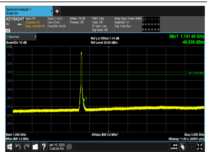
Band66-10MHz-QPSK-132022-50RB#0-1000~3000-PASS
