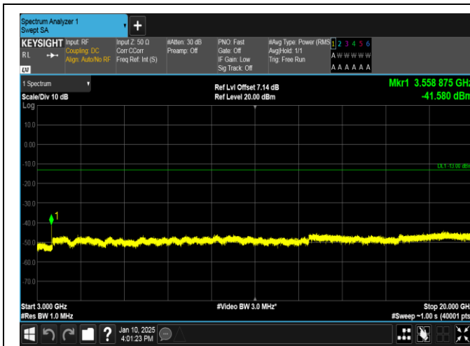
Band66-10MHz-16QAM-132622-1RB#49-3000~20000-PASS
