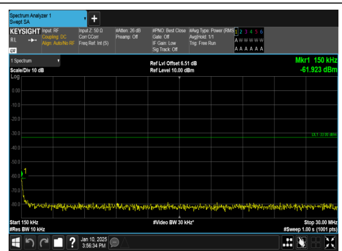
Band66-10MHz-QPSK-132622-1RB#0-0.15~30-PASS
