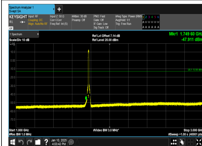
Band66-10MHz-16QAM-132622-50RB#0-1000~3000-PASS
