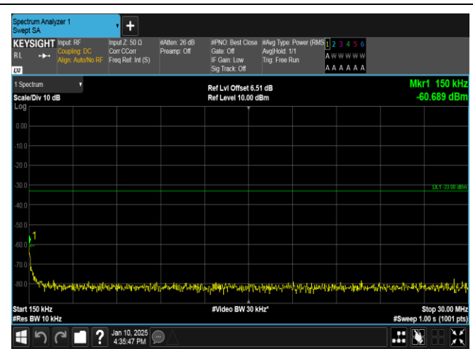
Band66-15MHz-QPSK-132047-1RB#0-0.15~30-PASS
