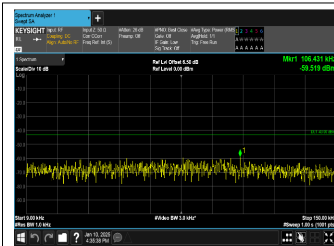
Band66-15MHz-QPSK-132047-1RB#0-0.009~0.15-PASS
