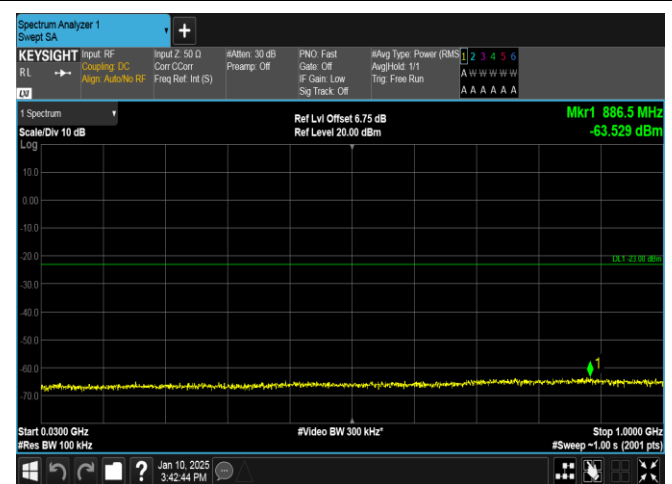
Band66-10MHz-16QAM-132022-1RB#0-30~1000-PASS
