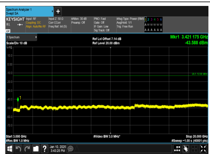
Band66-10MHz-16QAM-132022-1RB#0-3000~20000-PASS
