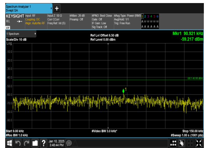
Band66-10MHz-QPSK-132322-1RB#0-0.009~0.15-PASS
