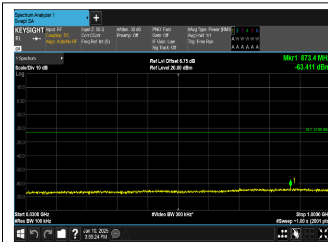
Band66-10MHz-16QAM-132322-50RB#0-30~1000-PASS
