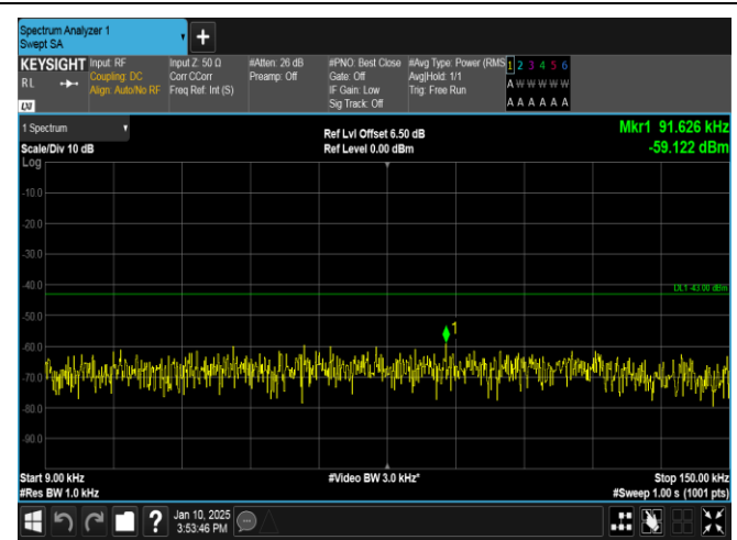
Band66-10MHz-QPSK-132322-50RB#0-0.009~0.15-PASS
