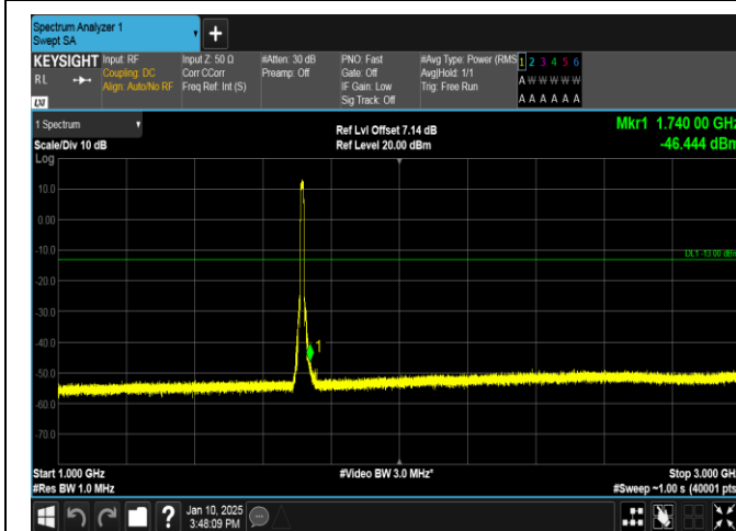
Band66-10MHz-16QAM-132022-50RB#0-1000~3000-PASS
