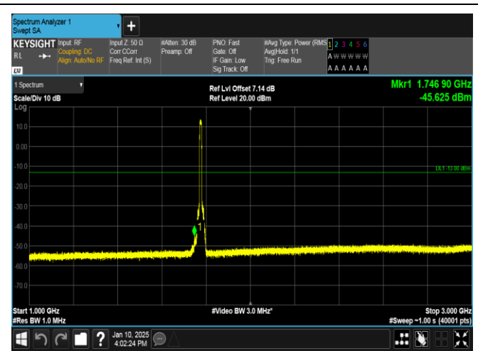
Band66-10MHz-QPSK-132622-50RB#0-1000~3000-PASS
