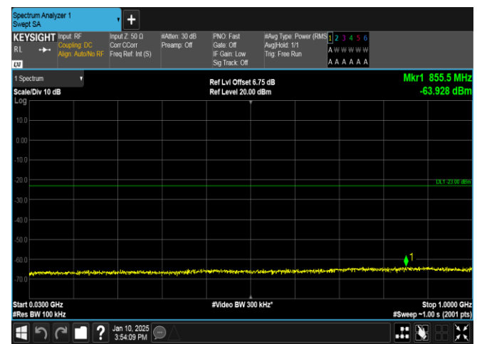
Band66-10MHz-QPSK-132322-50RB#0-30~1000-PASS
