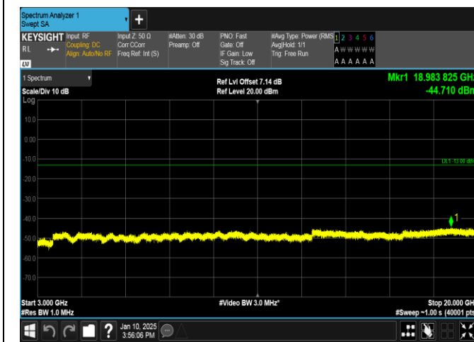
Band66-10MHz-16QAM-132322-50RB#0-3000~20000-PASS
