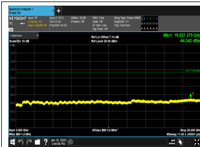
Band66-10MHz-16QAM-132022-1RB#49-3000~20000-PASS
