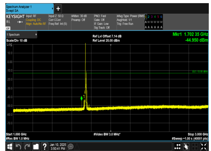
Band66-10MHz-16QAM-132322-1RB#0-1000~3000-PASS
