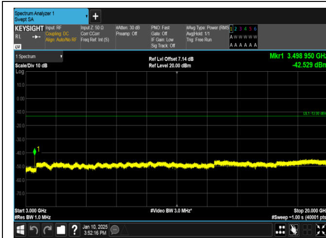
Band66-10MHz-QPSK-132322-1RB#49-3000~20000-PASS
