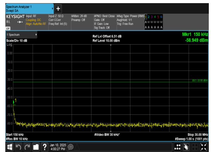
Band66-10MHz-16QAM-132622-1RB#49-0.15~30-PASS
