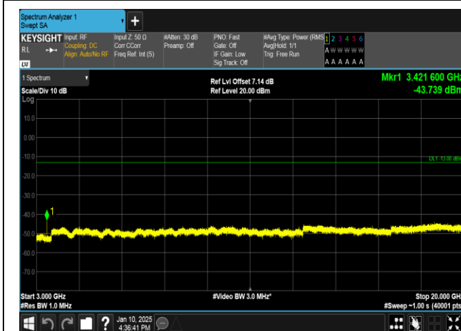
Band66-15MHz-QPSK-132047-1RB#0-3000~20000-PASS
