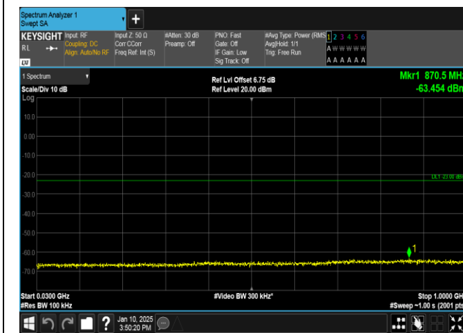
Band66-10MHz-16QAM-132322-1RB#0-30~1000-PASS
