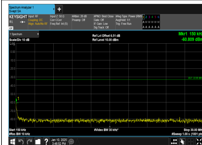
Band66-10MHz-QPSK-132322-1RB#0-0.15~30-PASS
