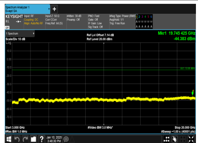
Band66-10MHz-16QAM-132022-50RB#0-3000~20000-PASS
