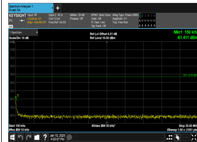
Band66-10MHz-16QAM-132622-50RB#0-0.15~30-PASS
