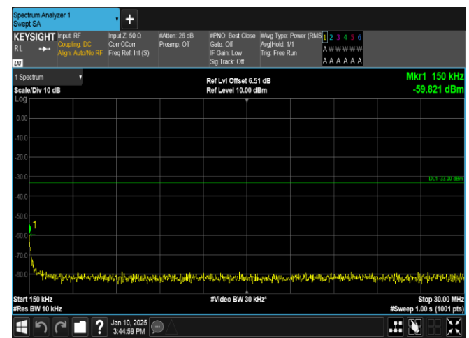
Band66-10MHz-16QAM-132022-1RB#49-0.15~30-PASS
