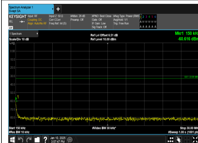
Band66-10MHz-16QAM-132622-1RB#0-0.15~30-PASS
