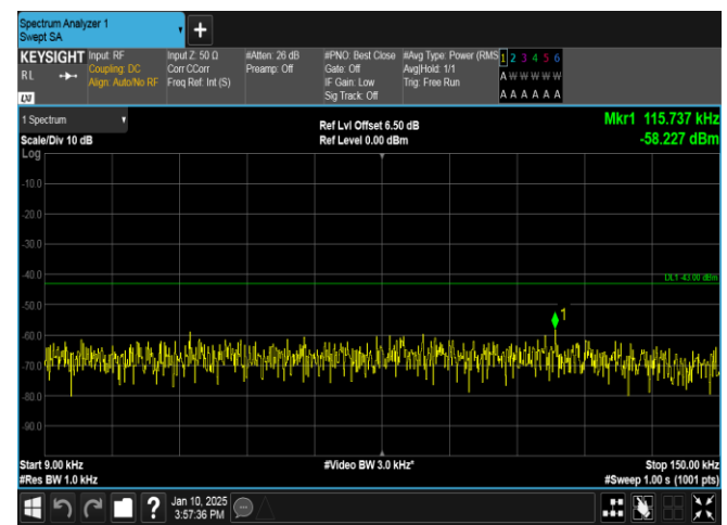
Band66-10MHz-16QAM-132622-1RB#0-0.009~0.15-PASS
