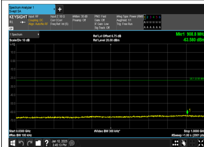
Band66-10MHz-16QAM-132022-1RB#49-30~1000-PASS
