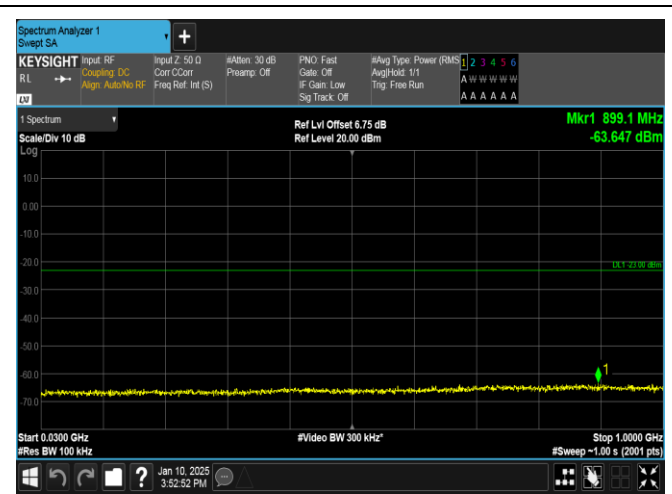
Band66-10MHz-16QAM-132322-1RB#49-30~1000-PASS
