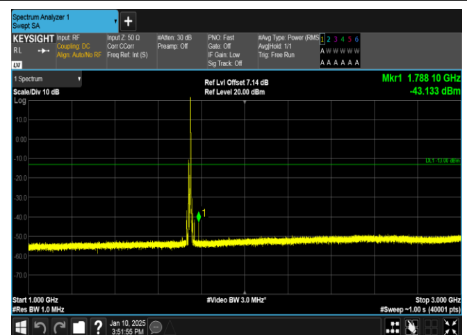
Band66-10MHz-QPSK-132322-1RB#49-1000~3000-PASS
