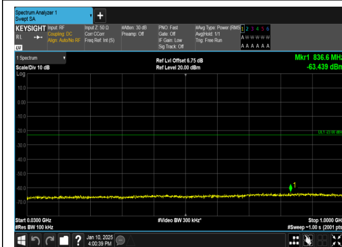
Band66-10MHz-16QAM-132622-1RB#49-30~1000-PASS
