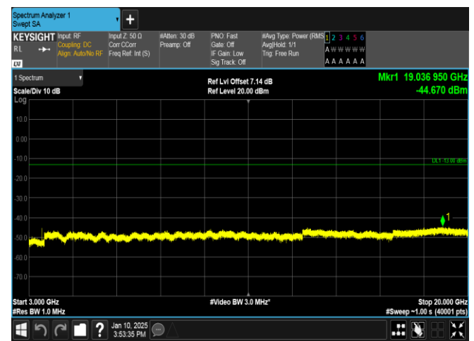
Band66-10MHz-16QAM-132322-1RB#49-3000~20000-PASS
