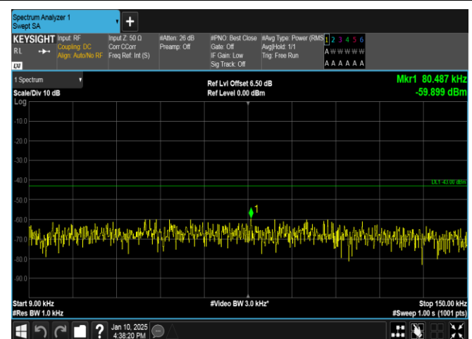
Band66-15MHz-QPSK-132047-1RB#74-0.009~0.15-PASS
