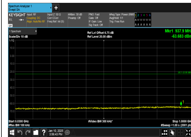
Band66-10MHz-QPSK-132622-1RB#0-30~1000-PASS
