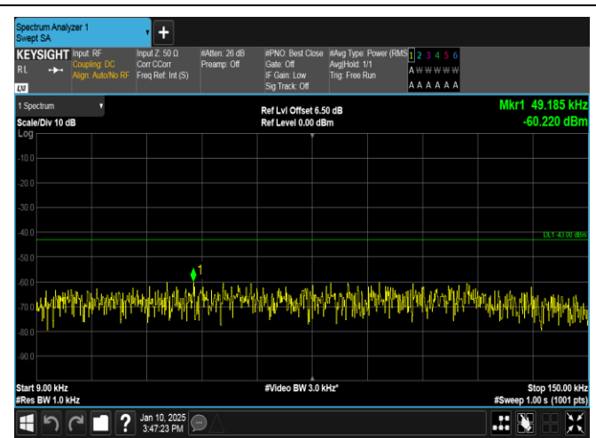
Band66-10MHz-16QAM-132022-50RB#0-0.009~0.15-PASS
