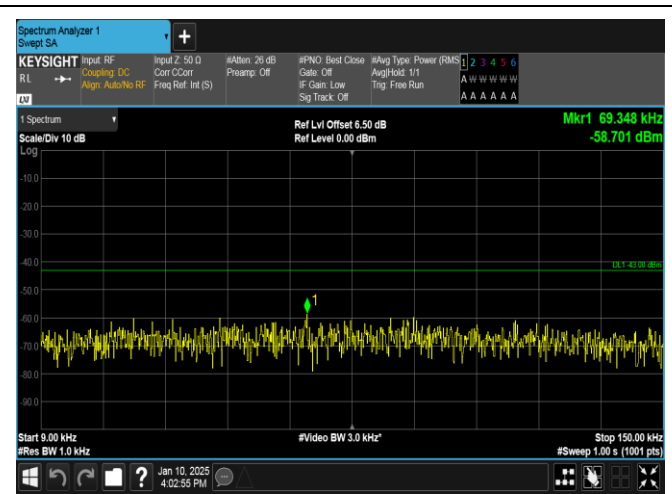
Band66-10MHz-16QAM-132622-50RB#0-0.009~0.15-PASS
