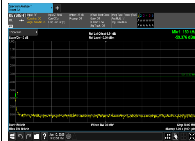
Band66-10MHz-QPSK-132322-50RB#0-0.15~30-PASS
