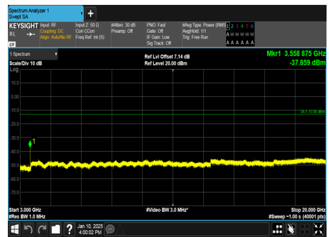
Band66-10MHz-QPSK-132622-1RB#49-3000~20000-PASS
