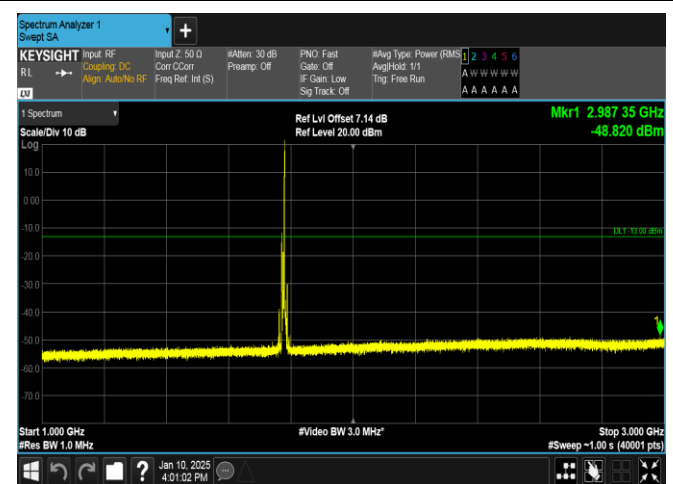
Band66-10MHz-16QAM-132622-1RB#49-1000~3000-PASS
