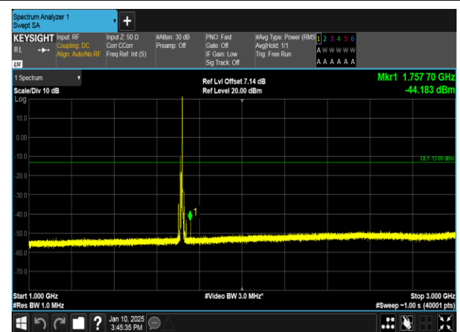
Band66-10MHz-16QAM-132022-1RB#49-1000~3000-PASS
