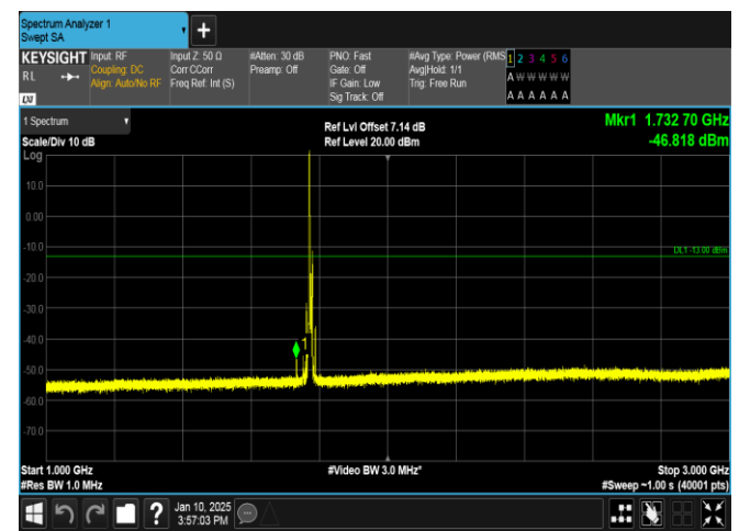
Band66-10MHz-QPSK-132622-1RB#0-1000~3000-PASS
