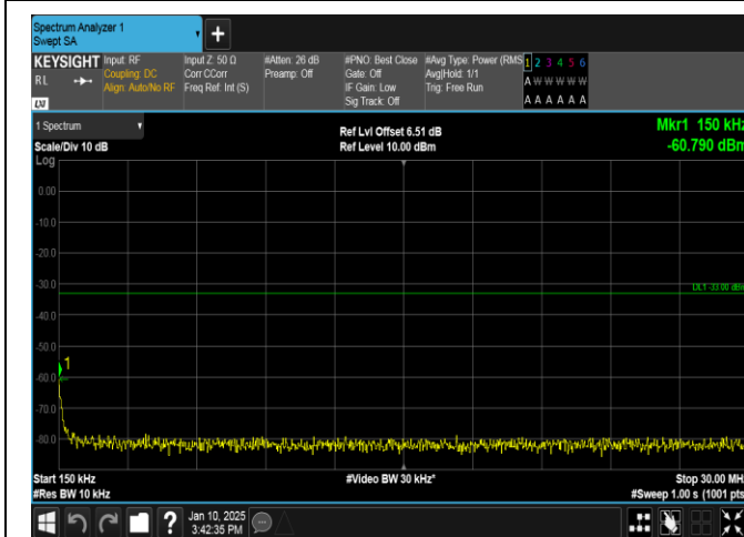
Band66-10MHz-16QAM-132022-1RB#0-0.15~30-PASS
