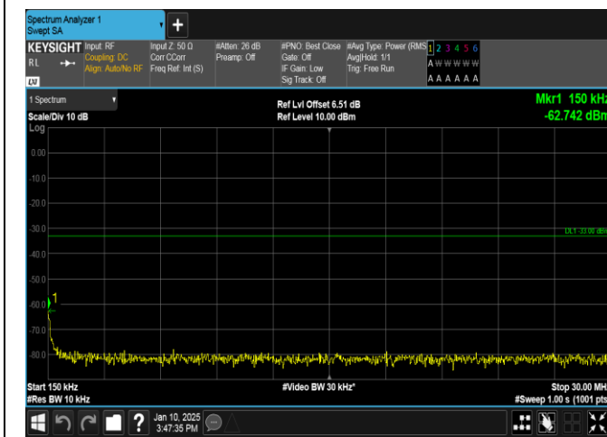
Band66-10MHz-16QAM-132022-50RB#0-0.15~30-PASS
