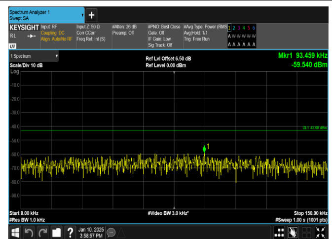
Band66-10MHz-QPSK-132622-1RB#49-0.009~0.15-PASS
