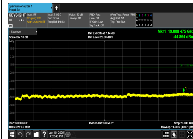
Band66-10MHz-QPSK-132622-50RB#0-3000~20000-PASS
