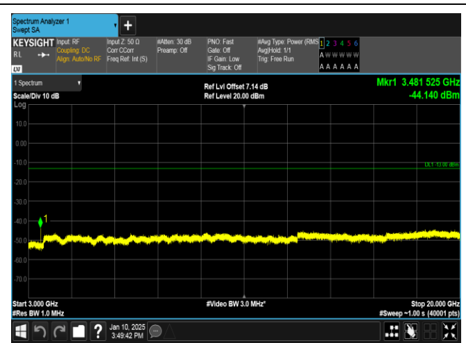
Band66-10MHz-QPSK-132322-1RB#0-3000~20000-PASS
