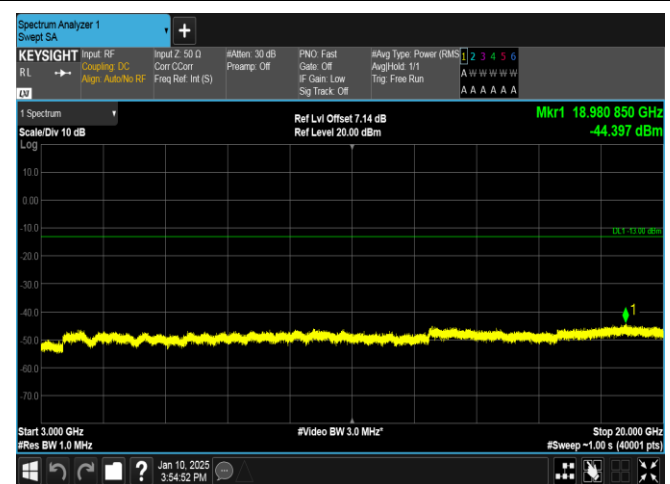
Band66-10MHz-QPSK-132322-50RB#0-3000~20000-PASS
