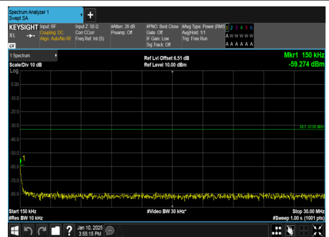
Band66-10MHz-16QAM-132322-50RB#0-0.15~30-PASS
