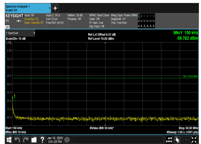
Band66-10MHz-QPSK-132322-1RB#49-0.15~30-PASS
