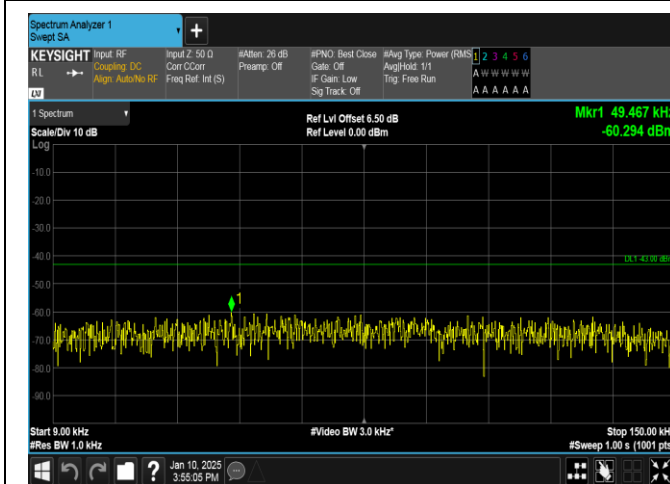
Band66-10MHz-16QAM-132322-50RB#0-0.009~0.15-PASS
