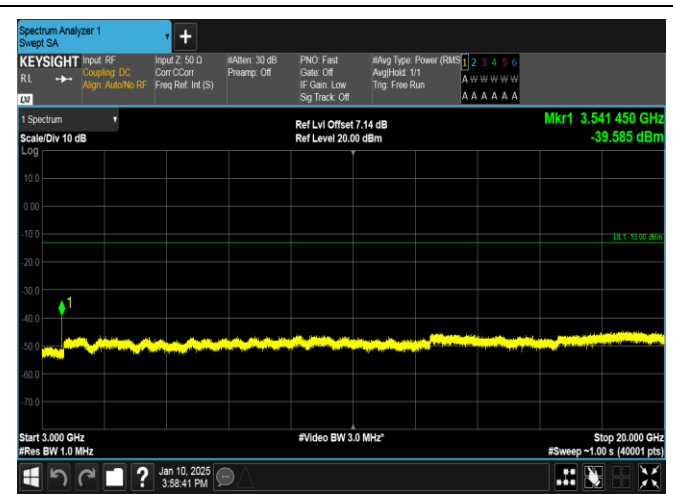
Band66-10MHz-16QAM-132622-1RB#0-3000~20000-PASS
