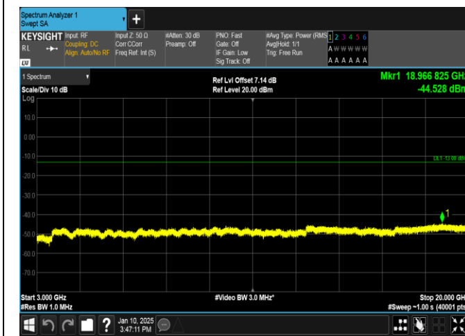
Band66-10MHz-QPSK-132022-50RB#0-3000~20000-PASS
