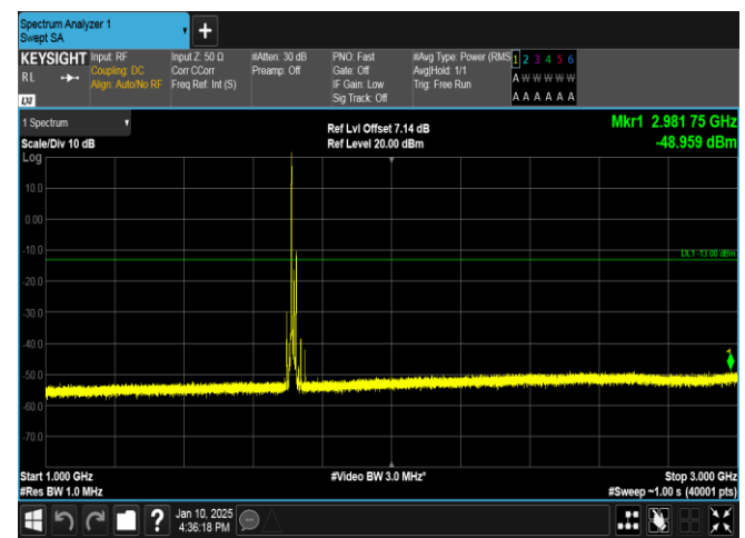
Band66-15MHz-QPSK-132047-1RB#0-1000~3000-PASS
