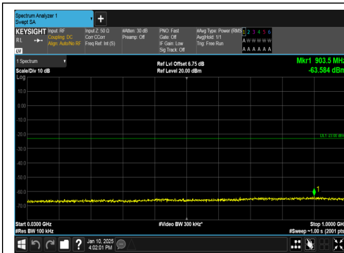
Band66-10MHz-QPSK-132622-50RB#0-30~1000-PASS
