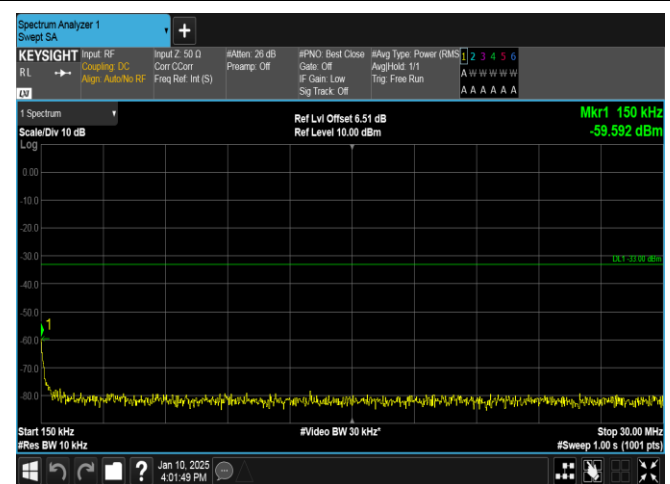
Band66-10MHz-QPSK-132622-50RB#0-0.15~30-PASS
