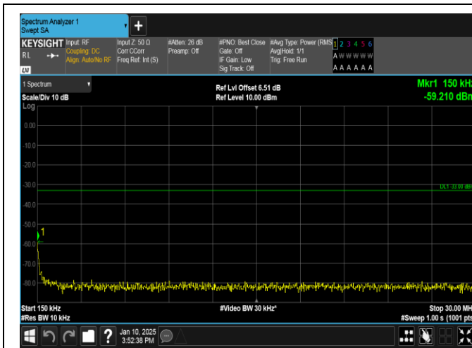
Band66-10MHz-16QAM-132322-1RB#49-0.15~30-PASS
