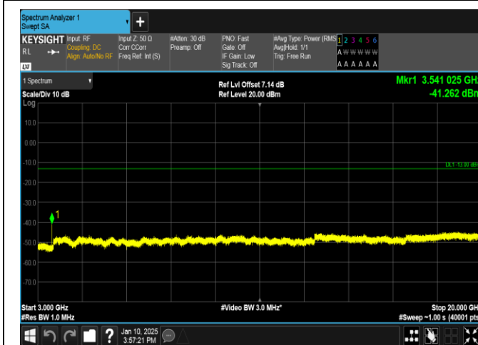
Band66-10MHz-QPSK-132622-1RB#0-3000~20000-PASS
