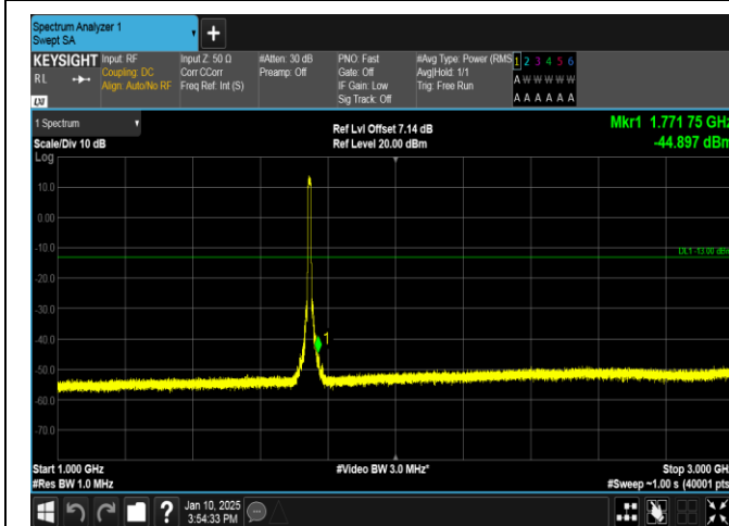
Band66-10MHz-QPSK-132322-50RB#0-1000~3000-PASS
