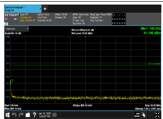
Band66-10MHz-16QAM-132322-1RB#0-0.15~30-PASS
