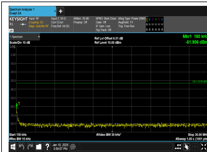
Band66-10MHz-QPSK-132622-1RB#49-0.15~30-PASS
