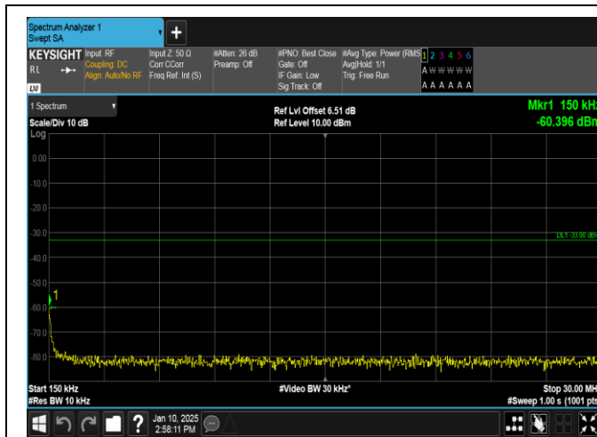
Band66-5MHz-16QAM-132322-1RB#24-0.15~30-PASS
