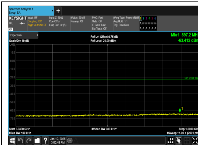
Band66-5MHz-16QAM-132322-25RB#0-30~1000-PASS
