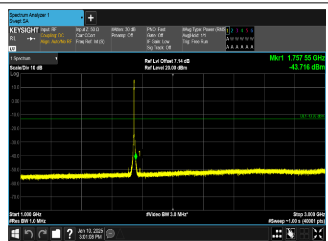
Band66-5MHz-16QAM-132322-25RB#0-1000~3000-PASS
