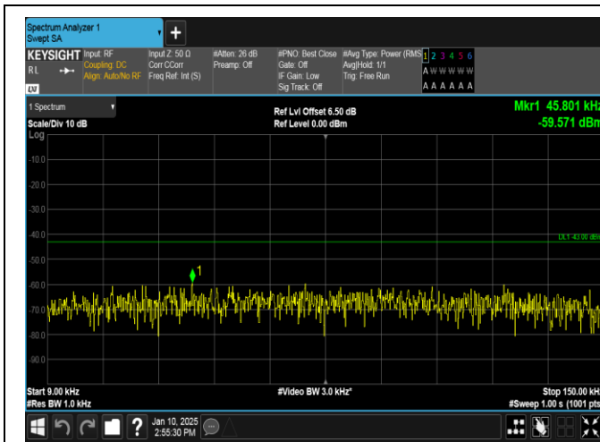
Band66-5MHz-16QAM-132322-1RB#0-0.009~0.15-PASS
