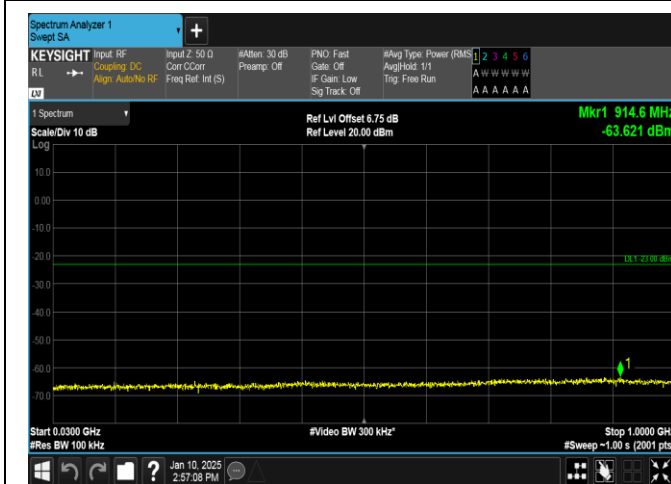
Band66-5MHz-QPSK-132322-1RB#24-30~1000-PASS
