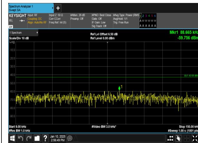
Band66-5MHz-QPSK-132322-1RB#24-0.009~0.15-PASS
