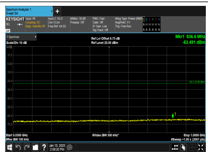
Band66-5MHz-16QAM-132322-1RB#24-30~1000-PASS
