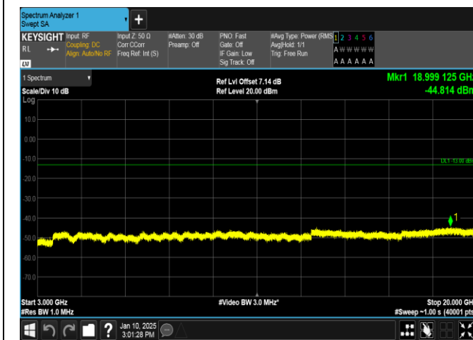
Band66-5MHz-16QAM-132322-25RB#0-3000~20000-PASS
