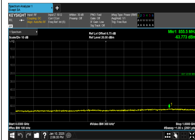
Band66-3MHz-QPSK-132657-1RB#0-30~1000-PASS
