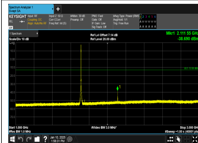
Band66-3MHz-16QAM-131987-15RB#0-1000~3000-PASS
