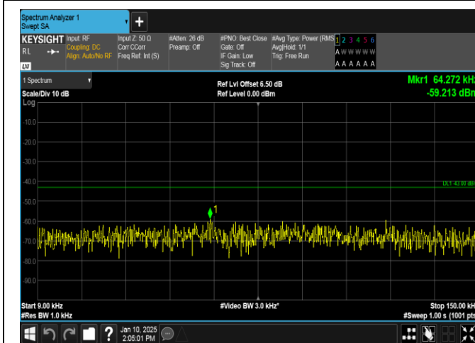
Band66-3MHz-16QAM-132322-15RB#0-0.009~0.15-PASS
