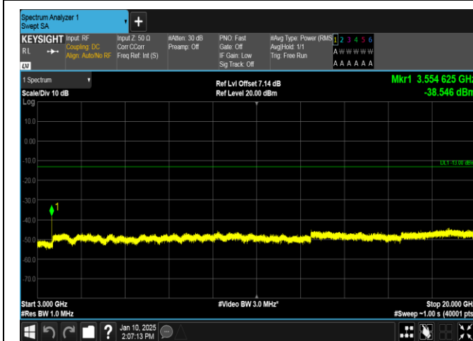
Band66-3MHz-QPSK-132657-1RB#0-3000~20000-PASS
