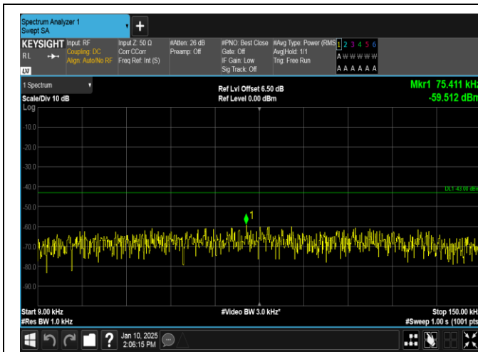
Band66-3MHz-QPSK-132657-1RB#0-0.009~0.15-PASS
