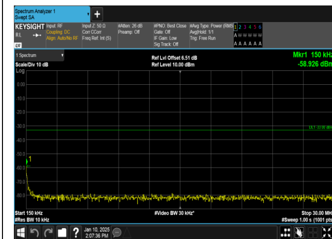
Band66-3MHz-16QAM-132657-1RB#0-0.15~30-PASS
