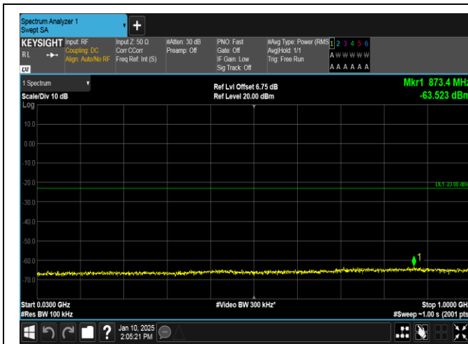
Band66-3MHz-16QAM-132322-15RB#0-30~1000-PASS
