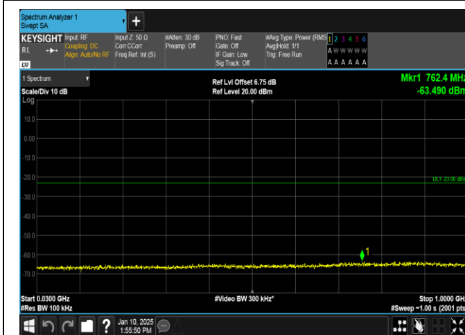
Band66-3MHz-16QAM-131987-1RB#14-30~1000-PASS
