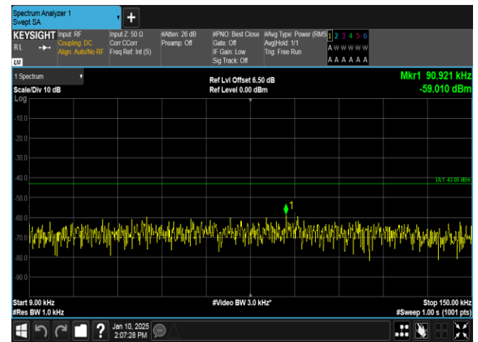
Band66-3MHz-16QAM-132657-1RB#0-0.009~0.15-PASS
