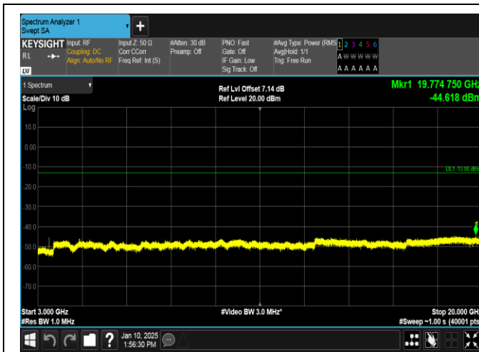
Band66-3MHz-16QAM-131987-1RB#14-3000~20000-PASS
