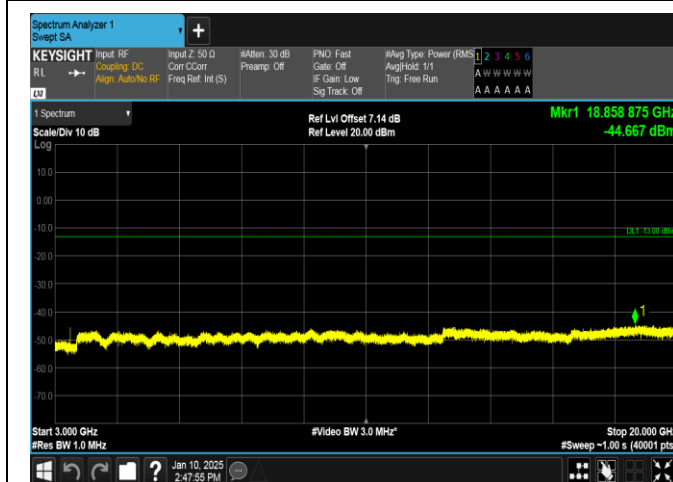
Band66-5MHz-QPSK-131997-1RB#0-3000~20000-PASS
