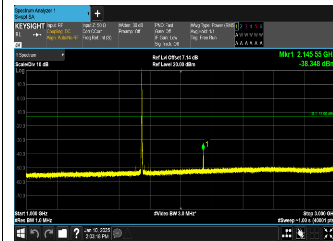
Band66-3MHz-16QAM-132322-1RB#14-1000~3000-PASS
