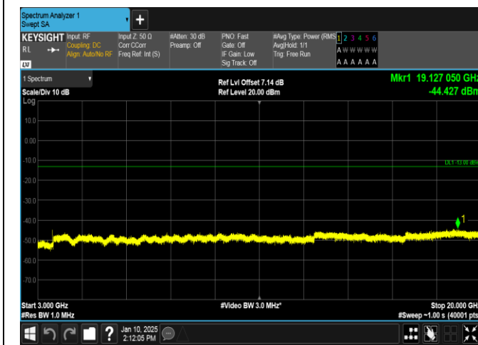
Band66-3MHz-QPSK-132657-15RB#0-3000~20000-PASS
