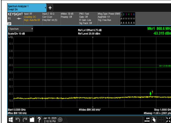
Band66-3MHz-16QAM-132657-1RB#14-30~1000-PASS
