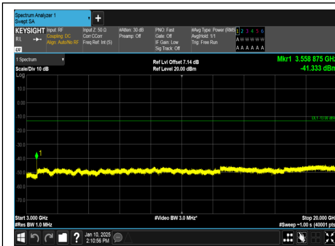
Band66-3MHz-16QAM-132657-1RB#14-3000~20000-PASS
