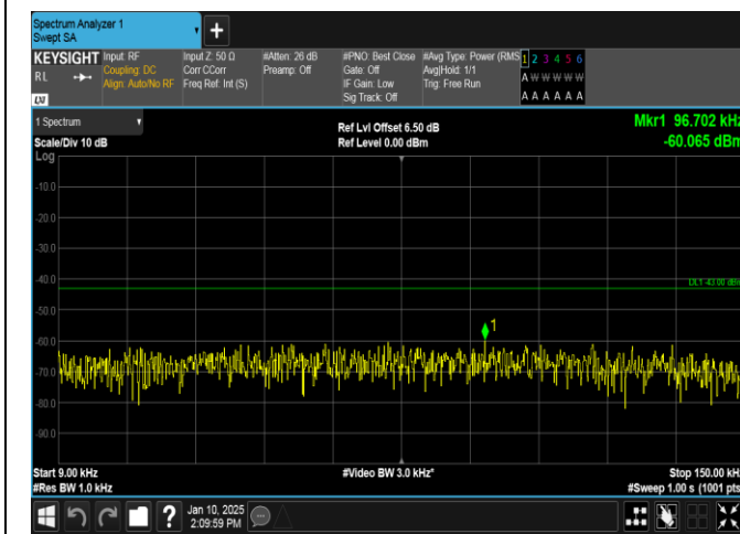
Band66-3MHz-16QAM-132657-1RB#14-0.009~0.15-PASS
