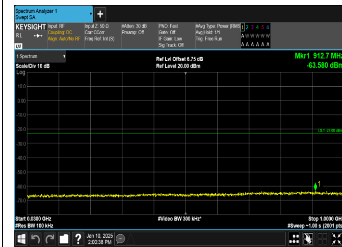
Band66-3MHz-16QAM-132322-1RB#0-30~1000-PASS
