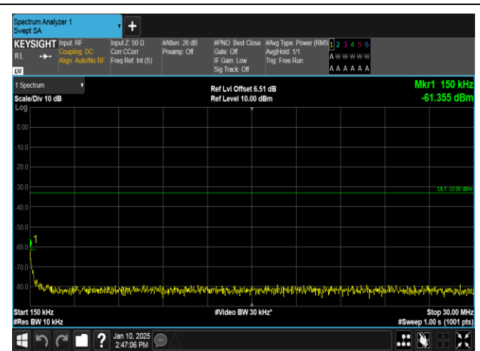
Band66-5MHz-QPSK-131997-1RB#0-0.15~30-PASS
