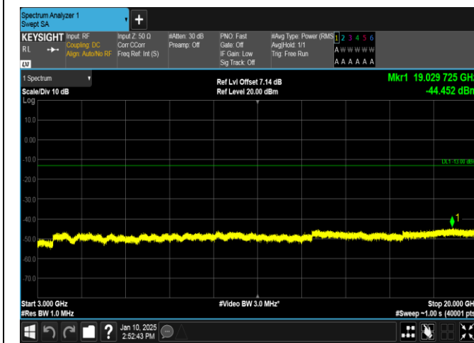
Band66-5MHz-QPSK-131997-25RB#0-3000~20000-PASS
