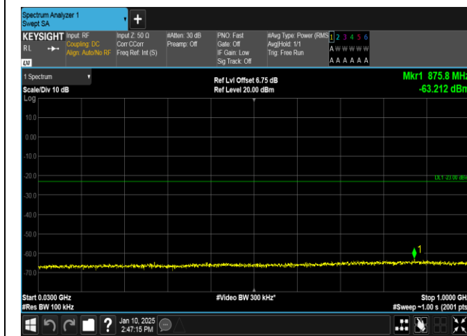
Band66-5MHz-QPSK-131997-1RB#0-30~1000-PASS
