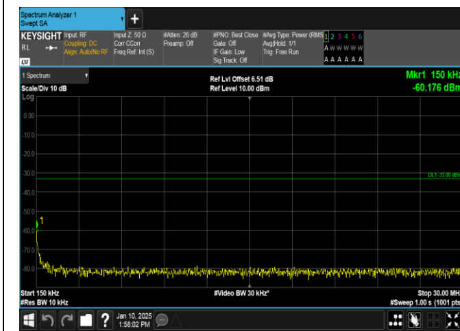
Band66-3MHz-16QAM-131987-15RB#0-0.15~30-PASS
