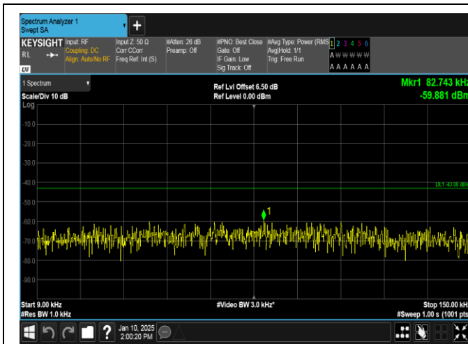
Band66-3MHz-16QAM-132322-1RB#0-0.009~0.15-PASS
