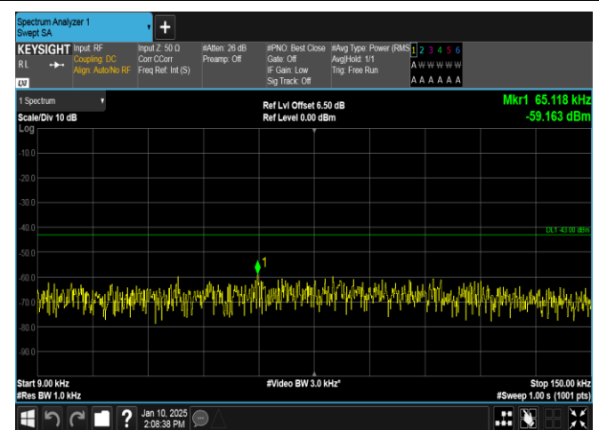
Band66-3MHz-QPSK-132657-1RB#14-0.009~0.15-PASS
