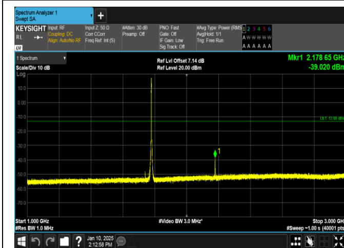
Band66-3MHz-16QAM-132657-15RB#0-1000~3000-PASS
