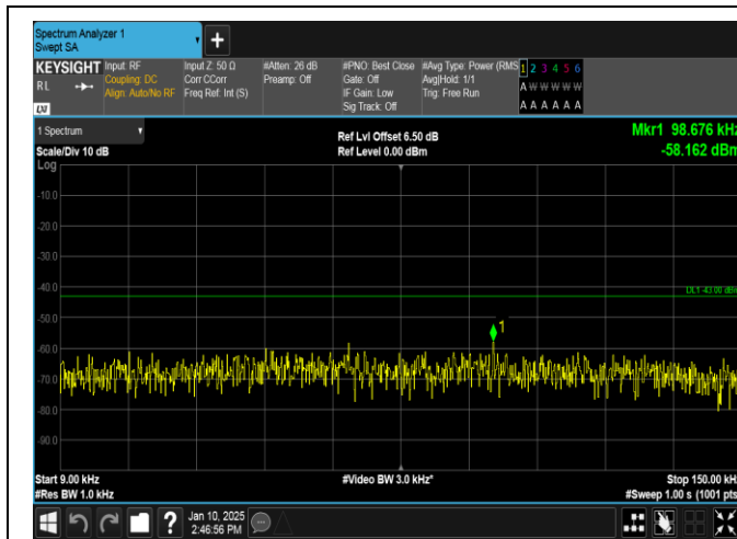
Band66-5MHz-QPSK-131997-1RB#0-0.009~0.15-PASS
