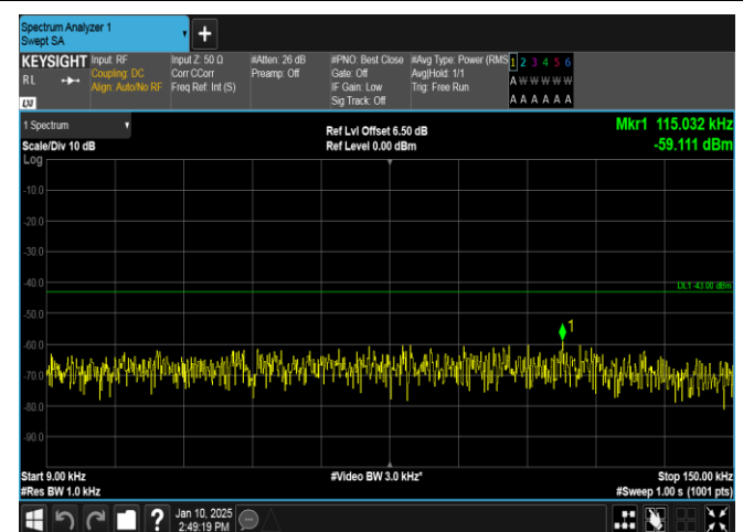
Band66-5MHz-QPSK-131997-1RB#24-0.009~0.15-PASS
