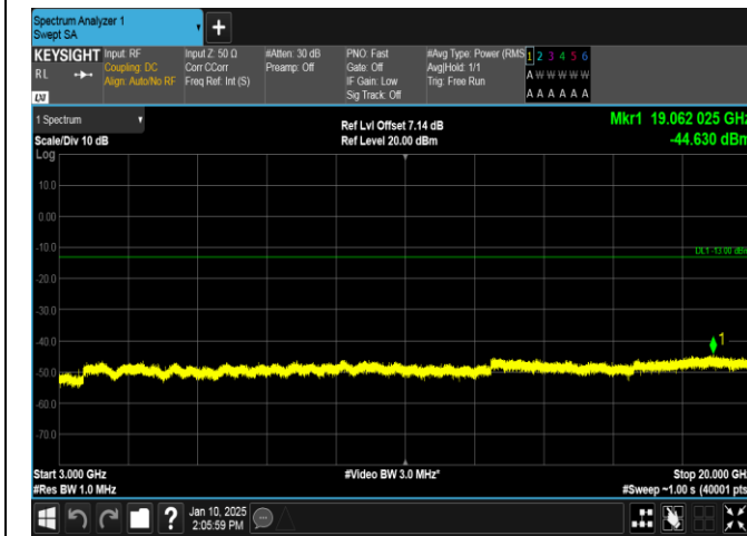
Band66-3MHz-16QAM-132322-15RB#0-3000~20000-PASS
