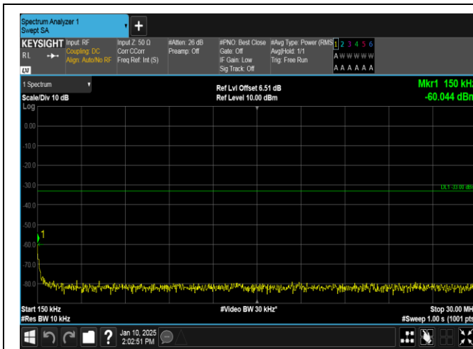
Band66-3MHz-16QAM-132322-1RB#14-0.15~30-PASS
