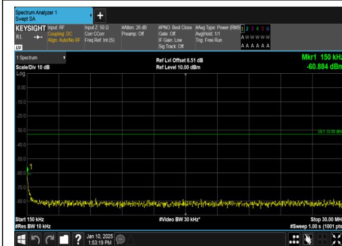
Band66-3MHz-16QAM-131987-1RB#0-0.15~30-PASS
