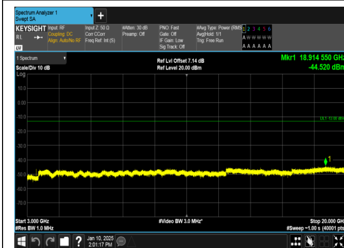
Band66-3MHz-16QAM-132322-1RB#0-3000~20000-PASS
