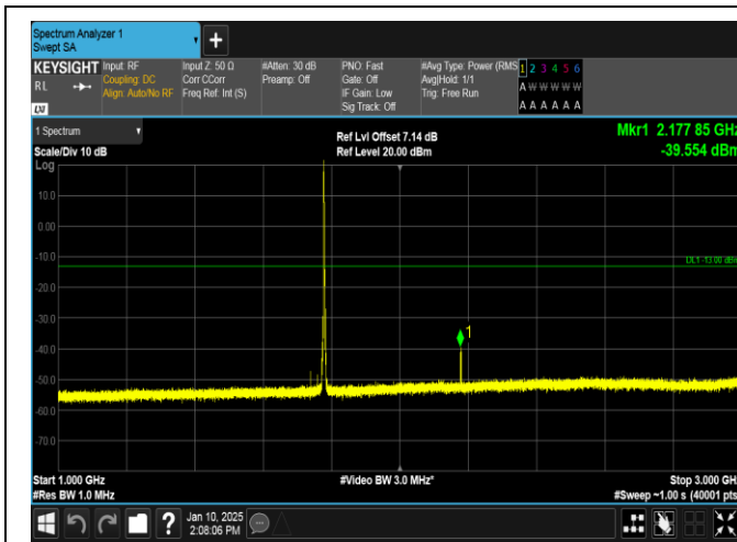
Band66-3MHz-16QAM-132657-1RB#0-1000~3000-PASS
