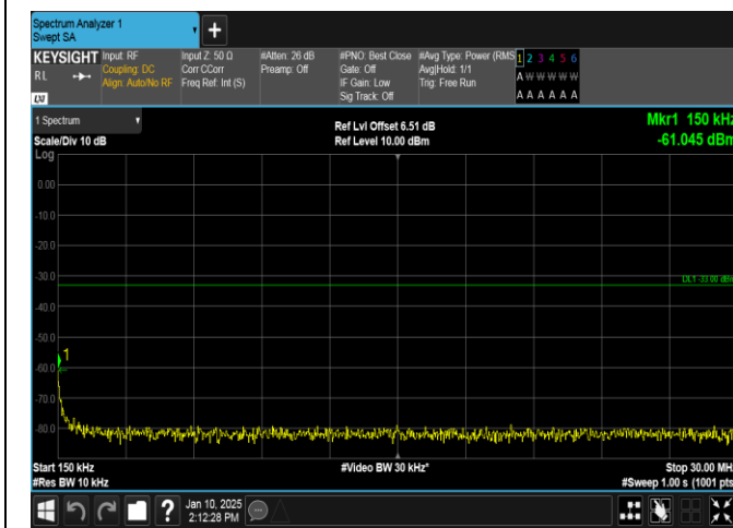
Band66-3MHz-16QAM-132657-15RB#0-0.15~30-PASS
