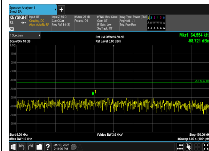
Band66-3MHz-QPSK-132657-15RB#0-0.009~0.15-PASS
