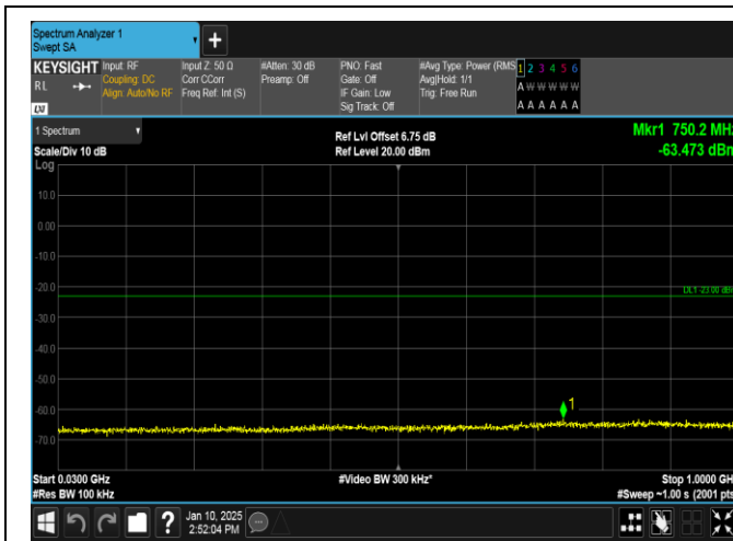
Band66-5MHz-QPSK-131997-25RB#0-30~1000-PASS
