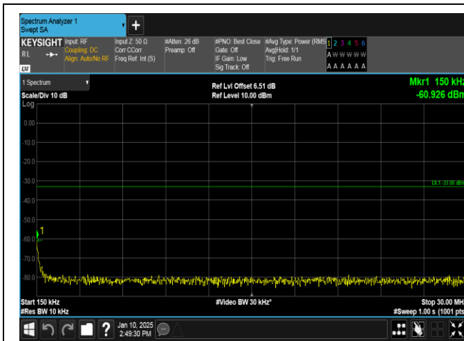
Band66-5MHz-QPSK-131997-1RB#24-0.15~30-PASS
