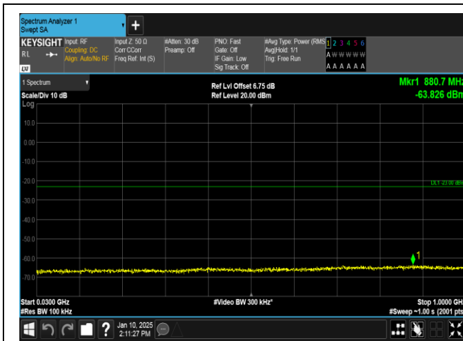
Band66-3MHz-QPSK-132657-15RB#0-30~1000-PASS
