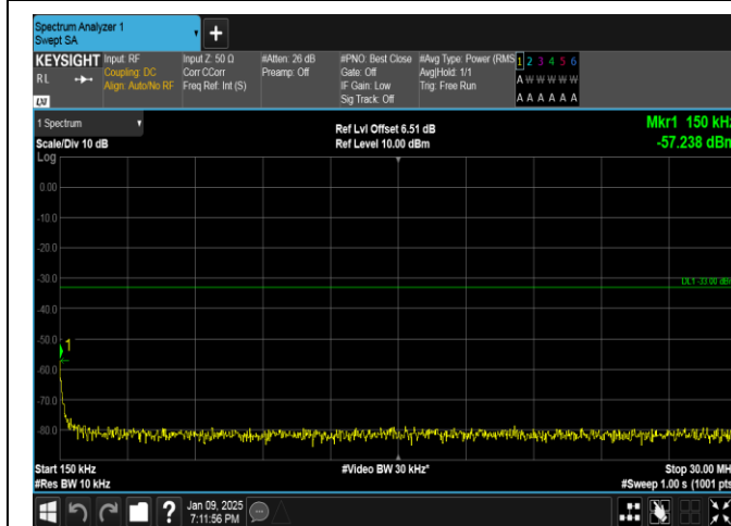
Band66-1.4MHz-16QAM-131979-1RB#0-0.15~30-PASS
