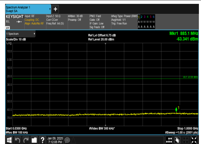
Band66-1.4MHz-16QAM-131979-1RB#0-30~1000-PASS
