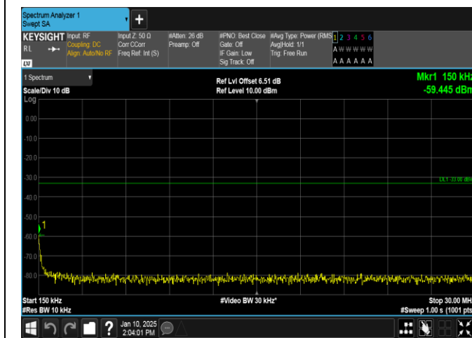
Band66-3MHz-QPSK-132322-15RB#0-0.15~30-PASS
