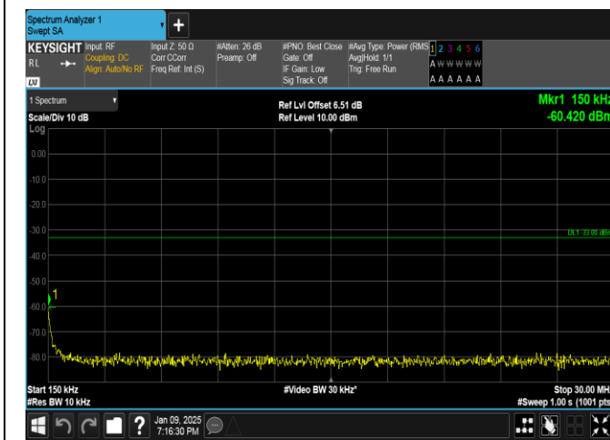
Band66-1.4MHz-16QAM-131979-6RB#0-0.15~30-PASS
