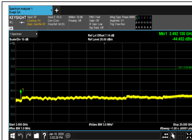
Band66-3MHz-QPSK-132322-1RB#14-3000~20000-PASS
