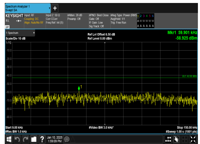
Band66-3MHz-QPSK-132322-1RB#0-0.009~0.15-PASS
