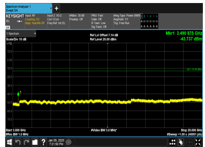
Band66-1.4MHz-16QAM-132322-1RB#5-3000~20000-PASS
