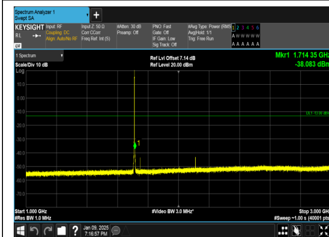
Band66-1.4MHz-16QAM-131979-6RB#0-1000~3000-PASS
