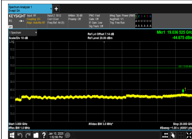
Band66-3MHz-QPSK-131987-1RB#0-3000~20000-PASS
