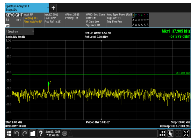
Band66-1.4MHz-16QAM-131979-1RB#0-0.009~0.15-PASS
