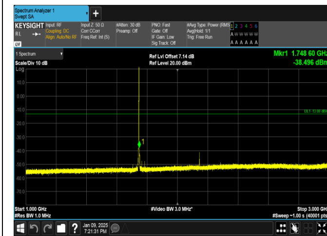
Band66-1.4MHz-16QAM-132322-1RB#5-1000~3000-PASS
