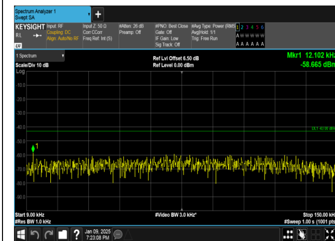
Band66-1.4MHz-16QAM-132322-6RB#0-0.009~0.15-PASS
