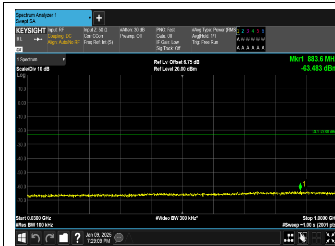
Band66-1.4MHz-QPSK-132665-6RB#0-30~1000-PASS
