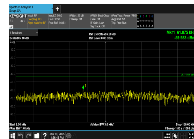
Band66-3MHz-QPSK-131987-15RB#0-0.009~0.15-PASS
