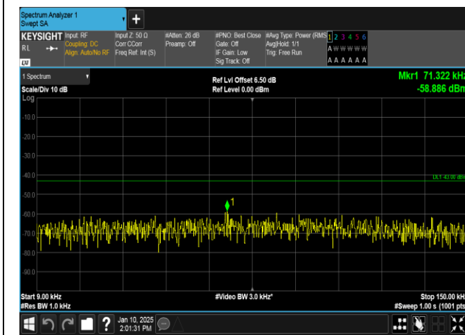
Band66-3MHz-QPSK-132322-1RB#14-0.009~0.15-PASS
