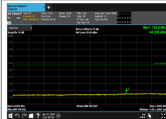
Band66-3MHz-QPSK-132322-1RB#14-30~1000-PASS
