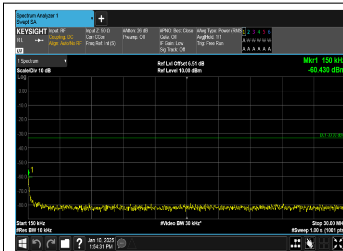
Band66-3MHz-QPSK-131987-1RB#14-0.15~30-PASS
