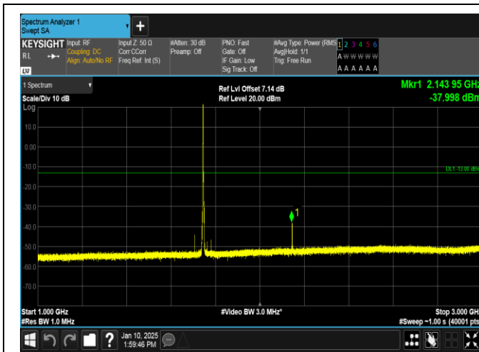
Band66-3MHz-QPSK-132322-1RB#0-1000~3000-PASS
