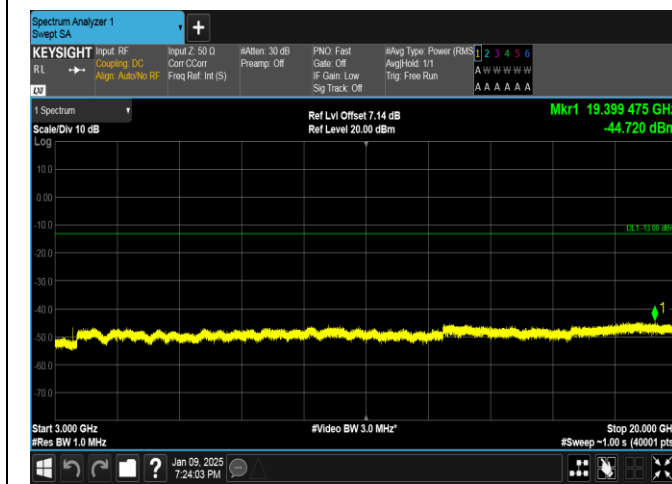
Band66-1.4MHz-16QAM-132322-6RB#0-3000~20000-PASS
