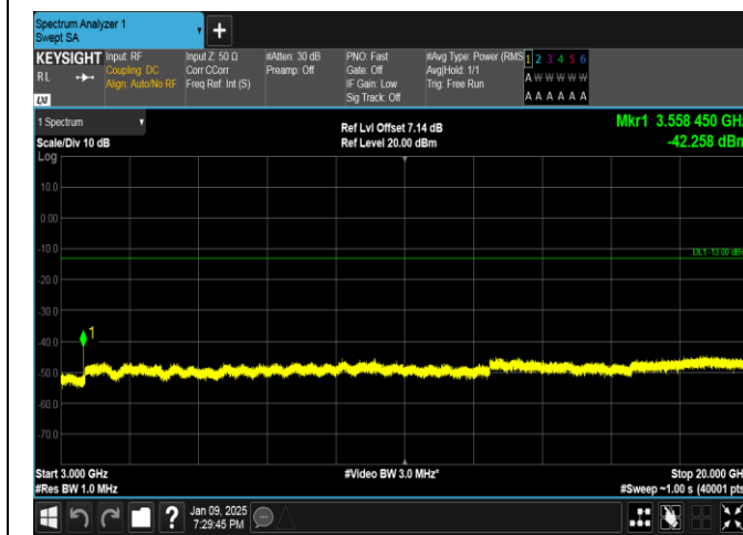
Band66-1.4MHz-QPSK-132665-6RB#0-3000~20000-PASS
