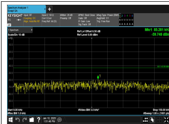
Band66-3MHz-QPSK-131987-1RB#0-0.009~0.15-PASS
