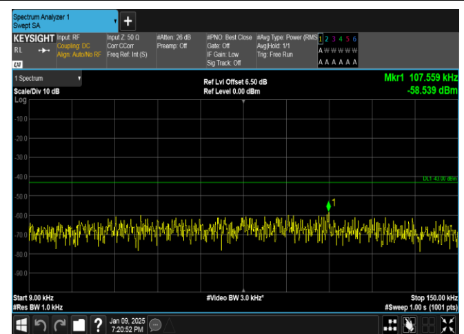
Band66-1.4MHz-16QAM-132322-1RB#5-0.009~0.15-PASS
