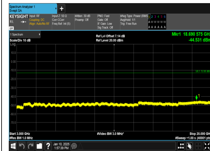
Band66-3MHz-QPSK-131987-15RB#0-3000~20000-PASS
