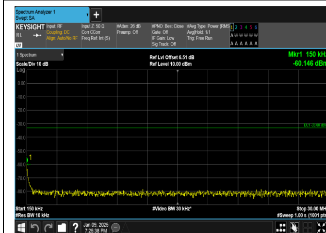
Band66-1.4MHz-16QAM-132665-1RB#0-0.15~30-PASS
