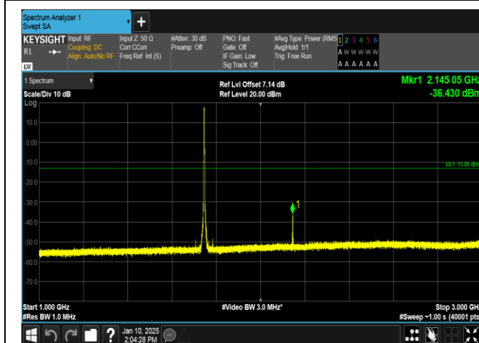
Band66-3MHz-QPSK-132322-15RB#0-1000~3000-PASS
