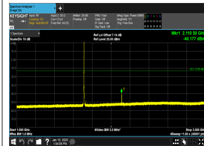
Band66-3MHz-QPSK-131987-1RB#14-1000~3000-PASS
