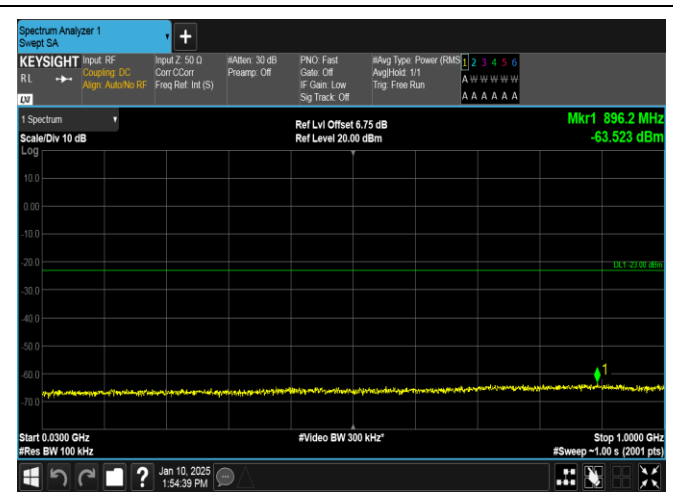
Band66-3MHz-QPSK-131987-1RB#14-30~1000-PASS
