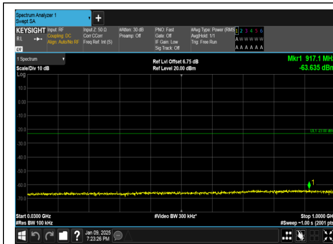
Band66-1.4MHz-16QAM-132322-6RB#0-30~1000-PASS
