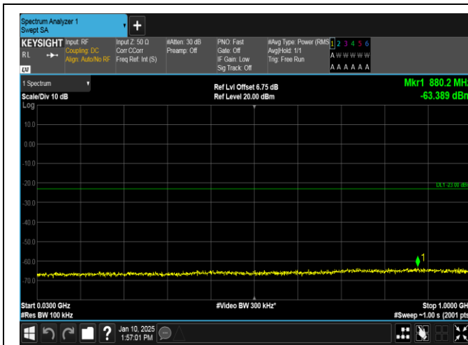
Band66-3MHz-QPSK-131987-15RB#0-30~1000-PASS
