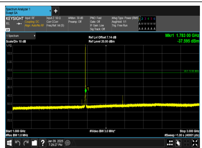
Band66-1.4MHz-QPSK-132665-6RB#0-1000~3000-PASS
