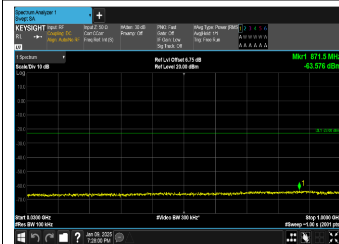
Band66-1.4MHz-16QAM-132665-1RB#5-30~1000-PASS
