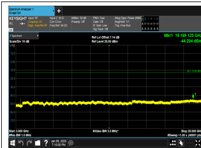
Band66-1.4MHz-16QAM-131979-1RB#5-3000~20000-PASS
