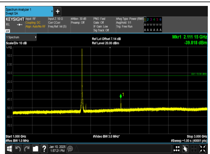
Band66-3MHz-QPSK-131987-15RB#0-1000~3000-PASS
