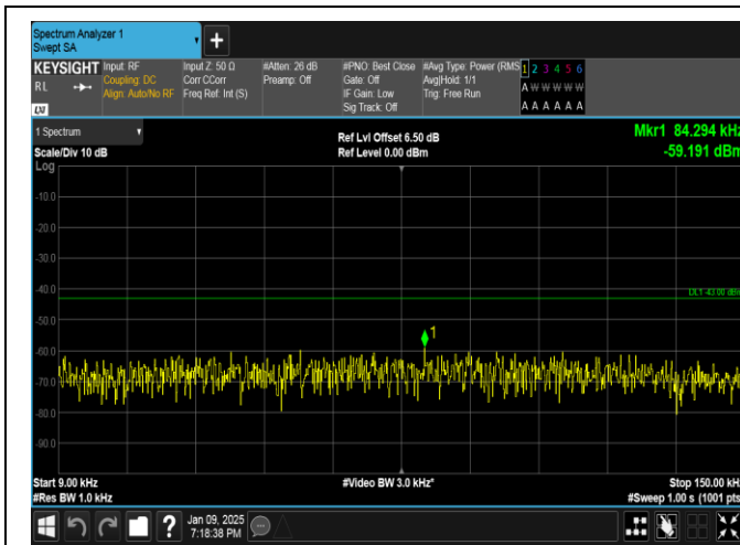
Band66-1.4MHz-16QAM-132322-1RB#0-0.009~0.15-PASS
