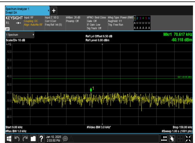
Band66-3MHz-QPSK-132322-15RB#0-0.009~0.15-PASS
