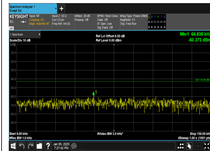
Band66-1.4MHz-16QAM-132665-1RB#5-0.009~0.15-PASS
