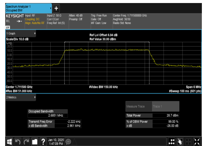
Band66-3MHz-16QAM-131987-15RB#0-PASS
