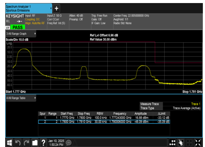
Band66-3MHz-16QAM-132657-1RB#0-PASS
