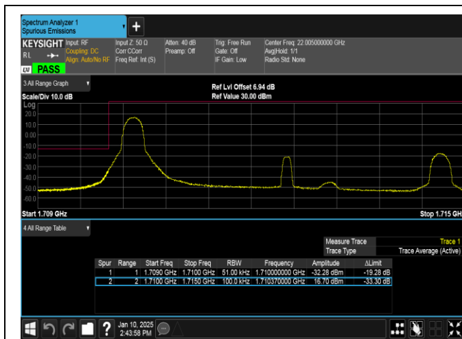
Band66-5MHz-16QAM-131997-1RB#0-PASS
