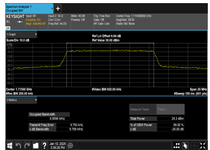
Band66-10MHz-16QAM-132022-50RB#0-PASS
