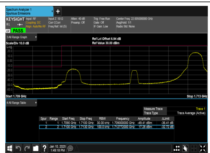
Band66-3MHz-16QAM-131987-1RB#14-PASS
