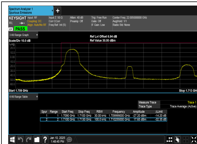
Band66-3MHz-16QAM-131987-1RB#0-PASS
