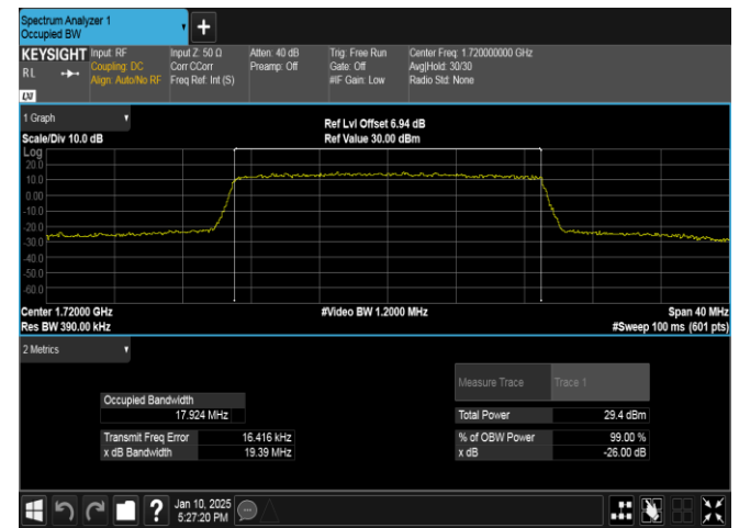
Band66-20MHz-16QAM-132072-100RB#0-PASS
