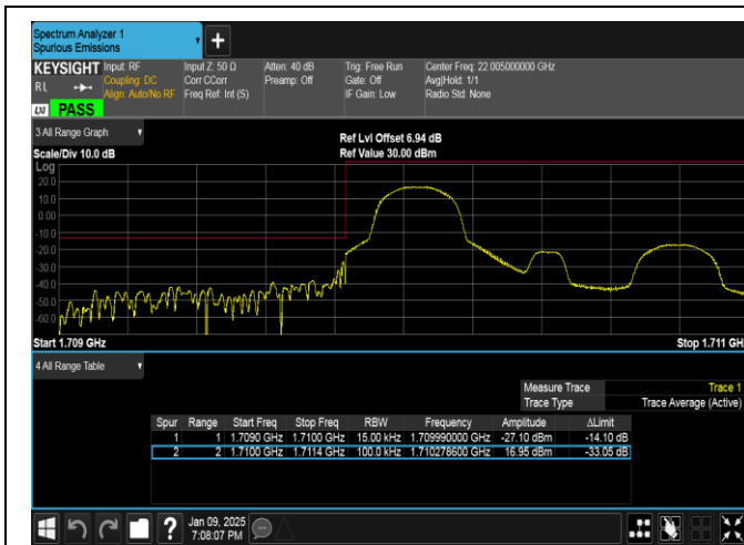
Band66-1.4MHz-16QAM-131979-1RB#0-PASS
