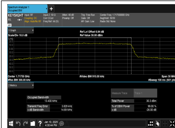
Band66-15MHz-QPSK-132047-75RB#0-PASS
