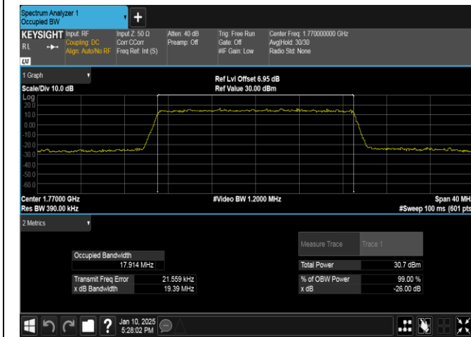
Band66-20MHz-QPSK-132572-100RB#0-PASS
