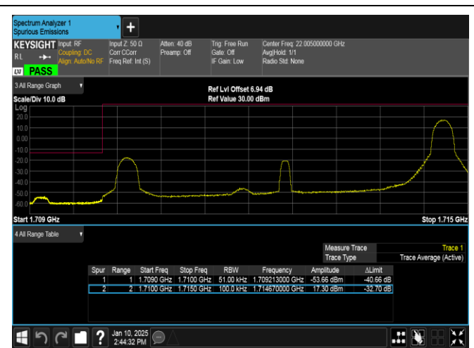
Band66-5MHz-16QAM-131997-1RB#24-PASS
