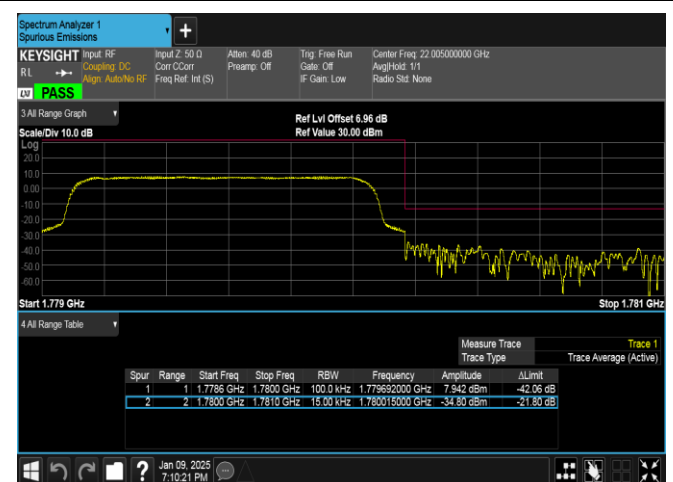
Band66-1.4MHz-16QAM-132665-6RB#0-PASS
