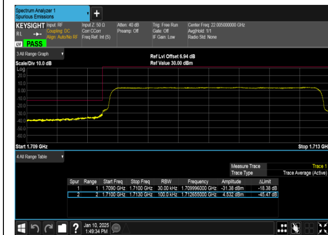
Band66-3MHz-QPSK-131987-15RB#0-PASS
