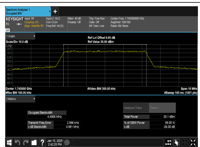
Band66-5MHz-QPSK-132322-25RB#0-PASS
