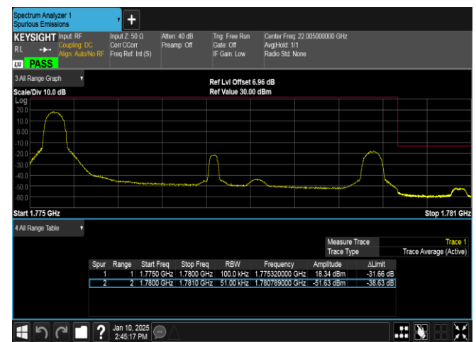
Band66-5MHz-QPSK-132647-1RB#0-PASS
