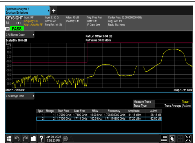
Band66-1.4MHz-16QAM-131979-1RB#5-PASS
