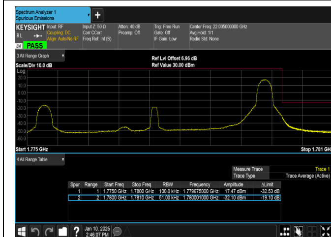
Band66-5MHz-16QAM-132647-1RB#24-PASS
