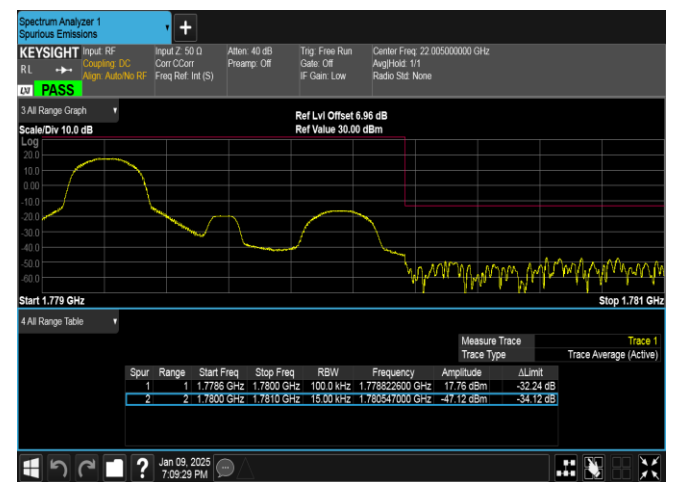
Band66-1.4MHz-16QAM-132665-1RB#0-PASS
