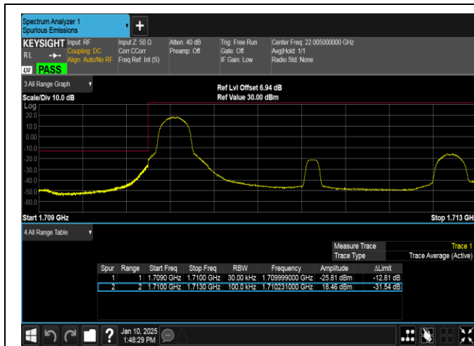
Band66-3MHz-QPSK-131987-1RB#0-PASS
