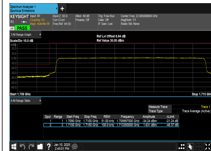
Band66-5MHz-16QAM-131997-25RB#0-PASS
