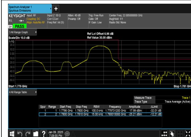
Band66-1.4MHz-16QAM-132665-1RB#5-PASS
