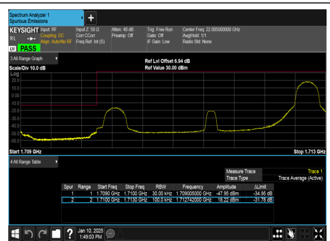
Band66-3MHz-QPSK-131987-1RB#14-PASS
