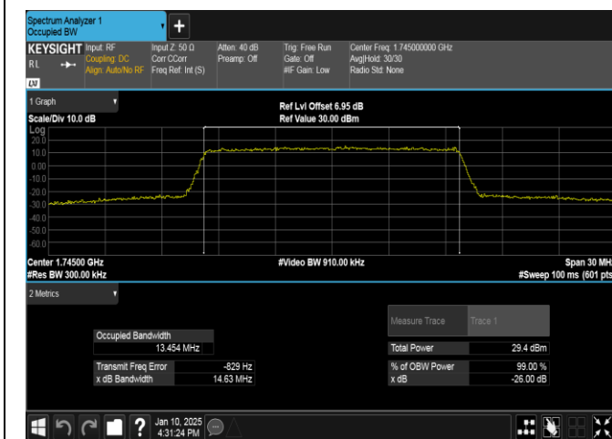
Band66-15MHz-16QAM-132322-75RB#0-PASS
