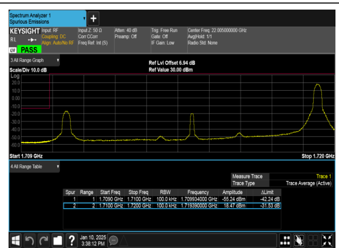
Band66-10MHz-QPSK-132022-1RB#49-PASS
