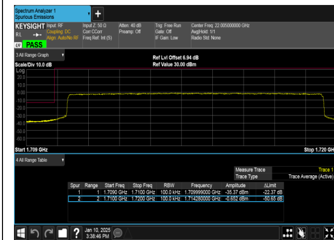
Band66-10MHz-QPSK-132022-50RB#0-PASS
