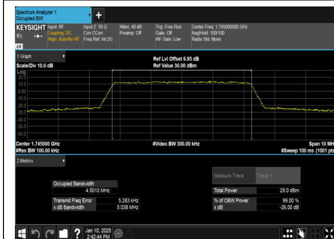
Band66-5MHz-16QAM-132322-25RB#0-PASS
