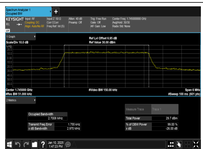
Band66-3MHz-QPSK-132322-15RB#0-PASS
