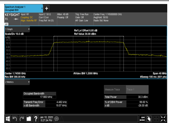
Band66-20MHz-QPSK-132322-100RB#0-PASS
