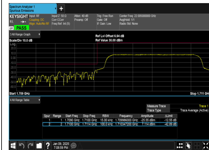
Band66-1.4MHz-16QAM-131979-6RB#0-PASS
