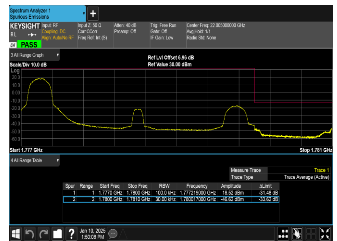
Band66-3MHz-QPSK-132657-1RB#0-PASS
