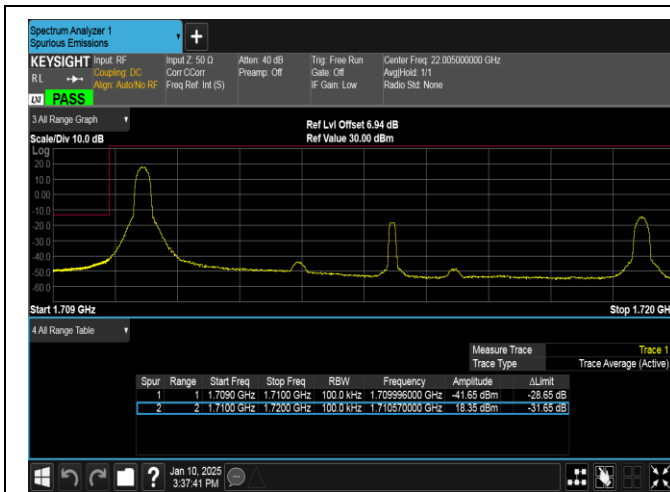
Band66-10MHz-QPSK-132022-1RB#0-PASS
