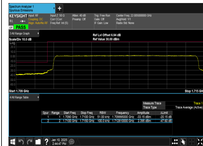
Band66-5MHz-QPSK-131997-25RB#0-PASS
