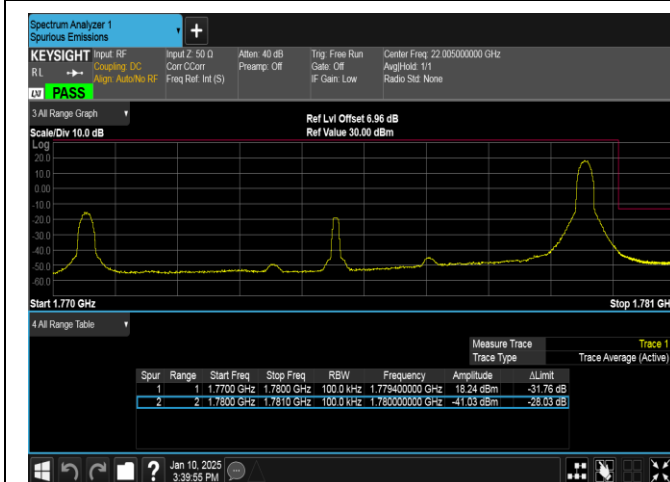
Band66-10MHz-QPSK-132622-1RB#49-PASS
