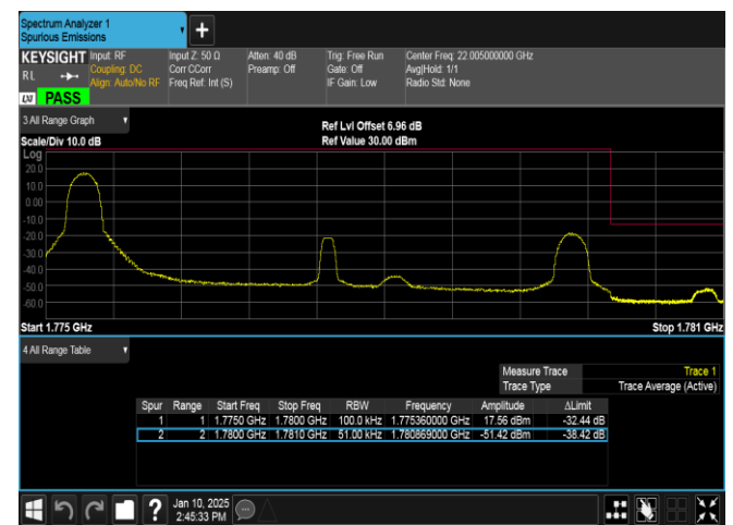
Band66-5MHz-16QAM-132647-1RB#0-PASS
