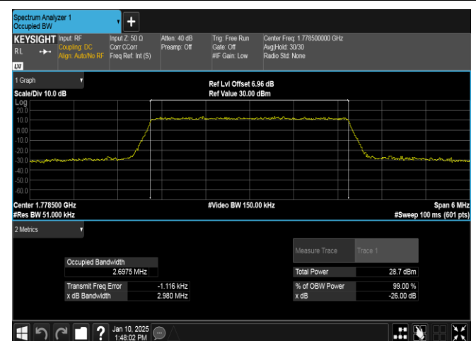
Band66-3MHz-16QAM-132657-15RB#0-PASS
