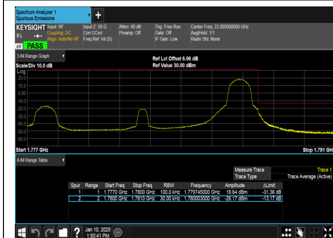
Band66-3MHz-QPSK-132657-1RB#14-PASS
