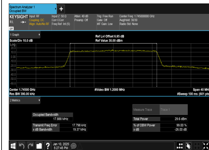
Band66-20MHz-16QAM-132322-100RB#0-PASS
