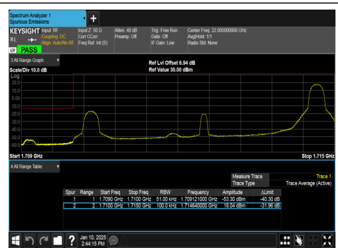
Band66-5MHz-QPSK-131997-1RB#24-PASS
