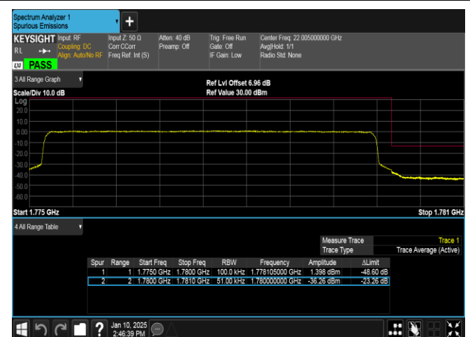
Band66-5MHz-16QAM-132647-25RB#0-PASS
