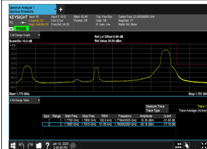
Band66-5MHz-QPSK-132647-1RB#24-PASS
