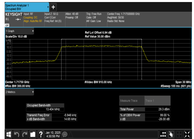
Band66-15MHz-16QAM-132047-75RB#0-PASS
