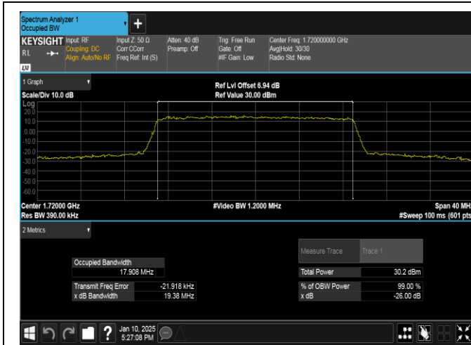
Band66-20MHz-QPSK-132072-100RB#0-PASS
