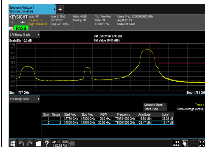
Band66-3MHz-16QAM-132657-1RB#14-PASS
