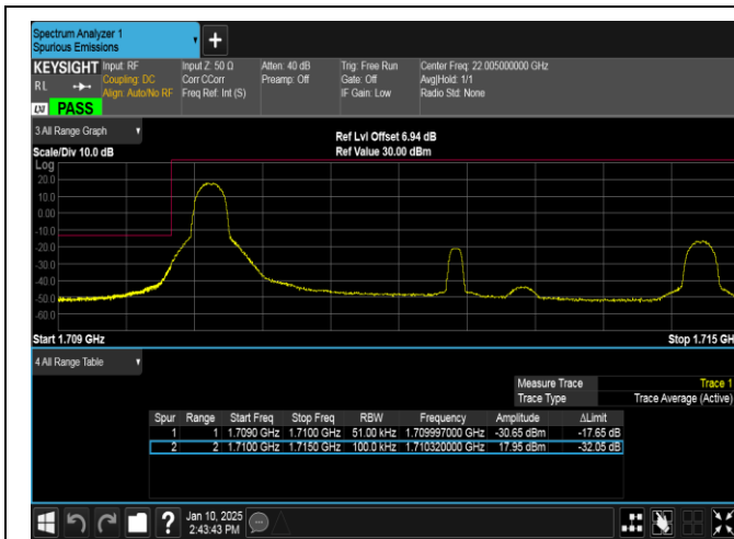
Band66-5MHz-QPSK-131997-1RB#0-PASS
