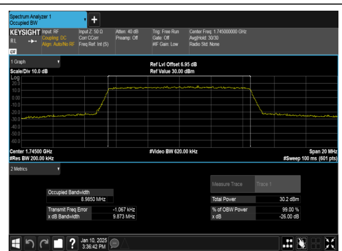
Band66-10MHz-QPSK-132322-50RB#0-PASS
