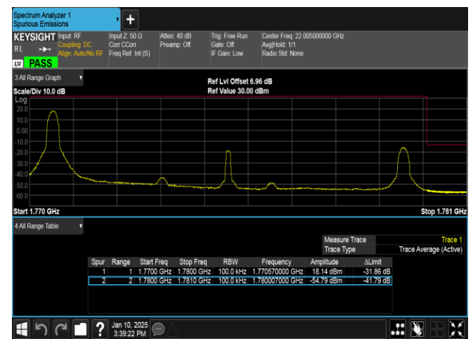
Band66-10MHz-QPSK-132622-1RB#0-PASS
