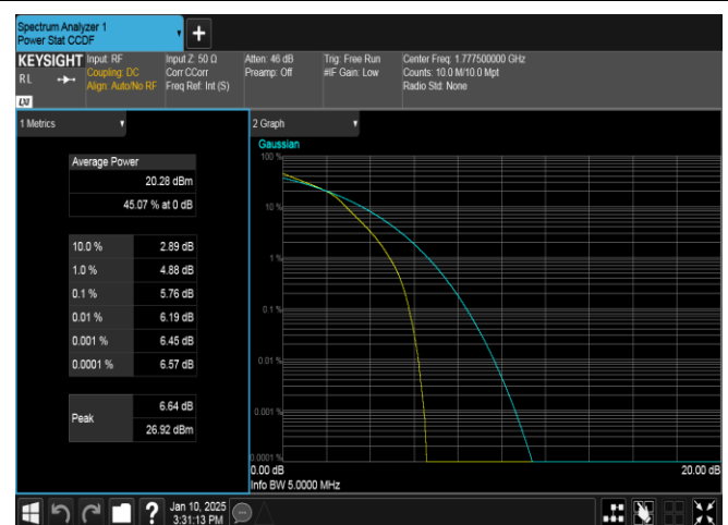
Band66-5MHz-16QAM-132647-25RB#0-PASS
