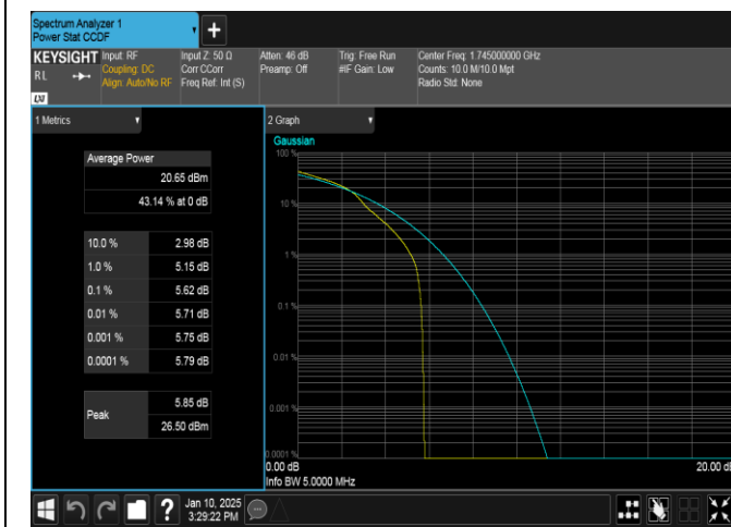
Band66-5MHz-16QAM-132322-1RB#0-PASS
