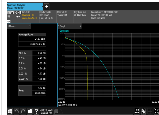
Band66-5MHz-QPSK-132322-1RB#0-PASS
