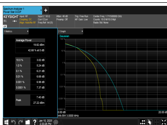
Band66-3MHz-16QAM-131987-15RB#0-PASS
