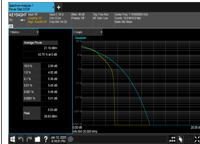
Band66-20MHz-16QAM-132322-1RB#0-PASS
