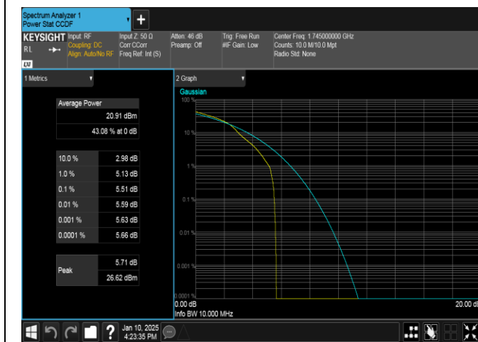
Band66-10MHz-16QAM-132322-1RB#0-PASS
