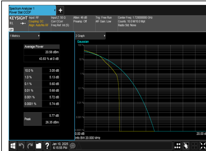
Band66-20MHz-16QAM-132072-1RB#0-PASS
