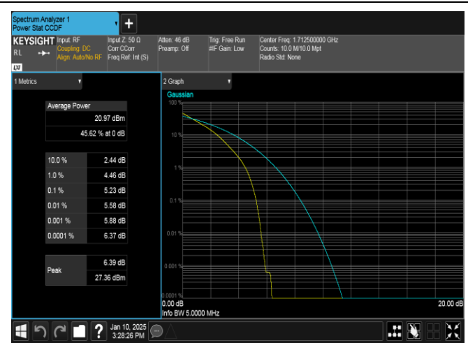
Band66-5MHz-QPSK-131997-25RB#0-PASS
