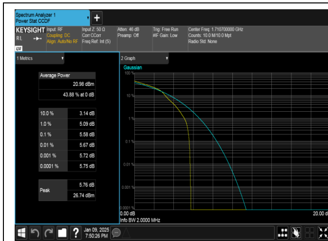
Band66-1.4MHz-16QAM-131979-1RB#0-PASS
