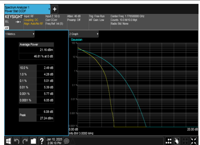
Band66-3MHz-QPSK-132657-15RB#0-PASS
