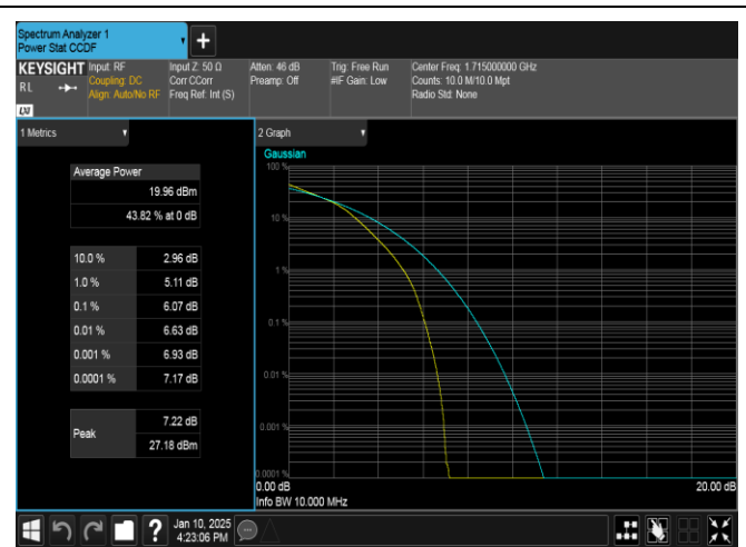
Band66-10MHz-16QAM-132022-50RB#0-PASS
