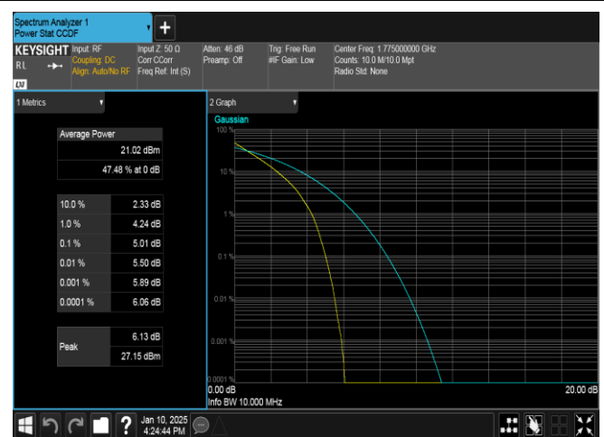
Band66-10MHz-QPSK-132622-50RB#0-PASS
