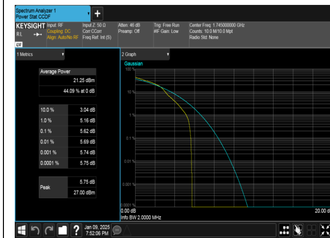
Band66-1.4MHz-16QAM-132322-1RB#0-PASS
