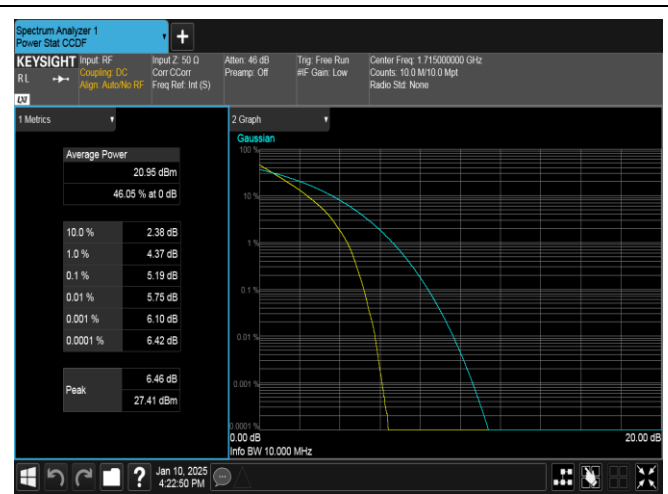
Band66-10MHz-QPSK-132022-50RB#0-PASS
