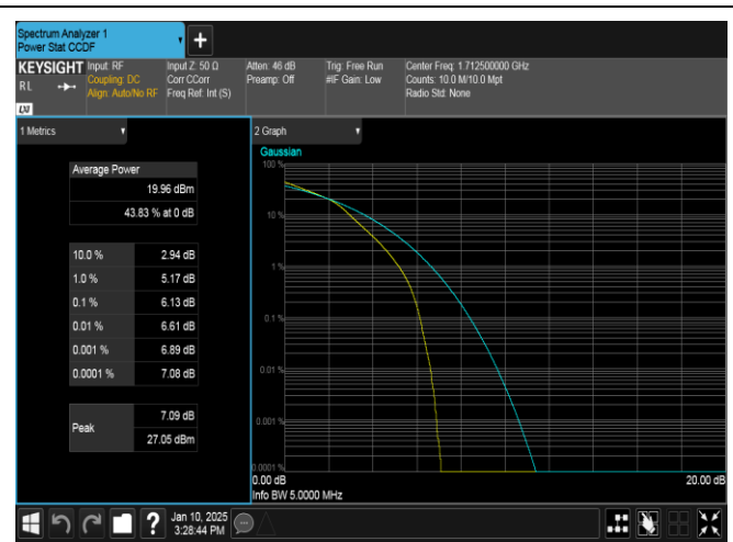
Band66-5MHz-16QAM-131997-25RB#0-PASS
