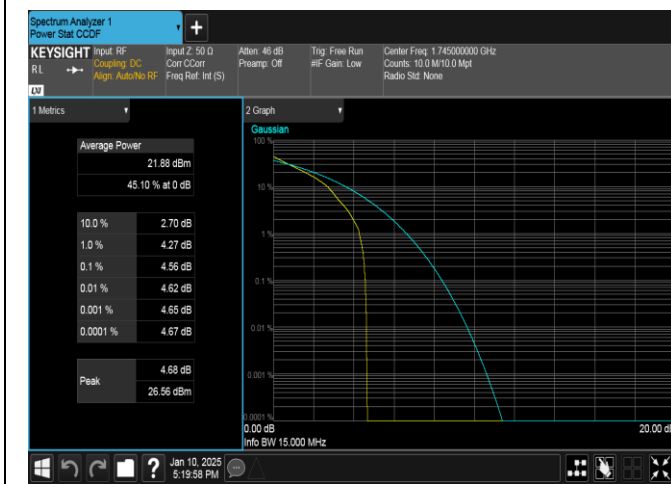
Band66-15MHz-QPSK-132322-1RB#0-PASS
