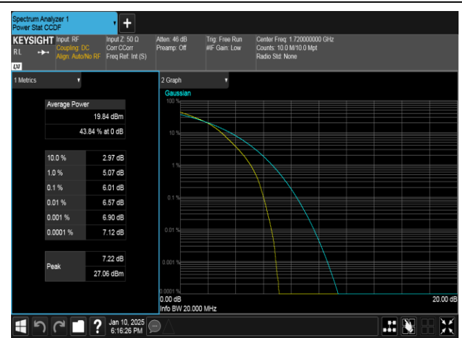
Band66-20MHz-16QAM-132072-100RB#0-PASS
