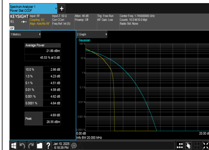
Band66-20MHz-QPSK-132322-1RB#0-PASS
