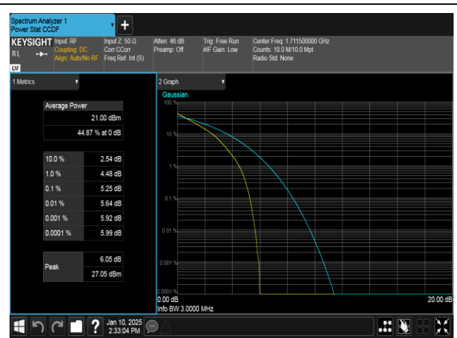
Band66-3MHz-QPSK-131987-15RB#0-PASS
