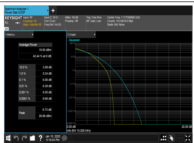
Band66-15MHz-16QAM-132047-75RB#0-PASS
