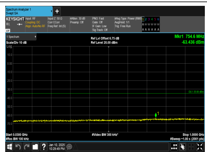
Band41-20MHz-16QAM-41490-100RB#0-30~1000-PASS
