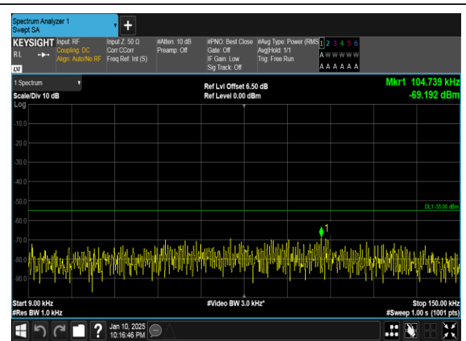
Band41-20MHz-QPSK-40620-1RB#0-0.009~0.15-PASS
