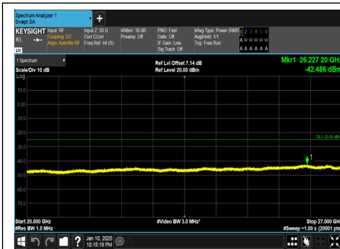
Band41-20MHz-QPSK-39750-100RB#0-20000~27000-PASS
