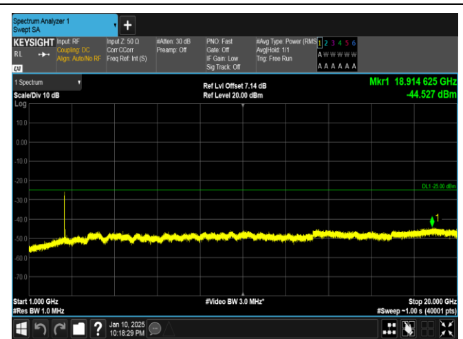
Band41-20MHz-16QAM-40620-1RB#0-1000~20000-PASS
