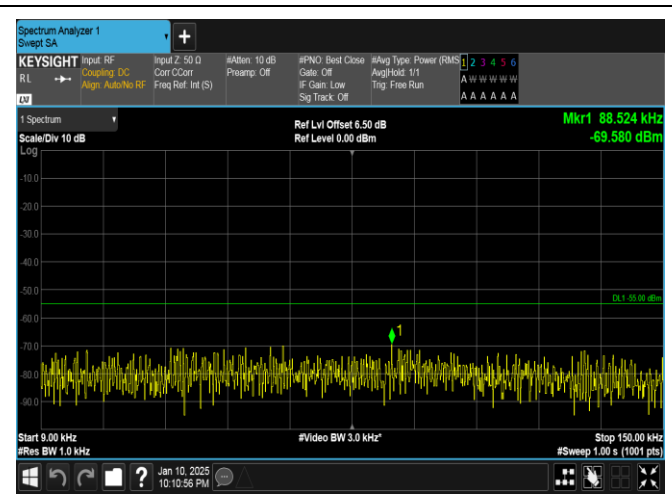
Band41-20MHz-16QAM-39750-1RB#0-0.009~0.15-PASS
