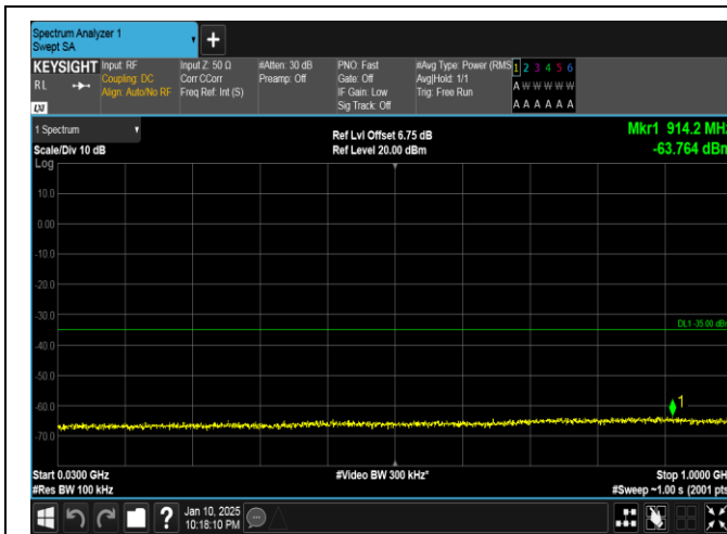
Band41-20MHz-16QAM-40620-1RB#0-30~1000-PASS
