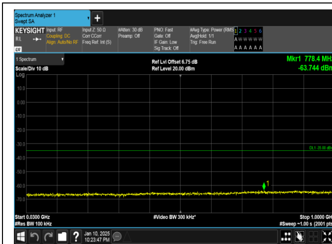
Band41-20MHz-QPSK-41490-1RB#0-30~1000-PASS
