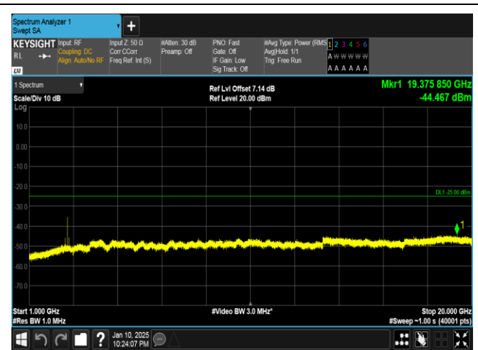
Band41-20MHz-QPSK-41490-1RB#0-1000~20000-PASS
