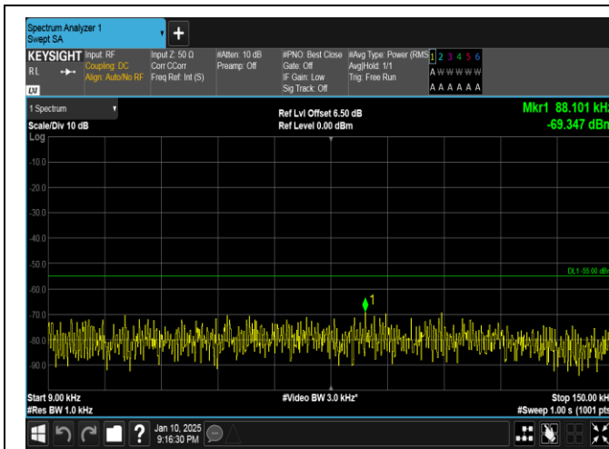
Band41-15MHz-16QAM-41515-1RB#74-0.009~0.15-PASS
