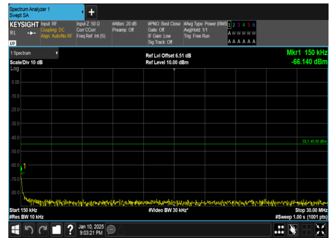
Band41-15MHz-16QAM-39725-1RB#74-0.15~30-PASS
