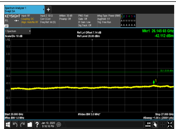
Band41-15MHz-QPSK-41515-1RB#74-20000~27000-PASS
