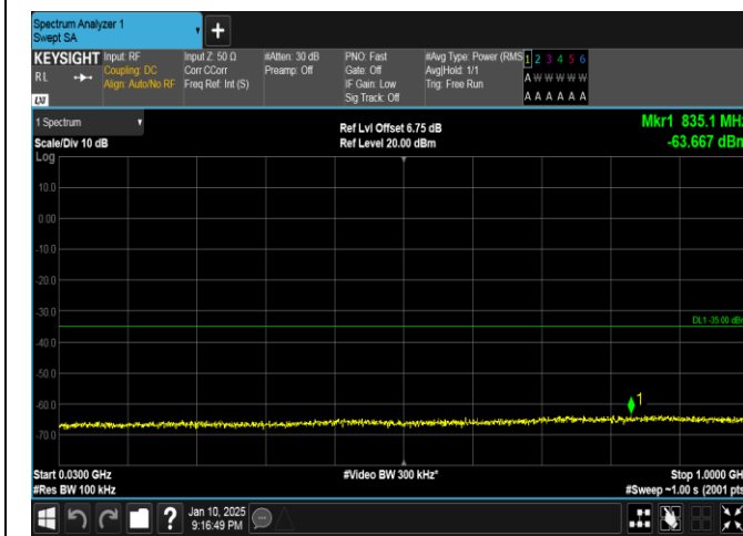
Band41-15MHz-16QAM-41515-1RB#74-30~1000-PASS
