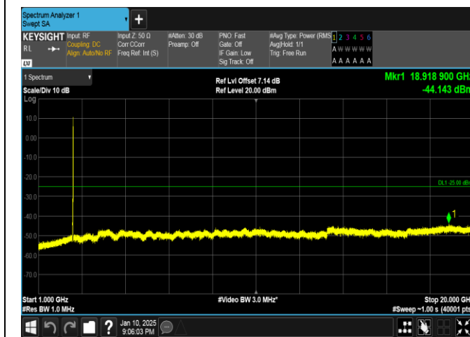
Band41-15MHz-16QAM-39725-75RB#0-1000~20000-PASS
