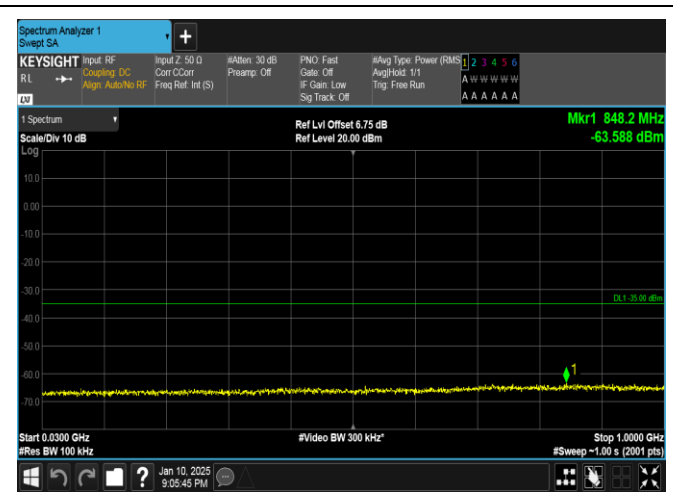
Band41-15MHz-16QAM-39725-75RB#0-30~1000-PASS
