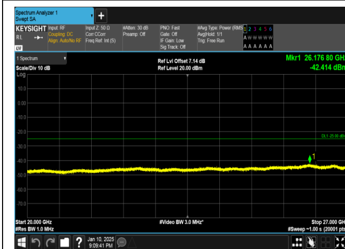
Band41-15MHz-QPSK-40620-1RB#74-20000~27000-PASS
