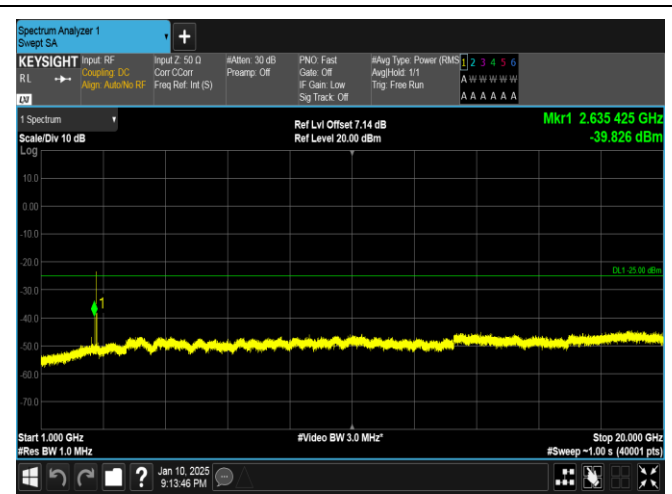
Band41-15MHz-QPSK-41515-1RB#0-1000~20000-PASS
