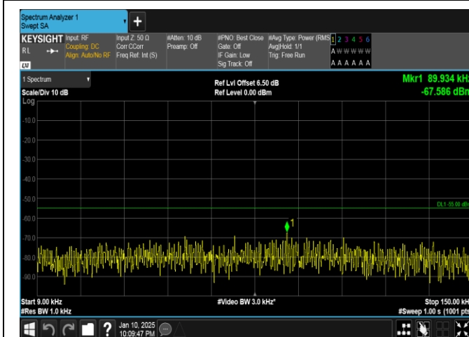
Band41-20MHz-QPSK-39750-1RB#0-0.009~0.15-PASS
