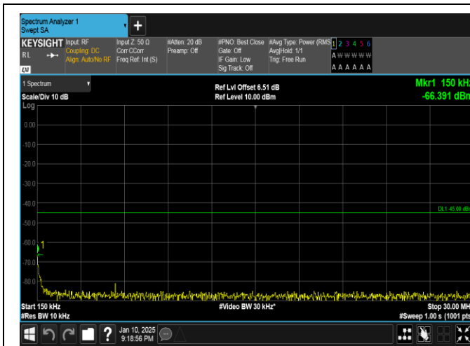
Band41-15MHz-16QAM-41515-75RB#0-0.15~30-PASS
