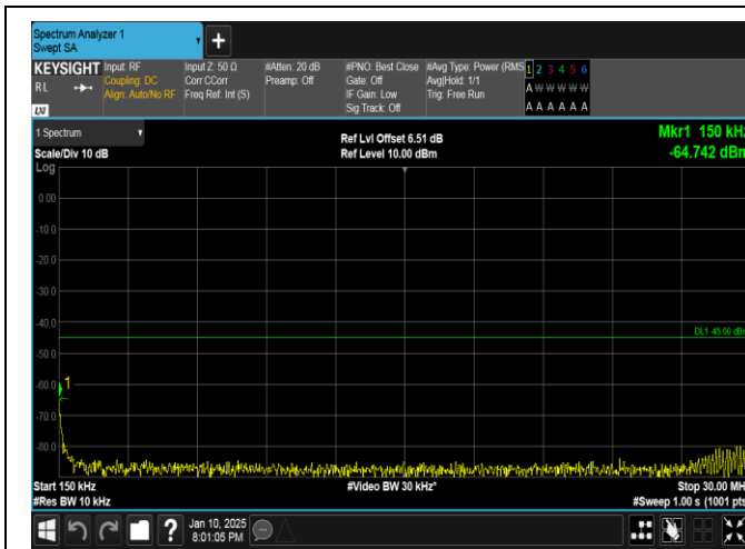
Band41-10MHz-QPSK-40620-50RB#0-0.15~30-PASS
