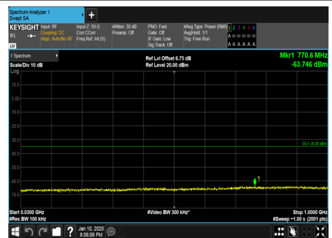
Band41-10MHz-QPSK-41540-1RB#49-30~1000-PASS
