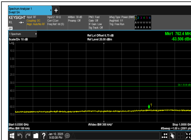
Band41-15MHz-QPSK-39725-1RB#0-30~1000-PASS
