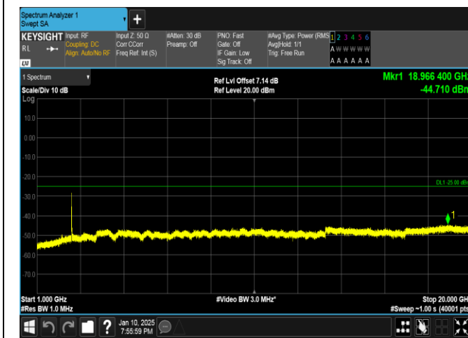
Band41-10MHz-16QAM-39700-50RB#0-1000~20000-PASS
