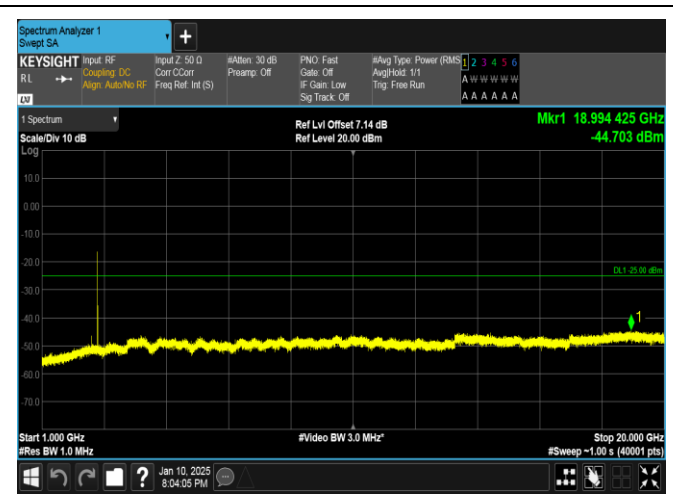
Band41-10MHz-QPSK-41540-1RB#0-1000~20000-PASS
