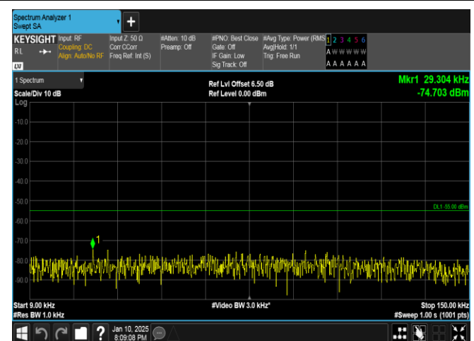
Band41-10MHz-16QAM-41540-50RB#0-0.009~0.15-PASS
