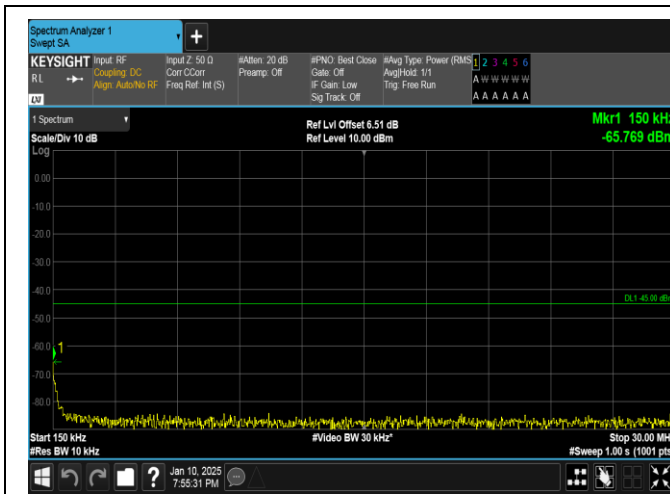
Band41-10MHz-16QAM-39700-50RB#0-0.15~30-PASS
