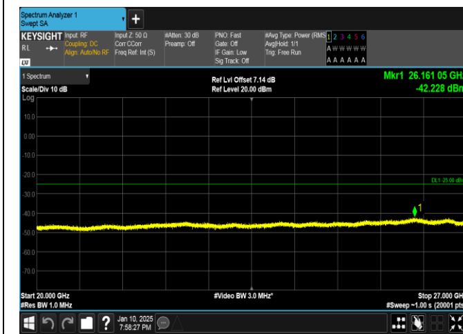
Band41-10MHz-16QAM-40620-1RB#0-20000~27000-PASS
