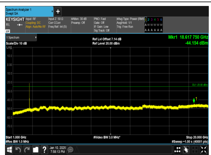
Band41-10MHz-16QAM-40620-1RB#0-1000~20000-PASS
