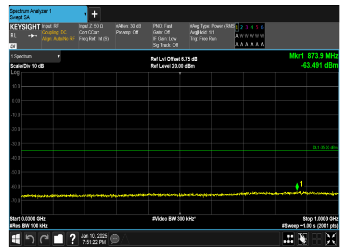
Band41-10MHz-16QAM-39700-1RB#0-30~1000-PASS
