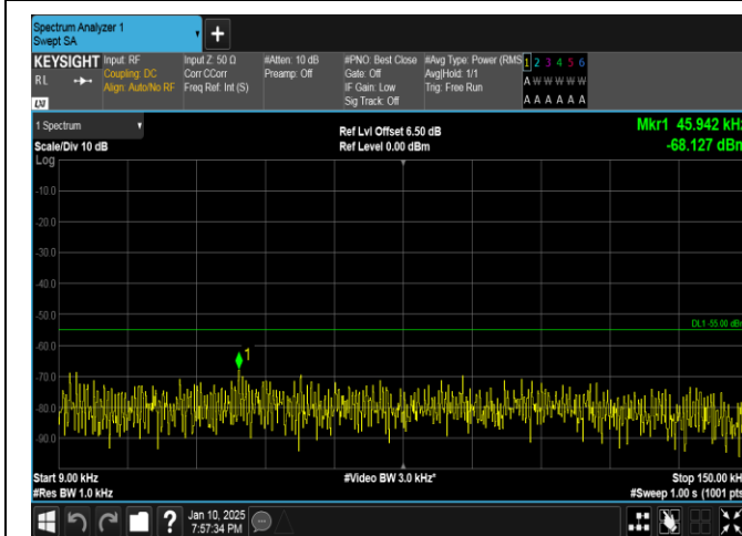
Band41-10MHz-16QAM-40620-1RB#0-0.009~0.15-PASS
