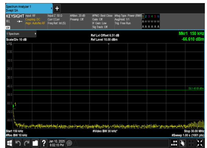
Band41-10MHz-16QAM-40620-50RB#0-0.15~30-PASS
