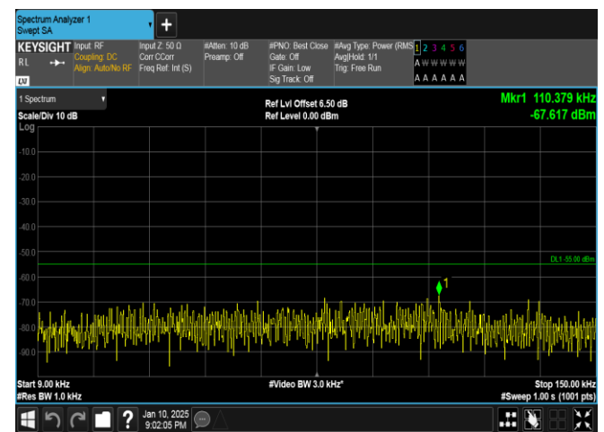
Band41-15MHz-QPSK-39725-1RB#74-0.009~0.15-PASS
