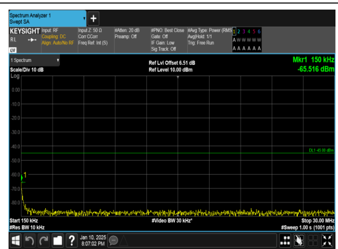
Band41-10MHz-16QAM-41540-1RB#49-0.15~30-PASS
