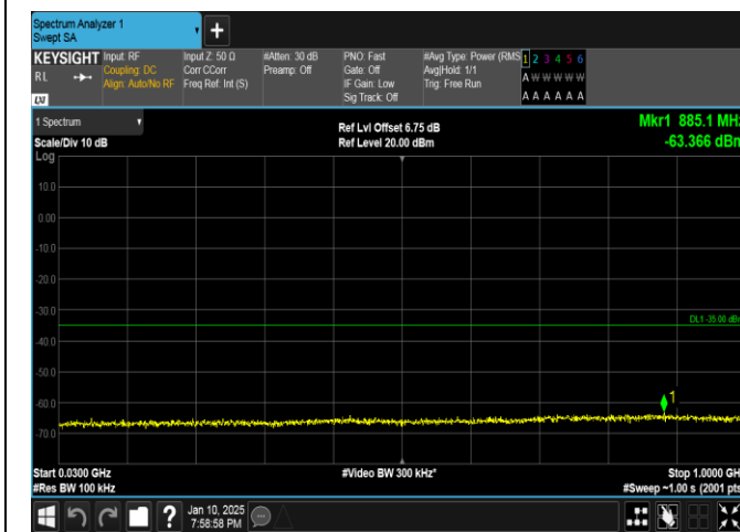
Band41-10MHz-QPSK-40620-1RB#49-30~1000-PASS
