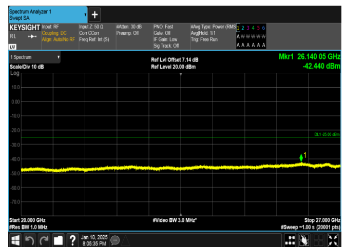
Band41-10MHz-16QAM-41540-1RB#0-20000~27000-PASS
