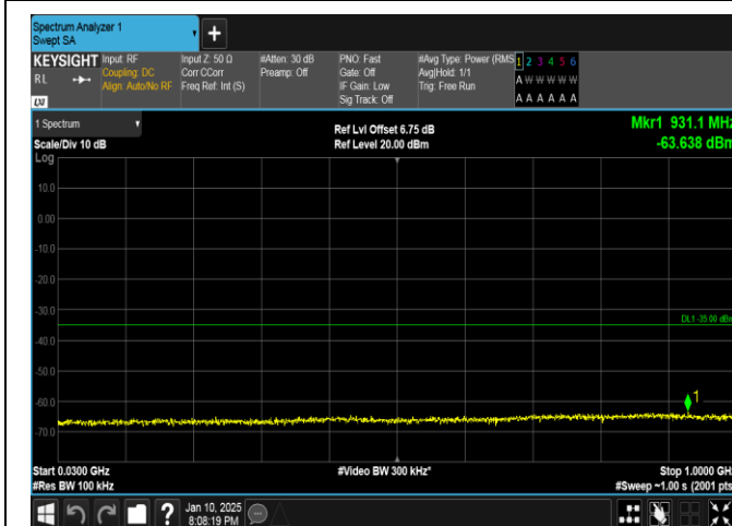
Band41-10MHz-QPSK-41540-50RB#0-30~1000-PASS
