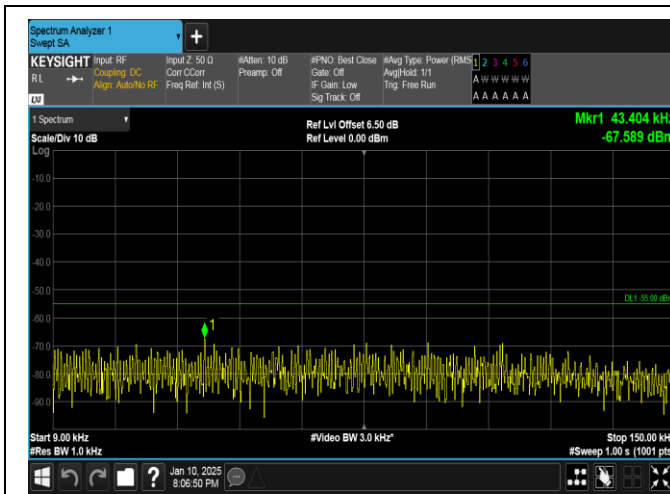
Band41-10MHz-16QAM-41540-1RB#49-0.009~0.15-PASS
