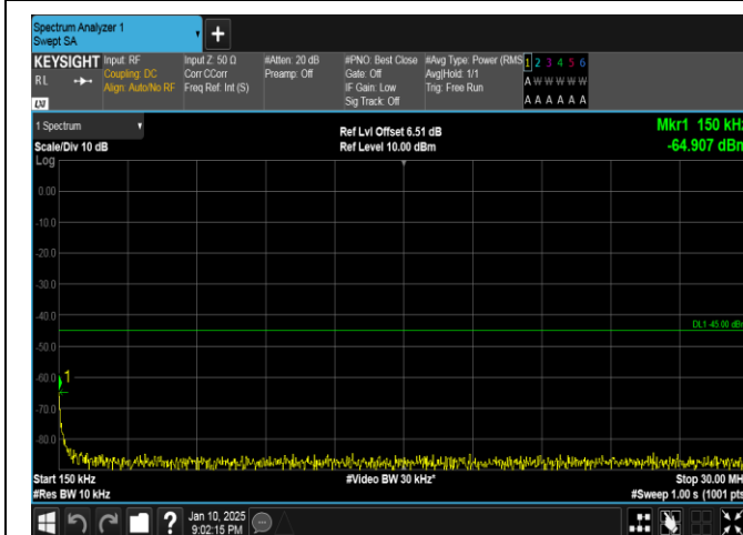
Band41-15MHz-QPSK-39725-1RB#74-0.15~30-PASS
