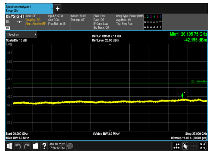
Band41-10MHz-16QAM-39700-50RB#0-20000~27000-PASS
