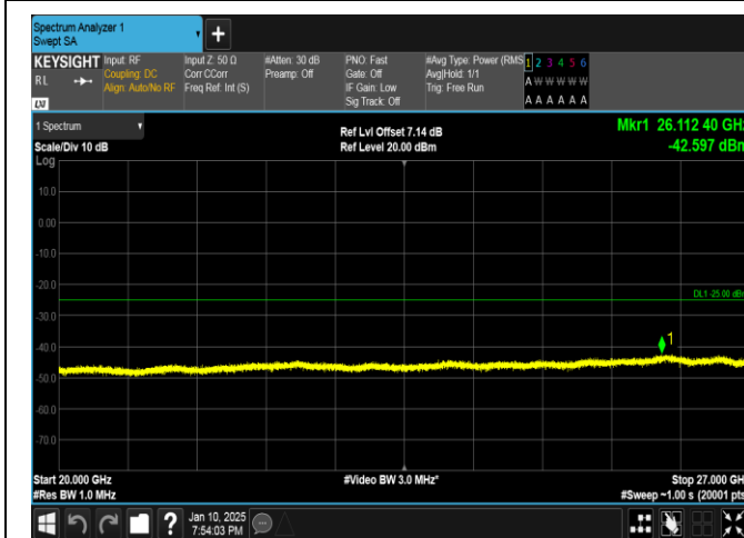
Band41-10MHz-16QAM-39700-1RB#49-20000~27000-PASS
