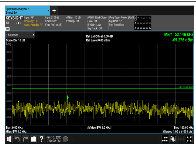
Band41-10MHz-16QAM-39700-1RB#0-0.009~0.15-PASS
