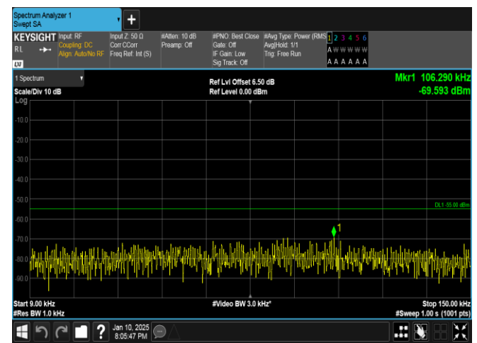
Band41-10MHz-QPSK-41540-1RB#49-0.009~0.15-PASS
