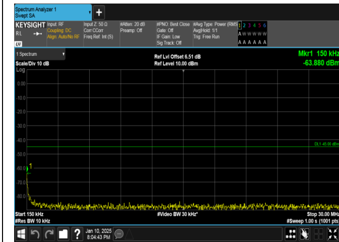
Band41-10MHz-16QAM-41540-1RB#0-0.15~30-PASS
