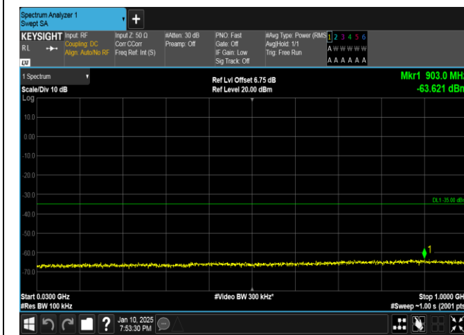
Band41-10MHz-16QAM-39700-1RB#49-30~1000-PASS
