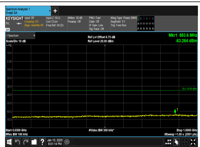
Band41-10MHz-QPSK-40620-50RB#0-30~1000-PASS
