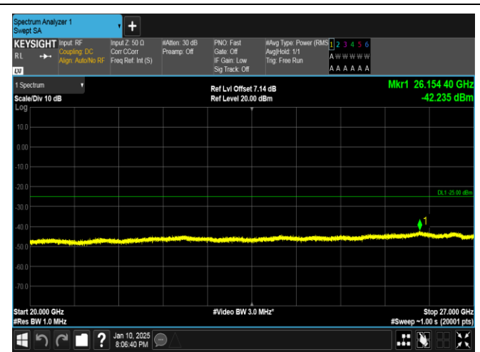
Band41-10MHz-QPSK-41540-1RB#49-20000~27000-PASS
