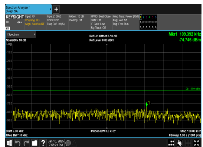
Band41-10MHz-16QAM-39700-50RB#0-0.009~0.15-PASS
