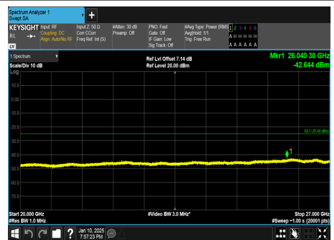
Band41-10MHz-QPSK-40620-1RB#0-20000~27000-PASS
