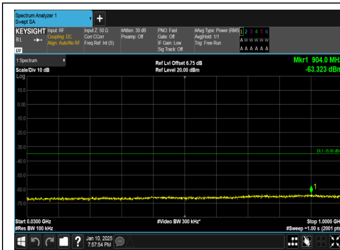
Band41-10MHz-16QAM-40620-1RB#0-30~1000-PASS
