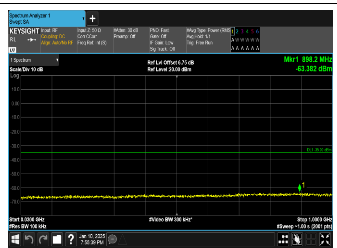
Band41-10MHz-16QAM-39700-50RB#0-30~1000-PASS
