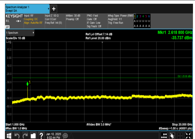
Band41-10MHz-16QAM-40620-50RB#0-1000~20000-PASS
