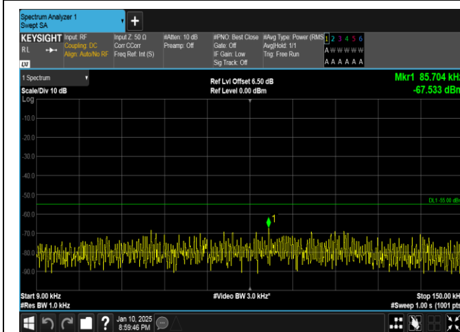
Band41-15MHz-QPSK-39725-1RB#0-0.009~0.15-PASS
