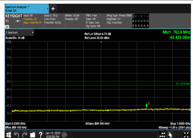
Band41-10MHz-16QAM-40620-1RB#49-30~1000-PASS
