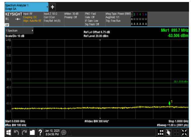
Band41-10MHz-16QAM-41540-1RB#0-30~1000-PASS
