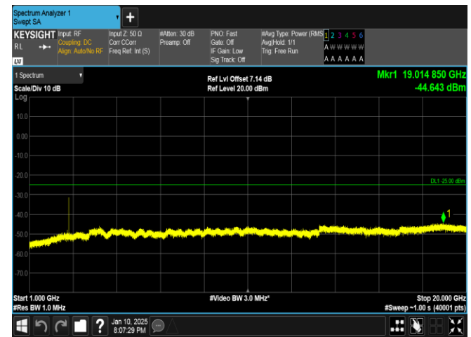
Band41-10MHz-16QAM-41540-1RB#49-1000~20000-PASS
