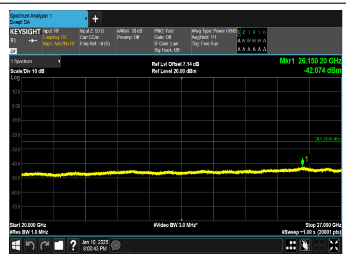
Band41-10MHz-16QAM-40620-1RB#49-20000~27000-PASS
