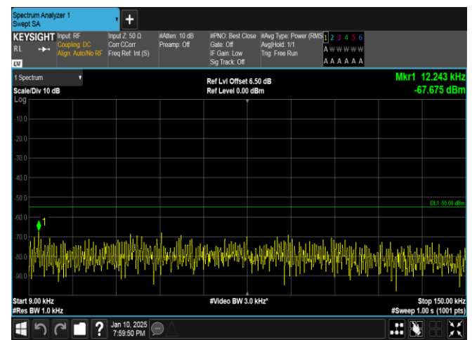
Band41-10MHz-16QAM-40620-1RB#49-0.009~0.15-PASS
