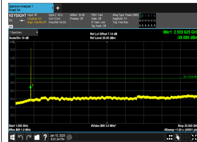
Band41-10MHz-QPSK-40620-50RB#0-1000~20000-PASS
