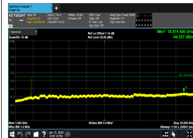
Band41-10MHz-16QAM-41540-1RB#0-1000~20000-PASS
