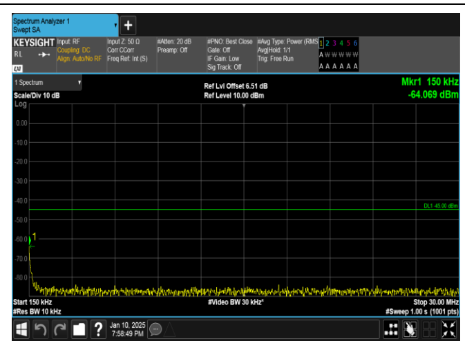
Band41-10MHz-QPSK-40620-1RB#49-0.15~30-PASS
