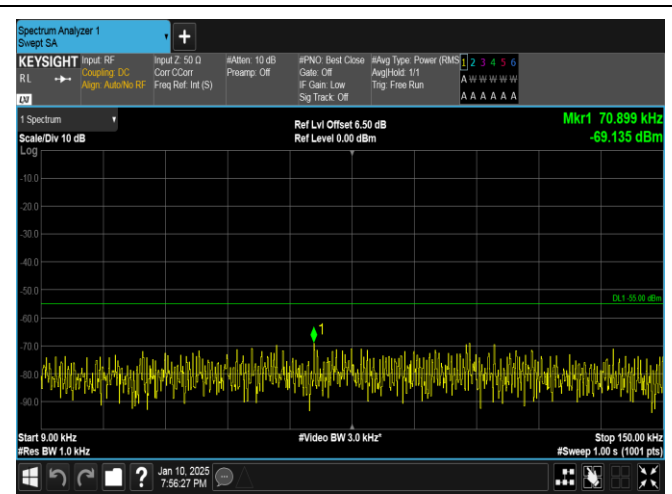
Band41-10MHz-QPSK-40620-1RB#0-0.009~0.15-PASS
