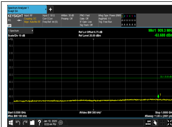
Band41-10MHz-QPSK-41540-1RB#0-30~1000-PASS
