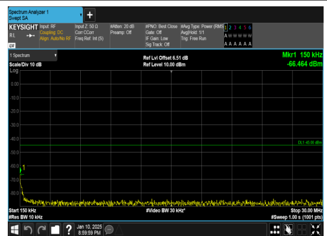
Band41-15MHz-QPSK-39725-1RB#0-0.15~30-PASS
