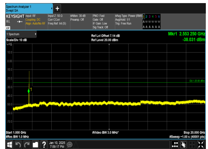
Band41-10MHz-QPSK-40620-1RB#49-1000~20000-PASS
