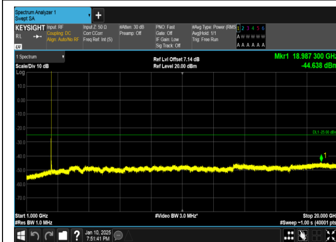
Band41-10MHz-16QAM-39700-1RB#0-1000~20000-PASS
