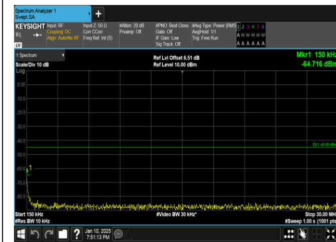
Band41-10MHz-16QAM-39700-1RB#0-0.15~30-PASS
