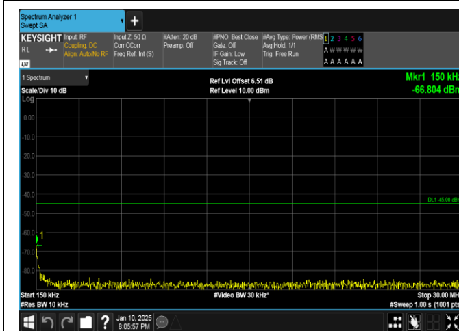
Band41-10MHz-QPSK-41540-1RB#49-0.15~30-PASS
