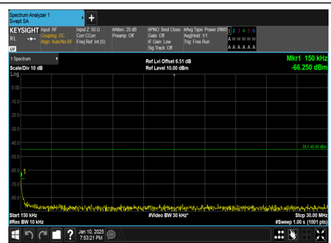
Band41-10MHz-16QAM-39700-1RB#49-0.15~30-PASS
