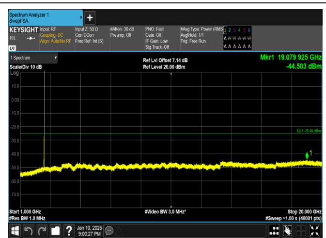
Band41-15MHz-QPSK-39725-1RB#0-1000~20000-PASS
