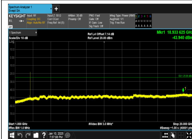
Band41-10MHz-QPSK-40620-1RB#0-1000~20000-PASS
