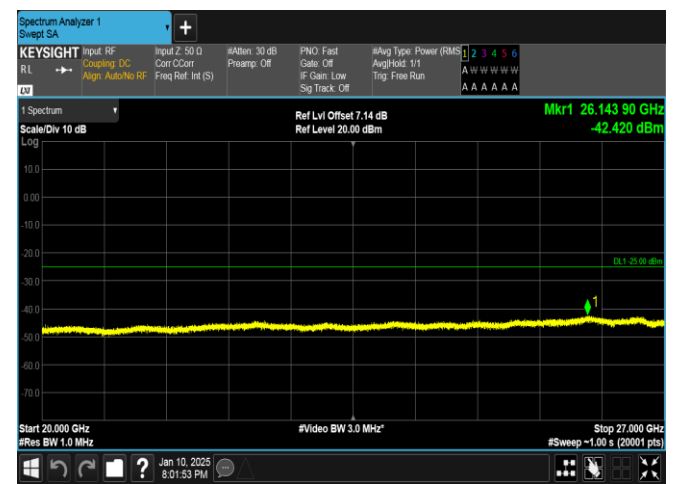
Band41-10MHz-QPSK-40620-50RB#0-20000~27000-PASS
