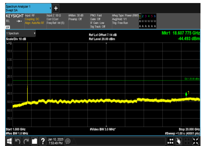
Band41-10MHz-16QAM-39700-1RB#49-1000~20000-PASS
