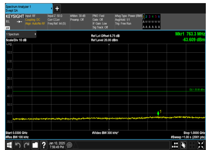
Band41-10MHz-QPSK-40620-1RB#0-30~1000-PASS
