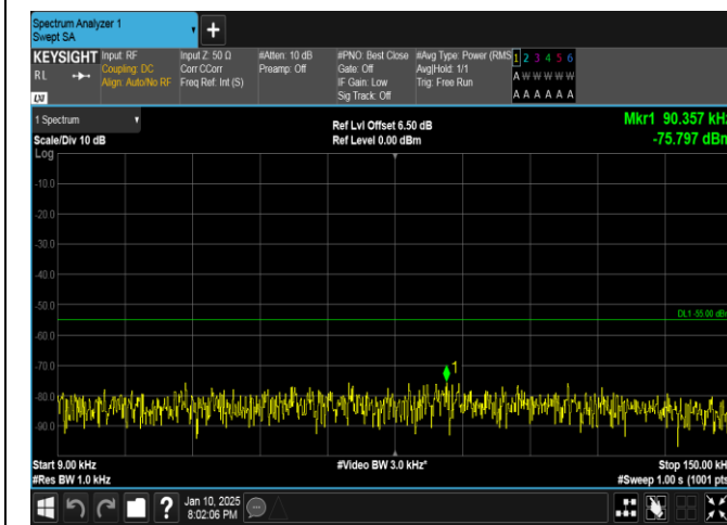
Band41-10MHz-16QAM-40620-50RB#0-0.009~0.15-PASS
