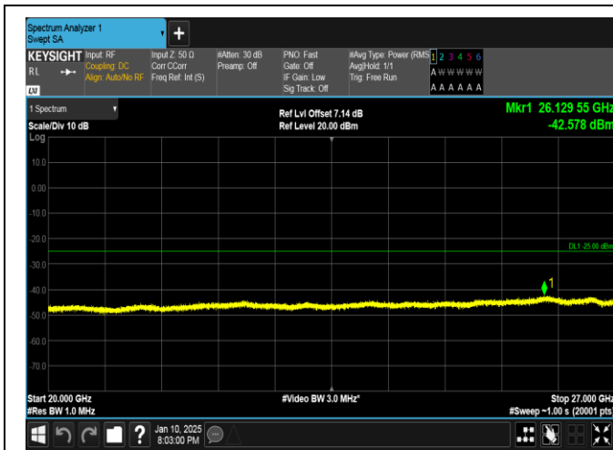
Band41-10MHz-16QAM-40620-50RB#0-20000~27000-PASS
