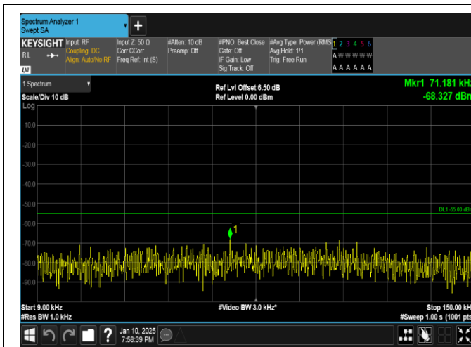
Band41-10MHz-QPSK-40620-1RB#49-0.009~0.15-PASS
