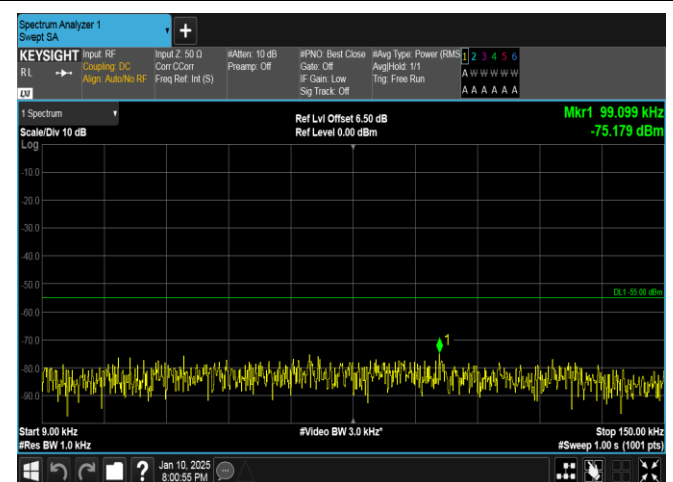
Band41-10MHz-QPSK-40620-50RB#0-0.009~0.15-PASS
