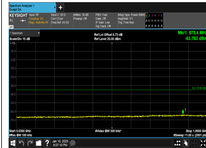
Band41-10MHz-16QAM-41540-1RB#49-30~1000-PASS
