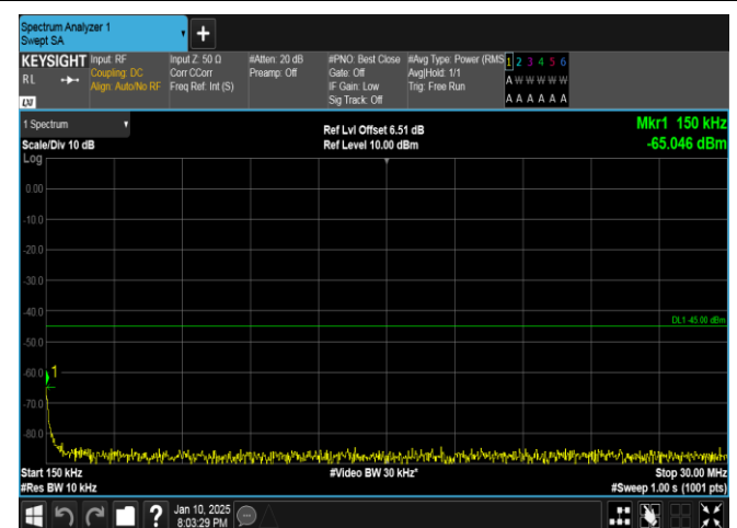
Band41-10MHz-QPSK-41540-1RB#0-0.15~30-PASS
