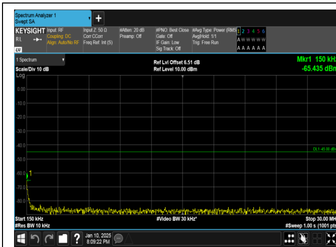
Band41-10MHz-16QAM-41540-50RB#0-0.15~30-PASS
