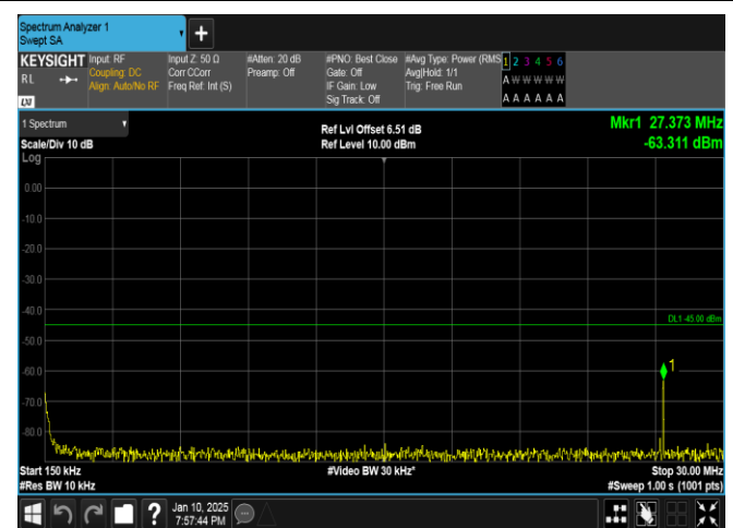
Band41-10MHz-16QAM-40620-1RB#0-0.15~30-PASS
