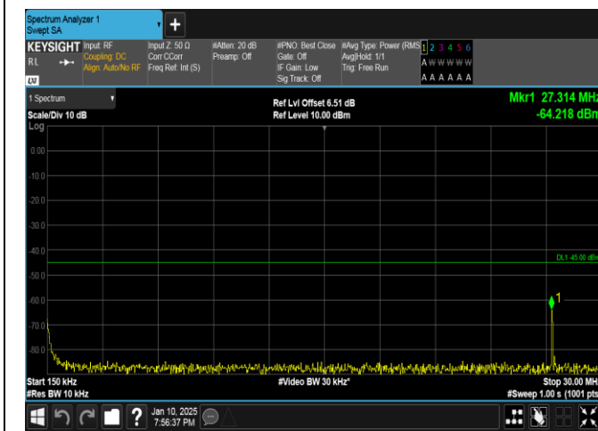
Band41-10MHz-QPSK-40620-1RB#0-0.15~30-PASS
