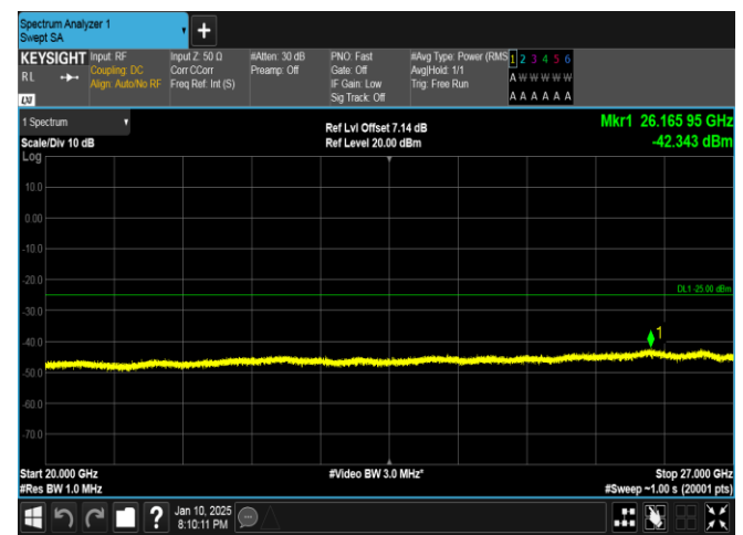
Band41-10MHz-16QAM-41540-50RB#0-20000~27000-PASS
