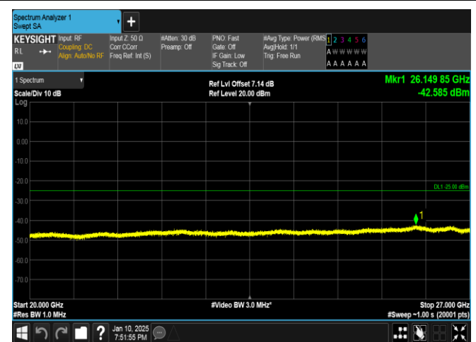
Band41-10MHz-16QAM-39700-1RB#0-20000~27000-PASS
