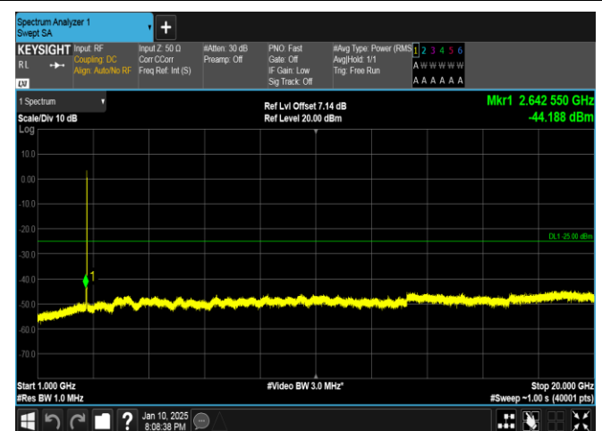
Band41-10MHz-QPSK-41540-50RB#0-1000~20000-PASS
