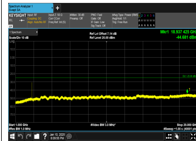
Band41-10MHz-16QAM-41540-50RB#0-1000~20000-PASS
