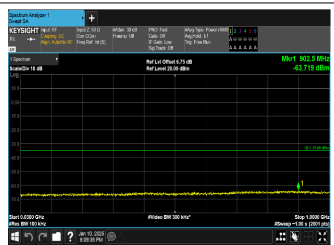
Band41-10MHz-16QAM-41540-50RB#0-30~1000-PASS
