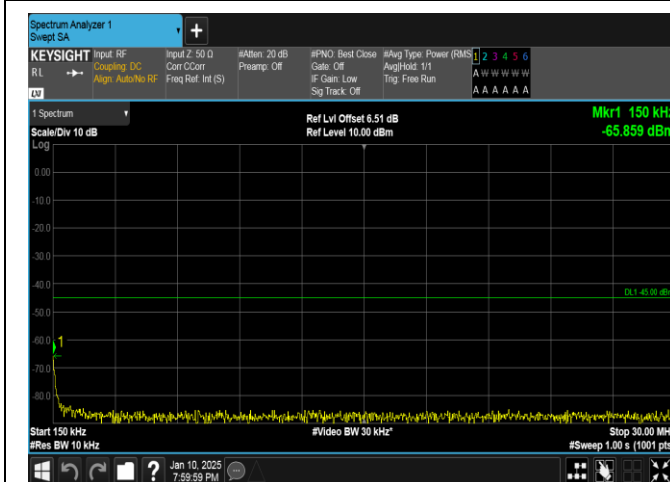
Band41-10MHz-16QAM-40620-1RB#49-0.15~30-PASS
