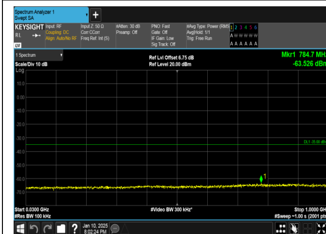
Band41-10MHz-16QAM-40620-50RB#0-30~1000-PASS
