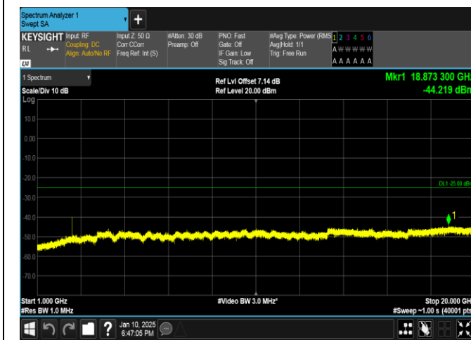
Band41-5MHz-16QAM-39675-25RB#0-1000~20000-PASS
