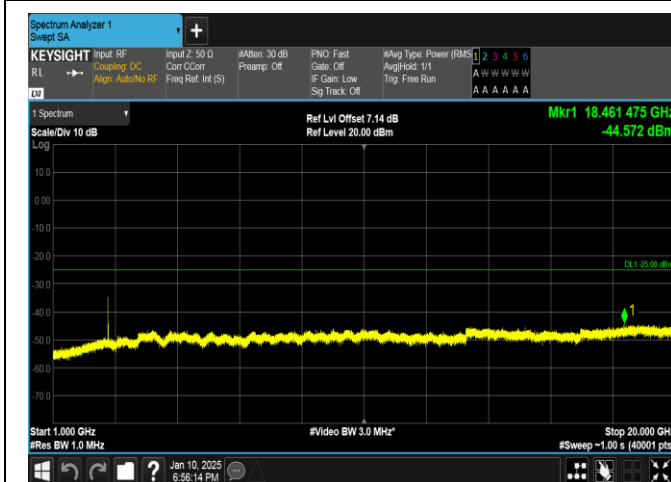
Band41-5MHz-16QAM-41565-1RB#0-1000~20000-PASS
