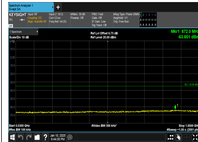
Band41-5MHz-16QAM-39675-1RB#24-30~1000-PASS
