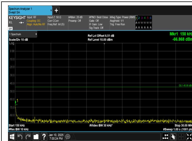
Band41-5MHz-16QAM-41565-25RB#0-0.15~30-PASS
