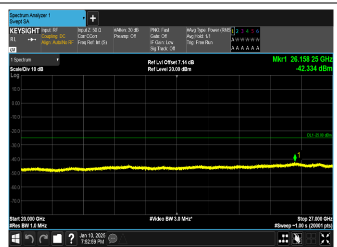
Band41-10MHz-QPSK-39700-1RB#49-20000~27000-PASS
