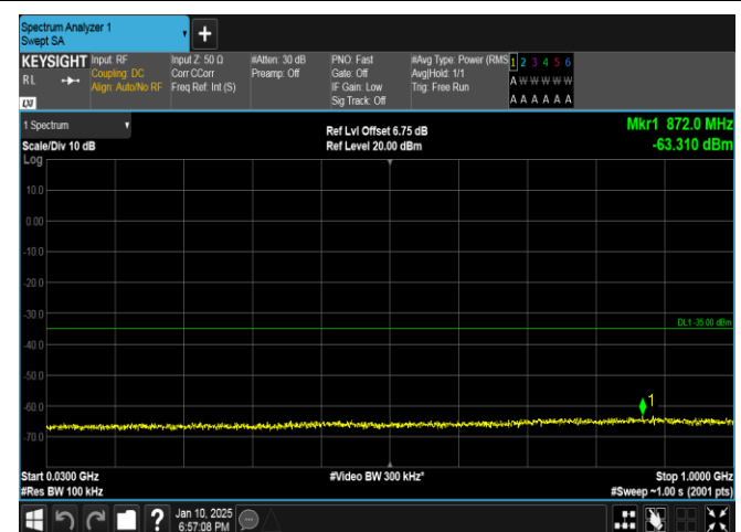
Band41-5MHz-QPSK-41565-1RB#24-30~1000-PASS
