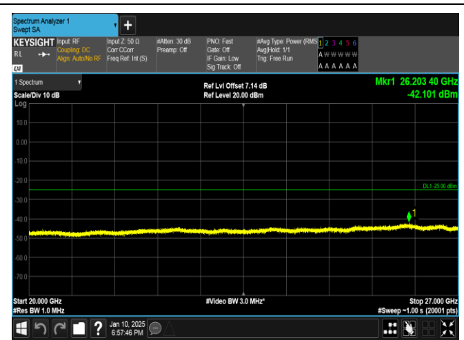
Band41-5MHz-QPSK-41565-1RB#24-20000~27000-PASS
