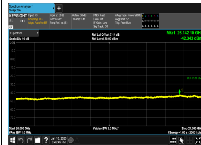
Band41-5MHz-16QAM-40620-1RB#0-20000~27000-PASS
