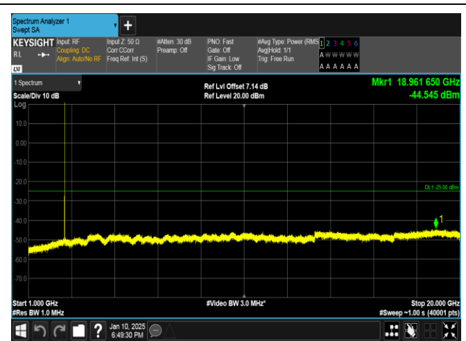
Band41-5MHz-16QAM-40620-1RB#0-1000~20000-PASS
