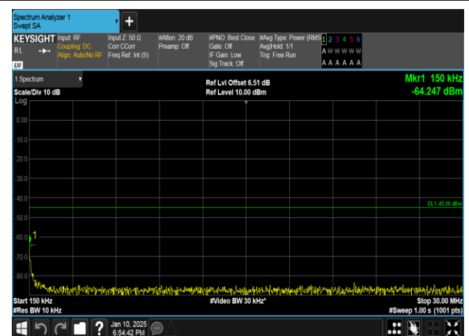
Band41-5MHz-QPSK-41565-1RB#0-0.15~30-PASS
