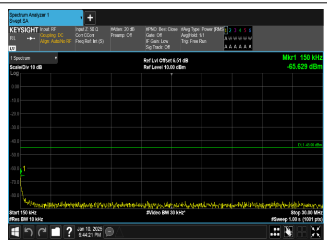
Band41-5MHz-16QAM-39675-1RB#24-0.15~30-PASS
