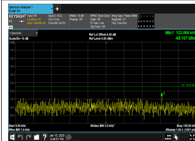
Band41-5MHz-16QAM-40620-1RB#0-0.009~0.15-PASS
