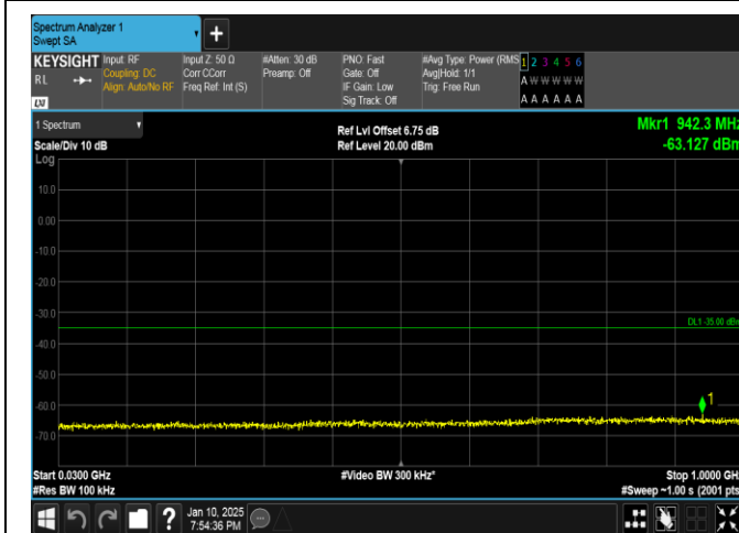
Band41-10MHz-QPSK-39700-50RB#0-30~1000-PASS
