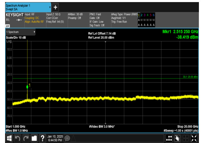
Band41-5MHz-16QAM-39675-1RB#24-1000~20000-PASS
