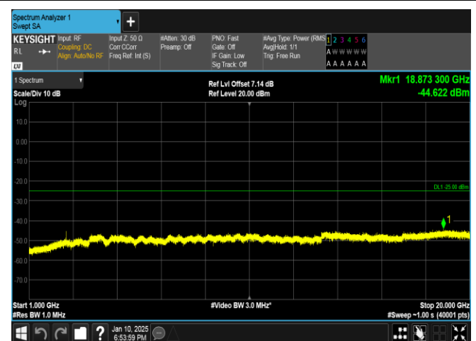
Band41-5MHz-16QAM-40620-25RB#0-1000~20000-PASS
