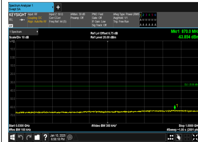
Band41-5MHz-16QAM-41565-1RB#24-30~1000-PASS
