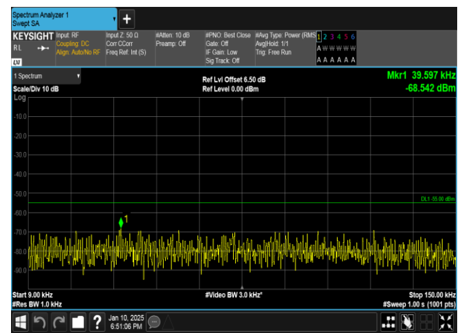
Band41-5MHz-16QAM-40620-1RB#24-0.009~0.15-PASS
