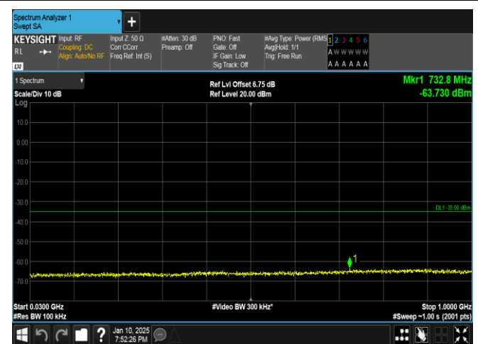
Band41-10MHz-QPSK-39700-1RB#49-30~1000-PASS
