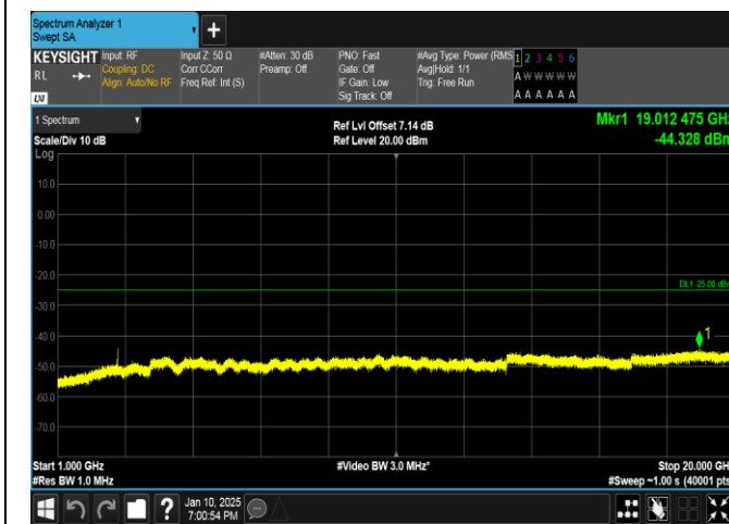
Band41-5MHz-16QAM-41565-25RB#0-1000~20000-PASS
