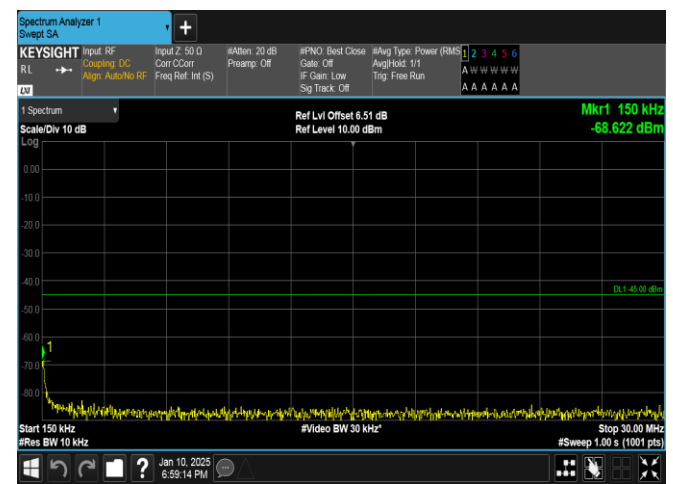
Band41-5MHz-QPSK-41565-25RB#0-0.15~30-PASS
