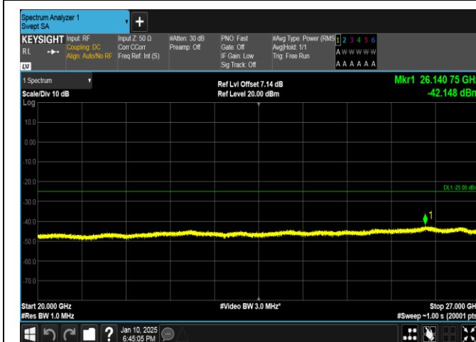
Band41-5MHz-16QAM-39675-1RB#24-20000~27000-PASS
