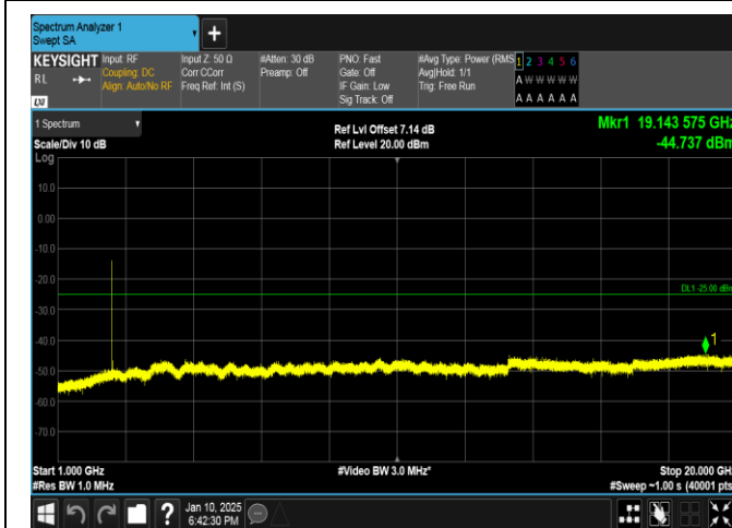
Band41-5MHz-16QAM-39675-1RB#0-1000~20000-PASS
