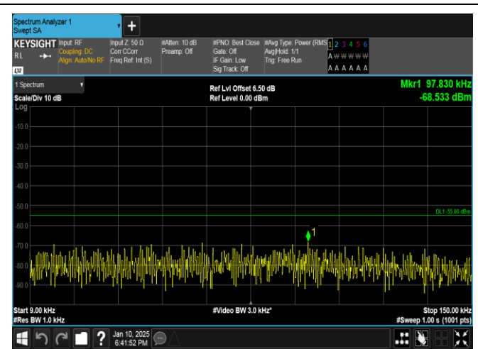
Band41-5MHz-16QAM-39675-1RB#0-0.009~0.15-PASS
