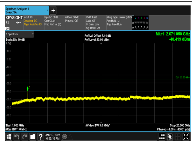
Band41-5MHz-QPSK-41565-1RB#0-1000~20000-PASS
