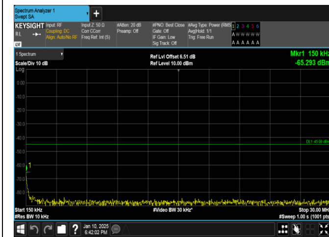
Band41-5MHz-16QAM-39675-1RB#0-0.15~30-PASS
