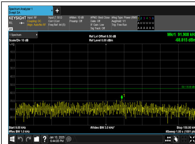
Band41-5MHz-16QAM-39675-1RB#24-0.009~0.15-PASS
