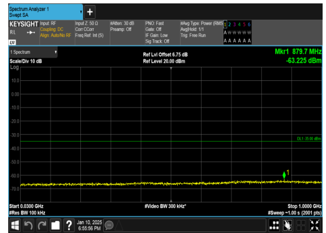
Band41-5MHz-16QAM-41565-1RB#0-30~1000-PASS
