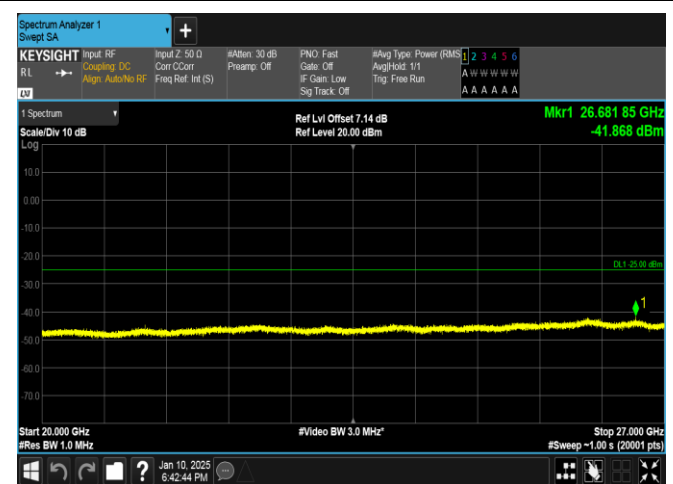
Band41-5MHz-16QAM-39675-1RB#0-20000~27000-PASS
