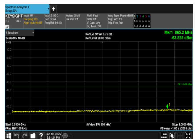
Band41-5MHz-16QAM-40620-1RB#24-30~1000-PASS
