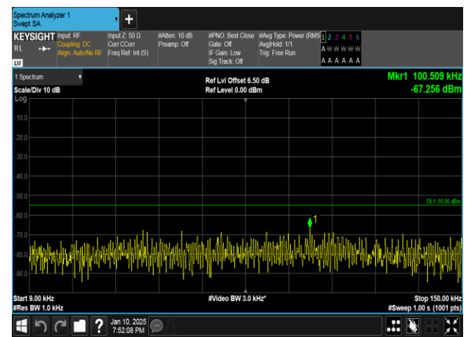
Band41-10MHz-QPSK-39700-1RB#49-0.009~0.15-PASS
