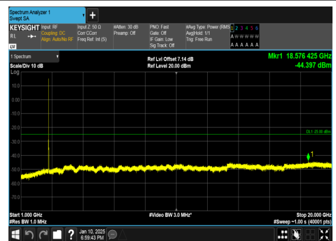
Band41-5MHz-QPSK-41565-25RB#0-1000~20000-PASS
