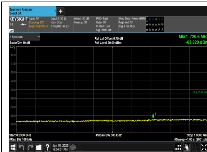
Band41-5MHz-QPSK-41565-1RB#0-30~1000-PASS
