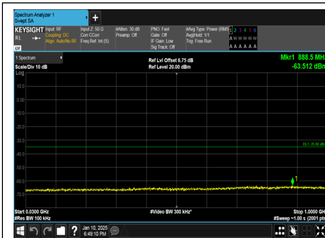
Band41-5MHz-16QAM-40620-1RB#0-30~1000-PASS
