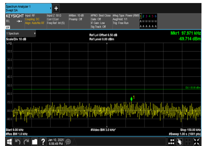
Band41-5MHz-QPSK-41565-1RB#24-0.009~0.15-PASS
