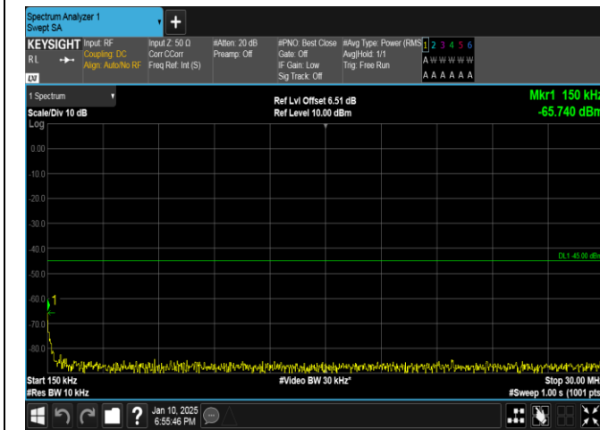
Band41-5MHz-16QAM-41565-1RB#0-0.15~30-PASS
