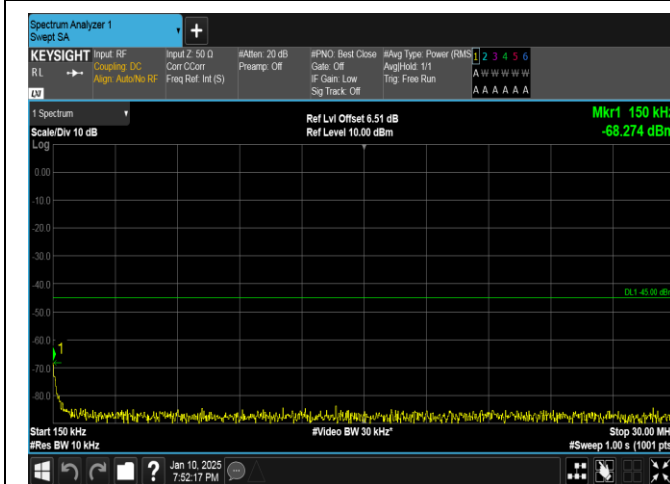
Band41-10MHz-QPSK-39700-1RB#49-0.15~30-PASS
