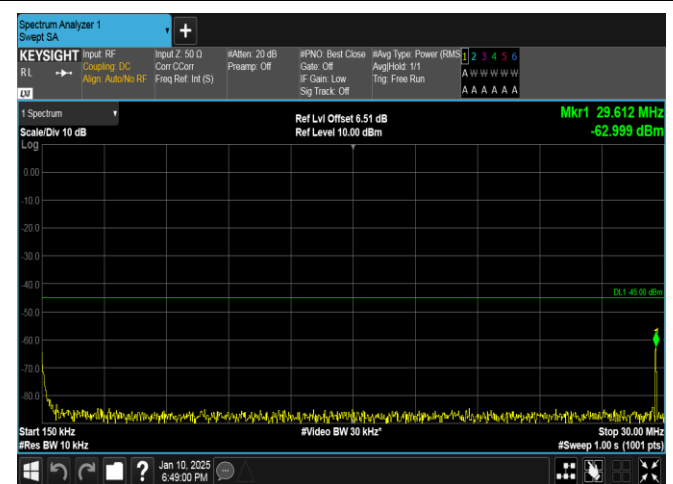
Band41-5MHz-16QAM-40620-1RB#0-0.15~30-PASS
