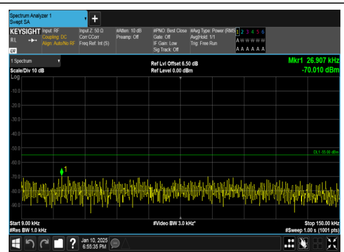
Band41-5MHz-16QAM-41565-1RB#0-0.009~0.15-PASS
