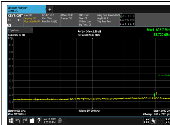
Band41-10MHz-QPSK-39700-1RB#0-30~1000-PASS
