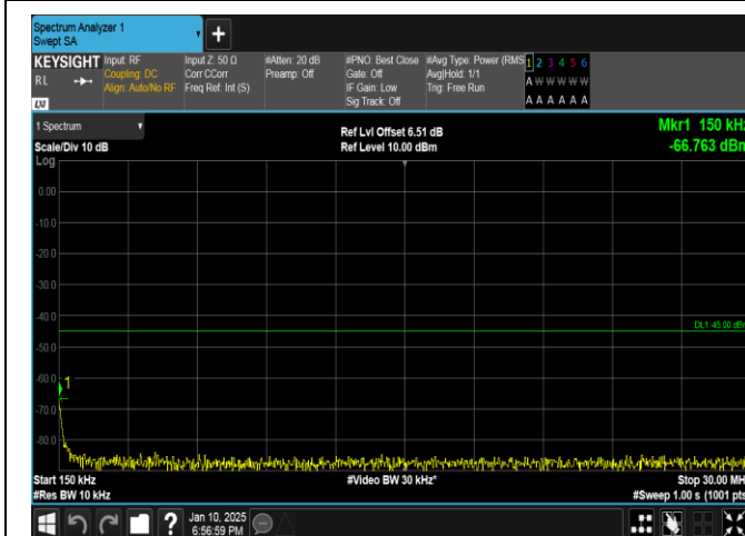
Band41-5MHz-QPSK-41565-1RB#24-0.15~30-PASS
