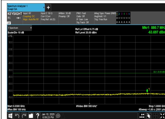
Band41-5MHz-QPSK-41565-25RB#0-30~1000-PASS
