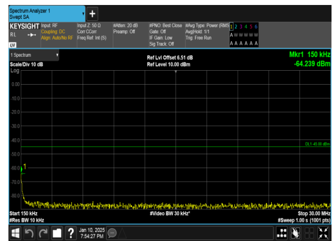
Band41-10MHz-QPSK-39700-50RB#0-0.15~30-PASS
