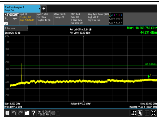
Band41-10MHz-QPSK-39700-1RB#0-1000~20000-PASS
