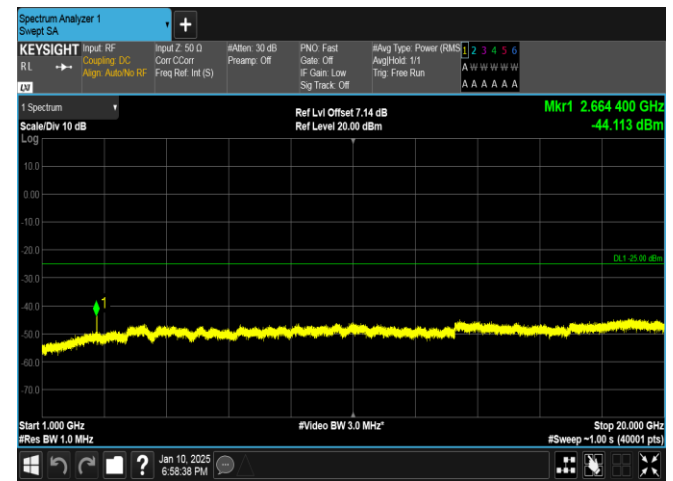
Band41-5MHz-16QAM-41565-1RB#24-1000~20000-PASS
