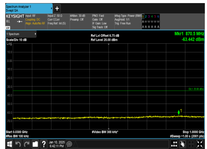
Band41-5MHz-16QAM-39675-1RB#0-30~1000-PASS
