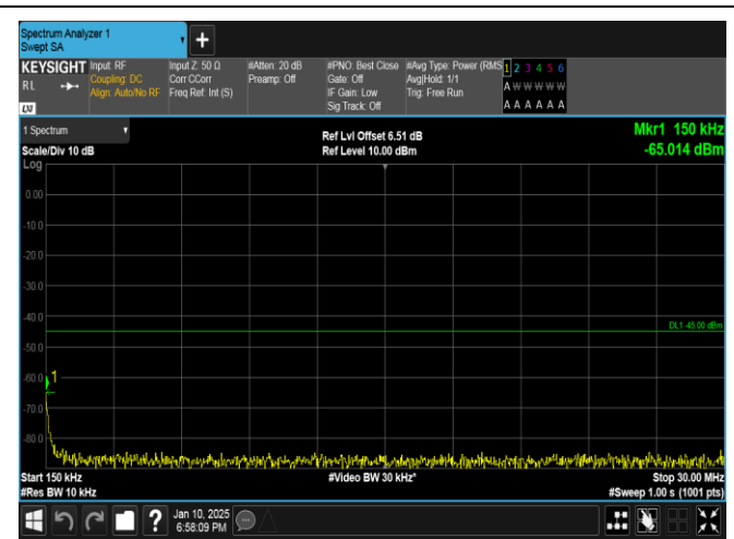
Band41-5MHz-16QAM-41565-1RB#24-0.15~30-PASS
