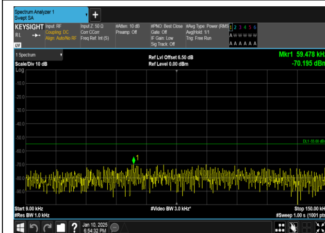
Band41-5MHz-QPSK-41565-1RB#0-0.009~0.15-PASS
