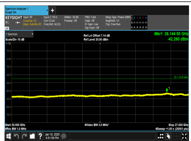
Band41-5MHz-16QAM-40620-1RB#24-20000~27000-PASS
