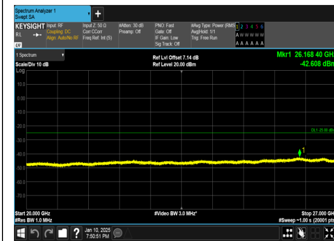
Band41-10MHz-QPSK-39700-1RB#0-20000~27000-PASS
