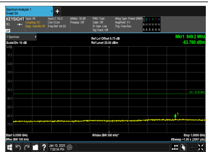
Band41-5MHz-16QAM-41565-25RB#0-30~1000-PASS
