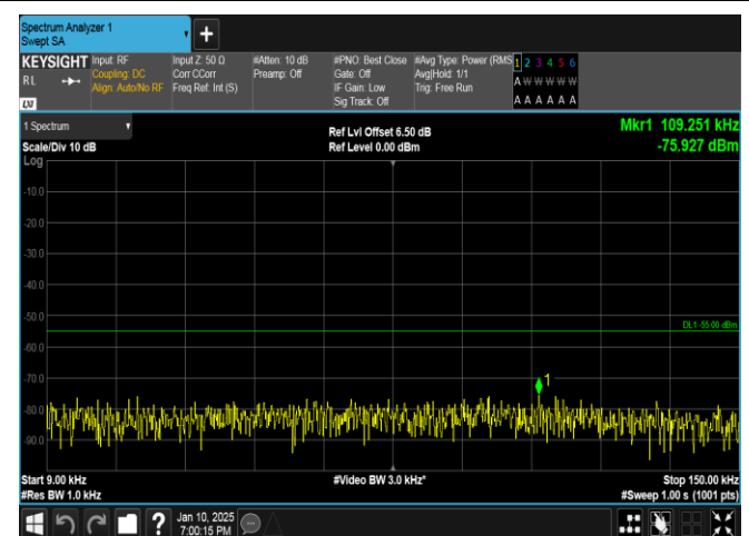
Band41-5MHz-16QAM-41565-25RB#0-0.009~0.15-PASS
