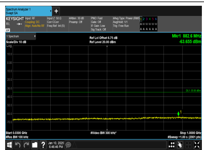
Band41-5MHz-16QAM-39675-25RB#0-30~1000-PASS
