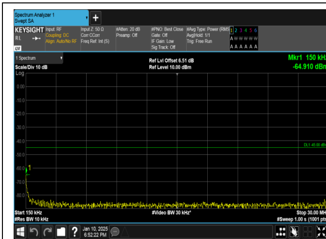
Band41-5MHz-QPSK-40620-25RB#0-0.15~30-PASS
