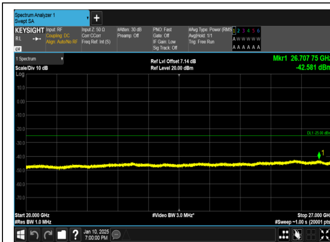
Band41-5MHz-QPSK-41565-25RB#0-20000~27000-PASS
