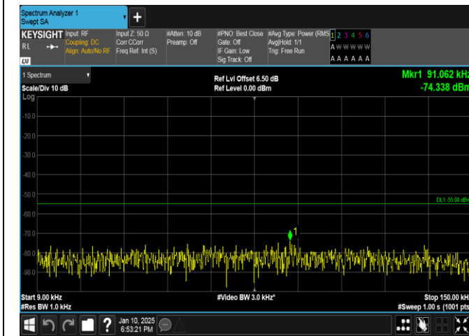
Band41-5MHz-16QAM-40620-25RB#0-0.009~0.15-PASS
