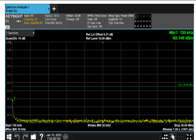
Band41-10MHz-QPSK-39700-1RB#0-0.15~30-PASS
