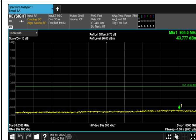
Band41-5MHz-16QAM-40620-25RB#0-30~1000-PASS
