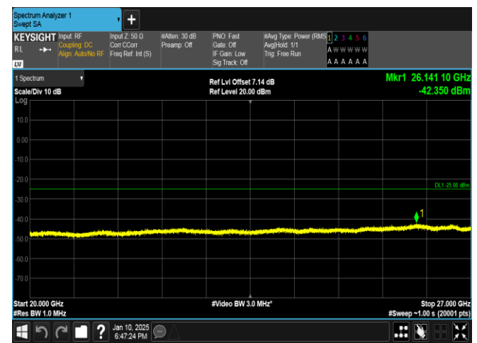
Band41-5MHz-16QAM-39675-25RB#0-20000~27000-PASS
