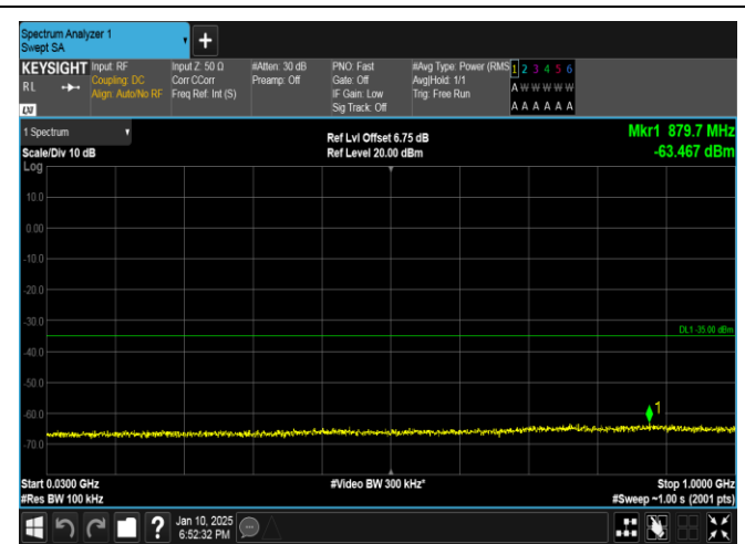
Band41-5MHz-QPSK-40620-25RB#0-30~1000-PASS
