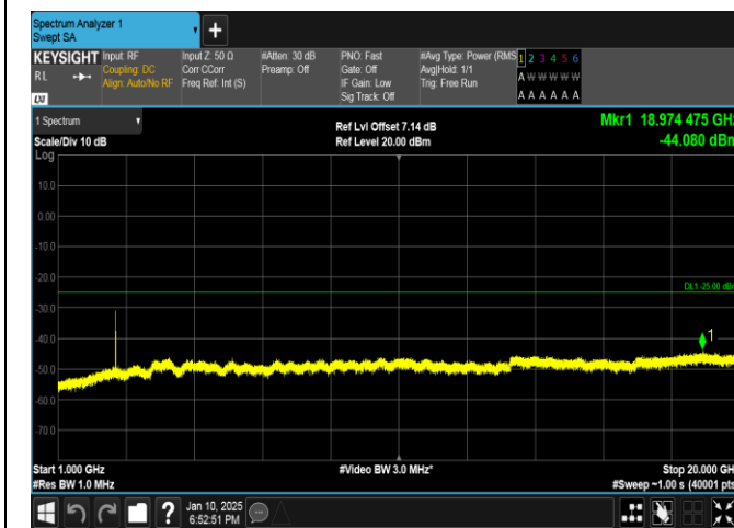
Band41-5MHz-QPSK-40620-25RB#0-1000~20000-PASS
