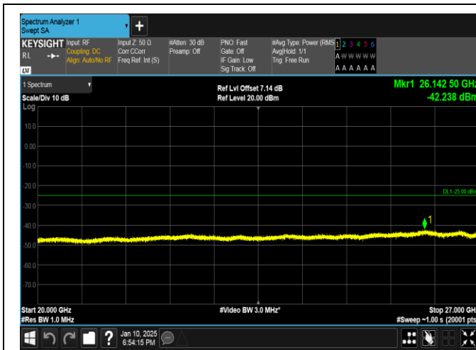
Band41-5MHz-16QAM-40620-25RB#0-20000~27000-PASS
