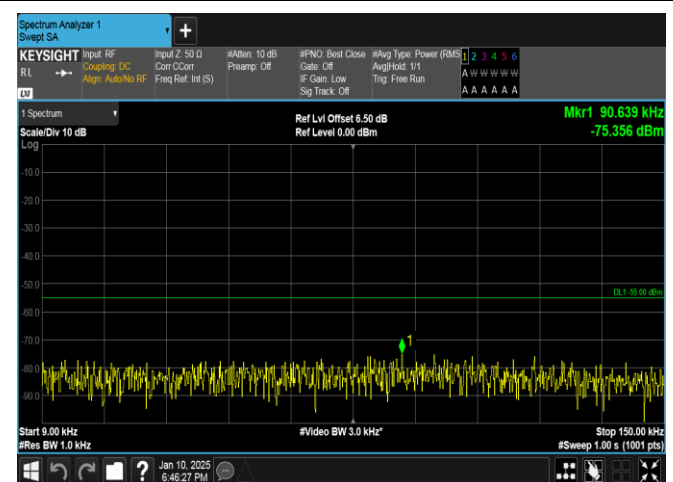
Band41-5MHz-16QAM-39675-25RB#0-0.009~0.15-PASS
