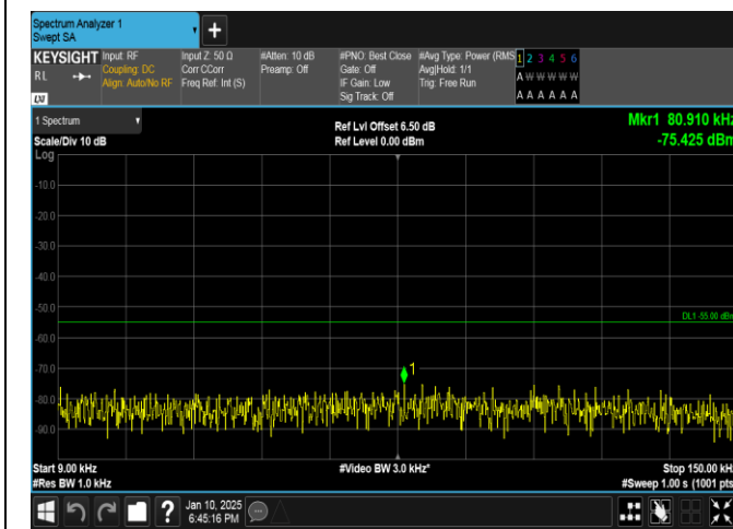
Band41-5MHz-QPSK-39675-25RB#0-0.009~0.15-PASS
