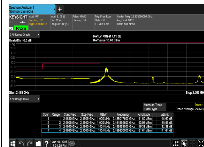
Band41-10MHz-QPSK-39700-1RB#0-PASS
