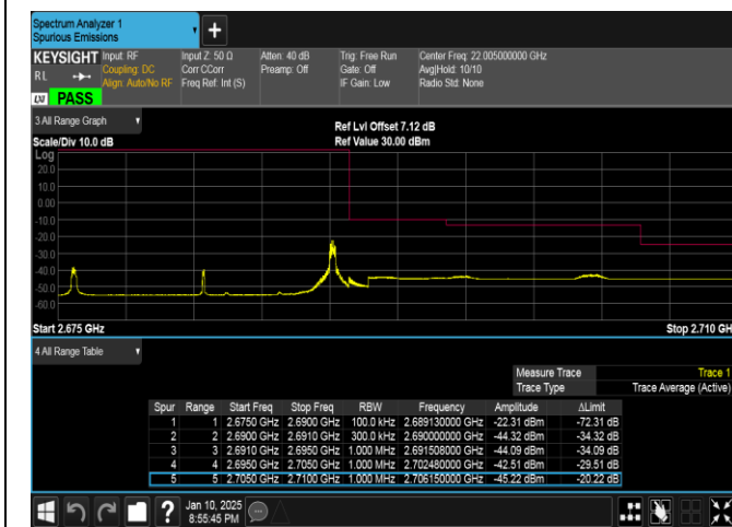
Band41-15MHz-16QAM-41515-1RB#74-PASS
