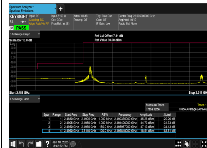
Band41-15MHz-16QAM-39725-1RB#0-PASS
