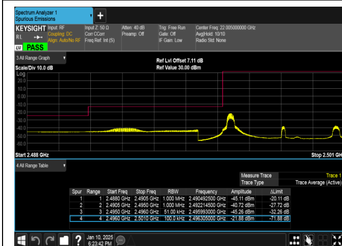
Band41-5MHz-16QAM-39675-1RB#0-PASS
