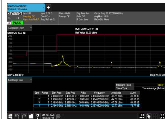
Band41-20MHz-16QAM-39750-1RB#0-PASS
