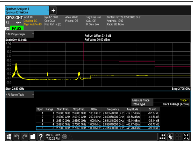
Band41-10MHz-16QAM-41540-1RB#0-PASS
