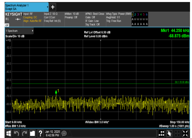
Band41-5MHz-QPSK-39675-1RB#24-0.009~0.15-PASS
