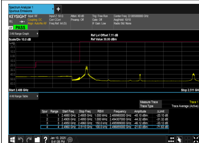
Band41-15MHz-QPSK-39725-1RB#0-PASS
