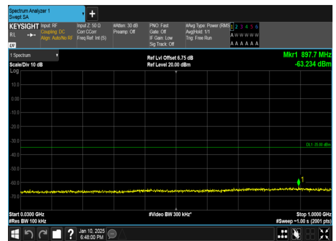
Band41-5MHz-QPSK-40620-1RB#0-30~1000-PASS
