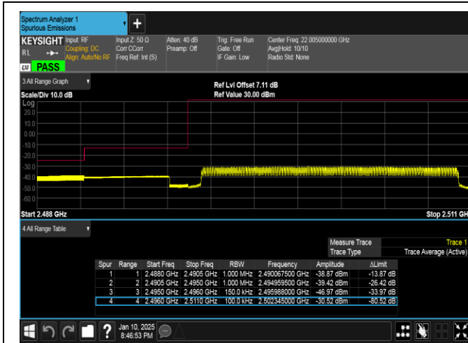
Band41-15MHz-QPSK-39725-75RB#0-PASS
