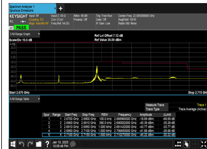
Band41-20MHz-16QAM-41490-1RB#99-PASS
