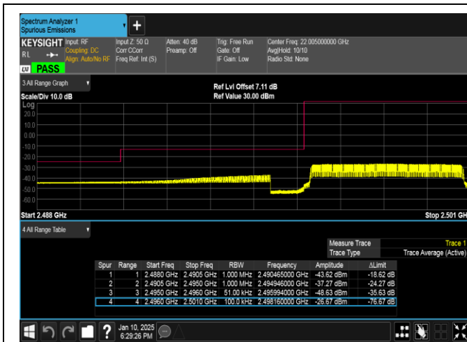
Band41-5MHz-16QAM-39675-25RB#0-PASS
