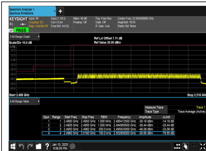
Band41-20MHz-QPSK-39750-100RB#0-PASS
