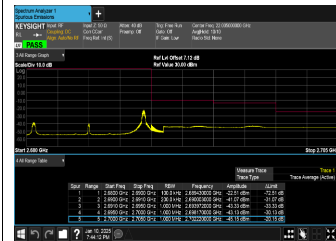
Band41-10MHz-QPSK-41540-1RB#49-PASS
