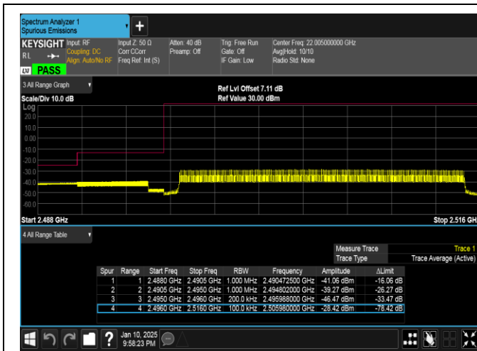
Band41-20MHz-16QAM-39750-100RB#0-PASS
