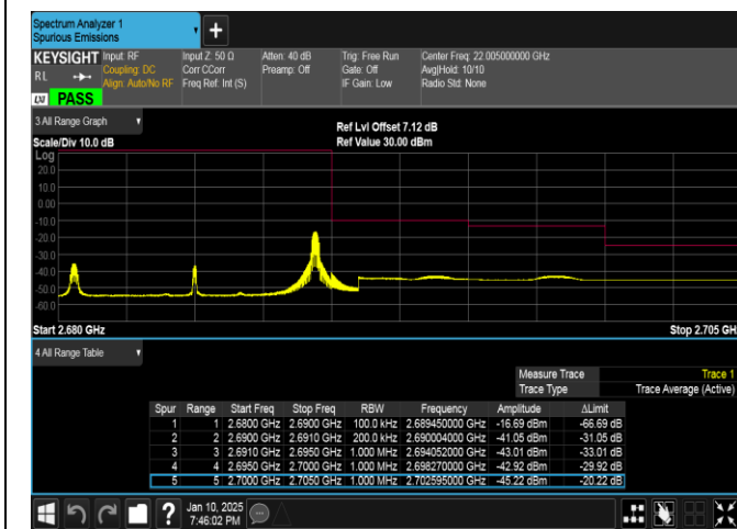
Band41-10MHz-16QAM-41540-1RB#49-PASS
