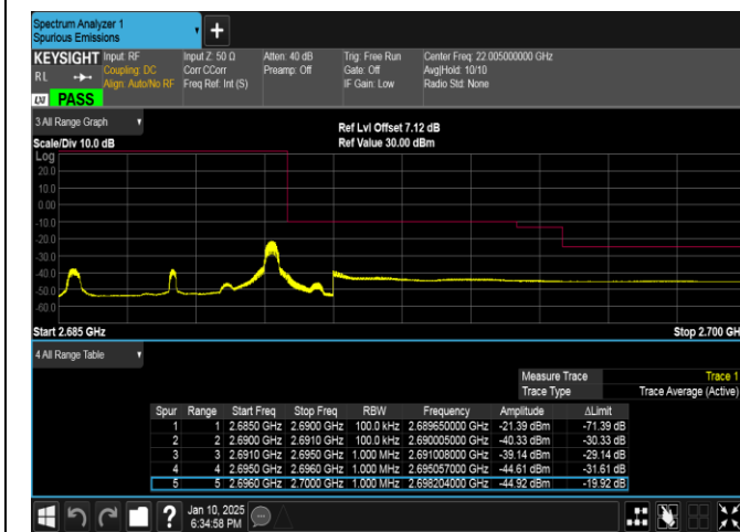
Band41-5MHz-QPSK-41565-1RB#24-PASS
