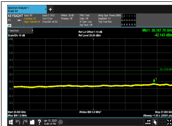
Band41-5MHz-QPSK-39675-25RB#0-20000~27000-PASS
