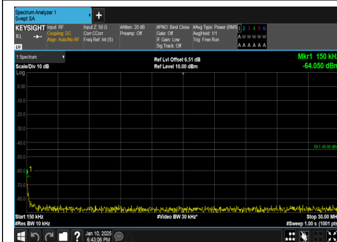
Band41-5MHz-QPSK-39675-1RB#24-0.15~30-PASS
