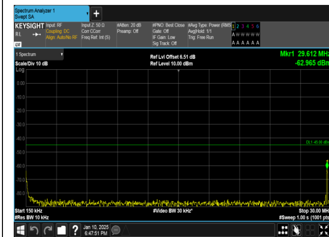
Band41-5MHz-QPSK-40620-1RB#0-0.15~30-PASS
