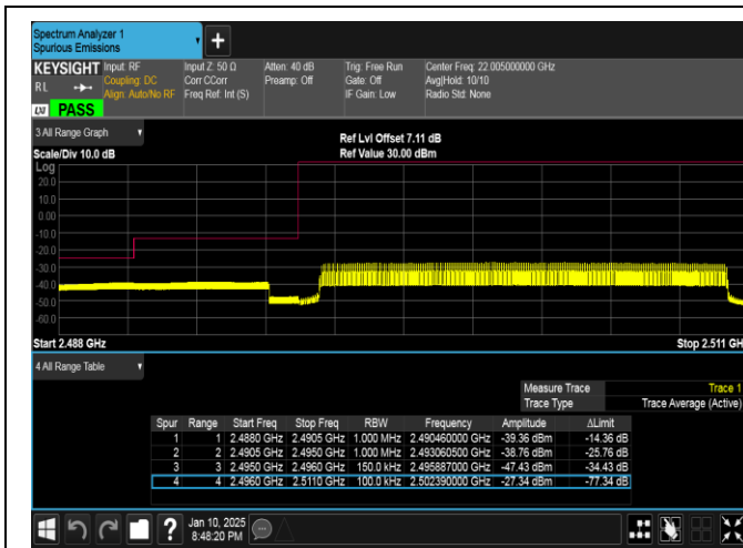
Band41-15MHz-16QAM-39725-75RB#0-PASS
