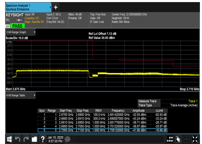
Band41-15MHz-QPSK-41515-75RB#0-PASS
