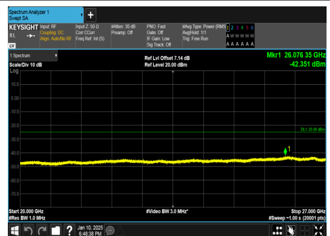
Band41-5MHz-QPSK-40620-1RB#0-20000~27000-PASS
