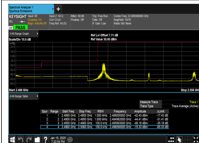
Band41-10MHz-16QAM-39700-1RB#0-PASS
