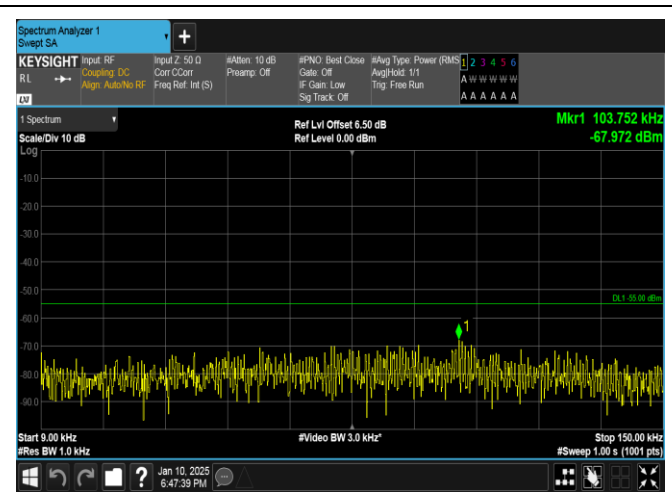
Band41-5MHz-QPSK-40620-1RB#0-0.009~0.15-PASS
