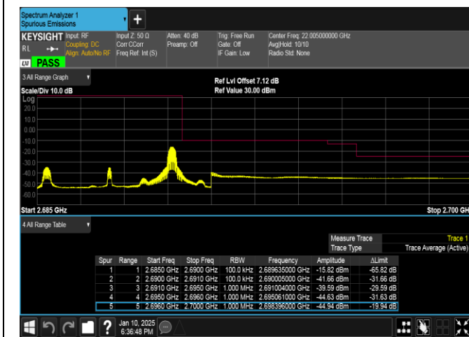
Band41-5MHz-16QAM-41565-1RB#24-PASS
