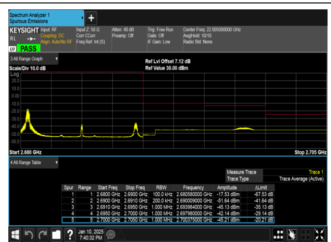
Band41-10MHz-QPSK-41540-1RB#0-PASS
