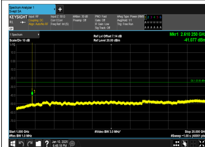
Band41-5MHz-QPSK-40620-1RB#0-1000~20000-PASS
