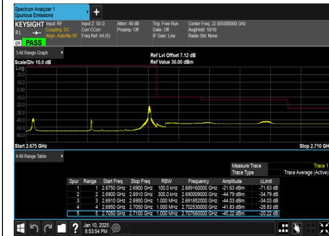
Band41-15MHz-QPSK-41515-1RB#74-PASS
