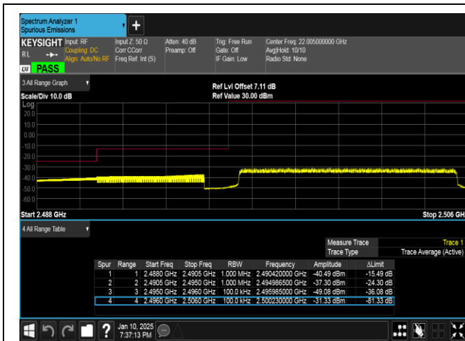
Band41-10MHz-QPSK-39700-50RB#0-PASS
