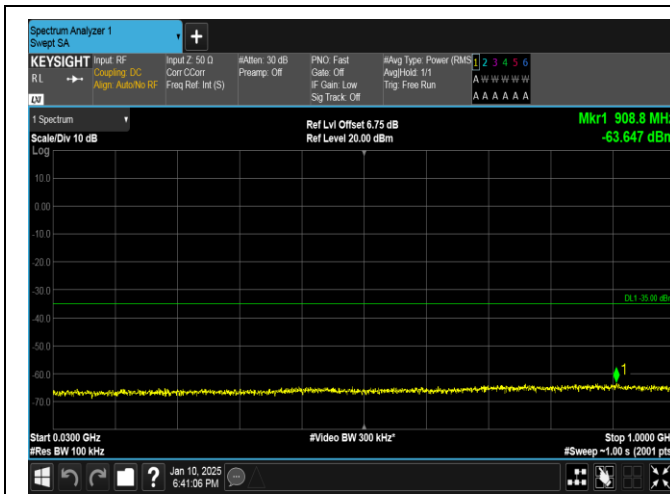
Band41-5MHz-QPSK-39675-1RB#0-30~1000-PASS
