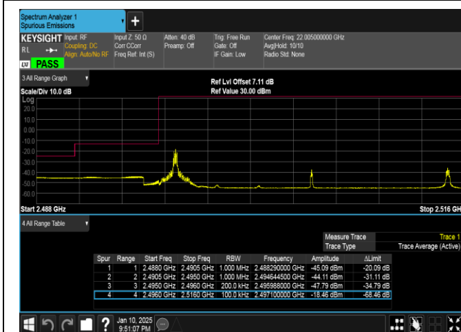
Band41-20MHz-QPSK-39750-1RB#0-PASS
