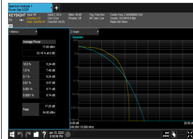
Band41-10MHz-QPSK-40620-1RB#0-PASS
