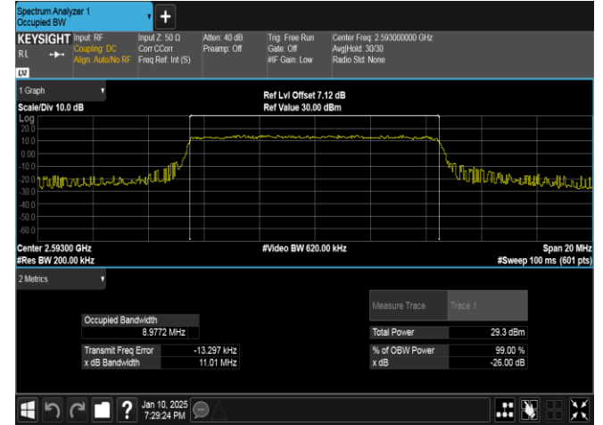
Band41-10MHz-QPSK-40620-50RB#0-PASS
