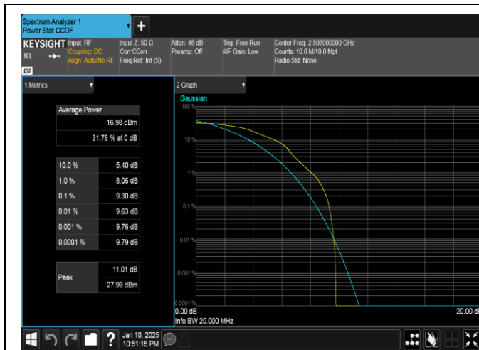
Band41-20MHz-16QAM-39750-1RB#0-PASS
