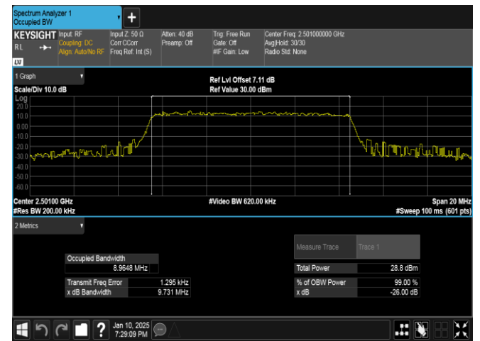
Band41-10MHz-16QAM-39700-50RB#0-PASS
