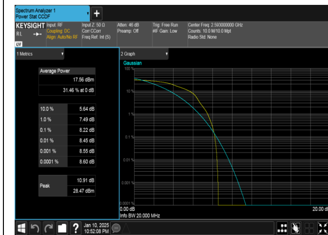
Band41-20MHz-16QAM-40620-1RB#0-PASS
