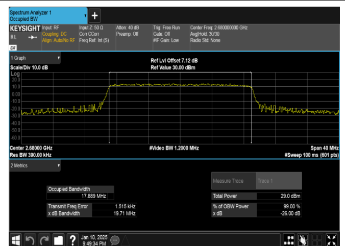
Band41-20MHz-16QAM-41490-100RB#0-PASS
