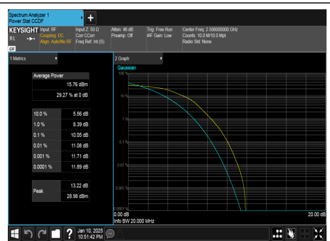
Band41-20MHz-16QAM-39750-100RB#0-PASS
