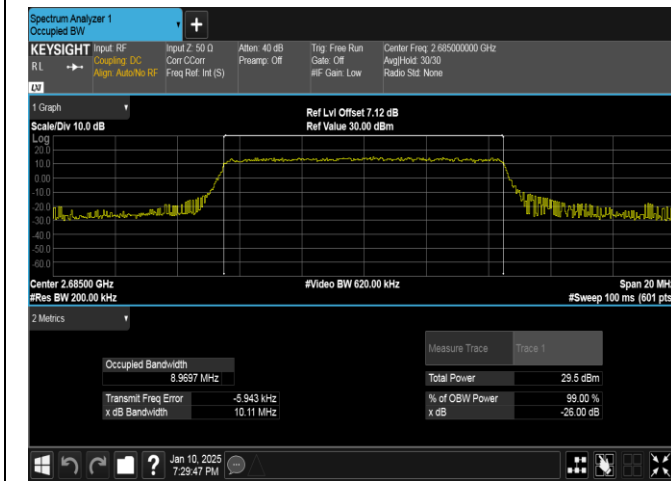
Band41-10MHz-QPSK-41540-50RB#0-PASS
