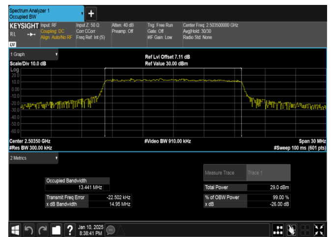
Band41-15MHz-16QAM-39725-75RB#0-PASS
