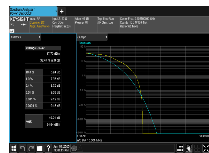
Band41-15MHz-QPSK-39725-1RB#0-PASS
