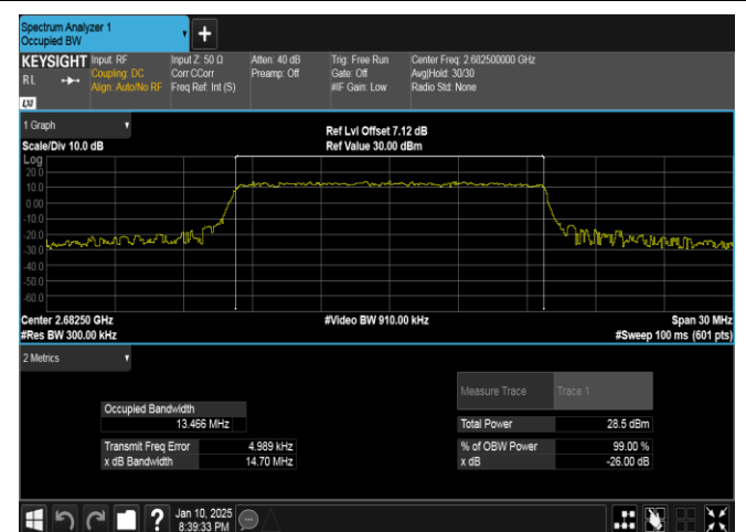
Band41-15MHz-16QAM-41515-75RB#0-PASS
