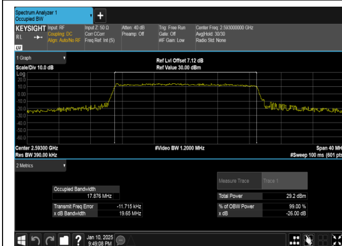
Band41-20MHz-16QAM-40620-100RB#0-PASS
