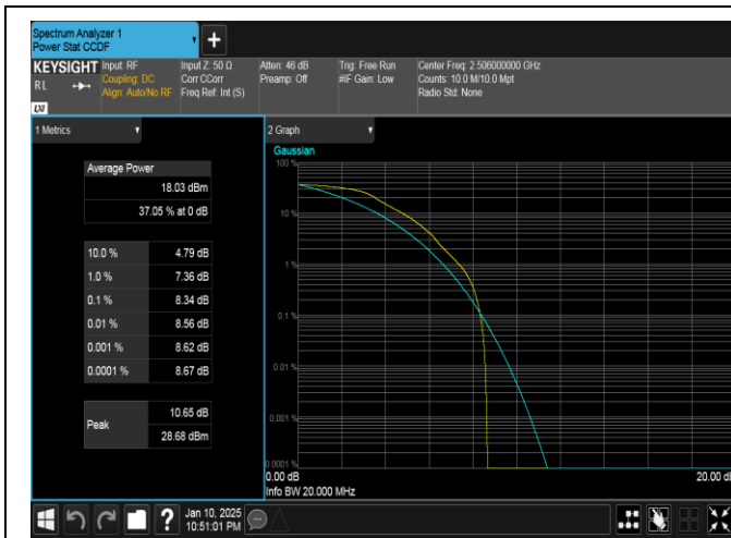
Band41-20MHz-QPSK-39750-1RB#0-PASS
