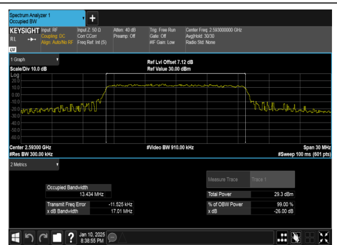
Band41-15MHz-QPSK-40620-75RB#0-PASS
