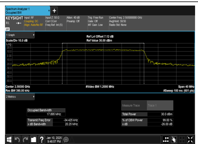
Band41-20MHz-QPSK-40620-100RB#0-PASS
