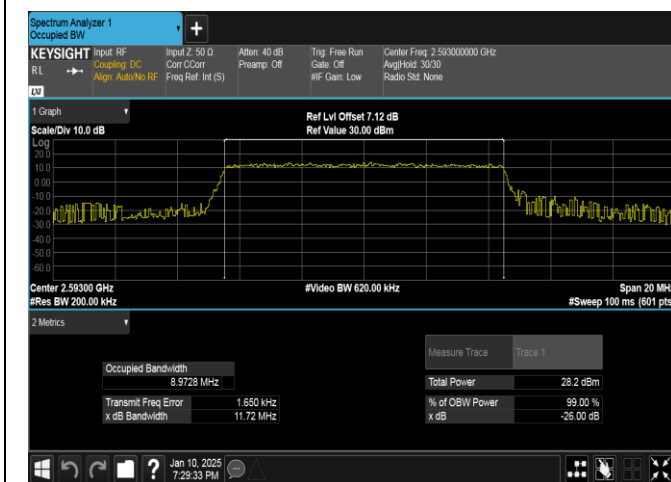
Band41-10MHz-16QAM-40620-50RB#0-PASS
