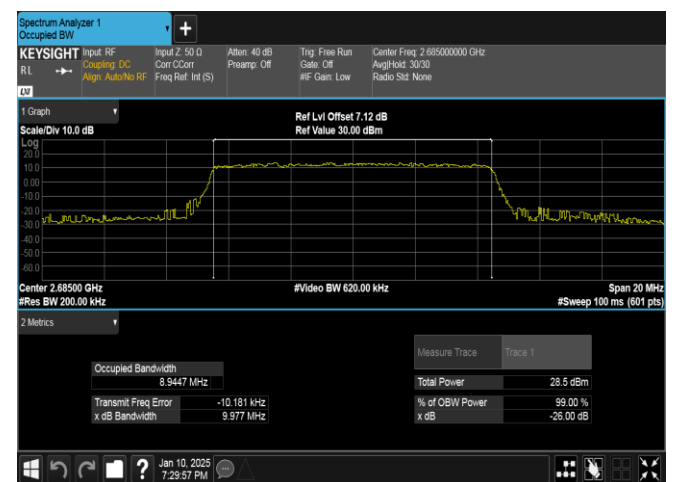
Band41-10MHz-16QAM-41540-50RB#0-PASS
