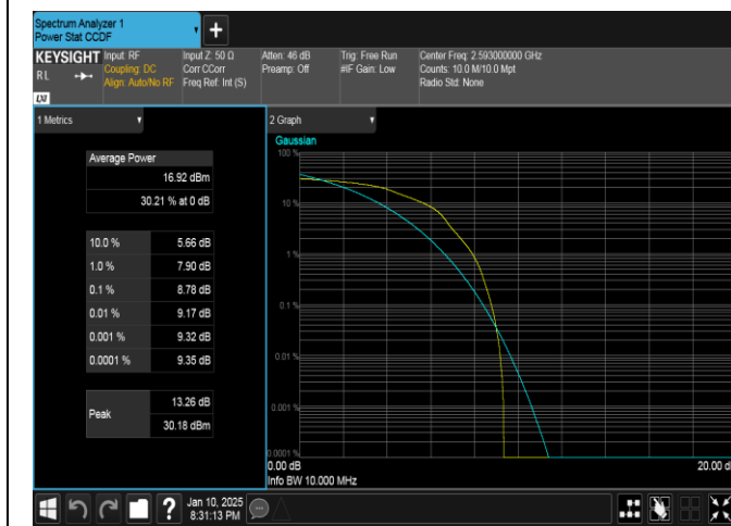
Band41-10MHz-16QAM-40620-1RB#0-PASS
