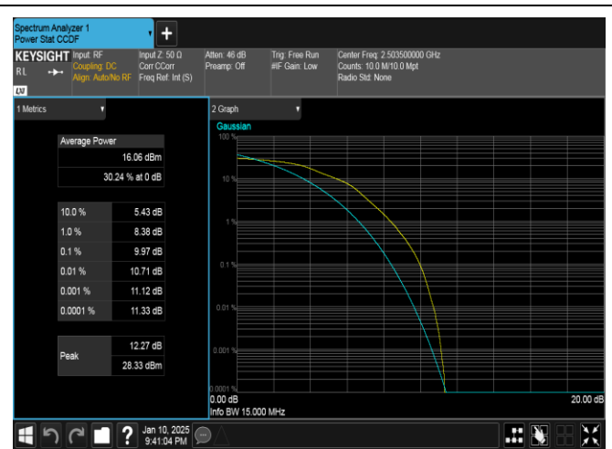
Band41-15MHz-16QAM-39725-75RB#0-PASS
