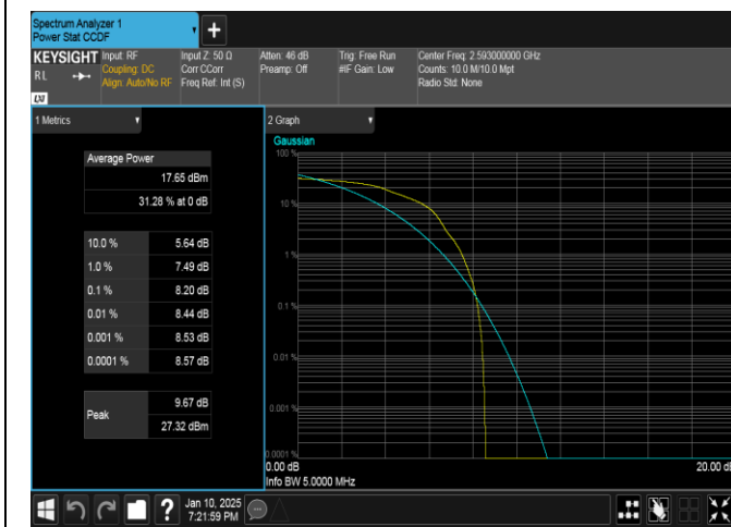
Band41-5MHz-16QAM-40620-1RB#0-PASS
