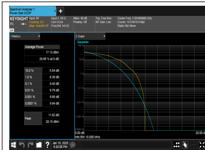
Band41-10MHz-16QAM-39700-1RB#0-PASS
