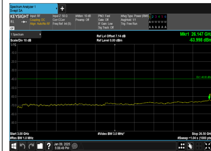
Band40(2350-2360)-5MHz-16QAM-39200-25RB#0-3000~26500-PASS
