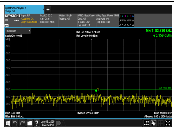
Band40(2350-2360)-10MHz-16QAM-39200-50RB#0-0.009-0.15-PASS
