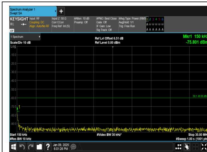
Band40(2350-2360)-10MHz-QPSK-39200-1RB#49-0.15~30-PASS
