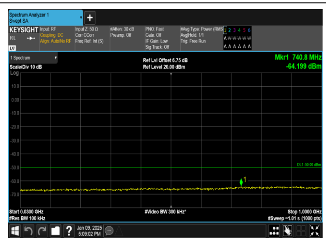
Band40(2350-2360)-5MHz-QPSK-39225-1RB#24-30~1000-PASS
