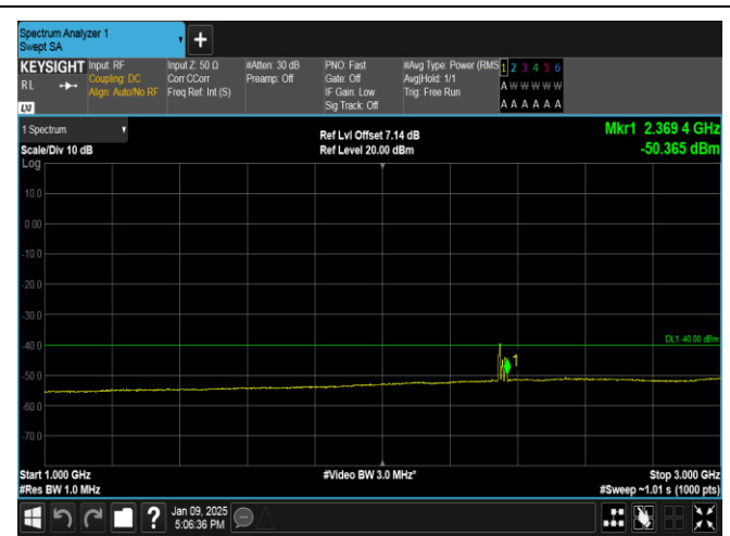
Band40(2350-2360)-5MHz-16QAM-39200-25RB#0-1000~3000-PASS
