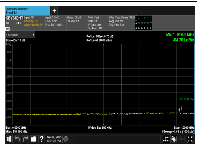
Band40(2350-2360)-10MHz-QPSK-39200-1RB#49-30~1000-PASS
