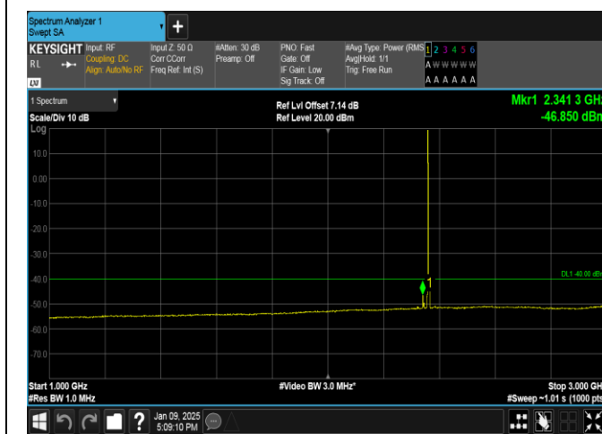
Band40(2350-2360)-5MHz-QPSK-39225-1RB#24-1000~3000-PASS
