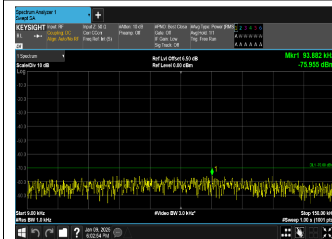
Band40(2350-2360)-10MHz-QPSK-39200-50RB#0-0.009~0.15-PASS
