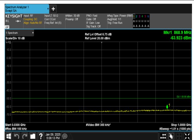
Band40(2350-2360)-5MHz-16QAM-39225-1RB#0-30~1000-PASS
