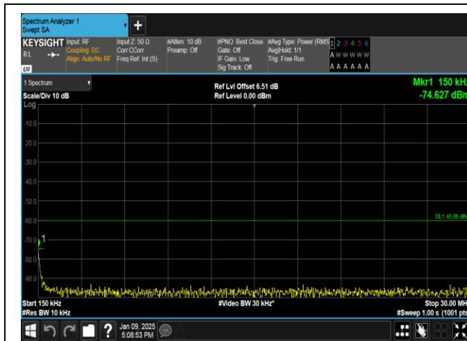
Band40(2350-2360)-5MHz-QPSK-39225-1RB#24-0.15~30-PASS
