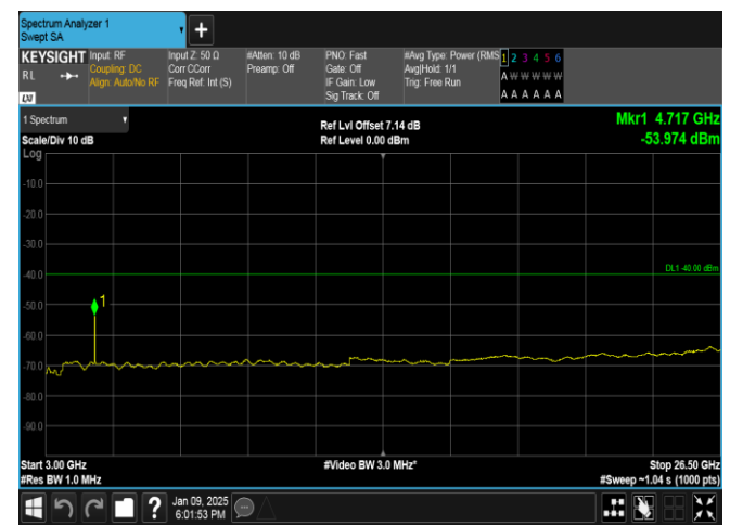
Band40(2350-2360)-10MHz-QPSK-39200-1RB#49-3000~26500-PASS
