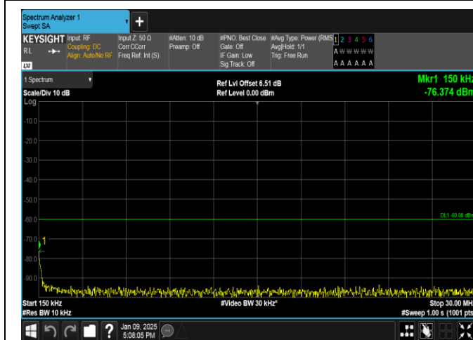
Band40(2350-2360)-5MHz-16QAM-39225-1RB#0-0.15~30-PASS
