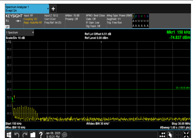
Band40(2350-2360)-5MHz-QPSK-39225-25RB#0-0.15~30-PASS
