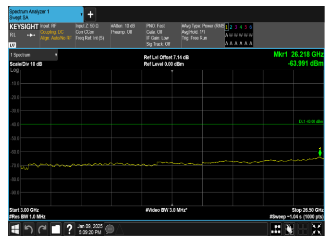
Band40(2350-2360)-5MHz-QPSK-39225-1RB#24-3000~26500-PASS
