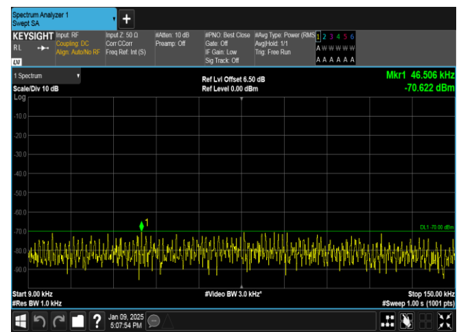
Band40(2350-2360)-5MHz-16QAM-39225-1RB#0-0.009~0.15-PASS
