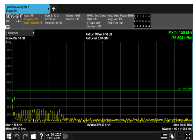
Band40(2350-2360)-10MHz-QPSK-39200-50RB#0-0.15~30-PASS
