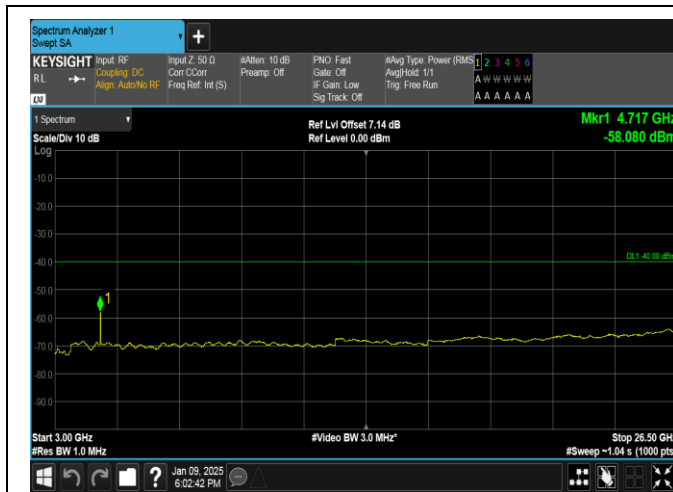
Band40(2350-2360)-10MHz-16QAM-39200-1RB#49-3000-26500-PASS
