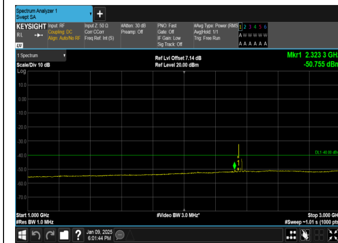
Band40(2350-2360)-10MHz-QPSK-39200-1RB#49-1000~3000-PASS
