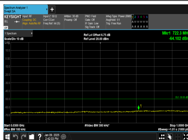
Band40(2305-2315)-5MHz-16QAM-38725-1RB#0-30~1000-PASS
