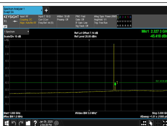
Band40(2305-2315)-5MHz-QPSK-38775-25RB#0-1000~3000-PASS
