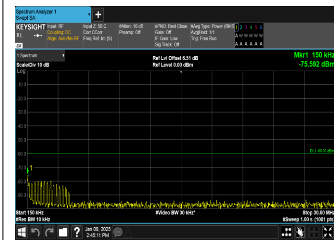
Band40(2305-2315)-5MHz-16QAM-38725-25RB#0-0.15~30-PASS
