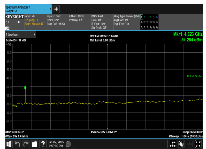
Band40(2305-2315)-5MHz-QPSK-38775-1RB#24-3000~26500-PASS
