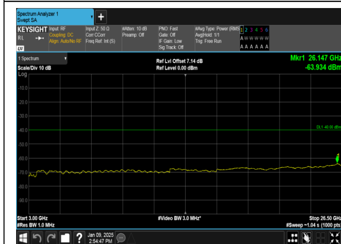
Band40(2305-2315)-5MHz-QPSK-38775-25RB#0-3000~26500-PASS
