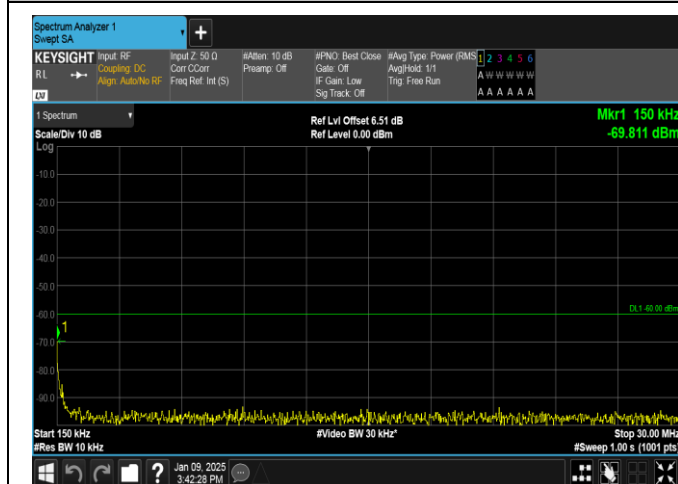
Band40(2305-2315)-10MHz-16QAM-38750-1RB#0-0.15~30-PASS
