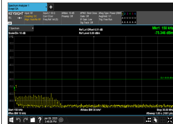
Band40(2305-2315)-10MHz-16QAM-38750-50RB#0-0.15~30-PASS
