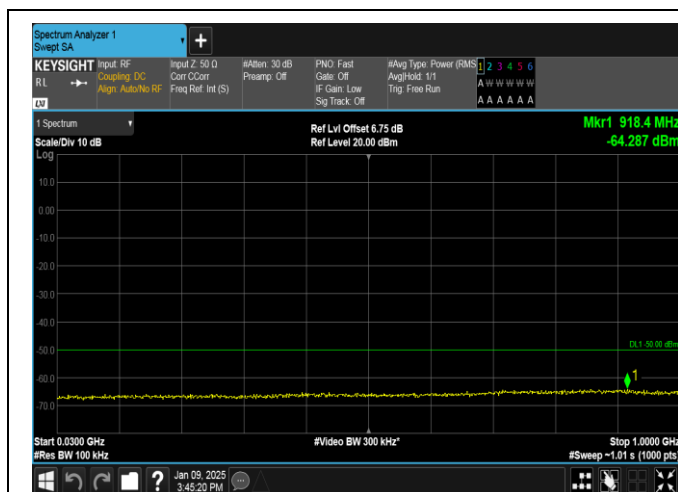
Band40(2305-2315)-10MHz-QPSK-38750-50RB#0-30~1000-PASS
