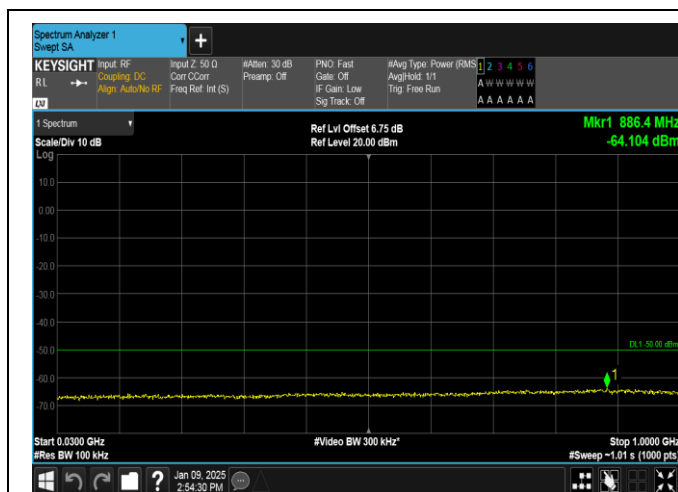
Band40(2305-2315)-5MHz-QPSK-38775-25RB#0-30~1000-PASS
