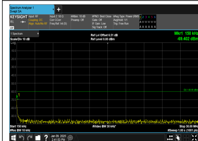
Band40(2305-2315)-5MHz-16QAM-38725-1RB#0-0.15~30-PASS
