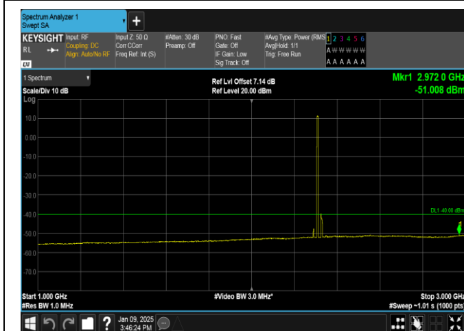
Band40(2305-2315)-10MHz-16QAM-38750-50RB#0-1000~3000-PASS
