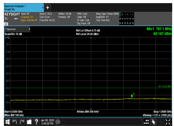
Band40(2305-2315)-5MHz-16QAM-38725-25RB#0-30~1000-PASS
