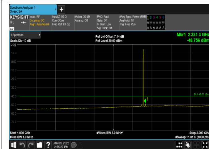
Band40(2305-2315)-5MHz-16QAM-38775-25RB#0-1000~3000-PASS
