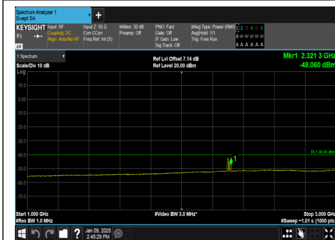
Band40(2305-2315)-5MHz-16QAM-38725-25RB#0-1000~3000-PASS
