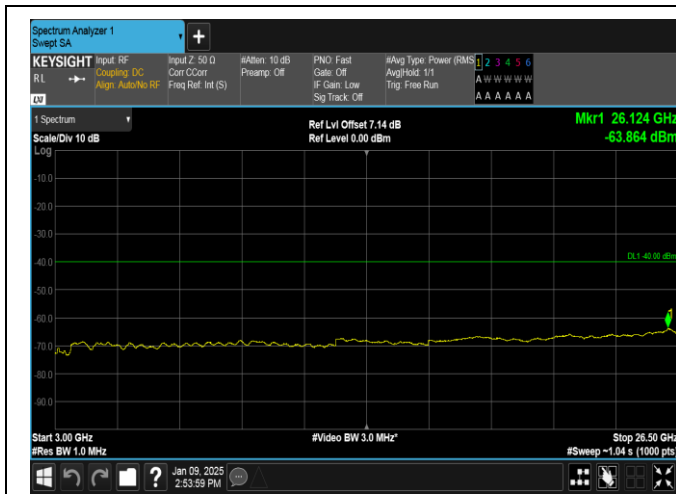
Band40(2305-2315)-5MHz-16QAM-38775-1RB#24-3000~26500-PASS
