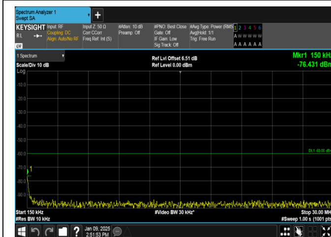
Band40(2305-2315)-5MHz-16QAM-38775-1RB#0-0.15~30-PASS
