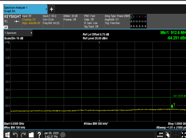
Band40(2305-2315)-10MHz-16QAM-38750-1RB#0-30~1000-PASS
