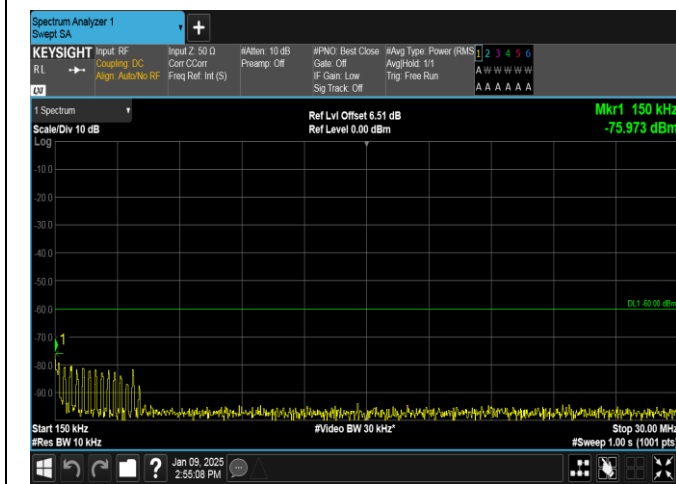
Band40(2305-2315)-5MHz-16QAM-38775-25RB#0-0.15~30-PASS
