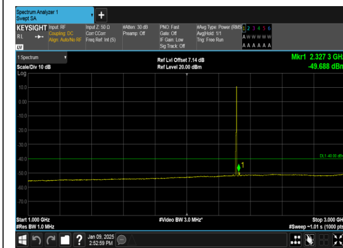
Band40(2305-2315)-5MHz-QPSK-38775-1RB#24-1000~3000-PASS
