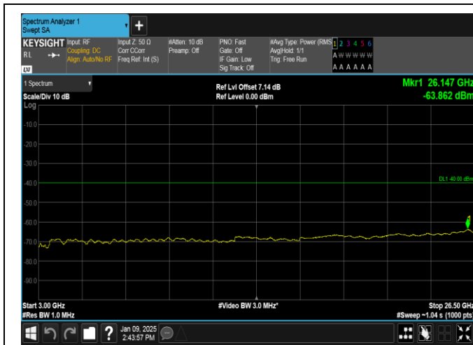
Band40(2305-2315)-5MHz-16QAM-38725-1RB#24-3000~26500-PASS
