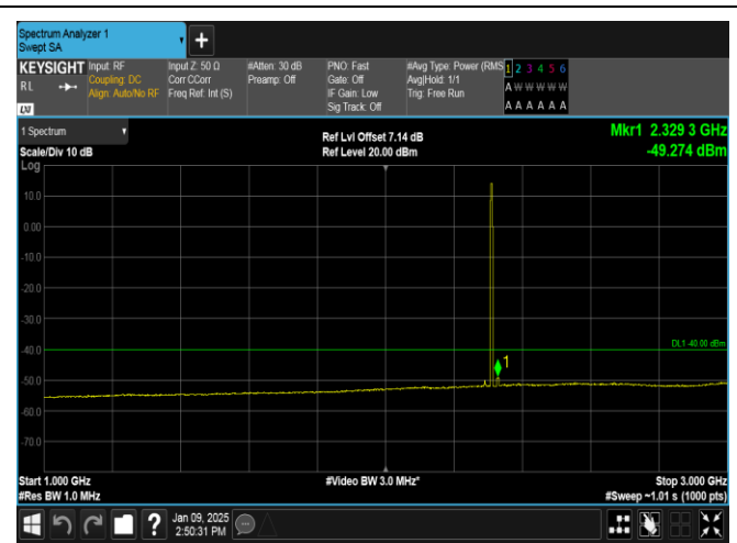
Band40(2305-2315)-5MHz-16QAM-38750-25RB#0-1000~3000-PASS
