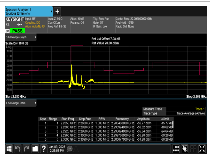
Band40(2305-2315)-5MHz-16QAM-38775-1RB#0-PASS
