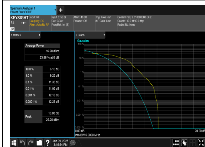
Band40(2305-2315)-5MHz-16QAM-38750-1RB#0-PASS
