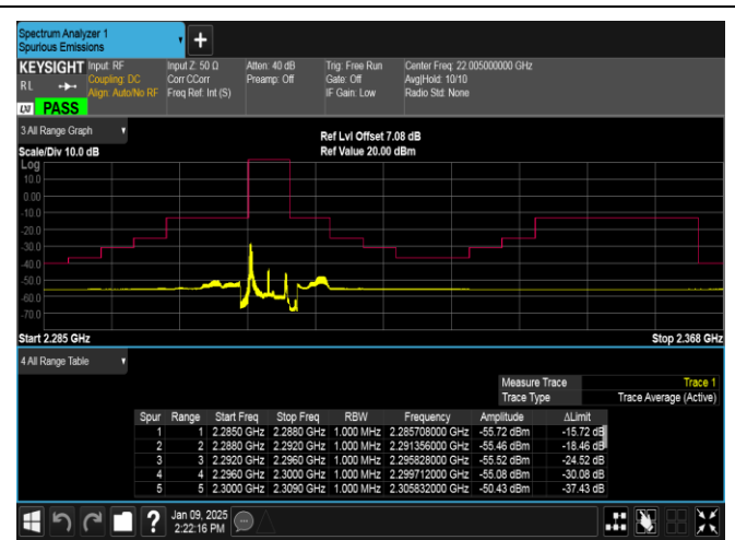
Band40(2305-2315)-5MHz-QPSK-38775-1RB#0-PASS
