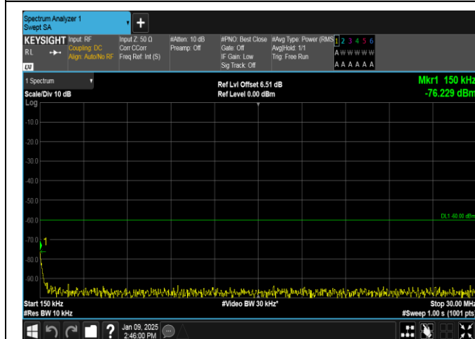
Band40(2305-2315)-5MHz-QPSK-38750-1RB#0-0.15~30-PASS
