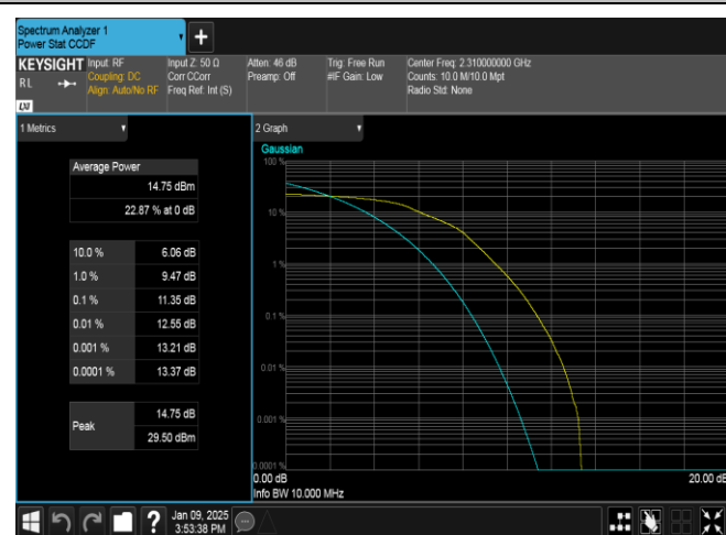
Band40(2305-2315)-10MHz-16QAM-38750-50RB#0-PASS
