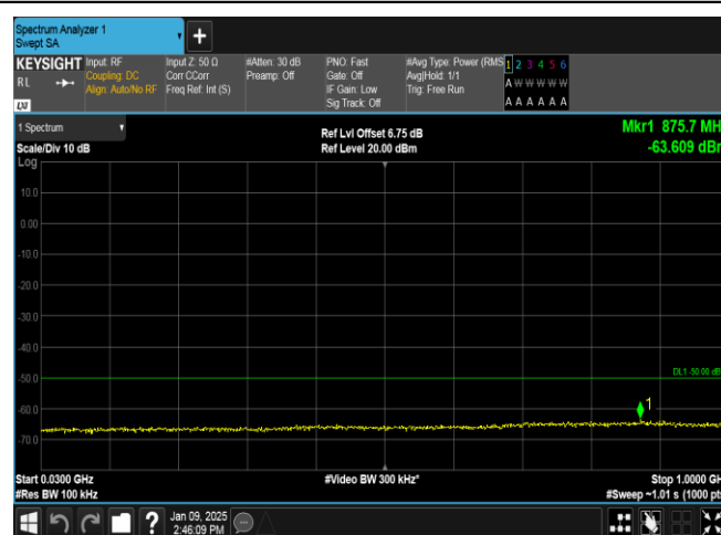
Band40(2305-2315)-5MHz-QPSK-38750-1RB#0-30~1000-PASS
