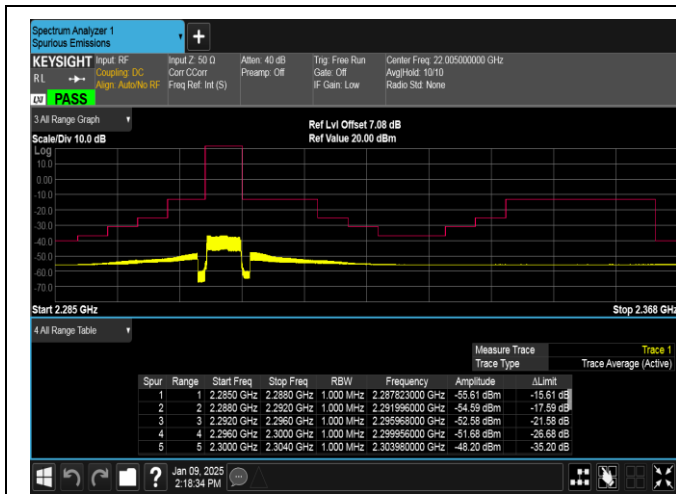
Band40(2305-2315)-5MHz-16QAM-38725-25RB#0-PASS
