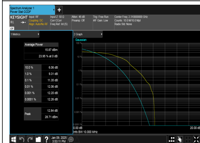
Band40(2305-2315)-10MHz-16QAM-38750-1RB#0-PASS
