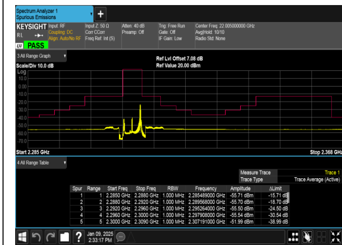
Band40(2305-2315)-5MHz-16QAM-38775-1RB#24-PASS
