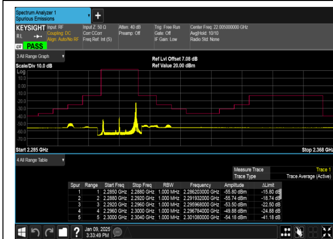
Band40(2305-2315)-10MHz-16QAM-38750-1RB#49-PASS
