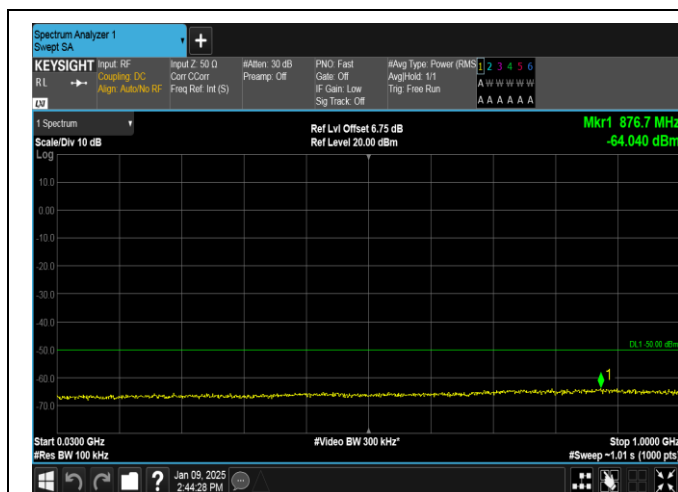
Band40(2305-2315)-5MHz-QPSK-38725-25RB#0-30~1000-PASS
