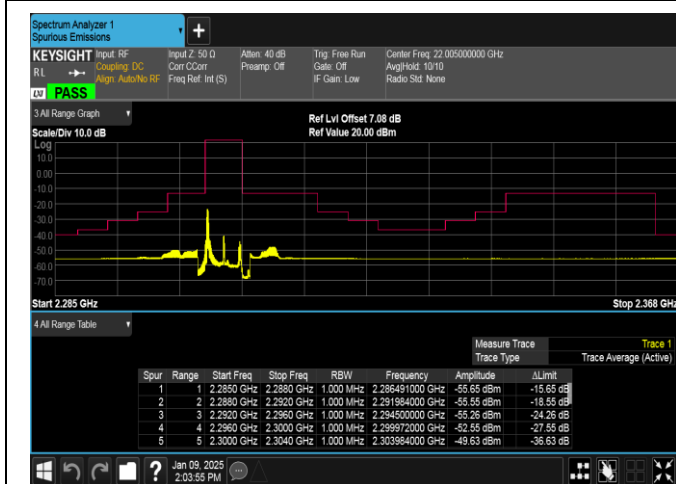
Band40(2305-2315)-5MHz-16QAM-38725-1RB#0-PASS
