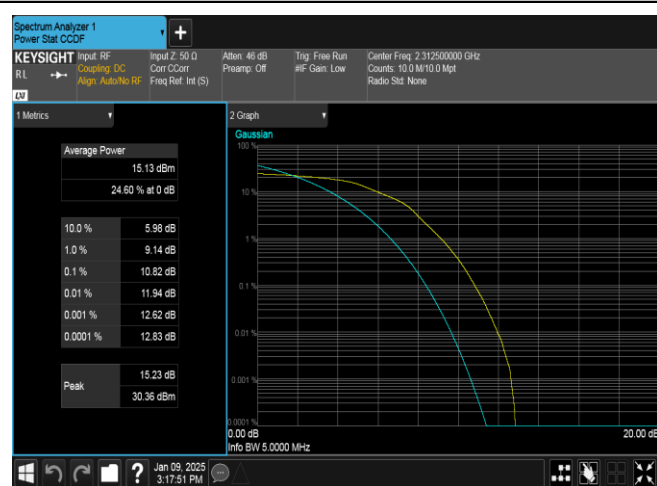
Band40(2305-2315)-5MHz-16QAM-38775-25RB#0-PASS
