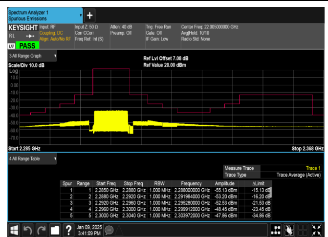
Band40(2305-2315)-10MHz-16QAM-38750-50RB#0-PASS
