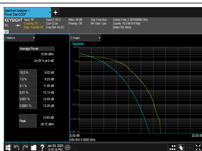
Band40(2305-2315)-5MHz-16QAM-38725-25RB#0-PASS
