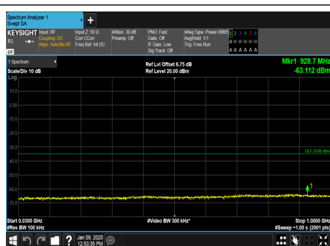
Band38-20MHz-16QAM-38150-100RB#0-30~1000-PASS
