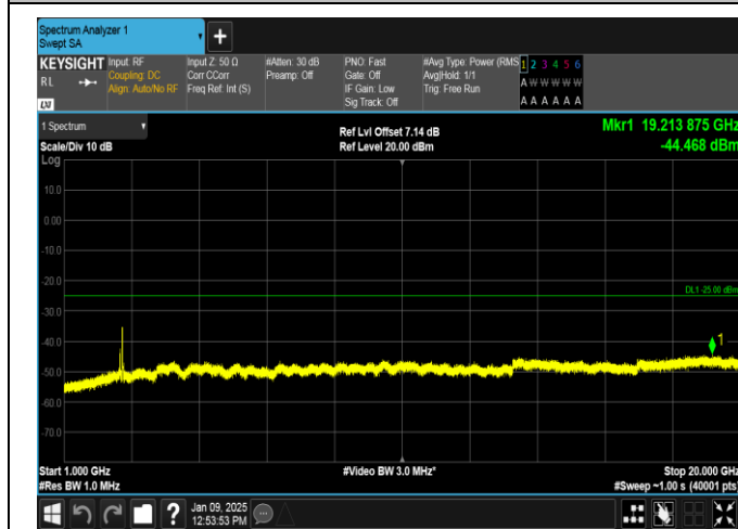
Band38-20MHz-16QAM-38150-100RB#0-1000~20000-PASS
