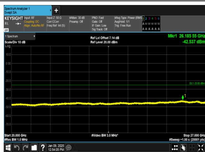
Band38-20MHz-16QAM-38150-100RB#0-20000~27000-PASS
