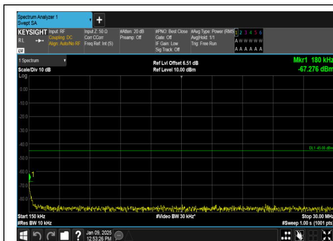
Band38-20MHz-16QAM-38150-100RB#0-0.15~30-PASS
