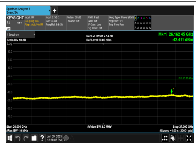
Band38-20MHz-QPSK-37850-1RB#99-20000~27000-PASS
