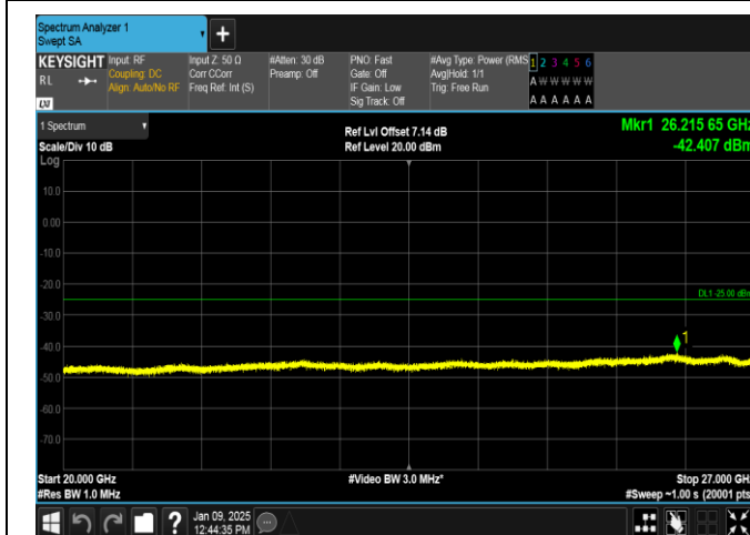
Band38-20MHz-QPSK-38000-1RB#99-20000~27000-PASS
