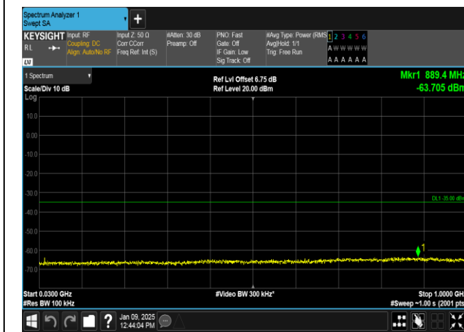
Band38-20MHz-QPSK-38000-1RB#99-30~1000-PASS
