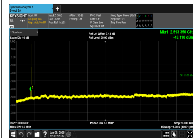
Band38-20MHz-16QAM-37850-1RB#0-1000~20000-PASS
