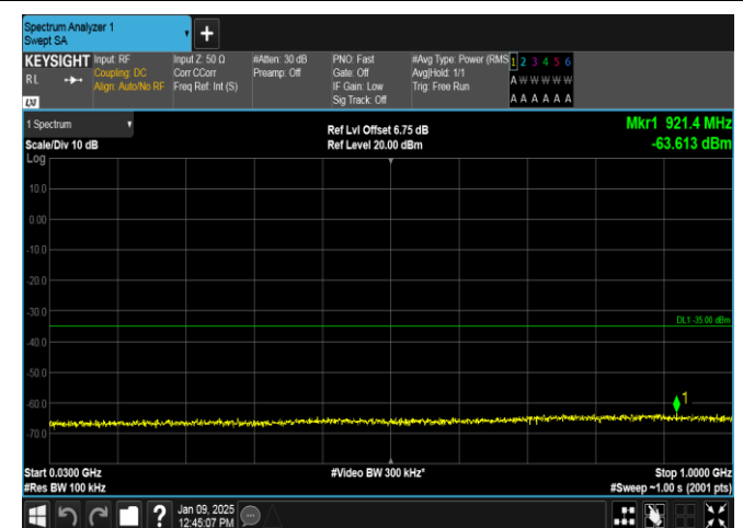
Band38-20MHz-16QAM-38000-1RB#99-30~1000-PASS
