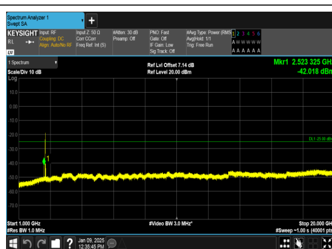
Band38-20MHz-QPSK-37850-1RB#0-1000~20000-PASS
