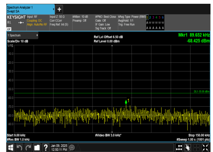
Band38-20MHz-QPSK-38150-1RB#99-0.009~0.15-PASS
