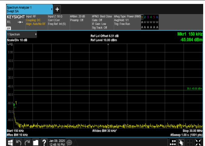
Band38-20MHz-QPSK-38150-1RB#0-0.15~30-PASS
