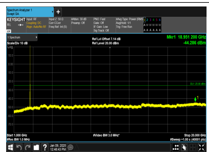
Band38-20MHz-QPSK-38150-1RB#0-1000~20000-PASS
