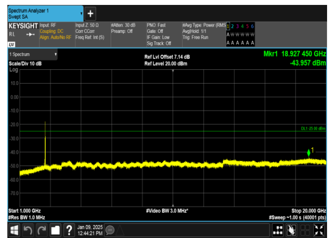
Band38-20MHz-QPSK-38000-1RB#99-1000~20000-PASS
