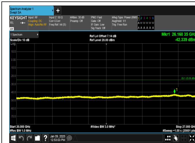
Band38-20MHz-QPSK-38150-100RB#0-20000~27000-PASS
