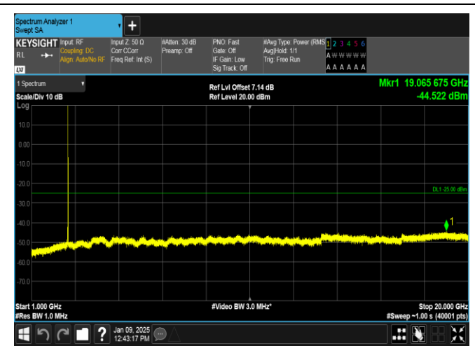
Band38-20MHz-16QAM-38000-1RB#0-1000~20000-PASS
