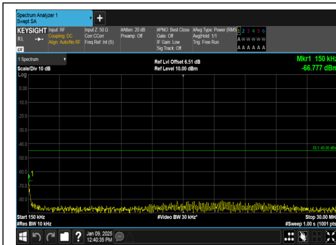
Band38-20MHz-16QAM-37850-100RB#0-0.15~30-PASS
