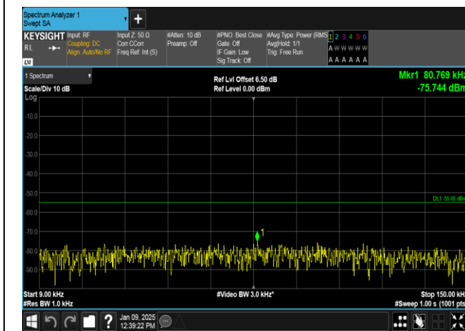
Band38-20MHz-QPSK-37850-100RB#0-0.009~0.15-PASS
