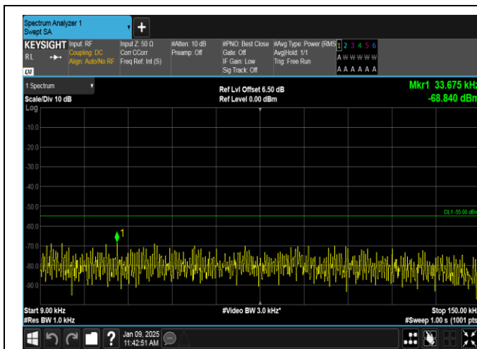
Band38-15MHz-16QAM-38175-1RB#74-0.009~0.15-PASS
