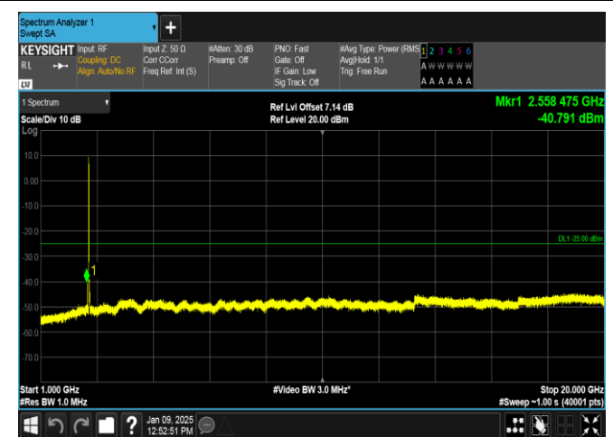
Band38-20MHz-QPSK-38150-100RB#0-1000~20000-PASS
