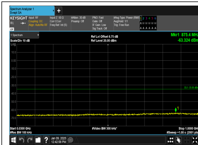
Band38-20MHz-16QAM-38000-1RB#0-30~1000-PASS
