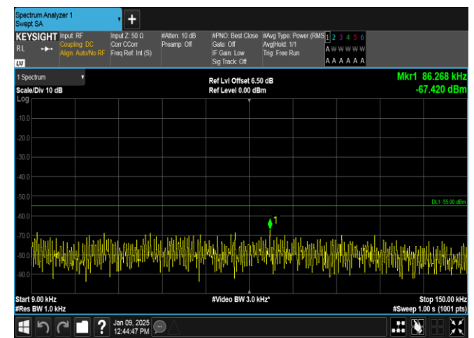
Band38-20MHz-16QAM-38000-1RB#99-0.009~0.15-PASS
