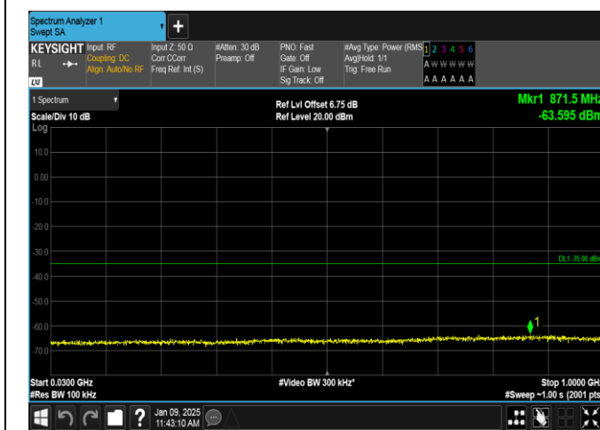
Band38-15MHz-16QAM-38175-1RB#74-30~1000-PASS
