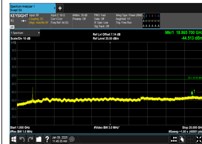
Band38-15MHz-16QAM-38175-75RB#0-1000~20000-PASS
