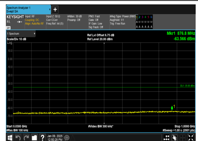
Band38-20MHz-QPSK-38150-1RB#99-30~1000-PASS
