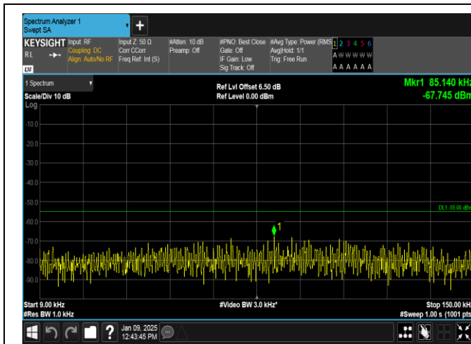
Band38-20MHz-QPSK-38000-1RB#99-0.009~0.15-PASS
