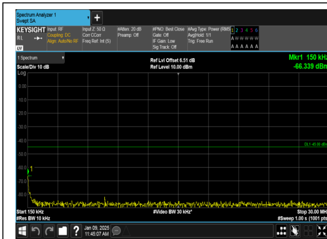
Band38-15MHz-16QAM-38175-75RB#0-0.15~30-PASS
