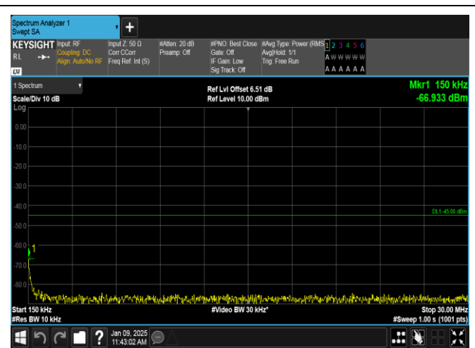
Band38-15MHz-16QAM-38175-1RB#74-0.15~30-PASS
