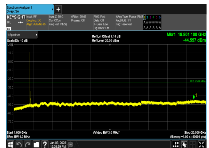
Band38-20MHz-QPSK-37850-100RB#0-1000~20000-PASS
