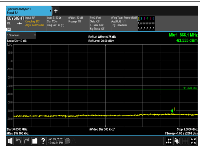
Band38-20MHz-QPSK-38000-100RB#0-30~1000-PASS
