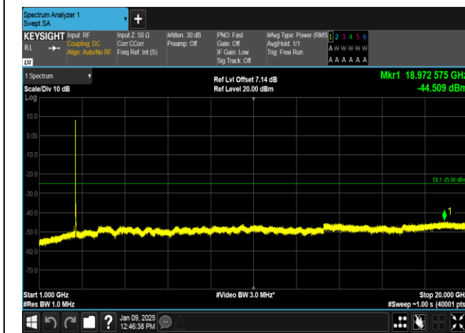
Band38-20MHz-QPSK-38000-100RB#0-1000~20000-PASS
