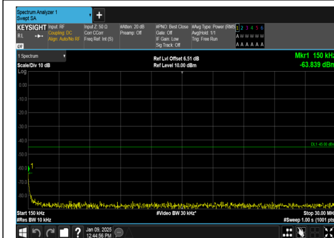
Band38-20MHz-16QAM-38000-1RB#99-0.15~30-PASS
