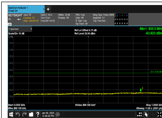
Band38-20MHz-QPSK-38150-1RB#0-30~1000-PASS
