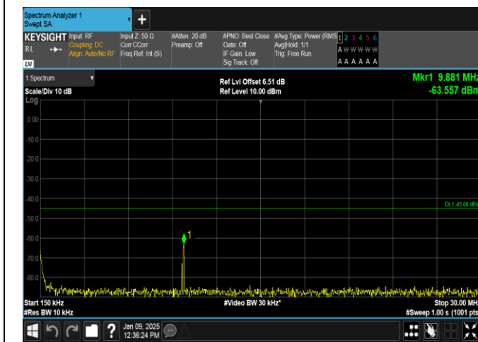
Band38-20MHz-16QAM-37850-1RB#0-0.15~30-PASS
