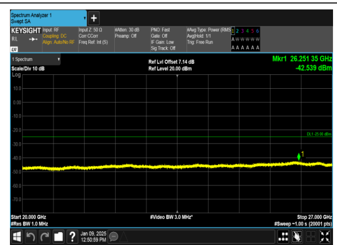
Band38-20MHz-QPSK-38150-1RB#99-20000~27000-PASS
