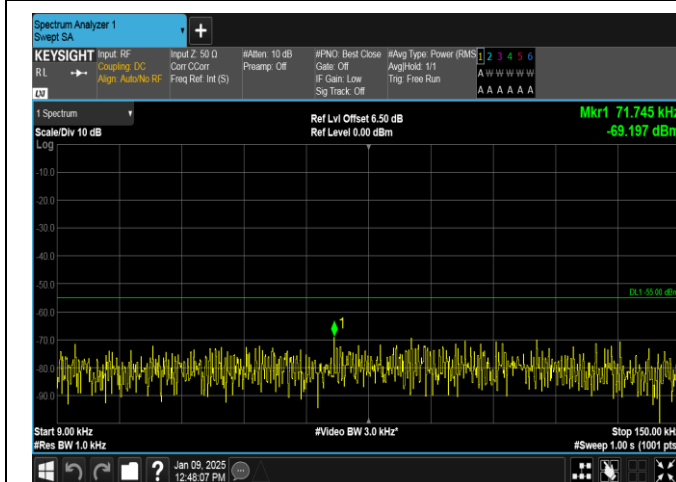
Band38-20MHz-QPSK-38150-1RB#0-0.009~0.15-PASS
