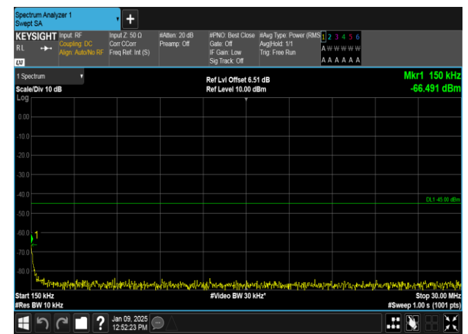
Band38-20MHz-QPSK-38150-100RB#0-0.15~30-PASS
