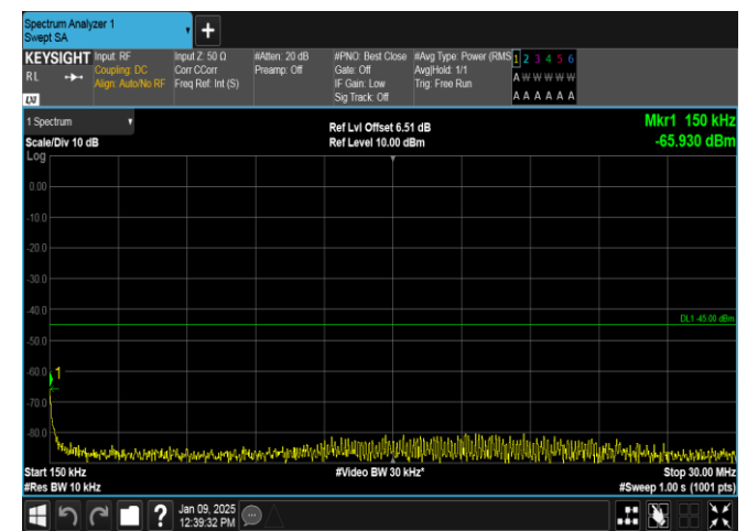
Band38-20MHz-QPSK-37850-100RB#0-0.15~30-PASS
