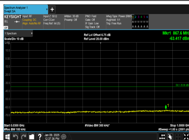
Band38-20MHz-QPSK-37850-1RB#99-30~1000-PASS
