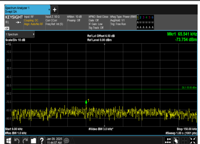
Band38-15MHz-16QAM-38175-75RB#0-0.009~0.15-PASS
