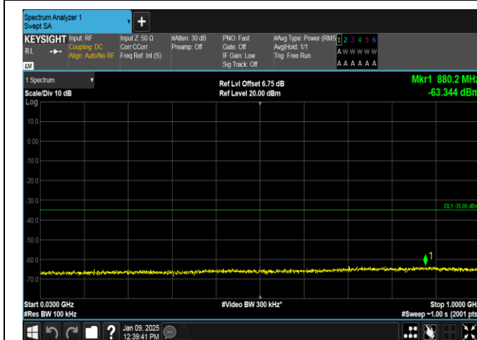
Band38-20MHz-QPSK-37850-100RB#0-30~1000-PASS
