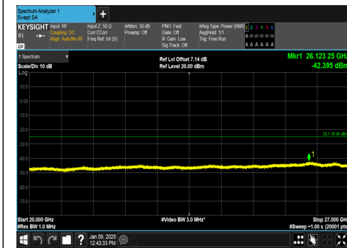
Band38-20MHz-16QAM-38000-1RB#0-20000~27000-PASS
