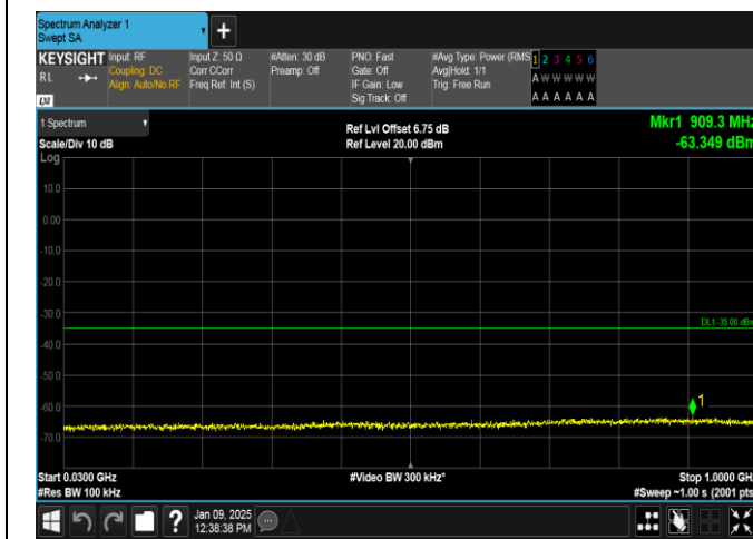
Band38-20MHz-16QAM-37850-1RB#99-30~1000-PASS
