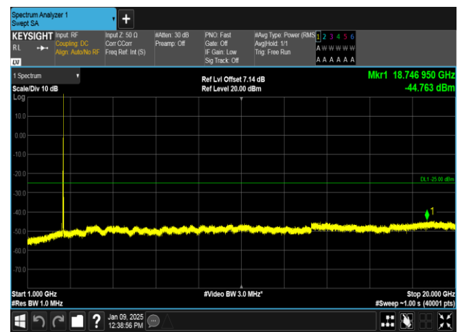
Band38-20MHz-16QAM-37850-1RB#99-1000~20000-PASS
