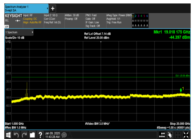
Band38-15MHz-16QAM-38175-1RB#74-1000~20000-PASS
