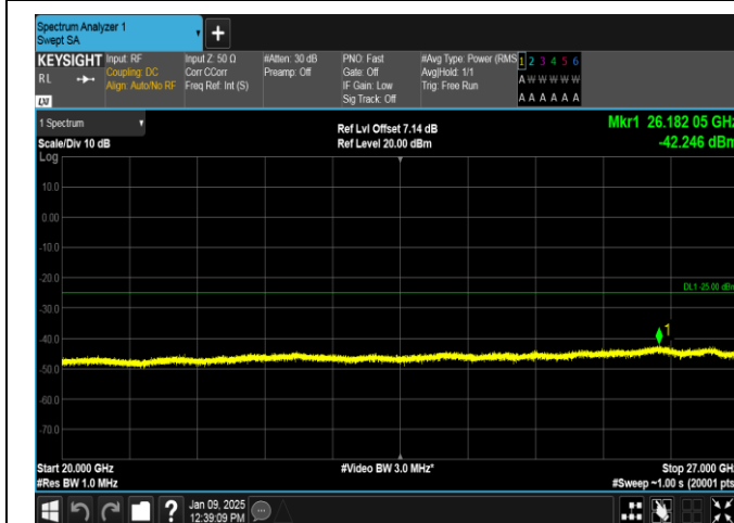
Band38-20MHz-16QAM-37850-1RB#99-20000~27000-PASS
