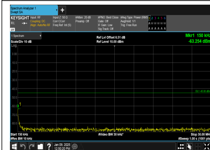
Band38-20MHz-QPSK-38150-1RB#99-0.15~30-PASS
