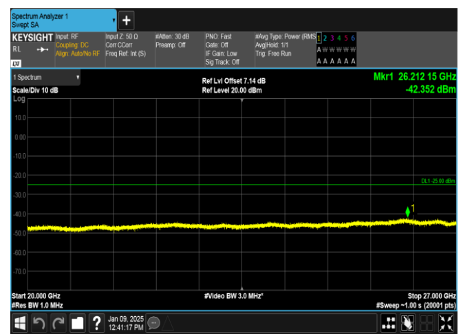
Band38-20MHz-16QAM-37850-100RB#0-20000~27000-PASS
