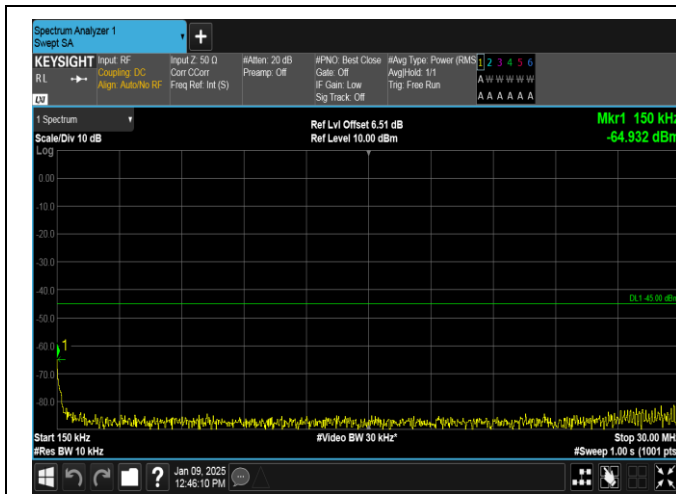
Band38-20MHz-QPSK-38000-100RB#0-0.15~30-PASS
