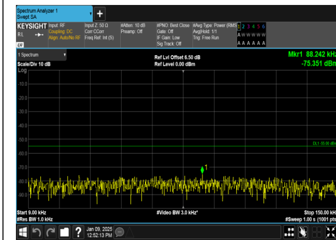
Band38-20MHz-QPSK-38150-100RB#0-0.009~0.15-PASS
