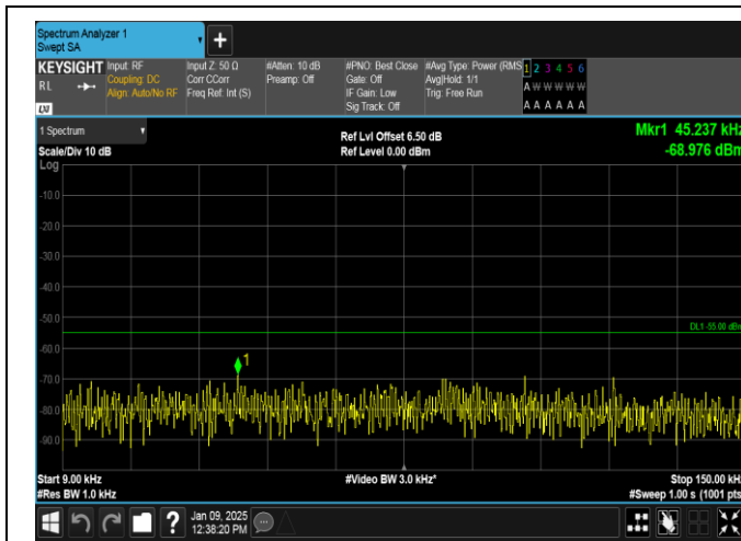
Band38-20MHz-16QAM-37850-1RB#99-0.009~0.15-PASS
