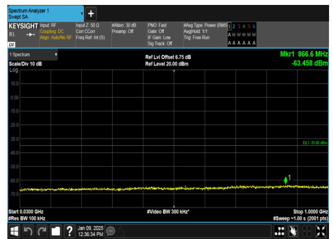
Band38-20MHz-16QAM-37850-1RB#0-30~1000-PASS
