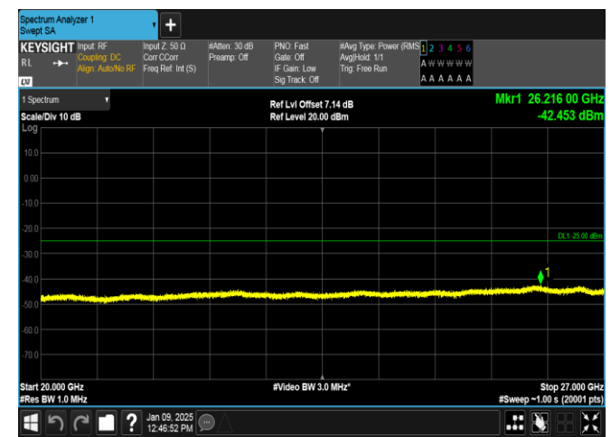
Band38-20MHz-QPSK-38000-100RB#0-20000~27000-PASS
