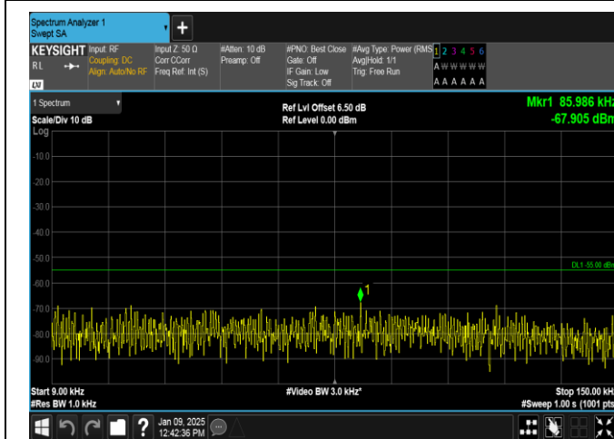
Band38-20MHz-16QAM-38000-1RB#0-0.009~0.15-PASS
