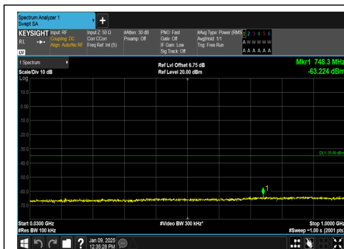
Band38-20MHz-QPSK-37850-1RB#0-30~1000-PASS
