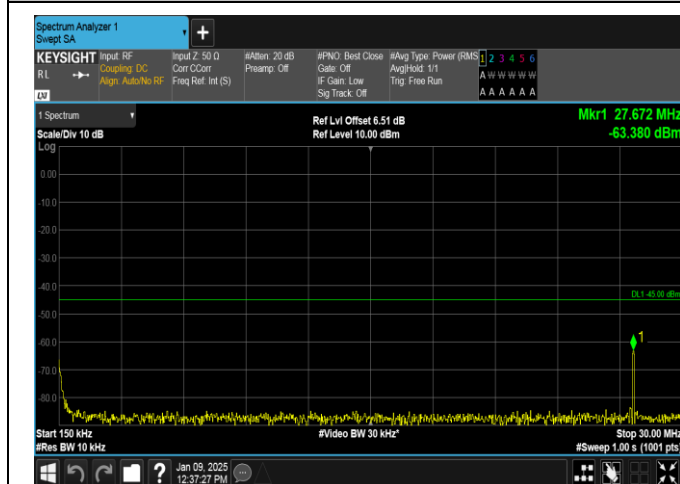
Band38-20MHz-QPSK-37850-1RB#99-0.15~30-PASS
