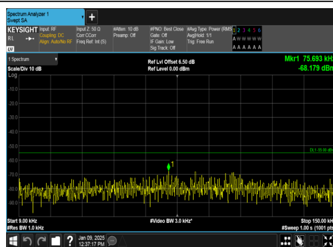
Band38-20MHz-QPSK-37850-1RB#99-0.009~0.15-PASS
