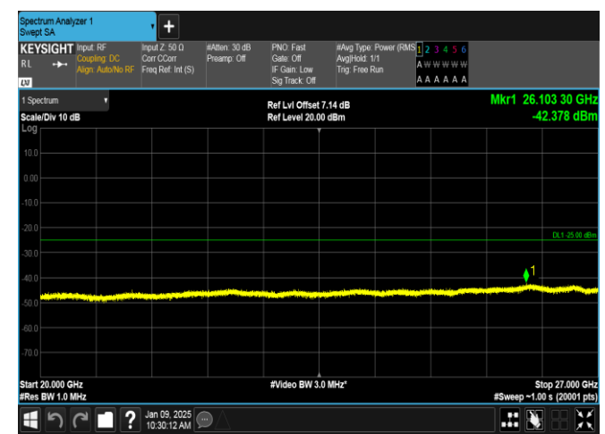
Band38-10MHz-QPSK-38000-50RB#0-20000~27000-PASS
