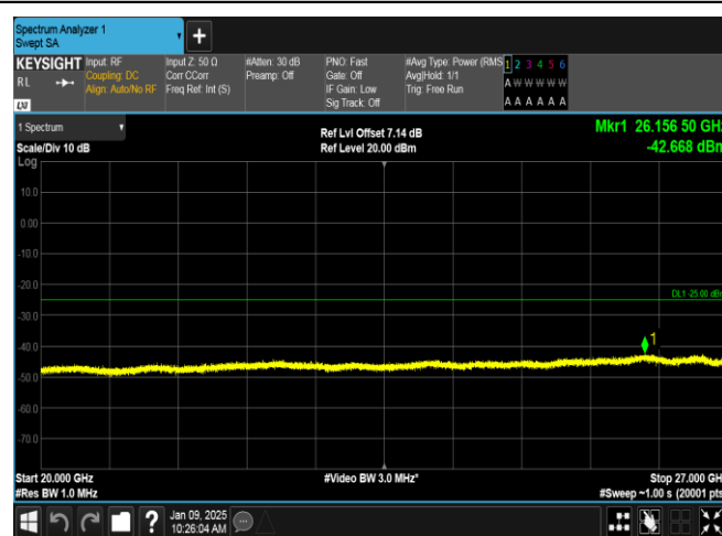
Band38-10MHz-QPSK-38000-1RB#0-20000~27000-PASS
