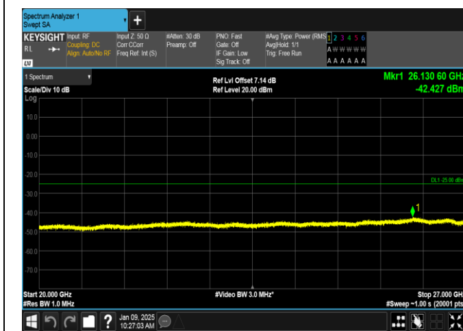
Band38-10MHz-16QAM-38000-1RB#0-20000~27000-PASS
