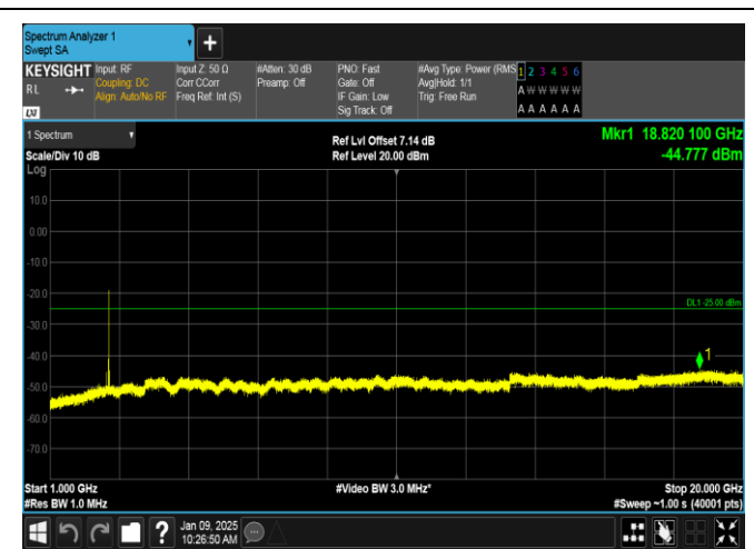
Band38-10MHz-16QAM-38000-1RB#0-1000~20000-PASS
