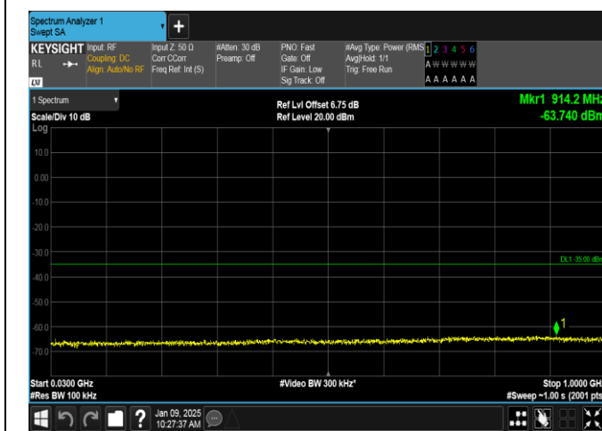
Band38-10MHz-QPSK-38000-1RB#49-30~1000-PASS
