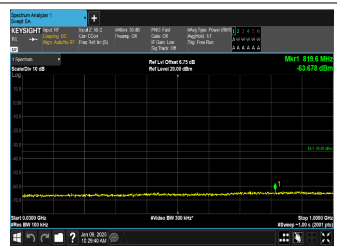
Band38-10MHz-QPSK-38000-50RB#0-30~1000-PASS
