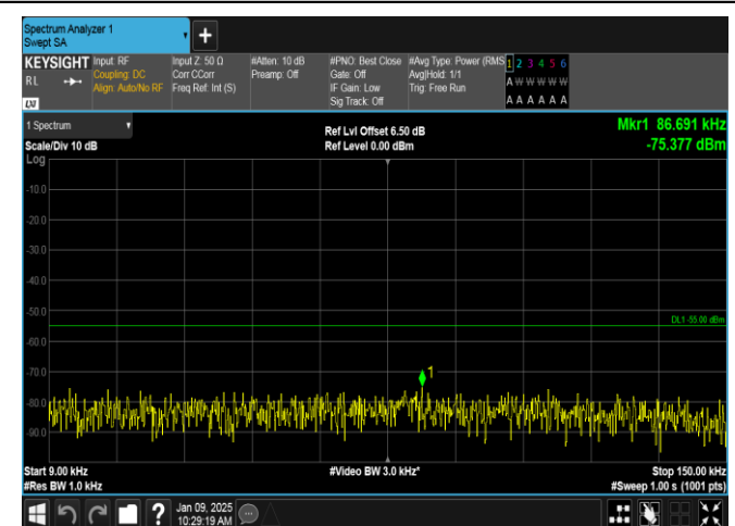
Band38-10MHz-QPSK-38000-50RB#0-0.009~0.15-PASS
