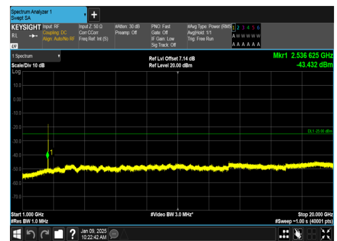
Band38-10MHz-16QAM-37800-1RB#49-1000~20000-PASS
