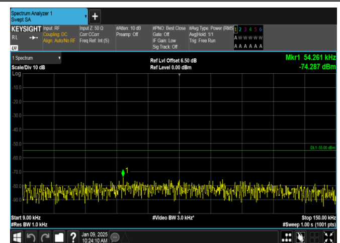
Band38-10MHz-16QAM-37800-50RB#0-0.009~0.15-PASS
