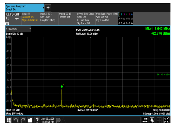
Band38-15MHz-QPSK-37825-1RB#0-0.15~30-PASS
