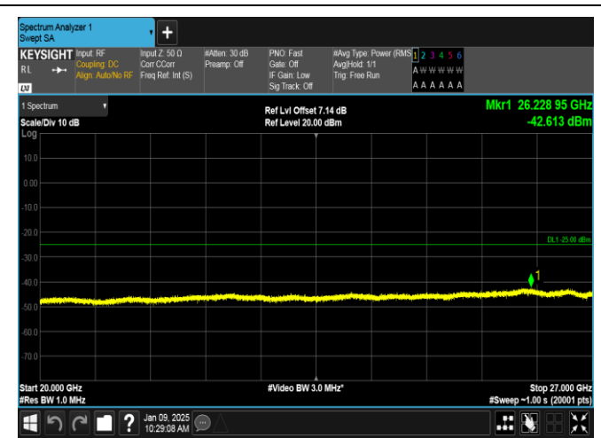
Band38-10MHz-16QAM-38000-1RB#49-20000~27000-PASS
