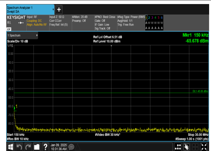
Band38-10MHz-QPSK-38200-1RB#0-0.15~30-PASS
