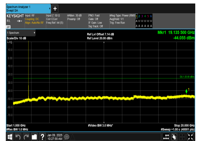
Band38-10MHz-QPSK-38000-1RB#49-1000~20000-PASS
