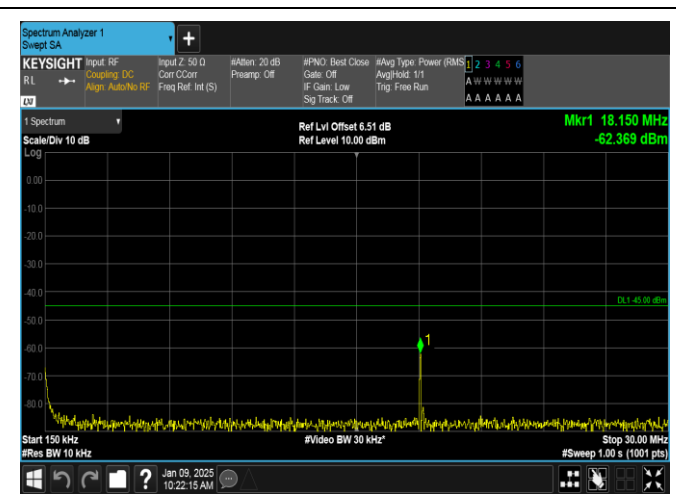
Band38-10MHz-16QAM-37800-1RB#49-0.15~30-PASS
