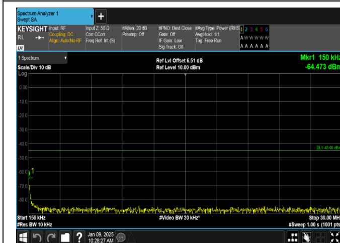
Band38-10MHz-16QAM-38000-1RB#49-0.15~30-PASS
