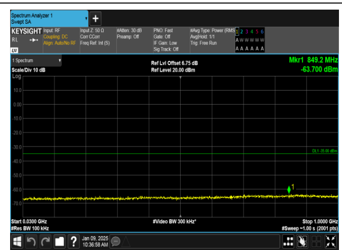
Band38-10MHz-16QAM-38200-50RB#0-30~1000-PASS
