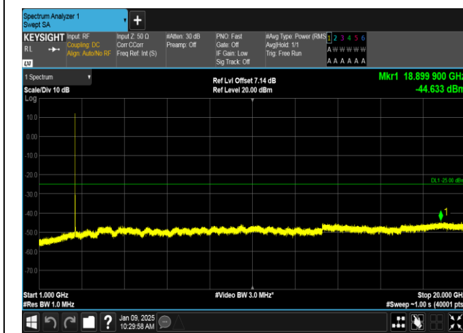
Band38-10MHz-QPSK-38000-50RB#0-1000~20000-PASS
