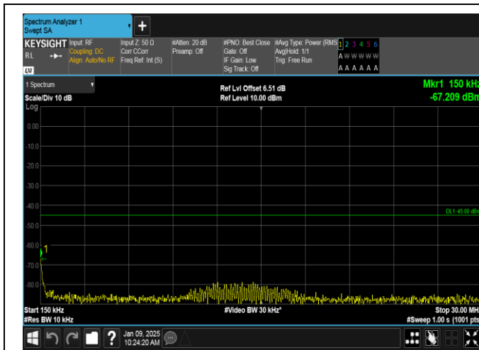
Band38-10MHz-16QAM-37800-50RB#0-0.15~30-PASS
