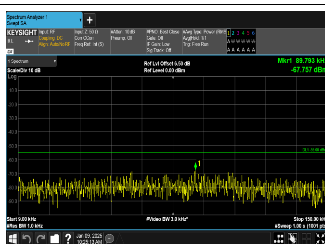
Band38-10MHz-OPSK-38000-1RB#0-0.009~0.15-PASS
