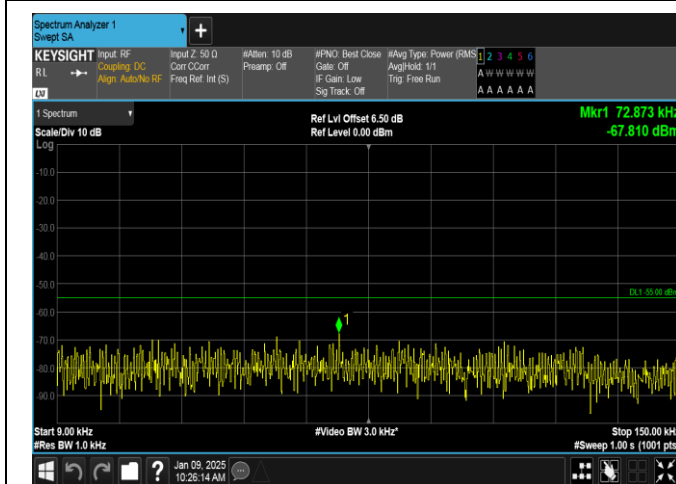
Band38-10MHz-16QAM-38000-1RB#0-0.009~0.15-PASS
