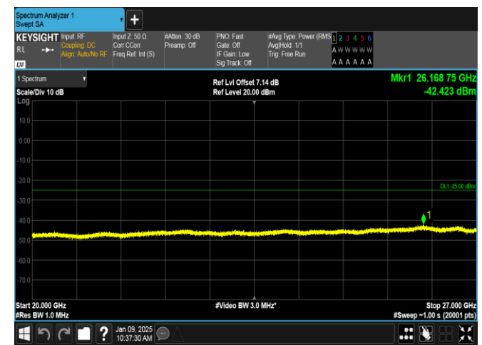
Band38-10MHz-16QAM-38200-50RB#0-20000~27000-PASS
