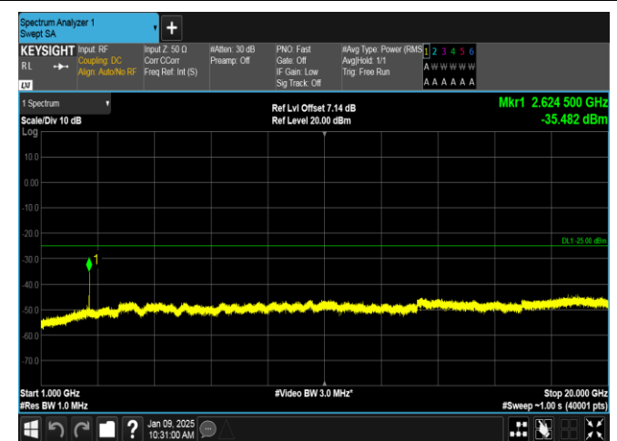
Band38-10MHz-16QAM-38000-50RB#0-1000~20000-PASS
