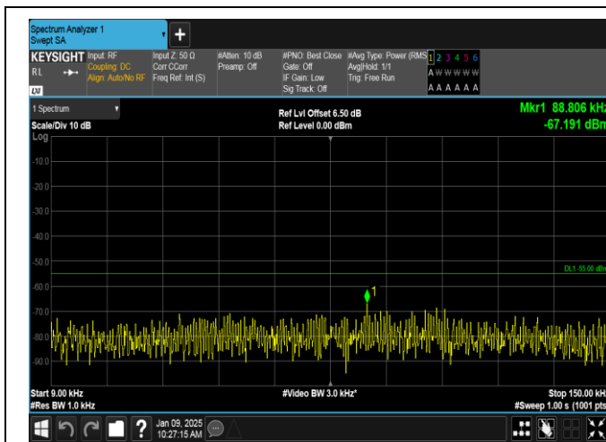
Band38-10MHz-QPSK-38000-1RB#49-0.009~0.15-PASS
