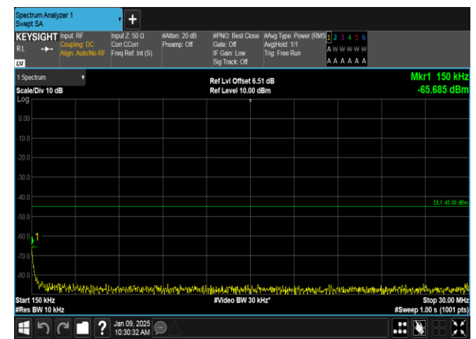
Band38-10MHz-16QAM-38000-50RB#0-0.15~30-PASS
