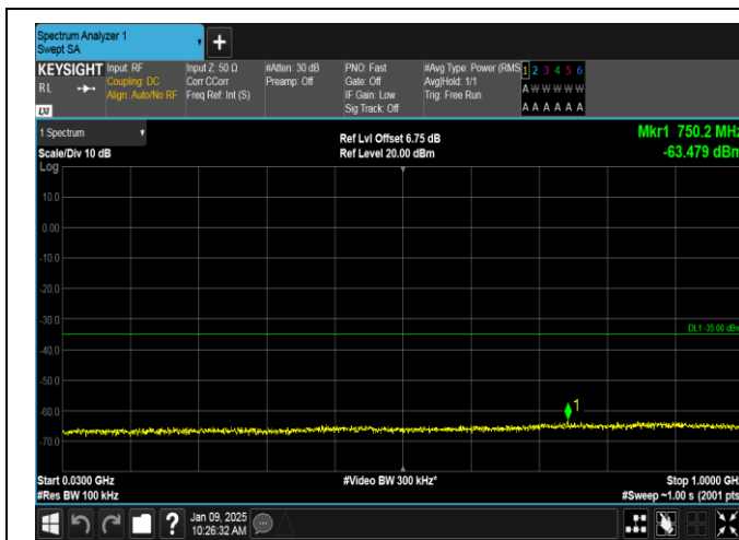
Band38-10MHz-16QAM-38000-1RB#0-30~1000-PASS
