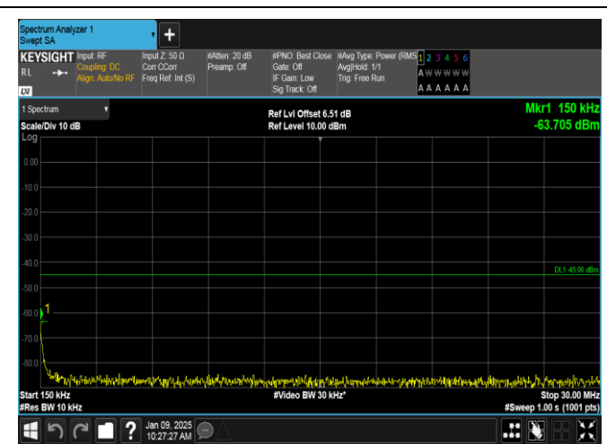
Band38-10MHz-QPSK-38000-1RB#49-0.15~30-PASS
