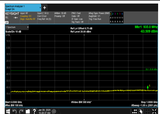
Band38-10MHz-16QAM-38000-1RB#49-30~1000-PASS
