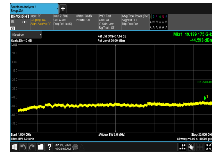
Band38-10MHz-16QAM-37800-50RB#0-1000~20000-PASS
