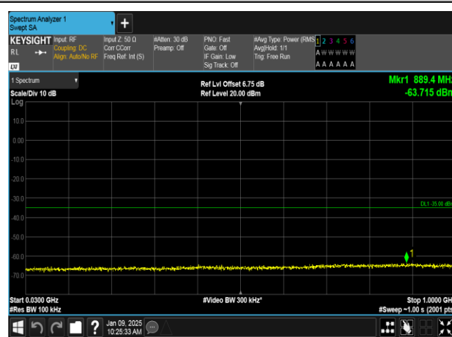
Band38-10MHz-QPSK-38000-1RB#0-30~1000-PASS
