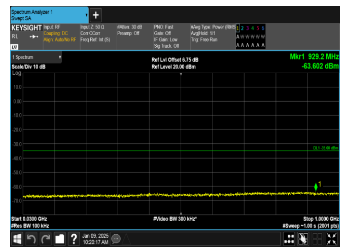
Band38-10MHz-16QAM-37800-1RB#0-30~1000-PASS
