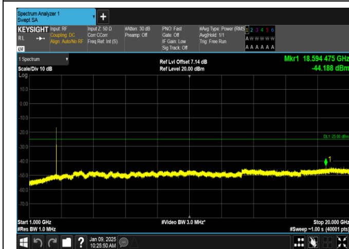
Band38-10MHz-QPSK-38000-1RB#0-1000~20000-PASS
