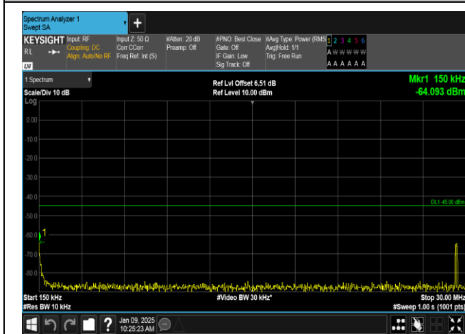
Band38-10MHz-QPSK-38000-1RB#0-0.15~30-PASS
