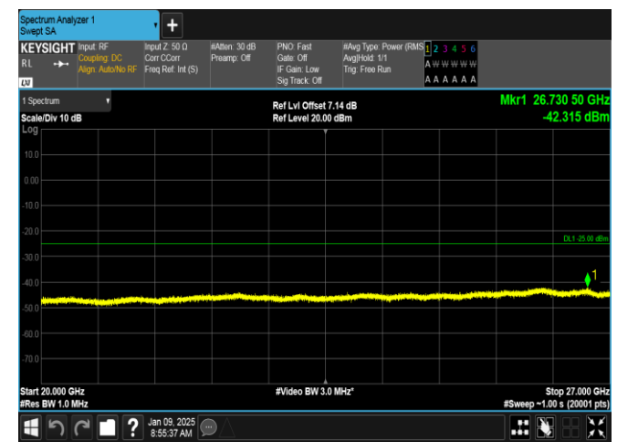
Band38-5MHz-16QAM-37775-25RB#0-20000~27000-PASS
