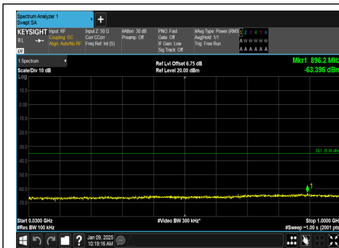
Band38-10MHz-QPSK-37800-1RB#0-30~1000-PASS
