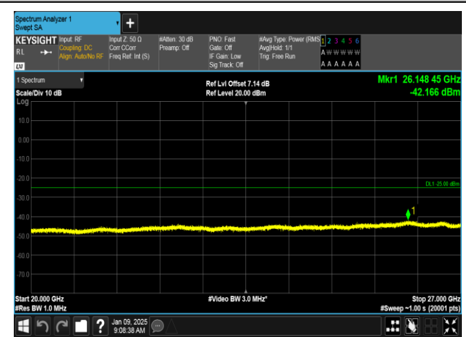
Band38-5MHz-16QAM-38225-25RB#0-20000~27000-PASS
