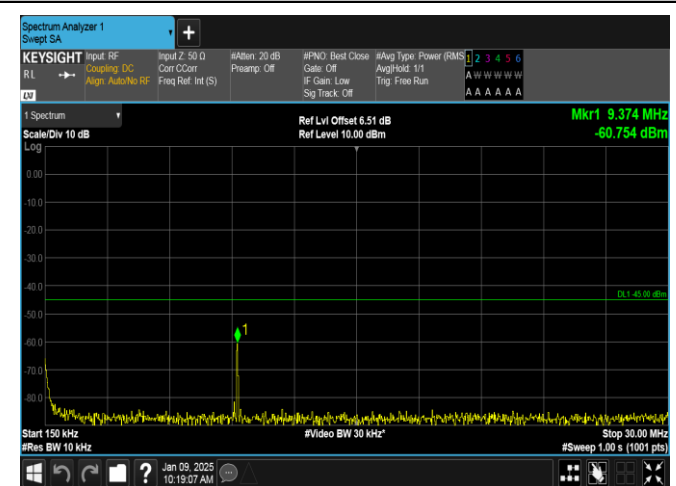
Band38-10MHz-QPSK-37800-1RB#0-0.15~30-PASS
