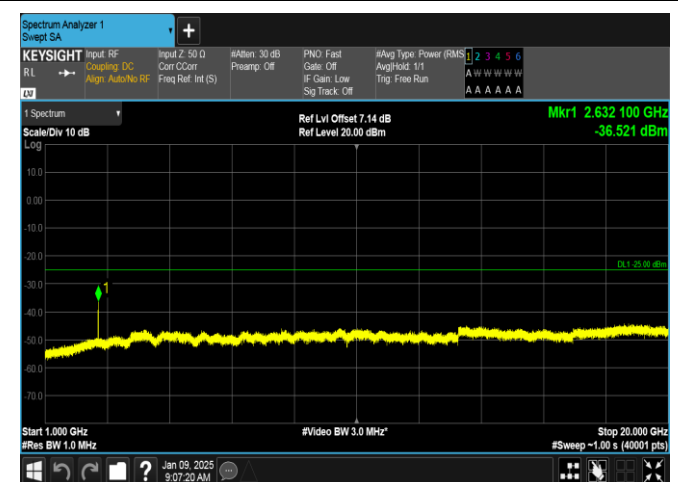
Band38-5MHz-QPSK-38225-25RB#0-1000~20000-PASS
