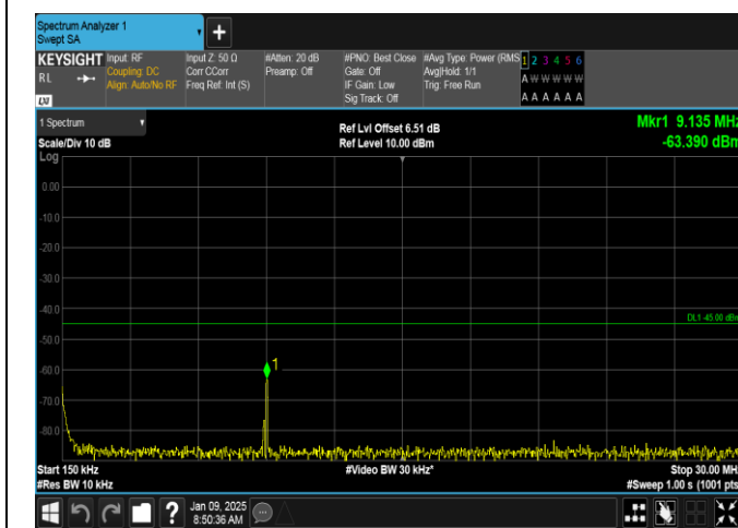
Band38-5MHz-16QAM-37775-1RB#0-0.15~30-PASS
