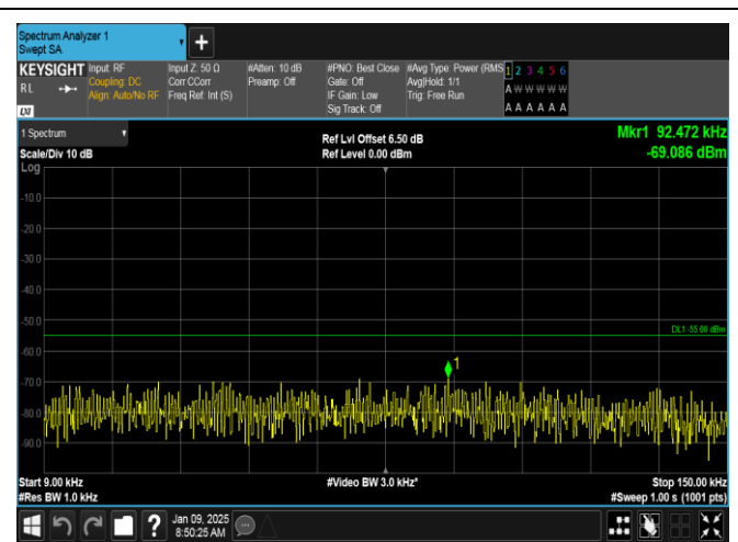
Band38-5MHz-16QAM-37775-1RB#0-0.009~0.15-PASS
