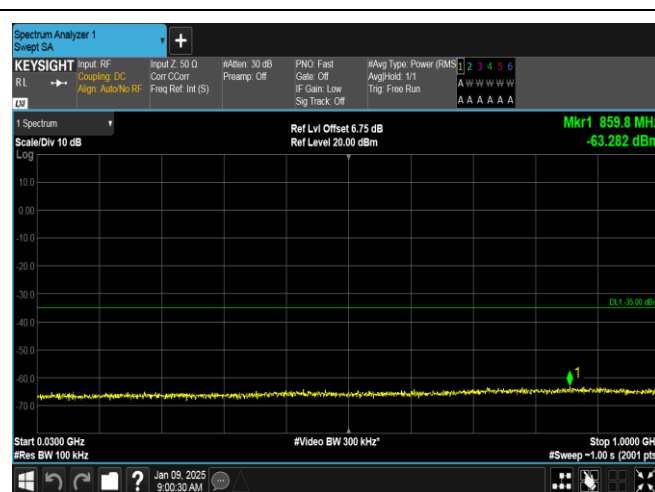
Band38-5MHz-QPSK-38000-25RB#0-30~1000-PASS
