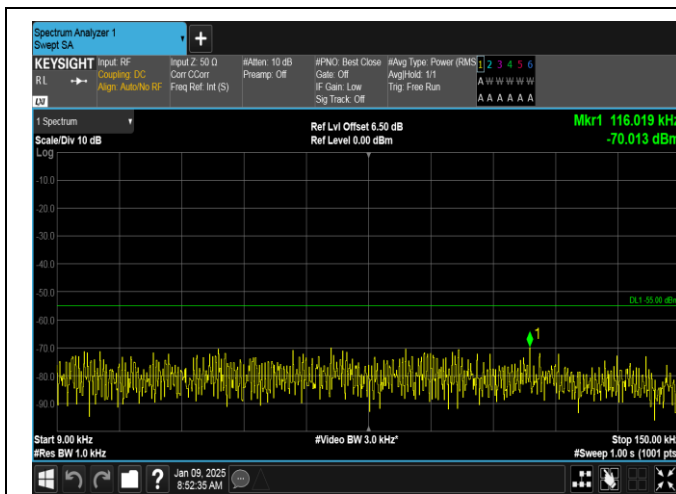
Band38-5MHz-16QAM-37775-1RB#24-0.009~0.15-PASS
