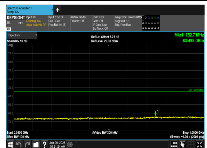
Band38-10MHz-QPSK-37800-1RB#49-30~1000-PASS
