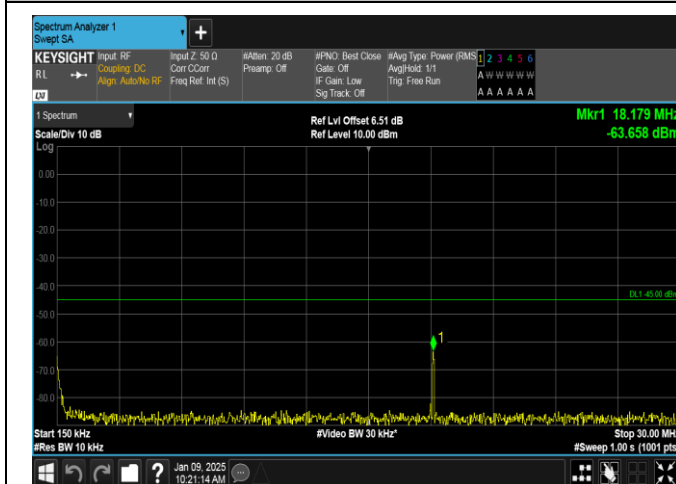
Band38-10MHz-QPSK-37800-1RB#49-0.15~30-PASS
