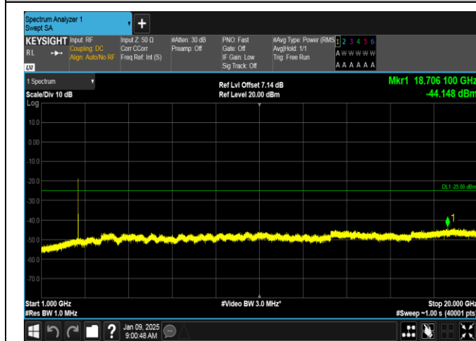
Band38-5MHz-QPSK-38000-25RB#0-1000~20000-PASS
