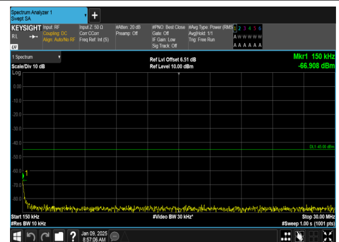
Band38-5MHz-16QAM-38000-1RB#0-0.15~30-PASS
