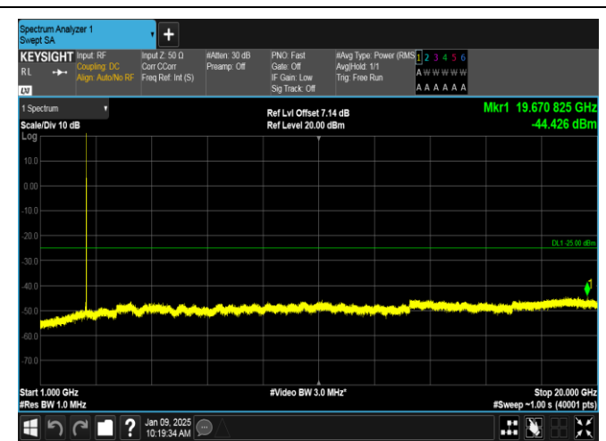
Band38-10MHz-QPSK-37800-1RB#0-1000~20000-PASS
