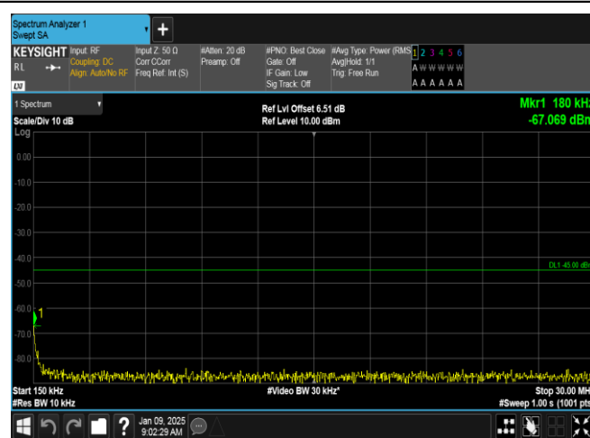
Band38-5MHz-QPSK-38225-1RB#0-0.15~30-PASS
