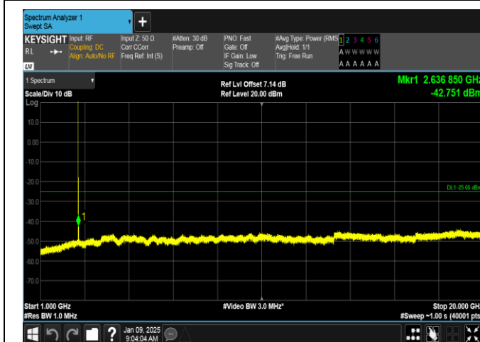
Band38-5MHz-16QAM-38225-1RB#0-1000~20000-PASS
