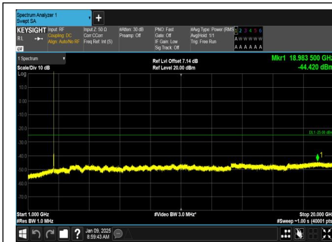
Band38-5MHz-16QAM-38000-1RB#24-1000~20000-PASS
