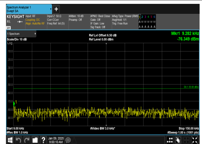
Band38-5MHz-QPSK-38000-25RB#0-0.009~0.15-PASS
