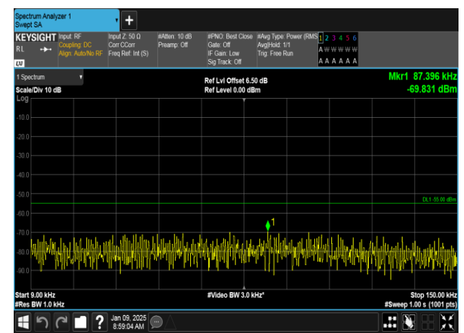
Band38-5MHz-16QAM-38000-1RB#24-0.009~0.15-PASS
