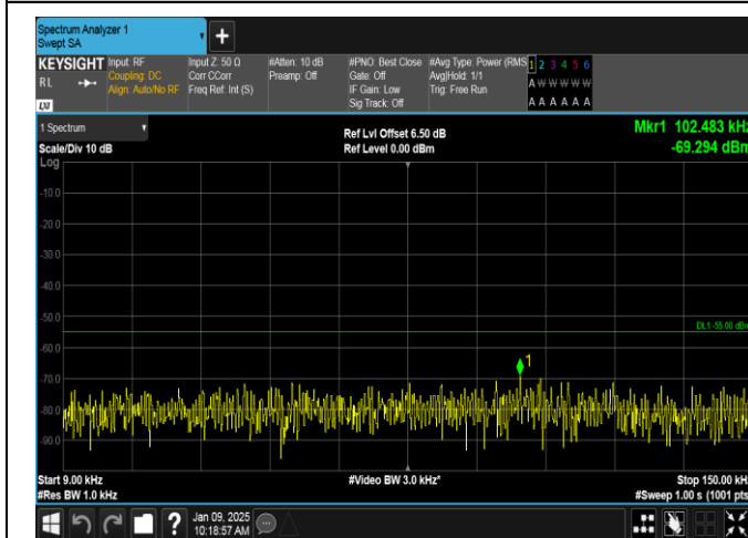
Band38-10MHz-QPSK-37800-1RB#0-0.009~0.15-PASS
