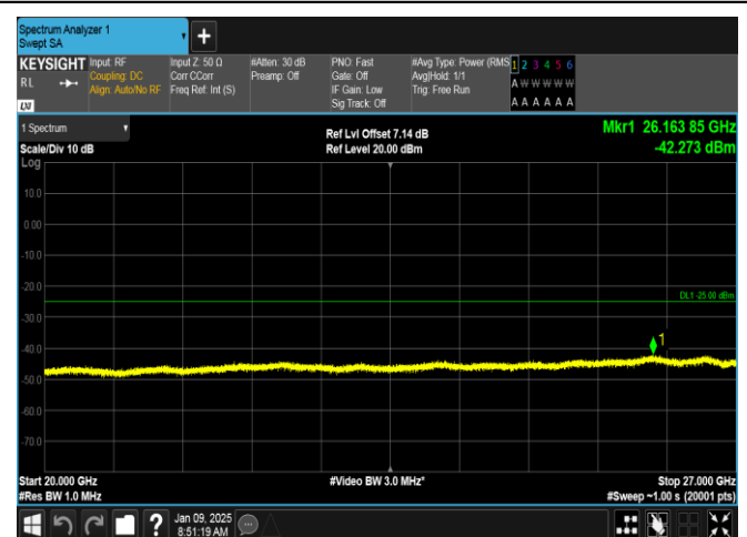
Band38-5MHz-16QAM-37775-1RB#0-20000~27000-PASS
