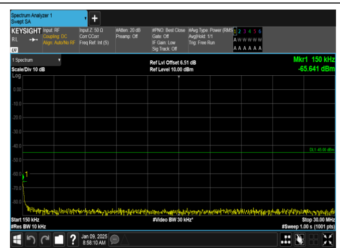
Band38-5MHz-QPSK-38000-1RB#24-0.15~30-PASS
