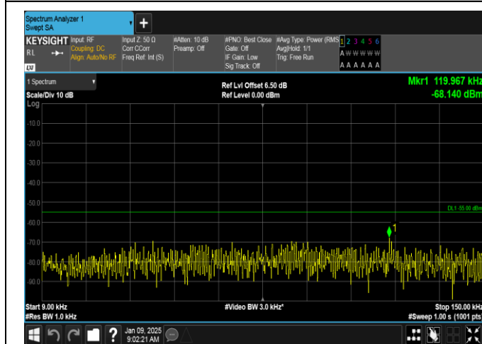
Band38-5MHz-QPSK-38225-1RB#0-0.009~0.15-PASS
