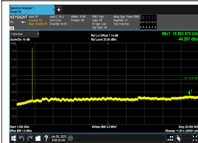
Band38-5MHz-16QAM-38225-25RB#0-1000~20000-PASS
