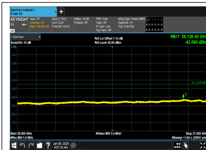
Band38-5MHz-QPSK-38225-25RB#0-20000~27000-PASS
