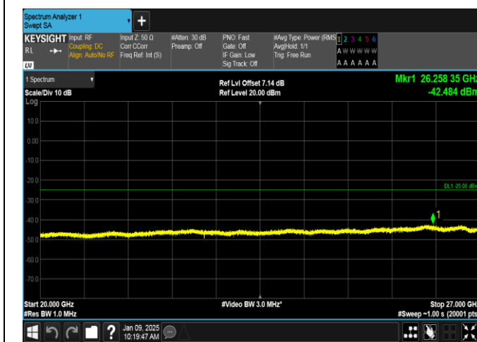
Band38-10MHz-QPSK-37800-1RB#0-20000~27000-PASS
