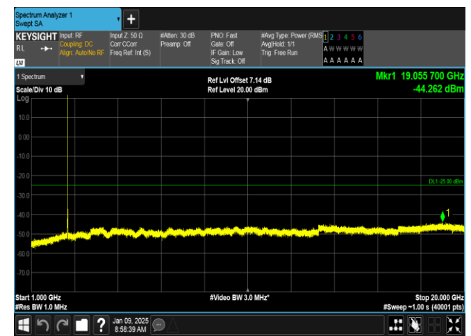
Band38-5MHz-QPSK-38000-1RB#24-1000~20000-PASS
