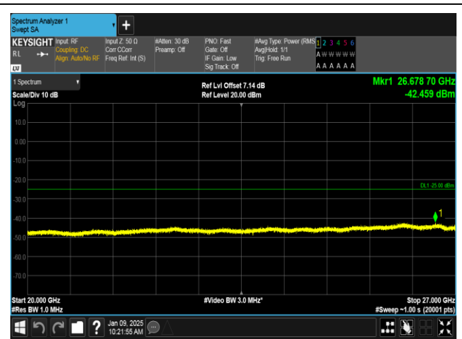
Band38-10MHz-QPSK-37800-1RB#49-20000~27000-PASS
