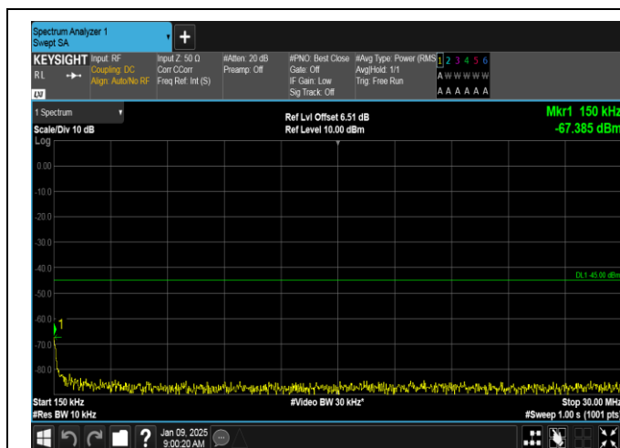
Band38-5MHz-QPSK-38000-25RB#0-0.15~30-PASS
