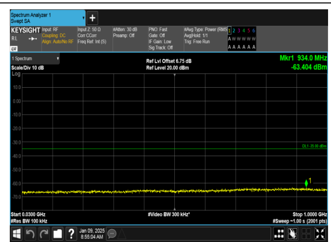
Band38-5MHz-16QAM-37775-25RB#0-30~1000-PASS
