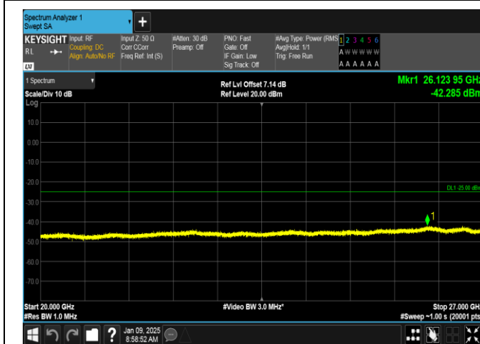
Band38-5MHz-QPSK-38000-1RB#24-20000~27000-PASS
