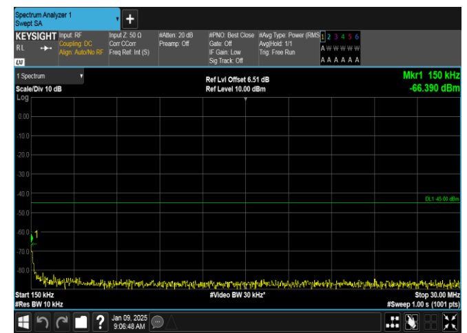
Band38-5MHz-QPSK-38225-25RB#0-0.15~30-PASS
