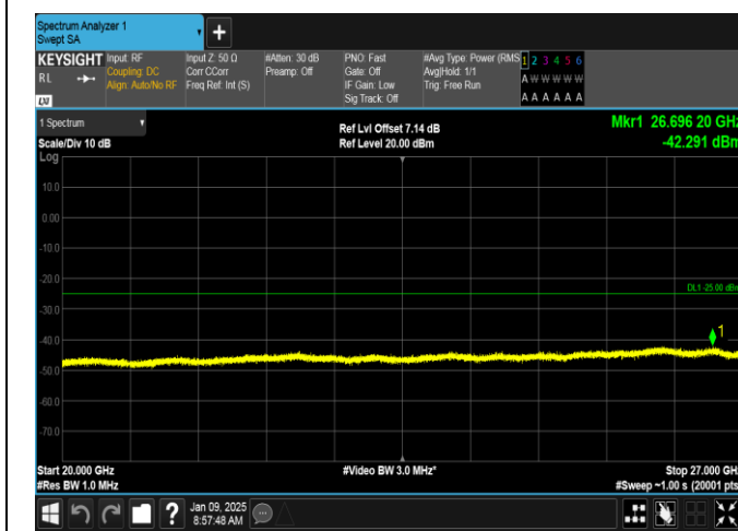
Band38-5MHz-16QAM-38000-1RB#0-20000~27000-PASS
