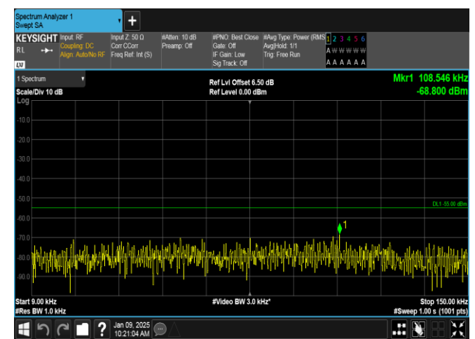
Band38-10MHz-QPSK-37800-1RB#49-0.009~0.15-PASS
