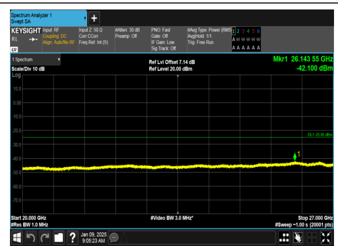
Band38-5MHz-QPSK-38225-1RB#24-20000~27000-PASS
