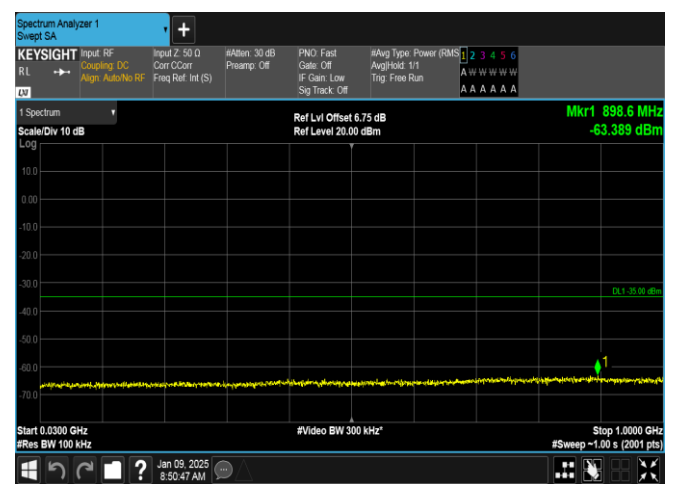
Band38-5MHz-16QAM-37775-1RB#0-30~1000-PASS
