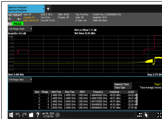
Band38-5MHz-QPSK-37775-25RB#0-PASS
