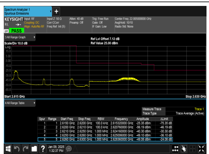
Band38-5MHz-16QAM-38225-1RB#0-PASS
