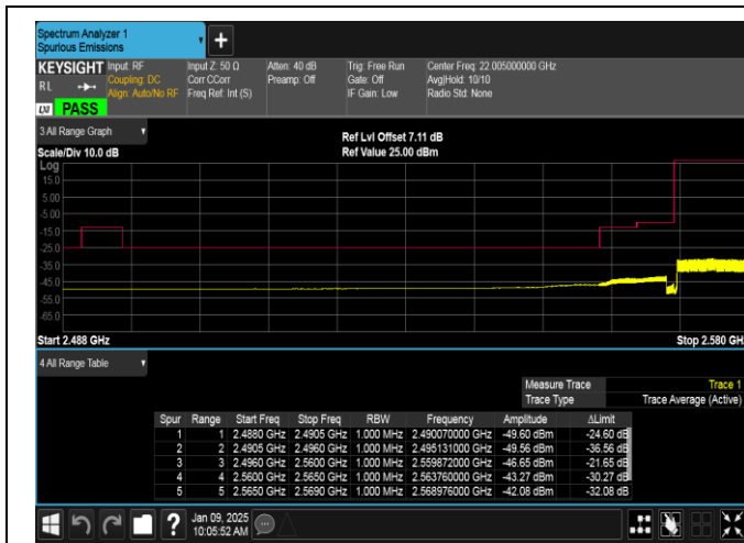
Band38-10MHz-QPSK-37800-50RB#0-PASS
