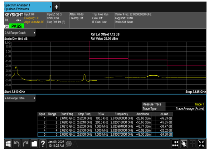
Band38-10MHz-16QAM-38200-1RB#0-PASS
