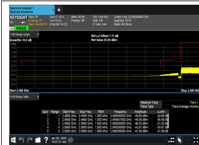
Band38-10MHz-16QAM-37800-50RB#0-PASS
