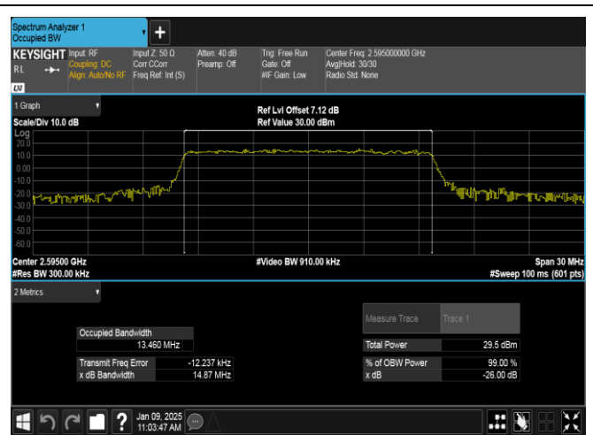
Band38-15MHz-QPSK-38000-75RB#0-PASS
