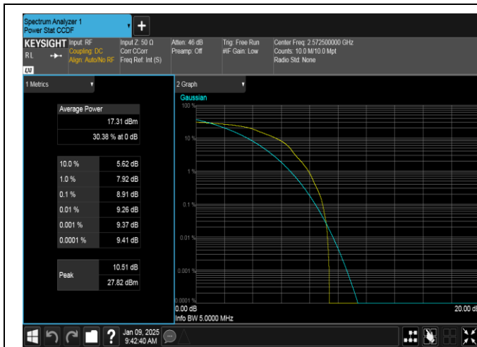
Band38-5MHz-16QAM-37775-1RB#0-PASS
