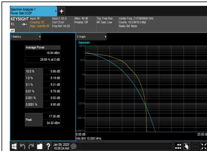
Band38-10MHz-16QAM-37800-1RB#0-PASS
