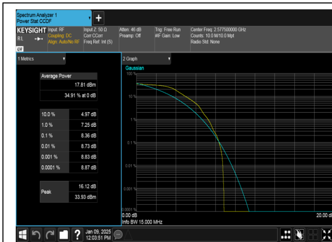
Band38-15MHz-QPSK-37825-1RB#0-PASS
