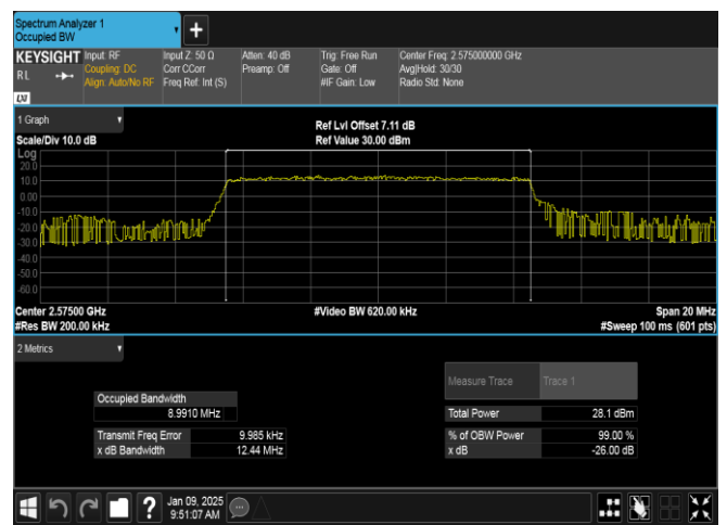
Band38-10MHz-16QAM-37800-50RB#0-PASS
