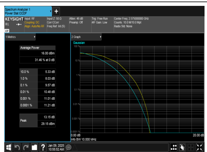
Band38-10MHz-16QAM-37800-50RB#0-PASS
