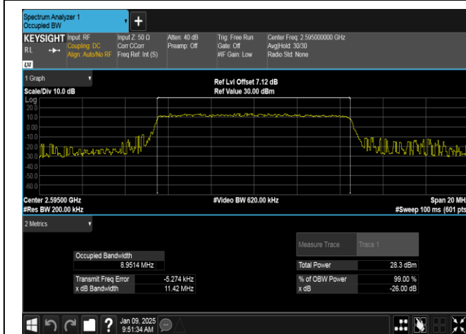
Band38-10MHz-16QAM-38000-50RB#0-PASS
