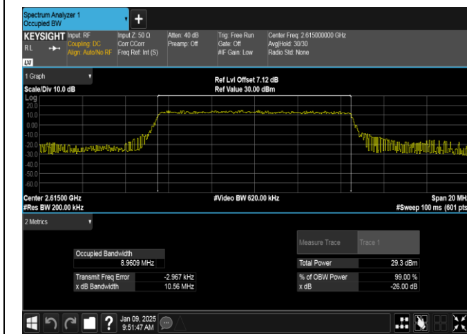
Band38-10MHz-QPSK-38200-50RB#0-PASS
