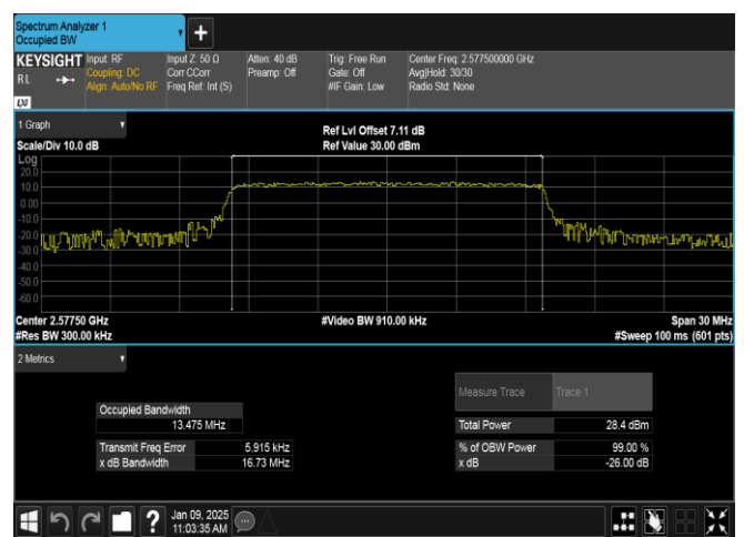
Band38-15MHz-16QAM-37825-75RB#0-PASS
