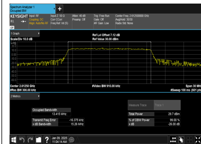
Band38-15MHz-QPSK-38175-75RB#0-PASS
