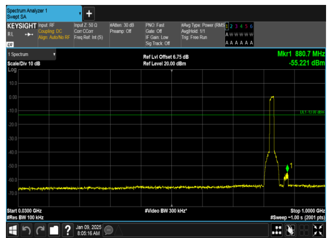
Band26(824-849)-15MHz-16QAM-26865-75RB#0-30~1000-PASS
