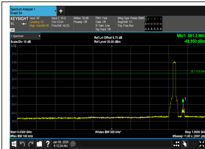
Band26(824-849)-15MHz-16QAM-26915-75RB#0-30~1000-PASS
