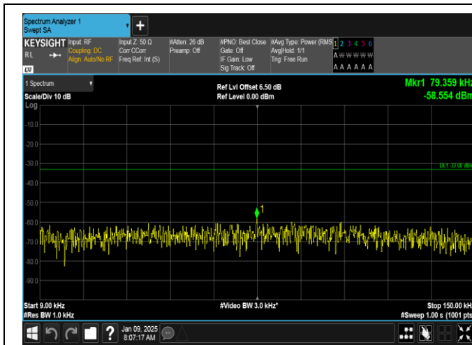
Band26(824-849)-15MHz-16QAM-26915-1RB#0-0.009~0.15-PASS
