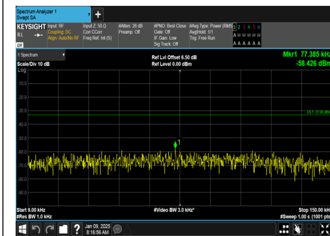
Band26(824-849)-15MHz-16QAM-26965-1RB#74-0.009~0.15-PASS
