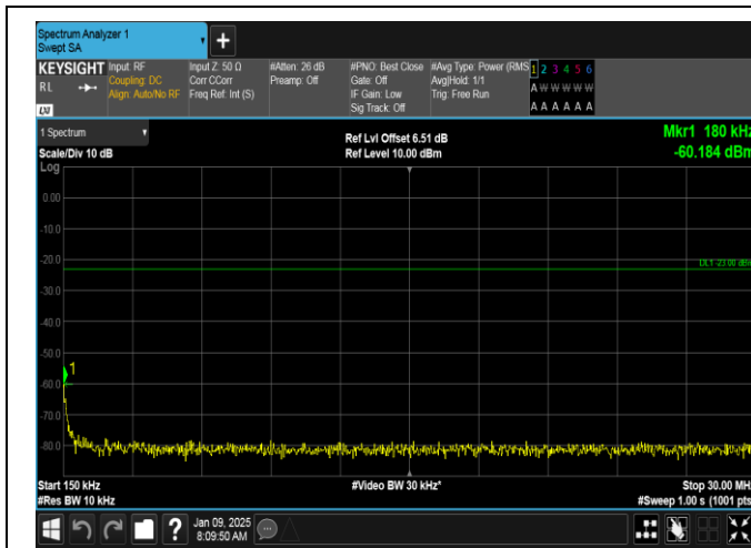
Band26(824-849)-15MHz-16QAM-26915-1RB#74-0.15~30-PASS
