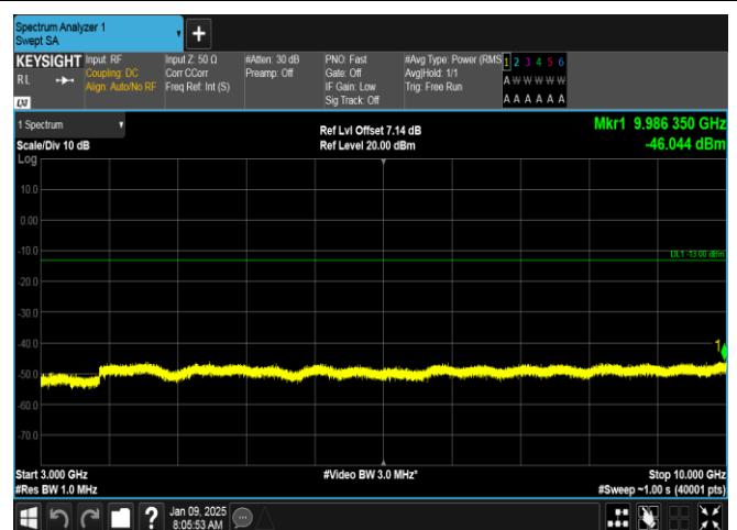
Band26(824-849)-15MHz-16QAM-26865-75RB#0-3000~10000-PASS
