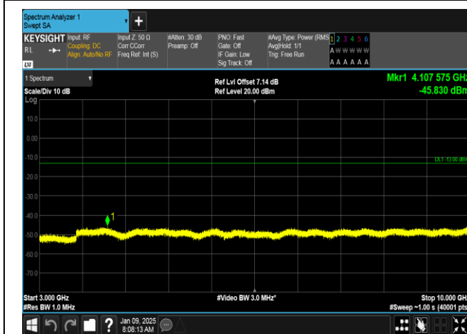
Band26(824-849)-15MHz-16QAM-26915-1RB#0-3000~10000-PASS
