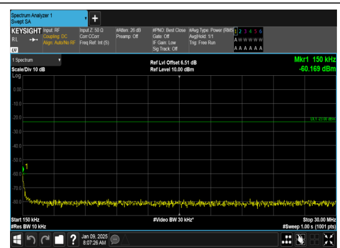
Band26(824-849)-15MHz-16QAM-26915-1RB#0-0.15~30-PASS
