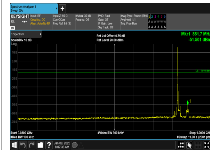
Band26(824-849)-15MHz-16QAM-26915-1RB#0-30~1000-PASS
