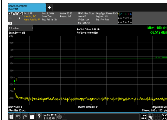
Band26(824-849)-15MHz-16QAM-26965-1RB#0-0.15~30-PASS
