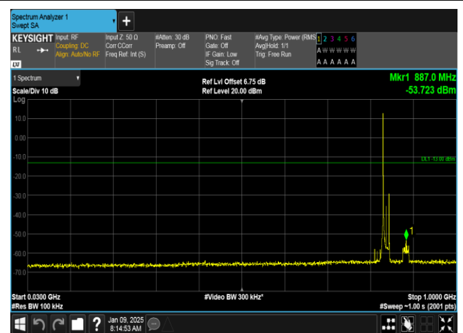
Band26(824-849)-15MHz-16QAM-26965-1RB#0-30~1000-PASS
