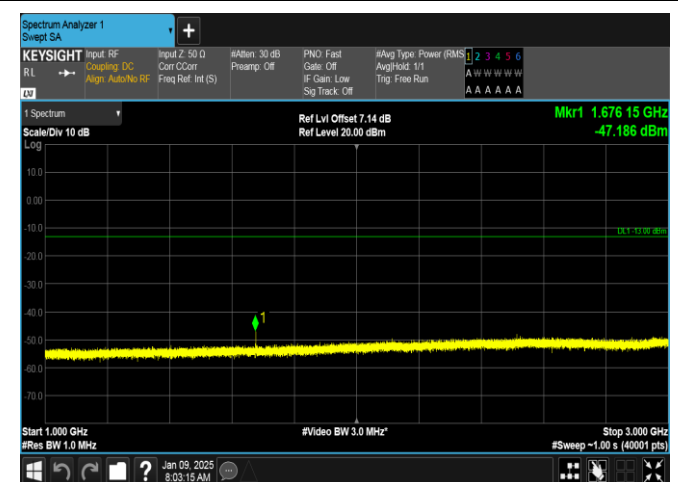
Band26(824-849)-15MHz-16QAM-26865-1RB#74-1000~3000-PASS
