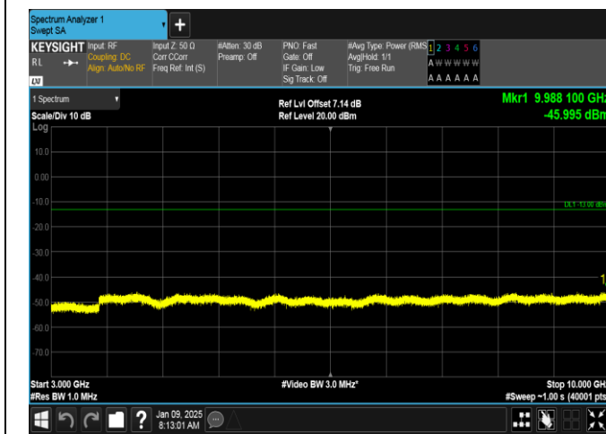
Band26(824-849)-15MHz-16QAM-26915-75RB#0-3000~10000-PASS
