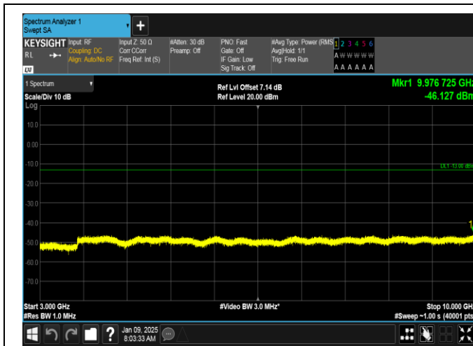
Band26(824-849)-15MHz-16QAM-26865-1RB#74-3000~10000-PASS
