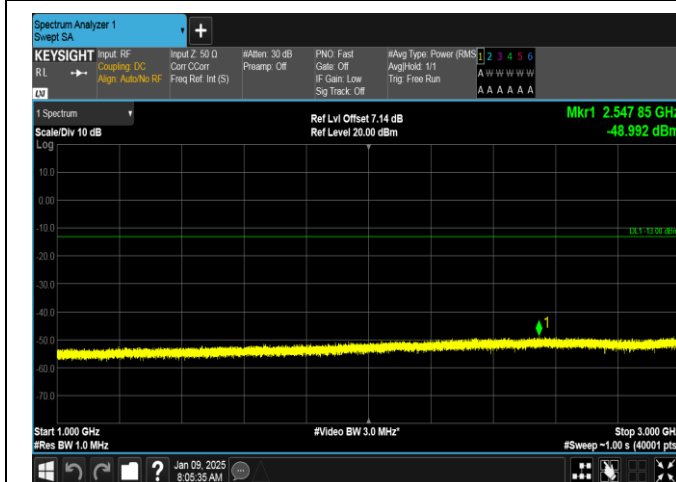
Band26(824-849)-15MHz-16QAM-26865-75RB#0-1000~3000-PASS
