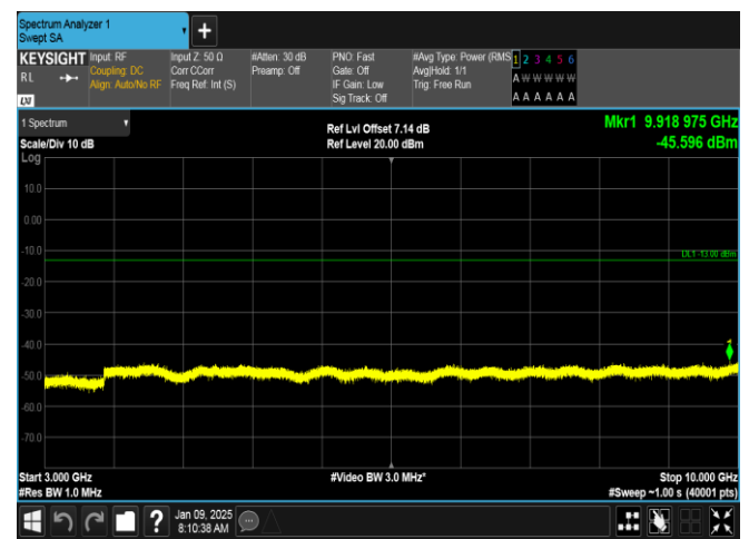
Band26(824-849)-15MHz-16QAM-26915-1RB#74-3000~10000-PASS
