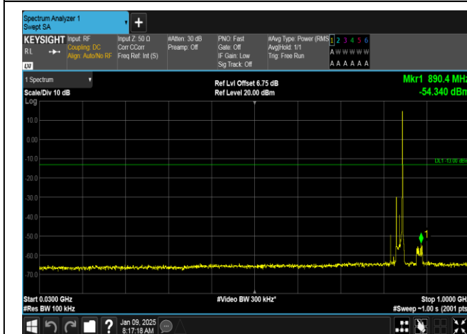
Band26(824-849)-15MHz-16QAM-26965-1RB#74-30~1000-PASS
