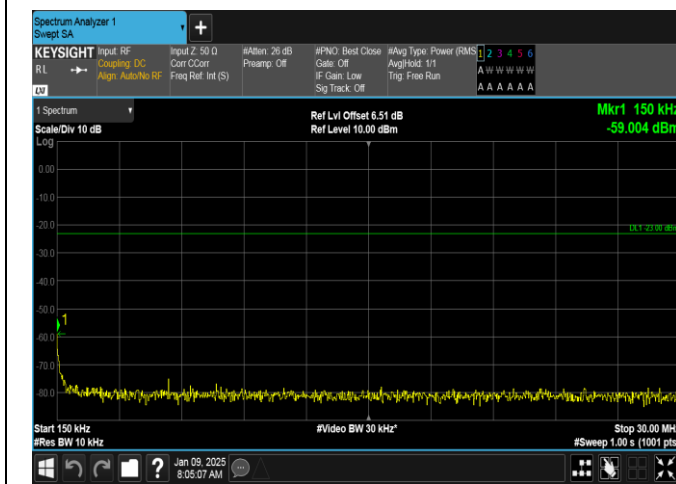
Band26(824-849)-15MHz-16QAM-26865-75RB#0-0.15~30-PASS
