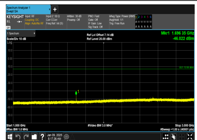
Band26(824-849)-15MHz-16QAM-26965-1RB#74-1000~3000-PASS
