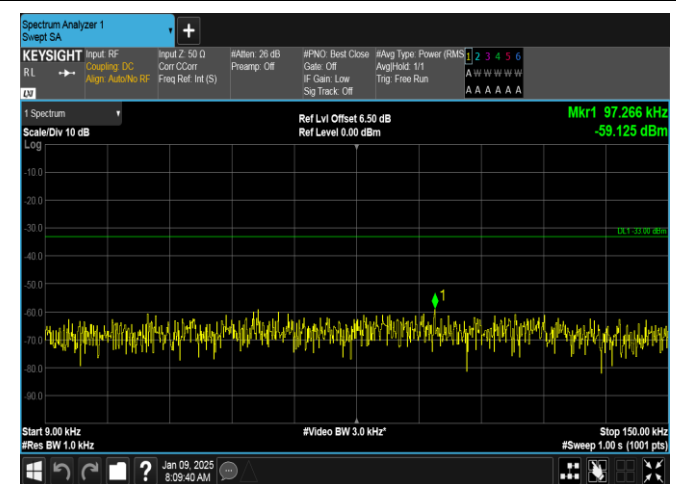
Band26(824-849)-15MHz-16QAM-26915-1RB#74-0.009~0.15-PASS
