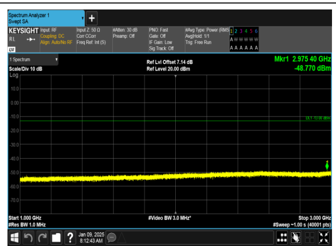
Band26(824-849)-15MHz-16QAM-26915-75RB#0-1000~3000-PASS
