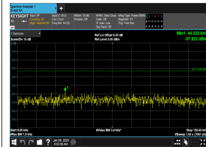
Band26(824-849)-15MHz-16QAM-26865-1RB#74-0.009~0.15-PASS
