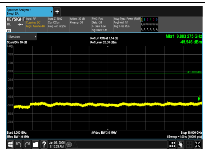
Band26(824-849)-15MHz-16QAM-26965-1RB#0-3000~10000-PASS
