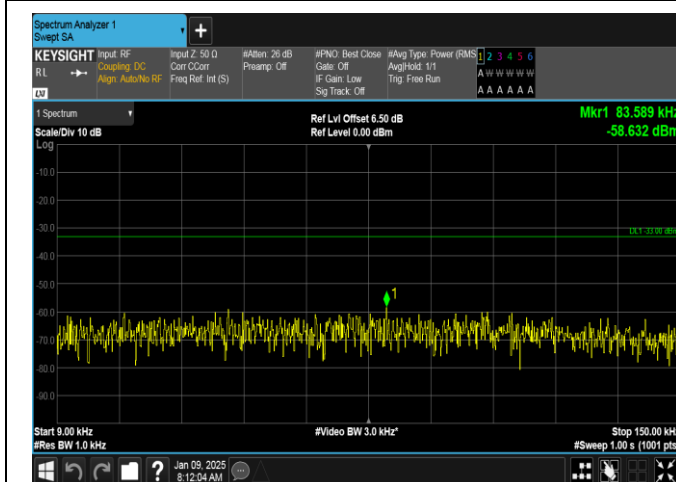
Band26(824-849)-15MHz-16QAM-26915-75RB#0-0.009~0.15-PASS
