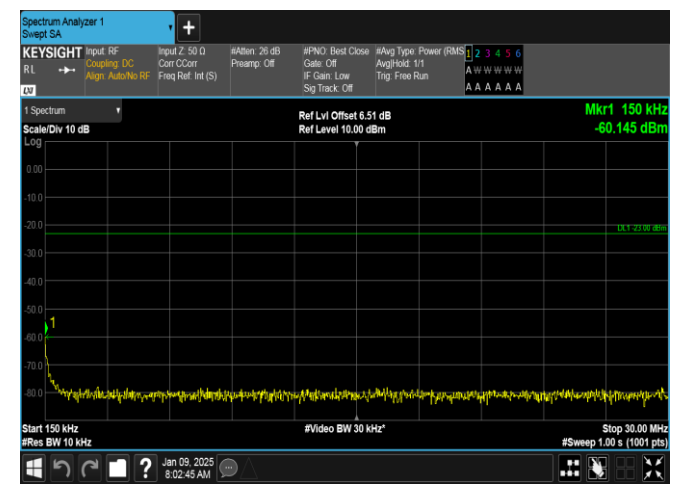
Band26(824-849)-15MHz-16QAM-26865-1RB#74-0.15~30-PASS
