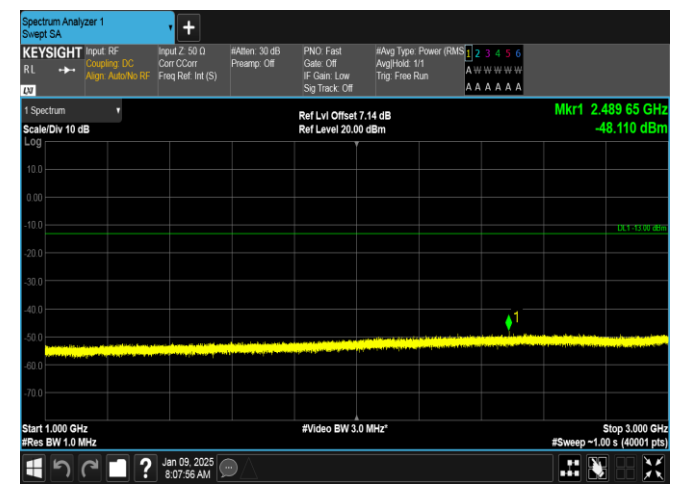
Band26(824-849)-15MHz-16QAM-26915-1RB#0-1000~3000-PASS
