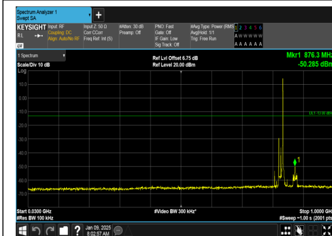
Band26(824-849)-15MHz-16QAM-26865-1RB#74-30~1000-PASS
