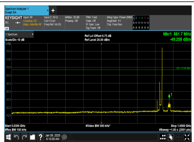
Band26(824-849)-15MHz-16QAM-26915-1RB#74-30~1000-PASS
