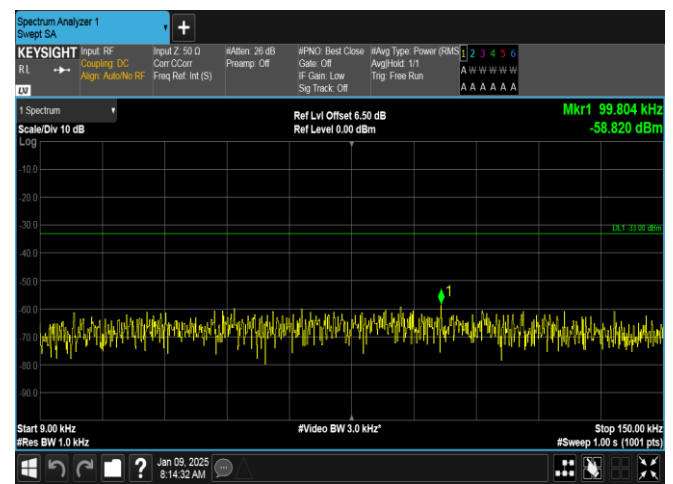
Band26(824-849)-15MHz-16QAM-26965-1RB#0-0.009~0.15-PASS
