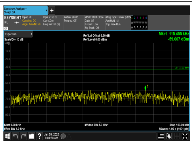
Band26(824-849)-15MHz-16QAM-26865-75RB#0-0.009~0.15-PASS
