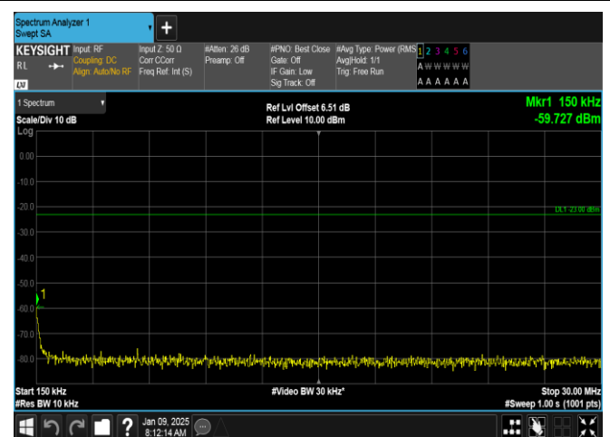
Band26(824-849)-15MHz-16QAM-26915-75RB#0-0.15~30-PASS
