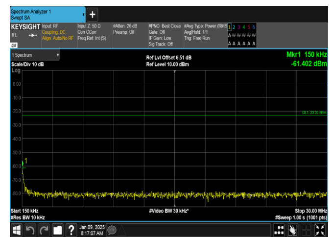
Band26(824-849)-15MHz-16QAM-26965-1RB#74-0.15~30-PASS
