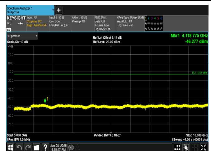
Band26(824-849)-10MHz-QPSK-26915-50RB#0-3000~10000-PASS
