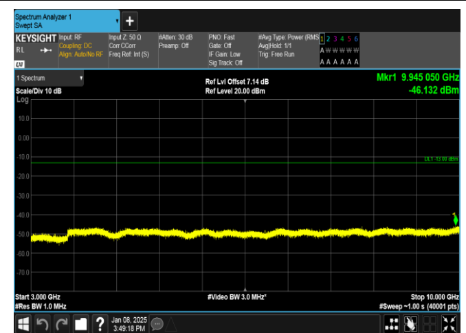
Band26(824-849)-5MHz-16QAM-27015-25RB#0-3000~10000-PASS
