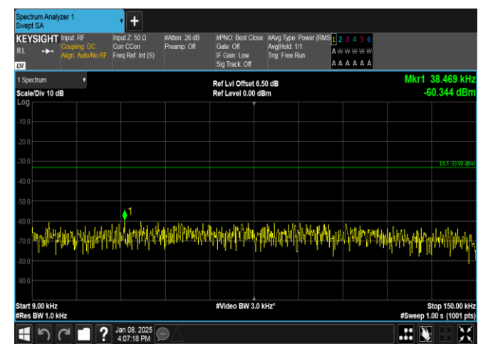
Band26(824-849)-10MHz-16QAM-26840-1RB#0-0.009~0.15-PASS
