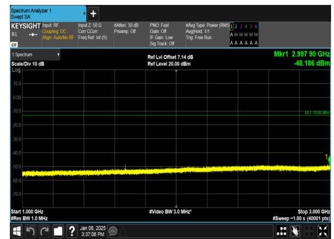
Band26(824-849)-5MHz-16QAM-26915-1RB#0-1000~3000-PASS
