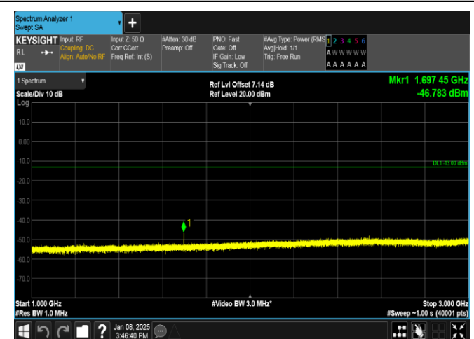
Band26(824-849)-5MHz-16QAM-27015-1RB#24-1000-3000-PASS
