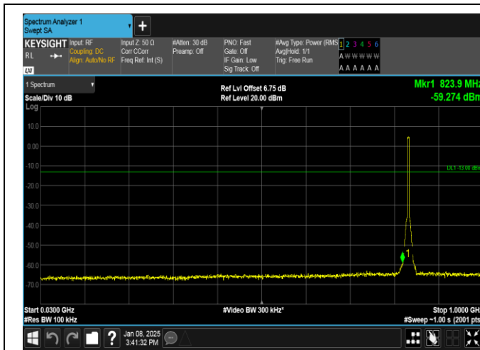
Band26(824-849)-5MHz-16QAM-26915-25RB#0-30~1000-PASS
