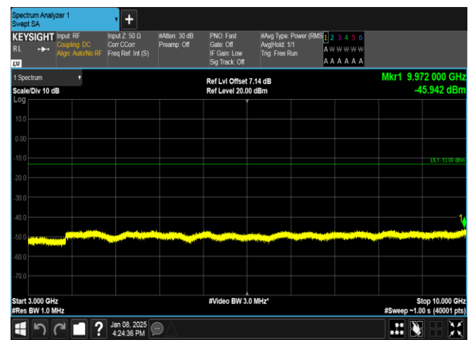
Band26(824-849)-10MHz-QPSK-26990-1RB#49-3000~10000-PASS
