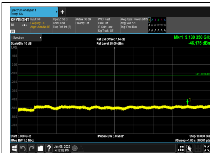
Band26(824-849)-10MHz-QPSK-26915-1RB#49-3000~10000-PASS
