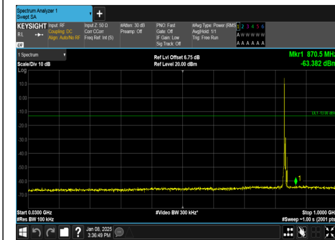
Band26(824-849)-5MHz-16QAM-26915-1RB#0-30~1000-PASS
