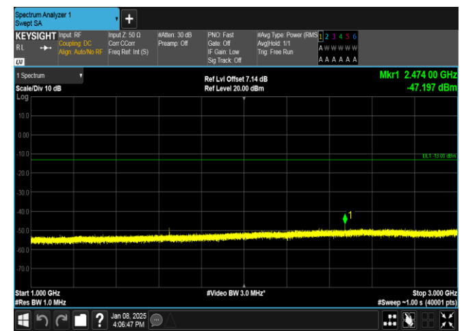
Band26(824-849)-10MHz-QPSK-26840-1RB#0-1000~3000-PASS
