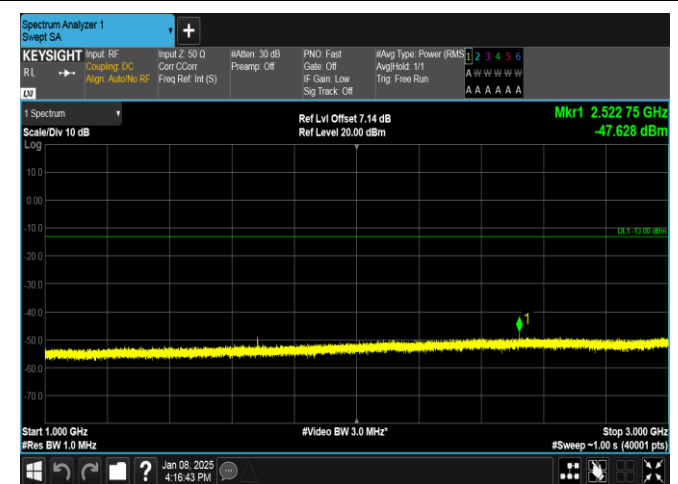
Band26(824-849)-10MHz-QPSK-26915-1RB#49-1000-3000-PASS
