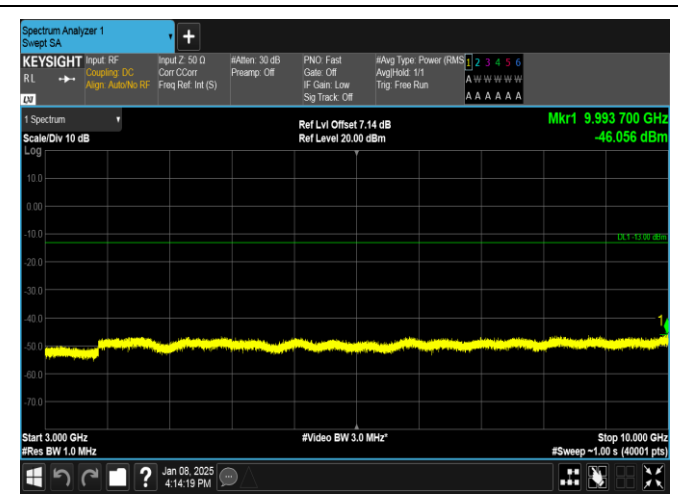
Band26(824-849)-10MHz-QPSK-26915-1RB#0-3000-10000-PASS
