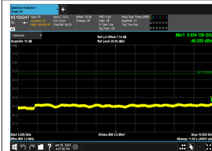
Band26(824-849)-10MHz-QPSK-26840-1RB#0-3000~10000-PASS
