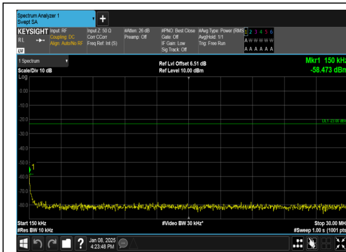
Band26(824-849)-10MHz-QPSK-26990-1RB#49-0.15~30-PASS
