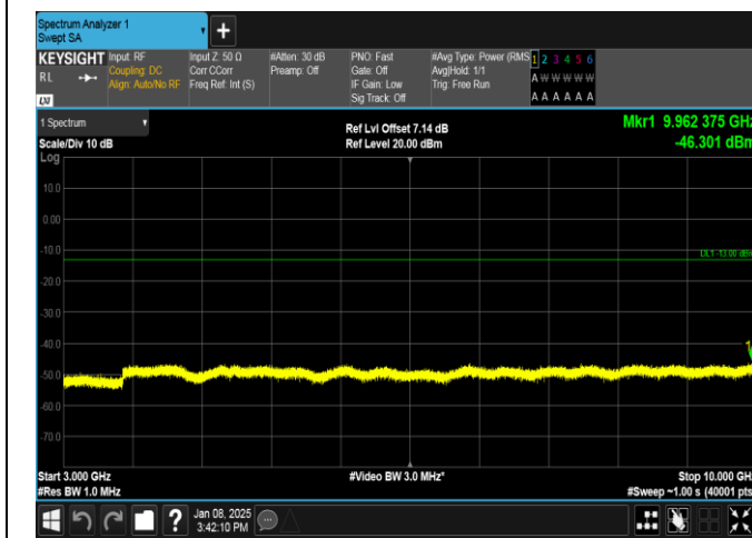
Band26(824-849)-5MHz-16QAM-26915-25RB#0-3000~10000-PASS
