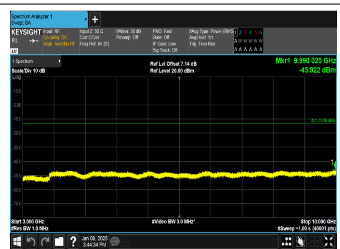
Band26(824-849)-5MHz-16QAM-27015-1RB#0-3000-10000-PASS
