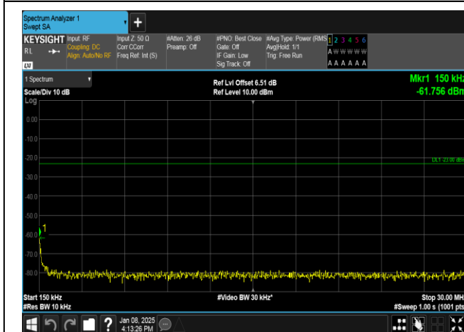
Band26(824-849)-10MHz-QPSK-26915-1RB#0-0.15~30-PASS
