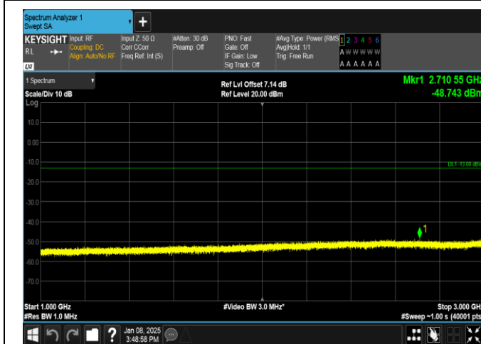
Band26(824-849)-5MHz-16QAM-27015-25RB#0-1000~3000-PASS
