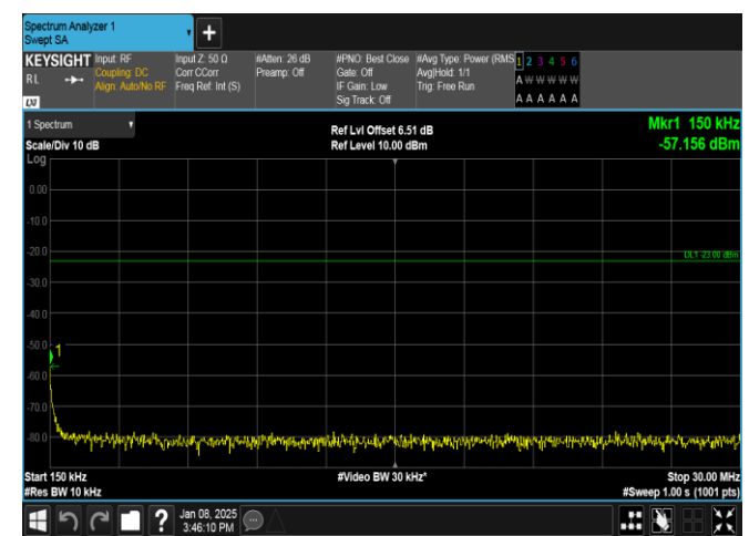
Band26(824-849)-5MHz-16QAM-27015-1RB#24-0.15-30-PASS
