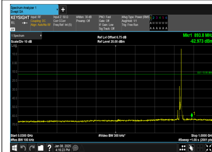
Band26(824-849)-10MHz-QPSK-26915-1RB#49-30-1000-PASS
