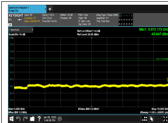
Band26(824-849)-5MHz-16QAM-27015-1RB#24-3000~10000-PASS
