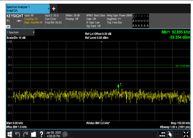
Band26(824-849)-10MHz-QPSK-26840-1RB#49-0.009~0.15-PASS
