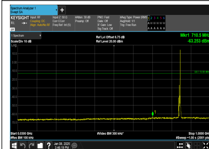
Band26(824-849)-5MHz-16QAM-27015-1RB#24-30-1000-PASS
