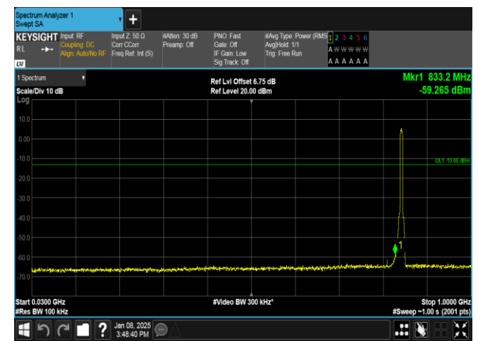
Band26(824-849)-5MHz-16QAM-27015-25RB#0-30~1000-PASS
