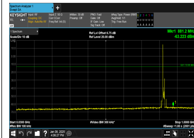
Band26(824-849)-10MHz-QPSK-26840-1RB#0-30~1000-PASS
