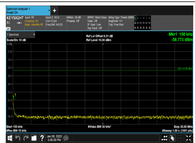
Band26(824-849)-5MHz-16QAM-26915-1RB#0-0.15~30-PASS
