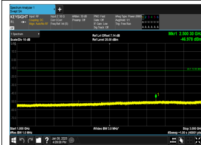
Band26(824-849)-10MHz-QPSK-26840-1RB#49-1000~3000-PASS
