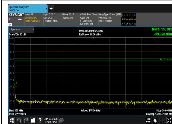
Band26(824-849)-10MHz-QPSK-26915-50RB#0-0.15~30-PASS
