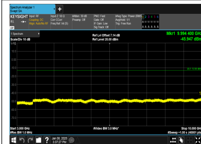
Band26(824-849)-5MHz-16QAM-26915-1RB#0-3000~10000-PASS
