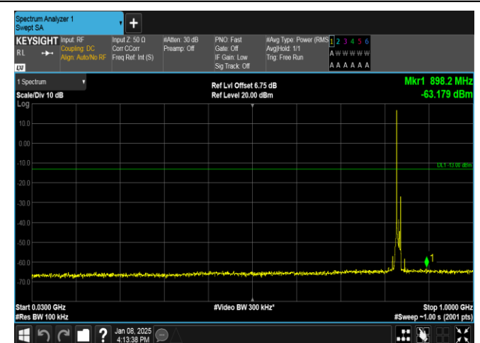
Band26(824-849)-10MHz-QPSK-26915-1RB#0-30~1000-PASS
