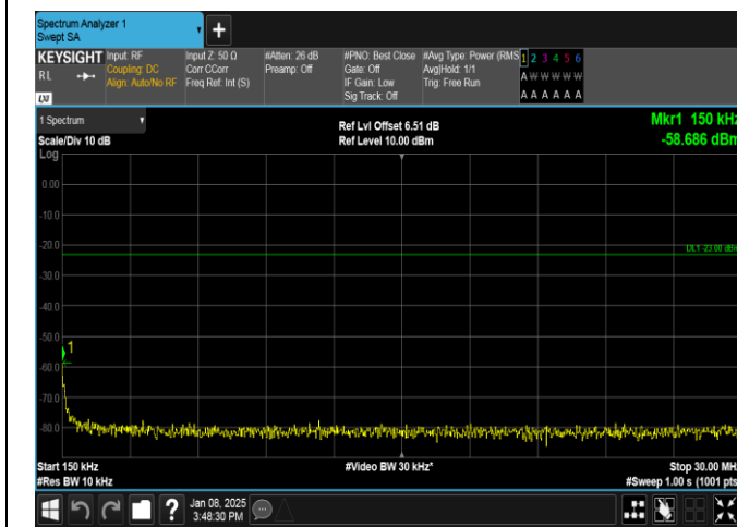
Band26(824-849)-5MHz-16QAM-27015-25RB#0-0.15~30-PASS
