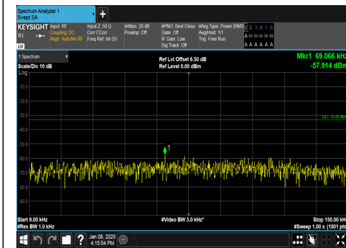
Band26(824-849)-10MHz-QPSK-26915-1RB#49-0.009-0.15-PASS
