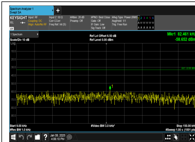
Band26(824-849)-10MHz-QPSK-26840-1RB#0-0.009~0.15-PASS
