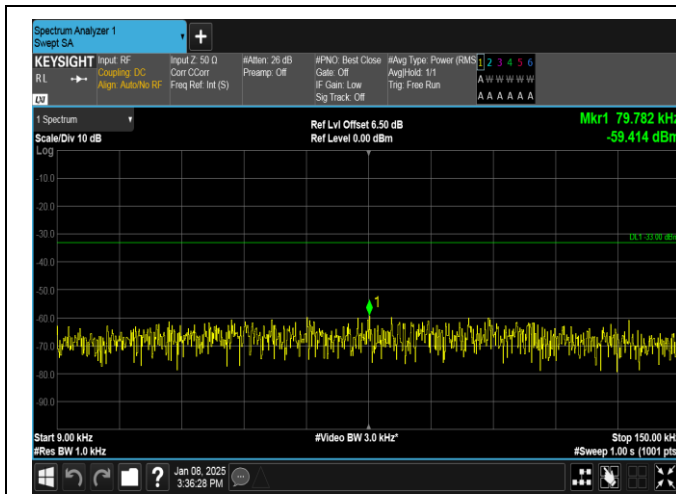
Band26(824-849)-5MHz-16QAM-26915-1RB#0-0.009~0.15-PASS
