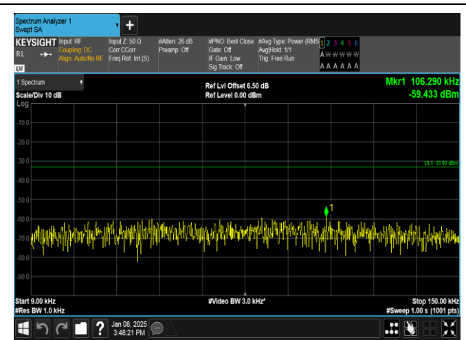
Band26(824-849)-5MHz-16QAM-27015-25RB#0-0.009~0.15-PASS
