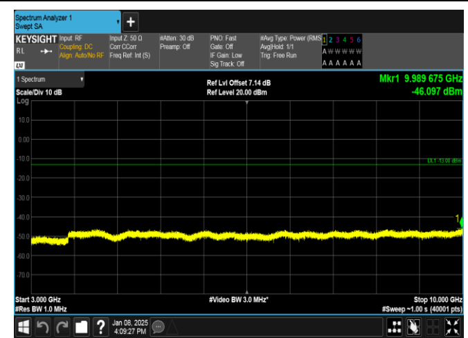
Band26(824-849)-10MHz-QPSK-26840-1RB#49-3000~10000-PASS
