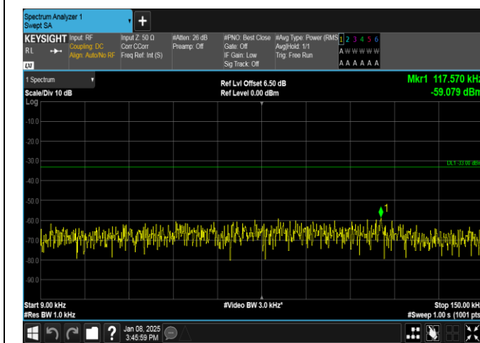
Band26(824-849)-5MHz-16QAM-27015-1RB#24-0.009-0.15-PASS
