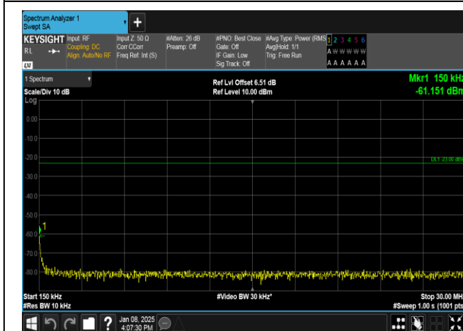
Band26(824-849)-10MHz-16QAM-26840-1RB#0-0.15~30-PASS
