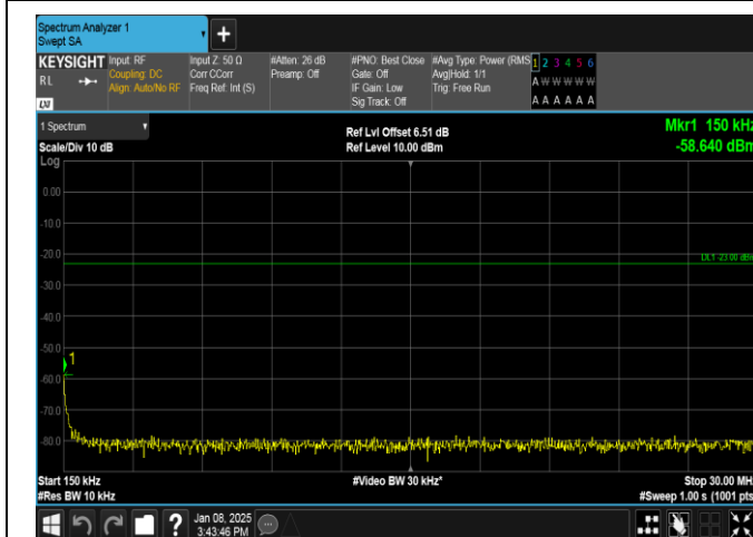
Band26(824-849)-5MHz-16QAM-27015-1RB#0-0.15~30-PASS
