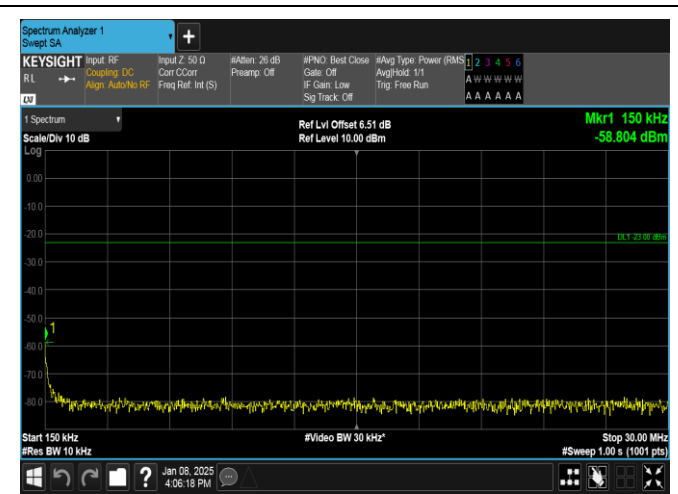
Band26(824-849)-10MHz-QPSK-26840-1RB#0-0.15~30-PASS
