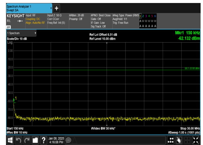
Band26(824-849)-10MHz-QPSK-26915-1RB#49-0.15-30-PASS
