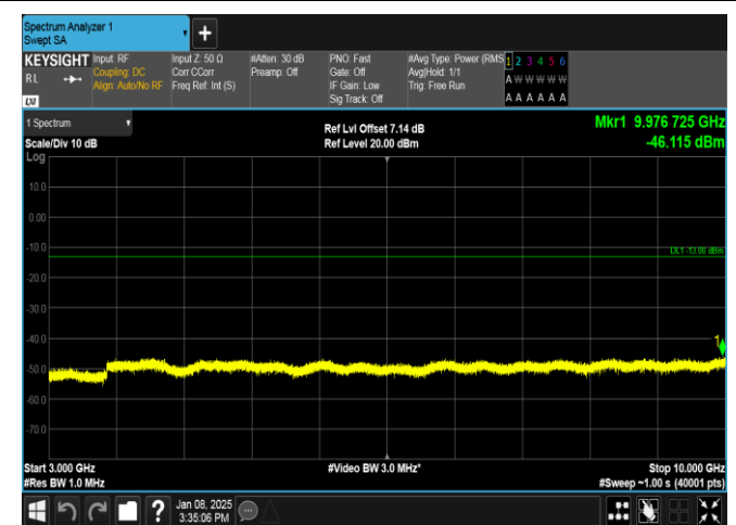
Band26(824-849)-5MHz-16QAM-26815-25RB#0-3000~10000-PASS
