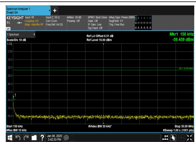
Band26(824-849)-5MHz-QPSK-27015-1RB#0-0.15~30-PASS
