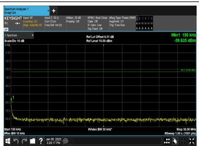
Band26(824-849)-5MHz-QPSK-26815-1RB#0-0.15~30-PASS
