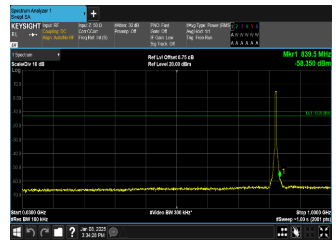
Band26(824-849)-5MHz-16QAM-26815-25RB#0-30~1000-PASS
