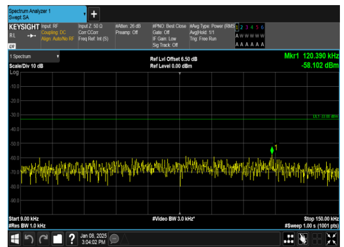
Band26(824-849)-3MHz-16QAM-27025-1RB#0-0.009~0.15-PASS
