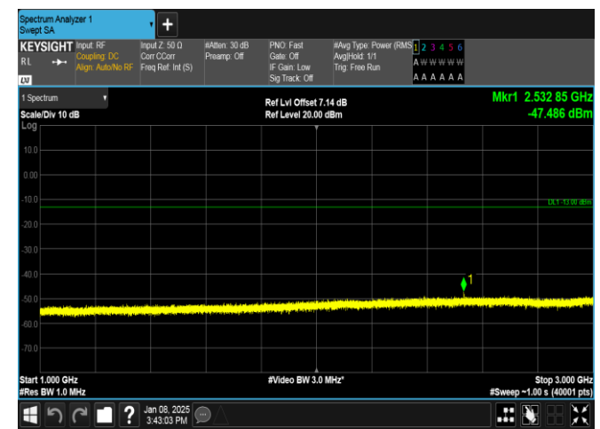
Band26(824-849)-5MHz-QPSK-27015-1RB#0-1000~3000-PASS
