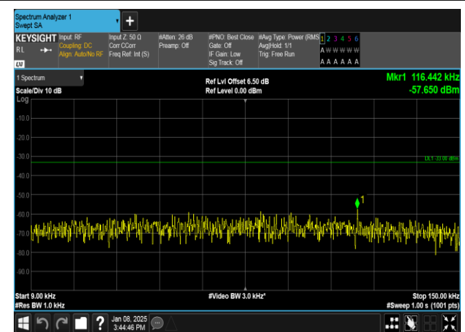
Band26(824-849)-5MHz-QPSK-27015-1RB#24-0.009~0.15-PASS
