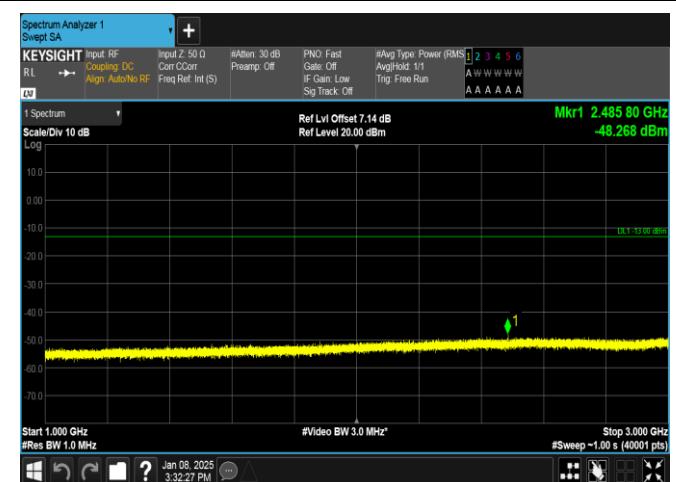
Band26(824-849)-5MHz-16QAM-26815-1RB#24-1000~3000-PASS
