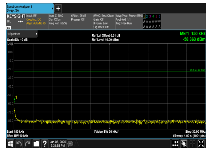
Band26(824-849)-5MHz-16QAM-26815-1RB#24-0.15~30-PASS
