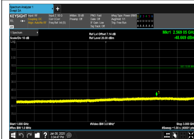
Band26(824-849)-5MHz-16QAM-26815-25RB#0-1000~3000-PASS
