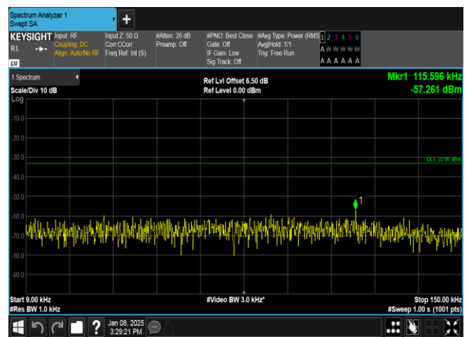
Band26(824-849)-5MHz-16QAM-26815-1RB#0-0.009~0.15-PASS
