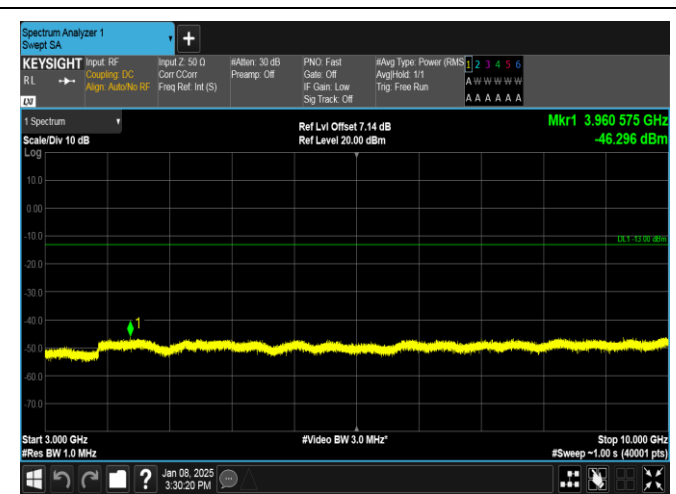
Band26(824-849)-5MHz-16QAM-26815-1RB#0-3000~10000-PASS
