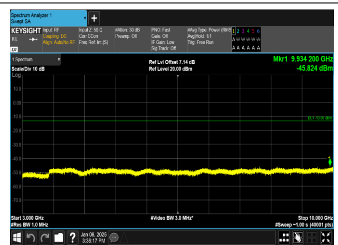
Band26(824-849)-5MHz-QPSK-26915-1RB#0-3000~10000-PASS
