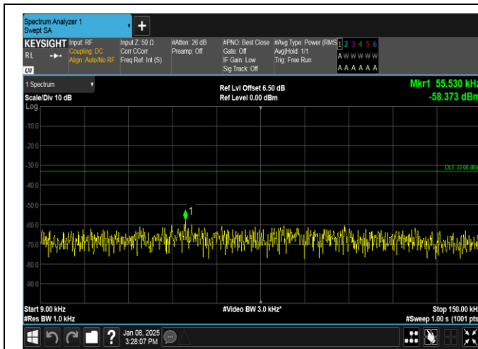
Band26(824-849)-5MHz-QPSK-26815-1RB#0-0.009~0.15-PASS
