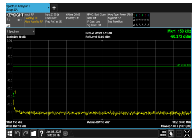
Band26(824-849)-3MHz-16QAM-27025-1RB#14-0.15~30-PASS
