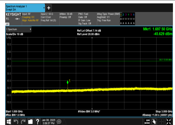
Band26(824-849)-3MHz-16QAM-27025-1RB#14-1000~3000-PASS
