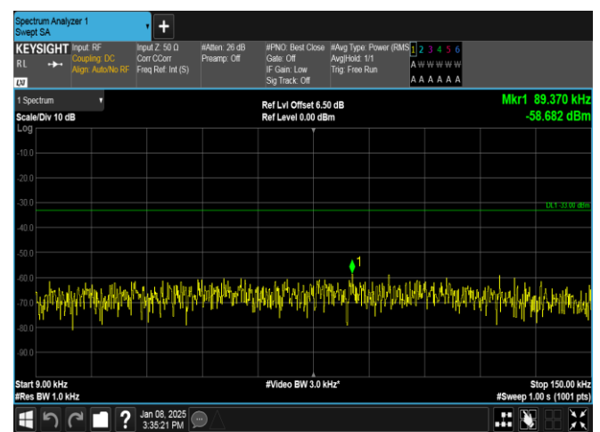
Band26(824-849)-5MHz-QPSK-26915-1RB#0-0.009~0.15-PASS
