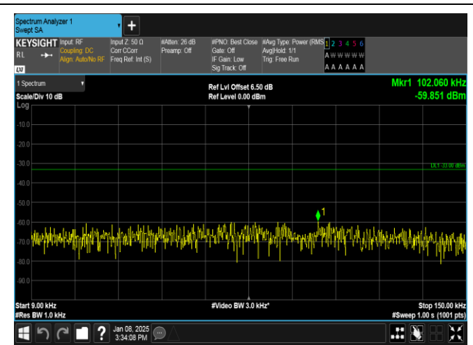
Band26(824-849)-5MHz-16QAM-26815-25RB#0-0.009~0.15-PASS
