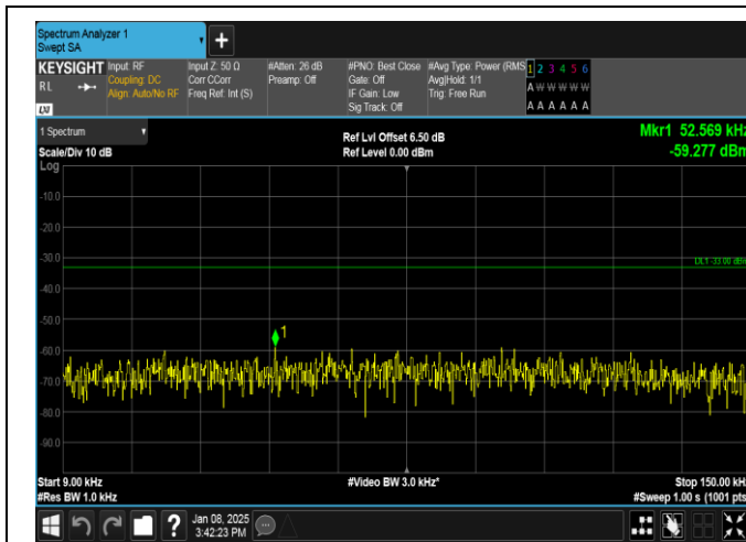
Band26(824-849)-5MHz-QPSK-27015-1RB#0-0.009~0.15-PASS
