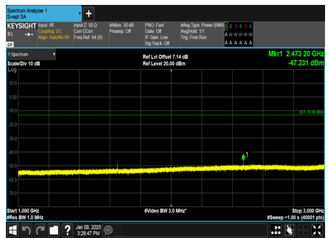
Band26(824-849)-5MHz-QPSK-26815-1RB#0-1000~3000-PASS
