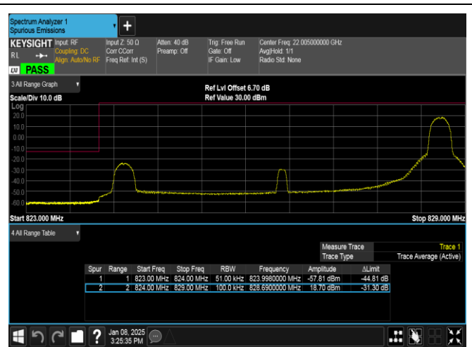
Band26(824-849)-5MHz-QPSK-26815-1RB#24-PASS
