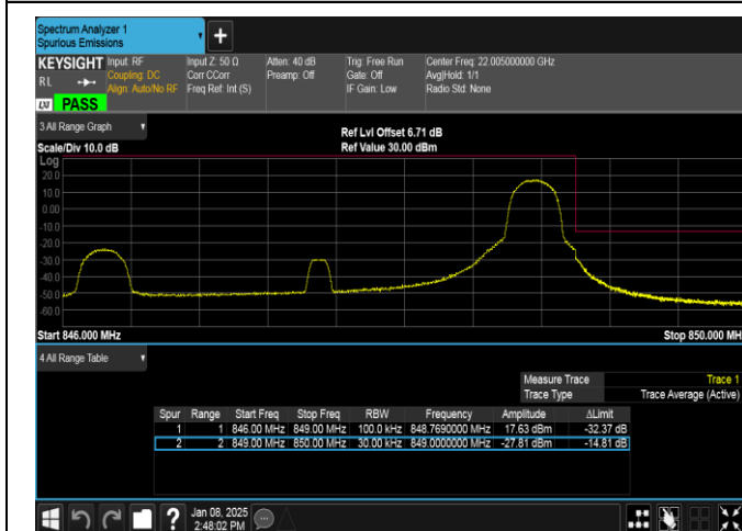
Band26(824-849)-3MHz-16QAM-27025-1RB#14-PASS
