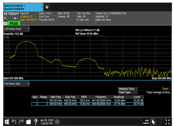
Band26(824-849)-1.4MHz-16QAM-27033-1RB#0-PASS
