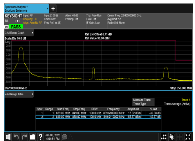
Band26(824-849)-10MHz-16QAM-26990-1RB#0-PASS
