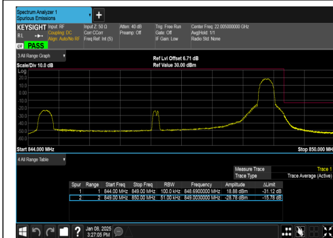
Band26(824-849)-5MHz-QPSK-27015-1RB#24-PASS
