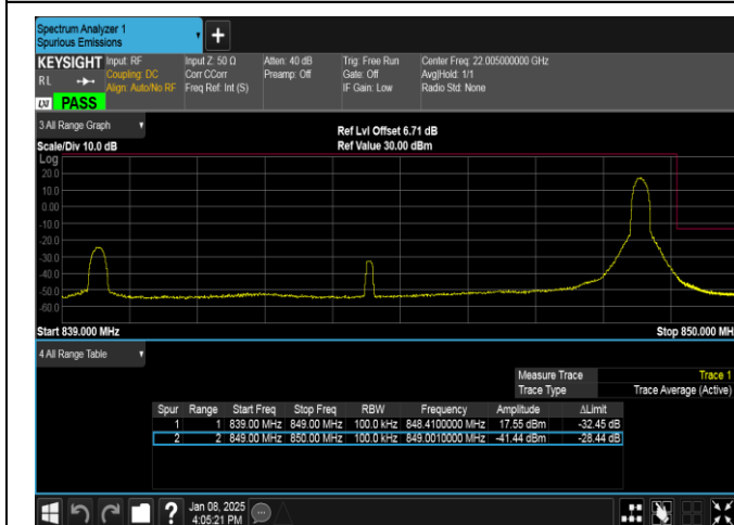
Band26(824-849)-10MHz-16QAM-26990-1RB#49-PASS
