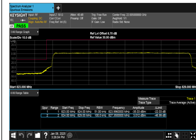
Band26(824-849)-5MHz-QPSK-26815-25RB#0-PASS
