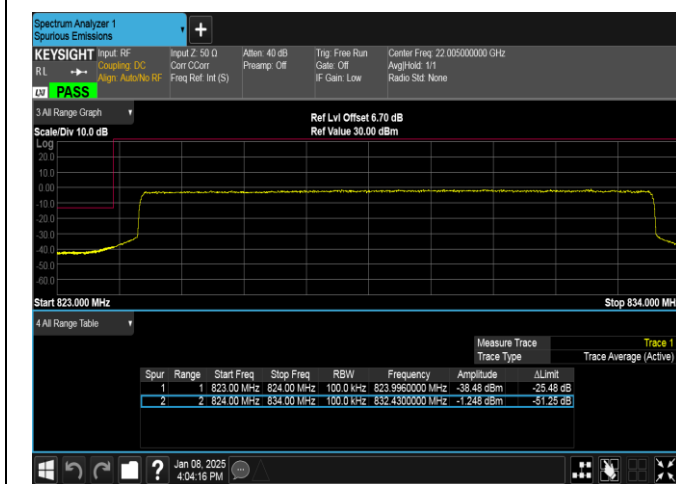
Band26(824-849)-10MHz-16QAM-26840-50RB#0-PASS
