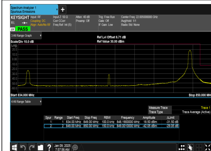
Band26(824-849)-15MHz-QPSK-26965-1RB#74-PASS
