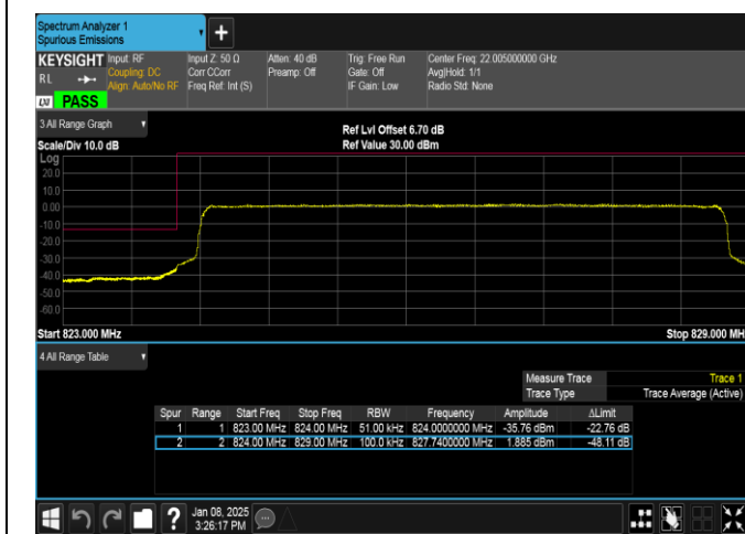
Band26(824-849)-5MHz-16QAM-26815-25RB#0-PASS
