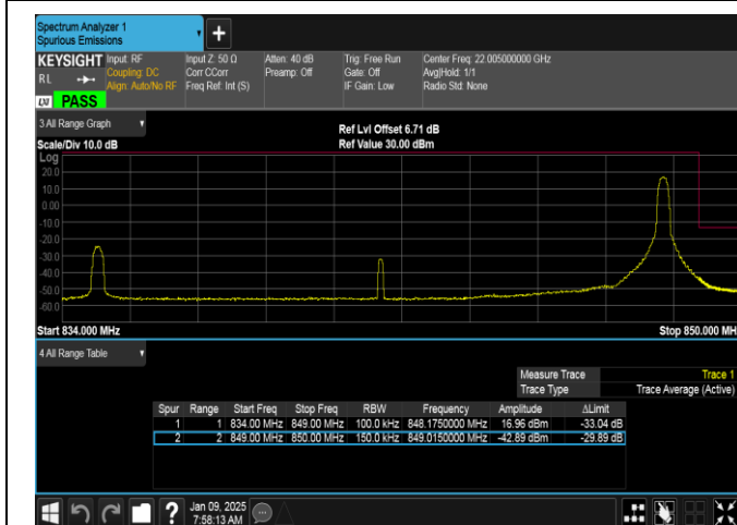
Band26(824-849)-15MHz-16QAM-26965-1RB#74-PASS
