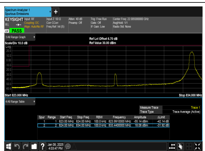
Band26(824-849)-10MHz-16QAM-26840-1RB#49-PASS
