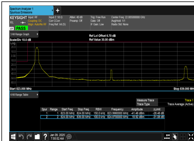
Band26(824-849)-15MHz-QPSK-26865-1RB#0-PASS
