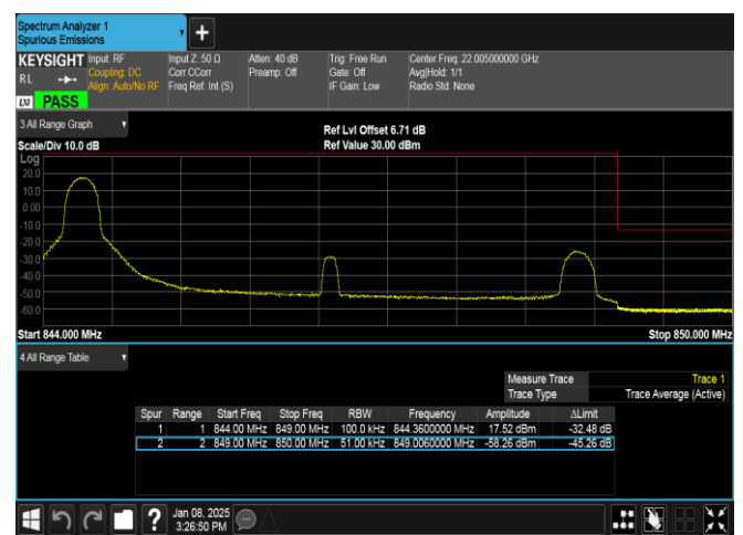
Band26(824-849)-5MHz-16QAM-27015-1RB#0-PASS
