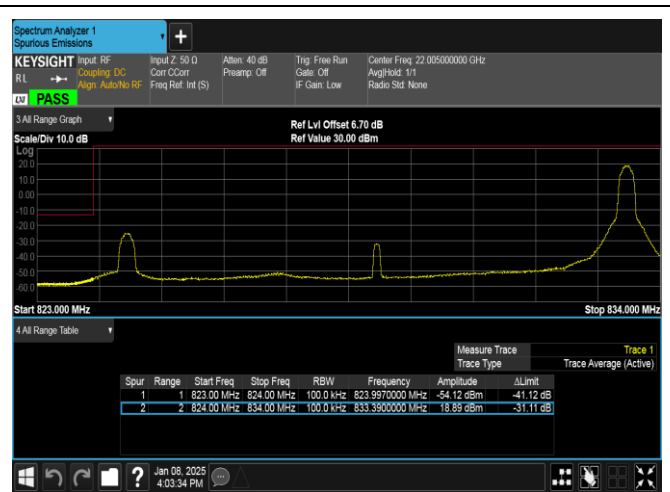
Band26(824-849)-10MHz-QPSK-26840-1RB#49-PASS
