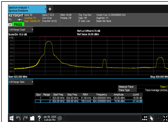
Band26(824-849)-5MHz-QPSK-26815-1RB#0-PASS
