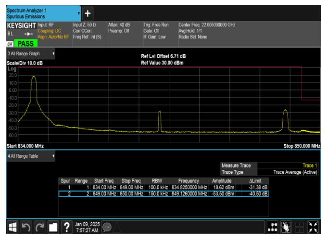
Band26(824-849)-15MHz-QPSK-26965-1RB#0-PASS
