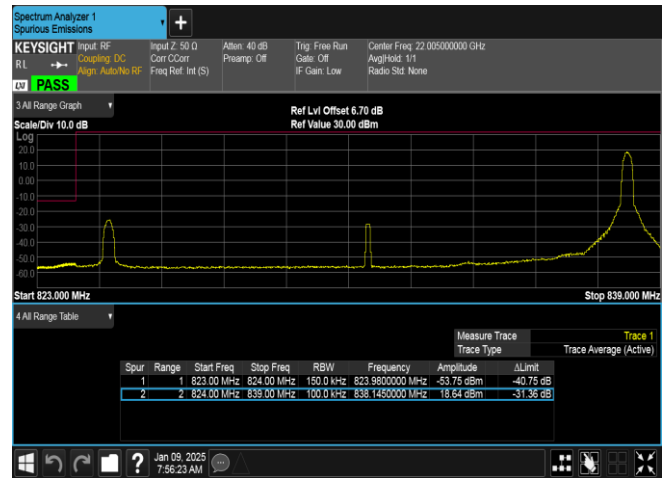
Band26(824-849)-15MHz-QPSK-26865-1RB#74-PASS
