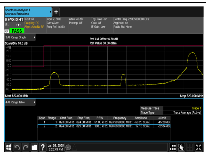
Band26(824-849)-5MHz-16QAM-26815-1RB#24-PASS
