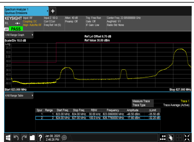
Band26(824-849)-3MHz-16QAM-26805-1RB#14-PASS
