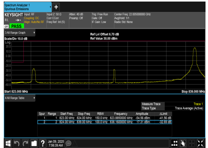
Band26(824-849)-15MHz-16QAM-26865-1RB#74-PASS
