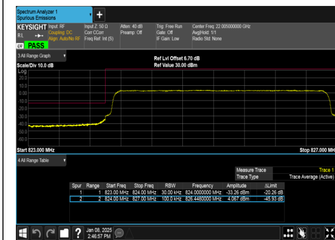
Band26(824-849)-3MHz-16QAM-26805-15RB#0-PASS
