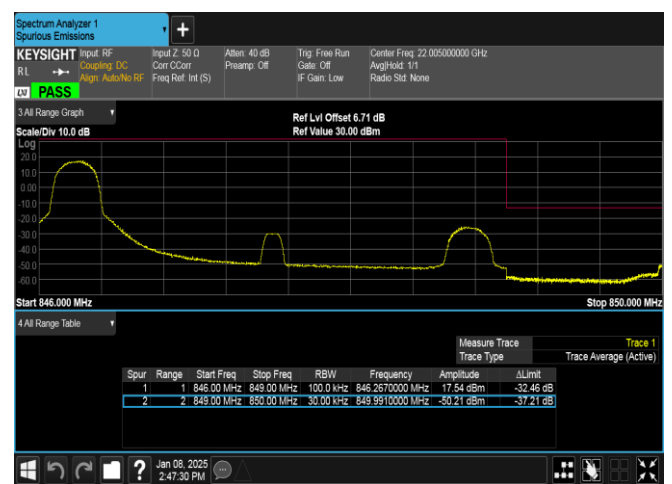
Band26(824-849)-3MHz-16QAM-27025-1RB#0-PASS
