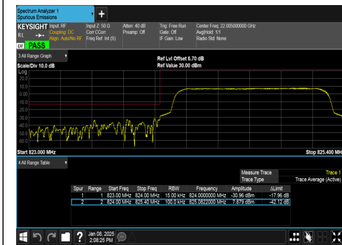
Band26(824-849)-1.4MHz-16QAM-26797-6RB#0-PASS
