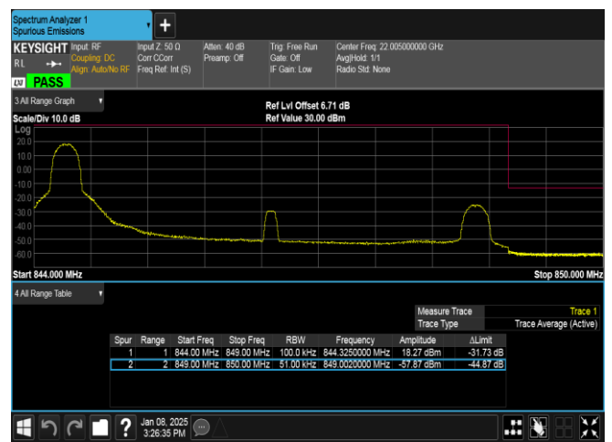
Band26(824-849)-5MHz-QPSK-27015-1RB#0-PASS
