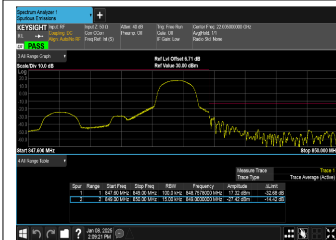
Band26(824-849)-1.4MHz-16QAM-27033-1RB#5-PASS
