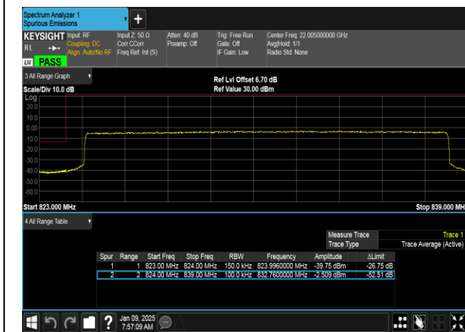
Band26(824-849)-15MHz-16QAM-26865-75RB#0-PASS
