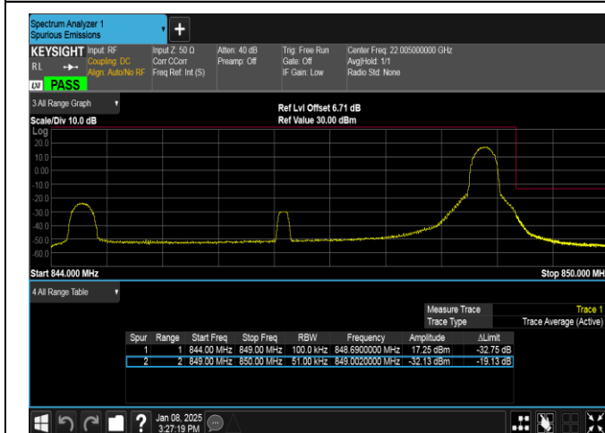
Band26(824-849)-5MHz-16QAM-27015-1RB#24-PASS
