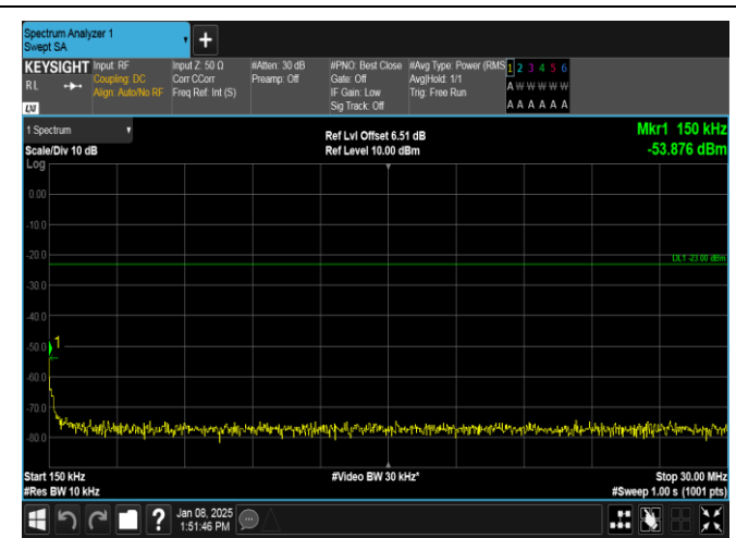
Band26(814-824)-10MHz-QPSK-26740-1RB#0-0.15~30-PASS
