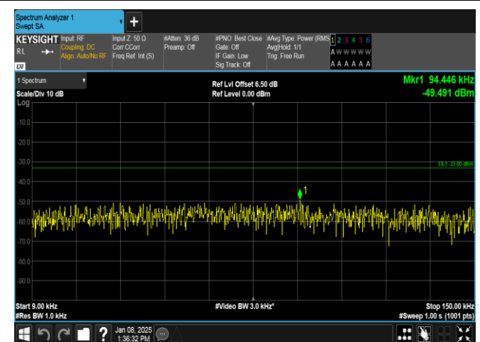
Band26(814-824)-5MHz-QPSK-26765-1RB#24-0.009~0.15-PASS
