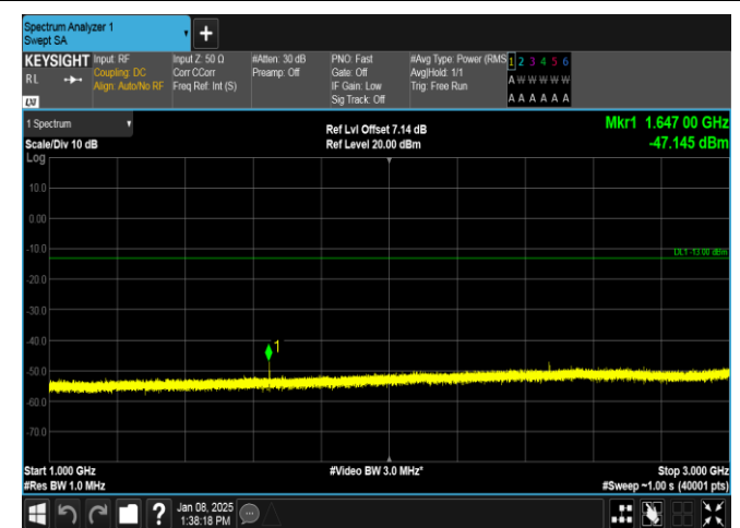
Band26(814-824)-5MHz-16QAM-26765-1RB#24-1000-3000-PASS
