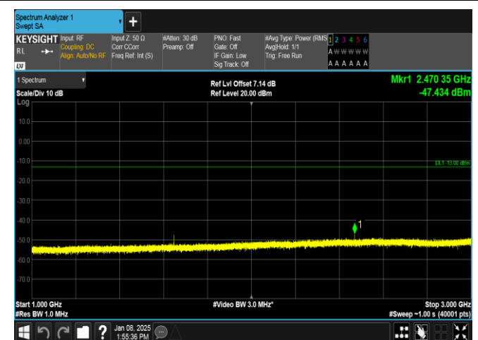
Band26(814-824)-10MHz-16QAM-26740-1RB#49-1000~3000-PASS
