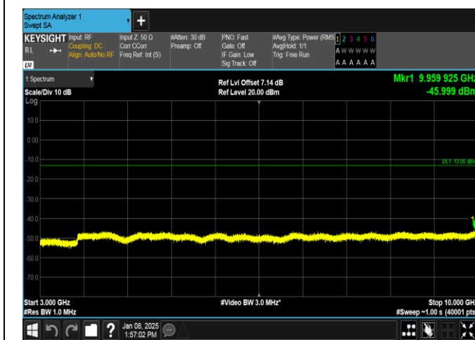
Band26(814-824)-10MHz-QPSK-26740-50RB#0-3000~10000-PASS
