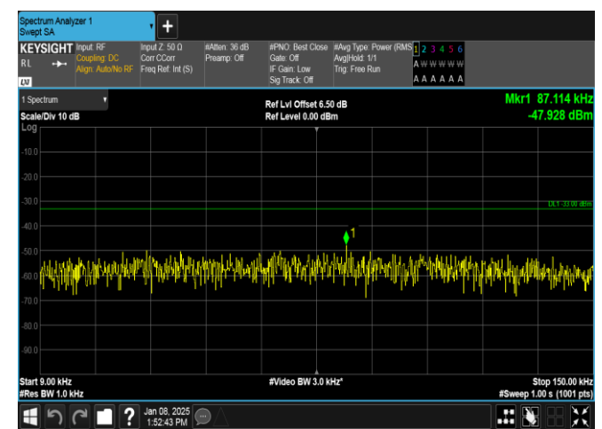
Band26(814-824)-10MHz-16QAM-26740-1RB#0-0.009~0.15-PASS
