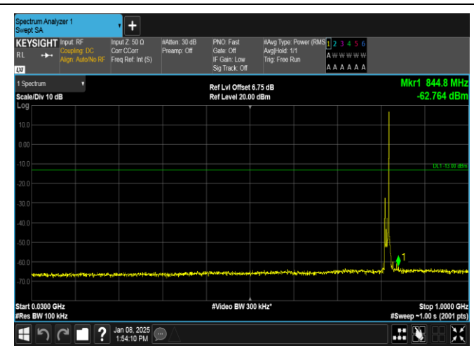
Band26(814-824)-10MHz-QPSK-26740-1RB#49-30~1000-PASS
