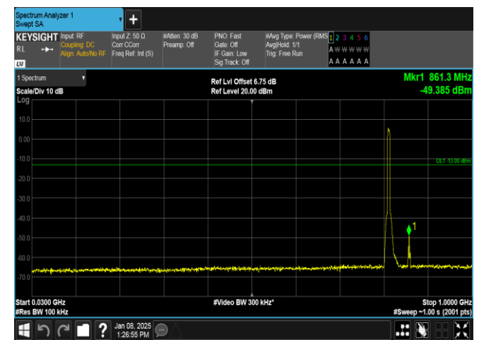
Band26(814-824)-5MHz-16QAM-26715-25RB#0-30~1000-PASS
