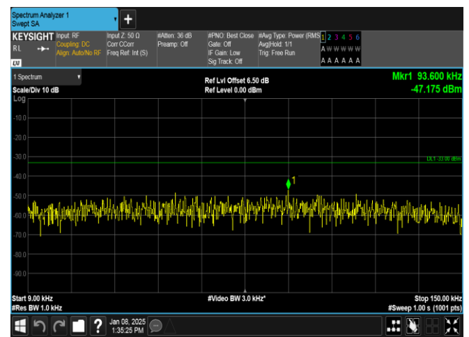
Band26(814-824)-5MHz-16QAM-26765-1RB#0-0.009~0.15-PASS
