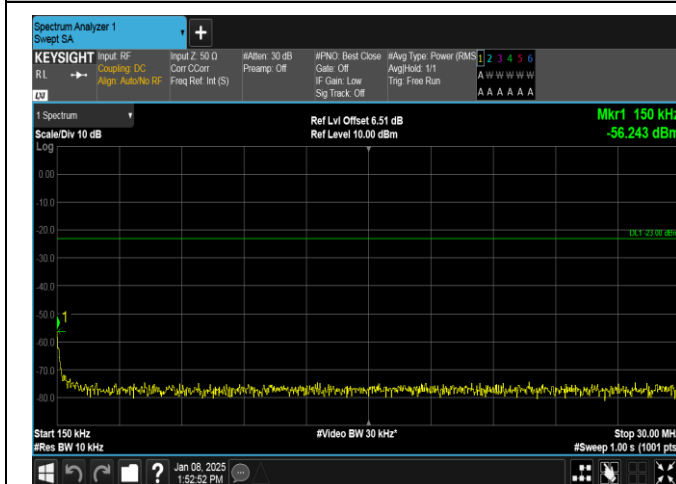
Band26(814-824)-10MHz-16QAM-26740-1RB#0-0.15~30-PASS
