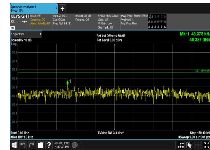
Band26(814-824)-5MHz-16QAM-26765-1RB#24-0.009-0.15-PASS
