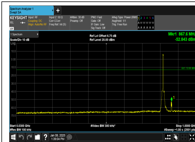
Band26(814-824)-5MHz-QPSK-26765-25RB#0-30~1000-PASS
