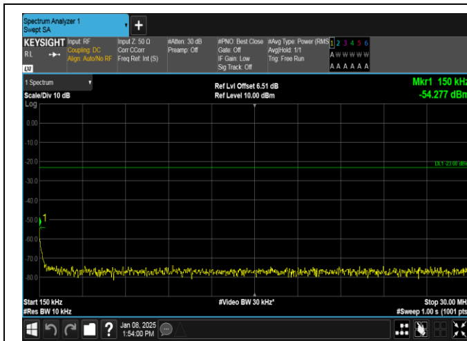
Band26(814-824)-10MHz-QPSK-26740-1RB#49-0.15~30-PASS
