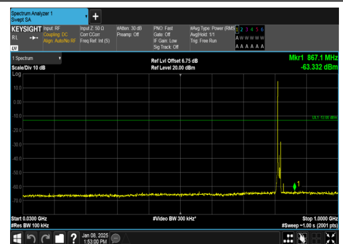
Band26(814-824)-10MHz-16QAM-26740-1RB#0-30~1000-PASS
