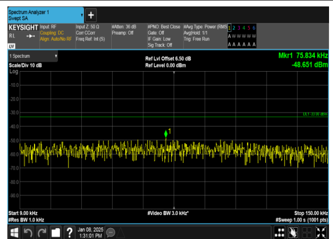
Band26(814-824)-5MHz-16QAM-26740-1RB#24-0.009~0.15-PASS
