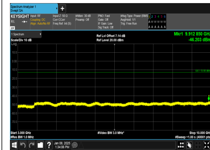
Band26(814-824)-5MHz-16QAM-26740-25RB#0-3000~10000-PASS
