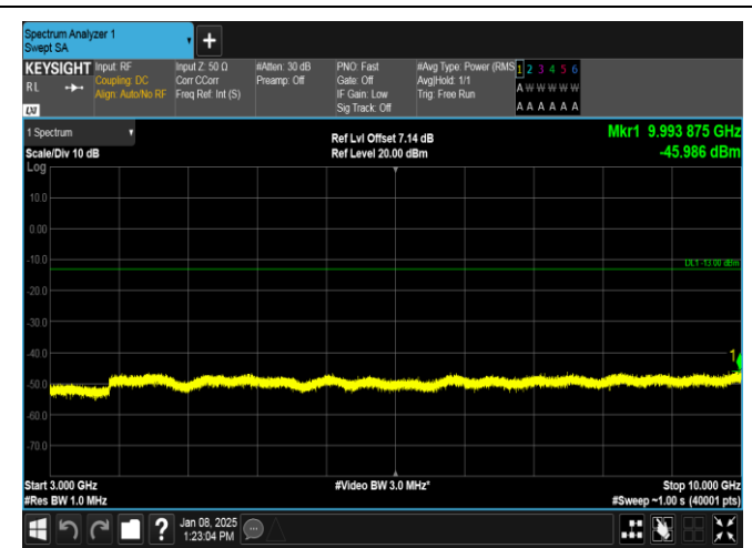
Band26(814-824)-5MHz-16QAM-26715-1RB#0-3000-10000-PASS
