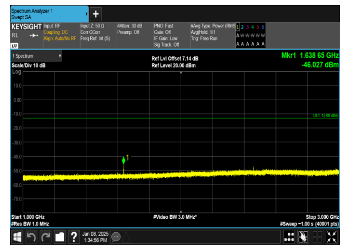
Band26(814-824)-5MHz-QPSK-26765-1RB#0-1000~3000-PASS
