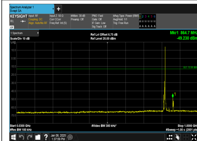
Band26(814-824)-5MHz-16QAM-26765-1RB#24-30-1000-PASS
