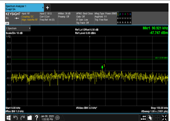
Band26(814-824)-10MHz-QPSK-26740-1RB#49-0.009~0.15-PASS
