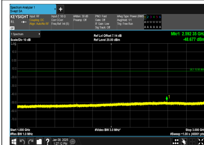
Band26(814-824)-5MHz-16QAM-26715-25RB#0-1000~3000-PASS
