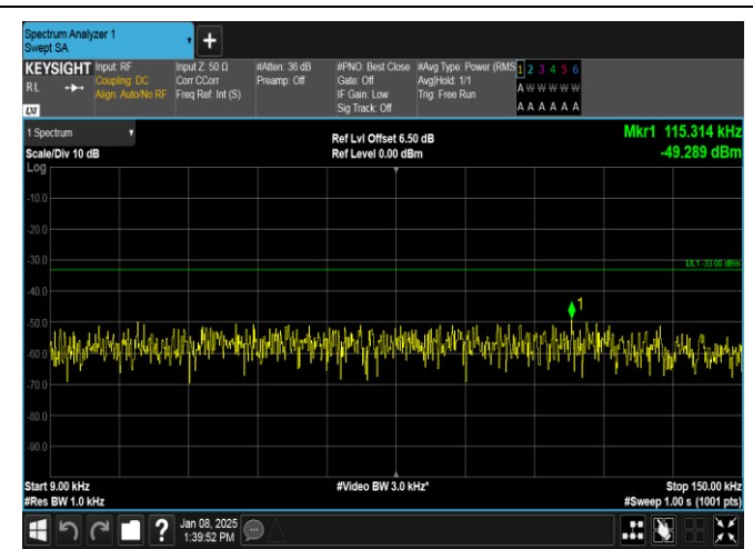
Band26(814-824)-5MHz-16QAM-26765-25RB#0-0.009~0.15-PASS
