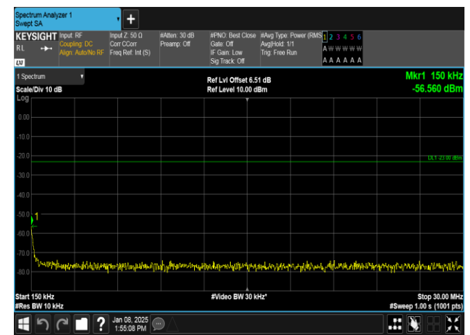
Band26(814-824)-10MHz-16QAM-26740-1RB#49-0.15~30-PASS
