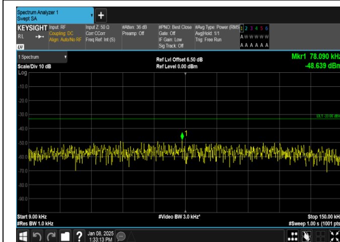
Band26(814-824)-5MHz-16QAM-26740-25RB#0-0.009~0.15-PASS
