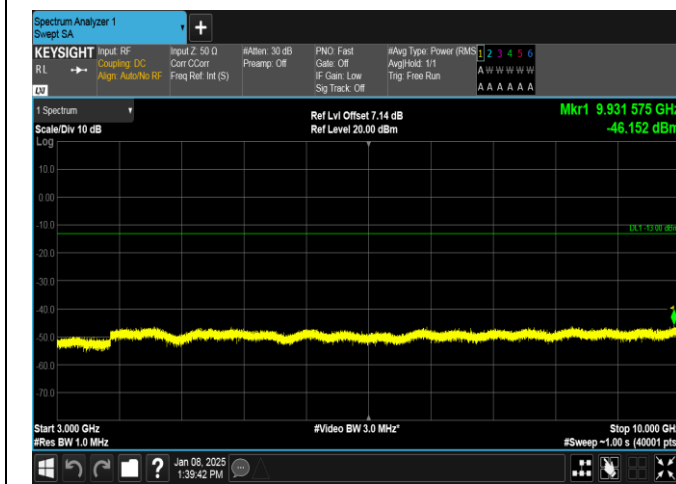
Band26(814-824)-5MHz-QPSK-26765-25RB#0-3000~10000-PASS
