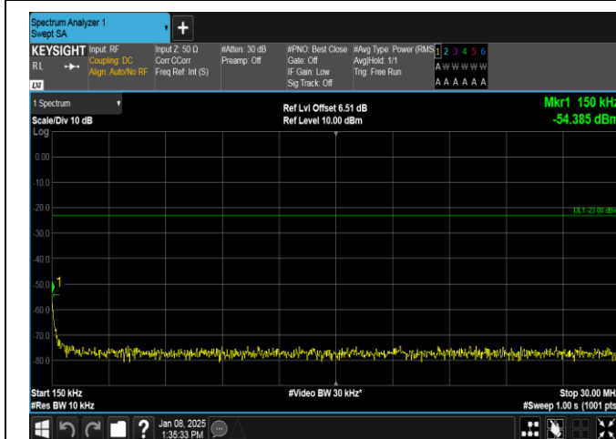
Band26(814-824)-5MHz-16QAM-26765-1RB#0-0.15~30-PASS
