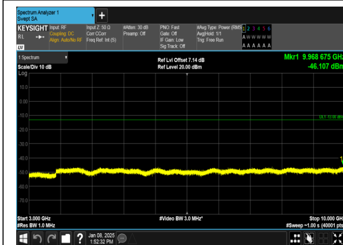
Band26(814-824)-10MHz-QPSK-26740-1RB#0-3000~10000-PASS
