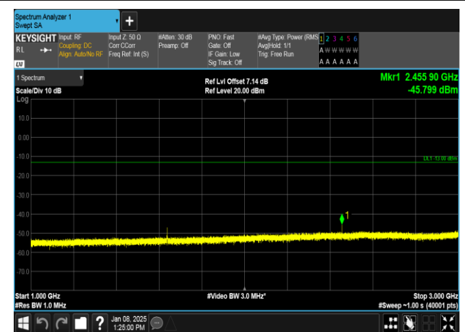
Band26(814-824)-5MHz-16QAM-26715-1RB#24-1000-3000-PASS
