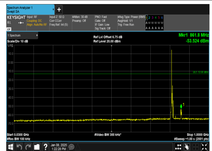
Band26(814-824)-5MHz-16QAM-26715-1RB#0-30~1000-PASS
