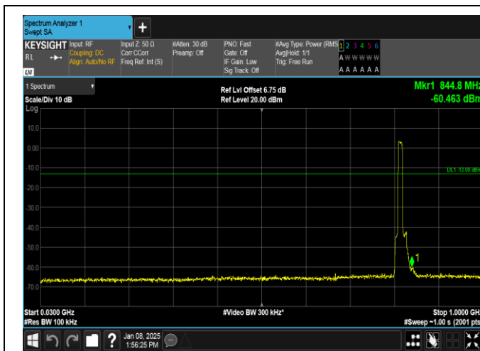
Band26(814-824)-10MHz-QPSK-26740-50RB#0-30~1000-PASS
