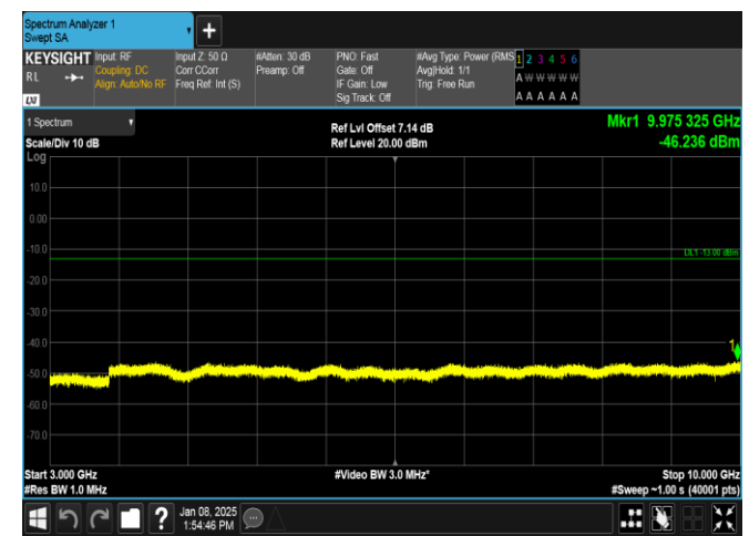
Band26(814-824)-10MHz-QPSK-26740-1RB#49-3000~10000-PASS
