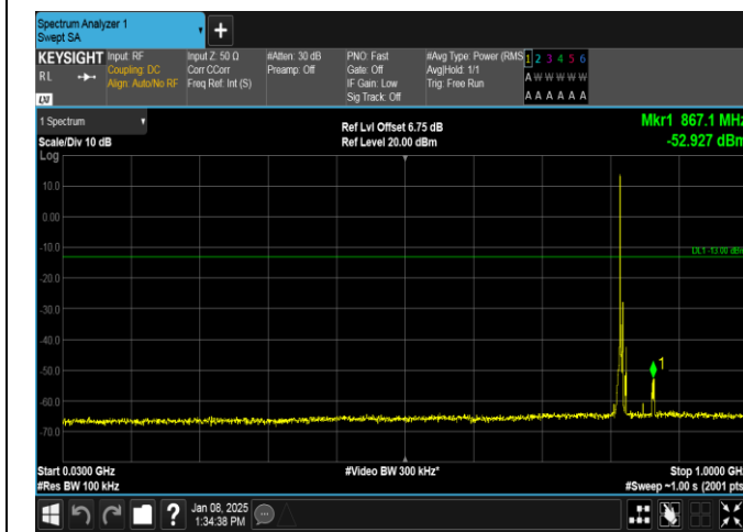
Band26(814-824)-5MHz-QPSK-26765-1RB#0-30~1000-PASS
