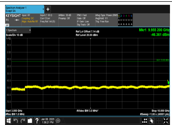
Band26(814-824)-5MHz-16QAM-26765-1RB#0-3000-10000-PASS
