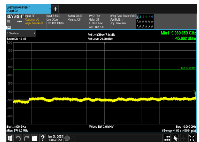
Band26(814-824)-5MHz-16QAM-26765-25RB#0-3000~10000-PASS
