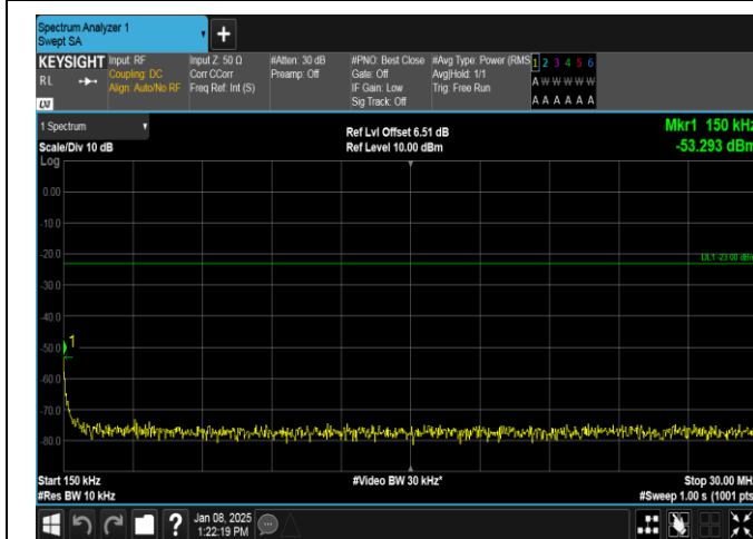
Band26(814-824)-5MHz-16QAM-26715-1RB#0-0.15~30-PASS
