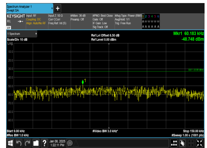
Band26(814-824)-5MHz-16QAM-26715-1RB#0-0.009~0.15-PASS
