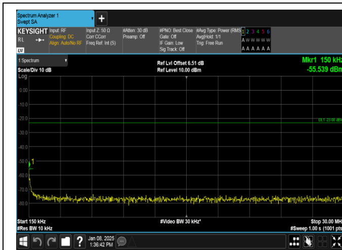
Band26(814-824)-5MHz-QPSK-26765-1RB#24-0.15~30-PASS
