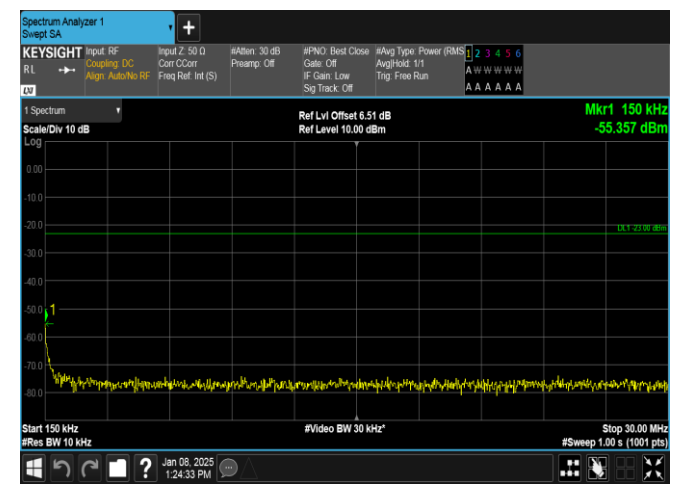
Band26(814-824)-5MHz-16QAM-26715-1RB#24-0.15-30-PASS
