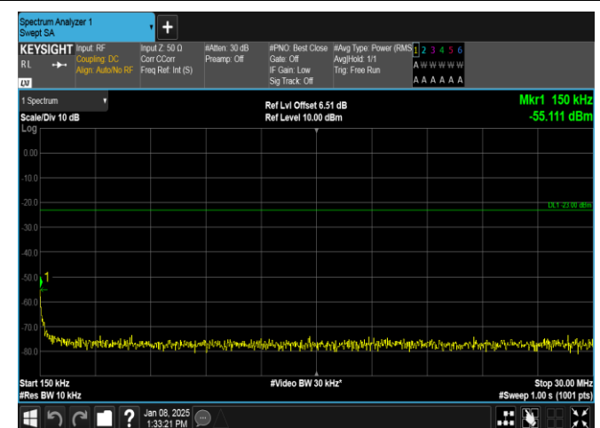
Band26(814-824)-5MHz-16QAM-26740-25RB#0-0.15~30-PASS
