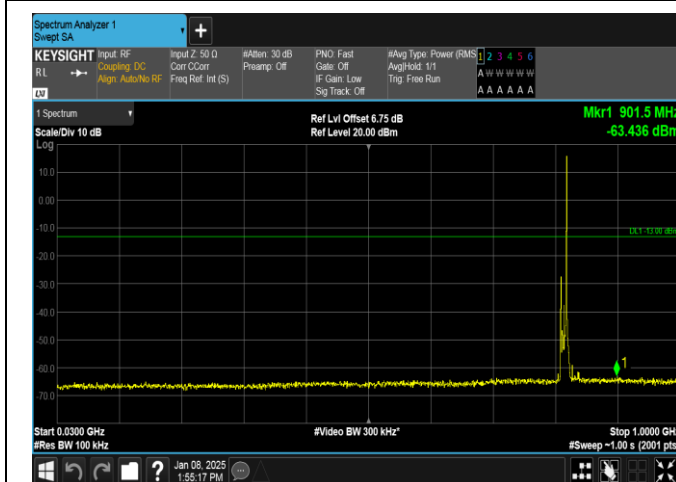
Band26(814-824)-10MHz-16QAM-26740-1RB#49-30~1000-PASS
