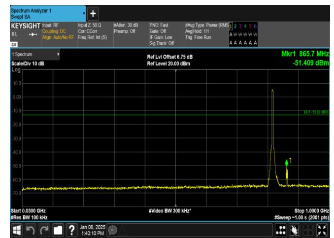
Band26(814-824)-5MHz-16QAM-26765-25RB#0-30~1000-PASS
