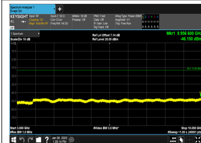
Band26(814-824)-5MHz-QPSK-26765-1RB#0-3000~10000-PASS
