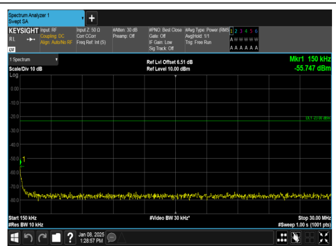
Band26(814-824)-5MHz-16QAM-26740-1RB#0-0.15~30-PASS
