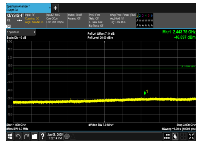
Band26(814-824)-10MHz-QPSK-26740-1RB#0-1000~3000-PASS
