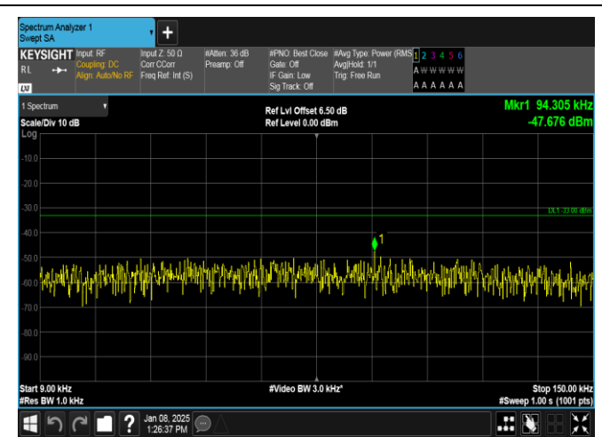
Band26(814-824)-5MHz-16QAM-26715-25RB#0-0.009~0.15-PASS
