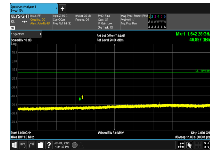
Band26(814-824)-5MHz-16QAM-26740-1RB#24-1000~3000-PASS
