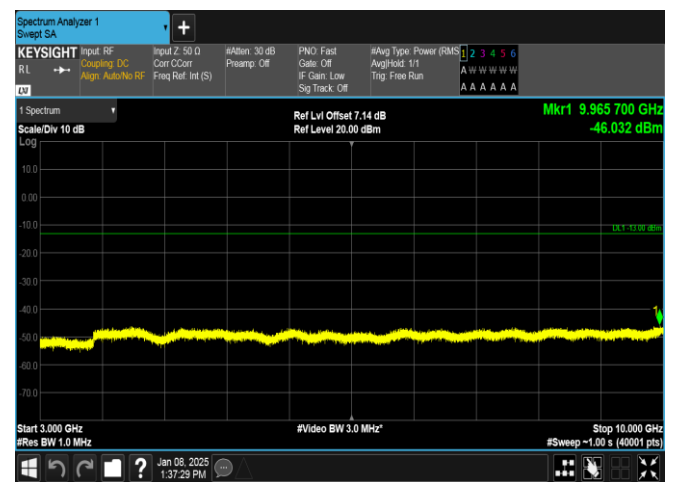
Band26(814-824)-5MHz-QPSK-26765-1RB#24-3000~10000-PASS
