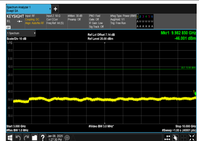
Band26(814-824)-5MHz-16QAM-26715-25RB#0-3000~10000-PASS
