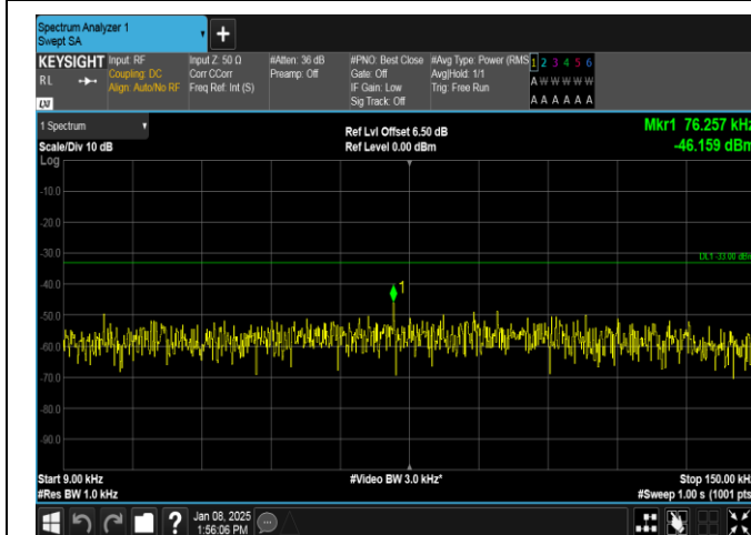
Band26(814-824)-10MHz-QPSK-26740-50RB#0-0.009~0.15-PASS
