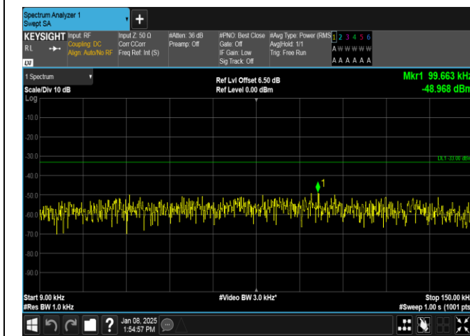
Band26(814-824)-10MHz-16QAM-26740-1RB#49-0.009~0.15-PASS
