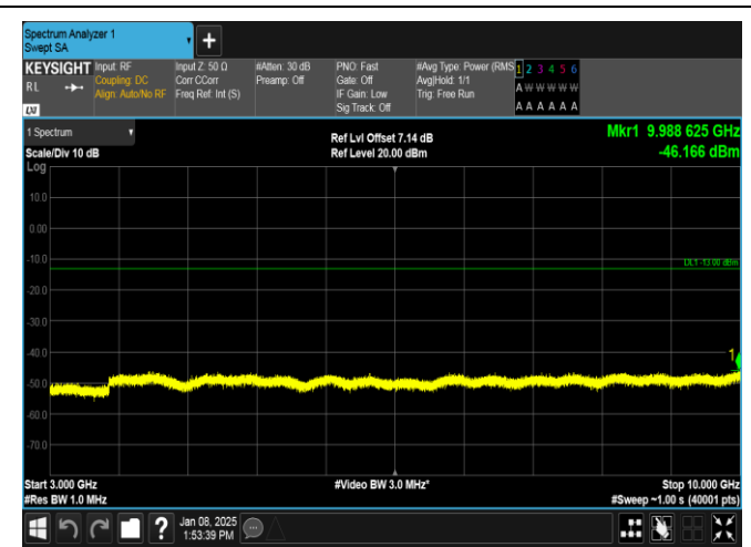
Band26(814-824)-10MHz-16QAM-26740-1RB#0-3000~10000-PASS
