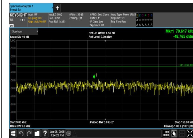
Band26(814-824)-5MHz-16QAM-26715-1RB#24-0.009-0.15-PASS
