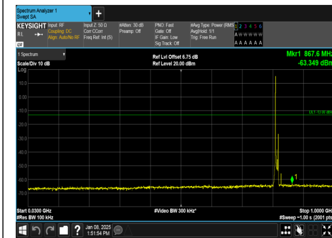
Band26(814-824)-10MHz-QPSK-26740-1RB#0-30~1000-PASS
