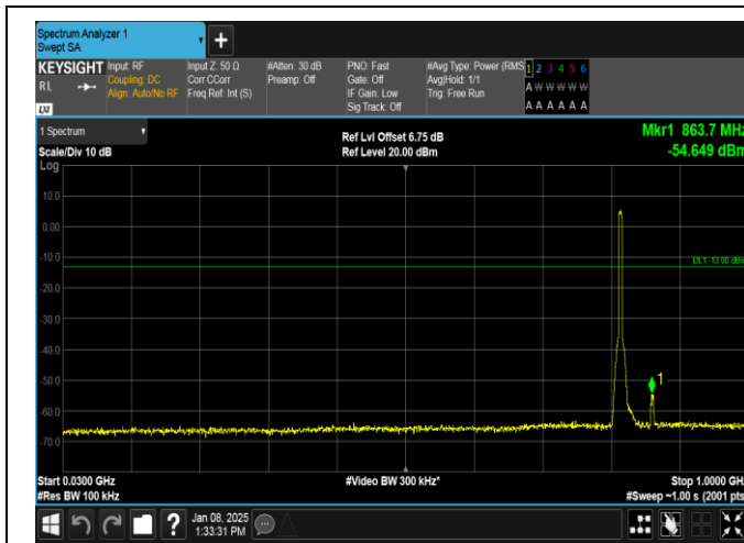
Band26(814-824)-5MHz-16QAM-26740-25RB#0-30~1000-PASS
