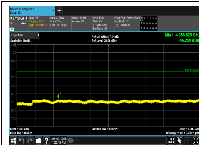
Band26(814-824)-5MHz-16QAM-26715-1RB#24-3000~10000-PASS
