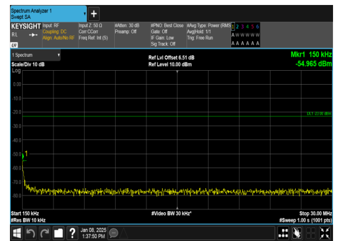
Band26(814-824)-5MHz-16QAM-26765-1RB#24-0.15-30-PASS
