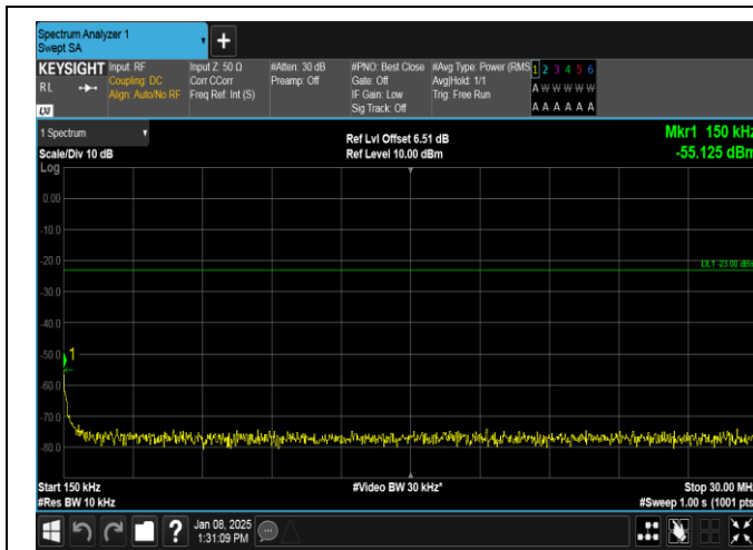
Band26(814-824)-5MHz-16QAM-26740-1RB#24-0.15~30-PASS
