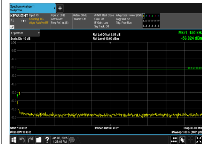
Band26(814-824)-5MHz-16QAM-26715-25RB#0-0.15~30-PASS
