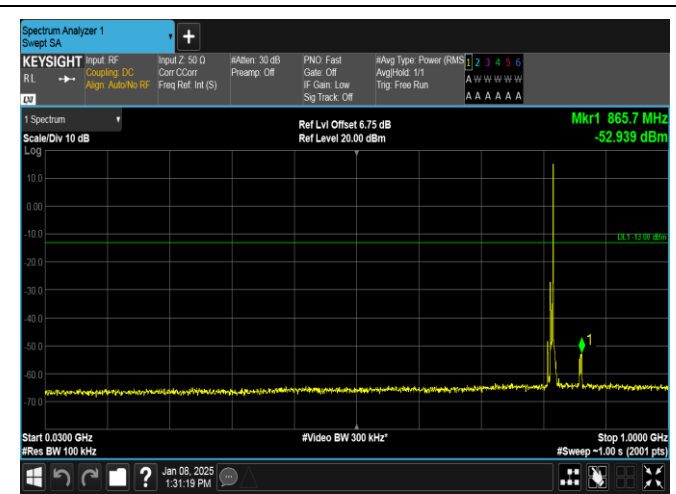
Band26(814-824)-5MHz-16QAM-26740-1RB#24-30~1000-PASS
