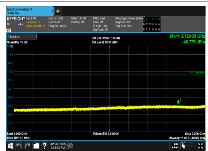
Band26(814-824)-5MHz-QPSK-26765-25RB#0-1000~3000-PASS
