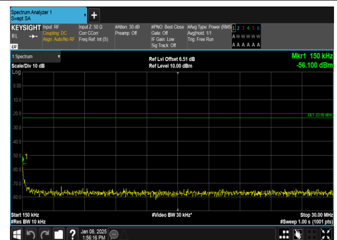
Band26(814-824)-10MHz-QPSK-26740-50RB#0-0.15~30-PASS
