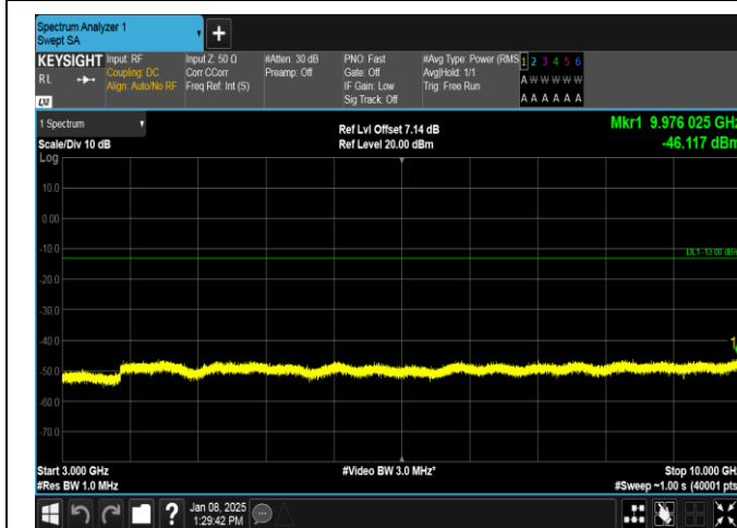
Band26(814-824)-5MHz-16QAM-26740-1RB#0-3000~10000-PASS
