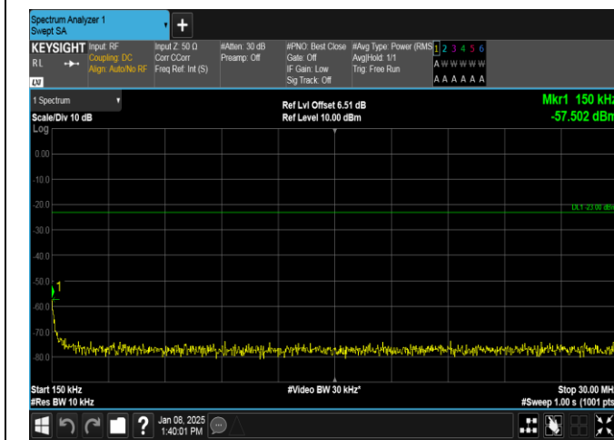
Band26(814-824)-5MHz-16QAM-26765-25RB#0-0.15~30-PASS
