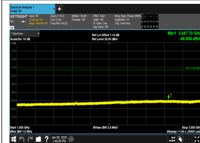
Band26(814-824)-5MHz-16QAM-26765-25RB#0-1000~3000-PASS
