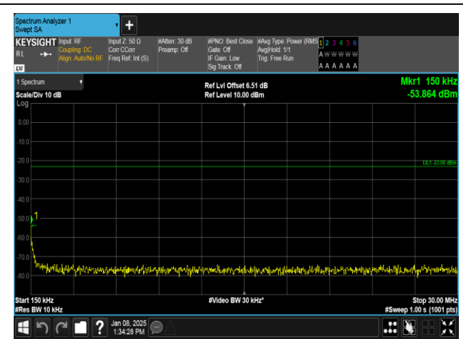
Band26(814-824)-5MHz-QPSK-26765-1RB#0-0.15~30-PASS
