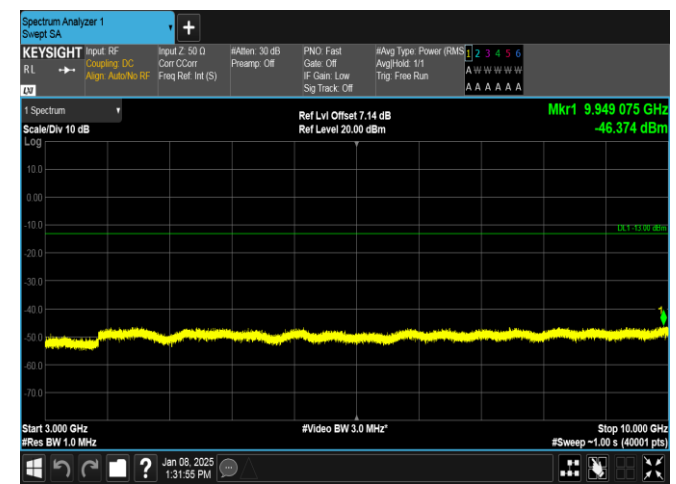
Band26(814-824)-5MHz-16QAM-26740-1RB#24-3000~10000-PASS
