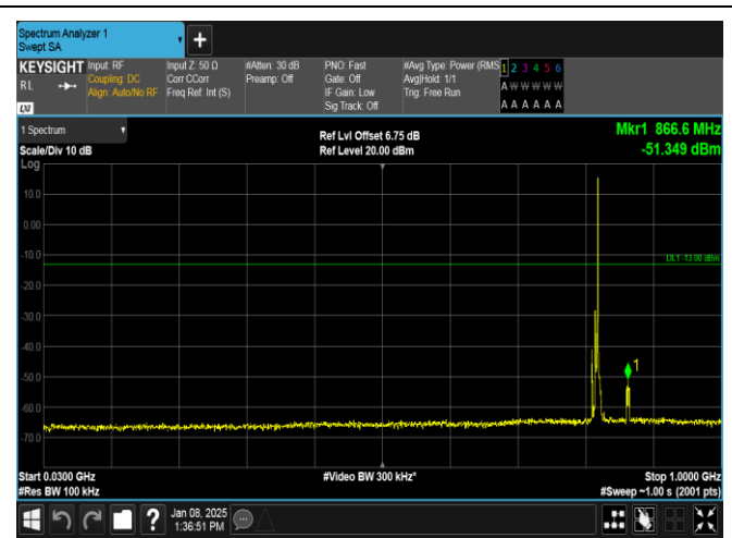
Band26(814-824)-5MHz-QPSK-26765-1RB#24-30~1000-PASS
