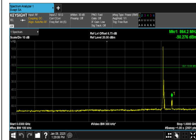
Band26(814-824)-5MHz-16QAM-26740-1RB#0-30~1000-PASS
