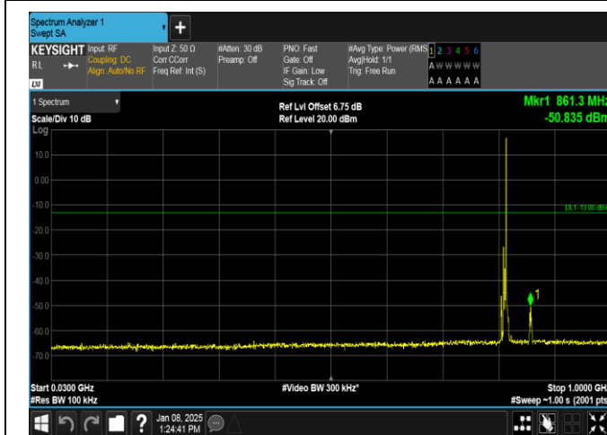
Band26(814-824)-5MHz-16QAM-26715-1RB#24-30-1000-PASS
