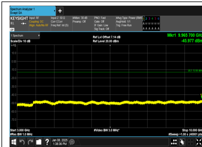
Band26(814-824)-5MHz-16QAM-26765-1RB#24-3000~10000-PASS
