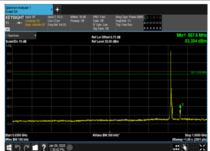
Band26(814-824)-5MHz-16QAM-26765-1RB#0-30~1000-PASS
