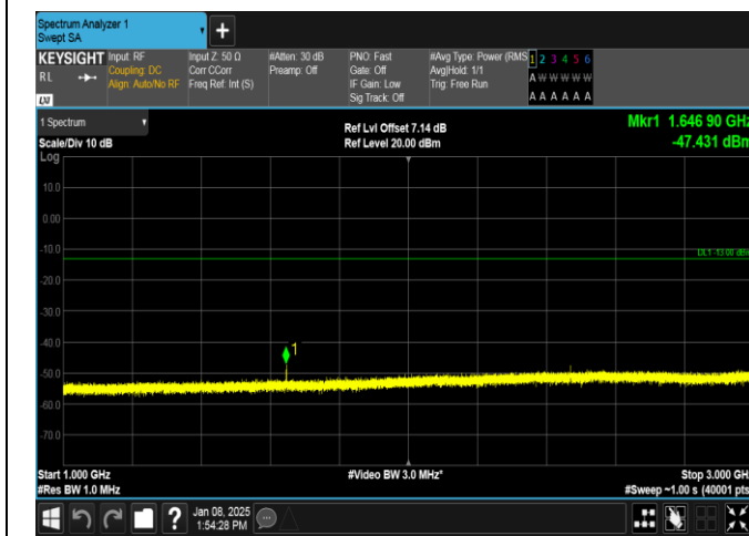
Band26(814-824)-10MHz-QPSK-26740-1RB#49-1000~3000-PASS
