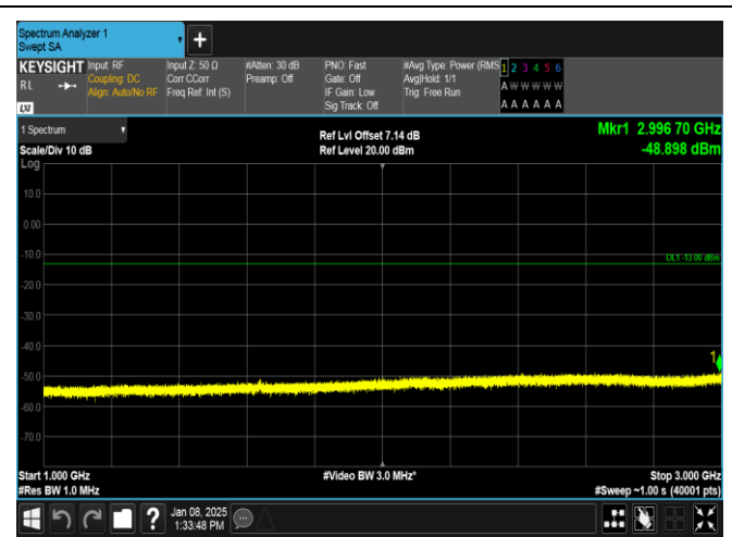
Band26(814-824)-5MHz-16QAM-26740-25RB#0-1000~3000-PASS
