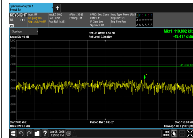
Band26(814-824)-5MHz-QPSK-26740-1RB#24-0.009~0.15-PASS
