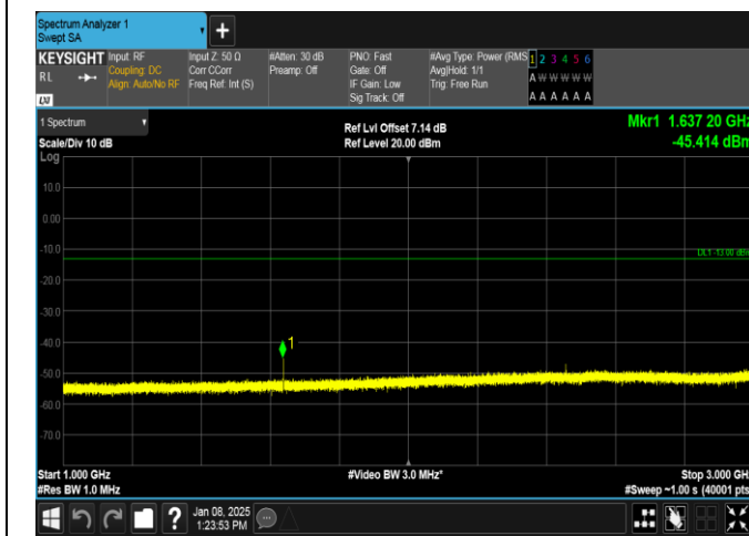
Band26(814-824)-5MHz-QPSK-26715-1RB#24-1000~3000-PASS
