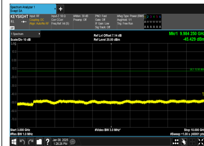
Band26(814-824)-5MHz-QPSK-26715-25RB#0-3000~10000-PASS
