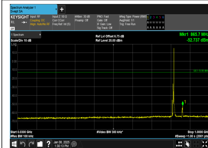
Band26(814-824)-5MHz-QPSK-26740-1RB#24-30~1000-PASS
