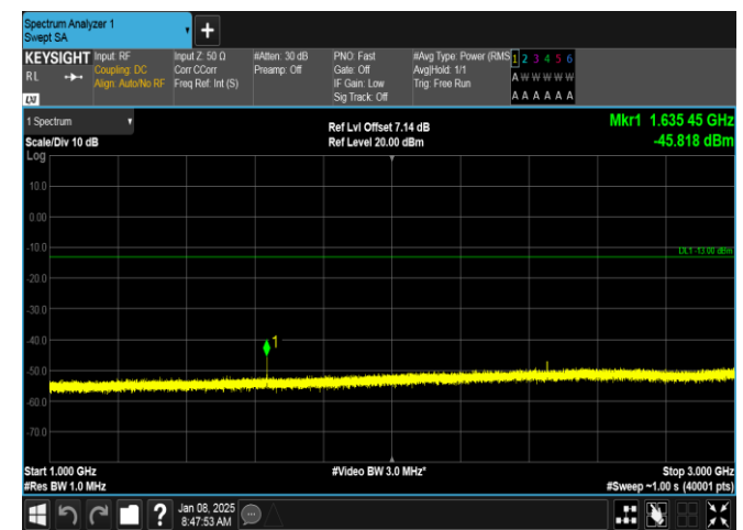
Band26(814-824)-3MHz-16QAM-26740-1RB#0-1000~3000-PASS
