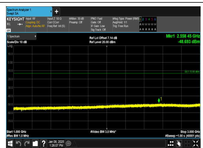
Band26(814-824)-5MHz-QPSK-26715-25RB#0-1000~3000-PASS
