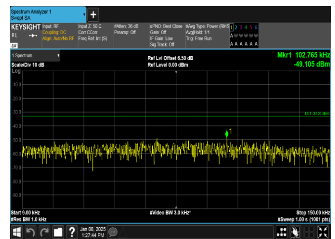
Band26(814-824)-5MHz-QPSK-26740-1RB#0-0.009~0.15-PASS
