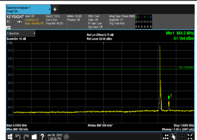
Band26(814-824)-5MHz-QPSK-26740-1RB#0-30~1000-PASS
