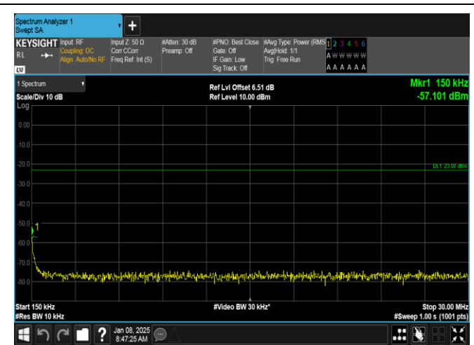
Band26(814-824)-3MHz-16QAM-26740-1RB#0-0.15~30-PASS
