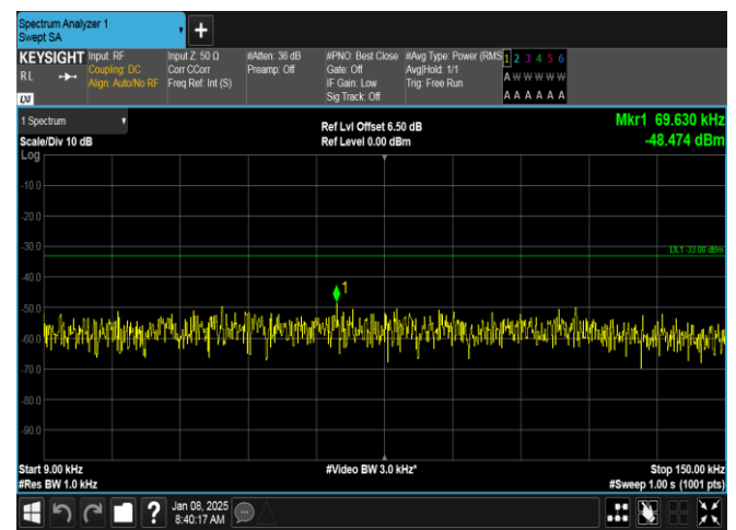
Band26(814-824)-3MHz-16QAM-26705-1RB#0-0.009~0.15-PASS
