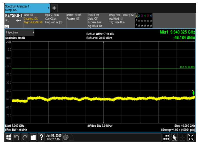
Band26(814-824)-3MHz-QPSK-26775-1RB#14-3000~10000-PASS
