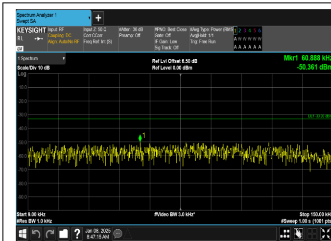
Band26(814-824)-3MHz-16QAM-26740-1RB#0-0.009~0.15-PASS
