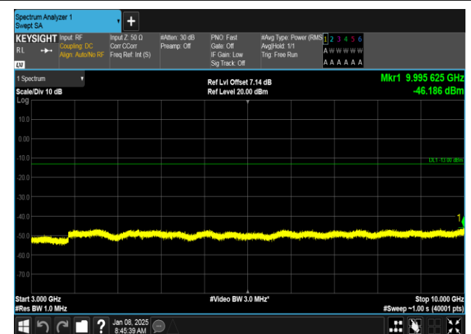
Band26(814-824)-3MHz-16QAM-26705-15RB#0-3000~10000-PASS
