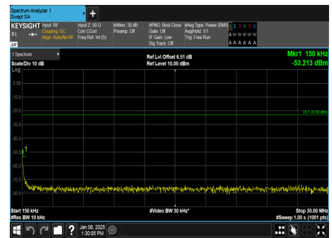
Band26(814-824)-5MHz-QPSK-26740-1RB#24-0.15~30-PASS
