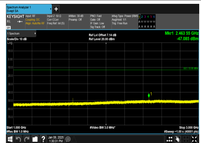
Band26(814-824)-5MHz-QPSK-26740-1RB#24-1000~3000-PASS
