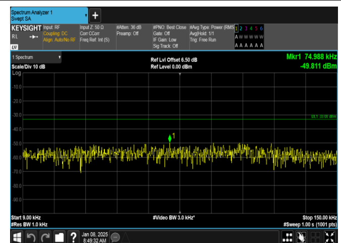
Band26(814-824)-3MHz-16QAM-26740-1RB#14-0.009~0.15-PASS
