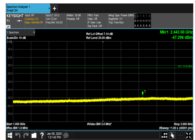
Band26(814-824)-5MHz-QPSK-26715-1RB#0-1000~3000-PASS
