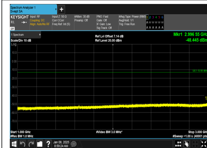
Band26(814-824)-3MHz-16QAM-26775-15RB#0-1000~3000-PASS
