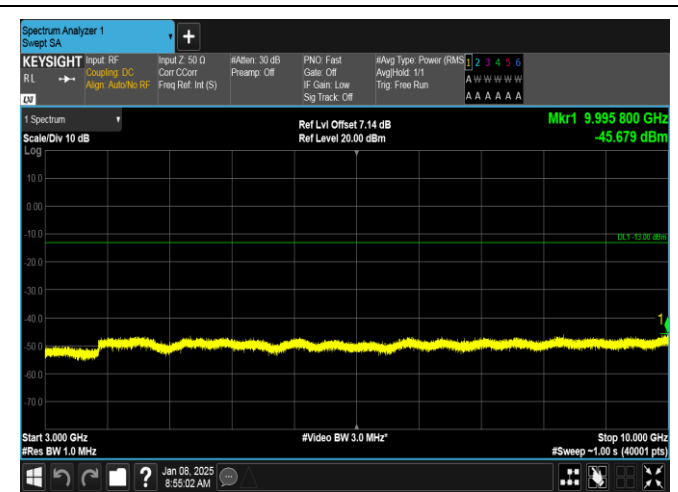
Band26(814-824)-3MHz-16QAM-26775-1RB#0-3000-10000-PASS
