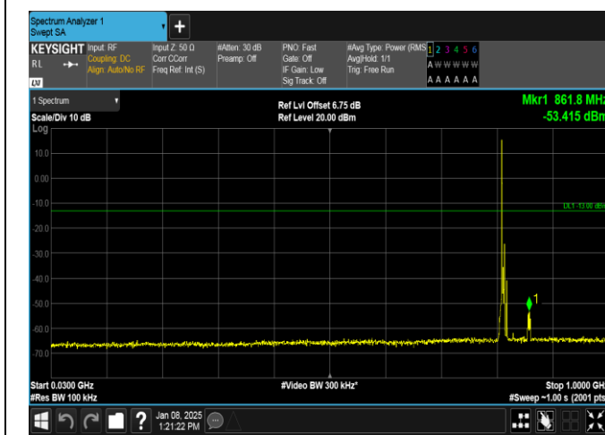
Band26(814-824)-5MHz-QPSK-26715-1RB#0-30~1000-PASS
