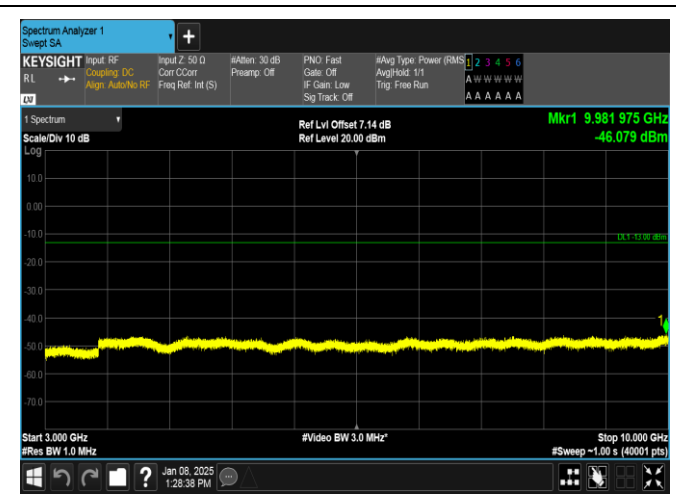
Band26(814-824)-5MHz-QPSK-26740-1RB#0-3000~10000-PASS
