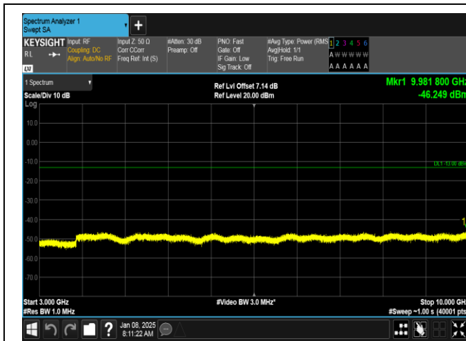
Band26(814-824)-1.4MHz-QPSK-26740-1RB#5-3000~10000-PASS
