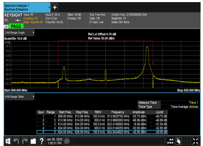
Band26(814-824)-10MHz-QPSK-26740-1RB#49-PASS
