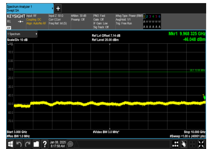
Band26(814-824)-1.4MHz-QPSK-26783-1RB#5-3000~10000-PASS
