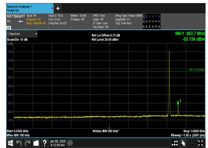
Band26(814-824)-1.4MHz-QPSK-26740-6RB#0-30~1000-PASS
