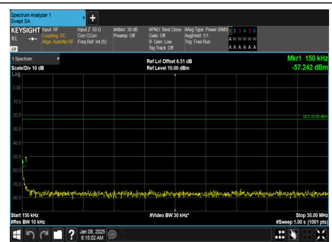
Band26(814-824)-1.4MHz-QPSK-26783-1RB#0-0.15~30-PASS
