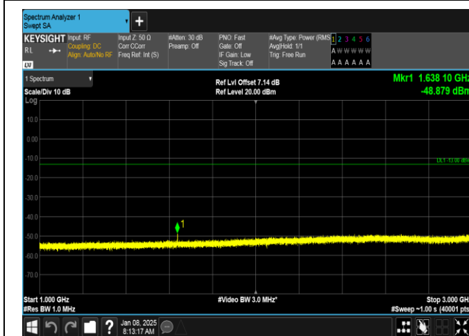
Band26(814-824)-1.4MHz-QPSK-26740-6RB#0-1000~3000-PASS
