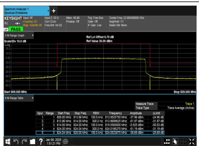
Band26(814-824)-10MHz-16QAM-26740-50RB#0-PASS
