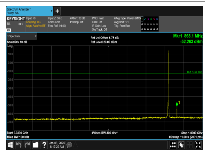
Band26(814-824)-1.4MHz-QPSK-26783-1RB#5-30~1000-PASS
