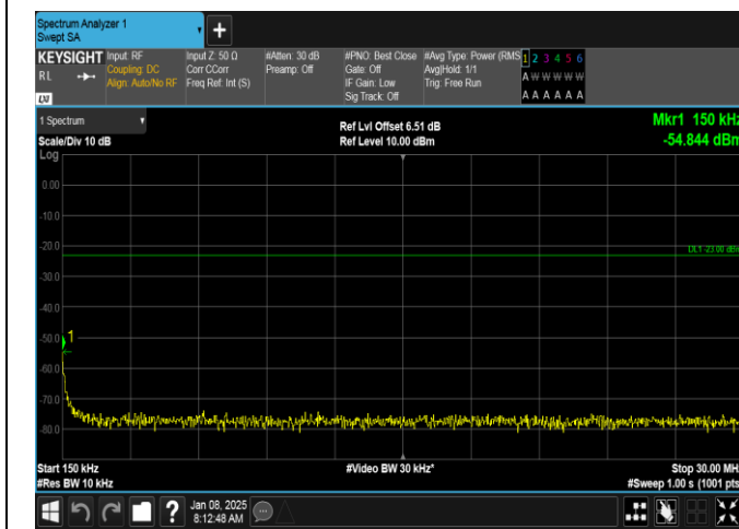
Band26(814-824)-1.4MHz-QPSK-26740-6RB#0-0.15~30-PASS
