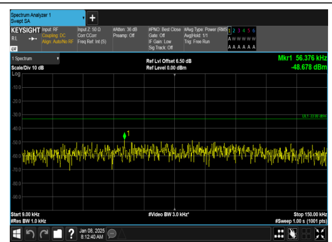
Band26(814-824)-1.4MHz-QPSK-26740-6RB#0-0.009~0.15-PASS
