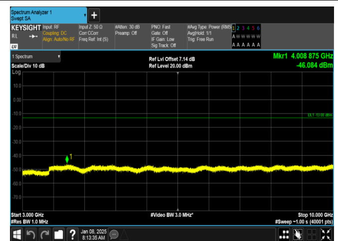
Band26(814-824)-1.4MHz-QPSK-26740-6RB#0-3000~10000-PASS
