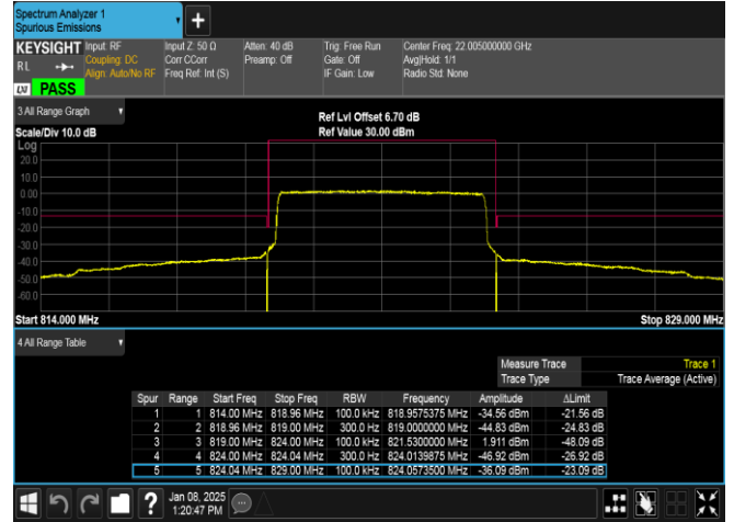
Band26(814-824)-5MHz-16QAM-26765-25RB#0-PASS
