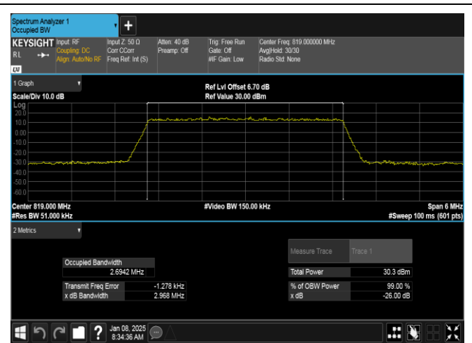
Band26(814-824)-3MHz-QPSK-26740-15RB#0-PASS
