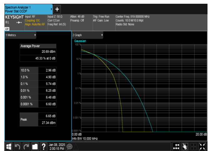
Band26(814-824)-10MHz-16QAM-26740-50RB#0-PASS
