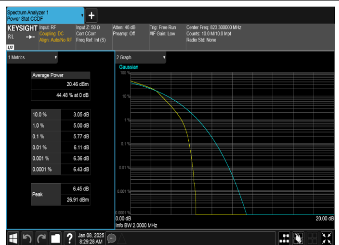
Band26(814-824)-1.4MHz-16QAM-26783-6RB#0-PASS
