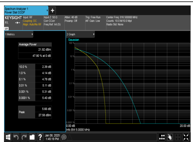
Band26(814-824)-5MHz-QPSK-26715-25RB#0-PASS
