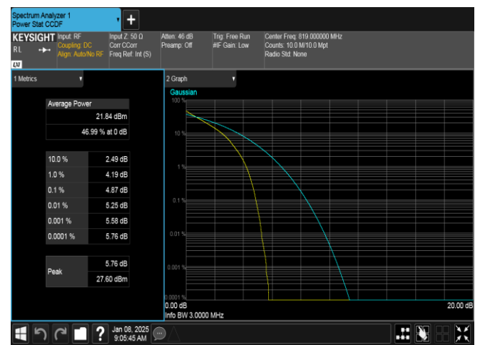
Band26(814-824)-3MHz-QPSK-26740-15RB#0-PASS
