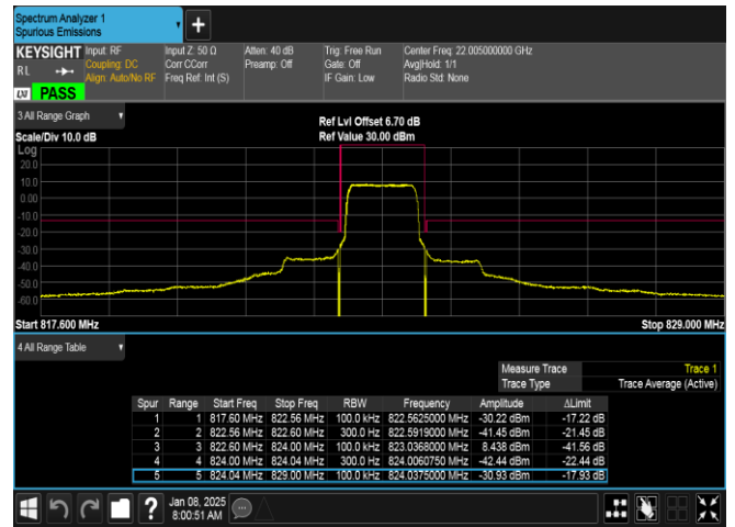
Band26(814-824)-1.4MHz-QPSK-26783-6RB#0-PASS
