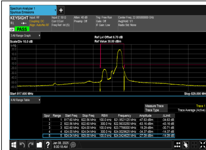
Band26(814-824)-1.4MHz-QPSK-26783-1RB#5-PASS
