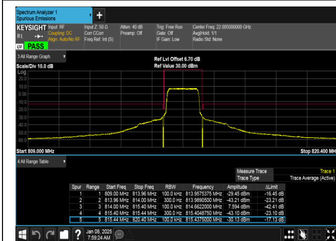
Band26(814-824)-1.4MHz-16QAM-26697-6RB#0-PASS
