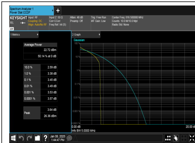
Band26(814-824)-5MHz-QPSK-26715-1RB#0-PASS
