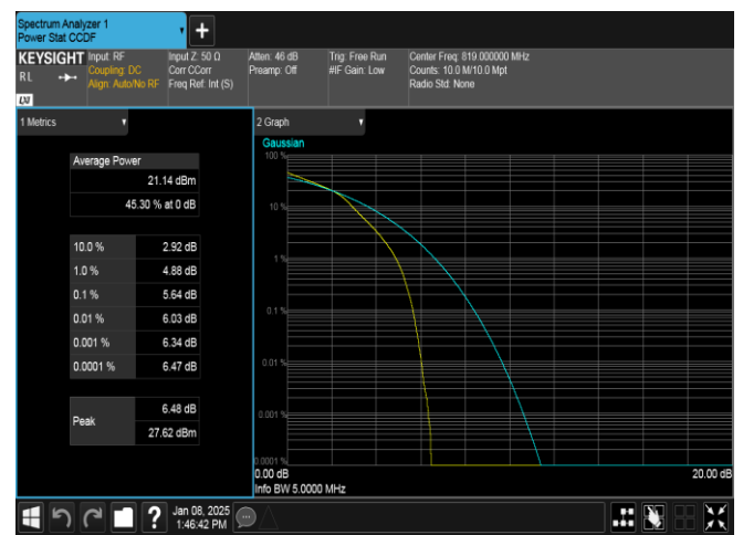
Band26(814-824)-5MHz-16QAM-26740-25RB#0-PASS
