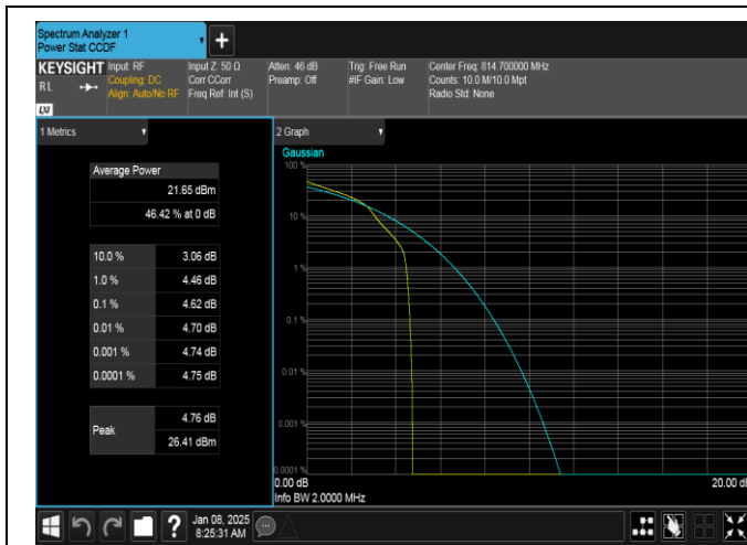
Band26(814-824)-1.4MHz-16QAM-26697-1RB#0-PASS
