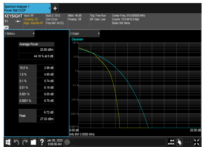
Band26(814-824)-3MHz-16QAM-26740-15RB#0-PASS
