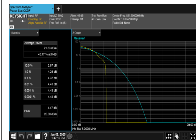
Band26(814-824)-5MHz-16QAM-26765-1RB#0-PASS
