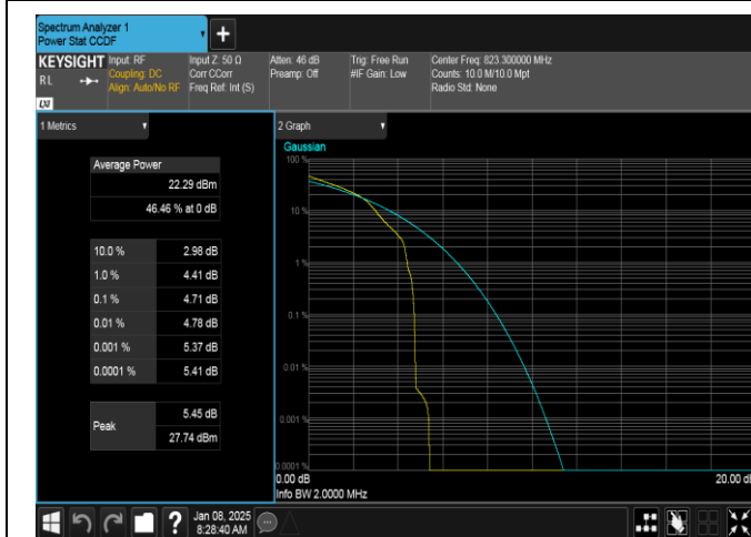
Band26(814-824)-1.4MHz-16QAM-26783-1RB#0-PASS
