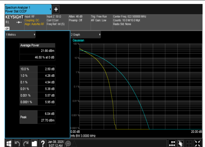
Band26(814-824)-3MHz-QPSK-26775-15RB#0-PASS
