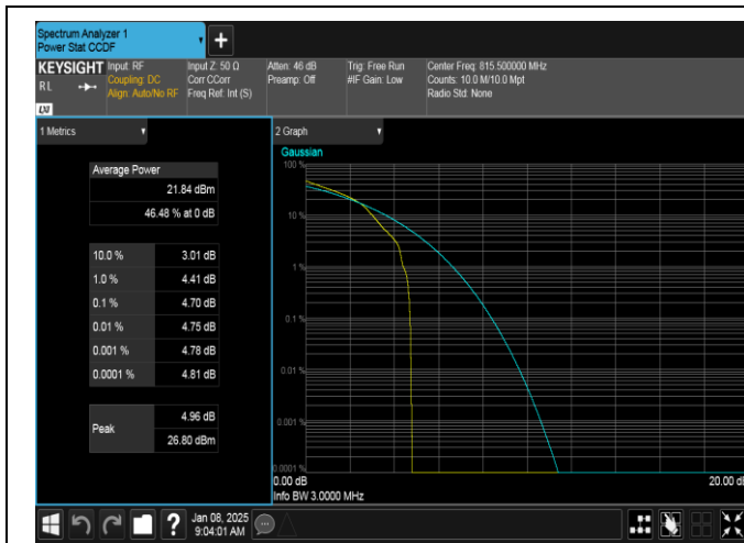
Band26(814-824)-3MHz-16QAM-26705-1RB#0-PASS
