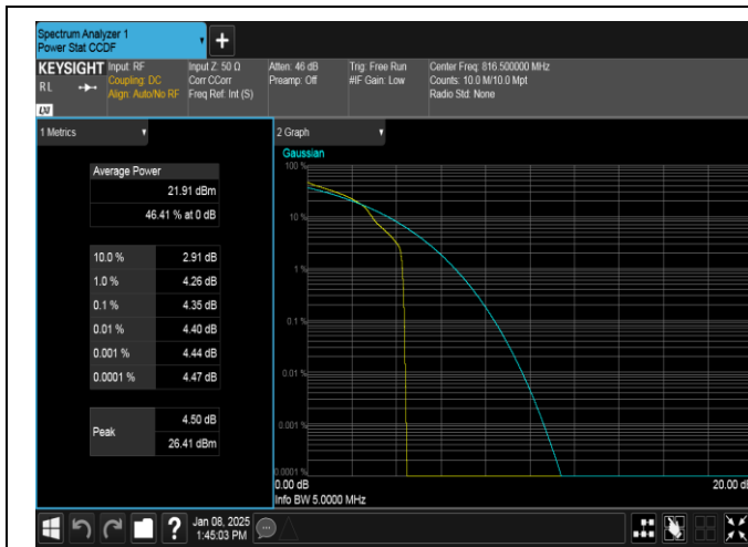
Band26(814-824)-5MHz-16QAM-26715-1RB#0-PASS
