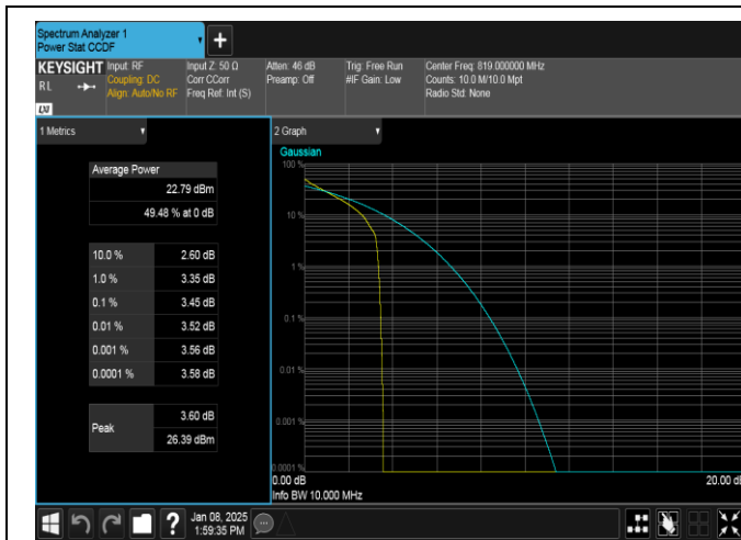
Band26(814-824)-10MHz-QPSK-26740-1RB#0-PASS
