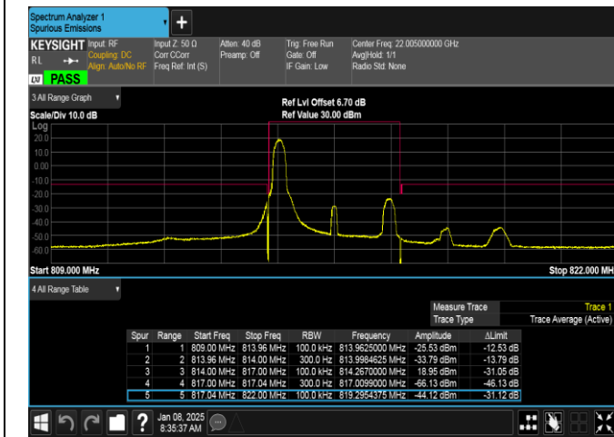
Band26(814-824)-3MHz-QPSK-26705-1RB#0-PASS
