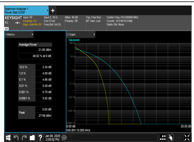
Band26(814-824)-10MHz-QPSK-26740-50RB#0-PASS
