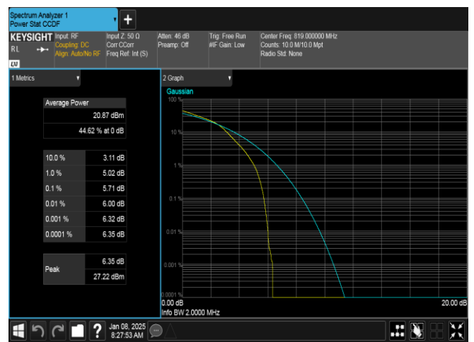
Band26(814-824)-1.4MHz-16QAM-26740-6RB#0-PASS
