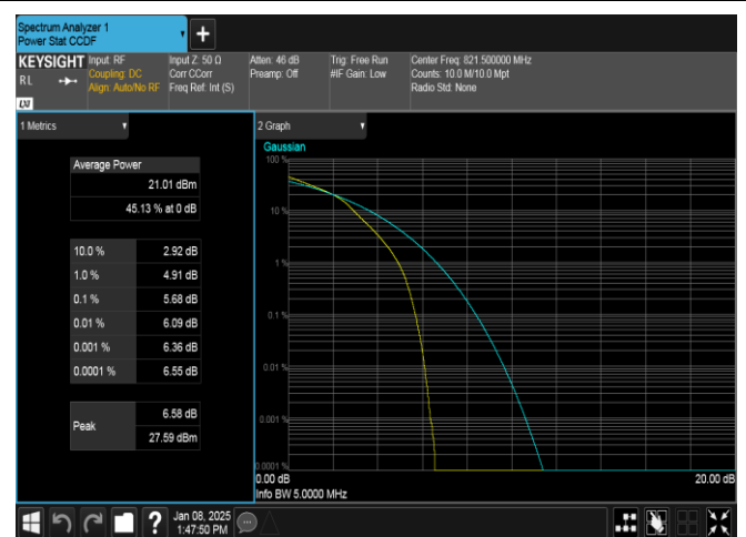
Band26(814-824)-5MHz-16QAM-26765-25RB#0-PASS
