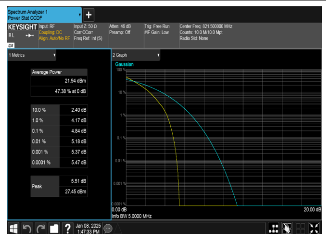
Band26(814-824)-5MHz-QPSK-26765-25RB#0-PASS
