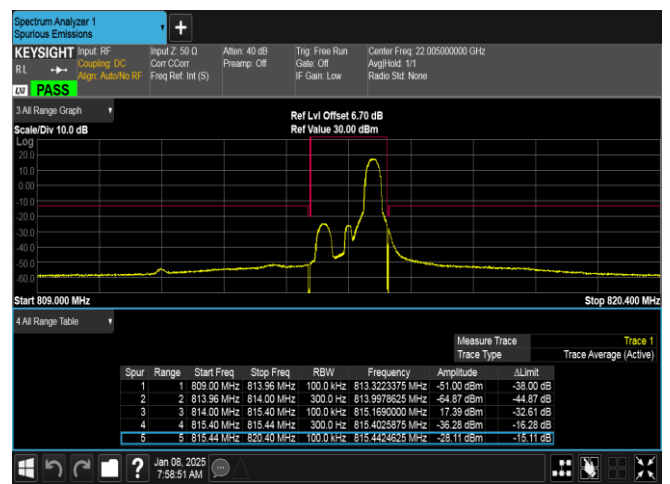
Band26(814-824)-1.4MHz-16QAM-26697-1RB#5-PASS
