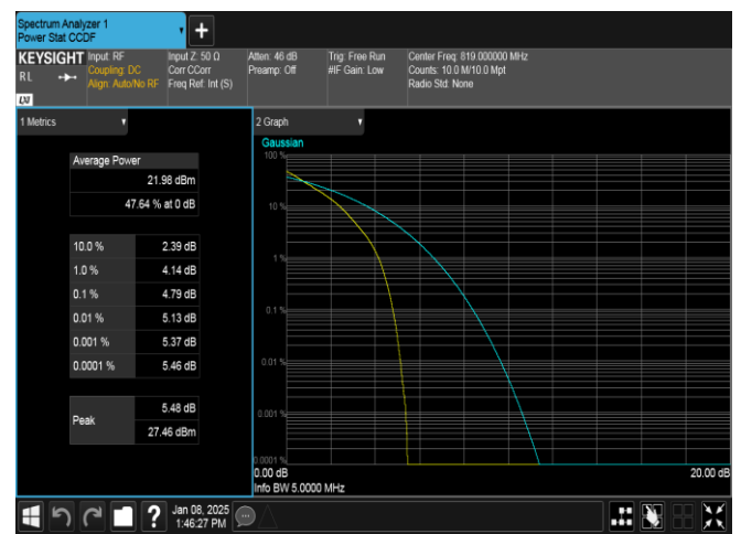
Band26(814-824)-5MHz-QPSK-26740-25RB#0-PASS
