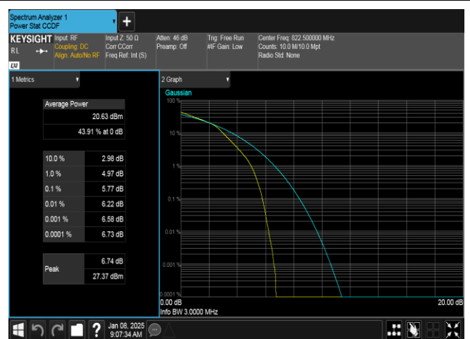
Band26(814-824)-3MHz-16QAM-26775-15RB#0-PASS
