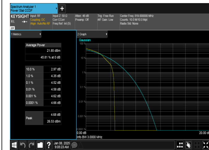
Band26(814-824)-3MHz-16QAM-26740-1RB#0-PASS
