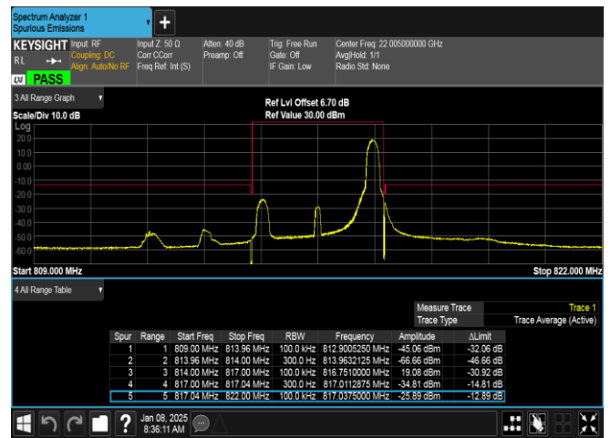
Band26(814-824)-3MHz-QPSK-26705-1RB#14-PASS
