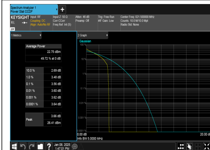
Band26(814-824)-5MHz-QPSK-26765-1RB#0-PASS
