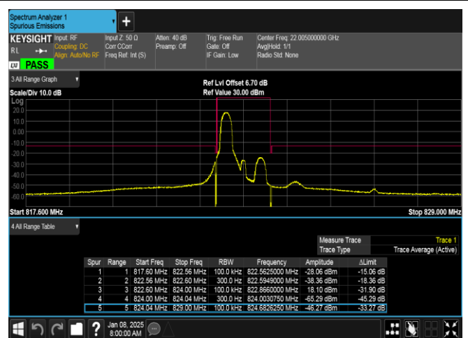
Band26(814-824)-1.4MHz-16QAM-26783-1RB#0-PASS
