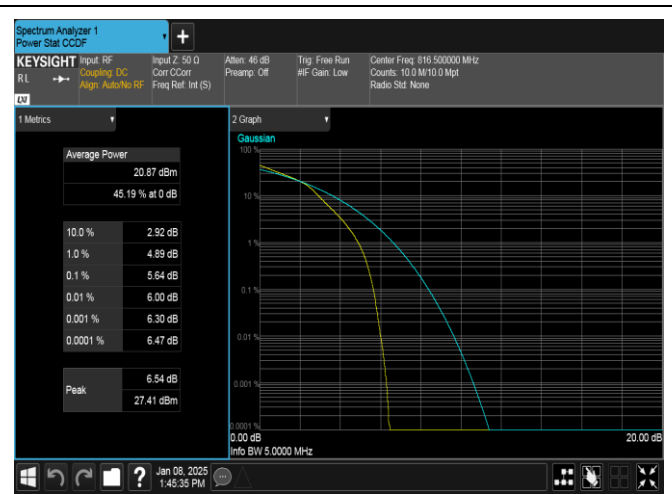
Band26(814-824)-5MHz-16QAM-26715-25RB#0-PASS
