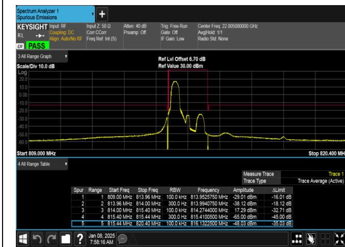
Band26(814-824)-1.4MHz-16QAM-26697-1RB#0-PASS
