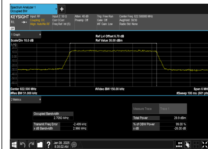
Band26(814-824)-3MHz-QPSK-26775-15RB#0-PASS
