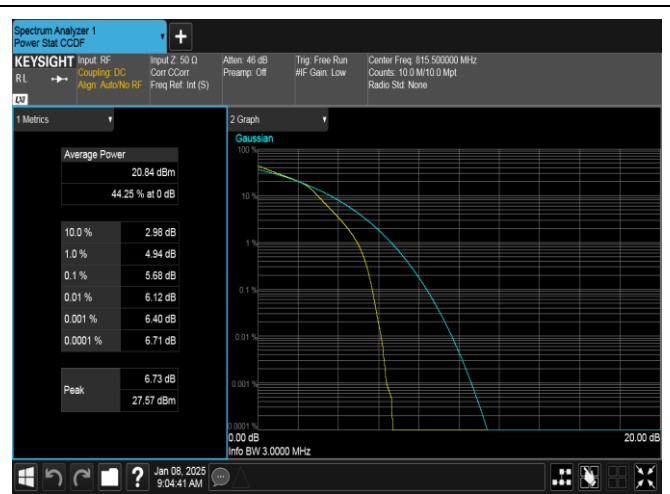
Band26(814-824)-3MHz-16QAM-26705-15RB#0-PASS
