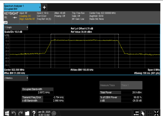
Band26(814-824)-3MHz-16QAM-26775-15RB#0-PASS
