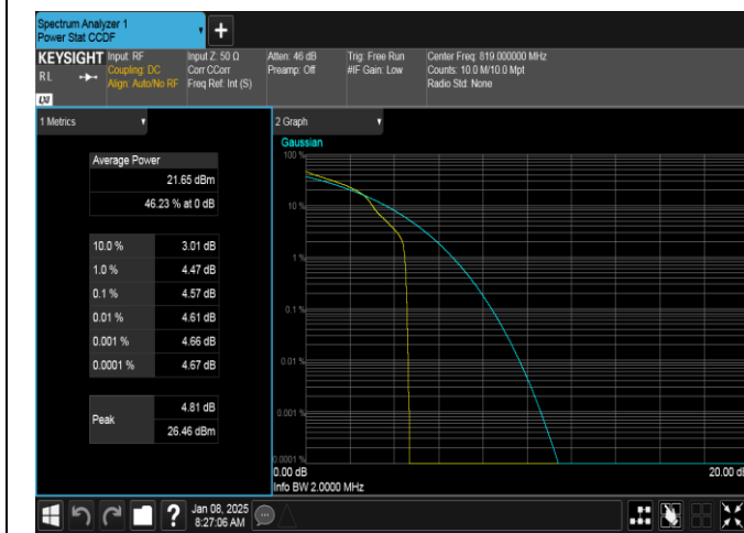
Band26(814-824)-1.4MHz-16QAM-26740-1RB#0-PASS
