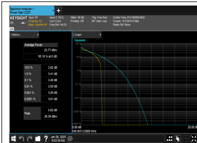
Band26(814-824)-3MHz-QPSK-26705-1RB#0-PASS
