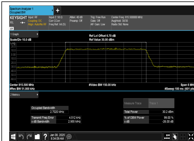
Band26(814-824)-3MHz-QPSK-26705-15RB#0-PASS
