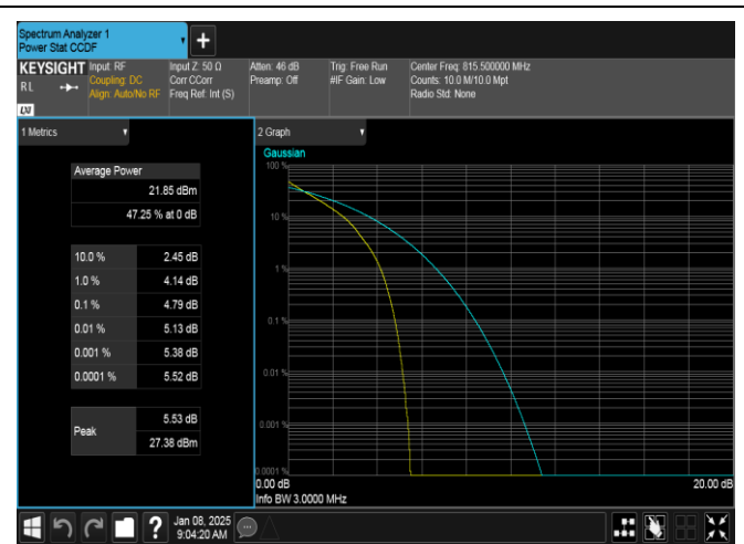
Band26(814-824)-3MHz-QPSK-26705-15RB#0-PASS
