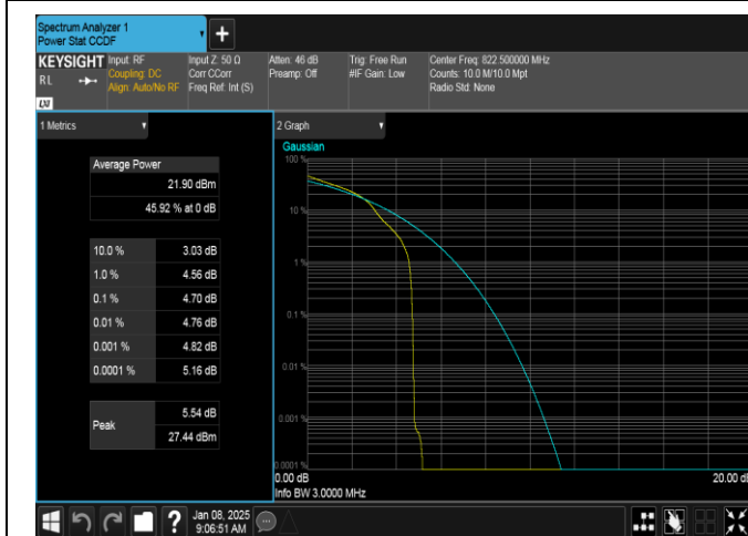
Band26(814-824)-3MHz-16QAM-26775-1RB#0-PASS
