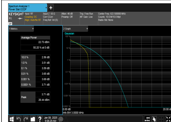
Band26(814-824)-3MHz-QPSK-26775-1RB#0-PASS
