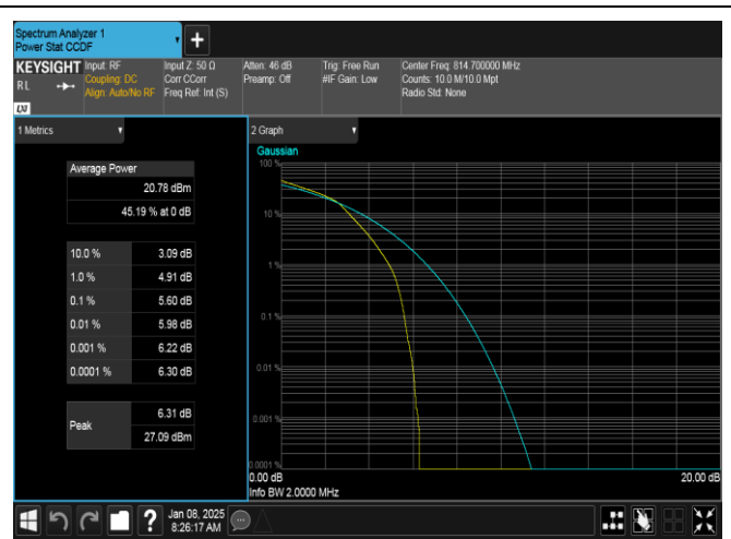
Band26(814-824)-1.4MHz-16QAM-26697-6RB#0-PASS
