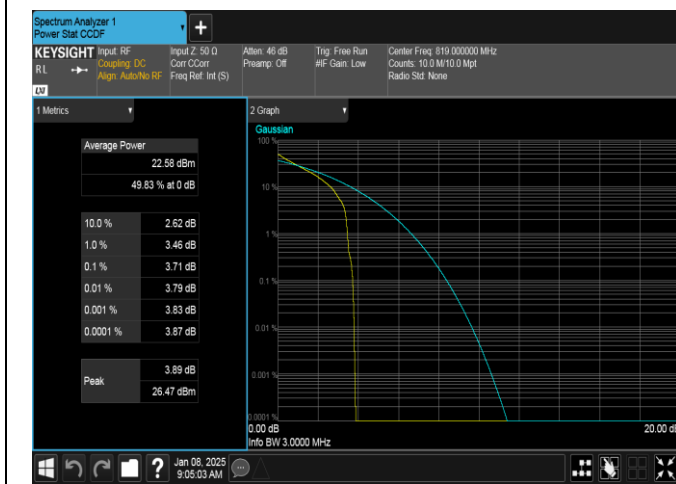
Band26(814-824)-3MHz-QPSK-26740-1RB#0-PASS
