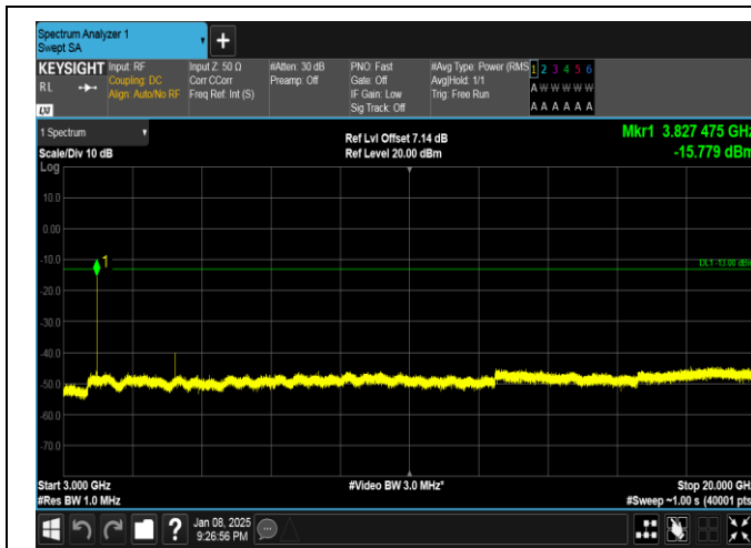
Band25-20MHz-16QAM-26590-1RB#99-3000~20000-PASS
