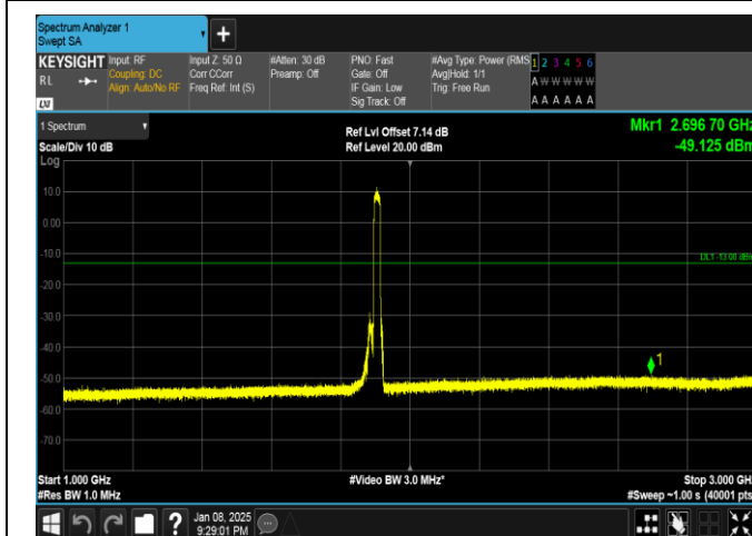
Band25-20MHz-16QAM-26590-100RB#0-1000~3000-PASS
