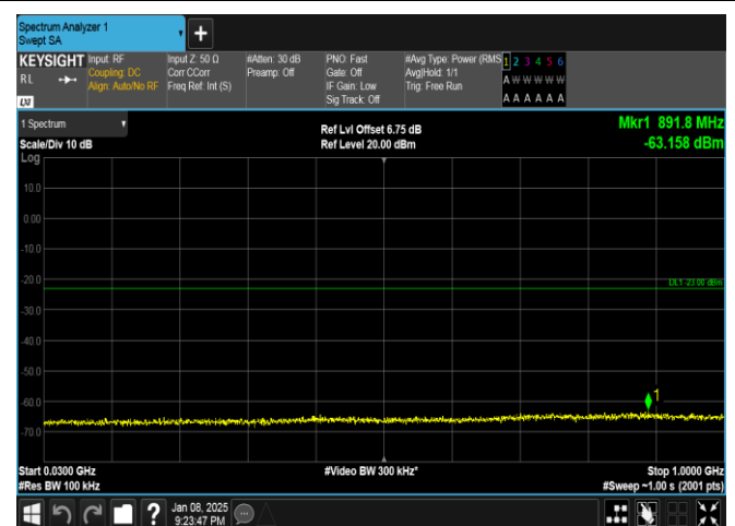
Band25-20MHz-16QAM-26590-1RB#0-30~1000-PASS
