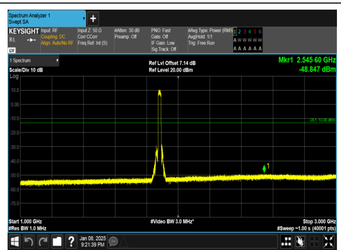
Band25-20MHz-16QAM-26365-100RB#0-1000~3000-PASS
