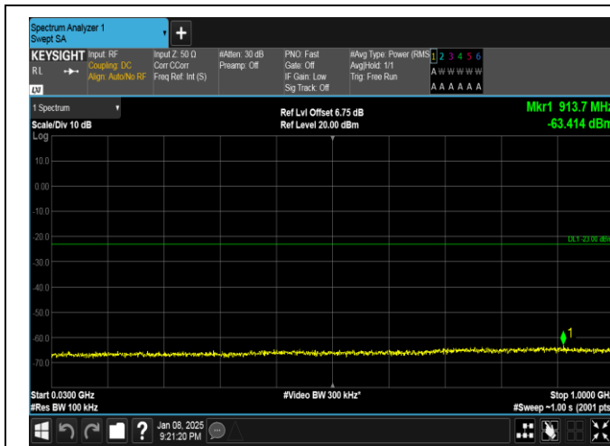
Band25-20MHz-16QAM-26365-100RB#0-30~1000-PASS
