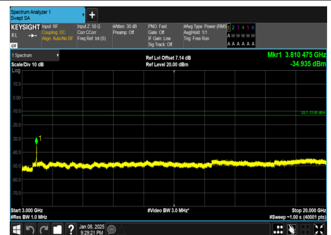
Band25-20MHz-16QAM-26590-100RB#0-3000~20000-PASS
