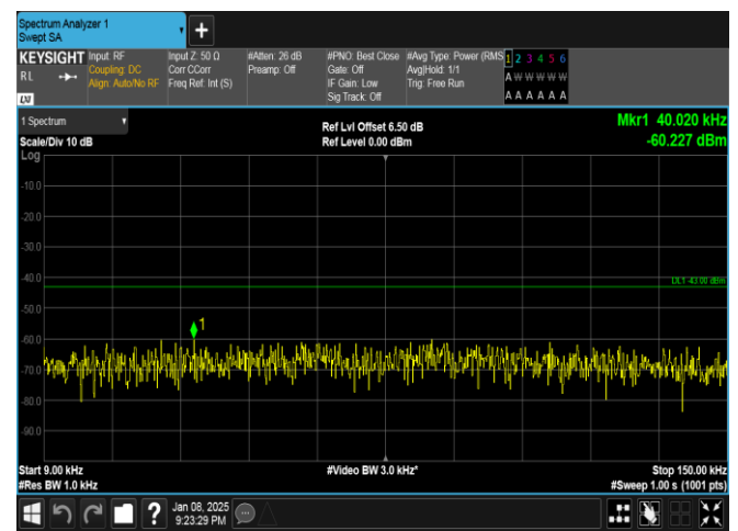
Band25-20MHz-16QAM-26590-1RB#0-0.009~0.15-PASS
