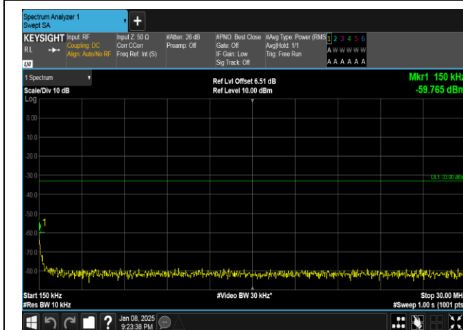
Band25-20MHz-16QAM-26590-1RB#0-0.15~30-PASS
