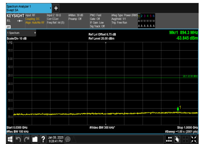
Band25-20MHz-16QAM-26590-100RB#0-30~1000-PASS
