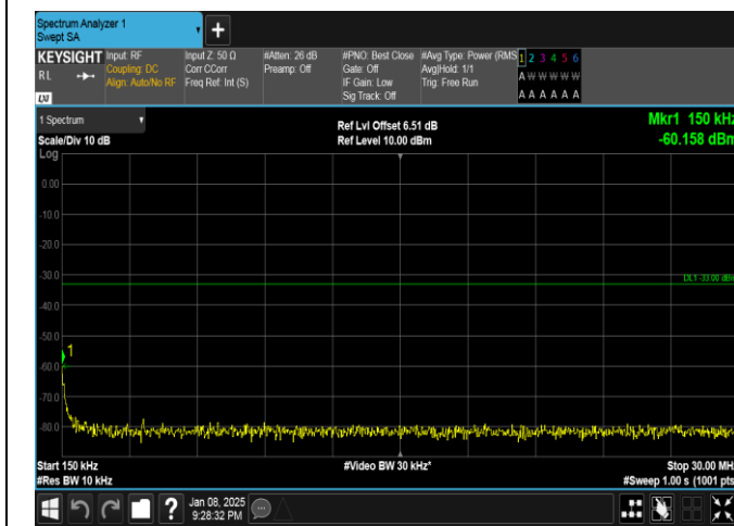
Band25-20MHz-16QAM-26590-100RB#0-0.15~30-PASS
