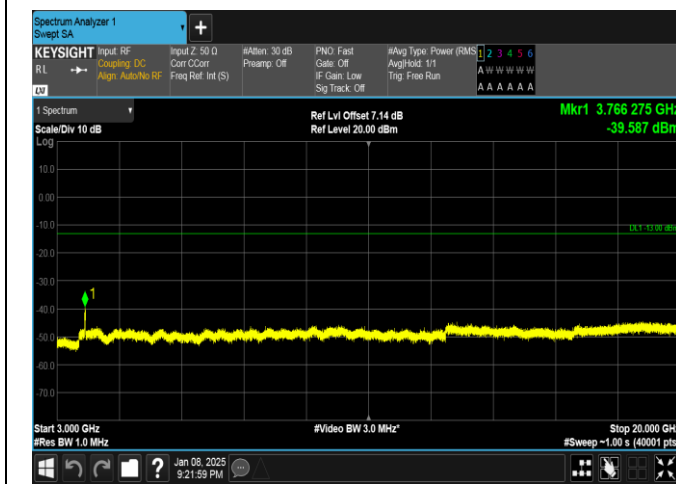
Band25-20MHz-16QAM-26365-100RB#0-3000~20000-PASS
