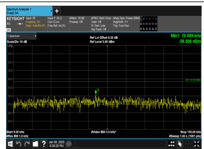
Band25-20MHz-16QAM-26590-100RB#0-0.009~0.15-PASS
