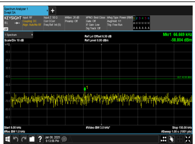
Band25-20MHz-16QAM-26140-100RB#0-0.009~0.15-PASS
