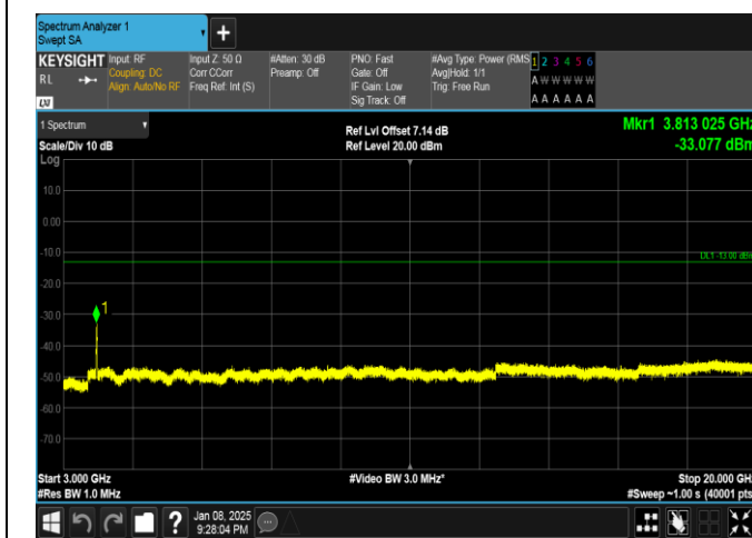
Band25-20MHz-QPSK-26590-100RB#0-3000~20000-PASS
