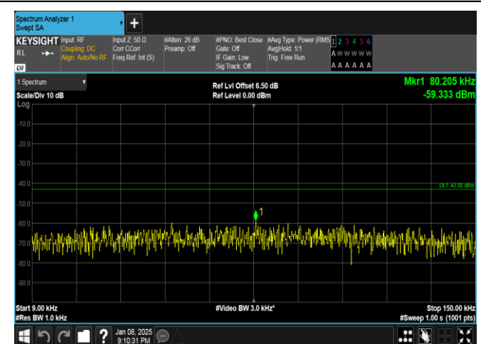
Band25-20MHz-QPSK-26140-1RB#99-0.009~0.15-PASS
