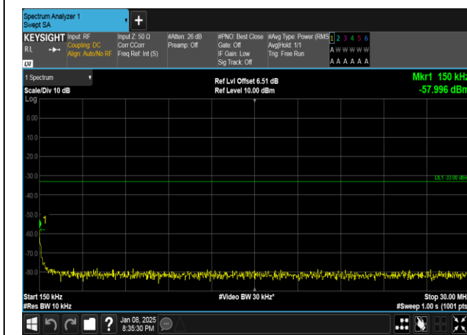
Band25-15MHz-16QAM-26615-75RB#0-0.15~30-PASS
