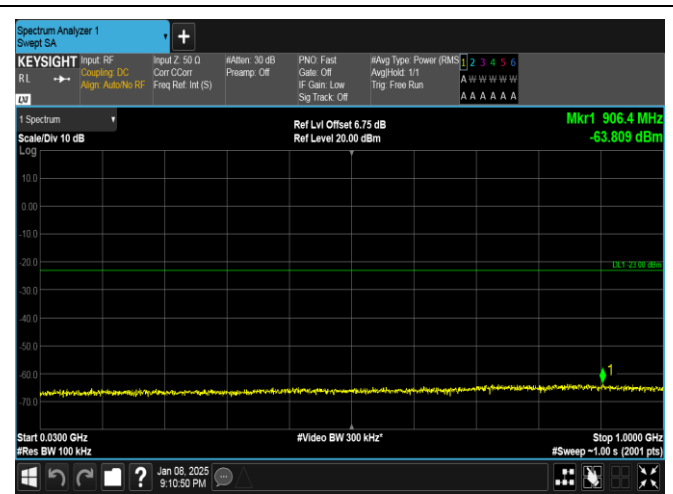
Band25-20MHz-QPSK-26140-1RB#99-30~1000-PASS
