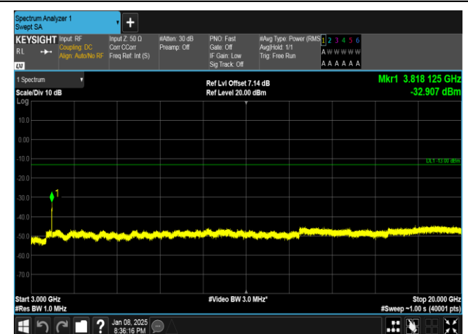
Band25-15MHz-16QAM-26615-75RB#0-3000~20000-PASS
