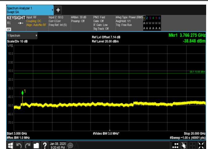
Band25-20MHz-QPSK-26365-100RB#0-3000~20000-PASS
