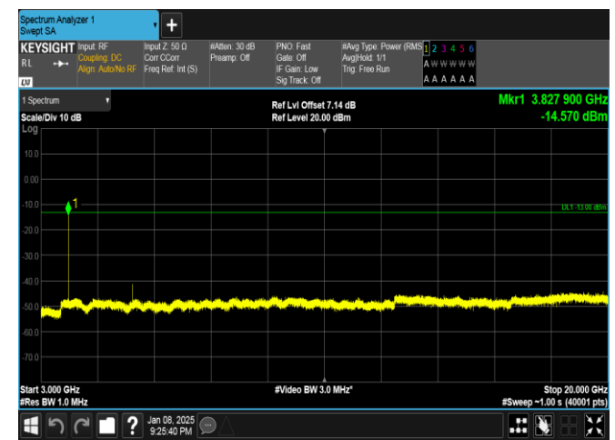
Band25-20MHz-QPSK-26590-1RB#99-3000~20000-PASS
