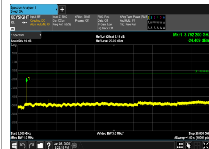
Band25-20MHz-QPSK-26590-1RB#0-3000~20000-PASS
