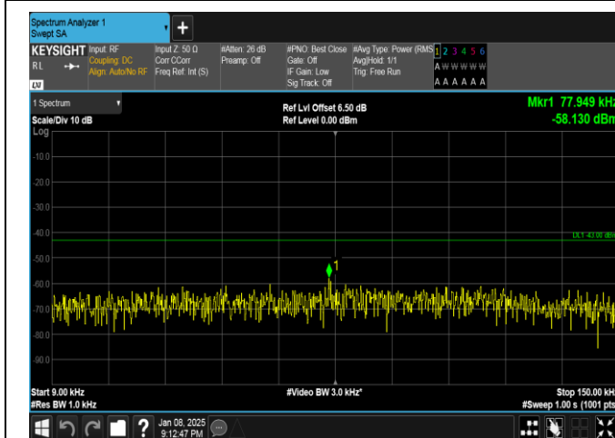
Band25-20MHz-QPSK-26140-100RB#0-0.009~0.15-PASS
