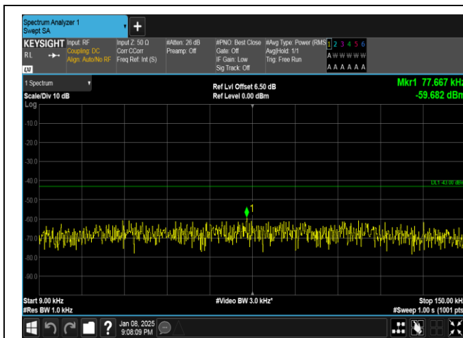
Band25-20MHz-QPSK-26140-1RB#0-0.009~0.15-PASS
