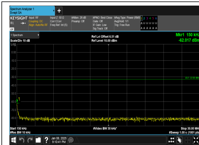
Band25-20MHz-QPSK-26140-1RB#99-0.15~30-PASS
