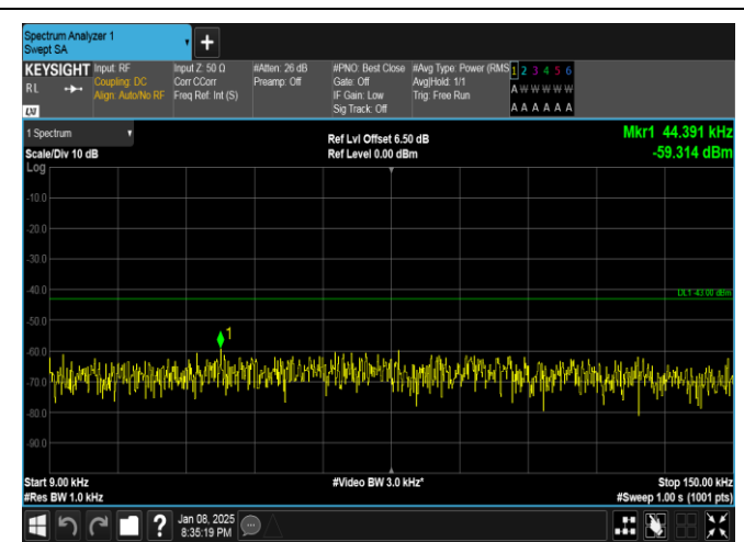
Band25-15MHz-16QAM-26615-75RB#0-0.009~0.15-PASS
