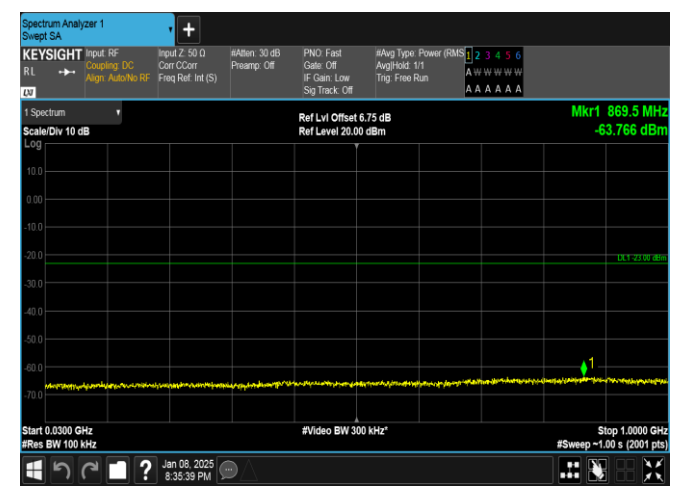
Band25-15MHz-16QAM-26615-75RB#0-30~1000-PASS
