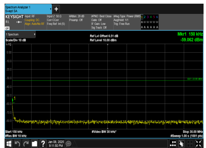
Band25-20MHz-16QAM-26140-1RB#99-0.15~30-PASS
