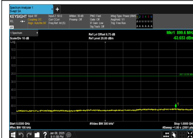
Band25-20MHz-16QAM-26140-1RB#99-30~1000-PASS
