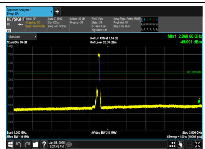
Band25-20MHz-QPSK-26590-100RB#0-1000~3000-PASS
