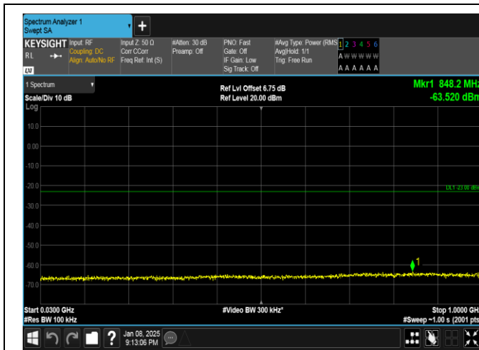
Band25-20MHz-QPSK-26140-100RB#0-30~1000-PASS
