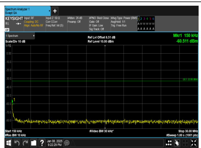
Band25-20MHz-QPSK-26590-1RB#0-0.15~30-PASS
