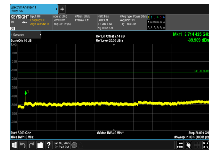
Band25-20MHz-QPSK-26140-100RB#0-3000~20000-PASS
