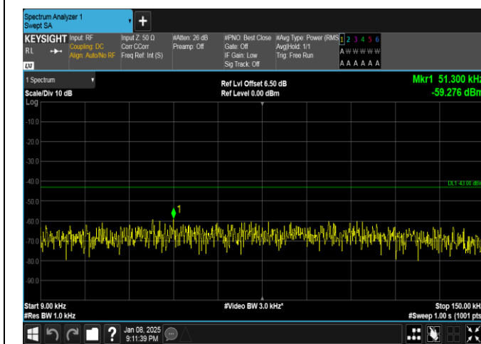
Band25-20MHz-16QAM-26140-1RB#99-0.009~0.15-PASS
