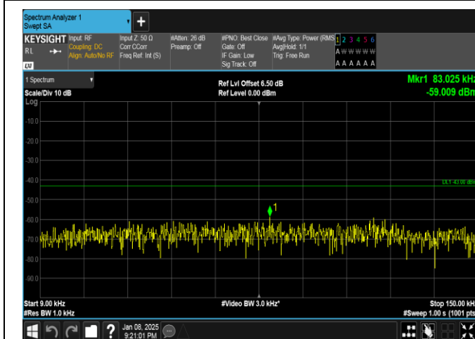
Band25-20MHz-16QAM-26365-100RB#0-0.009~0.15-PASS
