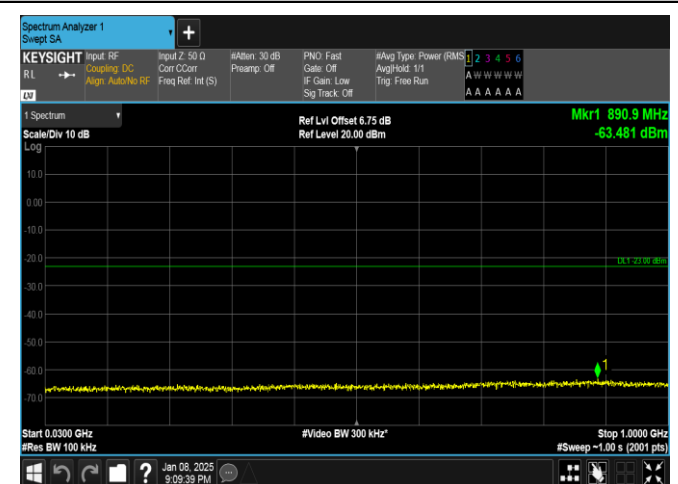
Band25-20MHz-16QAM-26140-1RB#0-30~1000-PASS
