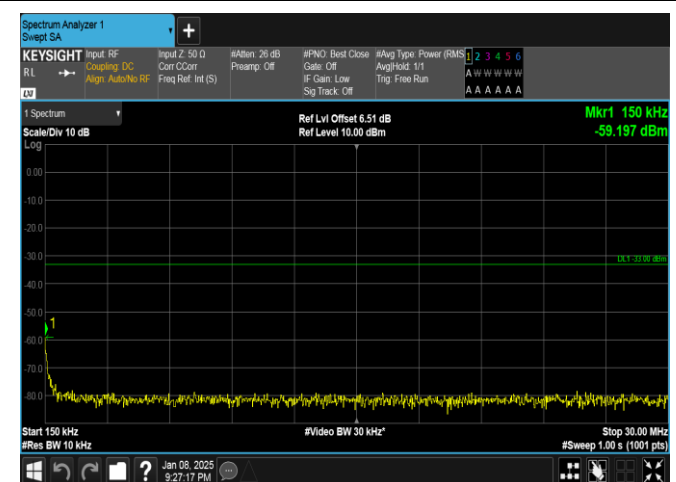
Band25-20MHz-QPSK-26590-100RB#0-0.15~30-PASS
