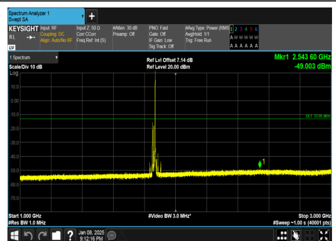
Band25-20MHz-16QAM-26140-1RB#99-1000~3000-PASS
