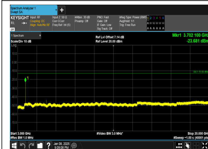
Band25-20MHz-QPSK-26140-1RB#0-3000~20000-PASS
