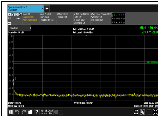
Band25-20MHz-16QAM-26365-1RB#99-0.15~30-PASS
