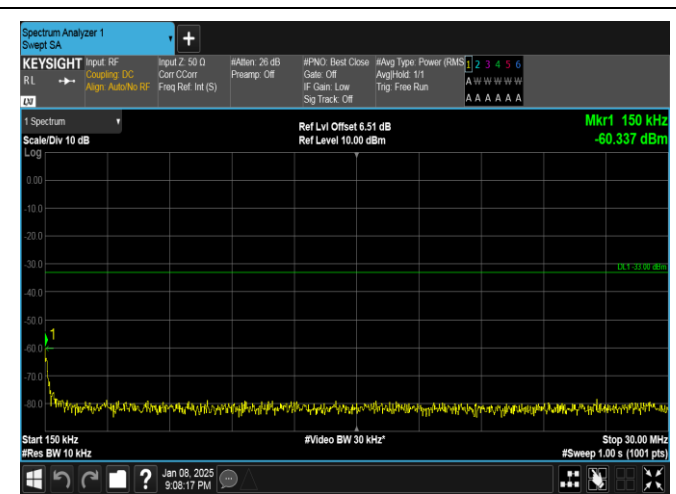
Band25-20MHz-QPSK-26140-1RB#0-0.15~30-PASS
