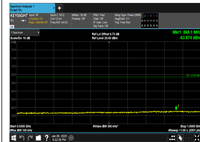
Band25-20MHz-QPSK-26590-1RB#0-30~1000-PASS
