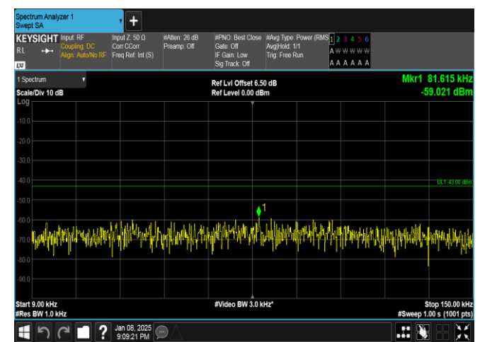
Band25-20MHz-16QAM-26140-1RB#0-0.009~0.15-PASS
