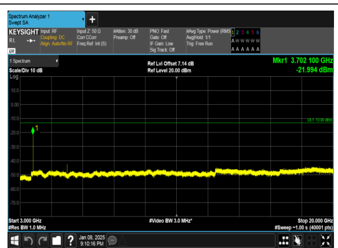
Band25-20MHz-16QAM-26140-1RB#0-3000~20000-PASS
