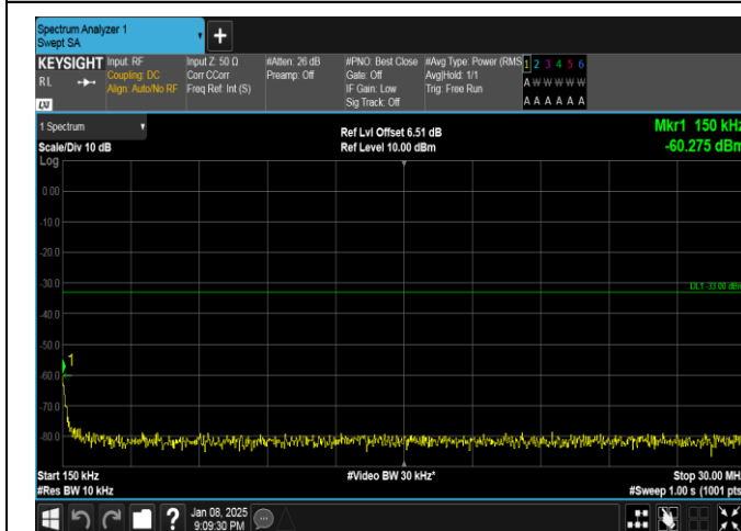
Band25-20MHz-16QAM-26140-1RB#0-0.15~30-PASS
