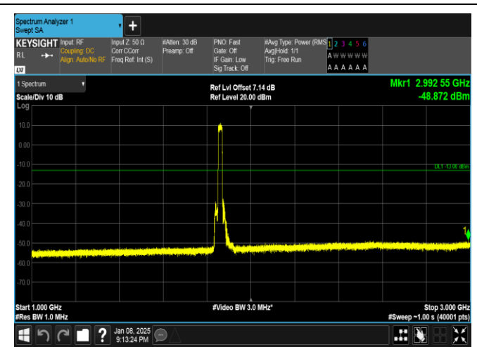
Band25-20MHz-QPSK-26140-100RB#0-1000~3000-PASS
