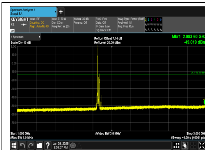
Band25-20MHz-16QAM-26140-1RB#0-1000~3000-PASS
