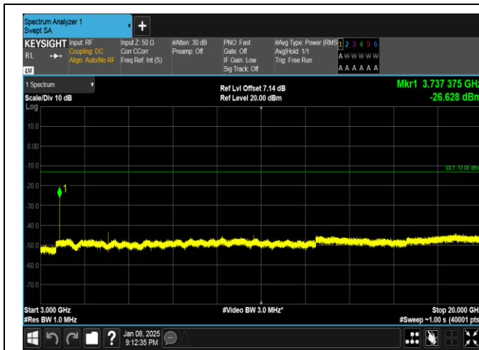
Band25-20MHz-16QAM-26140-1RB#99-3000~20000-PASS
