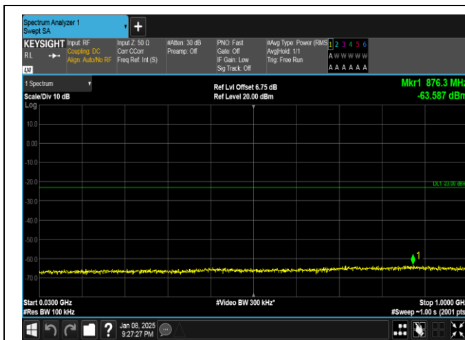
Band25-20MHz-QPSK-26590-100RB#0-30~1000-PASS
