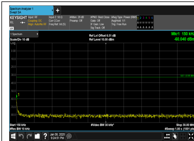
Band25-20MHz-QPSK-26590-1RB#99-0.15~30-PASS
