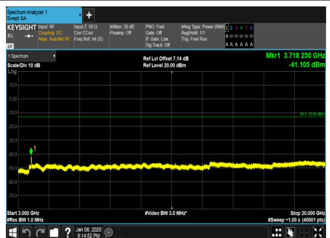
Band25-20MHz-16QAM-26140-100RB#0-3000~20000-PASS
