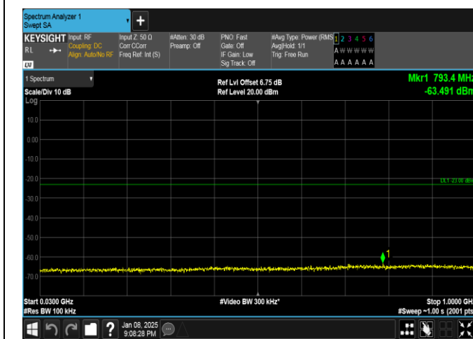
Band25-20MHz-QPSK-26140-1RB#0-30~1000-PASS
