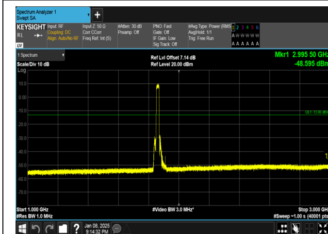
Band25-20MHz-16QAM-26140-100RB#0-1000~3000-PASS
