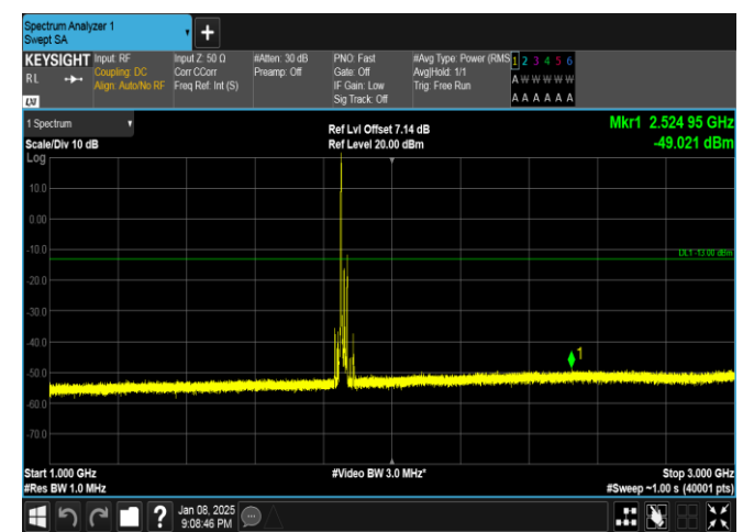
Band25-20MHz-QPSK-26140-1RB#0-1000~3000-PASS
