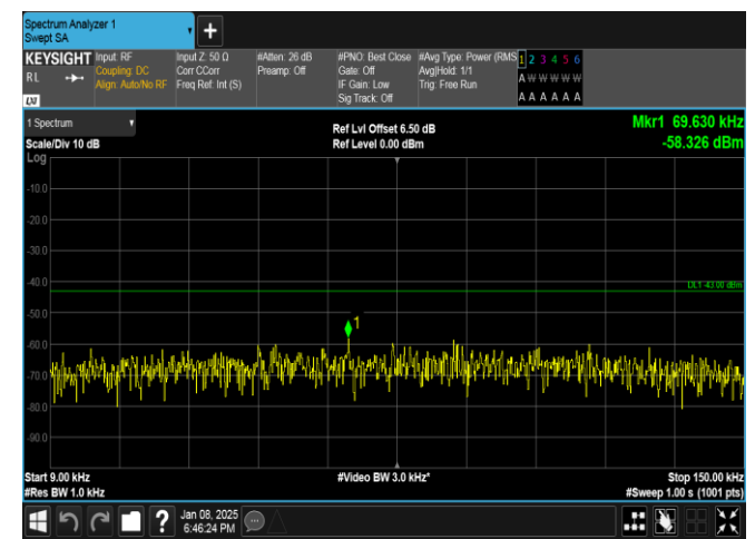
Band25-5MHz-16QAM-26665-1RB#0-0.009~0.15-PASS
