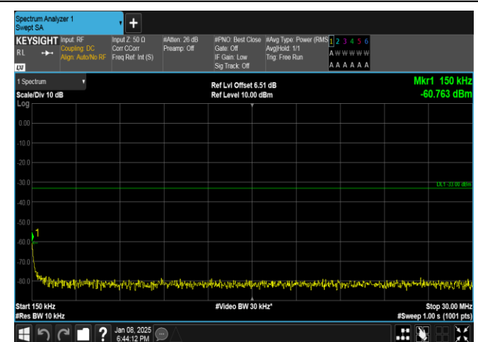
Band25-5MHz-16QAM-26365-25RB#0-0.15~30-PASS
