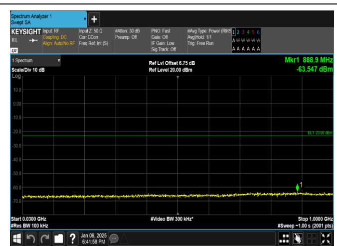
Band25-5MHz-16QAM-26365-1RB#24-30~1000-PASS
