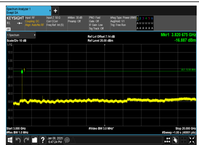
Band25-5MHz-16QAM-26665-1RB#0-3000~20000-PASS
