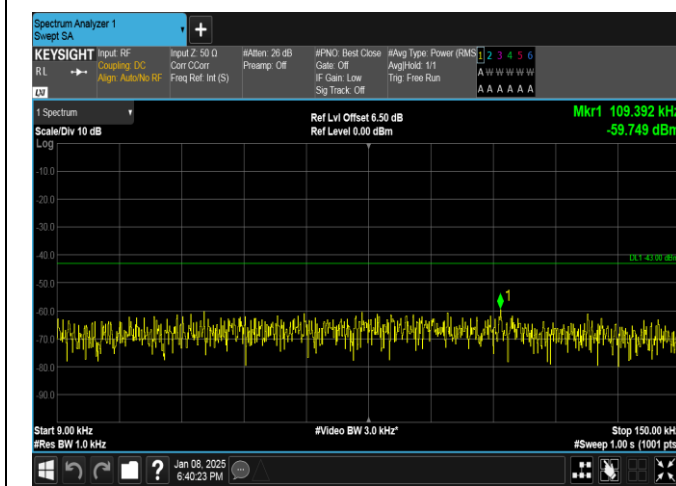
Band25-5MHz-QPSK-26365-1RB#24-0.009~0.15-PASS
