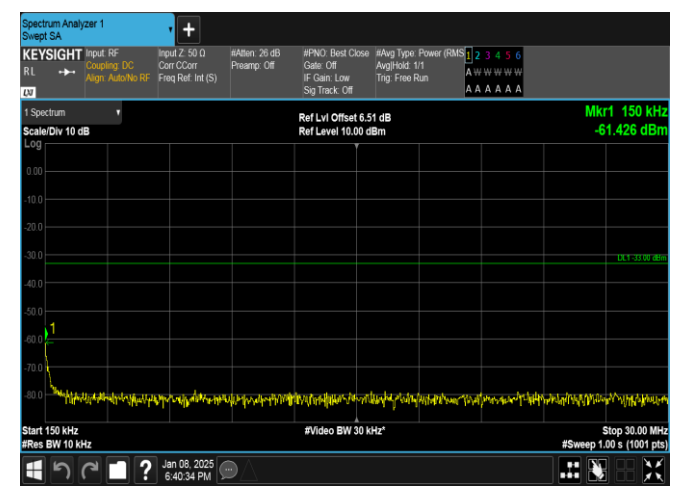
Band25-5MHz-QPSK-26365-1RB#24-0.15~30-PASS
