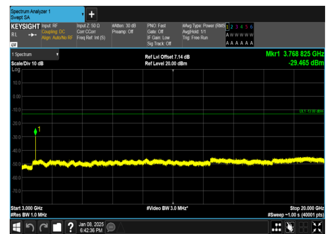
Band25-5MHz-16QAM-26365-1RB#24-3000~20000-PASS
