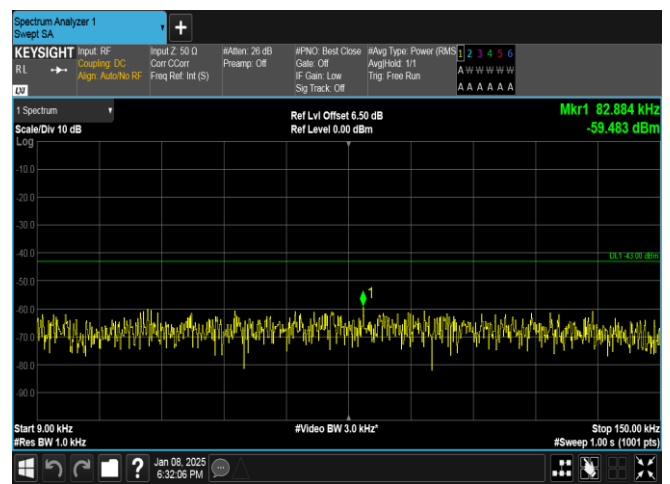
Band25-5MHz-16QAM-26065-1RB#0-0.009~0.15-PASS
