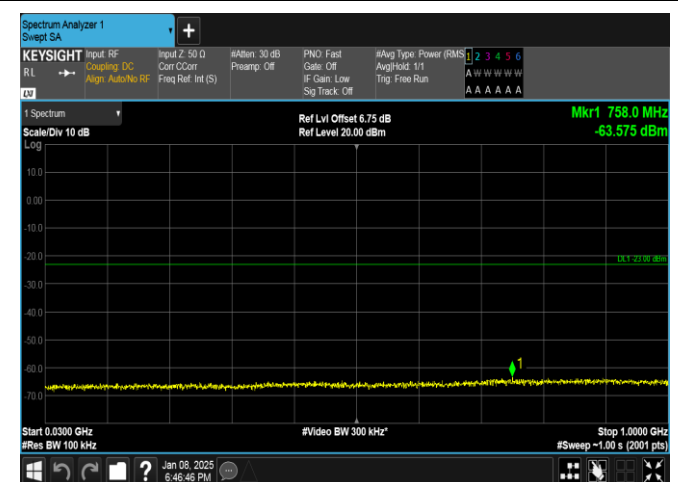
Band25-5MHz-16QAM-26665-1RB#0-30~1000-PASS
