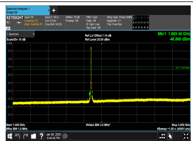
Band25-5MHz-16QAM-26365-25RB#0-1000~3000-PASS
