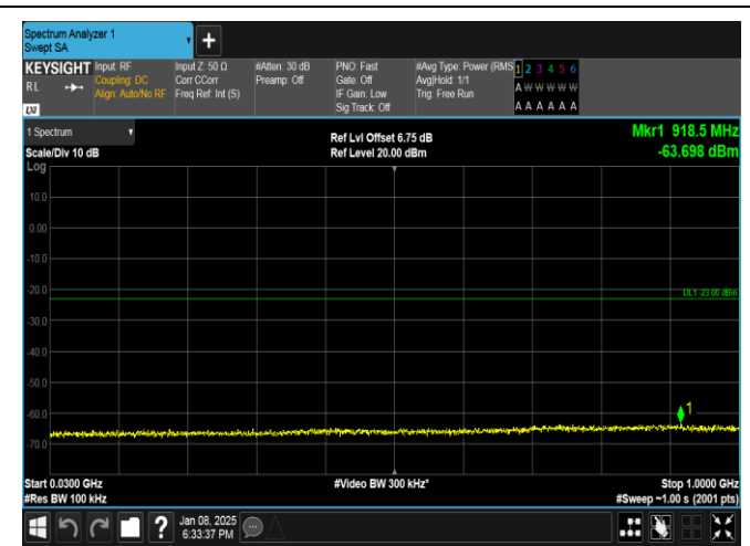
Band25-5MHz-QPSK-26065-1RB#24-30~1000-PASS
