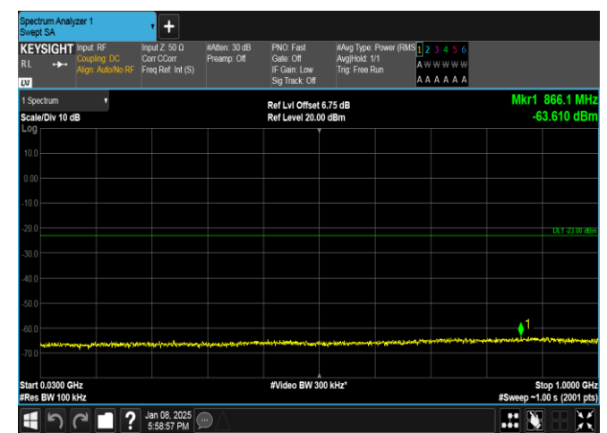
Band25-3MHz-16QAM-26675-15RB#0-30~1000-PASS
