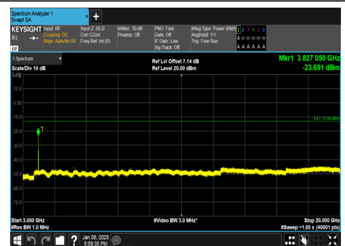
Band25-3MHz-16QAM-26675-15RB#0-3000~20000-PASS
