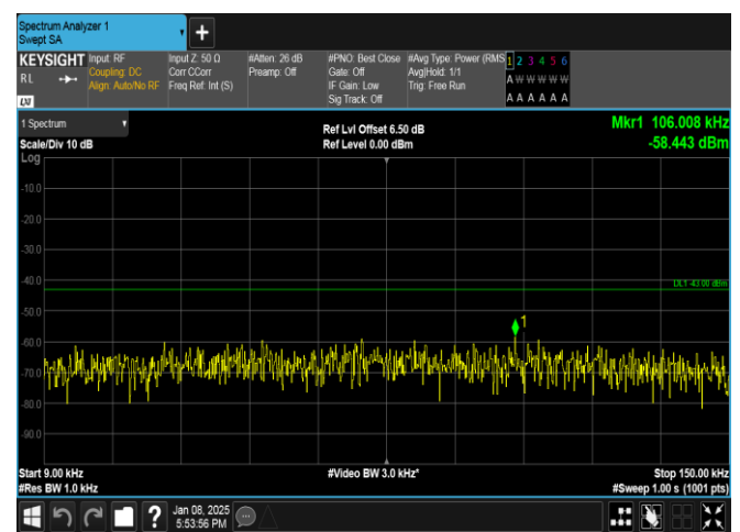
Band25-3MHz-16QAM-26675-1RB#0-0.009~0.15-PASS
