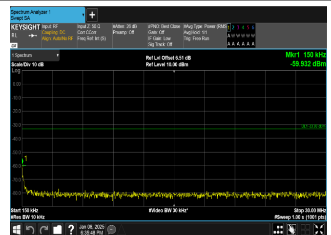
Band25-5MHz-QPSK-26065-25RB#0-0.15~30-PASS
