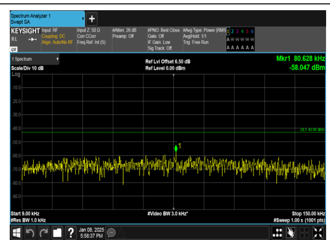
Band25-3MHz-16QAM-26675-15RB#0-0.009~0.15-PASS
