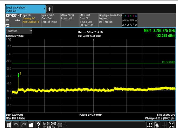
Band25-3MHz-16QAM-26055-15RB#0-3000~20000-PASS
