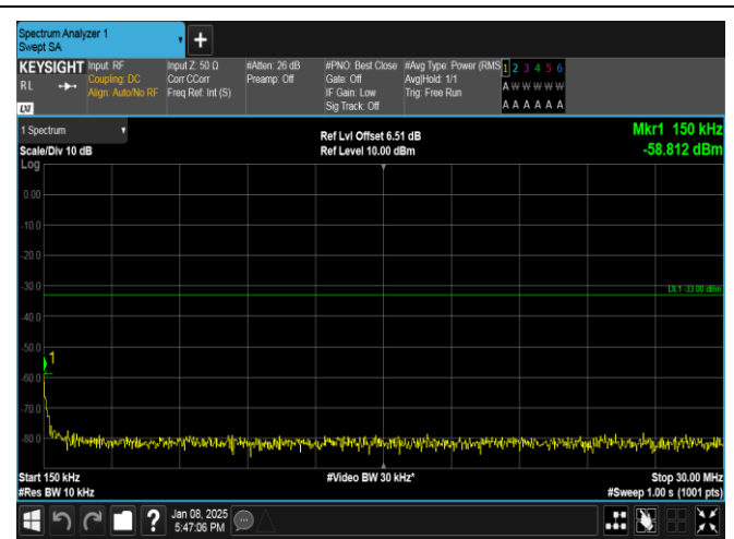
Band25-3MHz-16QAM-26365-1RB#0-0.15~30-PASS
