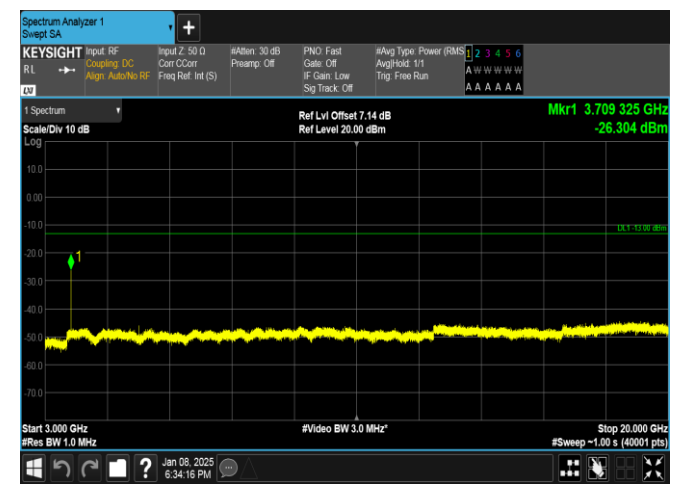
Band25-5MHz-QPSK-26065-1RB#24-3000~20000-PASS
