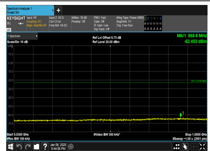
Band25-3MHz-16QAM-26055-15RB#0-30~1000-PASS
