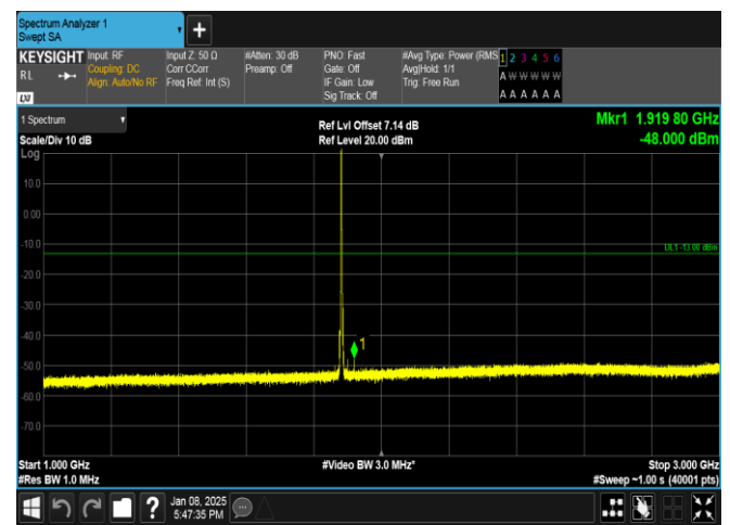
Band25-3MHz-16QAM-26365-1RB#0-1000~3000-PASS
