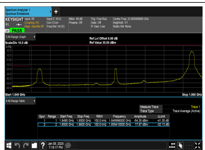
Band25-10MHz-QPSK-26090-1RB#49-PASS
