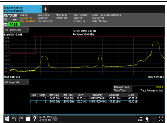
Band25-5MHz-QPSK-26065-1RB#24-PASS
