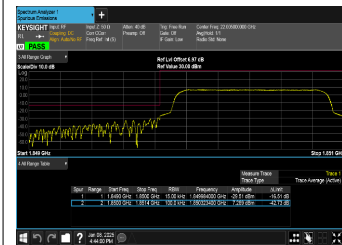
Band25-1.4MHz-16QAM-26047-6RB#0-PASS
