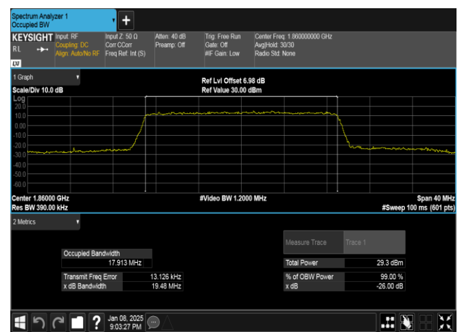
Band25-20MHz-16QAM-26140-100RB#0-PASS
