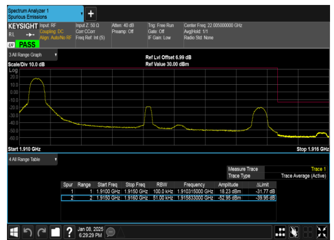
Band25-5MHz-QPSK-26665-1RB#0-PASS
