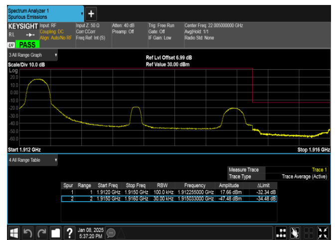
Band25-3MHz-16QAM-26675-1RB#0-PASS
