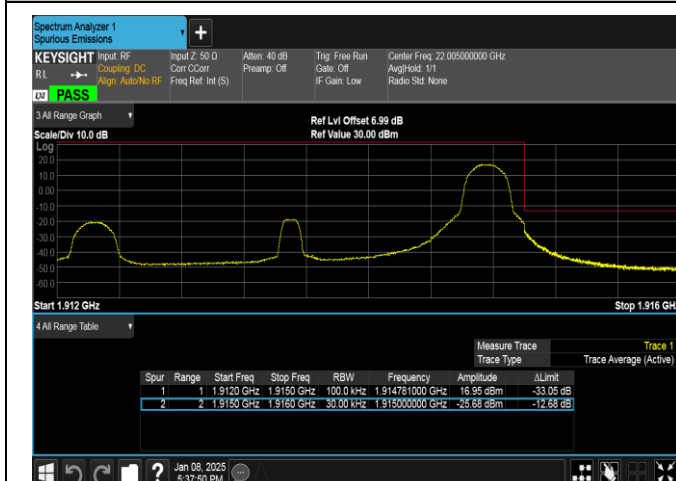
Band25-3MHz-16QAM-26675-1RB#14-PASS
