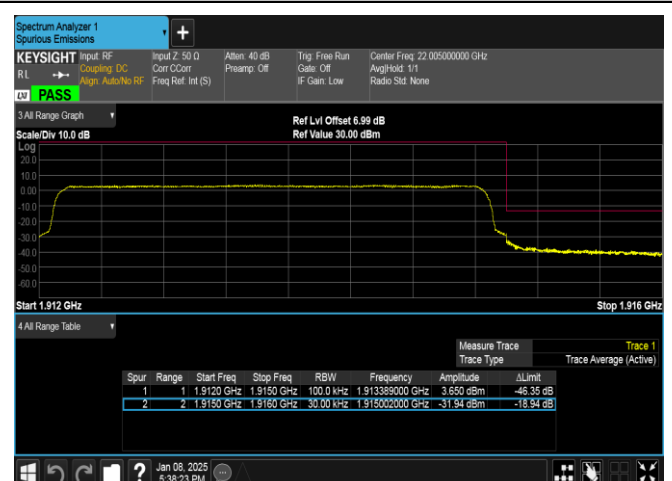
Band25-3MHz-16QAM-26675-15RB#0-PASS
