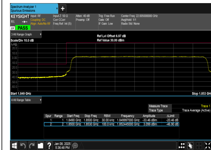
Band25-3MHz-16QAM-26055-15RB#0-PASS
