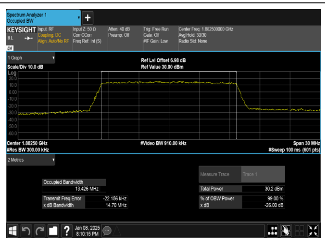
Band25-15MHz-QPSK-26365-75RB#0-PASS
