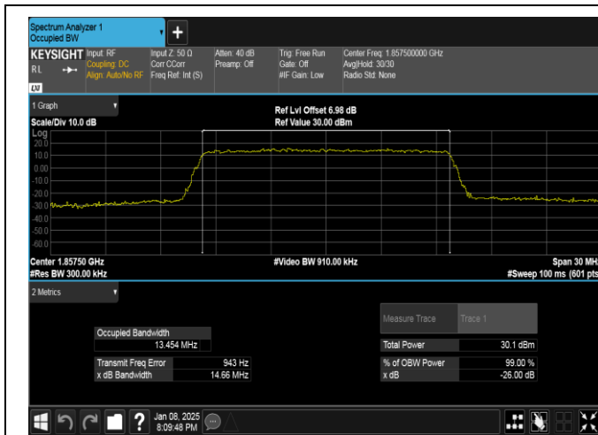
Band25-15MHz-QPSK-26115-75RB#0-PASS
