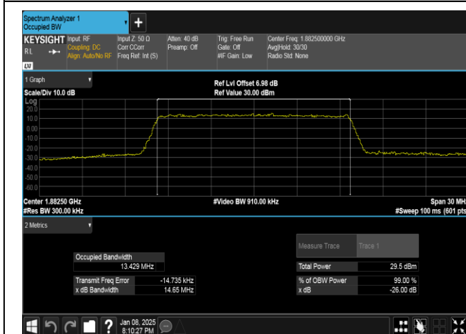
Band25-15MHz-16QAM-26365-75RB#0-PASS
