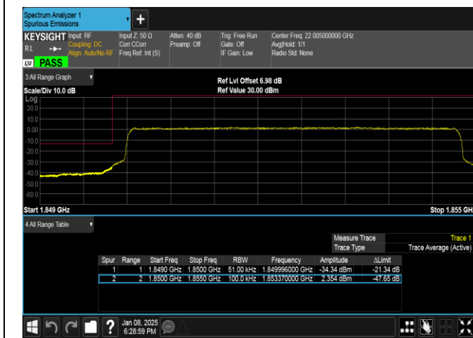
Band25-5MHz-QPSK-26065-25RB#0-PASS
