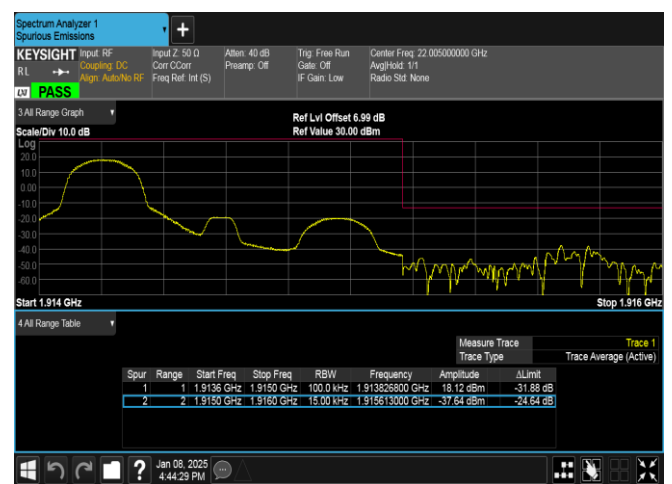
Band25-1.4MHz-16QAM-26683-1RB#0-PASS
