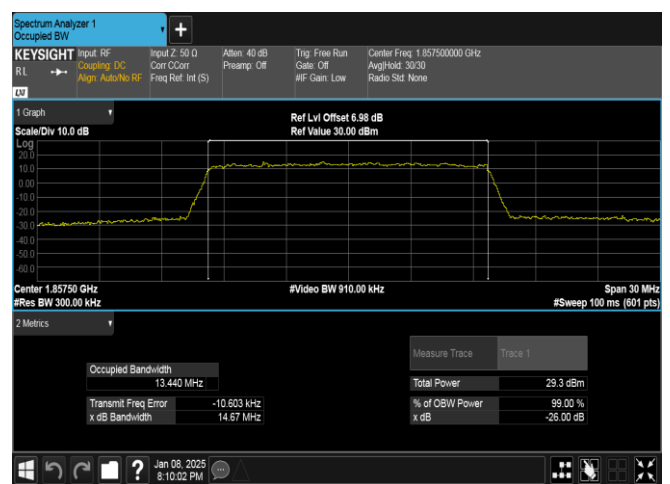
Band25-15MHz-16QAM-26115-75RB#0-PASS
