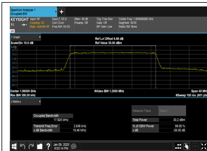
Band25-20MHz-QPSK-26140-100RB#0-PASS
