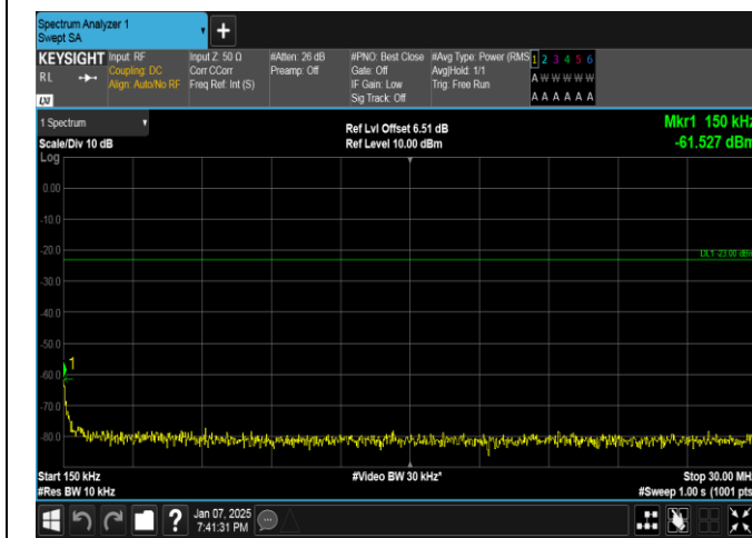
Band17-10MHz-16QAM-23800-50RB#0-0.15~30-PASS
