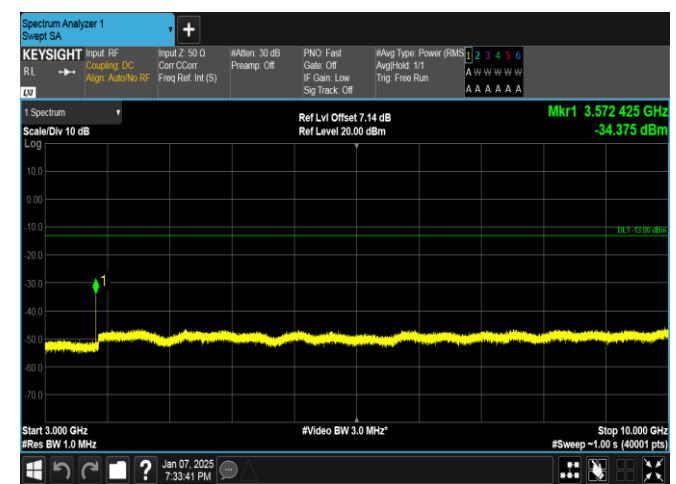
Band17-10MHz-16QAM-23790-1RB#49-3000~10000-PASS
