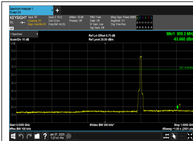
Band17-10MHz-QPSK-23780-50RB#0-30~1000-PASS
