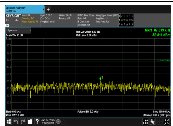
Band17-10MHz-16QAM-23780-50RB#0-0.009~0.15-PASS
