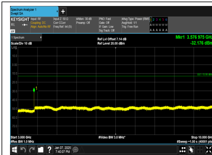
Band17-10MHz-16QAM-23800-1RB#49-3000~10000-PASS
