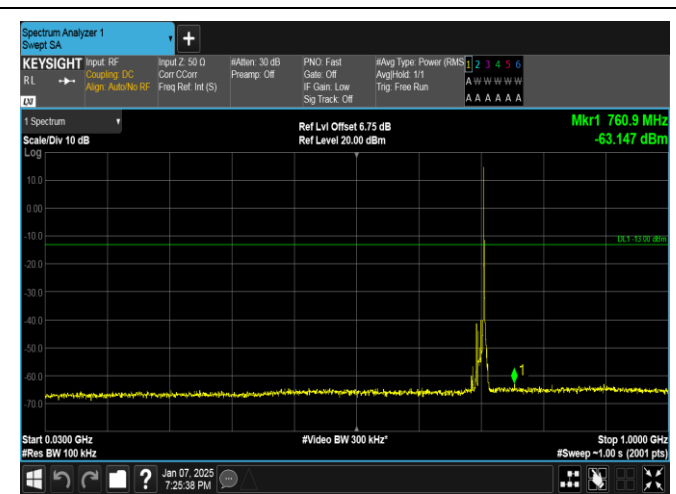
Band17-10MHz-QPSK-23780-1RB#49-30~1000-PASS
