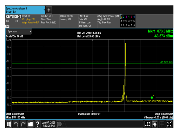
Band17-10MHz-16QAM-23790-1RB#49-30~1000-PASS
