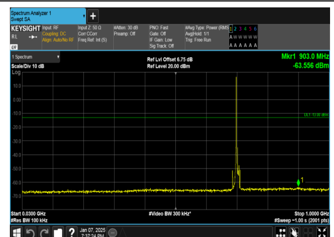
Band17-10MHz-16QAM-23800-1RB#0-30~1000-PASS
