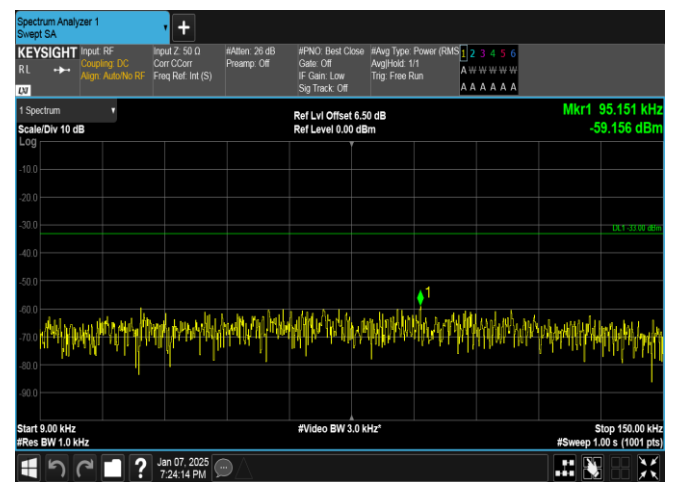
Band17-10MHz-16QAM-23780-1RB#0-0.009~0.15-PASS
