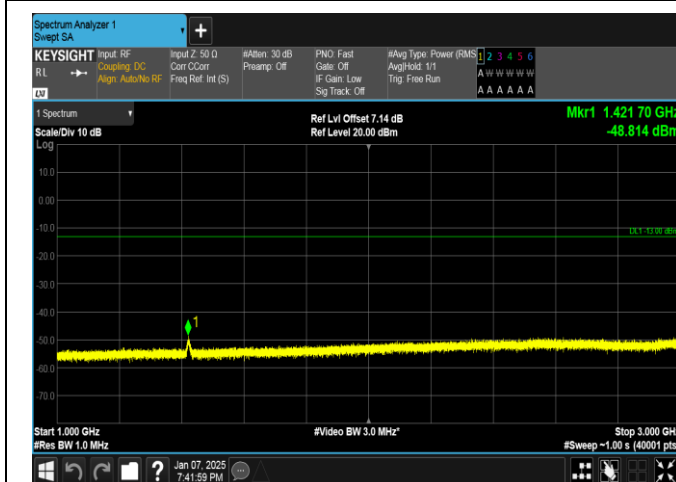
Band17-10MHz-16QAM-23800-50RB#0-1000~3000-PASS
