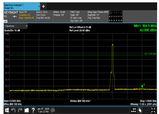
Band17-10MHz-QPSK-23790-50RB#0-30~1000-PASS
