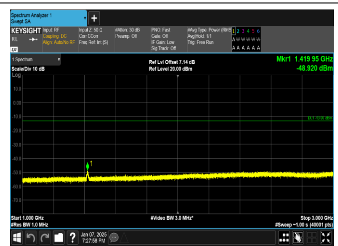
Band17-10MHz-QPSK-23780-50RB#0-1000~3000-PASS
