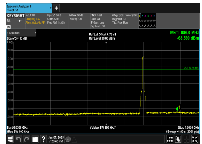
Band17-10MHz-16QAM-23780-50RB#0-30~1000-PASS
