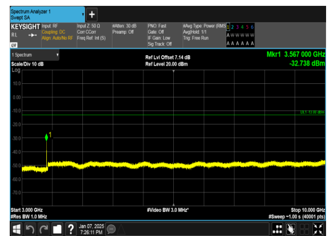
Band17-10MHz-QPSK-23780-1RB#49-3000~10000-PASS
