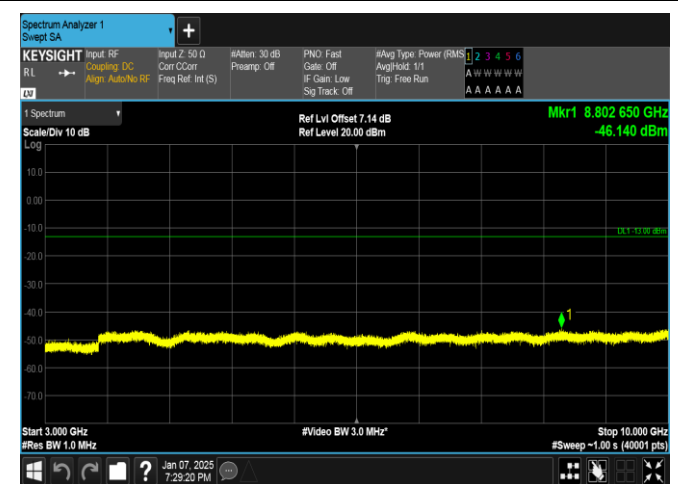
Band17-10MHz-16QAM-23780-50RB#0-3000~10000-PASS
