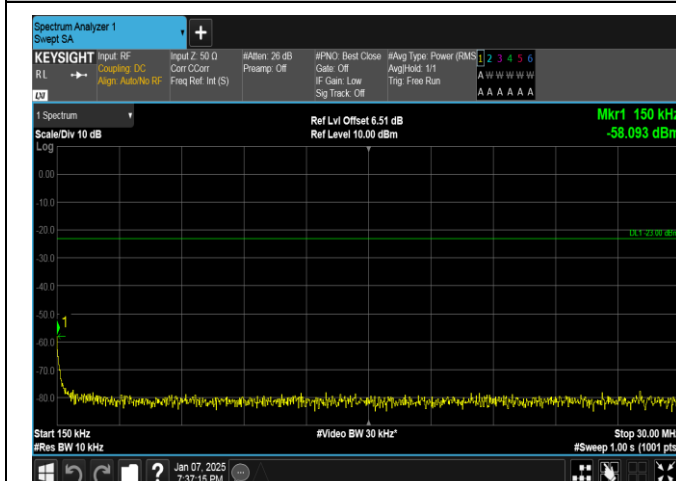
Band17-10MHz-16QAM-23800-1RB#0-0.15~30-PASS
