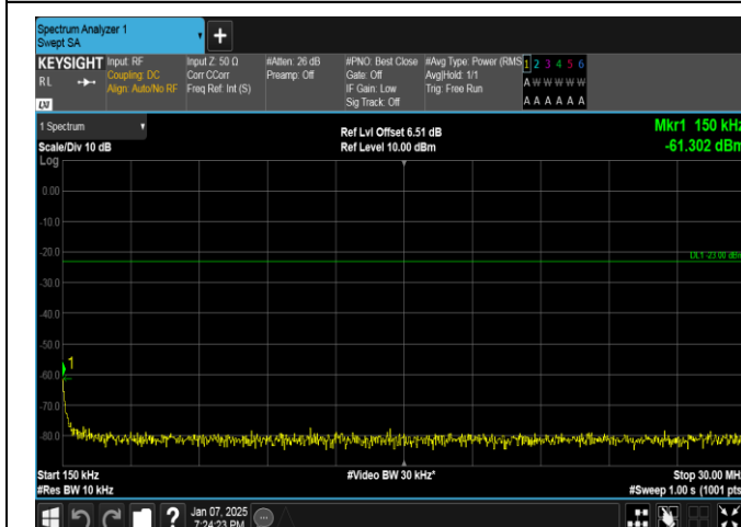
Band17-10MHz-16QAM-23780-1RB#0-0.15~30-PASS
