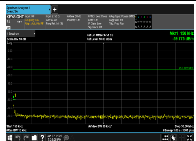
Band17-10MHz-16QAM-23790-50RB#0-0.15~30-PASS
