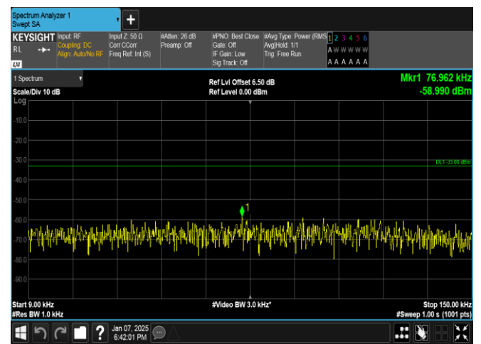
Band17-5MHz-QPSK-23790-1RB#0-0.009~0.15-PASS
