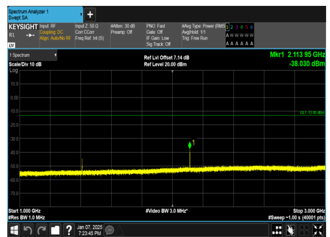
Band17-10MHz-QPSK-23780-1RB#0-1000~3000-PASS
