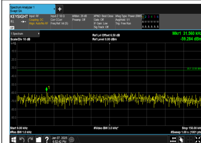
Band17-5MHz-QPSK-23825-25RB#0-0.009~0.15-PASS
