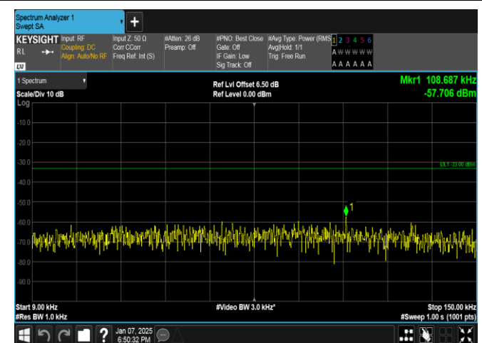
Band17-5MHz-QPSK-23825-1RB#24-0.009~0.15-PASS
