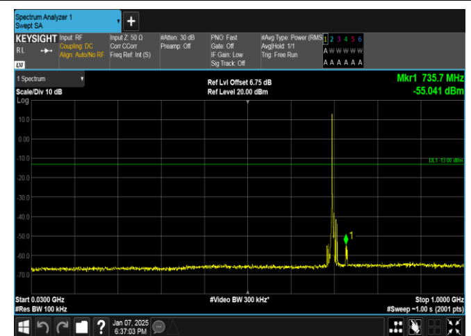
Band17-5MHz-16QAM-23755-1RB#0-30~1000-PASS
