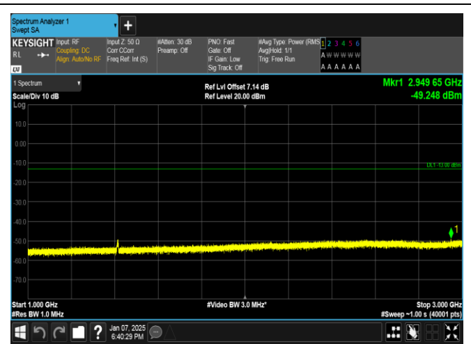
Band17-5MHz-QPSK-23755-25RB#0-1000~3000-PASS
