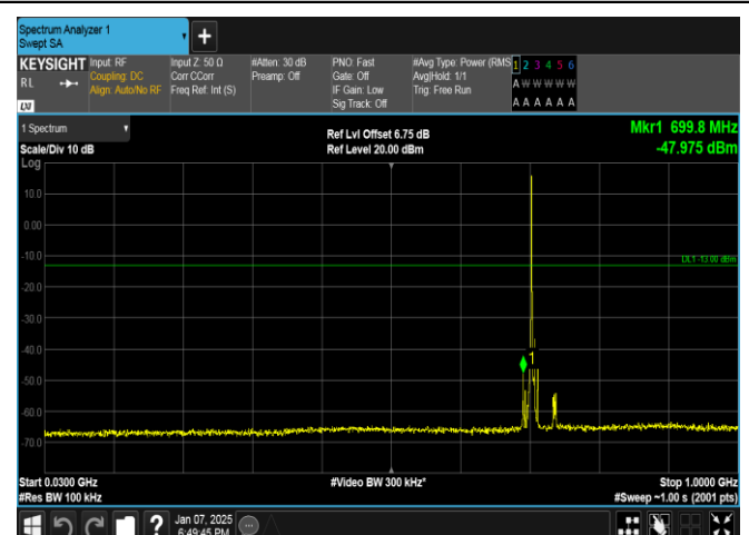
Band17-5MHz-16QAM-23825-1RB#0-30~1000-PASS
