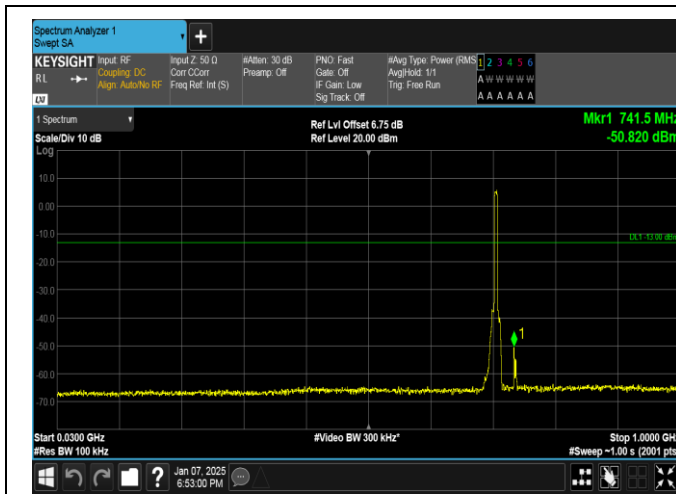
Band17-5MHz-QPSK-23825-25RB#0-30~1000-PASS
