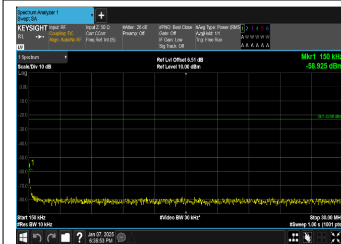
Band17-5MHz-16QAM-23755-1RB#0-0.15~30-PASS
