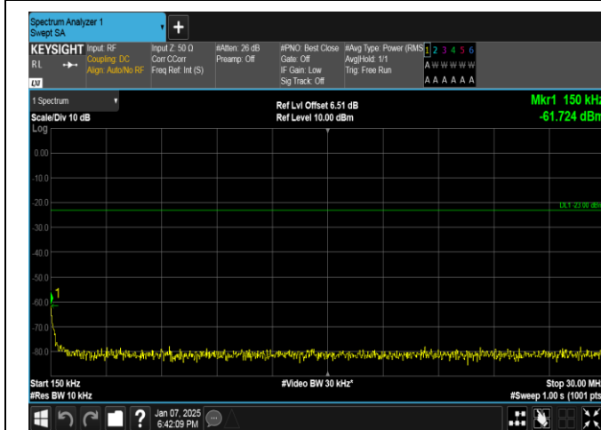
Band17-5MHz-QPSK-23790-1RB#0-0.15~30-PASS
