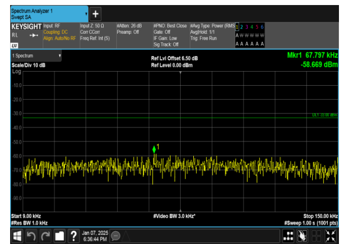
Band17-5MHz-16QAM-23755-1RB#0-0.009~0.15-PASS
