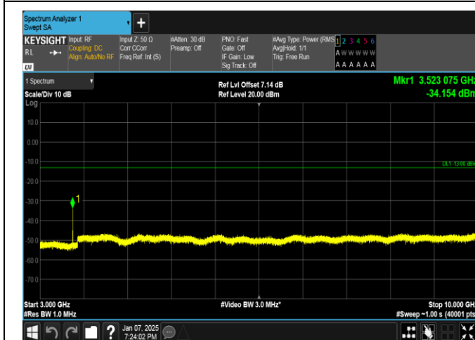
Band17-10MHz-QPSK-23780-1RB#0-3000~10000-PASS
