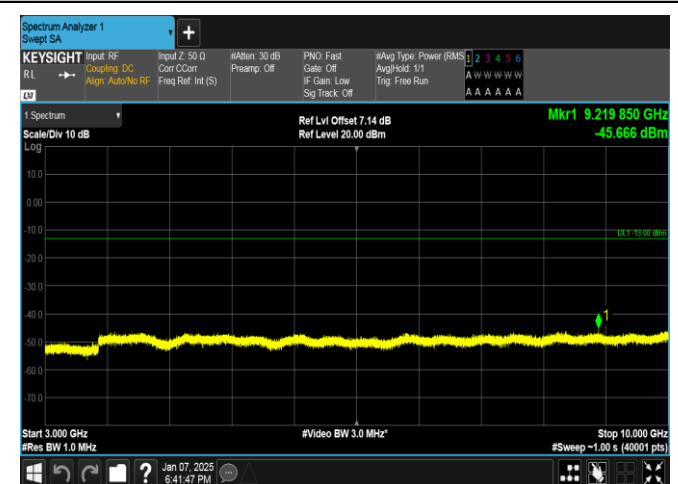
Band17-5MHz-16QAM-23755-25RB#0-3000~10000-PASS
