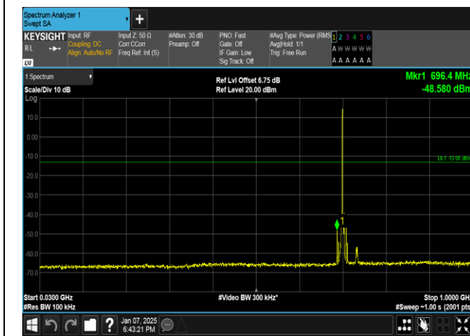
Band17-5MHz-16QAM-23790-1RB#0-30~1000-PASS
