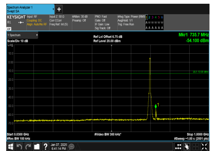
Band17-5MHz-16QAM-23755-25RB#0-30~1000-PASS
