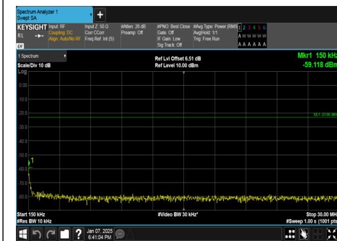
Band17-5MHz-16QAM-23755-25RB#0-0.15~30-PASS
