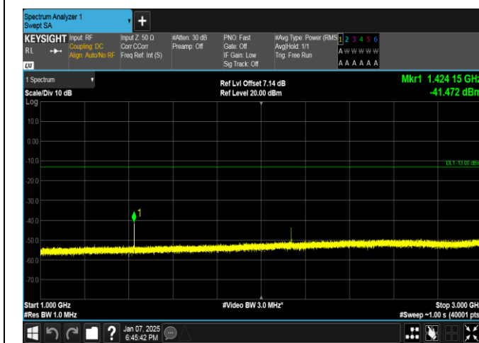
Band17-5MHz-16QAM-23790-1RB#24-1000~3000-PASS
