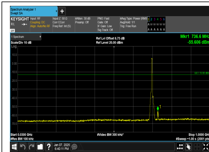
Band17-5MHz-QPSK-23755-25RB#0-30~1000-PASS
