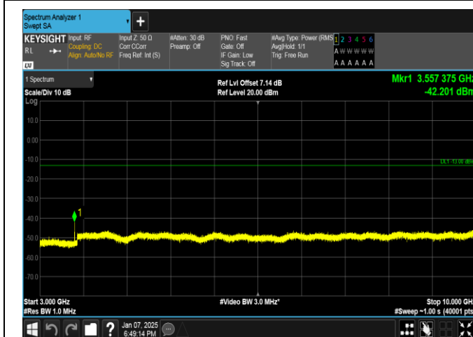
Band17-5MHz-QPSK-23825-1RB#0-3000~10000-PASS
