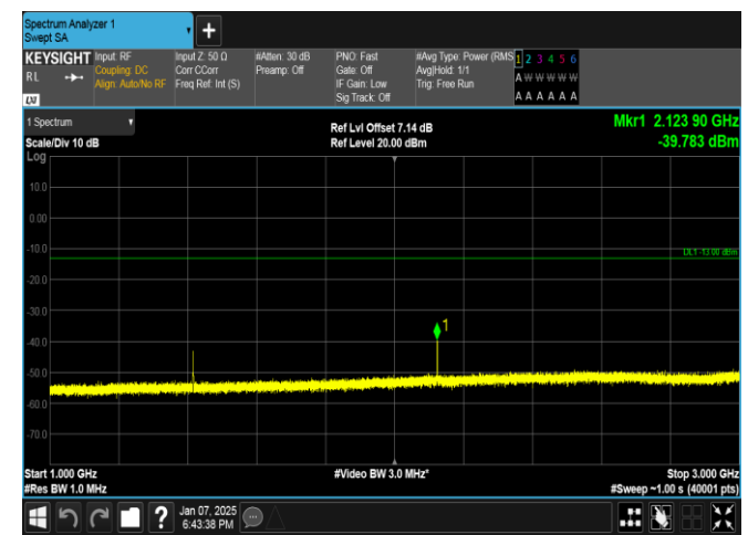
Band17-5MHz-16QAM-23790-1RB#0-1000~3000-PASS
