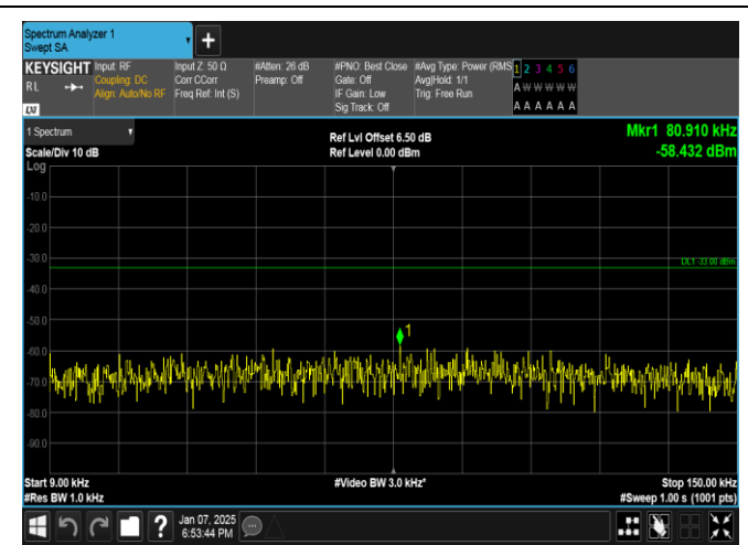
Band17-5MHz-16QAM-23825-25RB#0-0.009~0.15-PASS
