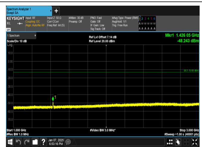
Band17-5MHz-QPSK-23825-25RB#0-1000~3000-PASS
