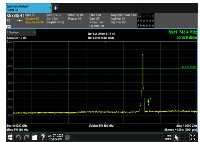
Band17-5MHz-16QAM-23825-25RB#0-30~1000-PASS
