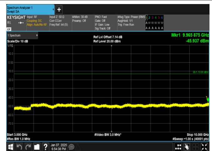
Band17-5MHz-16QAM-23825-25RB#0-3000~10000-PASS
