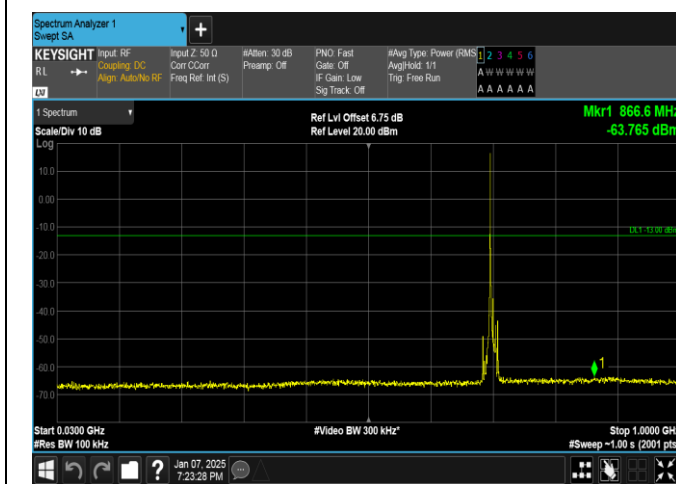
Band17-10MHz-QPSK-23780-1RB#0-30~1000-PASS
