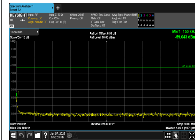
Band17-5MHz-16QAM-23825-25RB#0-0.15~30-PASS
