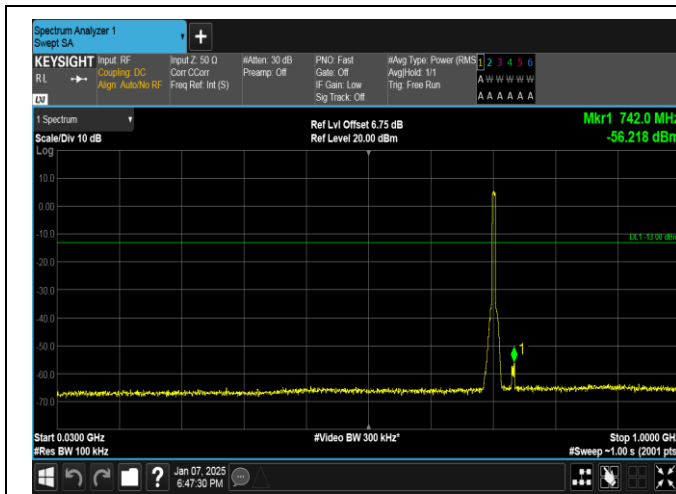
Band17-5MHz-16QAM-23790-25RB#0-30~1000-PASS
