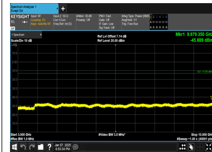
Band17-5MHz-QPSK-23825-25RB#0-3000~10000-PASS
