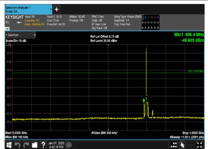
Band17-5MHz-QPSK-23790-1RB#0-30~1000-PASS
