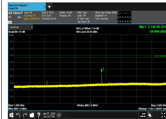
Band17-5MHz-QPSK-23825-1RB#24-1000~3000-PASS
