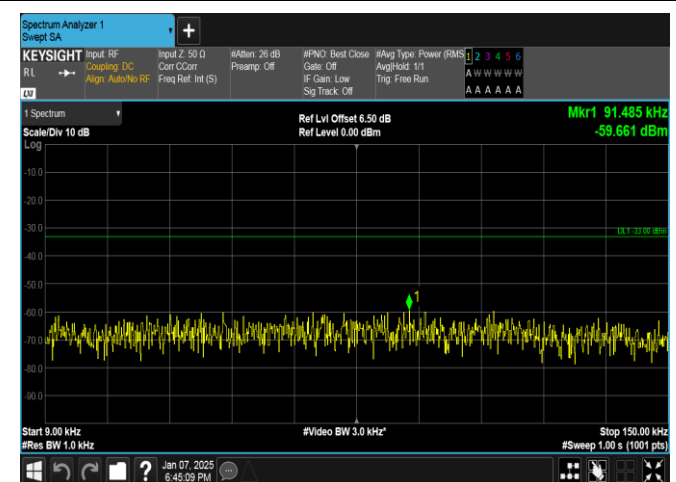
Band17-5MHz-16QAM-23790-1RB#24-0.009~0.15-PASS
