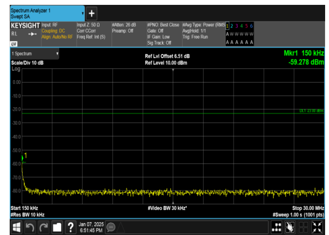
Band17-5MHz-16QAM-23825-1RB#24-0.15~30-PASS
