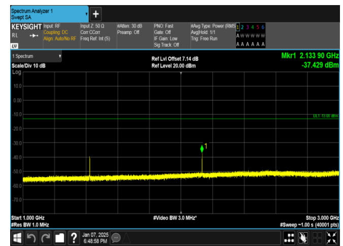
Band17-5MHz-QPSK-23825-1RB#0-1000~3000-PASS
