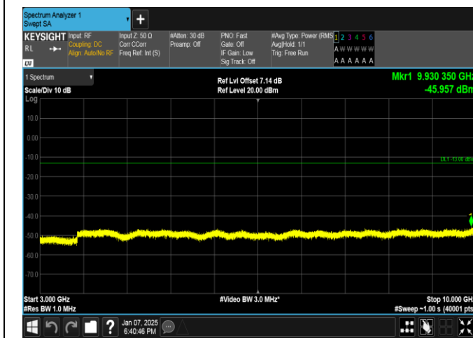
Band17-5MHz-QPSK-23755-25RB#0-3000~10000-PASS
