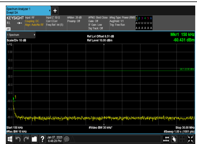
Band17-5MHz-QPSK-23825-1RB#0-0.15~30-PASS
