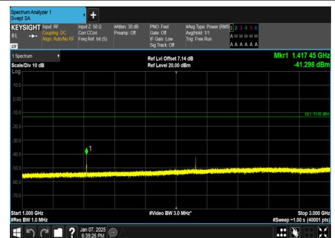
Band17-5MHz-16QAM-23755-1RB#24-1000~3000-PASS
