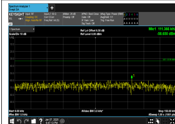
Band17-5MHz-16QAM-23790-25RB#0-0.009~0.15-PASS
