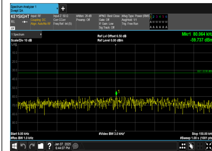
Band17-5MHz-QPSK-23790-1RB#24-0.009~0.15-PASS
