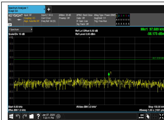
Band17-10MHz-QPSK-23780-1RB#0-0.009~0.15-PASS
