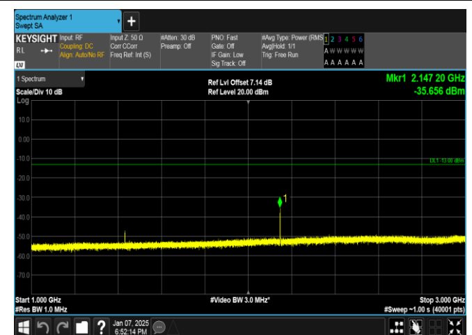
Band17-5MHz-16QAM-23825-1RB#24-1000~3000-PASS
