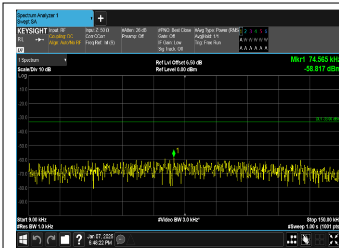
Band17-5MHz-QPSK-23825-1RB#0-0.009~0.15-PASS
