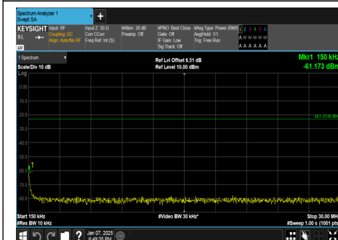
Band17-5MHz-16QAM-23825-1RB#0-0.15~30-PASS
