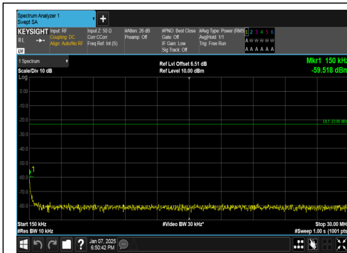
Band17-5MHz-QPSK-23825-1RB#24-0.15~30-PASS
