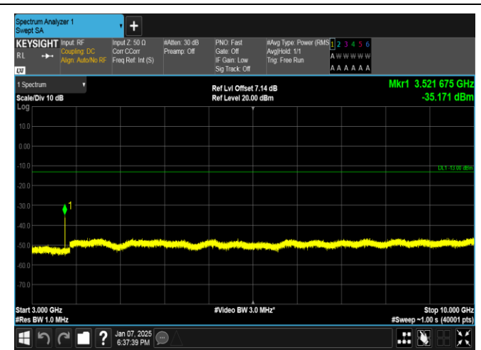
Band17-5MHz-16QAM-23755-1RB#0-3000~10000-PASS
