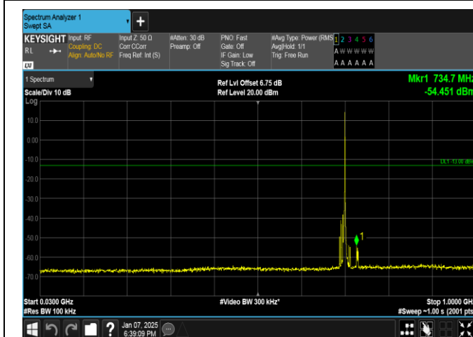
Band17-5MHz-16QAM-23755-1RB#24-30~1000-PASS
