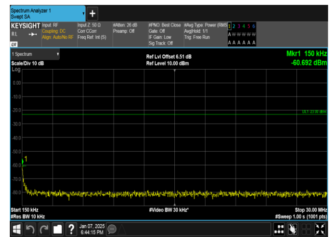
Band17-5MHz-QPSK-23790-1RB#24-0.15~30-PASS
