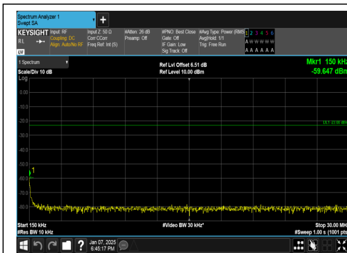
Band17-5MHz-16QAM-23790-1RB#24-0.15~30-PASS
