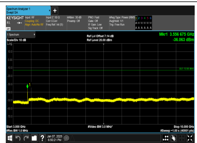
Band17-5MHz-16QAM-23825-1RB#0-3000~10000-PASS
