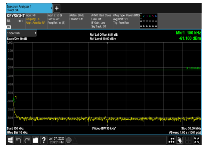
Band17-5MHz-16QAM-23755-1RB#24-0.15~30-PASS
