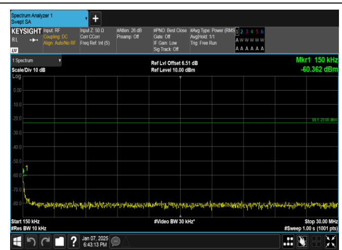
Band17-5MHz-16QAM-23790-1RB#0-0.15~30-PASS
