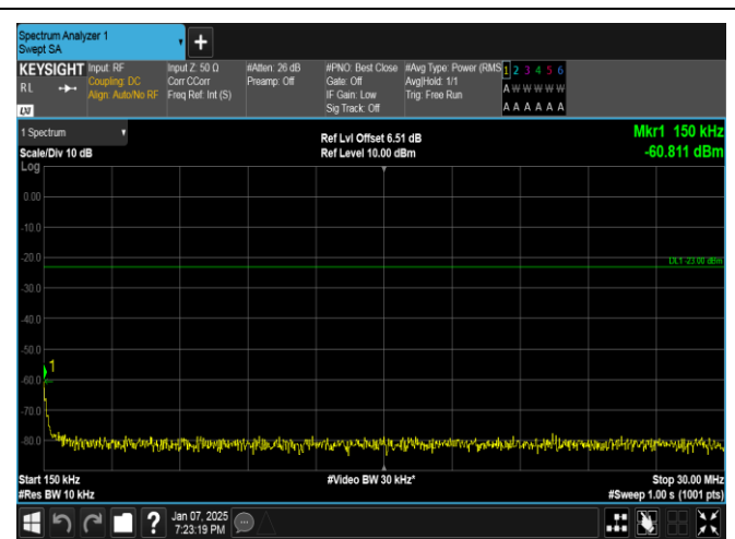
Band17-10MHz-QPSK-23780-1RB#0-0.15~30-PASS
