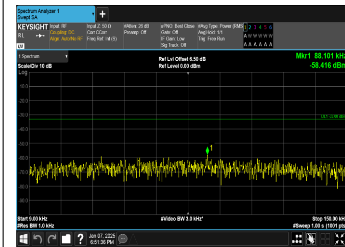
Band17-5MHz-16QAM-23825-1RB#24-0.009~0.15-PASS
