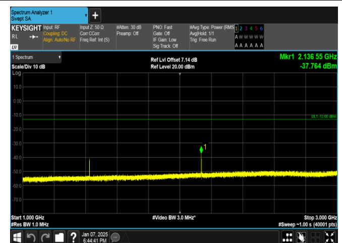
Band17-5MHz-QPSK-23790-1RB#24-1000~3000-PASS
