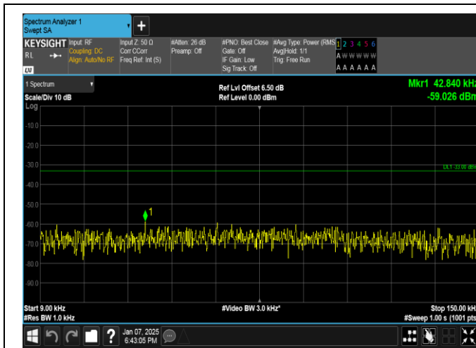
Band17-5MHz-16QAM-23790-1RB#0-0.009~0.15-PASS
