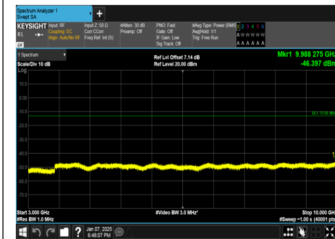
Band17-5MHz-16QAM-23790-25RB#0-3000~10000-PASS
