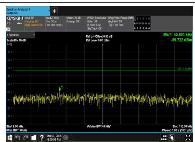
Band17-5MHz-16QAM-23755-25RB#0-0.009~0.15-PASS
