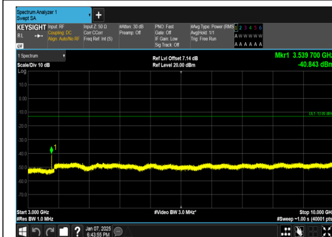
Band17-5MHz-16QAM-23790-1RB#0-3000~10000-PASS
