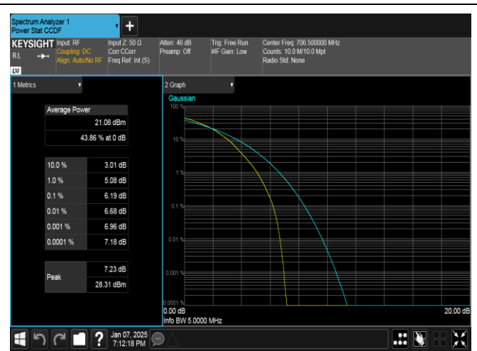
Band17-5MHz-16QAM-23755-25RB#0-PASS
