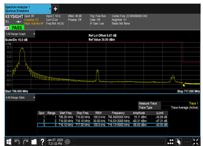
Band17-10MHz-QPSK-23800-1RB#0-PASS
