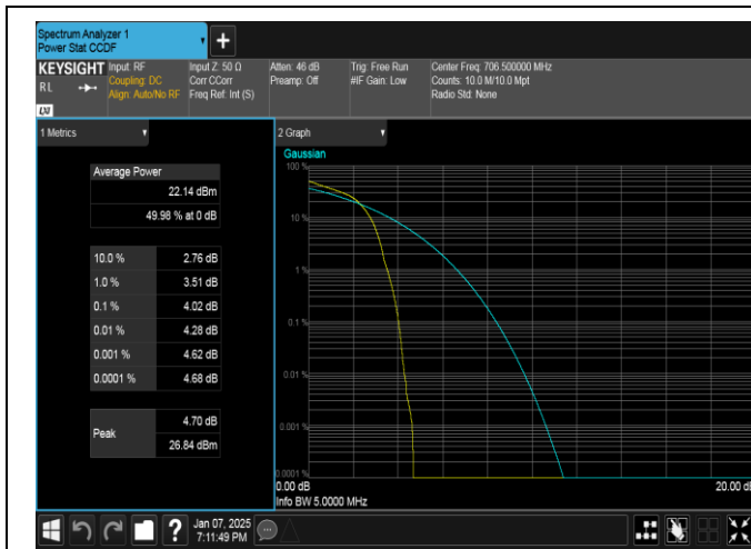
Band17-5MHz-16QAM-23755-1RB#0-PASS
