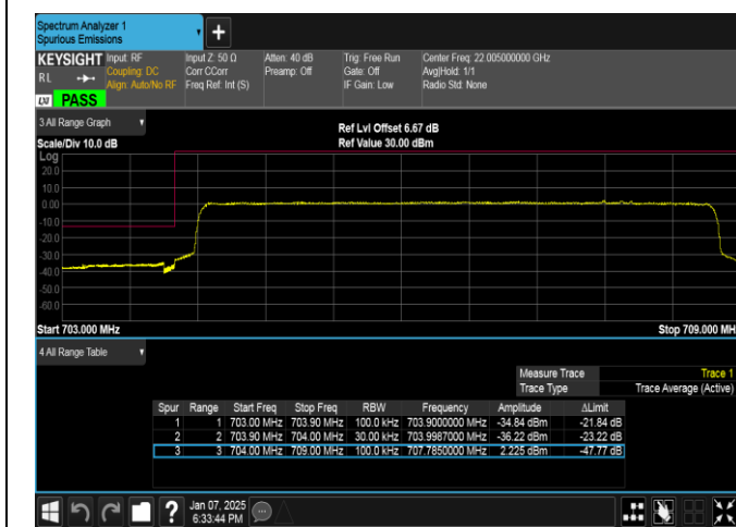
Band17-5MHz-16QAM-23755-25RB#0-PASS
