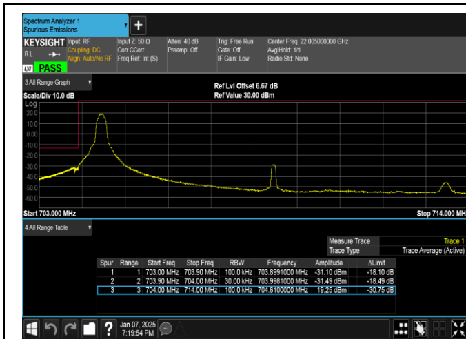
Band17-10MHz-QPSK-23780-1RB#0-PASS
