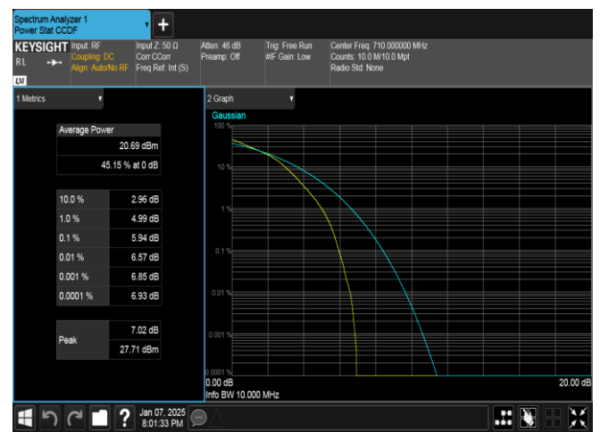
Band17-10MHz-16QAM-23790-50RB#0-PASS
