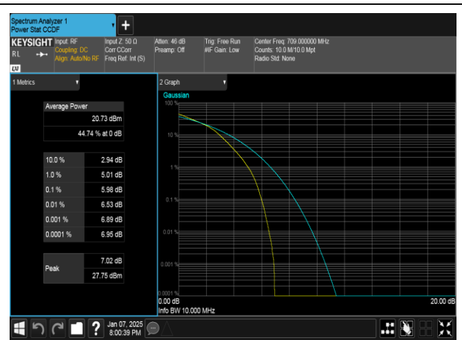
Band17-10MHz-16QAM-23780-50RB#0-PASS
