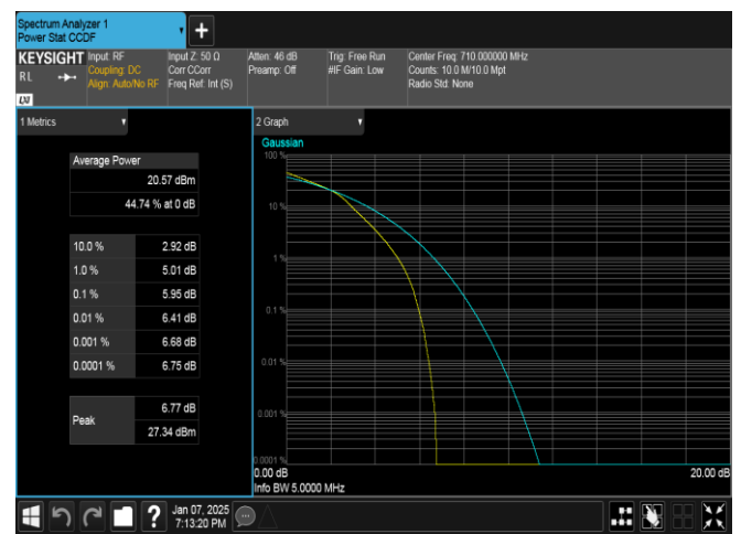
Band17-5MHz-16QAM-23790-25RB#0-PASS
