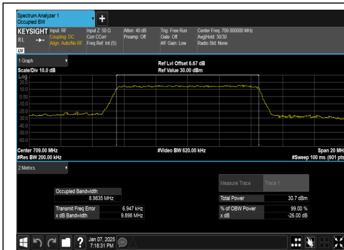
Band17-10MHz-QPSK-23780-50RB#0-PASS
