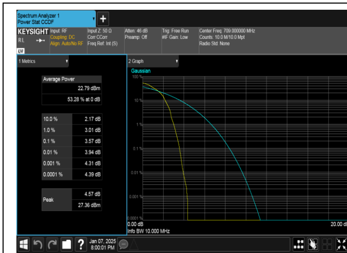
Band17-10MHz-QPSK-23780-1RB#0-PASS
