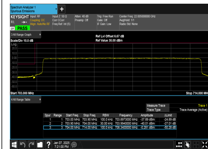
Band17-10MHz-QPSK-23780-50RB#0-PASS
