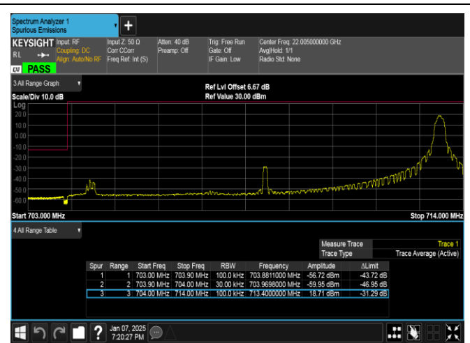
Band17-10MHz-QPSK-23780-1RB#49-PASS
