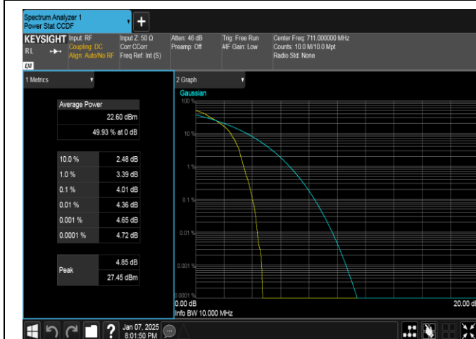
Band17-10MHz-QPSK-23800-1RB#0-PASS
