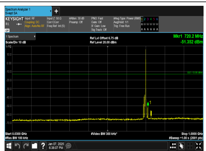
Band17-5MHz-QPSK-23755-1RB#24-30~1000-PASS
