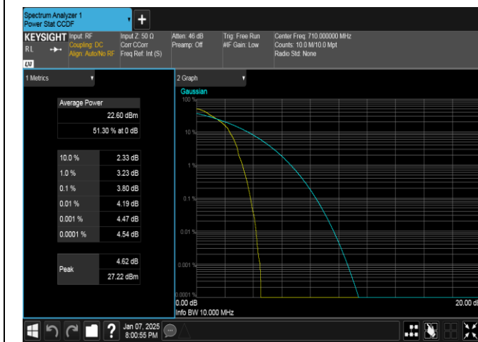
Band17-10MHz-QPSK-23790-1RB#0-PASS
