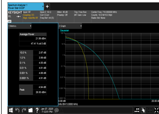
Band17-5MHz-16QAM-23790-1RB#0-PASS
