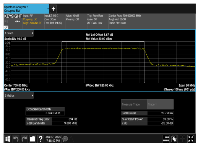
Band17-10MHz-16QAM-23780-50RB#0-PASS
