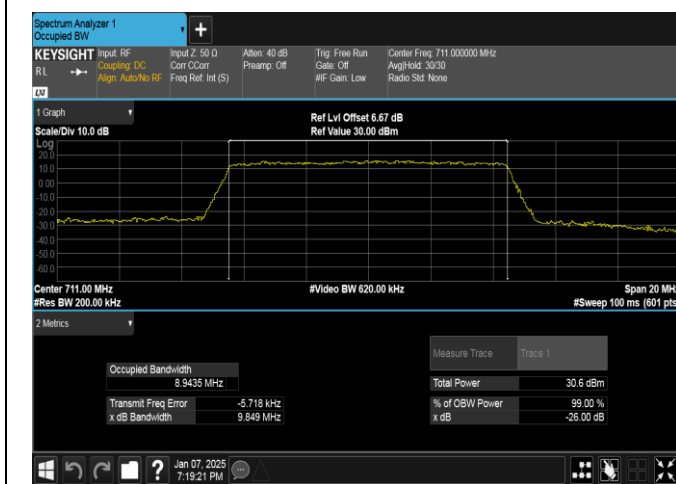
Band17-10MHz-QPSK-23800-50RB#0-PASS
