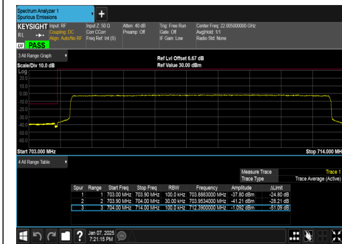
Band17-10MHz-16QAM-23780-50RB#0-PASS
