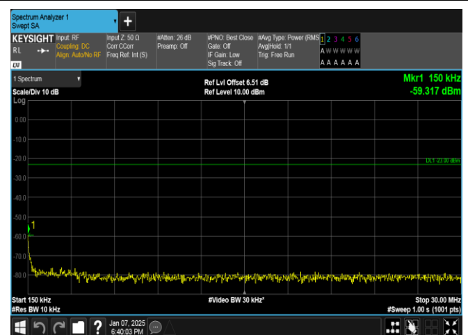
Band17-5MHz-QPSK-23755-25RB#0-0.15~30-PASS
