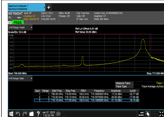
Band17-10MHz-16QAM-23800-1RB#49-PASS
