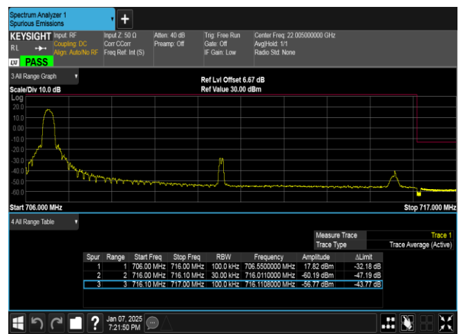
Band17-10MHz-16QAM-23800-1RB#0-PASS
