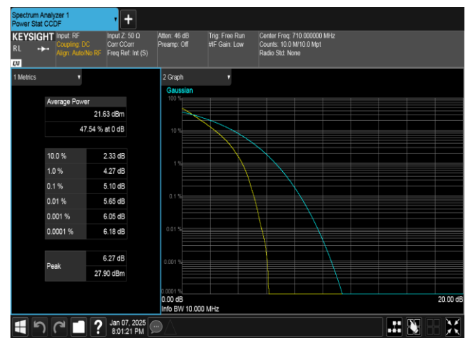
Band17-10MHz-QPSK-23790-50RB#0-PASS
