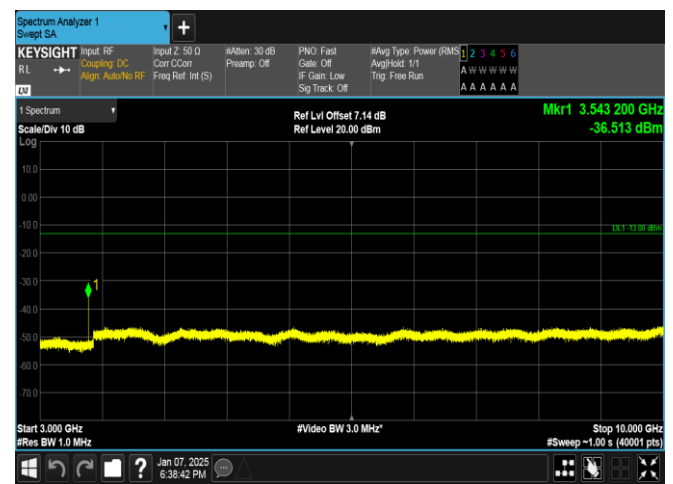
Band17-5MHz-QPSK-23755-1RB#24-3000~10000-PASS
