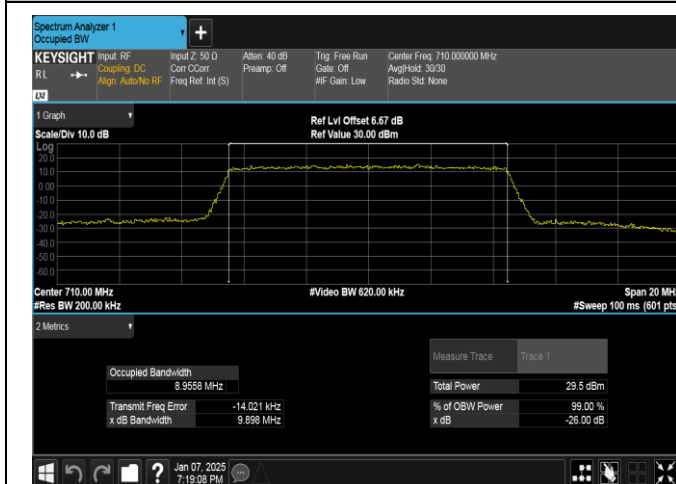
Band17-10MHz-16QAM-23790-50RB#0-PASS
