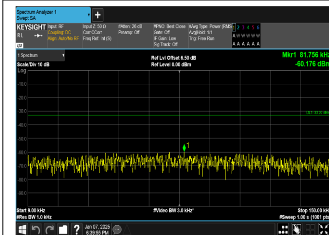
Band17-5MHz-QPSK-23755-25RB#0-0.009~0.15-PASS
