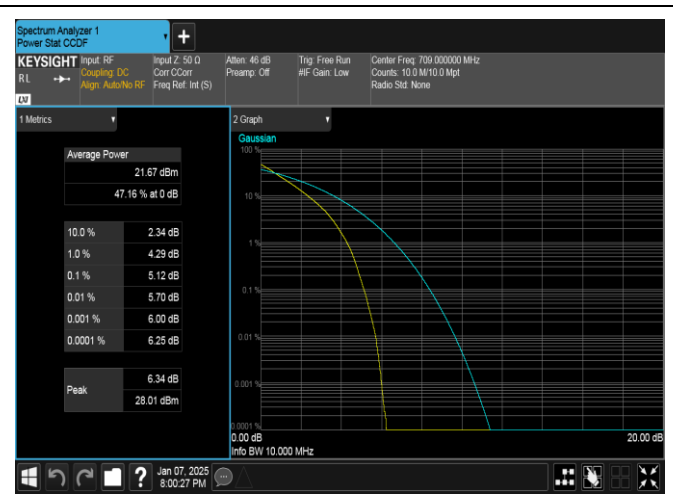
Band17-10MHz-QPSK-23780-50RB#0-PASS
