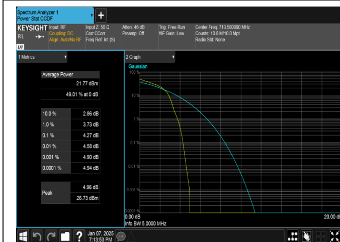
Band17-5MHz-16QAM-23825-1RB#0-PASS
