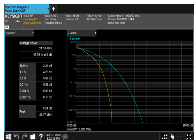
Band17-10MHz-QPSK-23800-50RB#0-PASS
