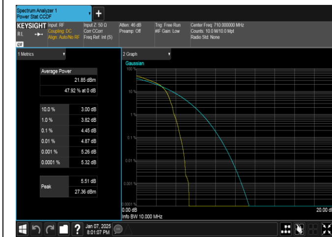
Band17-10MHz-16QAM-23790-1RB#0-PASS
