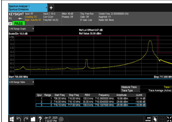
Band17-10MHz-QPSK-23800-1RB#49-PASS
