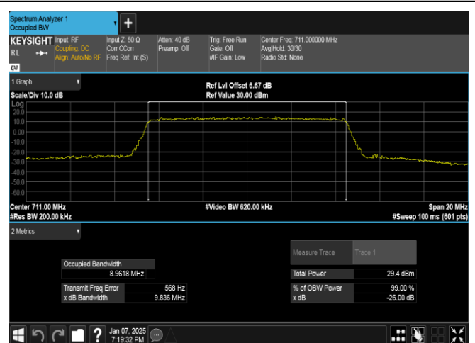
Band17-10MHz-16QAM-23800-50RB#0-PASS
