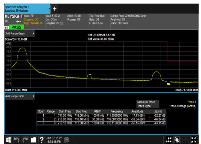
Band17-5MHz-16QAM-23825-1RB#0-PASS
