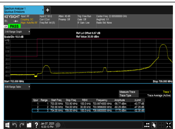
Band17-5MHz-16QAM-23755-1RB#24-PASS
