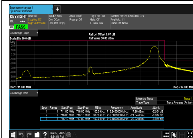
Band17-5MHz-16QAM-23825-1RB#24-PASS
