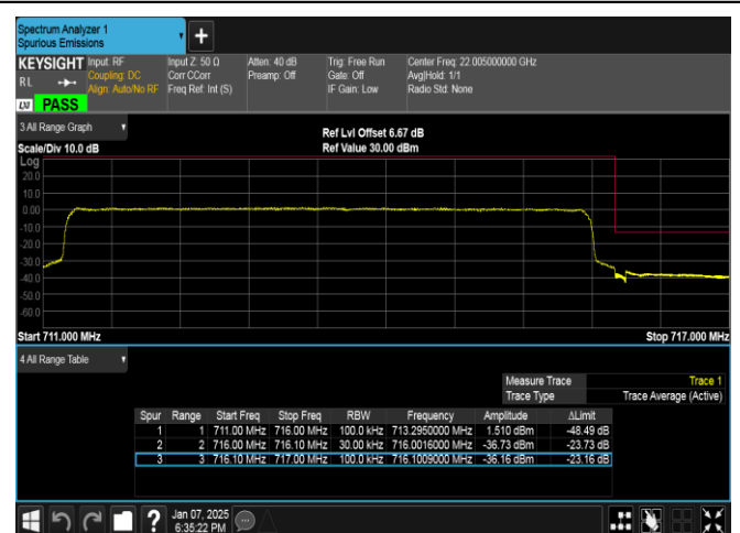
Band17-5MHz-16QAM-23825-25RB#0-PASS
