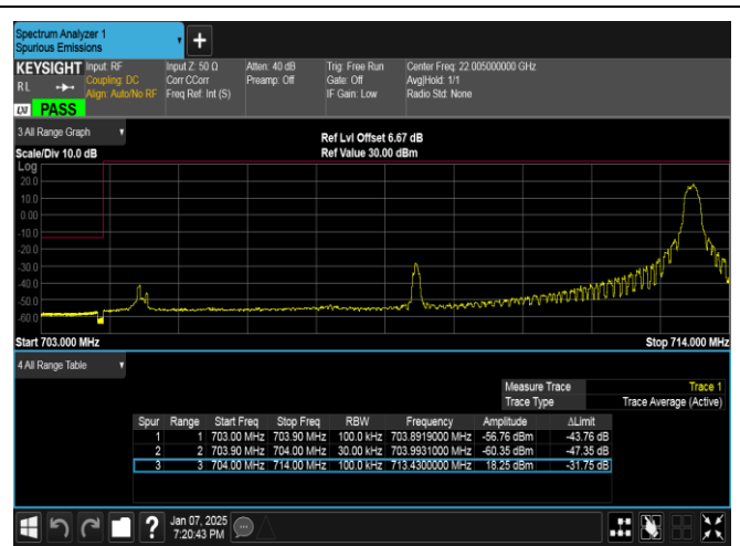
Band17-10MHz-16QAM-23780-1RB#49-PASS
