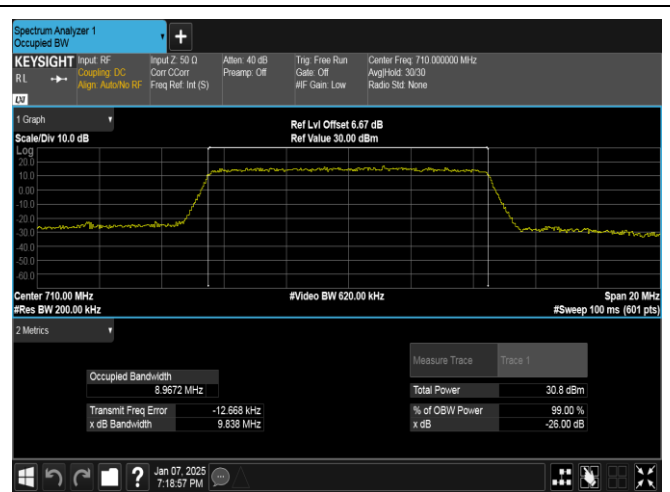
Band17-10MHz-QPSK-23790-50RB#0-PASS
