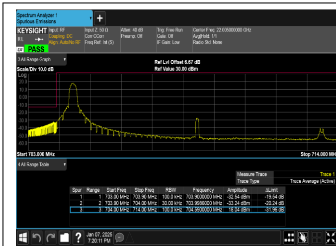
Band17-10MHz-16QAM-23780-1RB#0-PASS
