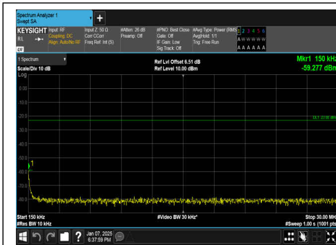
Band17-5MHz-QPSK-23755-1RB#24-0.15~30-PASS
