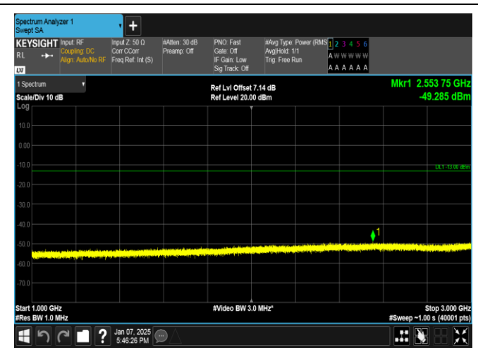
Band13-5MHz-16QAM-23255-1RB#24-1000~3000-PASS
