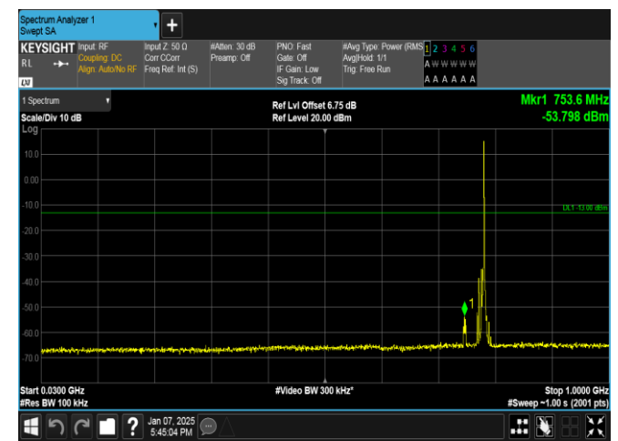
Band13-5MHz-QPSK-23255-1RB#24-30~1000-PASS
