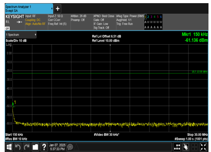
Band13-5MHz-16QAM-23230-1RB#0-0.15~30-PASS
