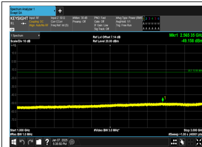
Band13-5MHz-16QAM-23205-25RB#0-1000~3000-PASS
