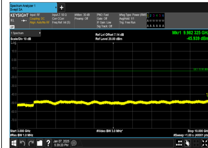
Band13-5MHz-QPSK-23230-1RB#24-3000~10000-PASS
