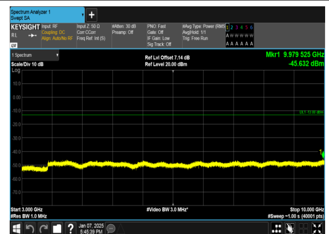
Band13-5MHz-QPSK-23255-1RB#24-3000~10000-PASS
