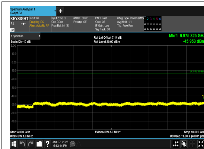
Band13-10MHz-QPSK-23230-1RB#0-3000~10000-PASS
