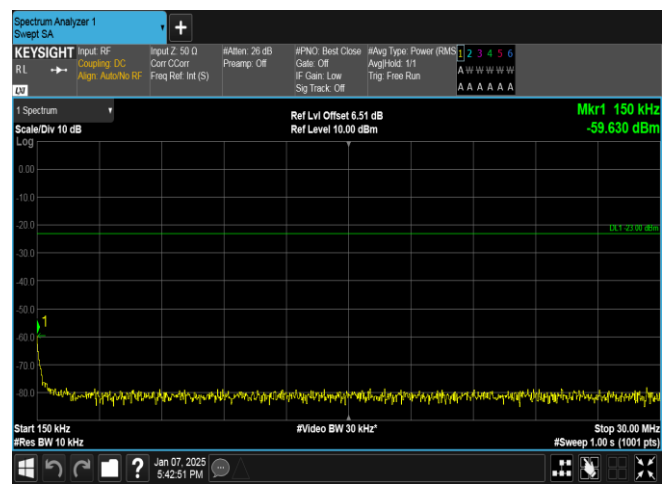
Band13-5MHz-QPSK-23255-1RB#0-0.15~30-PASS
