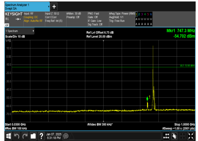
Band13-5MHz-16QAM-23205-1RB#0-30~1000-PASS
