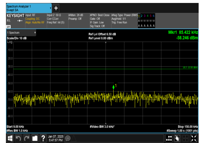
Band13-5MHz-16QAM-23255-25RB#0-0.009~0.15-PASS
