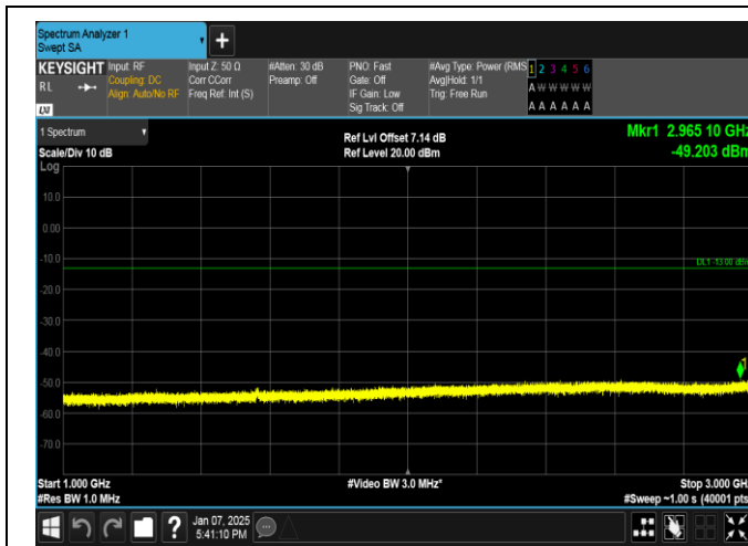
Band13-5MHz-QPSK-23230-25RB#0-1000~3000-PASS
