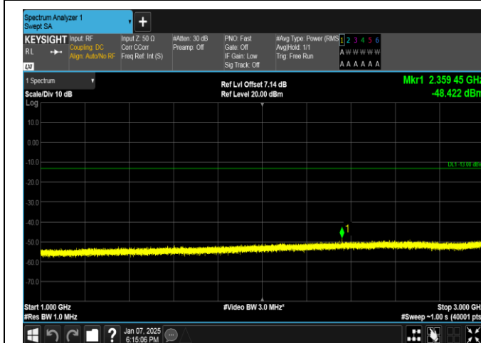
Band13-10MHz-QPSK-23230-1RB#49-1000~3000-PASS
