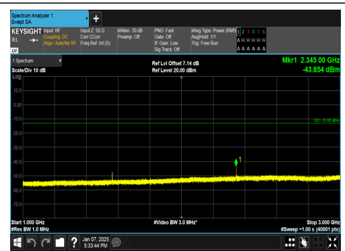
Band13-5MHz-16QAM-23205-1RB#24-1000~3000-PASS
