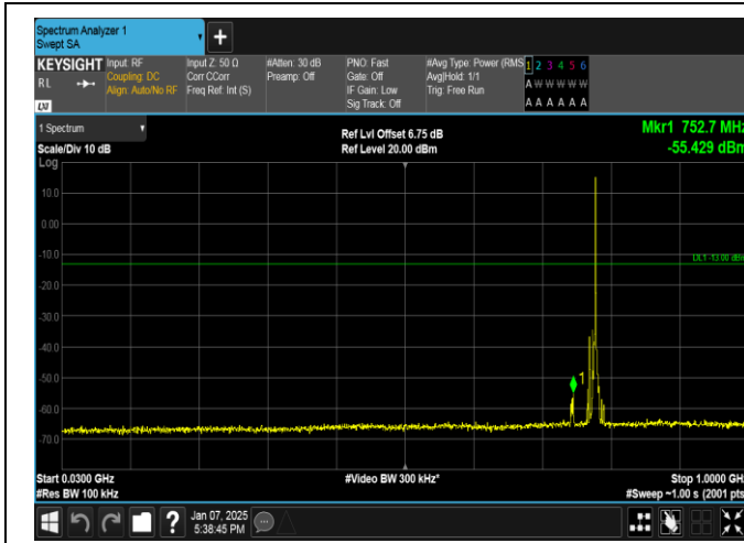
Band13-5MHz-QPSK-23230-1RB#24-30~1000-PASS
