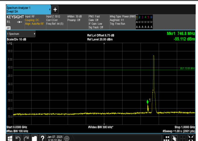
Band13-5MHz-16QAM-23205-25RB#0-30~1000-PASS
