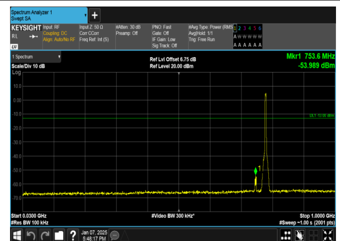
Band13-5MHz-16QAM-23255-25RB#0-30~1000-PASS
