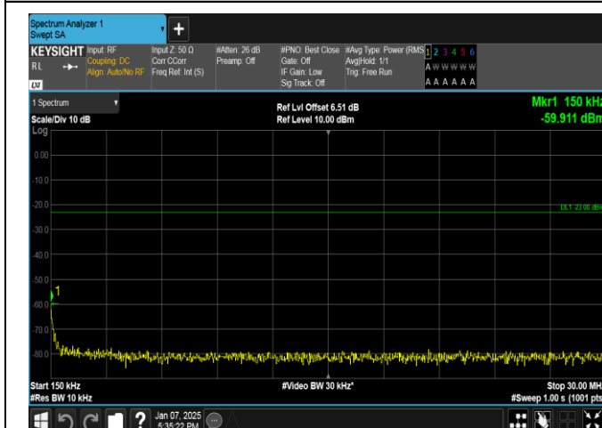
Band13-5MHz-16QAM-23205-25RB#0-0.15~30-PASS
