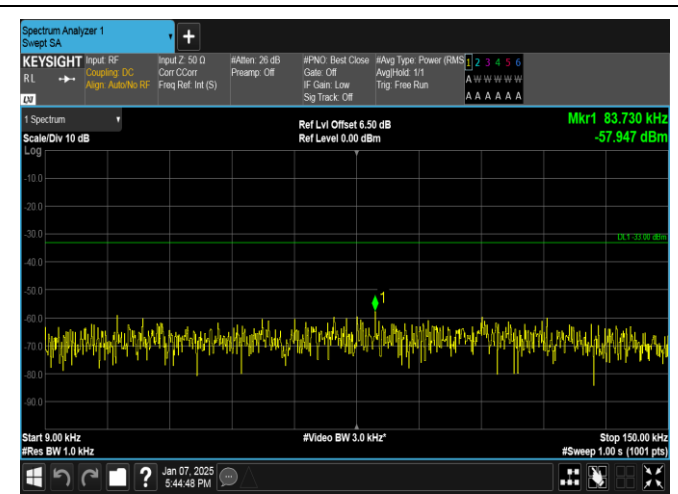
Band13-5MHz-QPSK-23255-1RB#24-0.009~0.15-PASS
