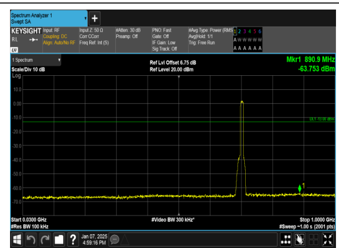
Band12-10MHz-16QAM-23130-50RB#0-30~1000-PASS
