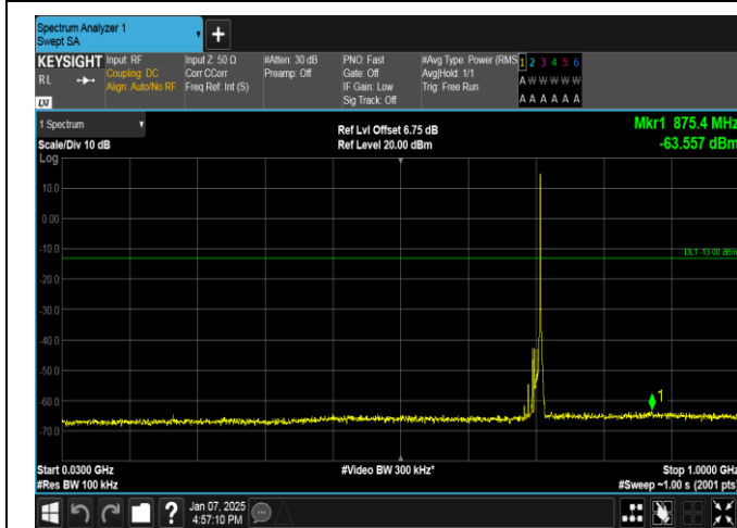
Band12-10MHz-16QAM-23130-1RB#49-30~1000-PASS
