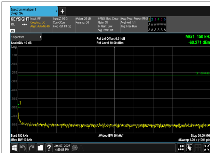
Band12-10MHz-16QAM-23130-50RB#0-0.15~30-PASS
