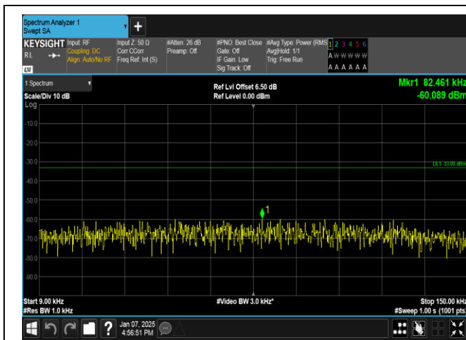
Band12-10MHz-16QAM-23130-1RB#49-0.009~0.15-PASS
