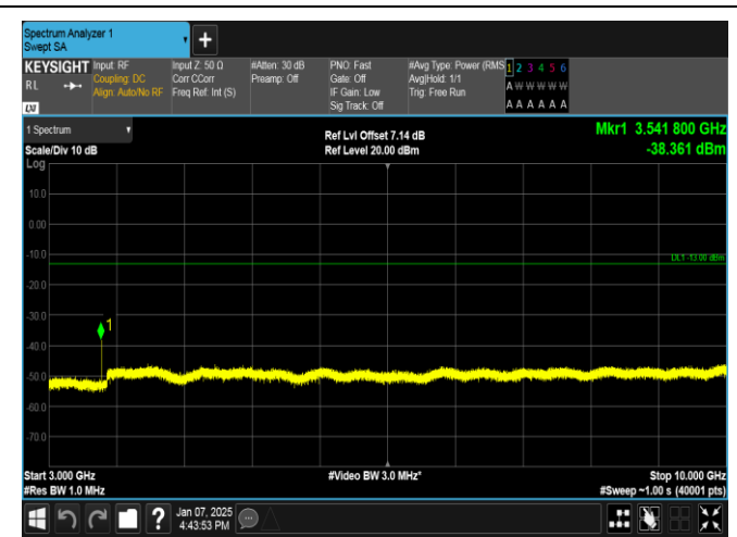
Band12-10MHz-QPSK-23060-1RB#49-3000~10000-PASS
