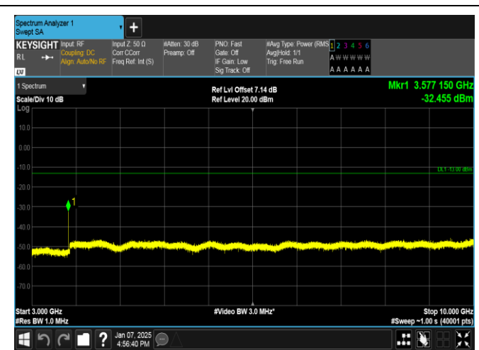
Band12-10MHz-QPSK-23130-1RB#49-3000~10000-PASS
