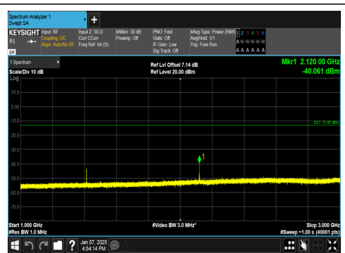
Band12-10MHz-QPSK-23130-1RB#0-1000~3000-PASS
