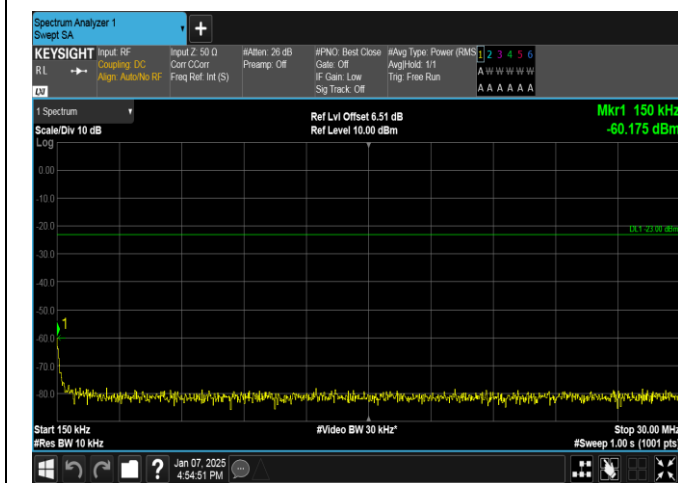
Band12-10MHz-16QAM-23130-1RB#0-0.15~30-PASS
