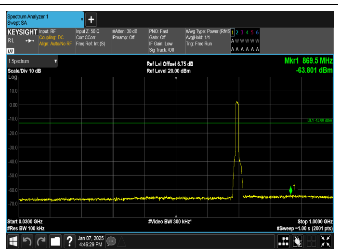
Band12-10MHz-16QAM-23060-50RB#0-30~1000-PASS
