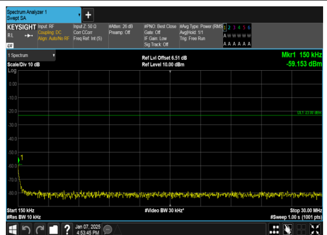
Band12-10MHz-QPSK-23130-1RB#0-0.15~30-PASS
