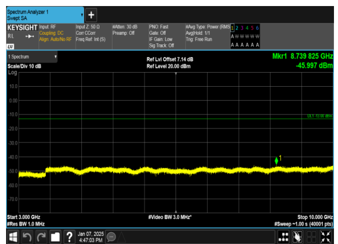
Band12-10MHz-16QAM-23060-50RB#0-3000~10000-PAS S
