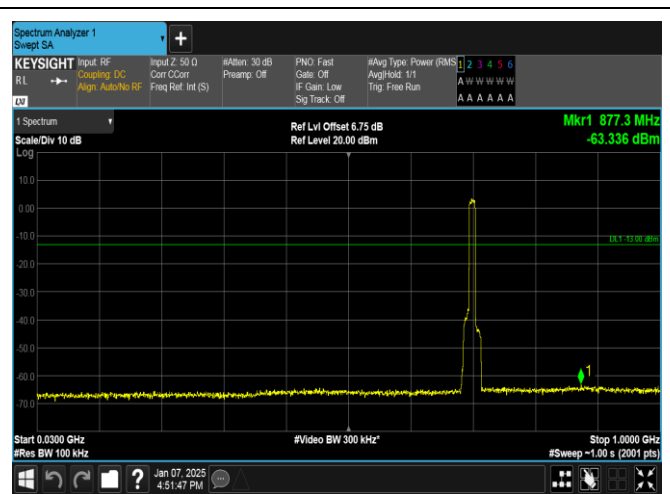
Band12-10MHz-QPSK-23095-50RB#0-30~1000-PASS
