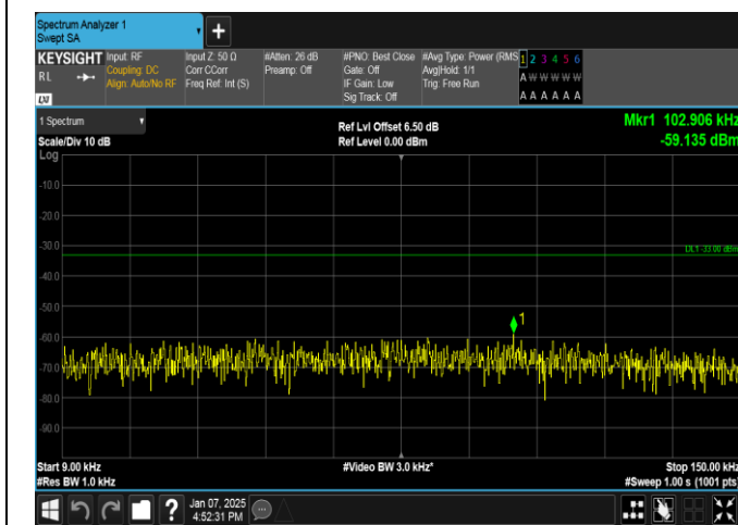
Band12-10MHz-16QAM-23095-50RB#0-0.009~0.15-PASS
