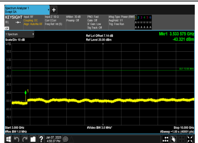
Band12-10MHz-16QAM-23130-1RB#0-3000~10000-PASS
