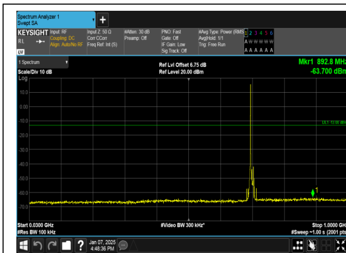
Band12-10MHz-16QAM-23095-1RB#0-30~1000-PASS
