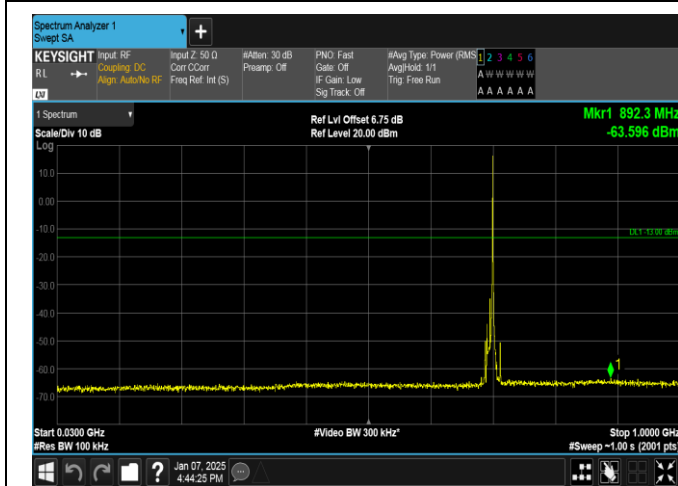
Band12-10MHz-16QAM-23060-1RB#49-30~1000-PASS
