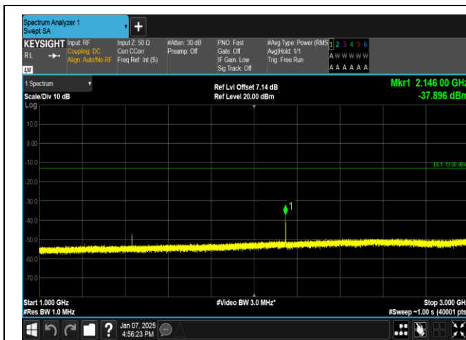
Band12-10MHz-QPSK-23130-1RB#49-1000~3000-PASS
