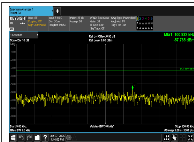
Band12-10MHz-16QAM-23060-1RB#49-0.009~0.15-PASS
