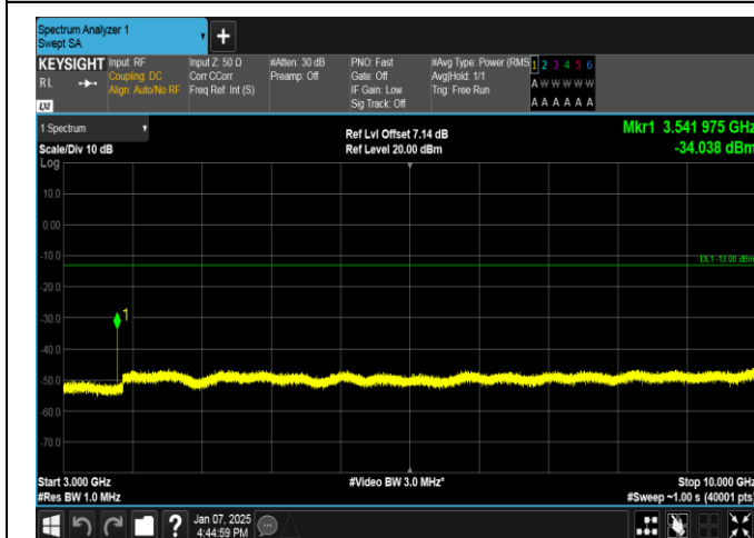
Band12-10MHz-16QAM-23060-1RB#49-3000~10000-PAS
