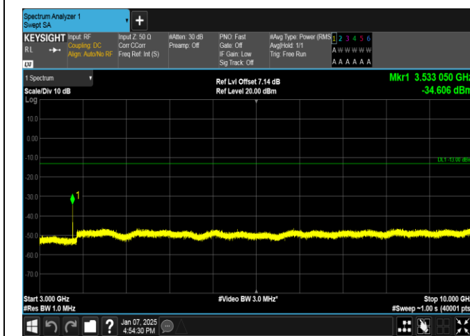
Band12-10MHz-QPSK-23130-1RB#0-3000~10000-PASS
