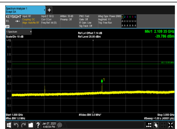
Band12-10MHz-16QAM-23095-1RB#0-1000~3000-PASS
