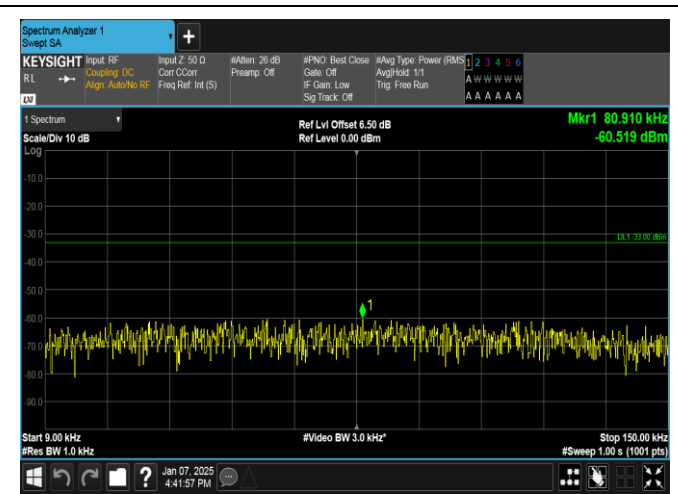
Band12-10MHz-16QAM-23060-1RB#0-0.009~0.15-PASS
