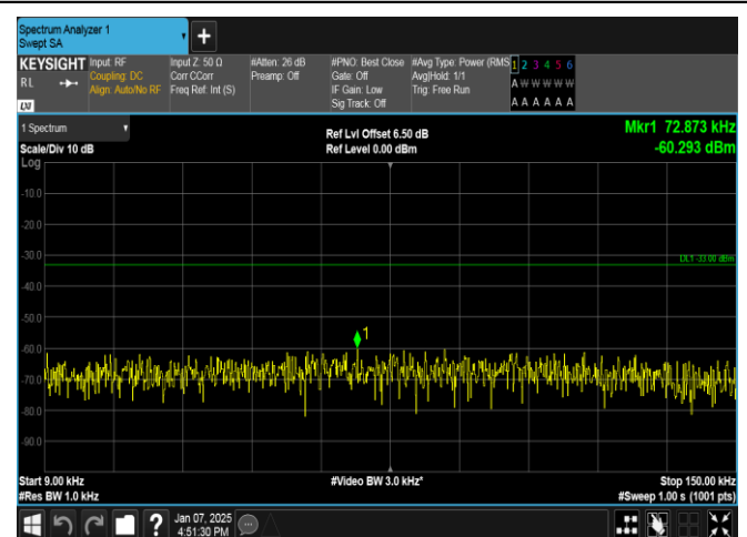
Band12-10MHz-QPSK-23095-50RB#0-0.009~0.15-PASS
