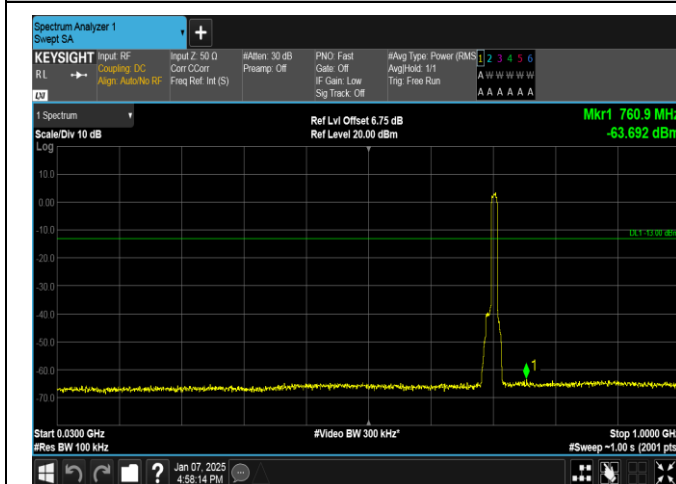
Band12-10MHz-QPSK-23130-50RB#0-30~1000-PASS
