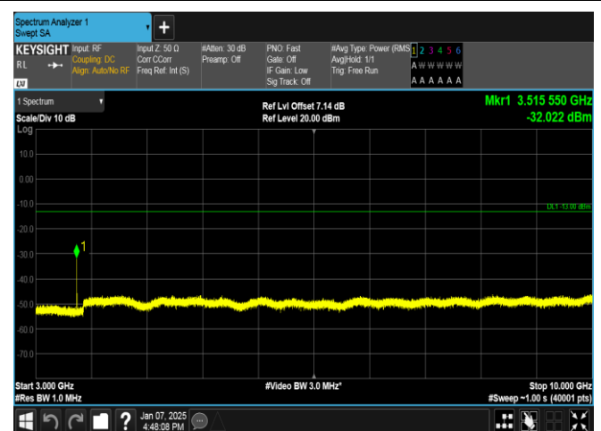
Band12-10MHz-QPSK-23095-1RB#0-3000~10000-PASS
