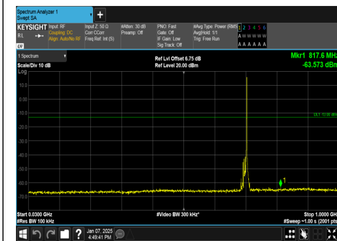
Band12-10MHz-QPSK-23095-1RB#49-30~1000-PASS
