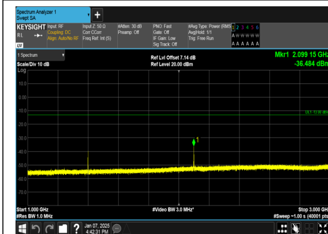
Band12-10MHz-16QAM-23060-1RB#0-1000~3000-PASS
