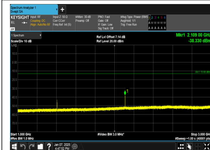
Band12-10MHz-QPSK-23095-1RB#0-1000~3000-PASS
