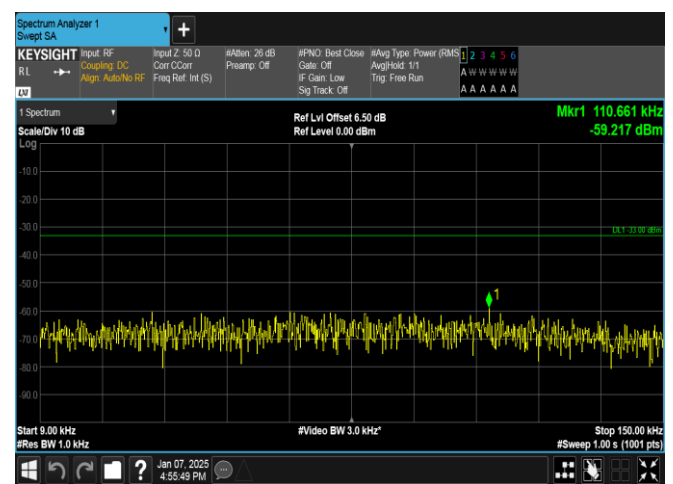
Band12-10MHz-QPSK-23130-1RB#49-0.009~0.15-PASS
