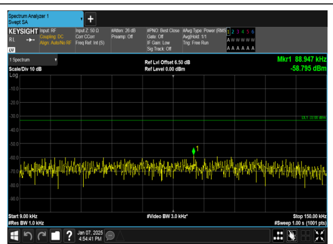
Band12-10MHz-16QAM-23130-1RB#0-0.009~0.15-PASS
