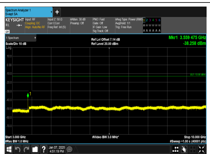
Band12-10MHz-16QAM-23095-1RB#49-3000~10000-PASS S
