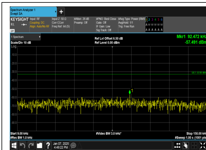
Band12-10MHz-QPSK-23095-1RB#49-0.009~0.15-PASS
