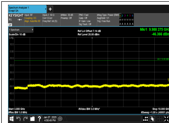
Band12-10MHz-QPSK-23130-50RB#0-3000~10000-PASS
