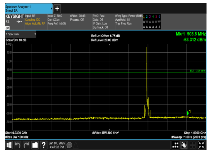
Band12-10MHz-QPSK-23095-1RB#0-30~1000-PASS
