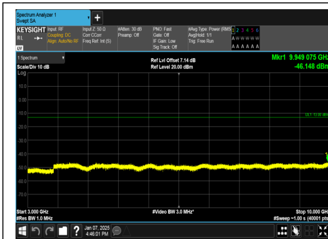
Band12-10MHz-QPSK-23060-50RB#0-3000~10000-PASS
