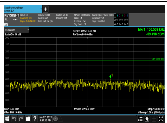
Band12-10MHz-QPSK-23095-1RB#0-0.009~0.15-PASS
