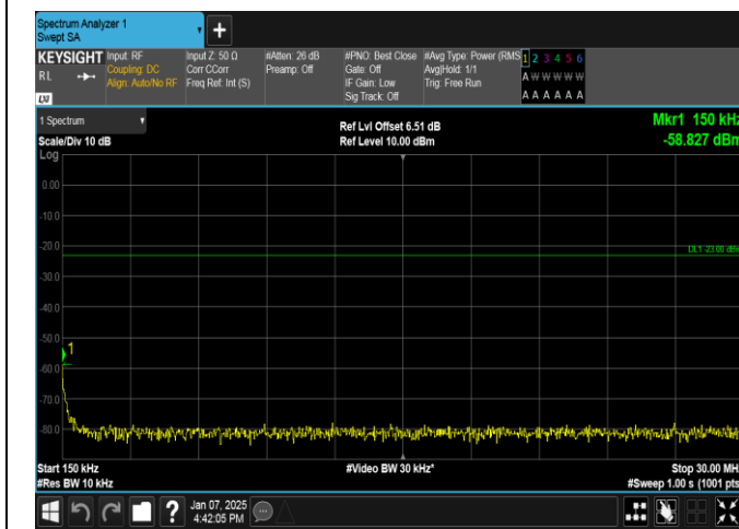
Band12-10MHz-16QAM-23060-1RB#0-0.15~30-PASS
