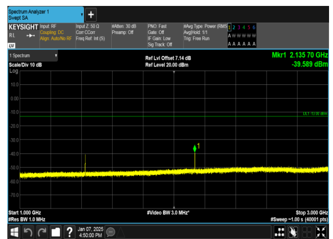
Band12-10MHz-QPSK-23095-1RB#49-1000~3000-PASS
