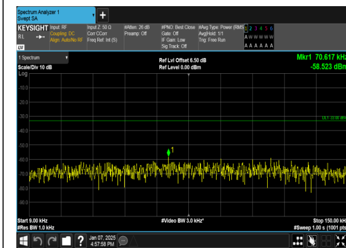
Band12-10MHz-QPSK-23130-50RB#0-0.009~0.15-PASS
