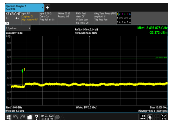
Band12-10MHz-16QAM-23060-1RB#0-3000~10000-PASS
