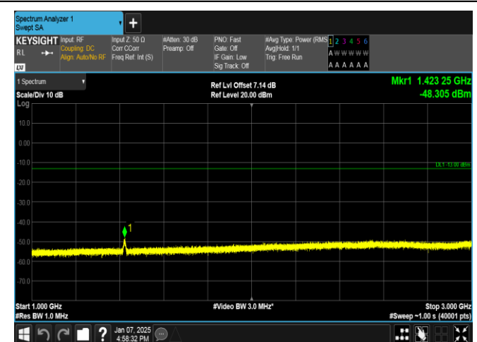
Band12-10MHz-QPSK-23130-50RB#0-1000~3000-PASS
