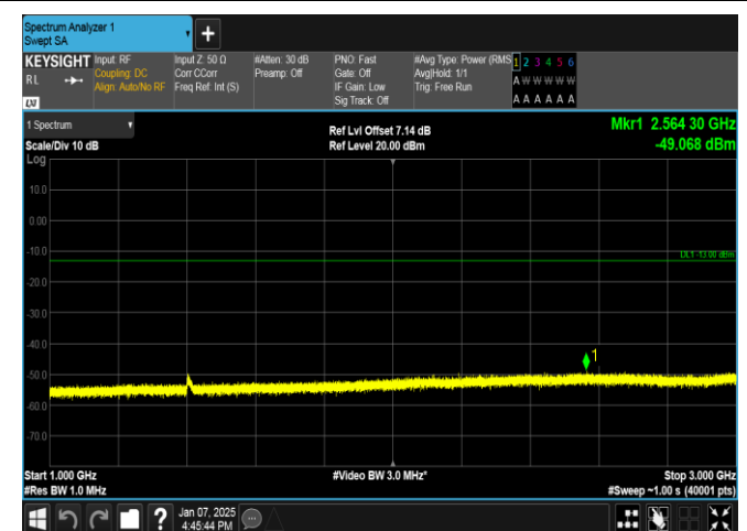
Band12-10MHz-QPSK-23060-50RB#0-1000~3000-PASS
