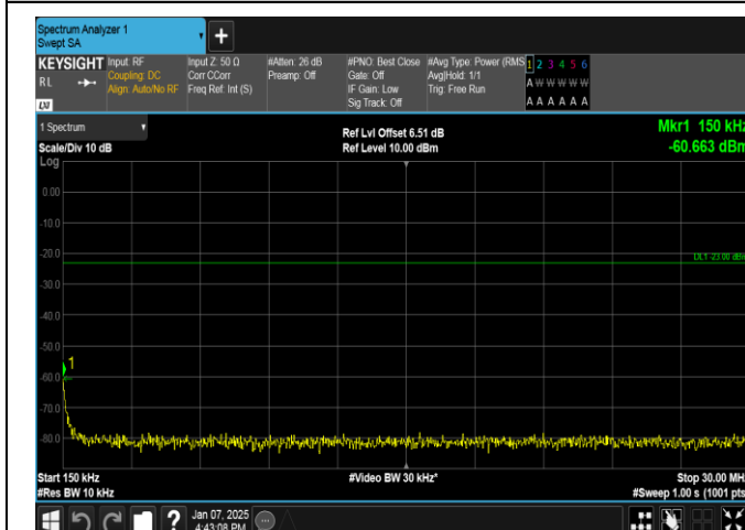
Band12-10MHz-QPSK-23060-1RB#49-0.15~30-PASS
