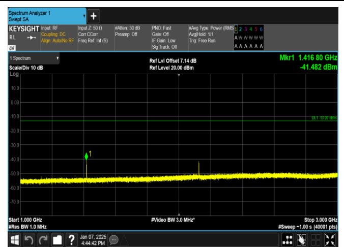
Band12-10MHz-16QAM-23060-1RB#49-1000~3000-PASS
