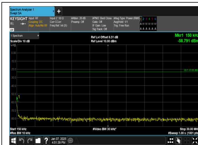
Band12-10MHz-QPSK-23095-50RB#0-0.15~30-PASS
