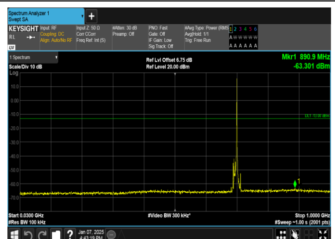
Band12-10MHz-QPSK-23060-1RB#49-30~1000-PASS
