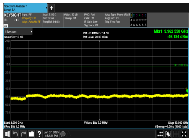
Band12-10MHz-QPSK-23095-50RB#0-3000~10000-PASS
