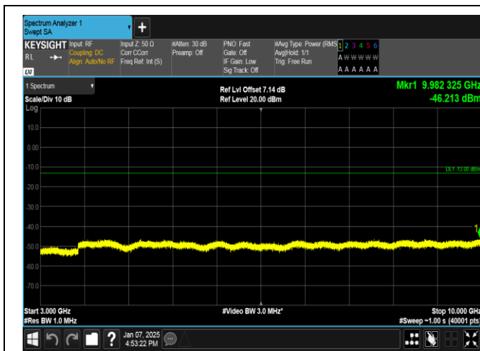
Band12-10MHz-16QAM-23095-50RB#0-3000~10000-PAS S
