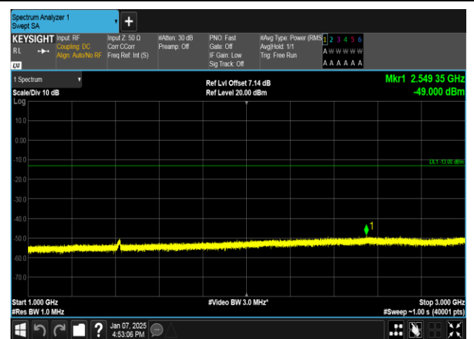
Band12-10MHz-16QAM-23095-50RB#0-1000~3000-PASS
