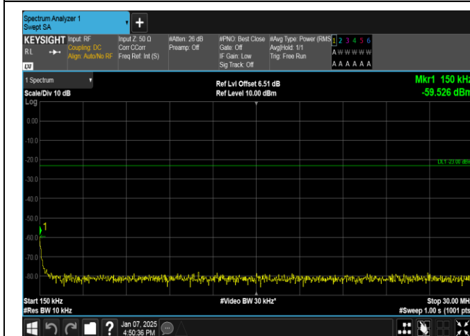
Band12-10MHz-16QAM-23095-1RB#49-0.15~30-PASS
