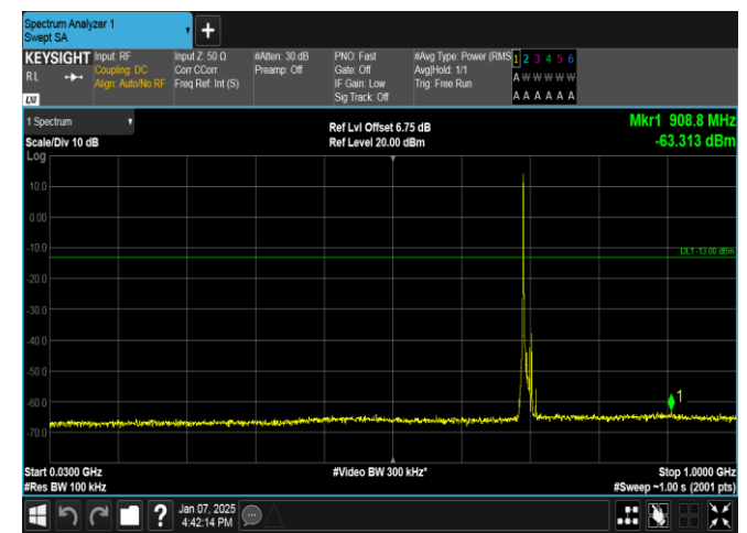
Band12-10MHz-16QAM-23060-1RB#0-30~1000-PASS
