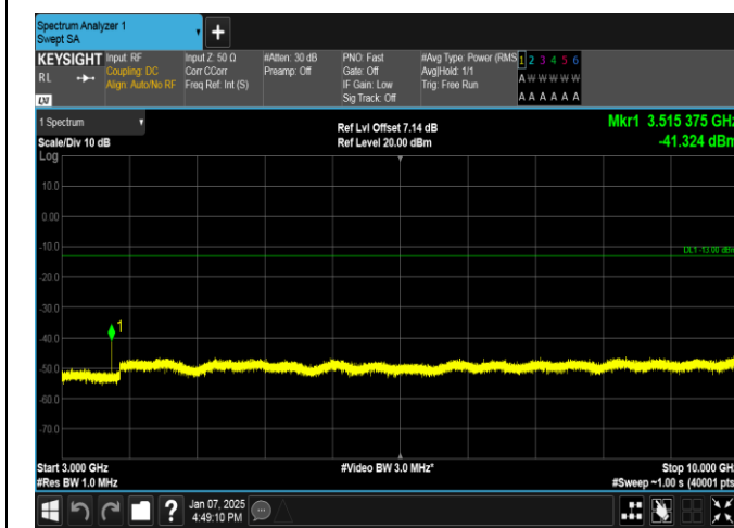
Band12-10MHz-16QAM-23095-1RB#0-3000~10000-PASS
