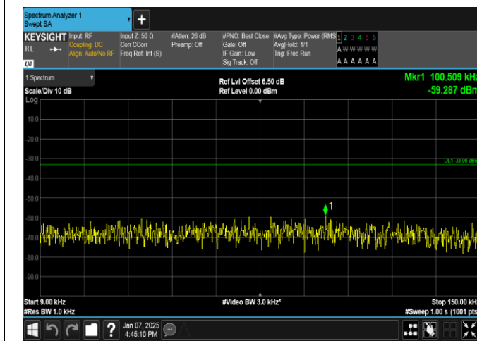
Band12-10MHz-QPSK-23060-50RB#0-0.009~0.15-PASS
