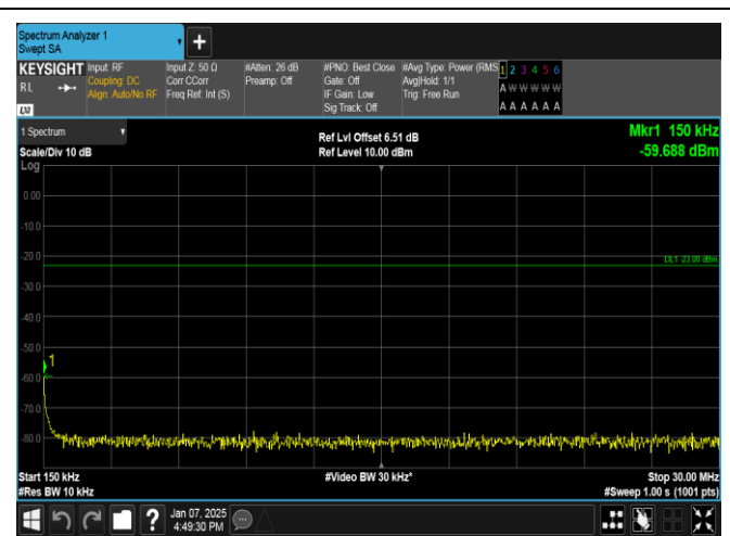
Band12-10MHz-QPSK-23095-1RB#49-0.15~30-PASS
