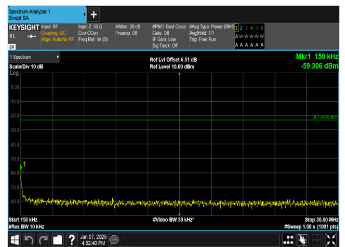
Band12-10MHz-16QAM-23095-50RB#0-0.15~30-PASS
