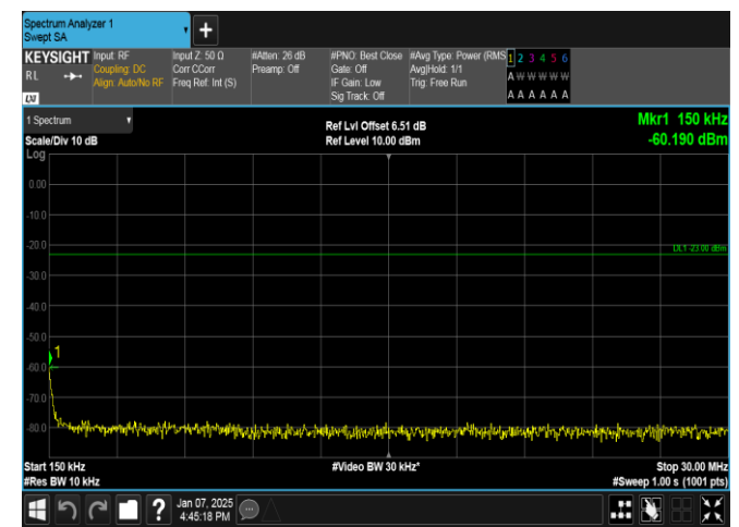
Band12-10MHz-QPSK-23060-50RB#0-0.15~30-PASS
