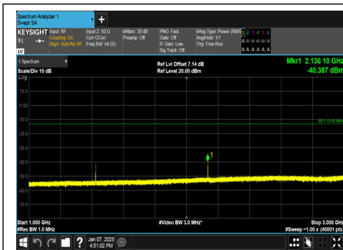
Band12-10MHz-16QAM-23095-1RB#49-1000~3000-PASS
