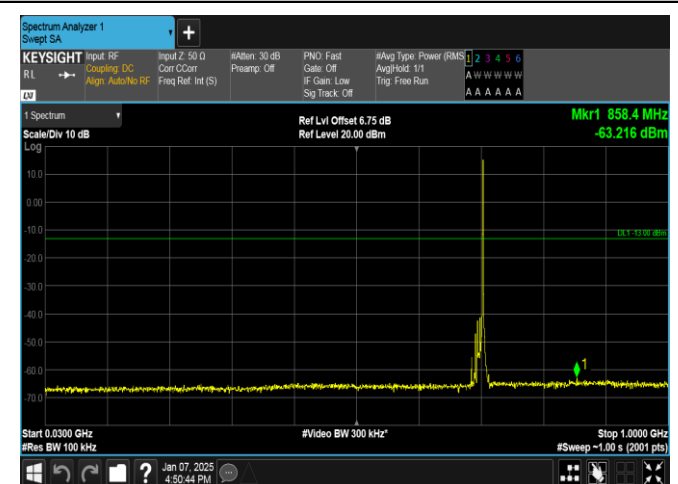
Band12-10MHz-16QAM-23095-1RB#49-30~1000-PASS
