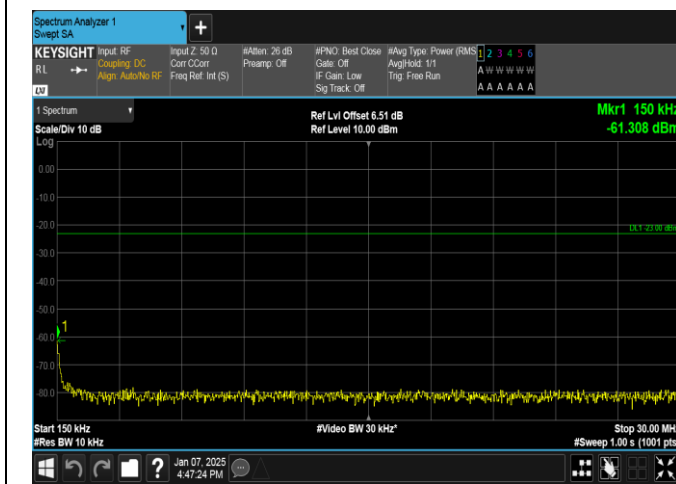
Band12-10MHz-QPSK-23095-1RB#0-0.15~30-PASS
