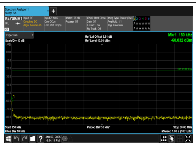
Band12-10MHz-16QAM-23060-1RB#49-0.15~30-PASS
