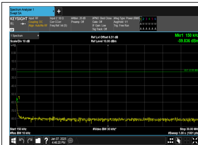
Band12-10MHz-16QAM-23060-50RB#0-0.15~30-PASS
