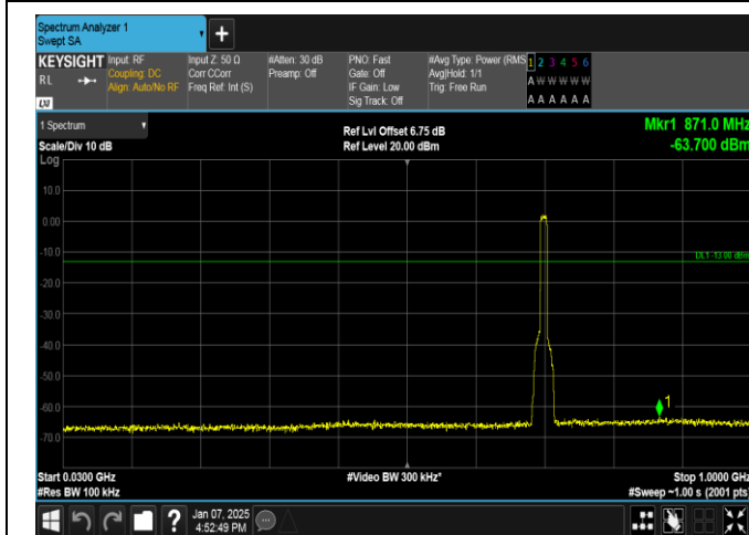
Band12-10MHz-16QAM-23095-50RB#0-30~1000-PASS
