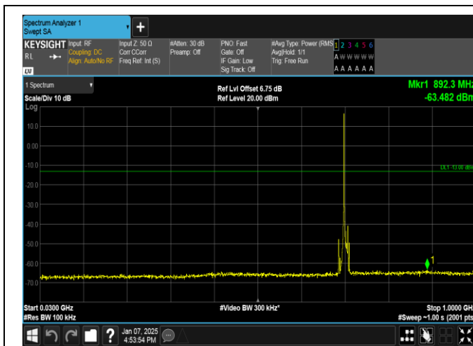
Band12-10MHz-QPSK-23130-1RB#0-30~1000-PASS
