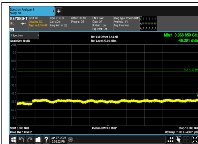
Band12-5MHz-QPSK-23035-25RB#0-3000~10000-PASS
