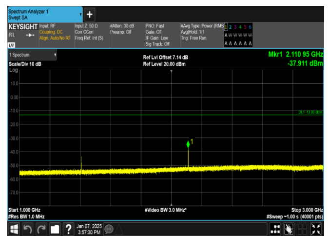
Band12-5MHz-16QAM-23035-1RB#24-1000~3000-PASS
