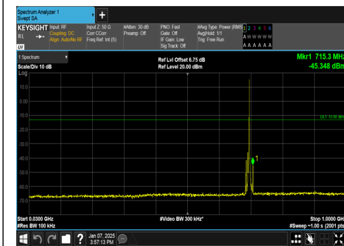
Band12-5MHz-16QAM-23035-1RB#24-30~1000-PASS
