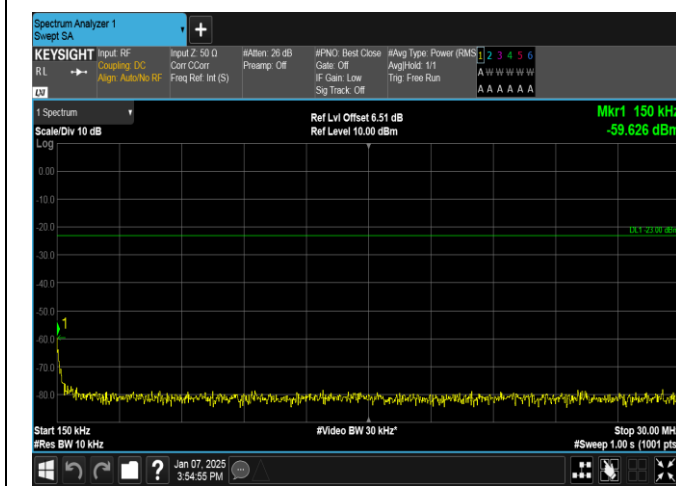
Band12-5MHz-16QAM-23035-1RB#0-0.15~30-PASS
