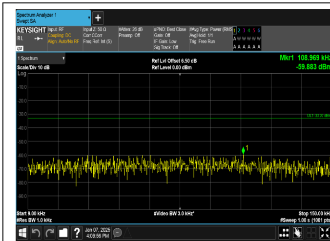
Band12-5MHz-16QAM-23155-1RB#24-0.009~0.15-PASS
