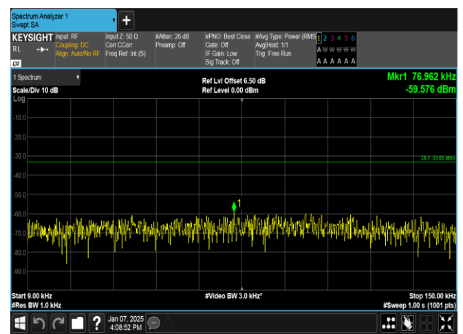
Band12-5MHz-QPSK-23155-1RB#24-0.009~0.15-PASS
