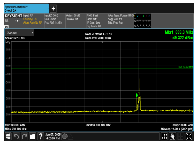
Band12-5MHz-16QAM-23155-1RB#0-30~1000-PASS
