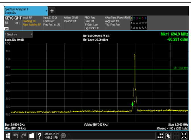
Band12-5MHz-QPSK-23095-25RB#0-30~1000-PASS
