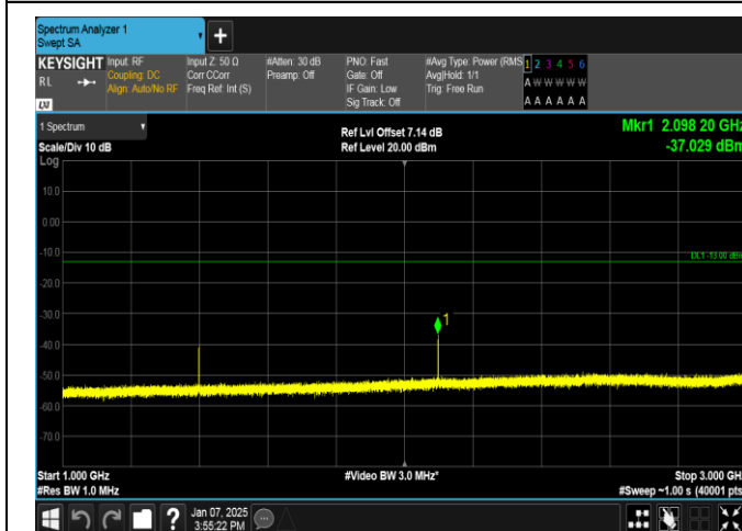
Band12-5MHz-16QAM-23035-1RB#0-1000~3000-PASS
