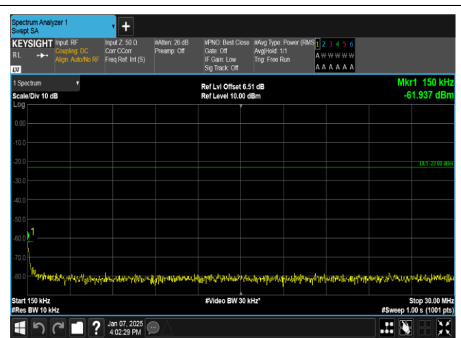
Band12-5MHz-QPSK-23095-1RB#24-0.15~30-PASS
