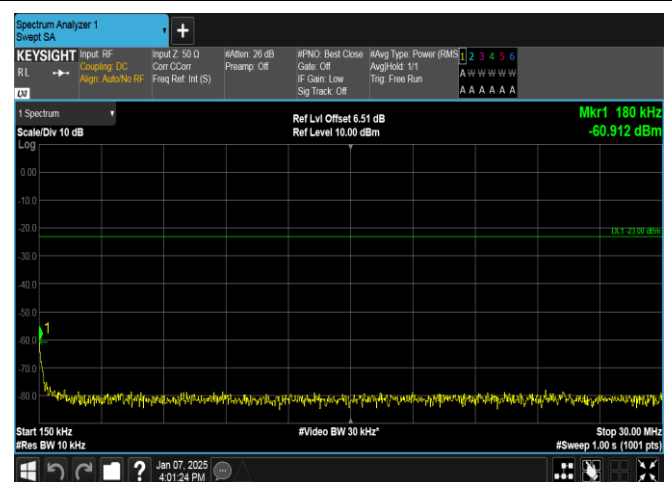
Band12-5MHz-16QAM-23095-1RB#0-0.15~30-PASS
