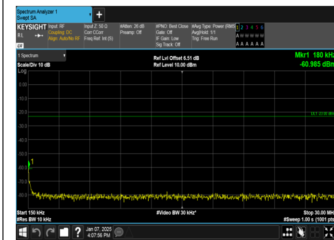
Band12-5MHz-16QAM-23155-1RB#0-0.15~30-PASS
