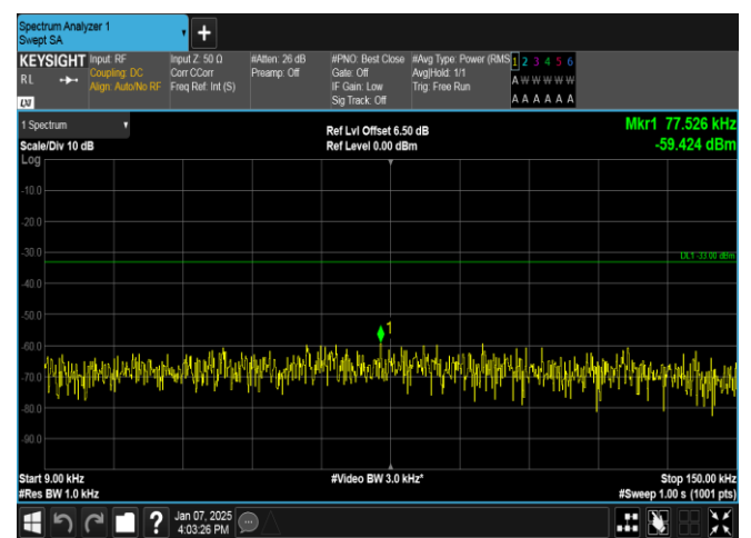
Band12-5MHz-16QAM-23095-1RB#24-0.009~0.15-PASS
