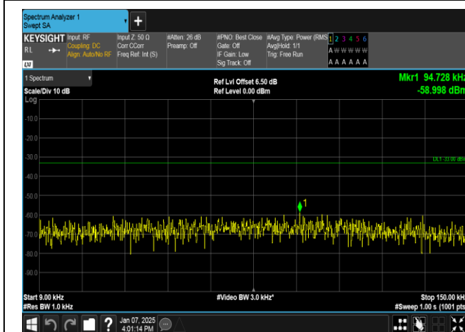
Band12-5MHz-16QAM-23095-1RB#0-0.009~0.15-PASS
