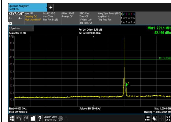
Band12-5MHz-QPSK-23095-1RB#24-30~1000-PASS
