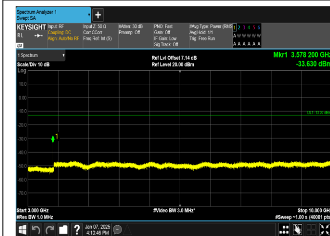
Band12-5MHz-16QAM-23155-1RB#24-3000~10000-PASS
