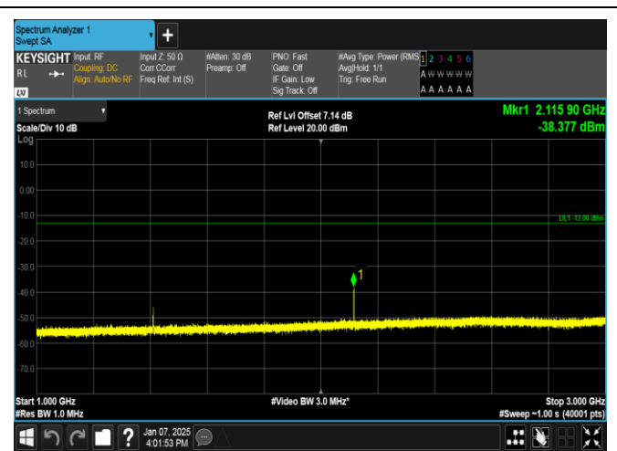
Band12-5MHz-16QAM-23095-1RB#0-1000~3000-PASS
