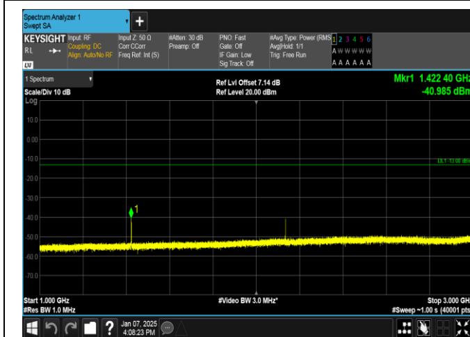
Band12-5MHz-16QAM-23155-1RB#0-1000~3000-PASS
