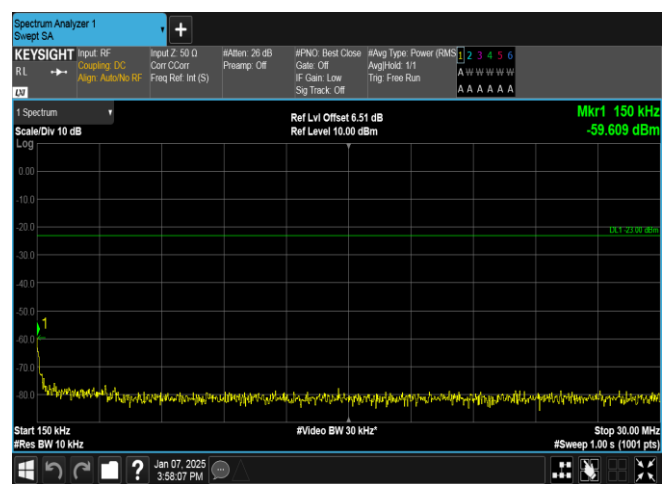
Band12-5MHz-QPSK-23035-25RB#0-0.15~30-PASS
