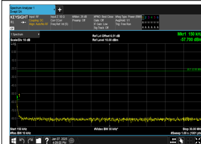
Band12-5MHz-QPSK-23155-1RB#24-0.15~30-PASS
