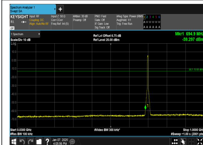
Band12-5MHz-16QAM-23095-25RB#0-30~1000-PASS
