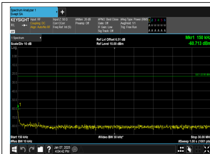
Band12-5MHz-QPSK-23095-25RB#0-0.15~30-PASS
