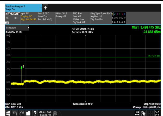
Band12-5MHz-16QAM-23035-1RB#0-3000~10000-PASS
