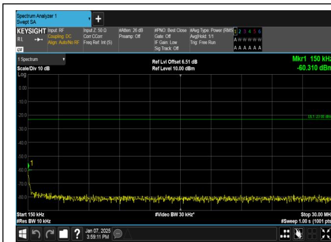
Band12-5MHz-16QAM-23035-25RB#0-0.15~30-PASS
