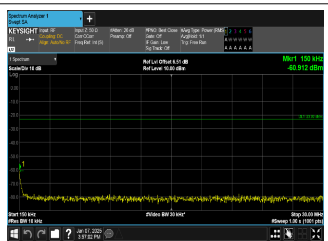
Band12-5MHz-16QAM-23035-1RB#24-0.15~30-PASS
