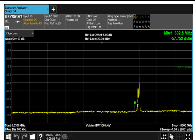
Band12-5MHz-QPSK-23155-1RB#24-30~1000-PASS
