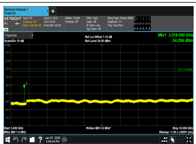
Band12-5MHz-QPSK-23035-1RB#24-3000~10000-PASS
