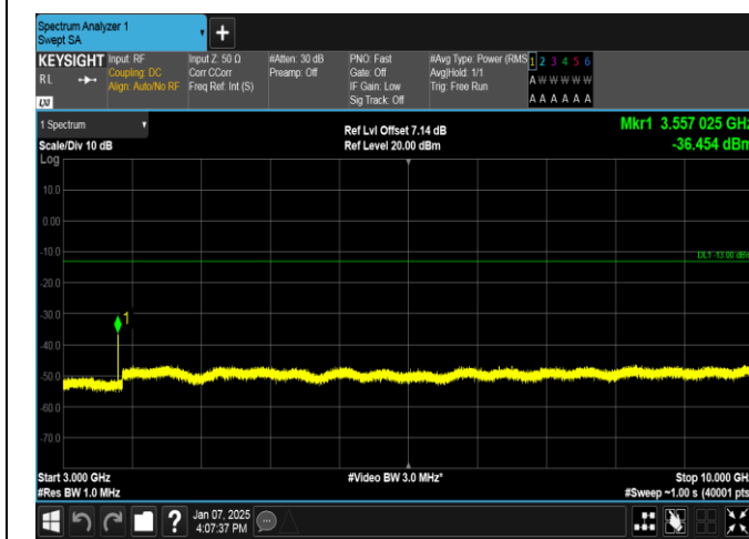
Band12-5MHz-QPSK-23155-1RB#0-3000~10000-PASS
