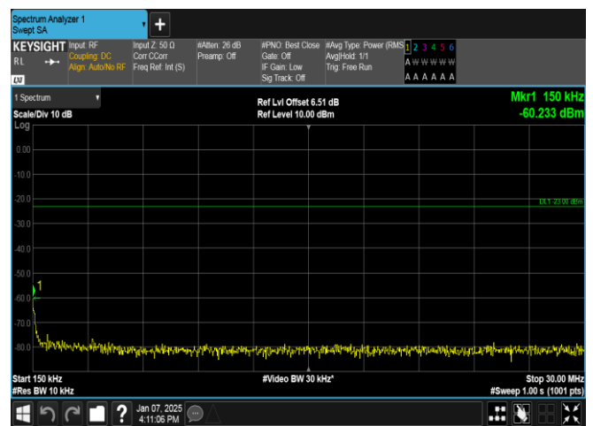
Band12-5MHz-QPSK-23155-25RB#0-0.15~30-PASS
