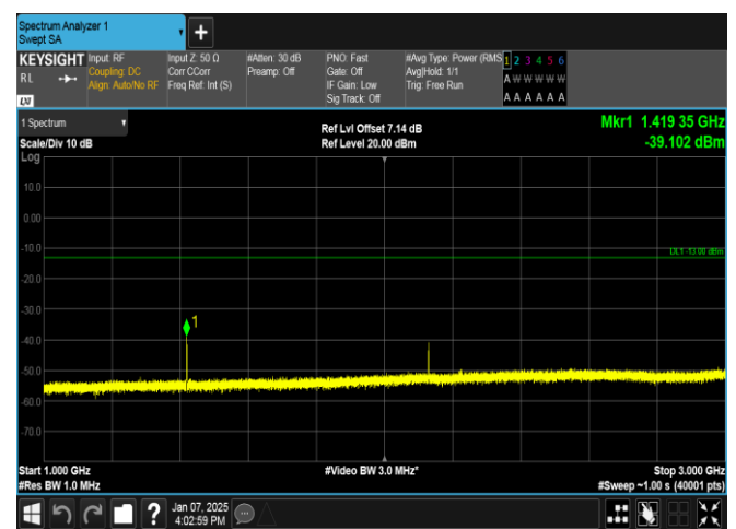
Band12-5MHz-QPSK-23095-1RB#24-1000~3000-PASS
