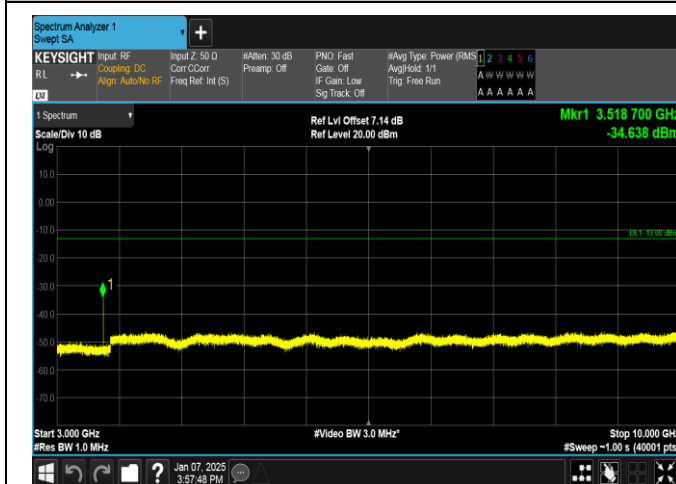
Band12-5MHz-16QAM-23035-1RB#24-3000~10000-PASS
