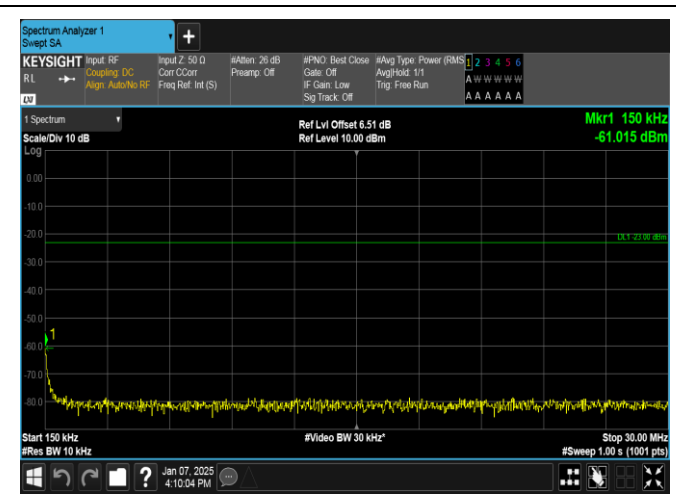
Band12-5MHz-16QAM-23155-1RB#24-0.15~30-PASS
