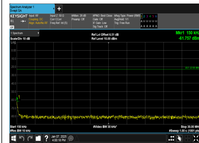
Band12-5MHz-QPSK-23095-1RB#0-0.15~30-PASS
