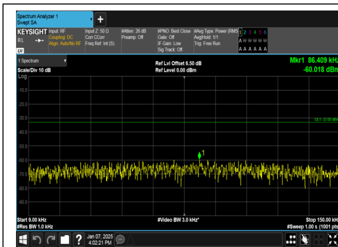
Band12-5MHz-QPSK-23095-1RB#24-0.009~0.15-PASS
