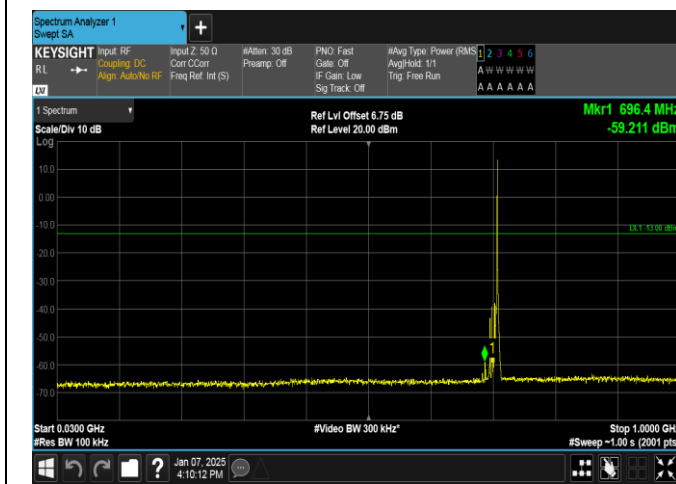
Band12-5MHz-16QAM-23155-1RB#24-30~1000-PASS
