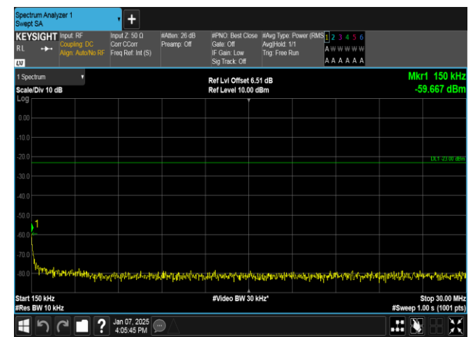
Band12-5MHz-16QAM-23095-25RB#0-0.15~30-PASS
