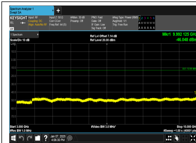
Band12-5MHz-16QAM-23095-25RB#0-3000~10000-PASS
