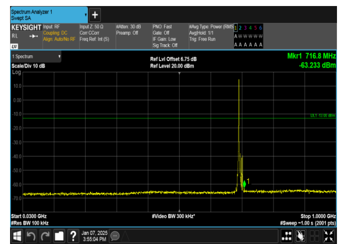
Band12-5MHz-16QAM-23035-1RB#0-30~1000-PASS
