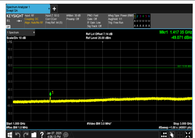
Band12-5MHz-16QAM-23095-25RB#0-1000~3000-PASS
