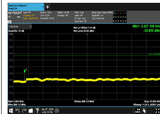
Band12-5MHz-16QAM-23095-1RB#0-3000~10000-PASS
