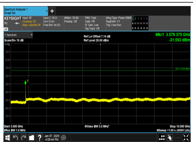
Band12-5MHz-QPSK-23155-1RB#24-3000~10000-PASS
