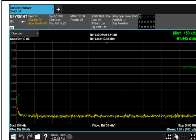
Band12-5MHz-16QAM-23095-1RB#24-0.15~30-PASS
