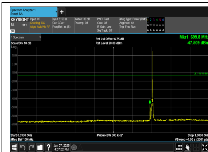
Band12-5MHz-QPSK-23155-1RB#0-30~1000-PASS
