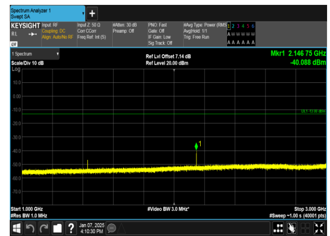
Band12-5MHz-16QAM-23155-1RB#24-1000~3000-PASS
