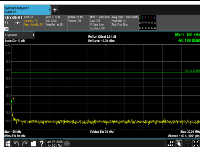
Band12-10MHz-QPSK-23060-1RB#0-0.15~30-PASS
