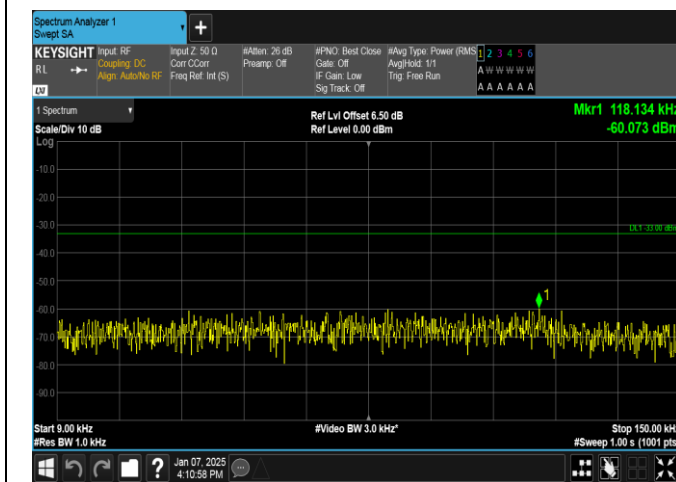
Band12-5MHz-QPSK-23155-25RB#0-0.009~0.15-PASS
