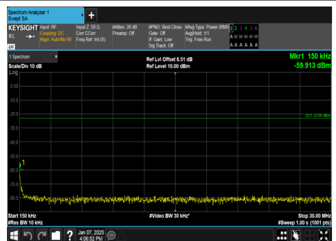
Band12-5MHz-QPSK-23155-1RB#0-0.15~30-PASS
