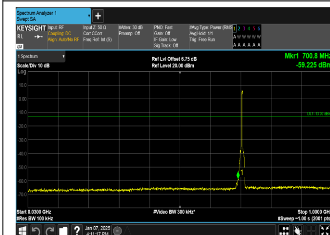
Band12-5MHz-QPSK-23155-25RB#0-30~1000-PASS
