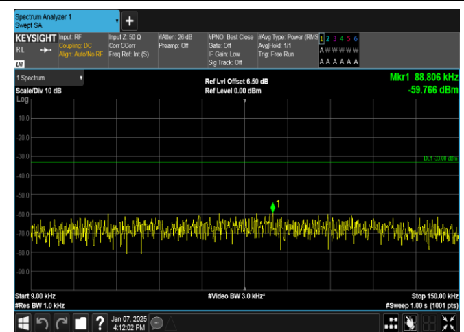
Band12-5MHz-16QAM-23155-25RB#0-0.009~0.15-PASS
