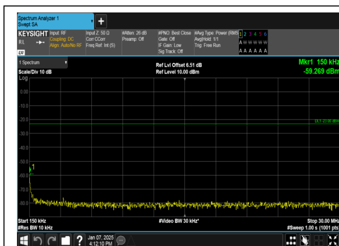
Band12-5MHz-16OAM-23155-25RB#0-0.15~30-PASS
