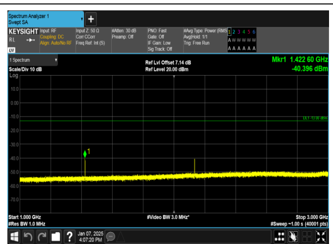
Band12-5MHz-QPSK-23155-1RB#0-1000~3000-PASS
