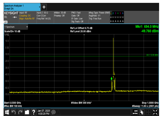
Band12-5MHz-QPSK-23095-1RB#0-30~1000-PASS
