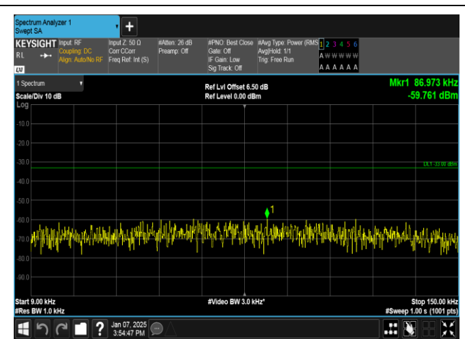
Band12-5MHz-16QAM-23035-1RB#0-0.009~0.15-PASS
