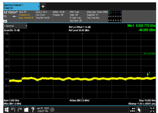
Band12-5MHz-16QAM-23035-25RB#0-3000~10000-PASS
