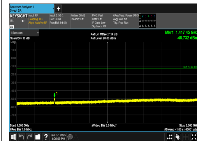
Band12-5MHz-QPSK-23095-25RB#0-1000~3000-PASS
