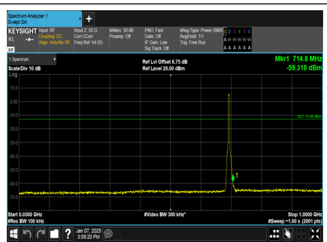
Band12-5MHz-16QAM-23035-25RB#0-30~1000-PASS
