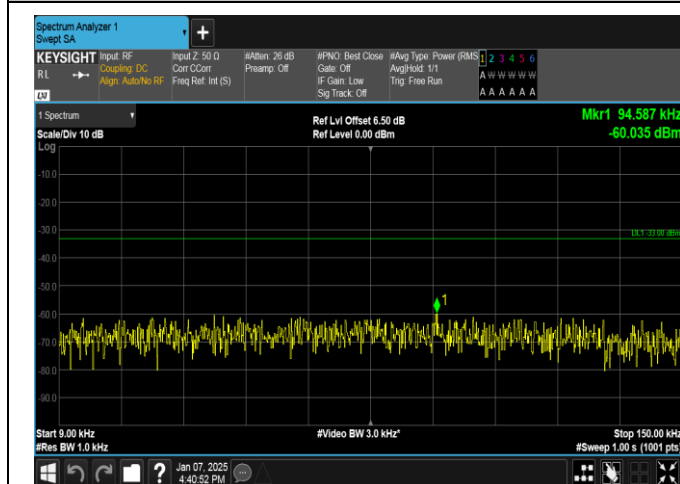
Band12-10MHz-QPSK-23060-1RB#0-0.009~0.15-PASS
