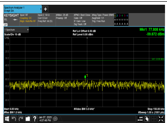
Band12-5MHz-16QAM-23155-1RB#0-0.009~0.15-PASS
