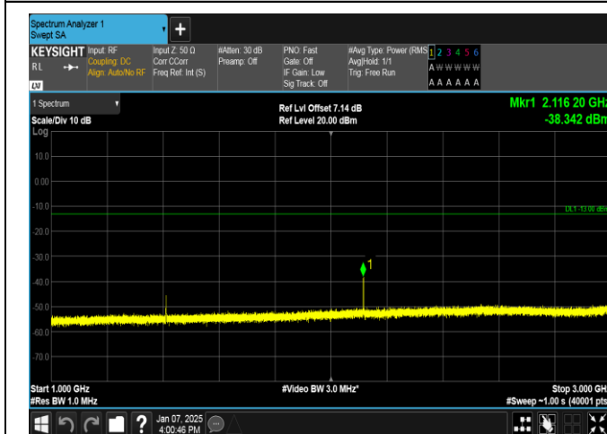
Band12-5MHz-QPSK-23095-1RB#0-1000~3000-PASS
