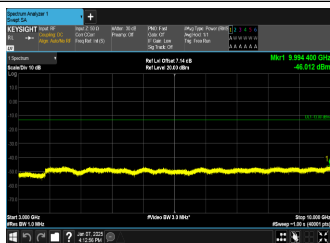
Band12-5MHz-16QAM-23155-25RB#0-3000~10000-PASS
