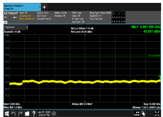
Band12-5MHz-QPSK-23095-25RB#0-3000~10000-PASS
