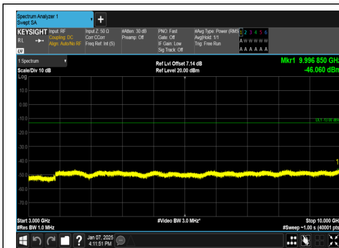
Band12-5MHz-QPSK-23155-25RB#0-3000~10000-PASS
