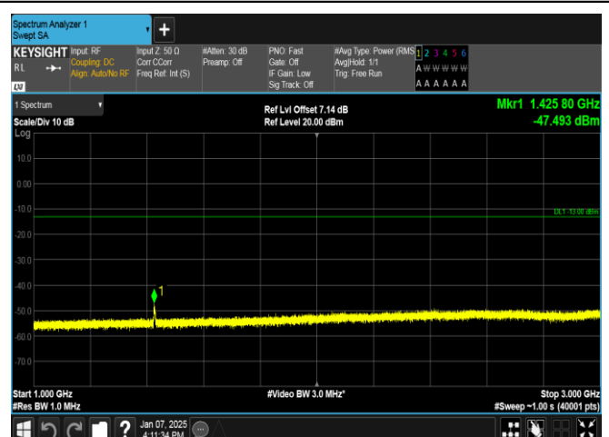
Band12-5MHz-QPSK-23155-25RB#0-1000~3000-PASS
