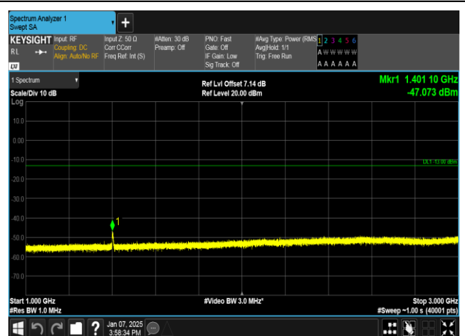
Band12-5MHz-QPSK-23035-25RB#0-1000~3000-PASS
