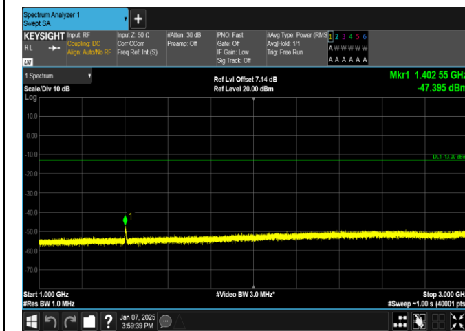
Band12-5MHz-16QAM-23035-25RB#0-1000~3000-PASS
