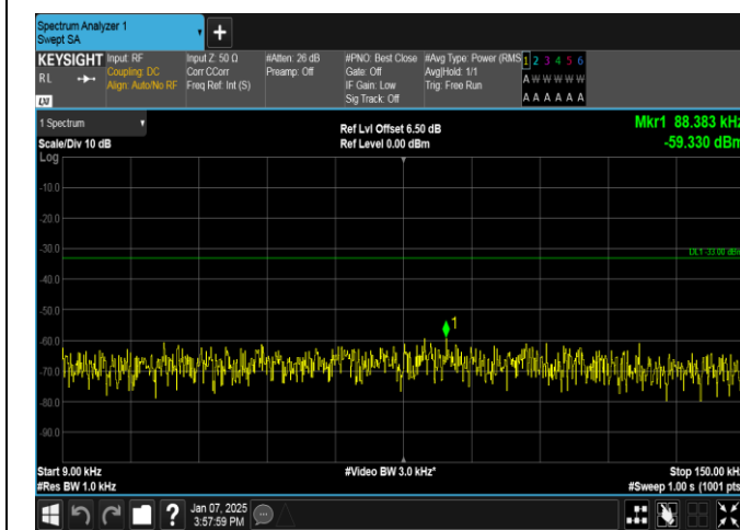
Band12-5MHz-QPSK-23035-25RB#0-0.009~0.15-PASS
