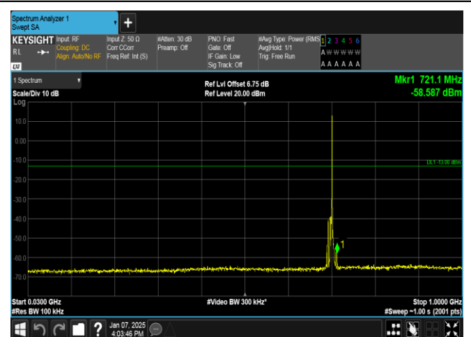
Band12-5MHz-16QAM-23095-1RB#24-30~1000-PASS
