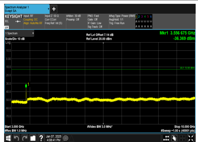
Band12-5MHz-16QAM-23155-1RB#0-3000~10000-PASS
