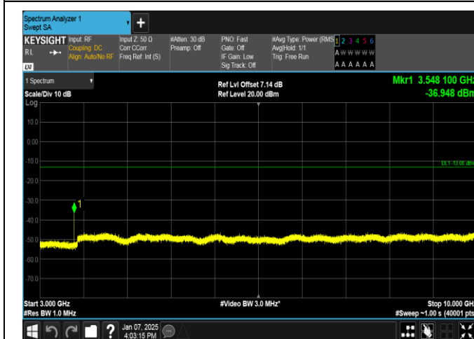
Band12-5MHz-QPSK-23095-1RB#24-3000~10000-PASS
