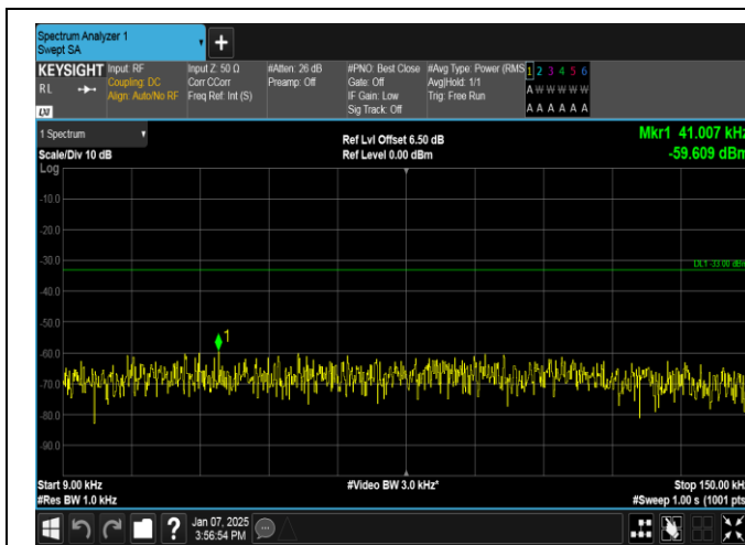
Band12-5MHz-16QAM-23035-1RB#24-0.009~0.15-PASS
