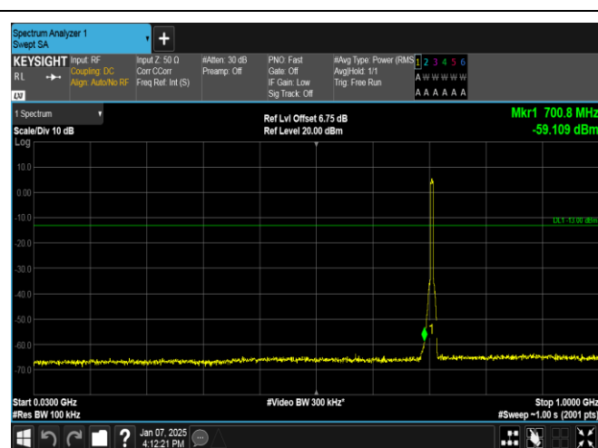
Band12-5MHz-16QAM-23155-25RB#0-30~1000-PASS
