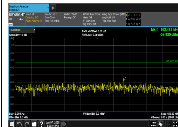
Band12-5MHz-QPSK-23155-1RB#0-0.009~0.15-PASS
