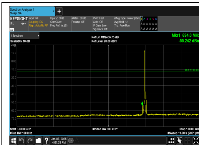
Band12-5MHz-16QAM-23095-1RB#0-30~1000-PASS
