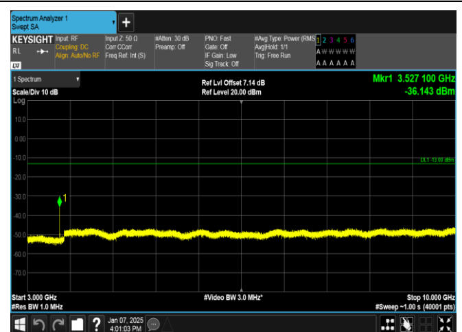
Band12-5MHz-QPSK-23095-1RB#0-3000~10000-PASS
