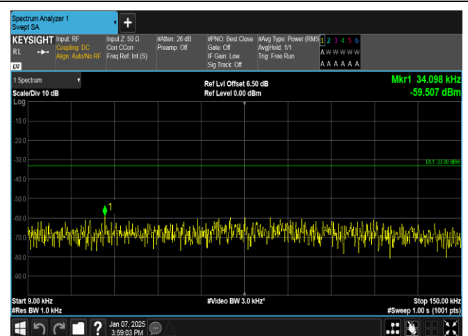
Band12-5MHz-16QAM-23035-25RB#0-0.009~0.15-PASS
