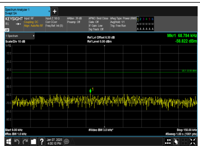
Band12-5MHz-QPSK-23095-1RB#0-0.009~0.15-PASS
