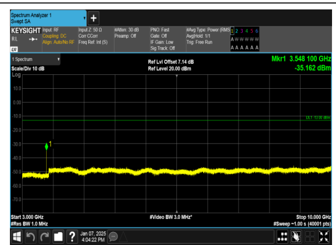
Band12-5MHz-16QAM-23095-1RB#24-3000~10000-PASS
