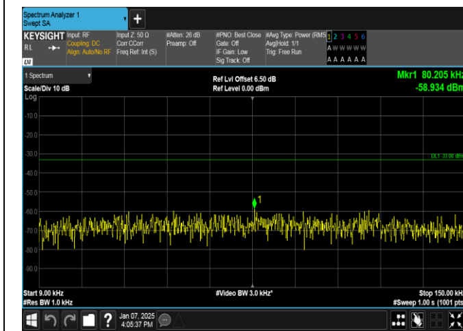
Band12-5MHz-16QAM-23095-25RB#0-0.009~0.15-PASS
