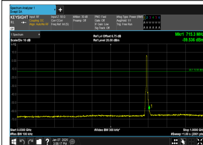
Band12-5MHz-QPSK-23035-25RB#0-30~1000-PASS
