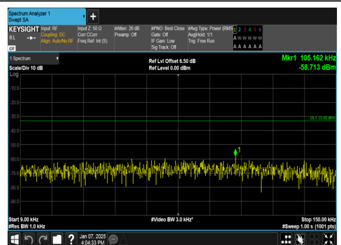
Band12-5MHz-QPSK-23095-25RB#0-0.009~0.15-PASS
