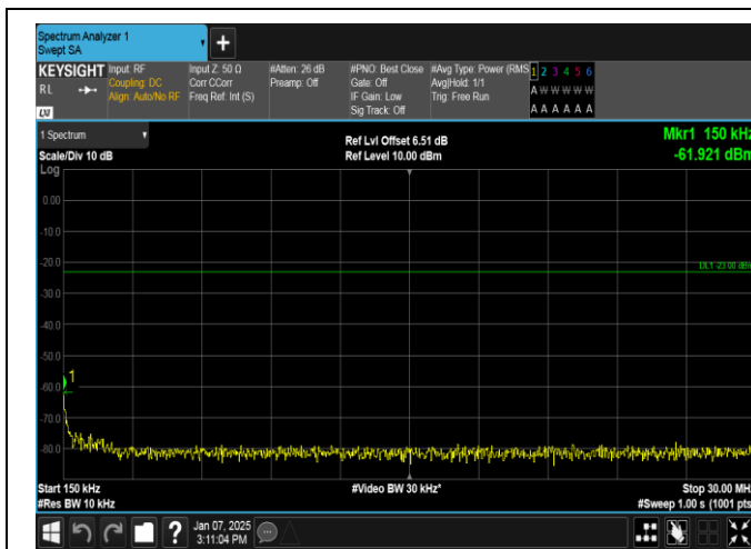
Band12-3MHz-16QAM-23025-15RB#0-0.15~30-PASS
