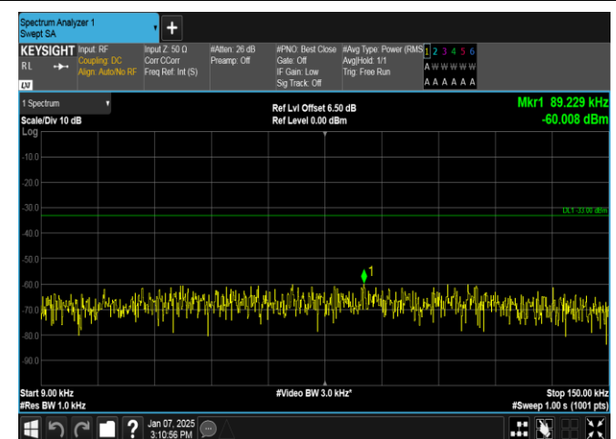
Band12-3MHz-16QAM-23025-15RB#0-0.009~0.15-PASS
