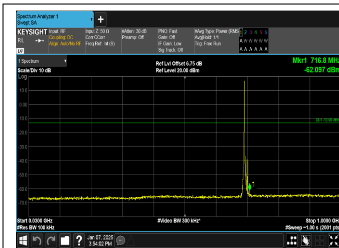
Band12-5MHz-QPSK-23035-1RB#0-30~1000-PASS
