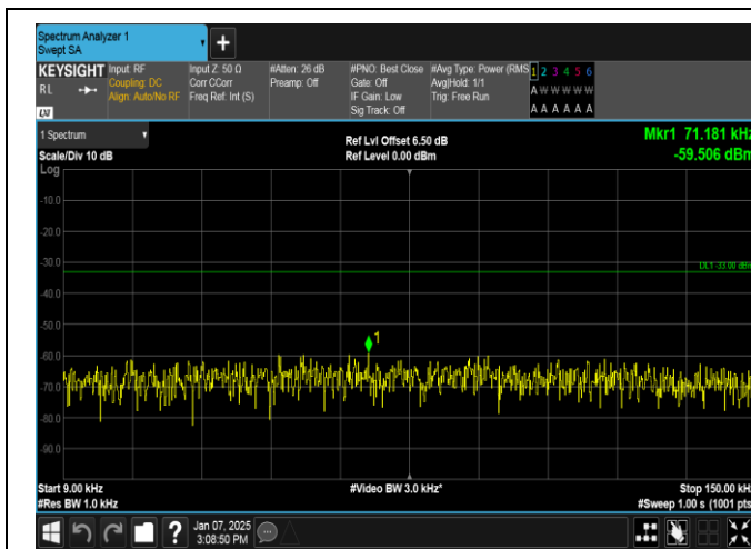
Band12-3MHz-16QAM-23025-1RB#14-0.009~0.15-PASS
