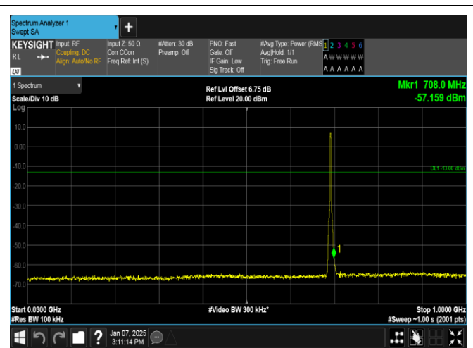
Band12-3MHz-16QAM-23025-15RB#0-30~1000-PASS
