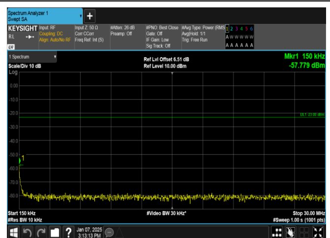
Band12-3MHz-16QAM-23095-1RB#0-0.15~30-PASS
