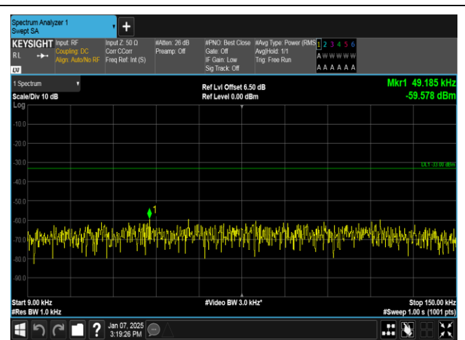
Band12-3MHz-16QAM-23165-1RB#0-0.009~0.15-PASS
