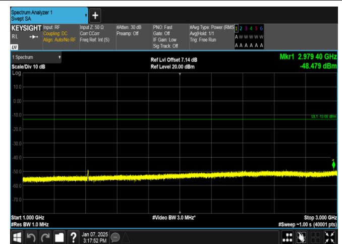
Band12-3MHz-16QAM-23095-15RB#0-1000~3000-PASS
