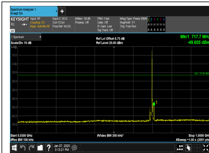
Band12-3MHz-16QAM-23095-1RB#0-30~1000-PASS
