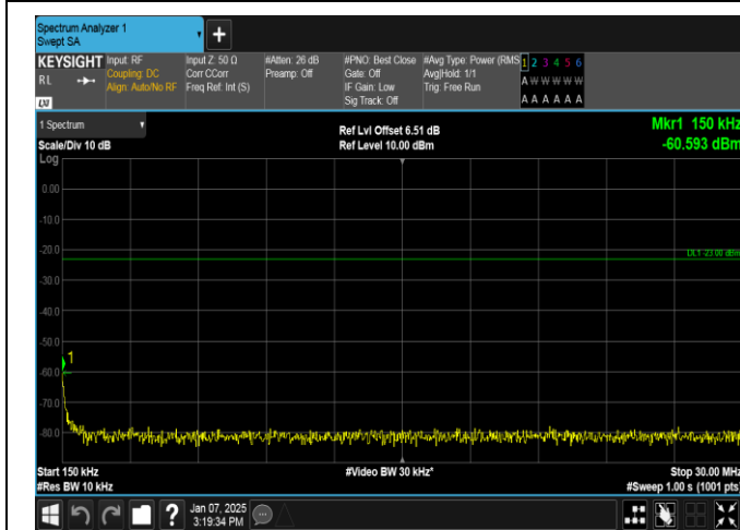
Band12-3MHz-16QAM-23165-1RB#0-0.15~30-PASS
