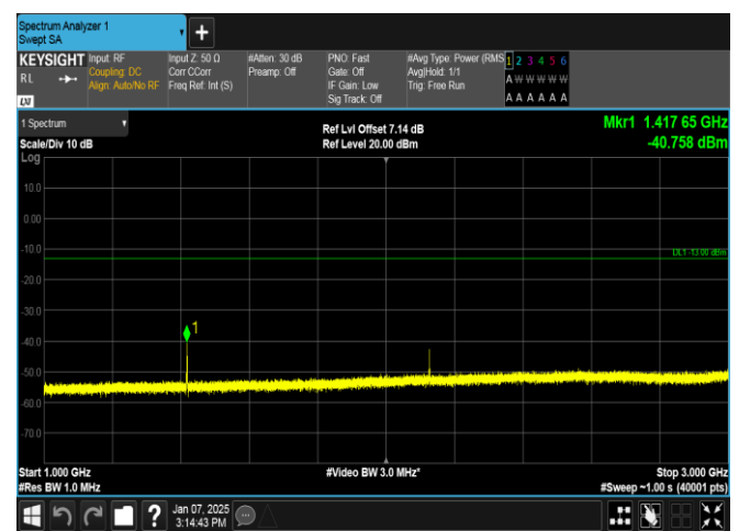
Band12-3MHz-QPSK-23095-1RB#14-1000~3000-PASS
