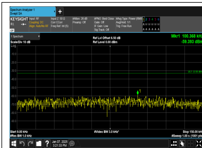
Band12-3MHz-16QAM-23165-1RB#14-0.009~0.15-PASS
