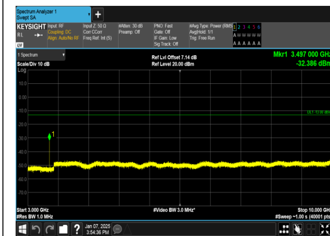
Band12-5MHz-QPSK-23035-1RB#0-3000~10000-PASS
