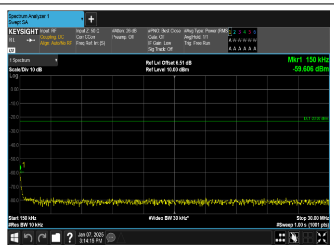
Band12-3MHz-QPSK-23095-1RB#14-0.15~30-PASS
