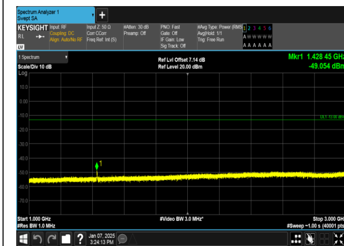
Band12-3MHz-16QAM-23165-15RB#0-1000~3000-PASS
