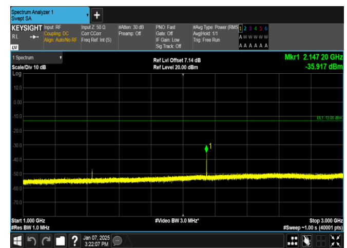
Band12-3MHz-16QAM-23165-1RB#14-1000~3000-PASS
