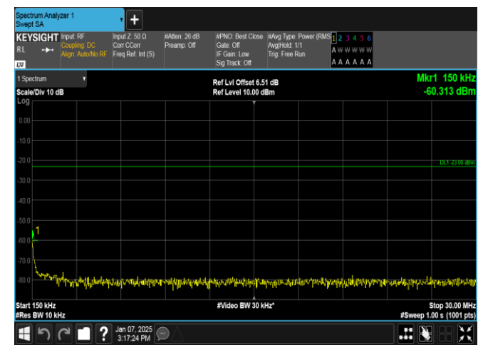
Band12-3MHz-16QAM-23095-15RB#0-0.15~30-PASS
