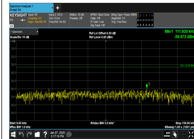
Band12-3MHz-16QAM-23095-15RB#0-0.009~0.15-PASS
