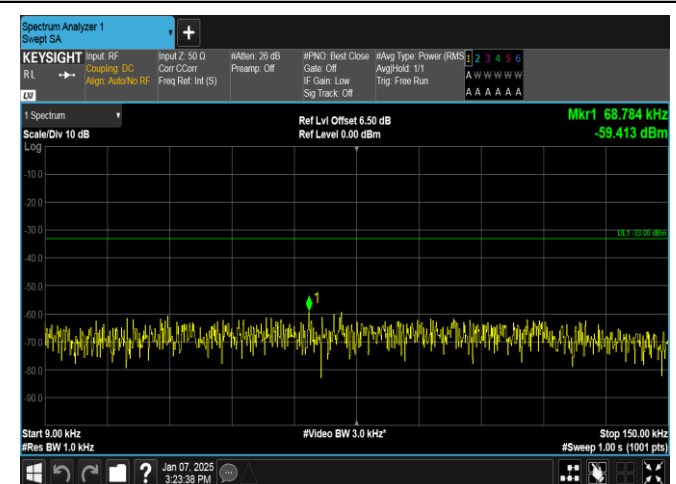
Band12-3MHz-16QAM-23165-15RB#0-0.009~0.15-PASS
