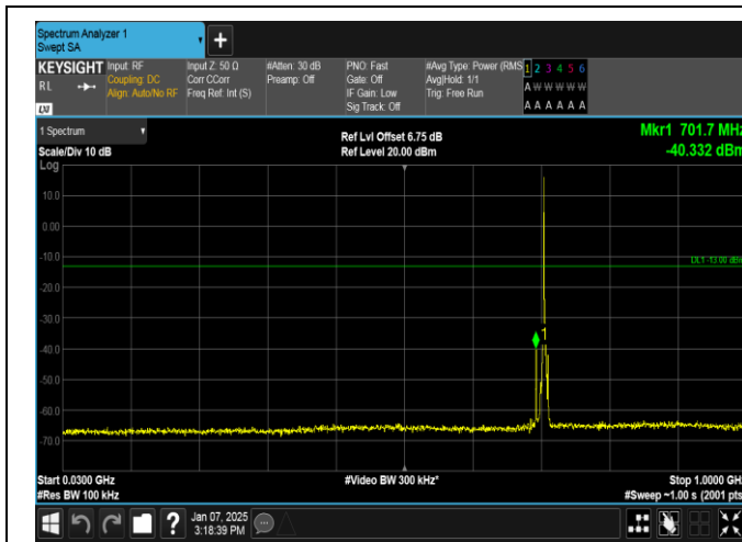
Band12-3MHz-QPSK-23165-1RB#0-30~1000-PASS
