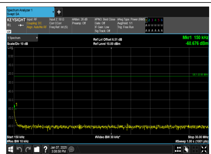
Band12-3MHz-16QAM-23025-1RB#14-0.15~30-PASS
