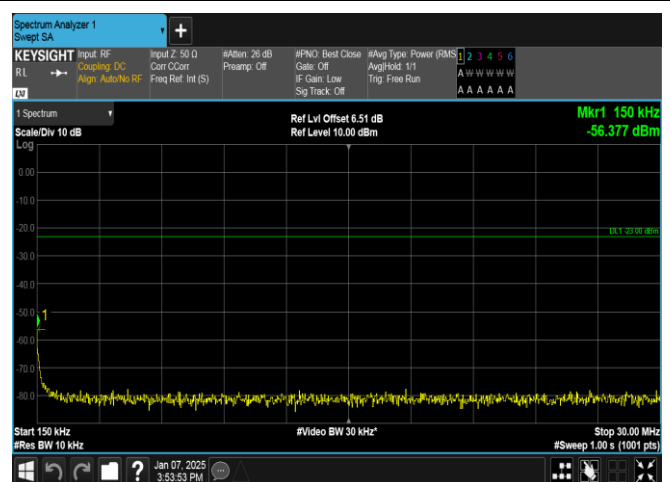
Band12-5MHz-QPSK-23035-1RB#0-0.15~30-PASS
