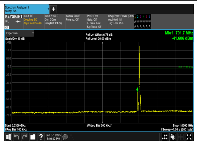
Band12-3MHz-16QAM-23165-1RB#0-30~1000-PASS
