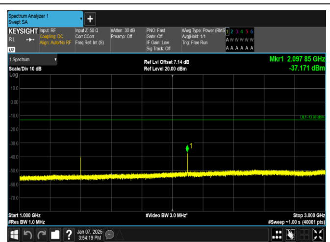
Band12-5MHz-QPSK-23035-1RB#0-1000~3000-PASS
