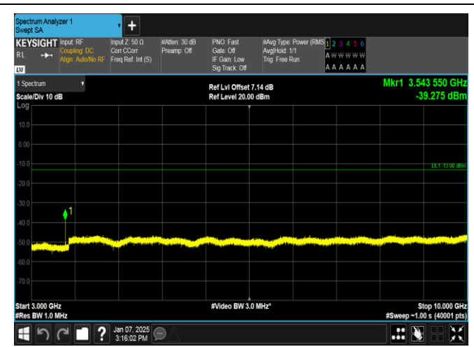
Band12-3MHz-16QAM-23095-1RB#14-3000~10000-PASS
