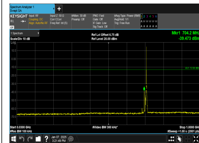
Band12-3MHz-16QAM-23165-1RB#14-30~1000-PASS
