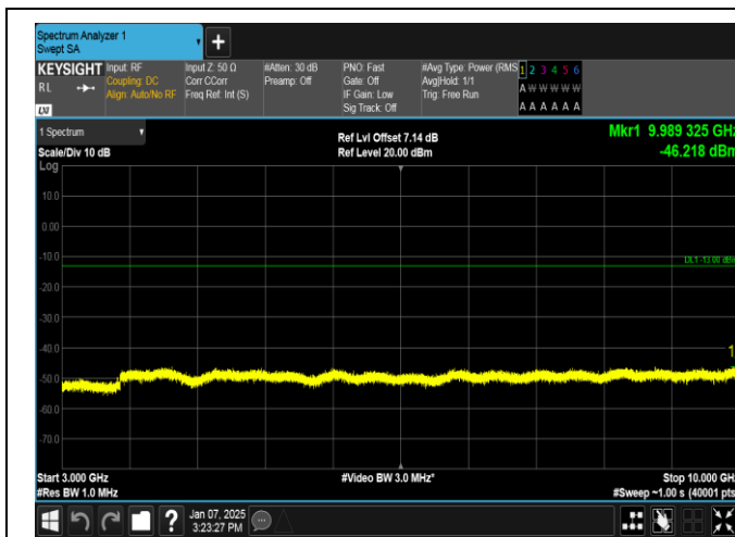
Band12-3MHz-QPSK-23165-15RB#0-3000~10000-PASS
