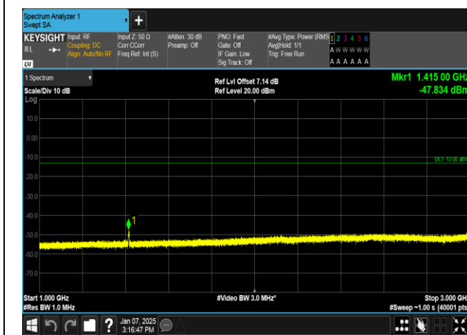
Band12-3MHz-QPSK-23095-15RB#0-1000~3000-PASS
