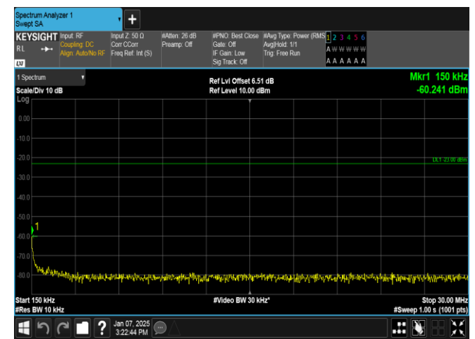
Band12-3MHz-QPSK-23165-15RB#0-0.15~30-PASS
