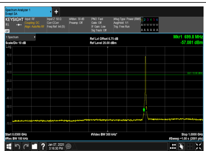
Band12-3MHz-QPSK-23095-15RB#0-30~1000-PASS
