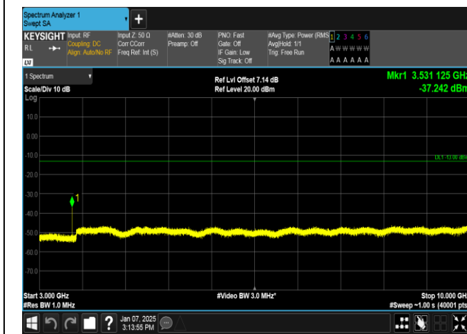
Band12-3MHz-16QAM-23095-1RB#0-3000~10000-PASS
