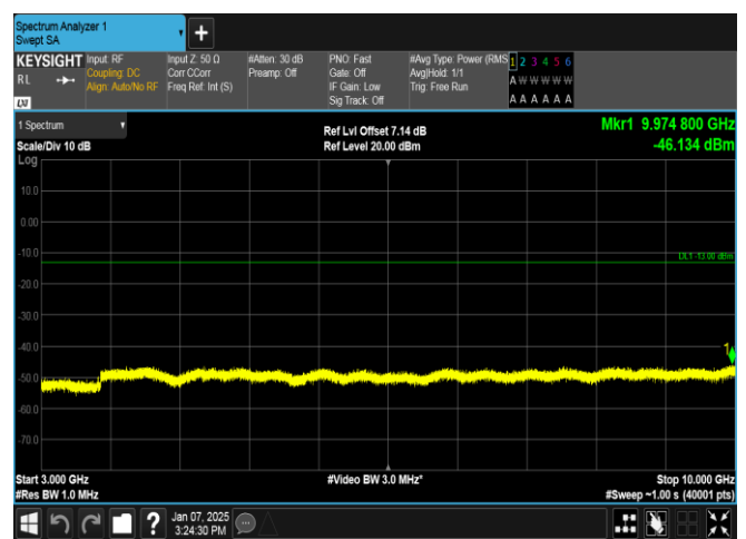
Band12-3MHz-16QAM-23165-15RB#0-3000~10000-PASS
