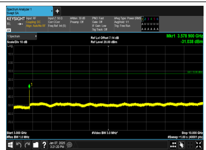
Band12-3MHz-QPSK-23165-1RB#14-3000~10000-PASS
