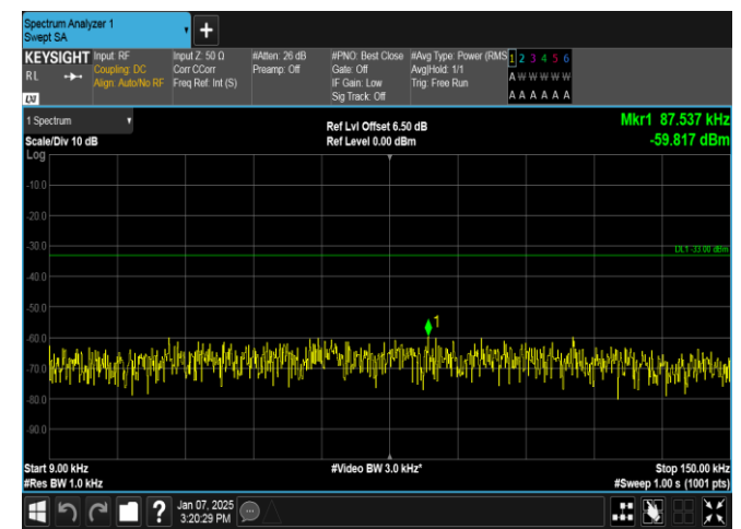
Band12-3MHz-QPSK-23165-1RB#14-0.009~0.15-PASS
