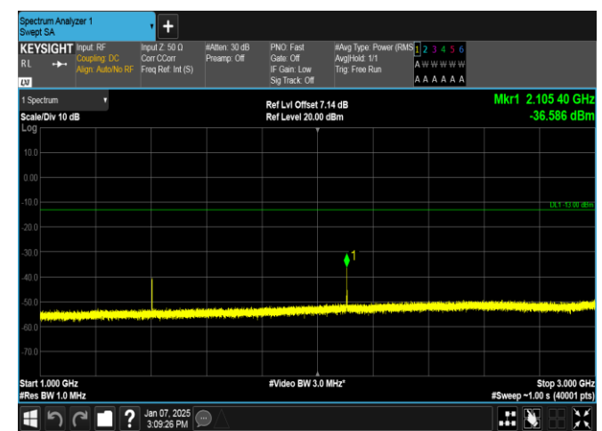
Band12-3MHz-16QAM-23025-1RB#14-1000~3000-PASS
