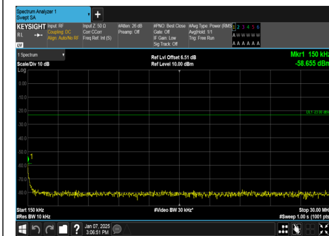
Band12-3MHz-16QAM-23025-1RB#0-0.15~30-PASS
