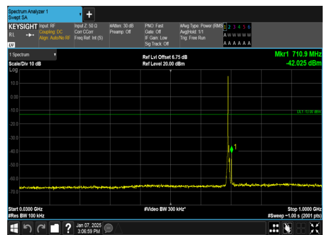
Band12-3MHz-16QAM-23025-1RB#0-30~1000-PASS
