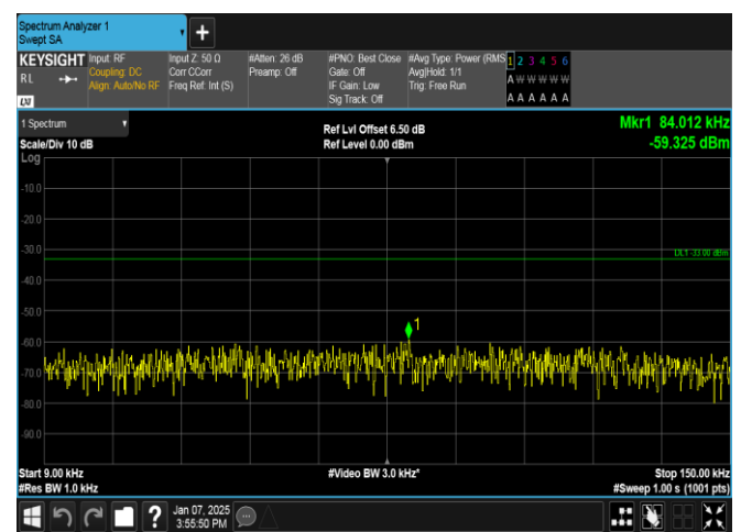
Band12-5MHz-QPSK-23035-1RB#24-0.009~0.15-PASS
