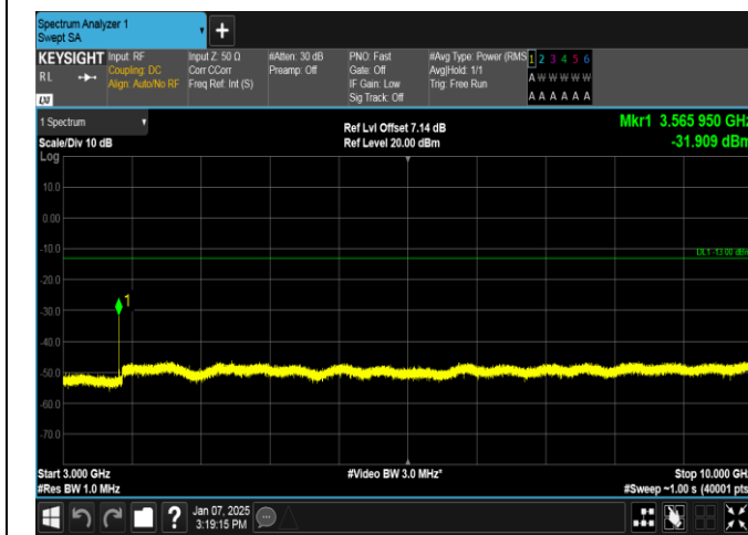
Band12-3MHz-QPSK-23165-1RB#0-3000~10000-PASS
