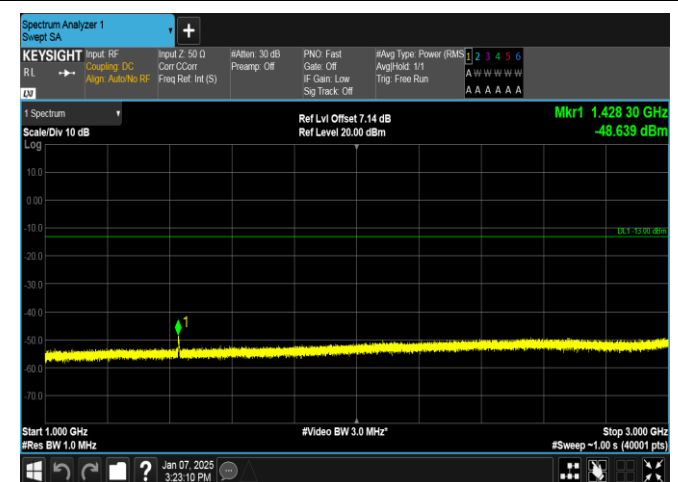
Band12-3MHz-QPSK-23165-15RB#0-1000~3000-PASS
