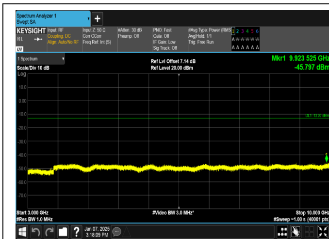
Band12-3MHz-16QAM-23095-15RB#0-3000~10000-PASS
