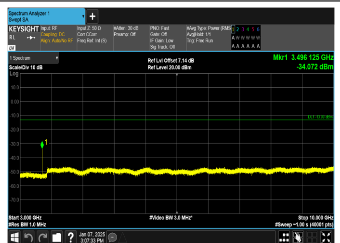
Band12-3MHz-16QAM-23025-1RB#0-3000~10000-PASS
