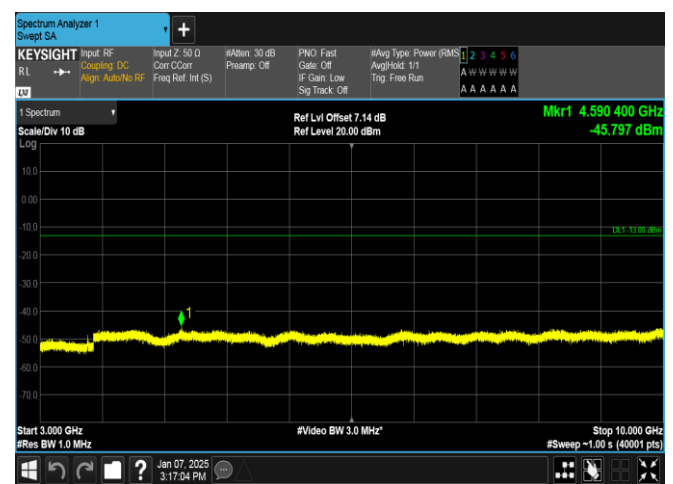
Band12-3MHz-QPSK-23095-15RB#0-3000~10000-PASS
