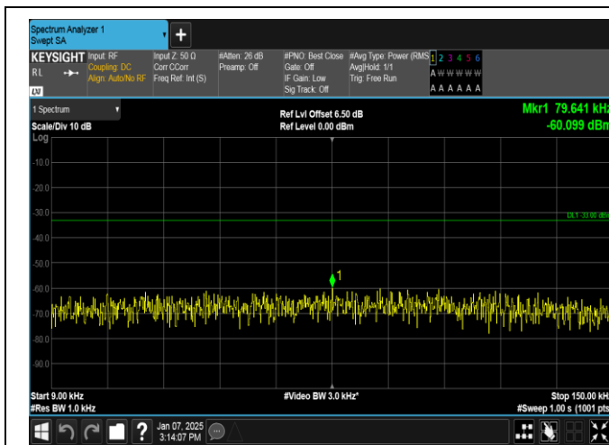
Band12-3MHz-QPSK-23095-1RB#14-0.009~0.15-PASS
