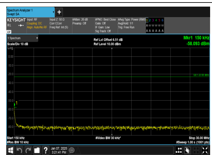
Band12-3MHz-16QAM-23165-1RB#14-0.15~30-PASS
