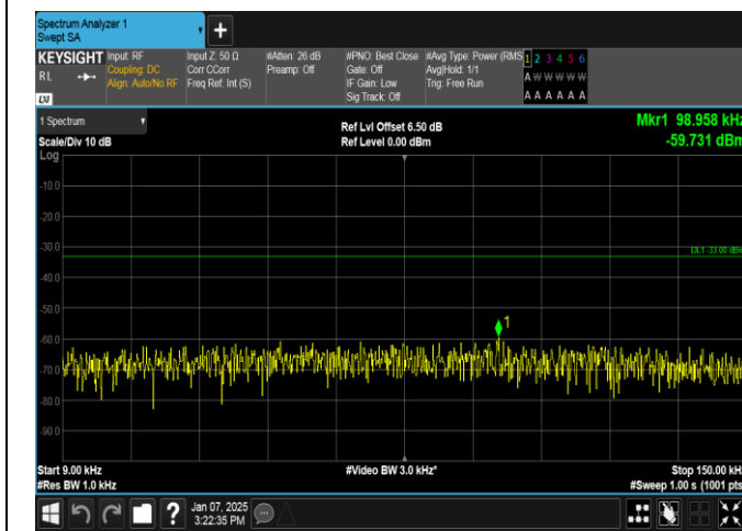
Band12-3MHz-QPSK-23165-15RB#0-0.009~0.15-PASS
