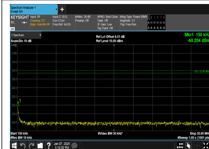
Band12-3MHz-16QAM-23095-1RB#14-0.15~30-PASS
