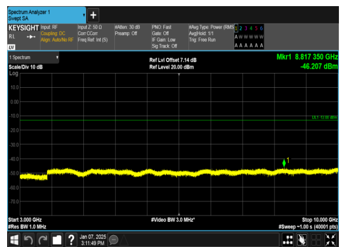
Band12-3MHz-16QAM-23025-15RB#0-3000~10000-PASS
