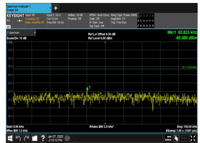
Band12-3MHz-16QAM-23095-1RB#14-0.009~0.15-PASS
