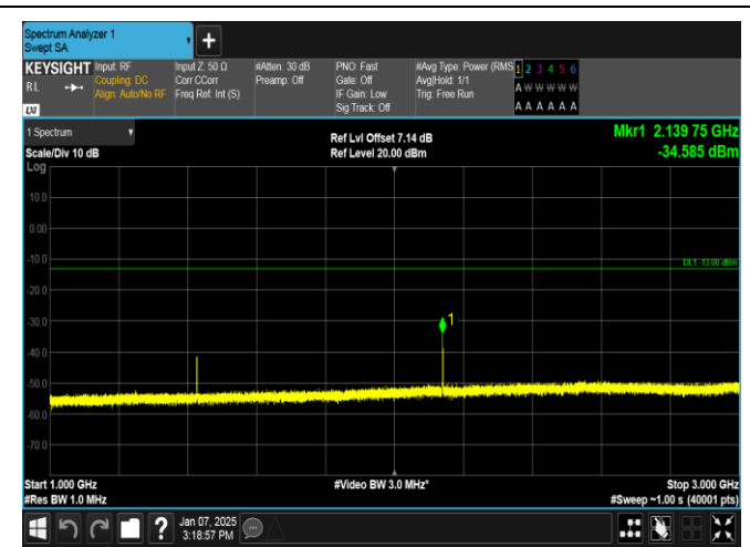
Band12-3MHz-QPSK-23165-1RB#0-1000~3000-PASS
