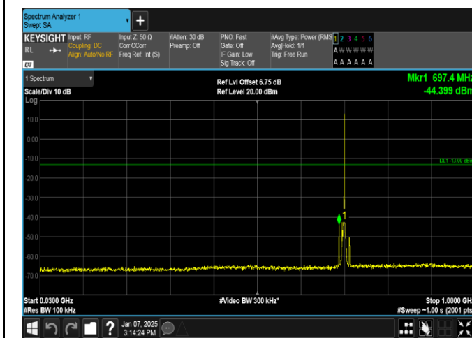
Band12-3MHz-QPSK-23095-1RB#14-30~1000-PASS
