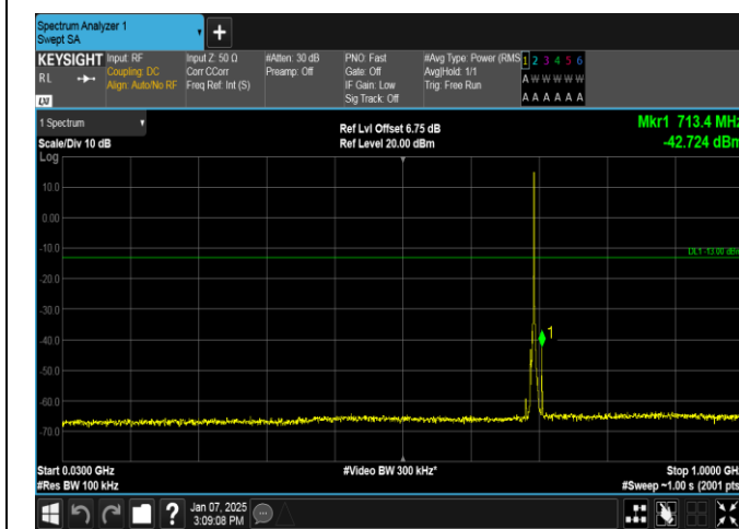
Band12-3MHz-16QAM-23025-1RB#14-30~1000-PASS
