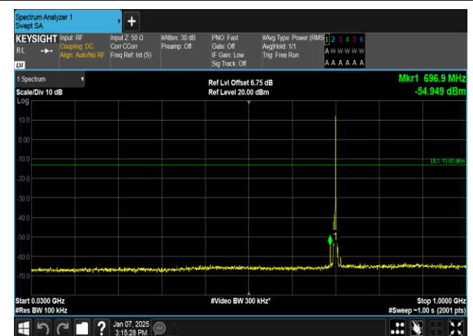
Band12-3MHz-16QAM-23095-1RB#14-30~1000-PASS
