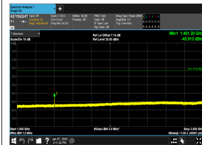
Band12-3MHz-16QAM-23025-15RB#0-1000~3000-PASS
