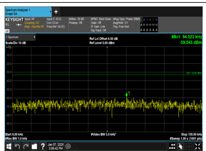
Band12-3MHz-16QAM-23025-1RB#0-0.009~0.15-PASS
