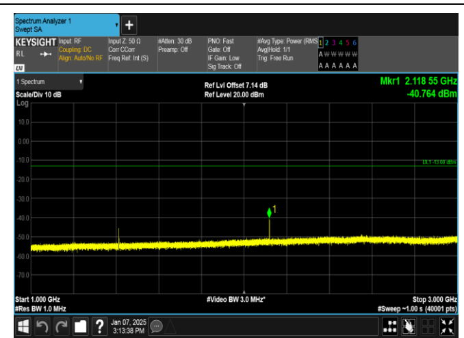
Band12-3MHz-16QAM-23095-1RB#0-1000~3000-PASS
