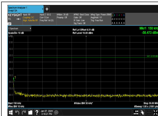
Band12-3MHz-QPSK-23095-15RB#0-0.15~30-PASS
