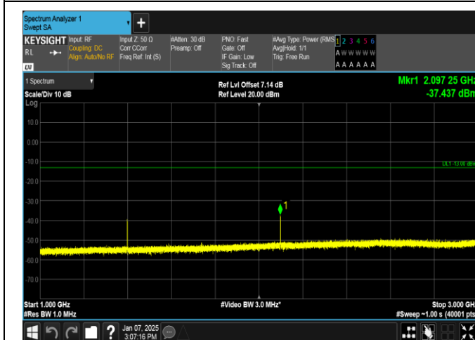
Band12-3MHz-16QAM-23025-1RB#0-1000~3000-PASS
