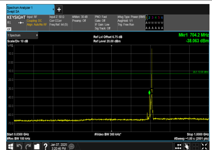
Band12-3MHz-QPSK-23165-1RB#14-30~1000-PASS
