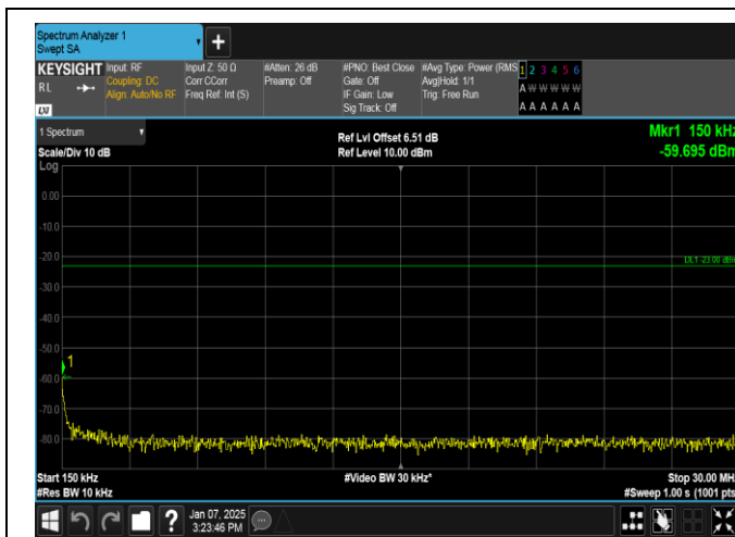
Band12-3MHz-16QAM-23165-15RB#0-0.15~30-PASS
