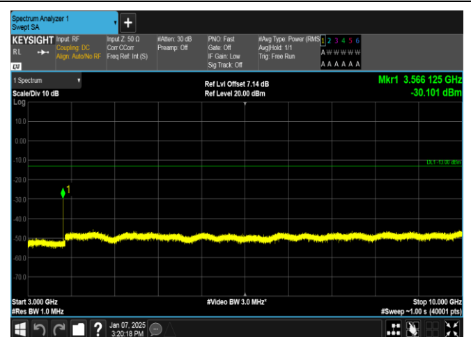
Band12-3MHz-16QAM-23165-1RB#0-3000~10000-PASS
